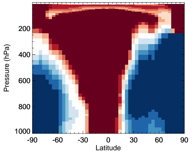
v11-02d / v11-02a LIMO - Zonal mean % diff for Apr
