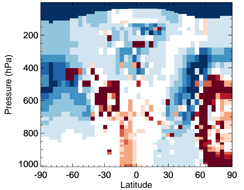
v11-02d / v11-02a NIT - Zonal mean % diff for Apr
