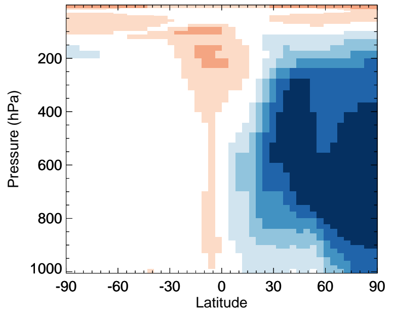
v11-02d / v11-02a SO2 - Zonal mean % diff for Apr
