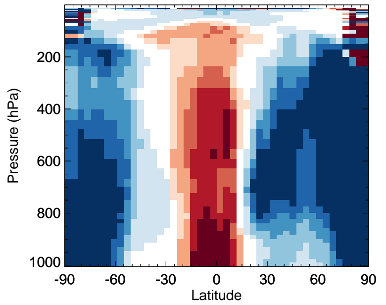
v11-02d / v11-02c LIMO - Zonal mean % diff for Apr
