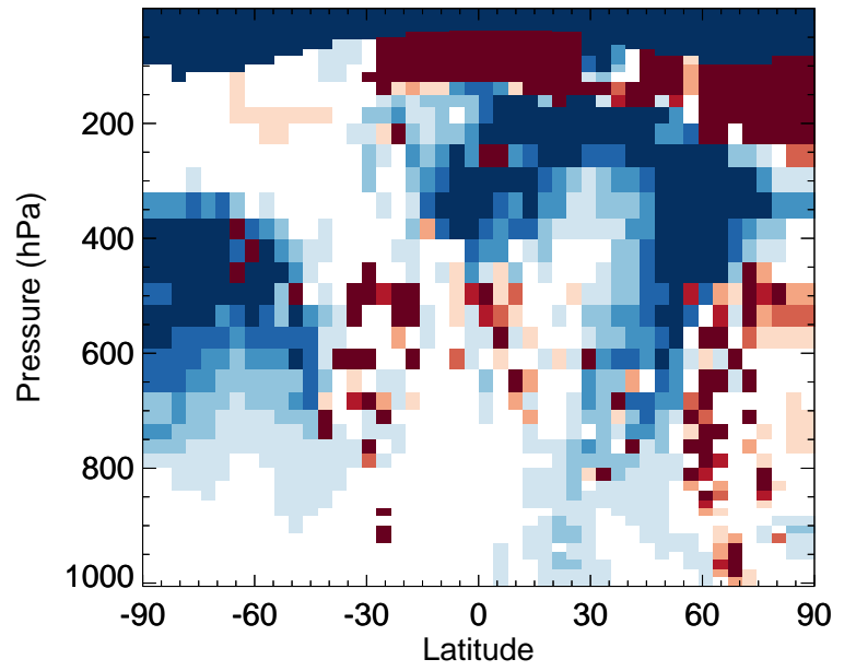
v11-02d / v11-02c NIT - Zonal mean % diff for Apr
