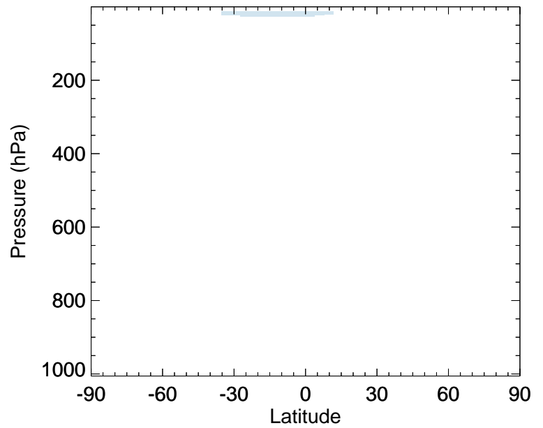
v11-02d / v11-02a CCI4 - Zonal mean % diff for Apr
