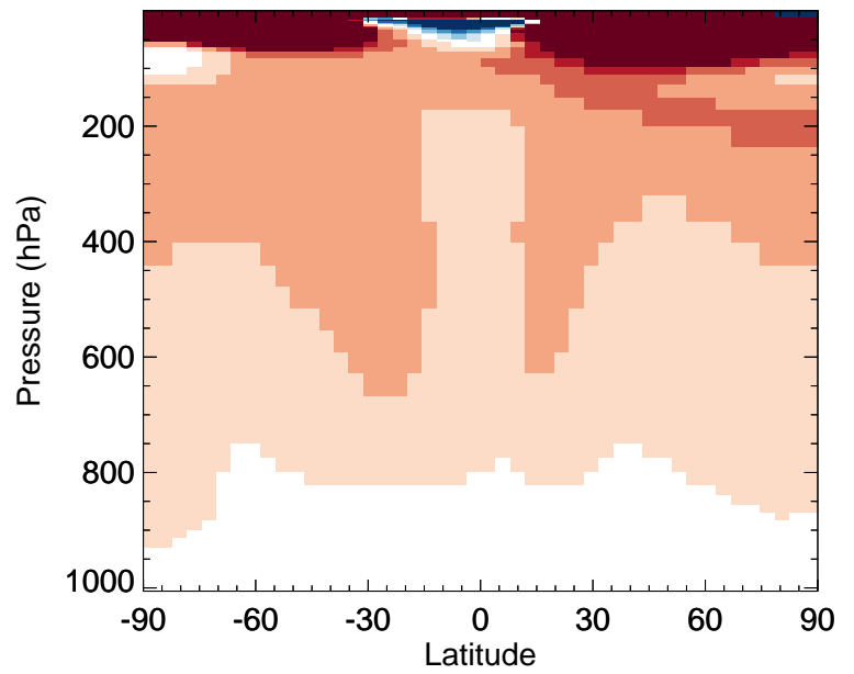
v11-02d / v11-02c CCI4 - Zonal mean % diff for Apr
