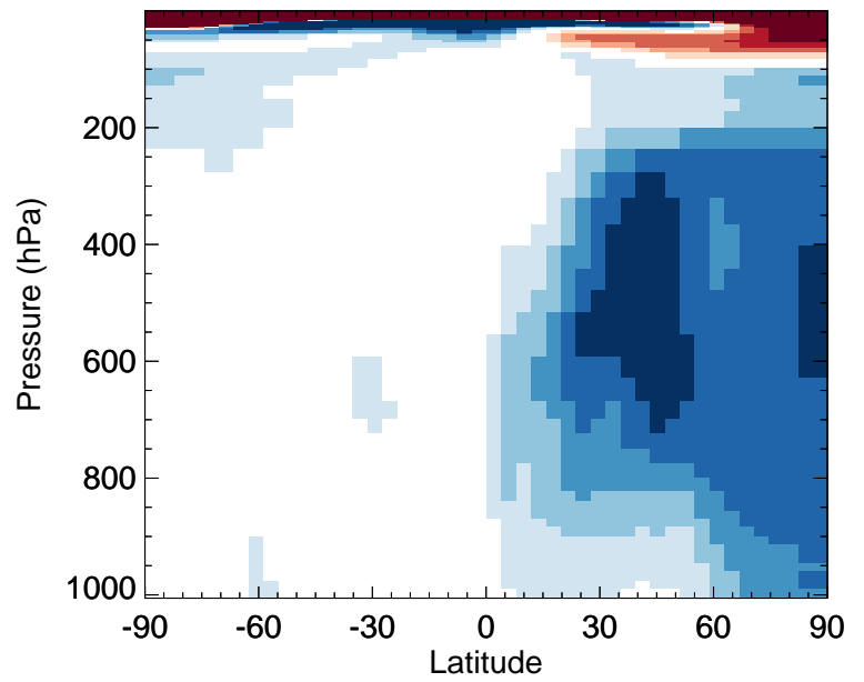
v11-02d / v11-02c SO2 - Zonal mean % diff for Apr
