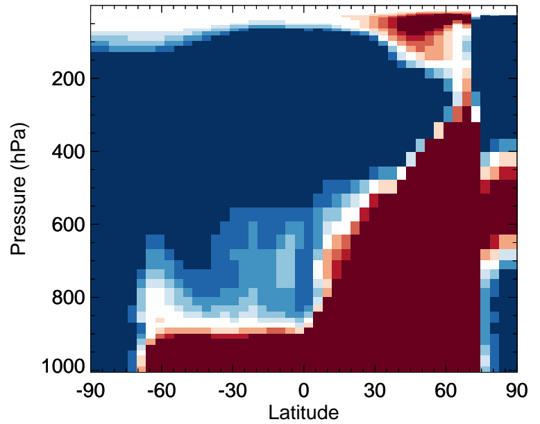
v11-02d / v11-02a ClOO - Zonal mean % diff for Jan
