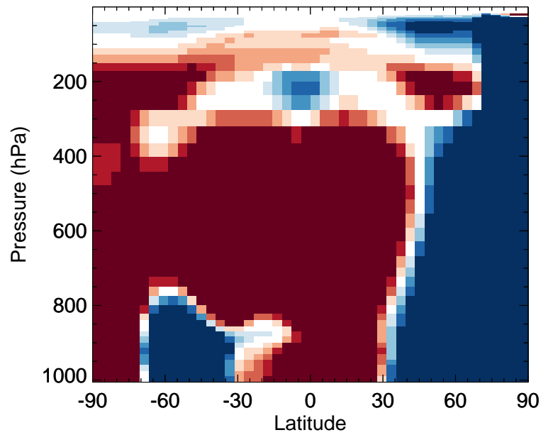
v11-02d / v11-02a BrO - Zonal mean % diff for Jan
