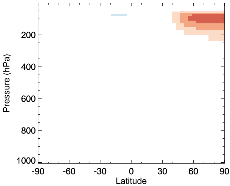
v11-02d - v11-02a MPN - Zonal mean abs diff for Jan
