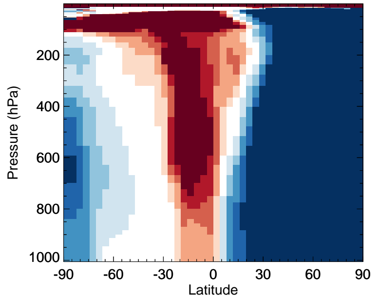
v11-02d / v11-02a DMS - Zonal mean % diff for Jan
