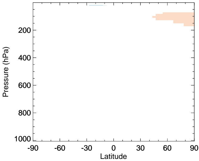
v11-02d - v11-02c MPN - Zonal mean abs diff for Jan
