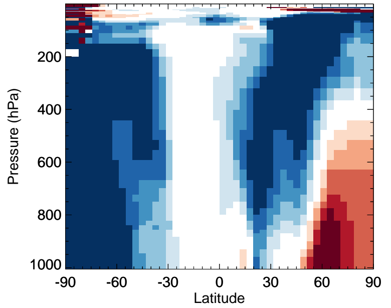
v11-02d / v11-02c RIPD - Zonal mean % diff for Jan
