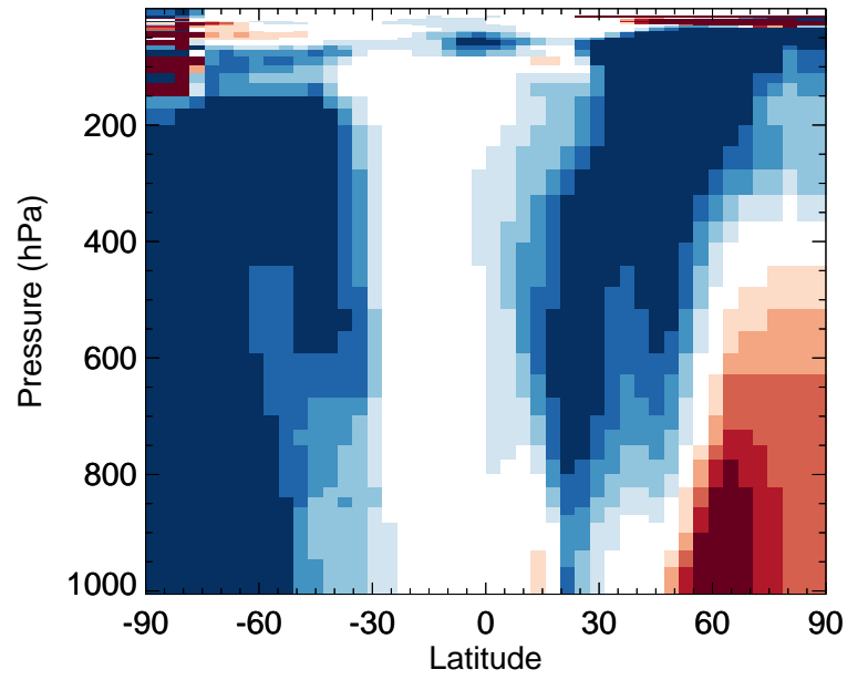
v11-02d / v11-02c RIPB - Zonal mean % diff for Jan
