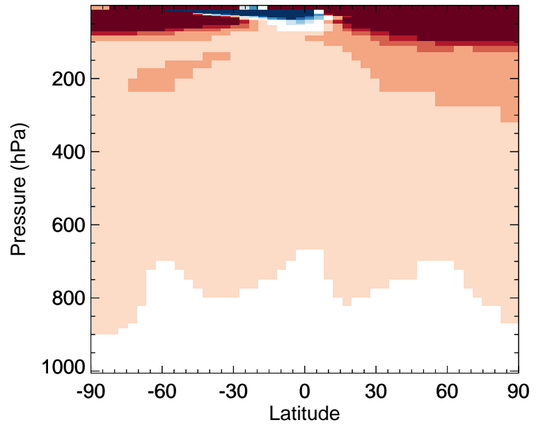
v11-02d / v11-02c CCI4 - Zonal mean % diff for Jan
