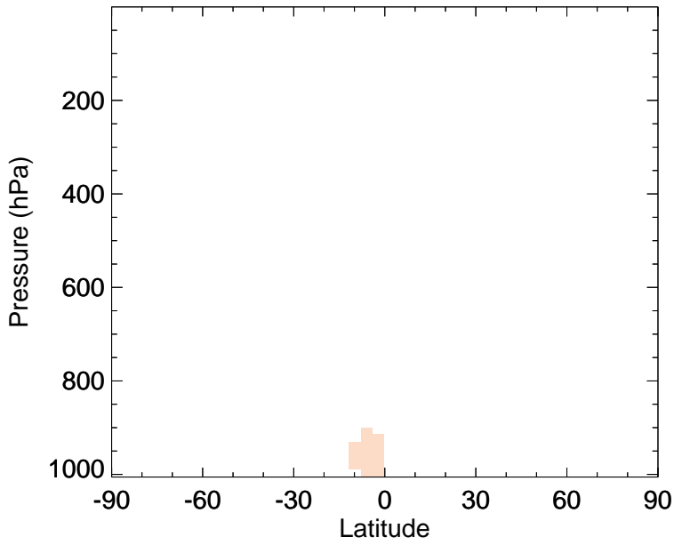
v11-02d - v11-02a RIPB - Zonal mean abs diff for Jan
