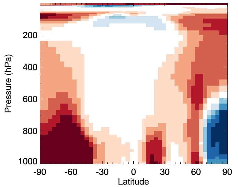
v11-02d / v11-02c MPN - Zonal mean % diff for Jan
