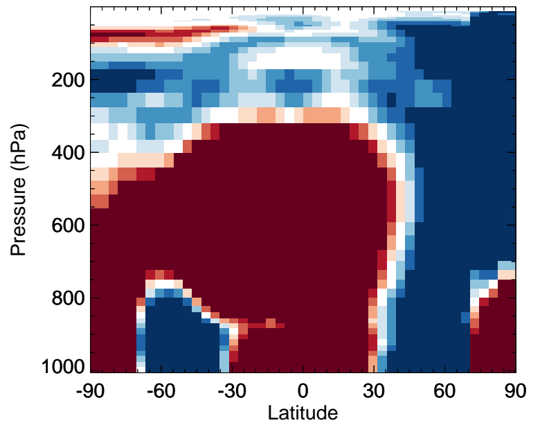
v11-02d / v11-02c BrO - Zonal mean % diff for Jan
