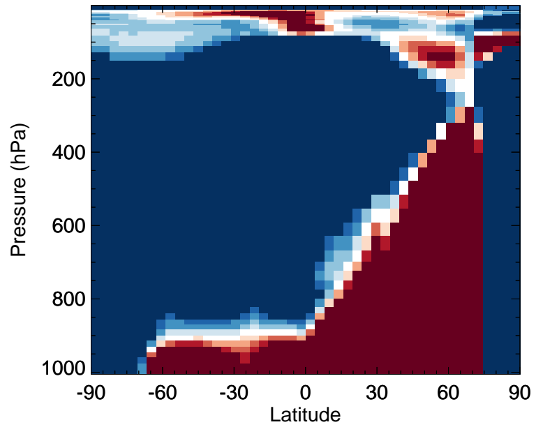
v11-02d / v11-02c ClOO - Zonal mean % diff for Jan
