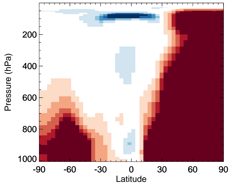
v11-02d / v11-02a MPN - Zonal mean % diff for Jan
