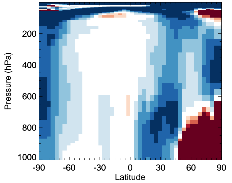
v11-02d / v11-02c DMS - Zonal mean % diff for Jan
