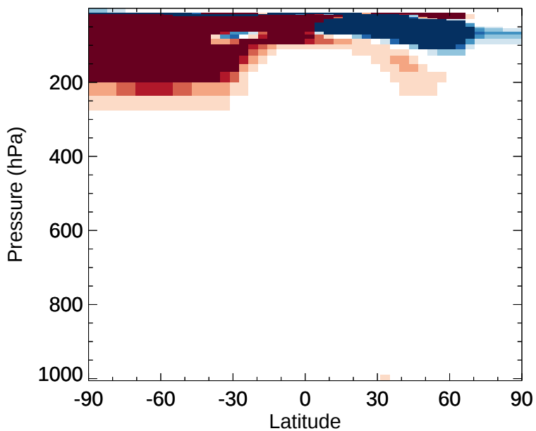
v11-02d - v11-02c N2O5 - Zonal mean abs diff for Jul
