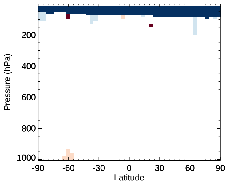
v11-02d / v11-02a SO 4 s - Zonal mean % diff for Jul
