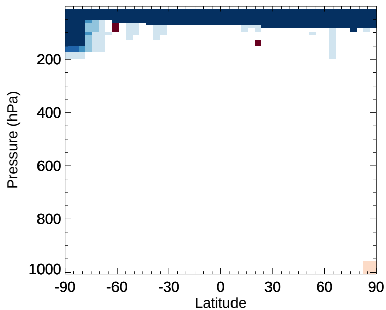
v11-02d / v11-02c SO 4 s - Zonal mean % diff for Jul
