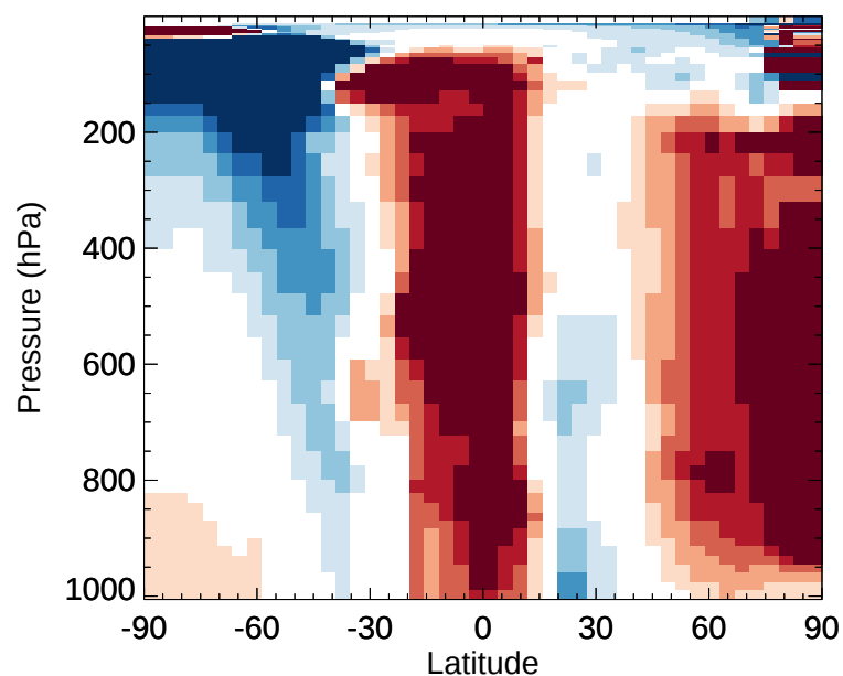
v11-02d / v11-02a ISOP - Zonal mean % diff for Jul
