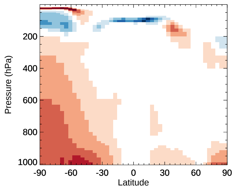
v11-02d / v11-02a CH 2 O - Zonal mean % diff for Jul
