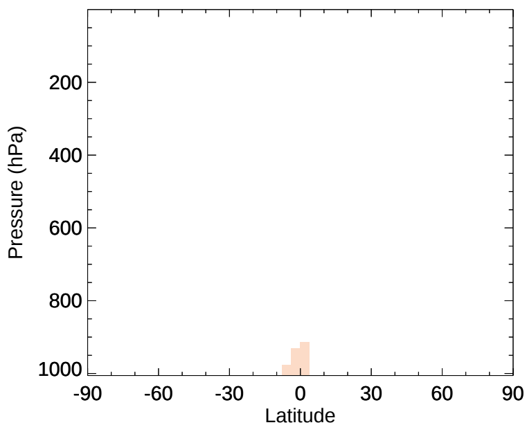
v11-02d - v11-02c ISOP - Zonal mean abs diff for Jul
