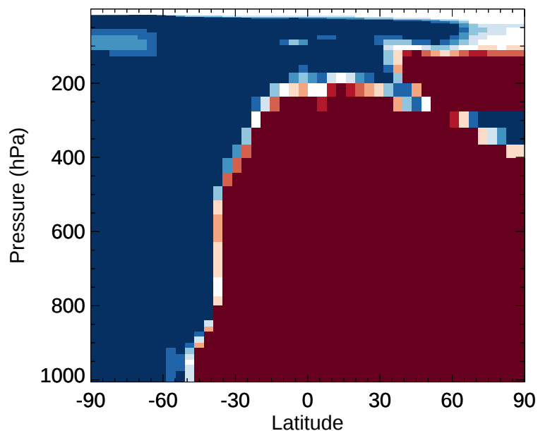
v11-02d / v11-02a OCIO - Zonal mean % diff for Jul
