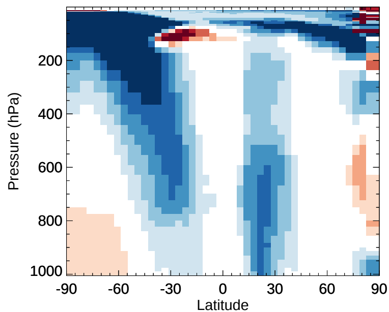
v11-02d / v11-02c ISOP - Zonal mean % diff for Jul
