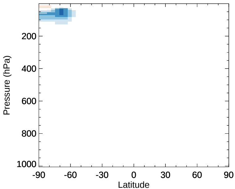
v11-02d - v11-02c OCIO - Zonal mean abs diff for Jul
