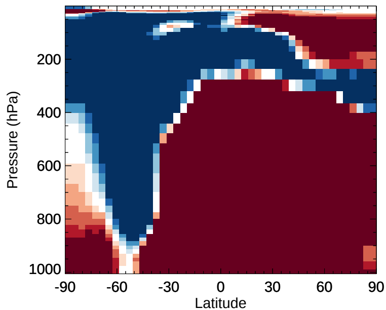
v11-02d / v11-02c OCIO - Zonal mean % diff for Jul
