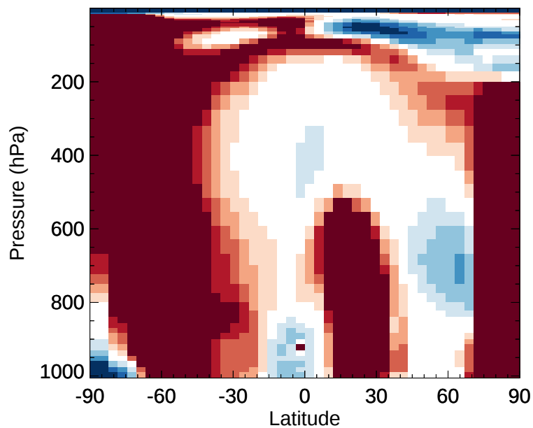
v11-02d / v11-02c N2O5 - Zonal mean % diff for Jul
