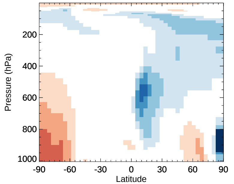
v11-02d / v11-02a SO 2 - Zonal mean % diff for Jul
