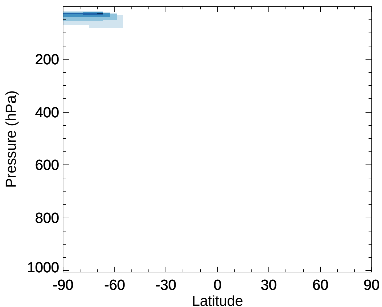
v11-02d - v11-02a OCIO - Zonal mean abs diff for Jul
