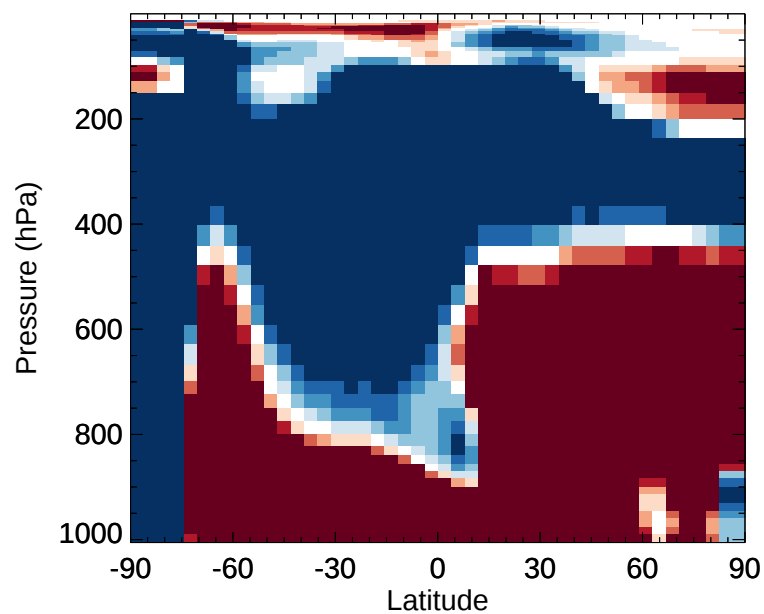
v11-02d / v11-02c Cl - Zonal mean % diff for Jul
