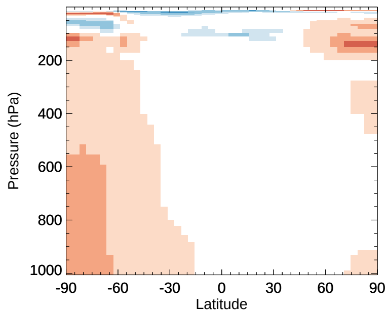
v11-02d / v11-02c CH 2 O - Zonal mean % diff for Jul
