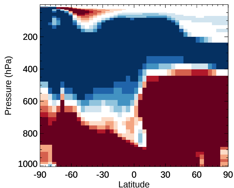
v11-02d / v11-02a Cl - Zonal mean % diff for Jul
