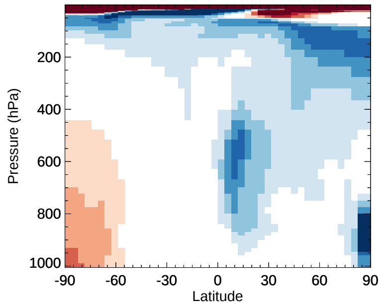
v11-02d / v11-02c SO 2 - Zonal mean % diff for Jul
