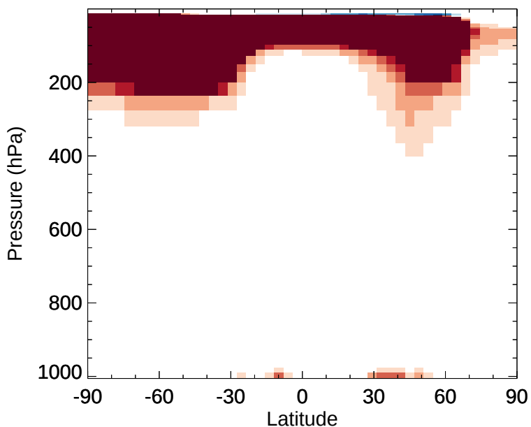
v11-02d - v11-02a N2O5 - Zonal mean abs diff for Jul
