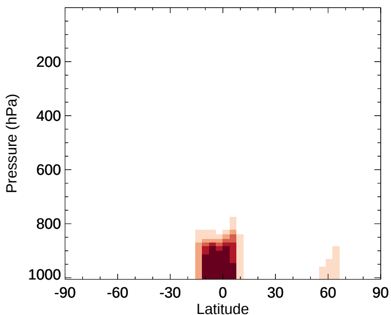
v11-02d - v11-02a ISOP - Zonal mean abs diff for Jul
