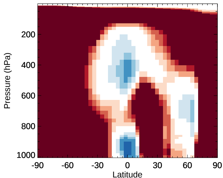
v11-02d / v11-02a N2O5 - Zonal mean % diff for Jul
