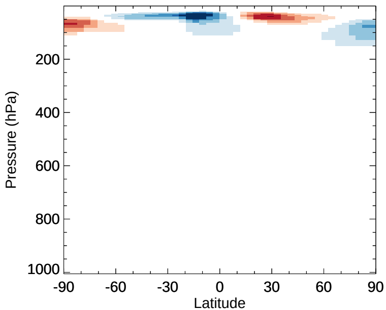
v11-02d - v11-02c OCS - Zonal mean abs diff for Oct
