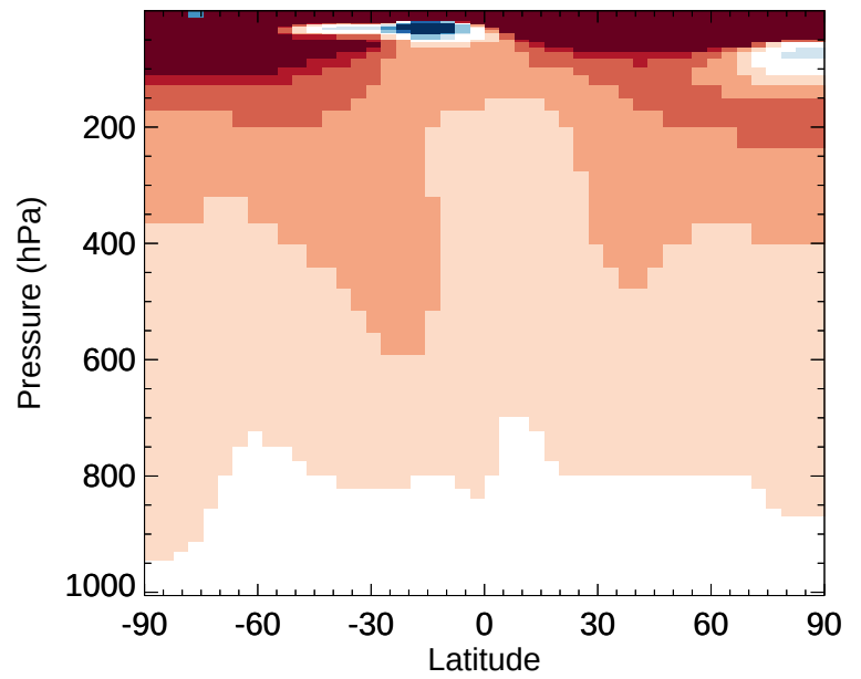
v11-02d / v11-02c CCl4 - Zonal mean % diff for Oct
