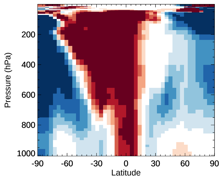
v11-02d / v11-02a MVK - Zonal mean % diff for Oct
