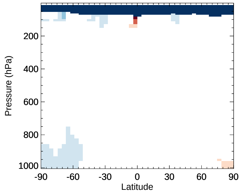
v11-02d / v11-02a SO4s - Zonal mean % diff for Oct
