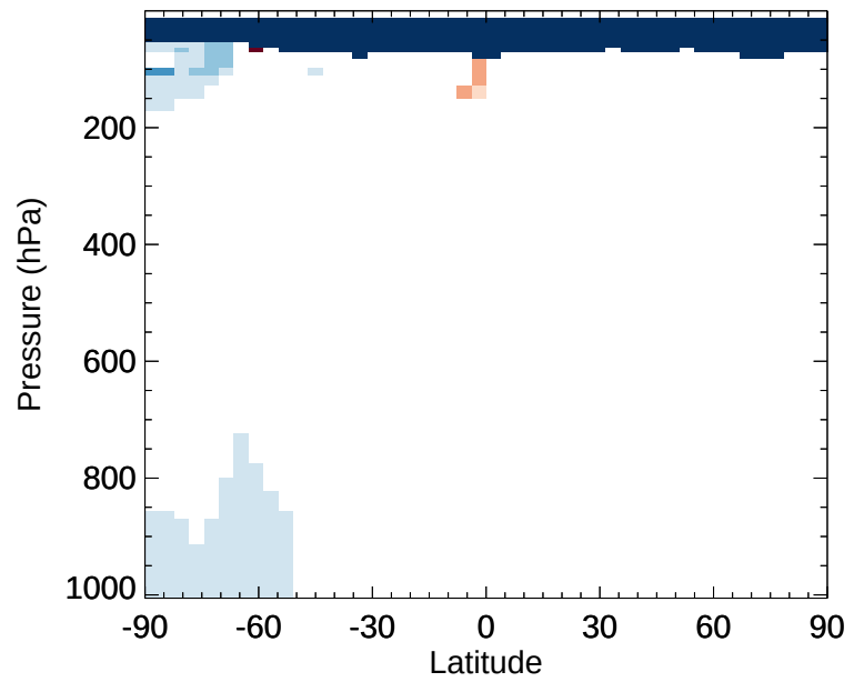
v11-02d / v11-02c SO4s - Zonal mean % diff for Oct
