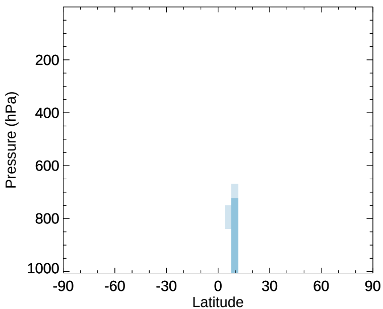
v11-02d - v11-02c MVK - Zonal mean abs diff for Oct
