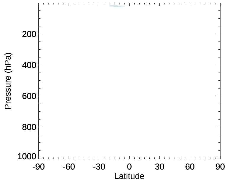
v11-02d / v11-02a CCl4 - Zonal mean % diff for Oct
