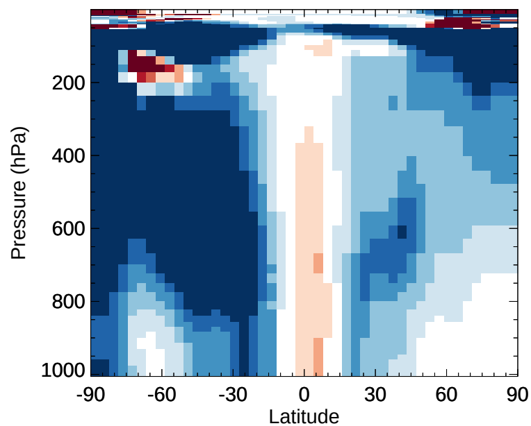
v11-02d / v11-02c MVK - Zonal mean % diff for Oct
