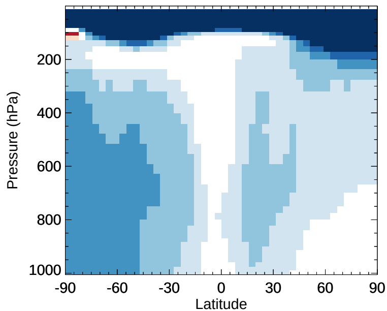
v11-02d / v11-02c EOH - Zonal mean % diff for Oct
