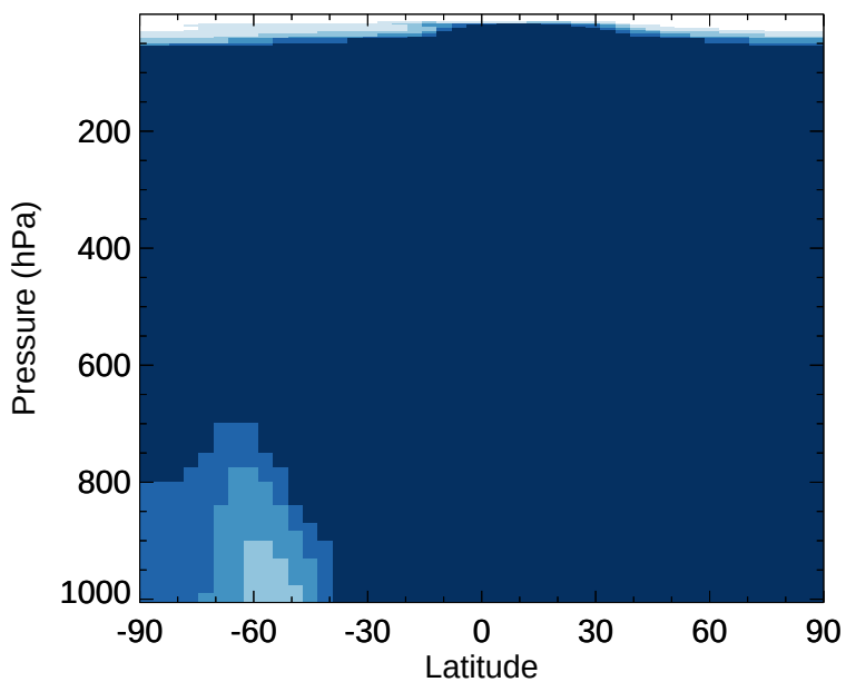
v11-02d - v11-02a EOH - Zonal mean abs diff for Oct
