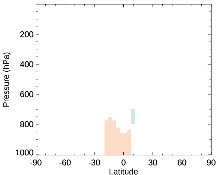
v11-02d - v11-02a MVK - Zonal mean abs diff for Oct
