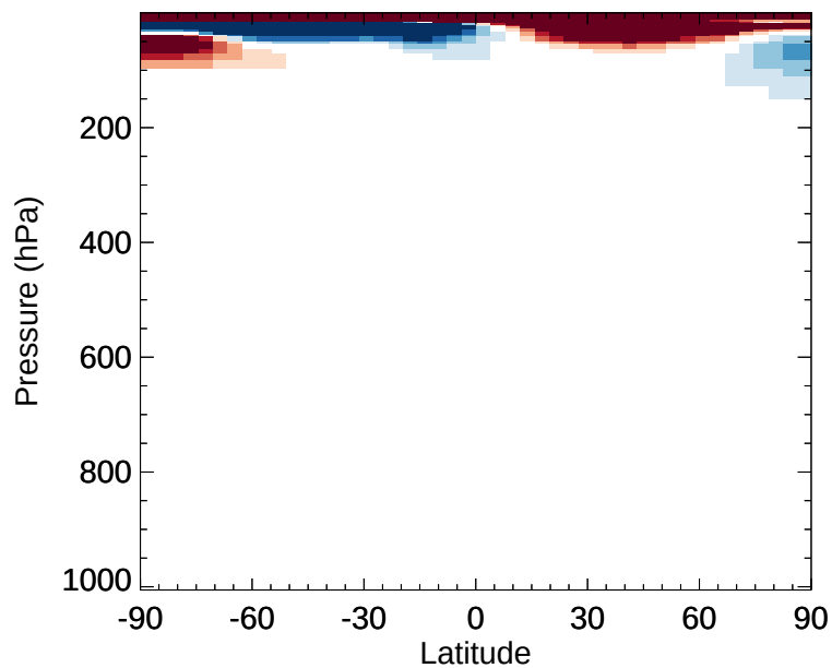
v11-02d / v11-02c OCS - Zonal mean % diff for Oct
