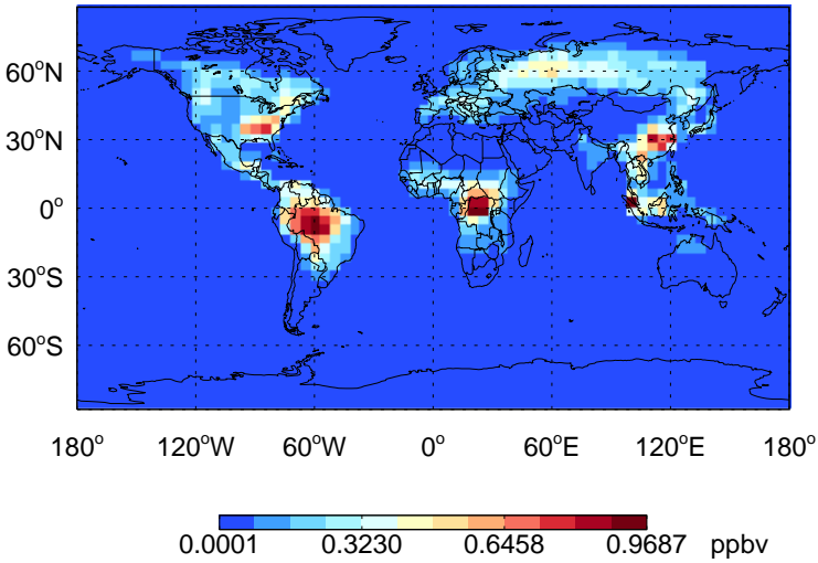
TSOG3 - Species map @ surface for Jul
