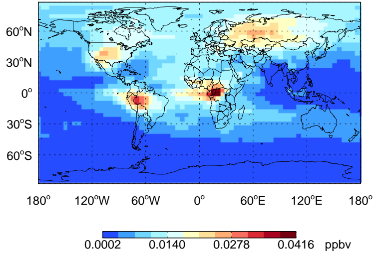
TSOG3 - Species map @ 500 hPa for Jul
