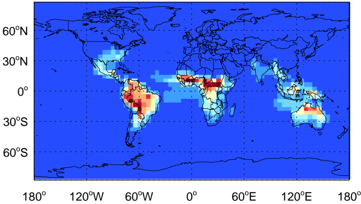
ISOOG1 - Species map @ surface for Oct
