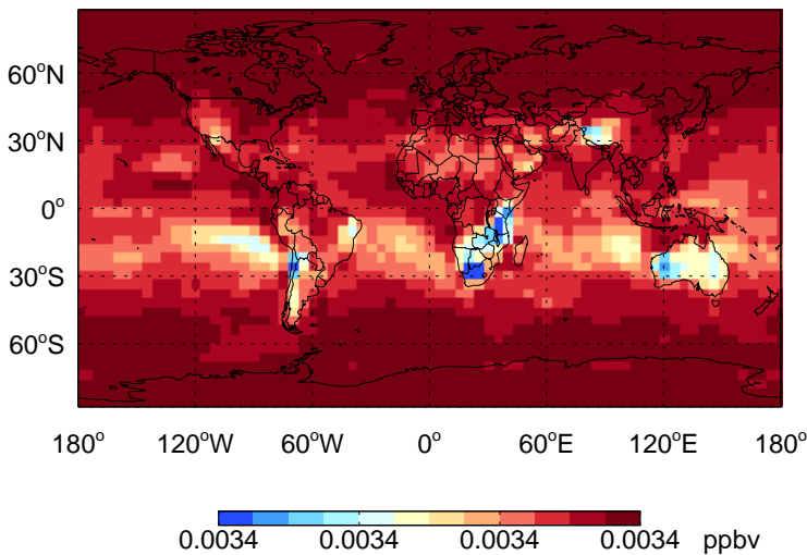
H1211 - Species map @ surface for Oct
