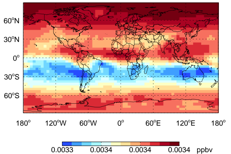
H1211 - Species map @ 500 hPa for Oct
