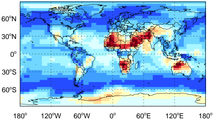
HCl - Species map @ surface for Oct
