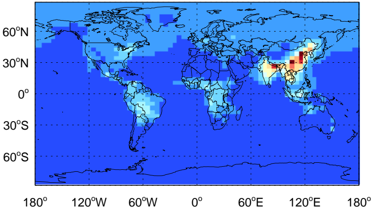
CO - Species map @ surface for Oct
