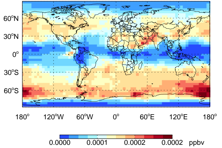
Br2 - Species map @ 500 hPa for Oct
