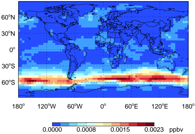
Br2 - Species map @ surface for Oct
