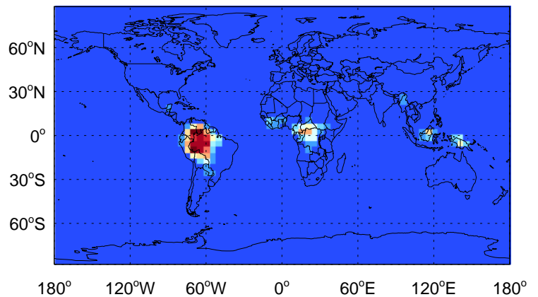
ISOPNB - Species map @ 500 hPa for Oct
