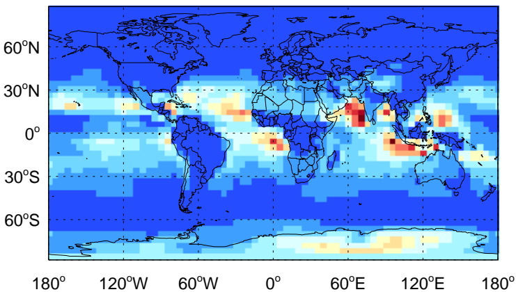
Br - Species map @ surface for Oct
