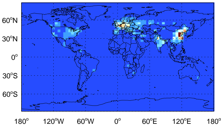
NO 2 - Species map @ surface for Oct
