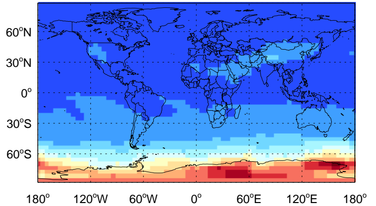
Br - Species map @ 500 hPa for Oct
