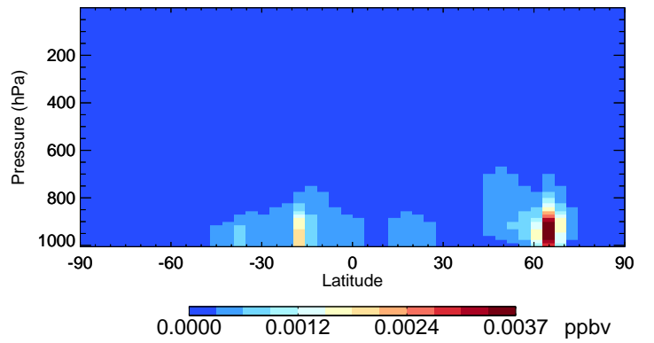
v11-02d MGLY - Species Curtain @ -180.000 for Jul
