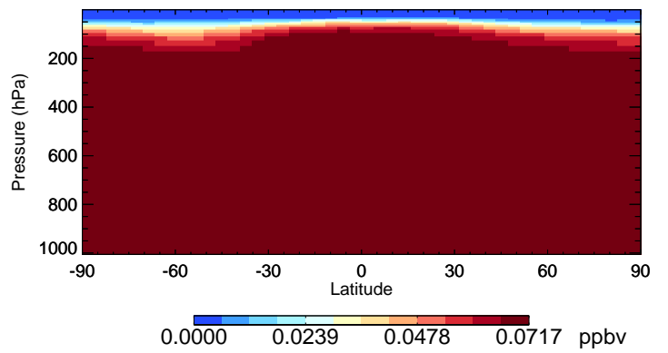
v11-02d CCI4 - Species Curtain @ -180.000 for Jul
