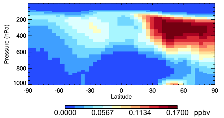
v11-02d PAN - Species Curtain @ -180.000 for Jul
