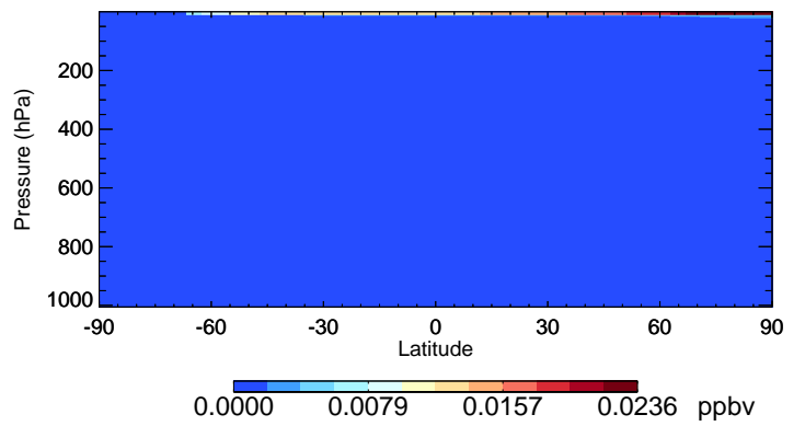
v11-02d Br - Species Curtain @ -180.000 for Jul
