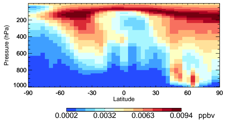
v11-02d ISOG3 - Species Curtain @ -180.000 for Jul
