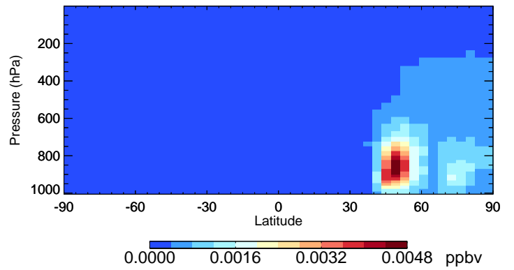
v11-02d SOAME - Species Curtain @ -180.000 for Jul
