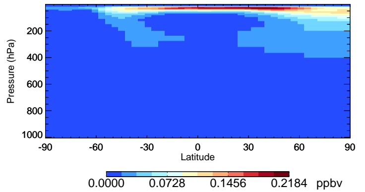
v11-02d HNO4 - Species Curtain @ -180.000 for Jul
