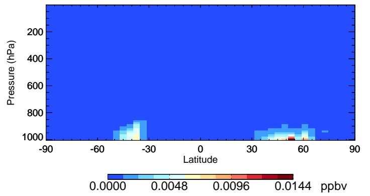
v11-02c BCPO - Species Curtain @ -180.000 for Jul
