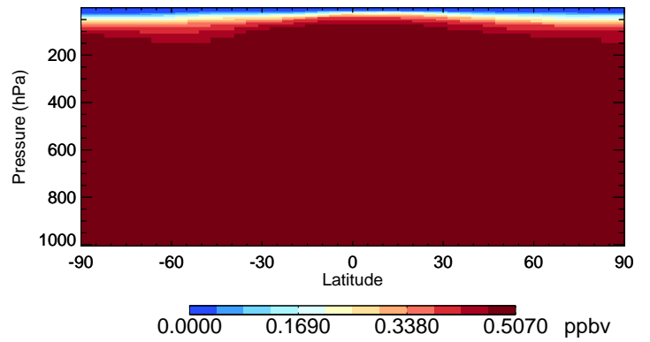
v11-02d CFC12 - Species Curtain @ -180.000 for Jul
