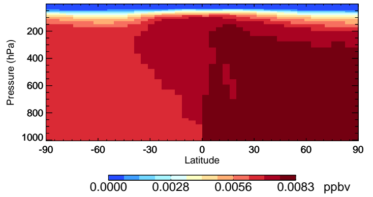
v11-02a CH3Br - Species Curtain @ -180.000 for Jul
