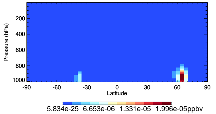
v11-02d MACRN - Species Curtain @ -180.000 for Jul
