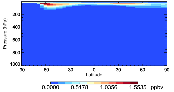
v11-02c ClNO3 - Species Curtain @ -180.000 for Jul
