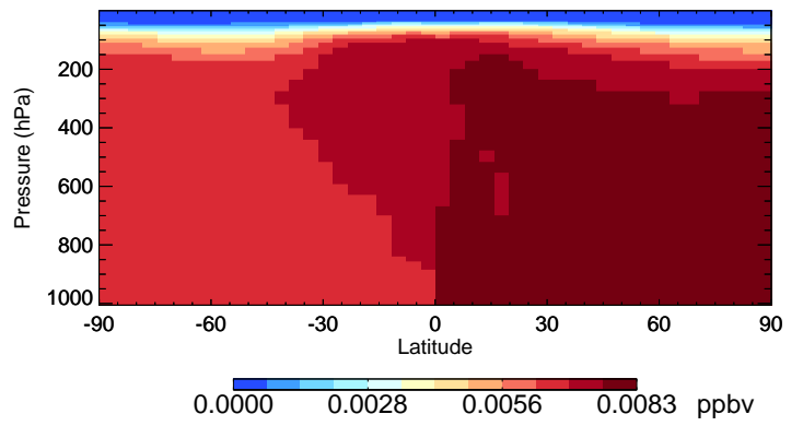
v11-02c CH3Br - Species Curtain @ -180.000 for Jul
