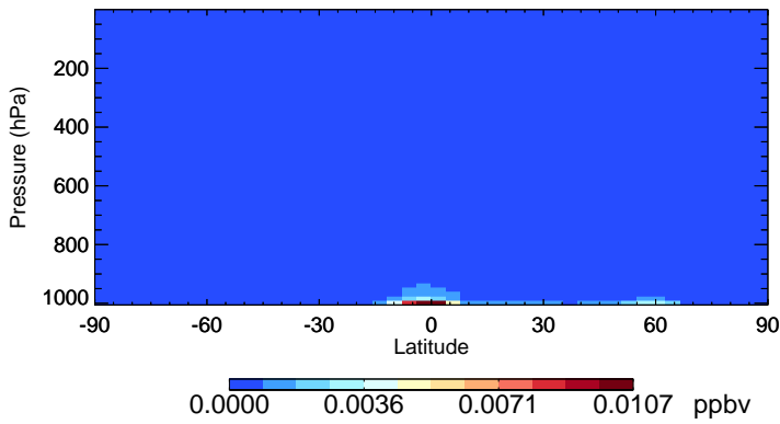
v11-02d MTPO - Species Zonal Mean for Jul
