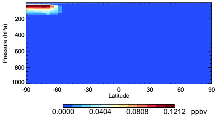
v11-02d OCIO - Species Zonal Mean for Jul
