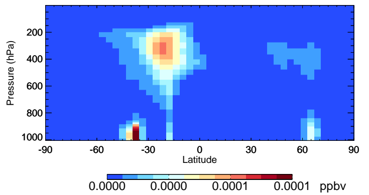
v11-02d HONIT - Species Curtain @ -180.000 for Jul
