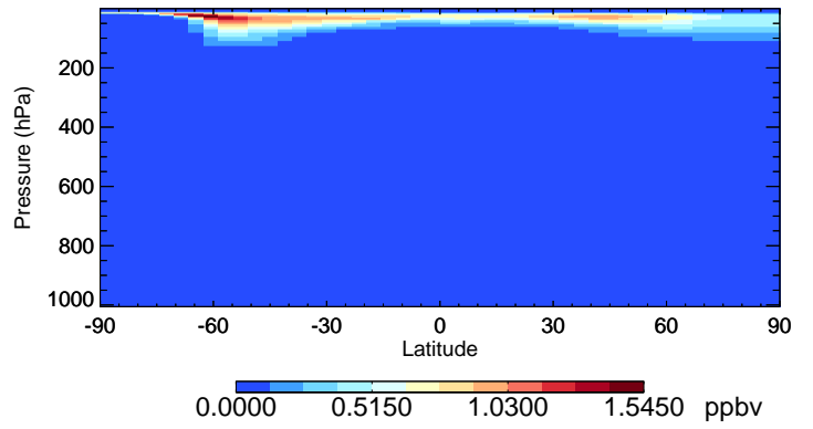
v11-02a ClNO3 - Species Curtain @ -180.000 for Jul
