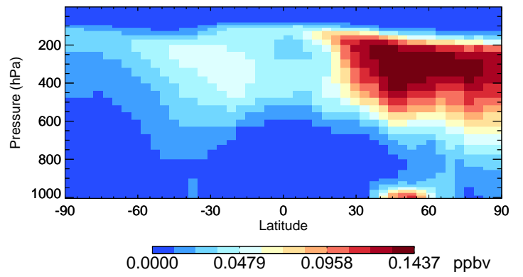
v11-02a PAN - Species Curtain @ -180.000 for Jul
