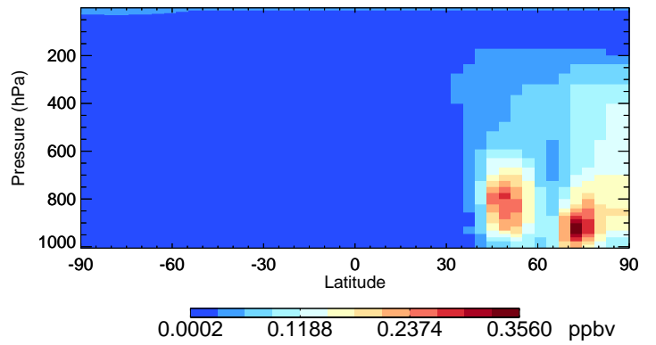
v11-02d OCPI - Species Curtain @ -180.000 for Jul
