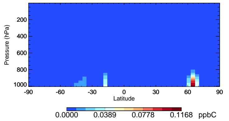
v11-02c PRPE - Species Curtain @ -180.000 for Jul
