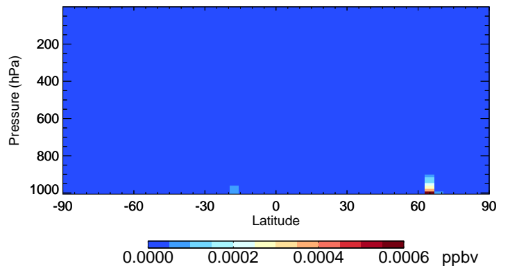
v11-02c LIMO - Species Curtain @ -180.000 for Jul
