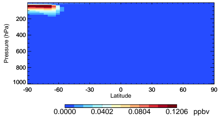
v11-02d OCIO - Species Curtain @ -180.000 for Jul
