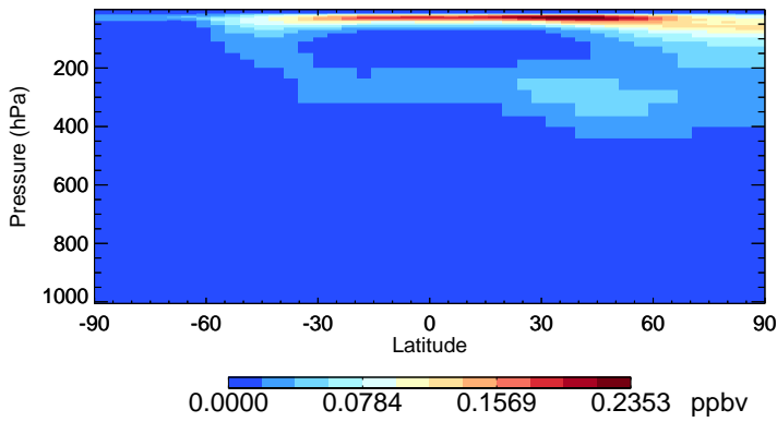
v11-02d HNO4 - Species Zonal Mean for Jul
