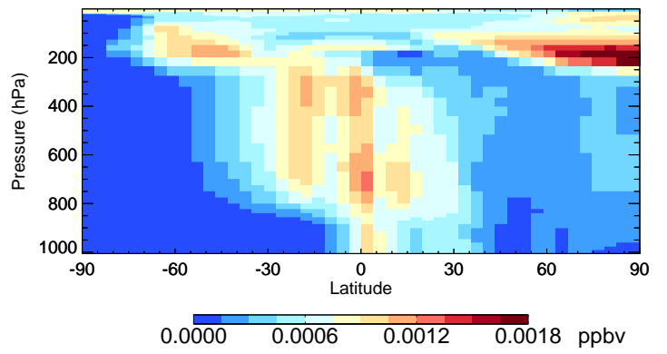
v11-02c HBr - Species Curtain @ -180.000 for Jul
