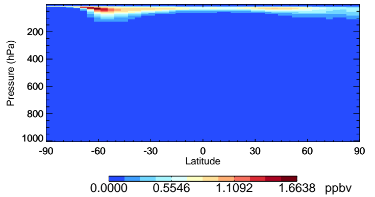
v11-02d ClNO3 - Species Curtain @ -180.000 for Jul
