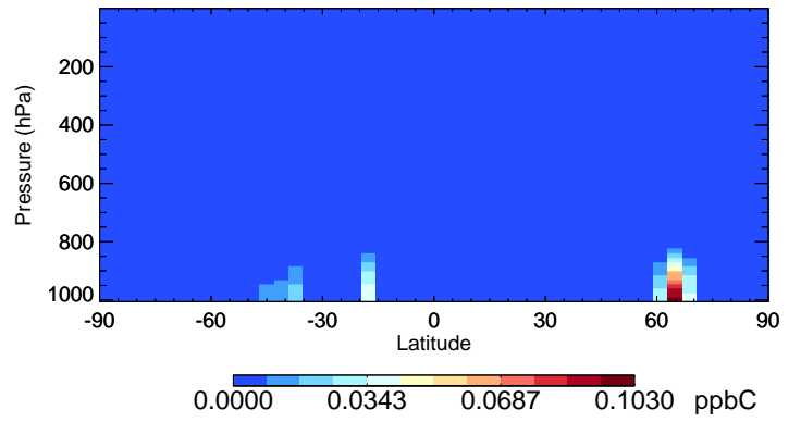
v11-02a PRPE - Species Curtain @ -180.000 for Jul
