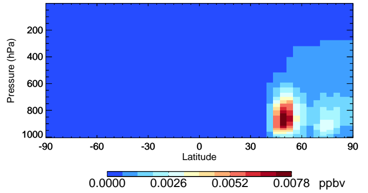
v11-02c SOAME - Species Curtain @ -180.000 for Jul
