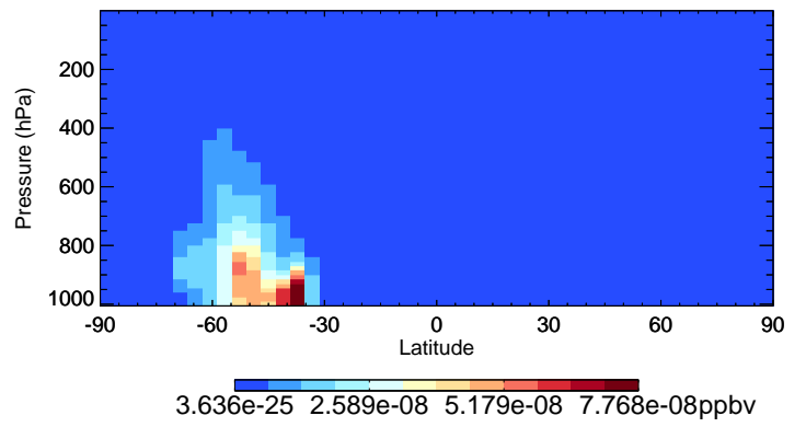
v11-02c NPMN - Species Curtain @ -180.000 for Jul
