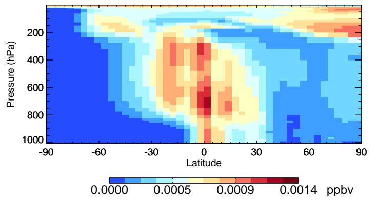
v11-02a HBr - Species Curtain @ -180.000 for Jul
