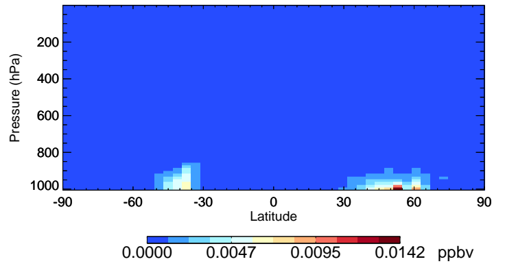
v11-02a BCPO - Species Curtain @ -180.000 for Jul
