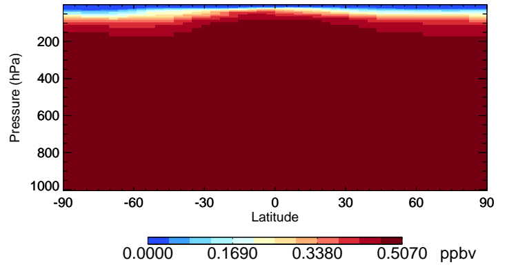
v11-02c CFC12 - Species Curtain @ -180.000 for Jul
