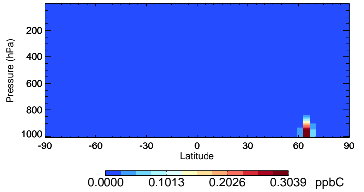
v11-02a ISOP - Species Curtain @ -180.000 for Jul
