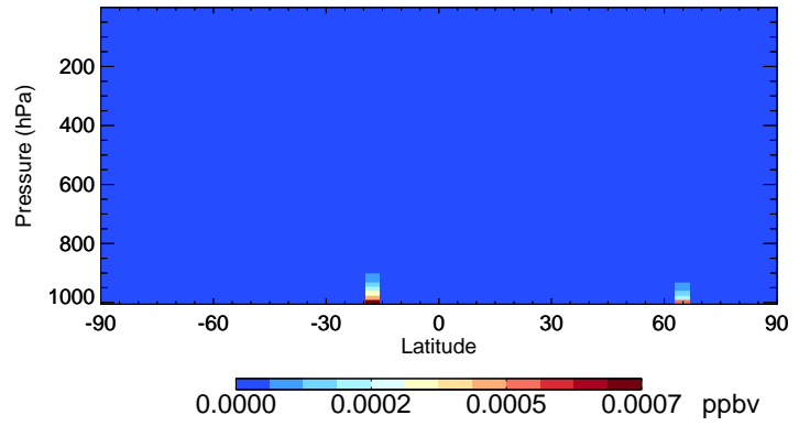
v11-02c MTPO - Species Curtain @ -180.000 for Jul
