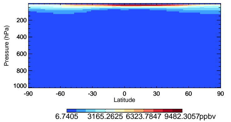
v11-02d O3 - Species Curtain @ -180.000 for Jul
