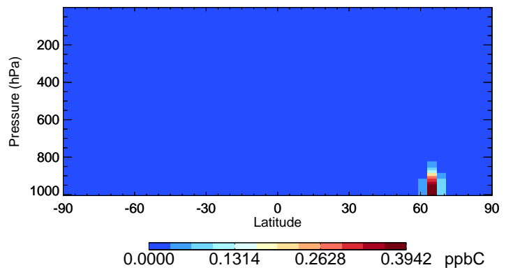
v11-02d ISOP - Species Curtain @ -180.000 for Jul
