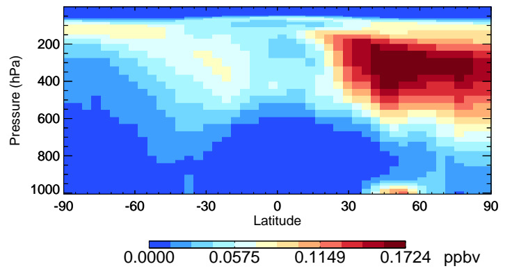
v11-02c PAN - Species Curtain @ -180.000 for Jul
