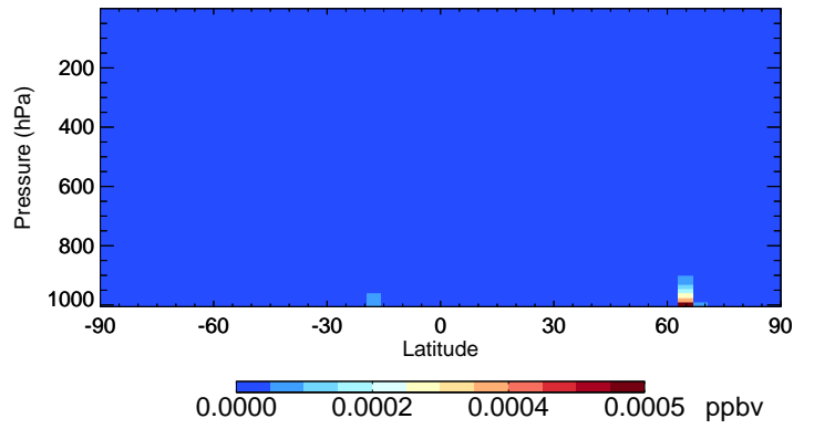
v11-02a LIMO - Species Curtain @ -180.000 for Jul
