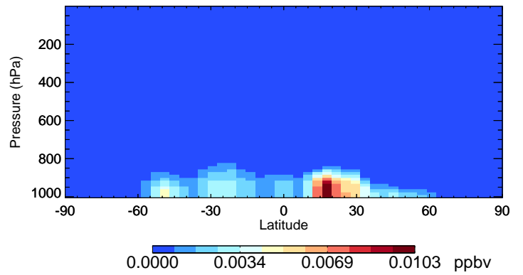
v11-02d NITs - Species Curtain @ -180.000 for Jul
