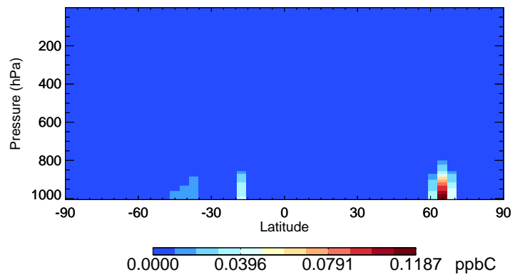
v11-02d PRPE - Species Curtain @ -180.000 for Jul
