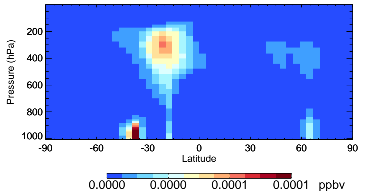
v11-02c HONIT - Species Curtain @ -180.000 for Jul
