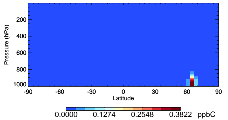
v11-02c ISOP - Species Curtain @ -180.000 for Jul
