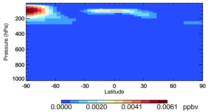
v11-02d ISOA3 - Species Curtain @ -180.000 for Jul
