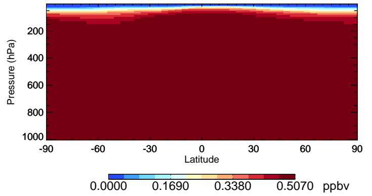
v11-02a CFC12 - Species Curtain @ -180.000 for Jul
