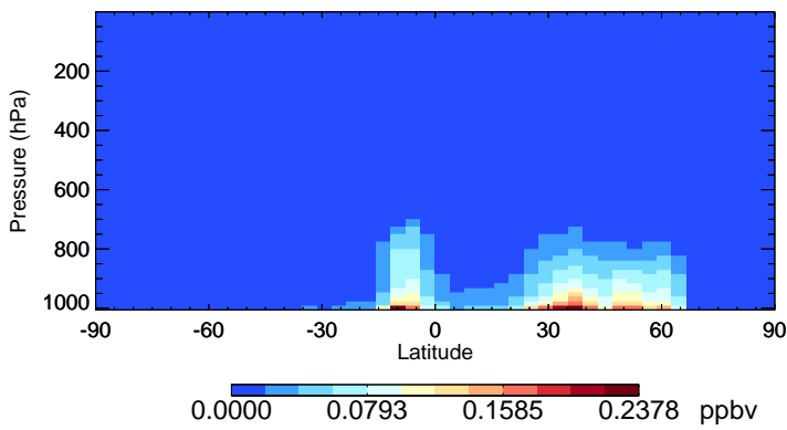
v11-02d BCPO - Species Zonal Mean for Jul
