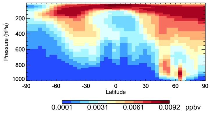
v11-02a ISOG3 - Species Curtain @ -180.000 for Jul
