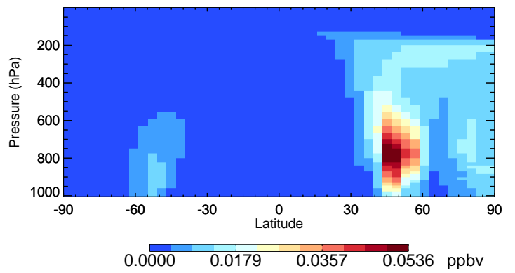
v11-02d DST1 - Species Curtain @ -180.000 for Jul
