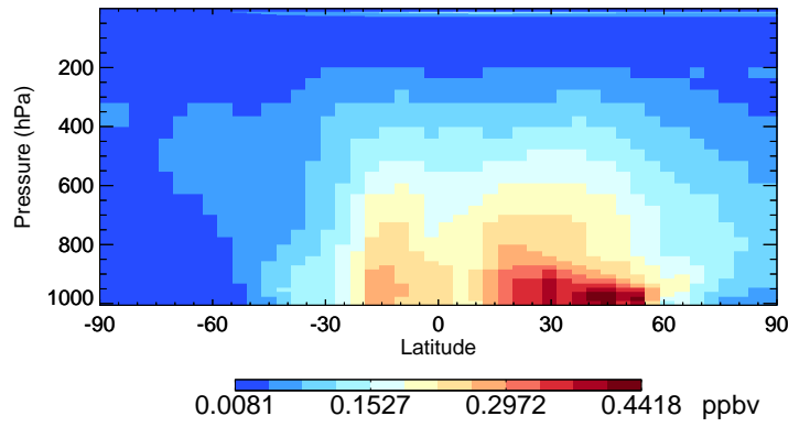
v11-02a CH2O - Species Curtain @ -180.000 for Jul
