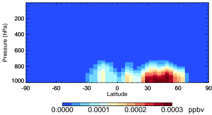
v11-02d MACRN - Species Zonal Mean for Jul
