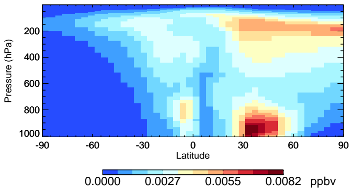
ASOG3 - Species Zonal Mean for Jul
