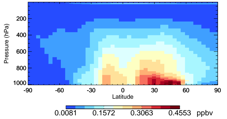
v11-02c CH2O - Species Curtain @ -180.000 for Jul
