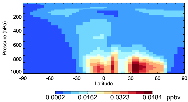
v11-02d ISOG3 - Species Zonal Mean for Jul
