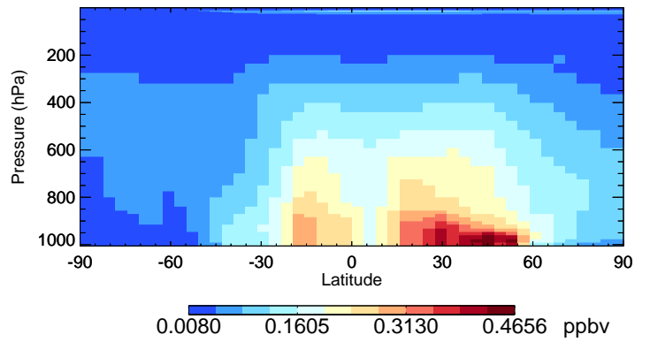
v11-02d CH2O - Species Curtain @ -180.000 for Jul
