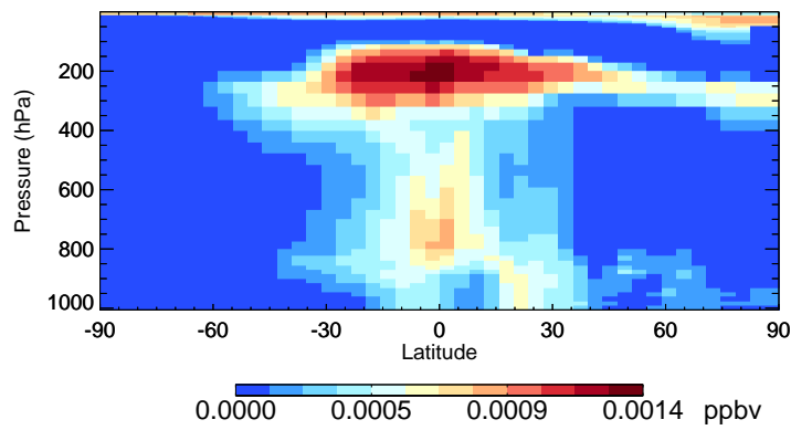
v11-02d HBr - Species Curtain @ -180.000 for Jul
