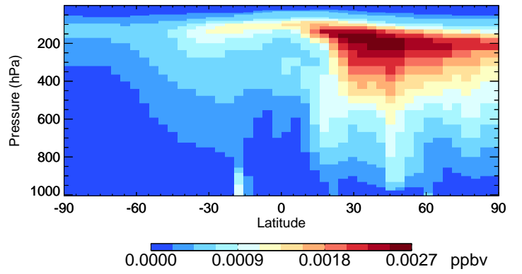
v11-02a MGLY - Species Curtain @ -180.000 for Jul
