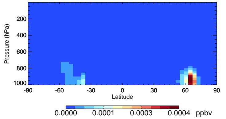
v11-02a NPMN - Species Curtain @ -180.000 for Jul
