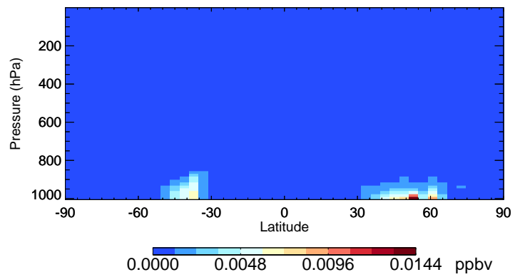
v11-02d BCPO - Species Curtain @ -180.000 for Jul
