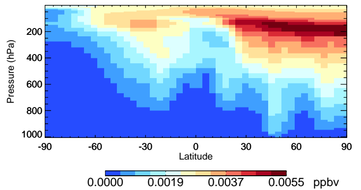
ASOG3 - Species Curtain @ -180.000 for Jul
