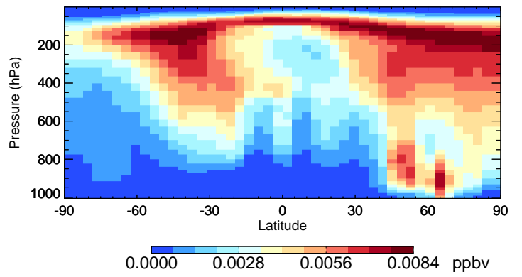
v11-02c ISOG3 - Species Curtain @ -180.000 for Jul
