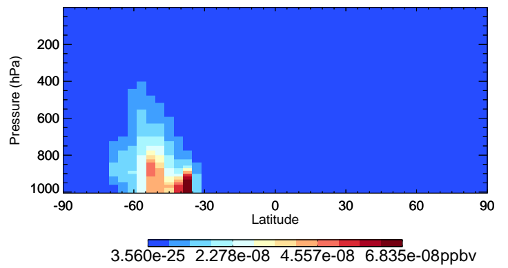
v11-02d NPMN - Species Curtain @ -180.000 for Jul
