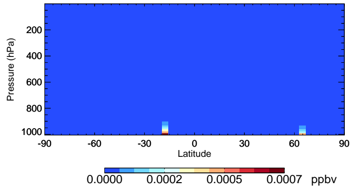
v11-02a MTPO - Species Curtain @ -180.000 for Jul
