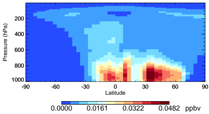
v11-02c ISOG3 - Species Zonal Mean for Jul
