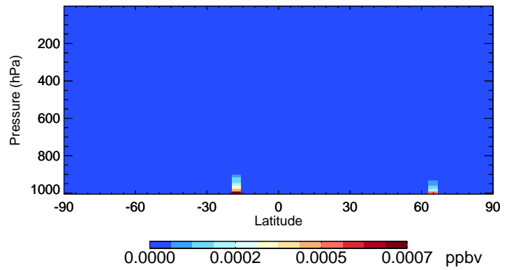
v11-02d MTPO - Species Curtain @ -180.000 for Jul
