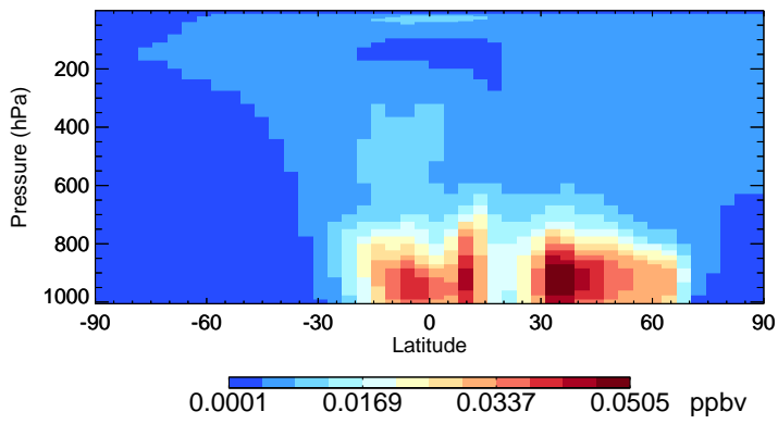
v11-02a ISOG3 - Species Zonal Mean for Jul
