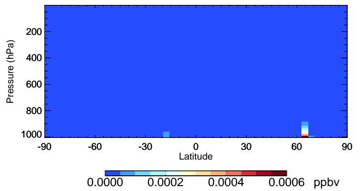
v11-02d LIMO - Species Curtain @ -180.000 for Jul
