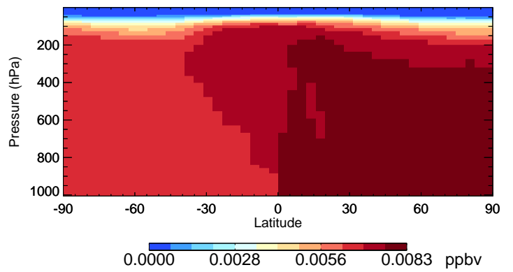
v11-02d CH3Br - Species Curtain @ -180.000 for Jul
