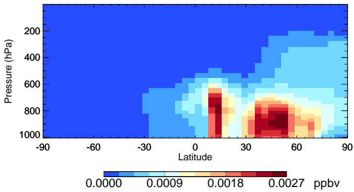
v11-02d SOAME - Species Zonal Mean for Jul
