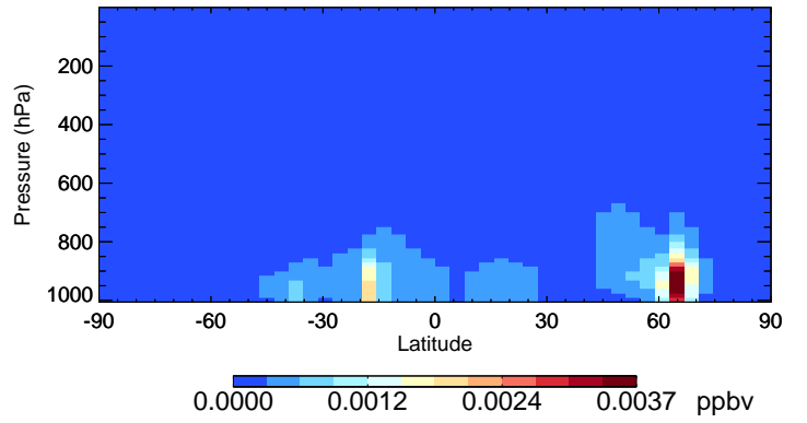
v11-02c MGLY - Species Curtain @ -180.000 for Jul
