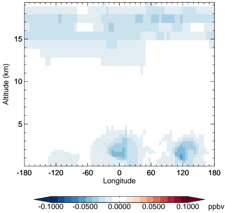
v11-02d - v11-02c HCl - Diff along 15S for Oct
