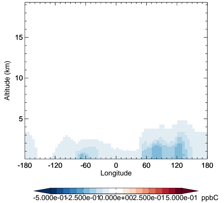
v11-02d - v11-02a ALK4 - Diff along 42N for Oct
