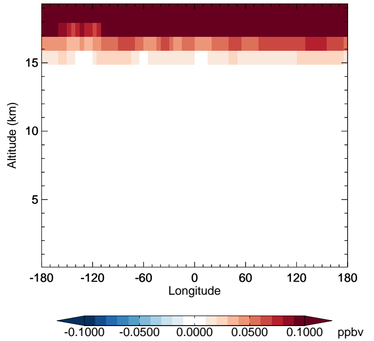
v11-02d - v11-02a HCl - Diff along 42N for Oct
