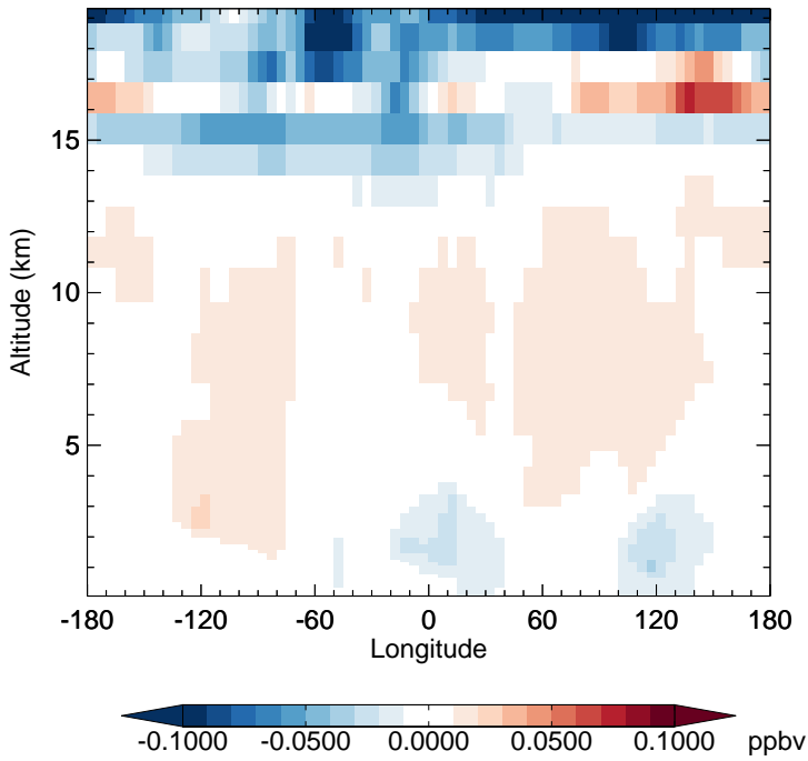
v11-02d - v11-02a HCl - Diff along 15S for Oct
