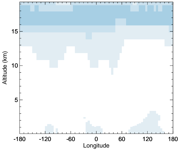
v11-02d - v11-02a C2H6 - Diff along 15S for Oct
