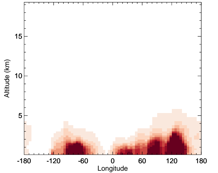
v11-02d - v11-02a SOAS - Diff along 42N for Oct
