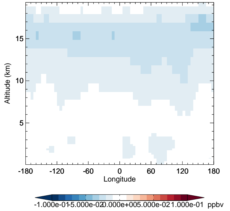
v11-02d - v11-02c HCl - Diff along 42N for Oct
