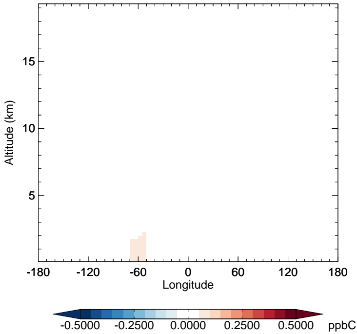
v11-02d - v11-02a ALK4 - Diff along 15S for Oct
