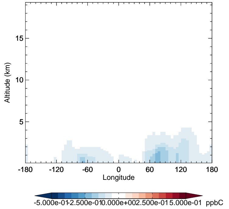
v11-02d - v11-02c ALK4 - Diff along 42N for Oct
