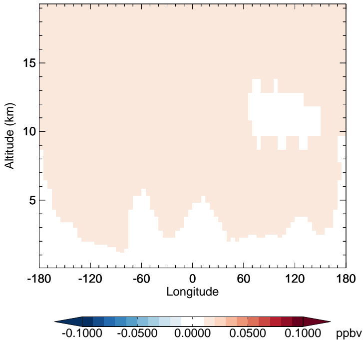
v11-02d - v11-02a HCFC141b - Diff along 15S for Oct
