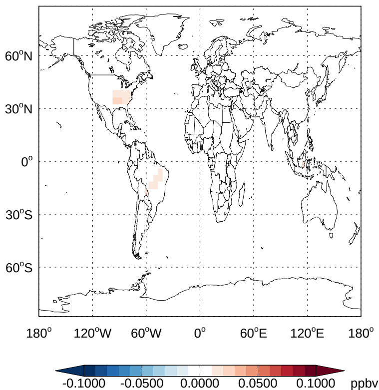
v11-02d - v11-02a ISOPNB - Diff @ Surface for Jul
