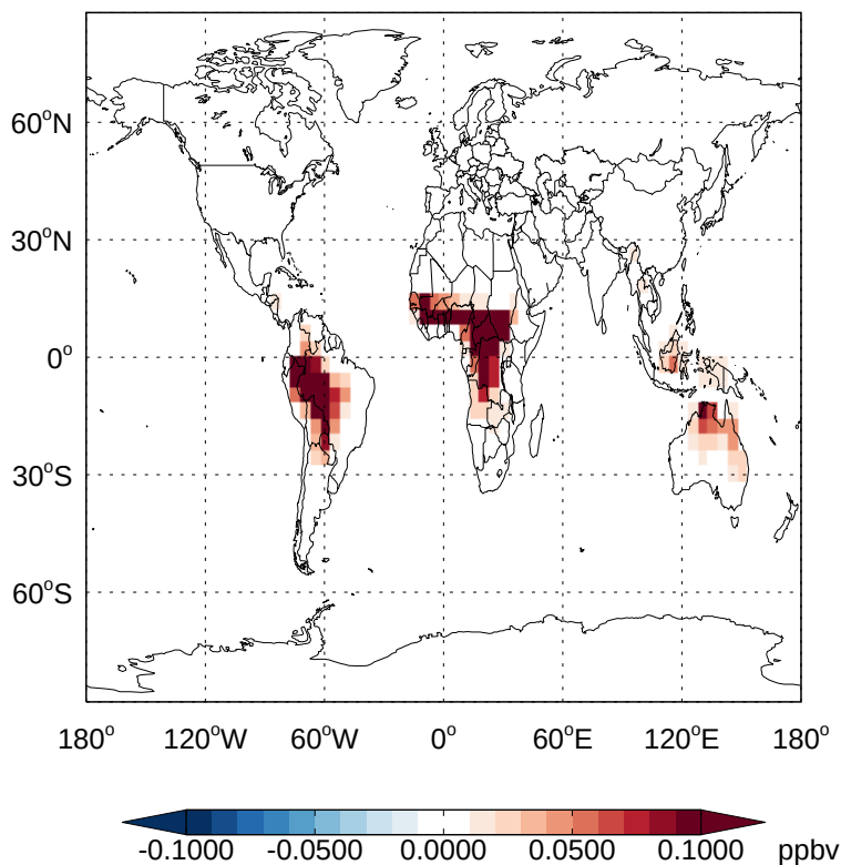
v11-02d - v11-02a IEPOXA - Diff @ Surface for Oct
