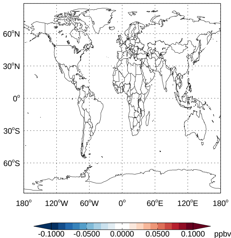
v11-02d - v11-02a CFC113 - Diff @ Surface for Oct
