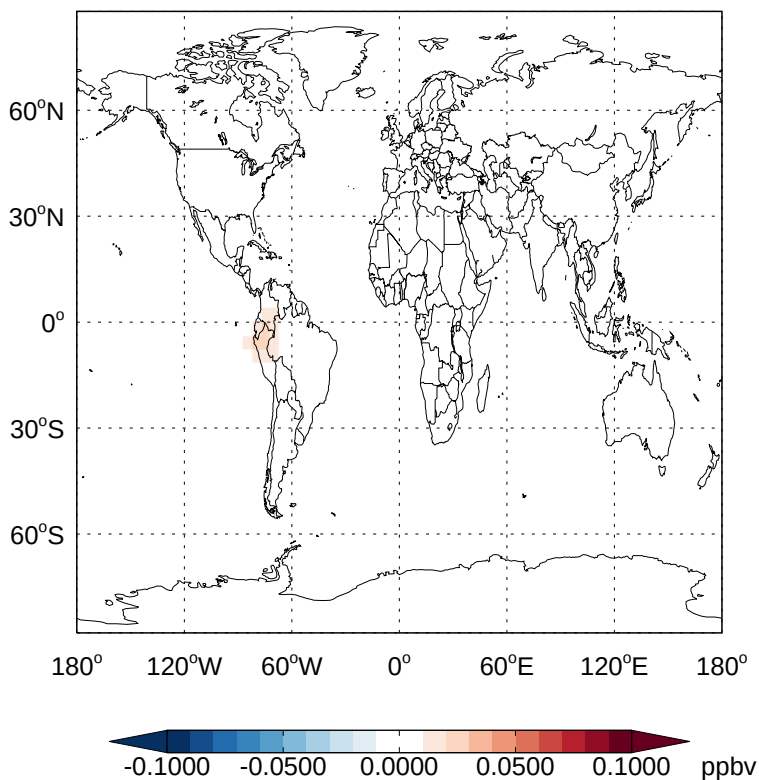
v11-02d - v11-02a IEPOXA- Diff @ 500 hPa for Oct
