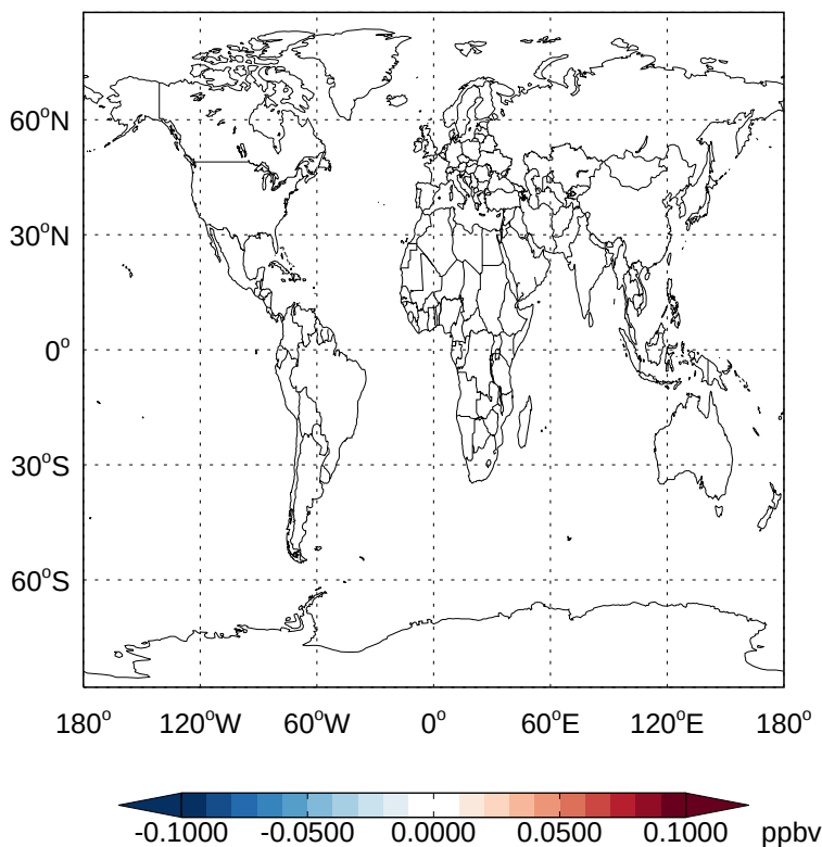
v11-02d - v11-02a ISOPND- Diff @ 500 hPa for Oct
