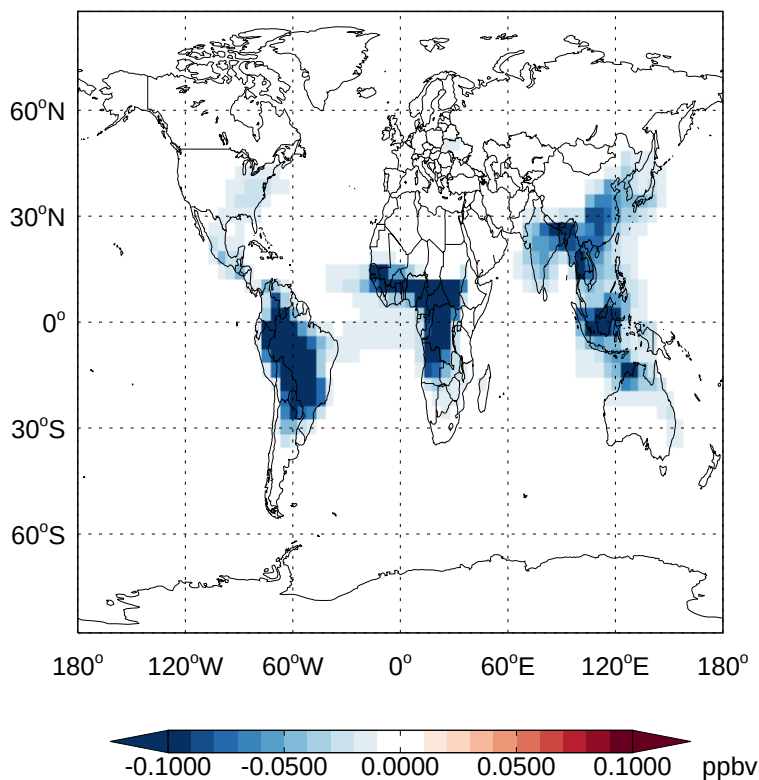
v11-02d - v11-02a SOAGX - Diff @ Surface for Oct
