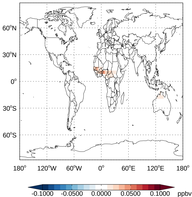
v11-02d - v11-02a MONITA - Diff @ Surface for Oct
