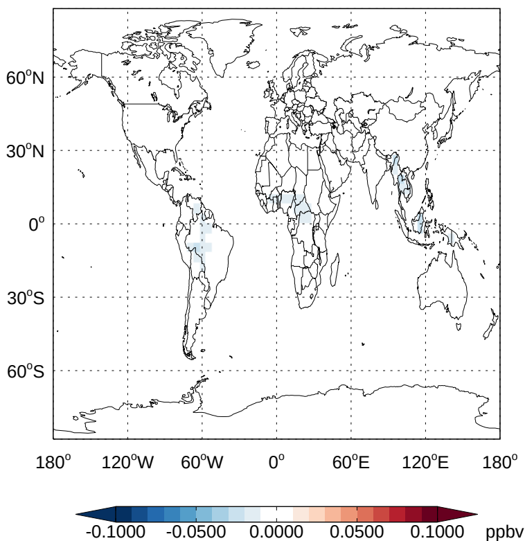
v11-02d - v11-02a ISOPND - Diff @ Surface for Oct
