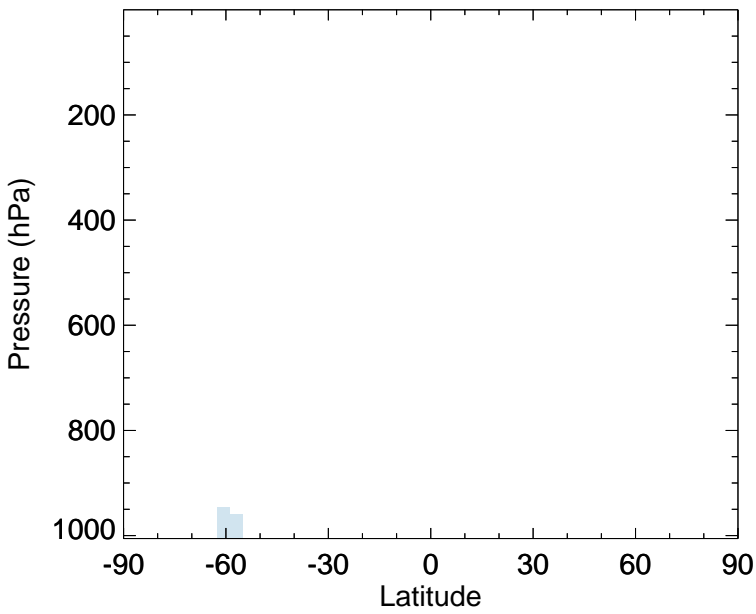
v11-02d - v11-02c BrO - Zonal mean abs diff for Apr
