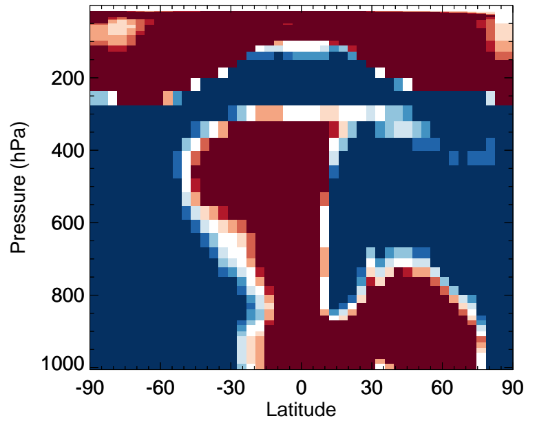
v11-02d / v11-02c Br2 - Zonal mean % diff for Apr
