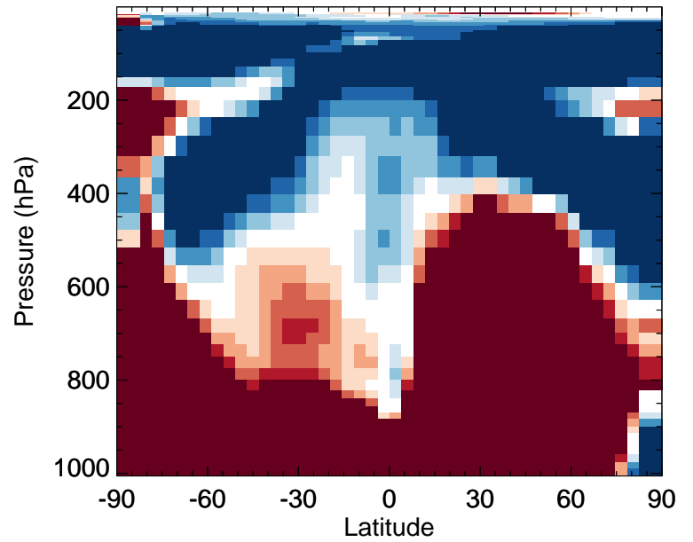
v11-02d / v11-02a ClO - Zonal mean % diff for Apr
