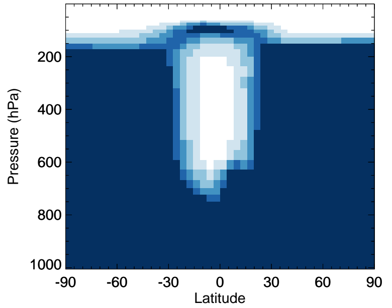
v11-02d / v11-02c HCl - Zonal mean % diff for Apr
