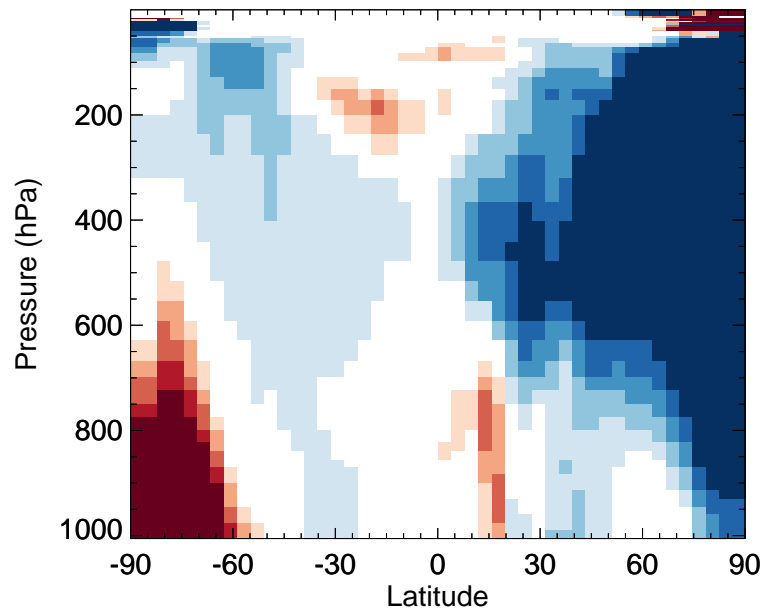
v11-02d / v11-02c ISN1 - Zonal mean % diff for Apr
