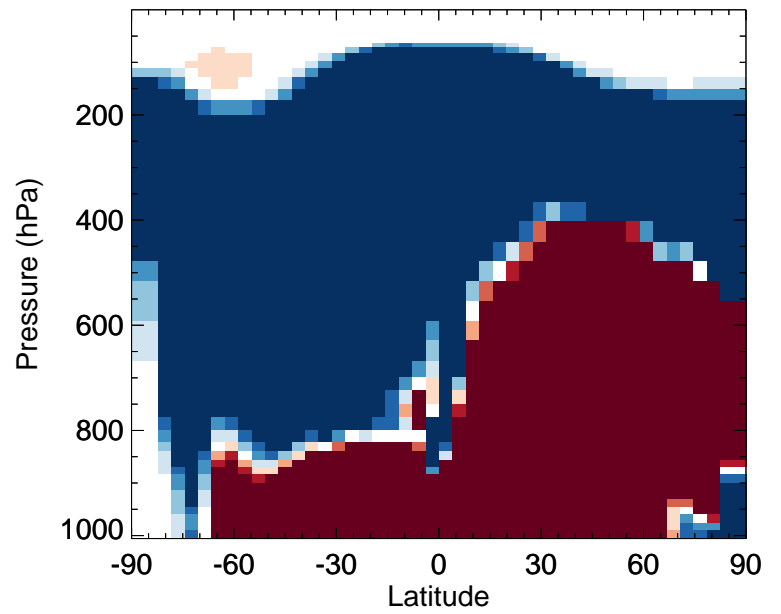
v11-02d / v11-02c Cl2 - Zonal mean % diff for Apr
