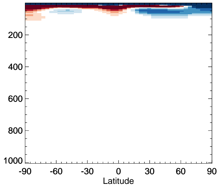
v11-02d / v11-02a OCS - Zonal mean % diff for Apr
