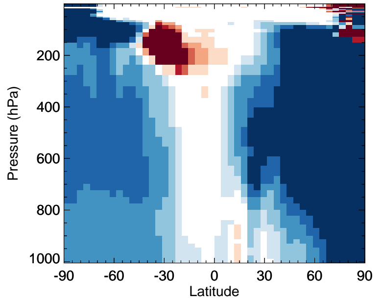
v11-02d / v11-02c RIPD - Zonal mean % diff for Apr
