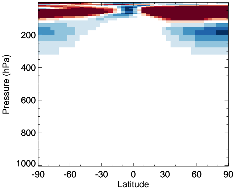
v11-02d - v11-02a HCl - Zonal mean abs diff for Apr
