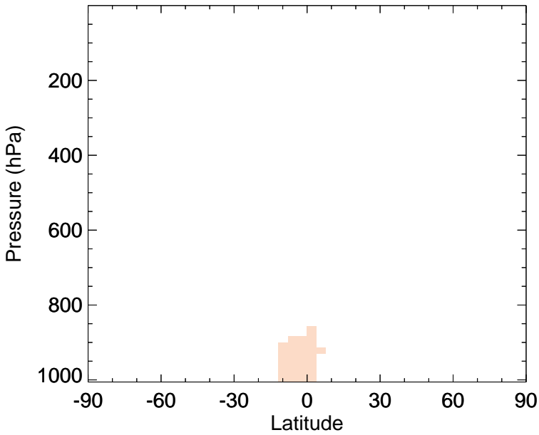
v11-02d - v11-02a RIPB - Zonal mean abs diff for Apr
