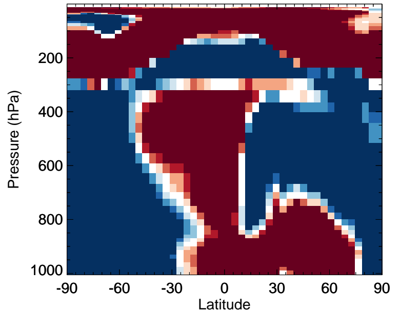
v11-02d / v11-02a Br2 - Zonal mean % diff for Apr
