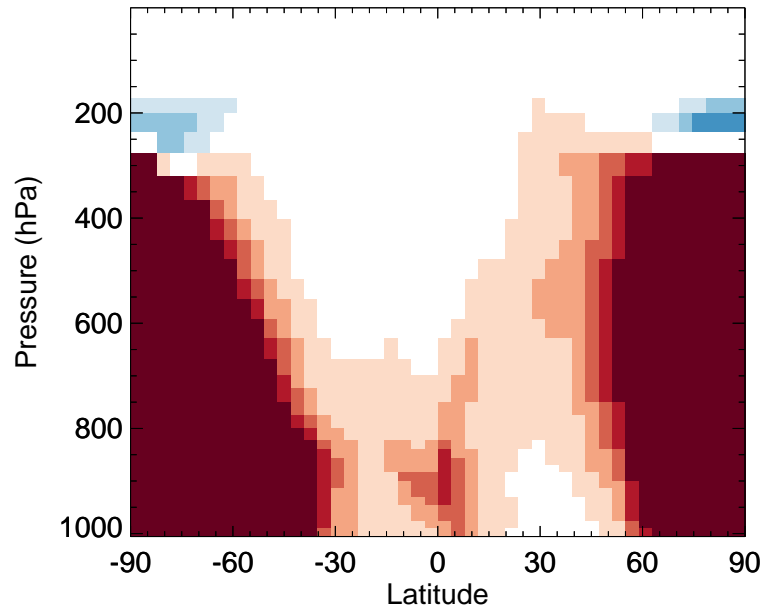
v11-02d / v11-02c NO - Zonal mean % diff for Apr
