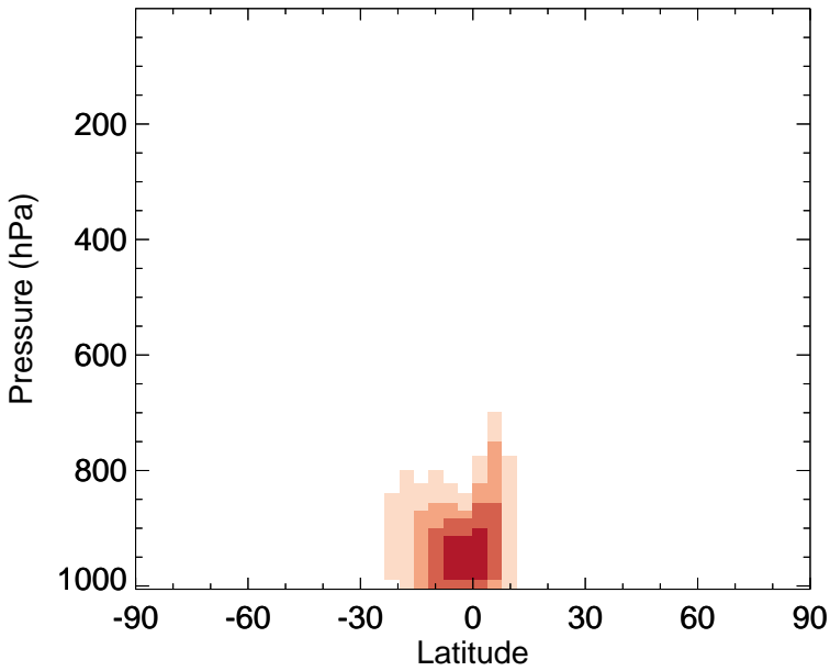
v11-02d - v11-02a RIPA - Zonal mean abs diff for Apr
