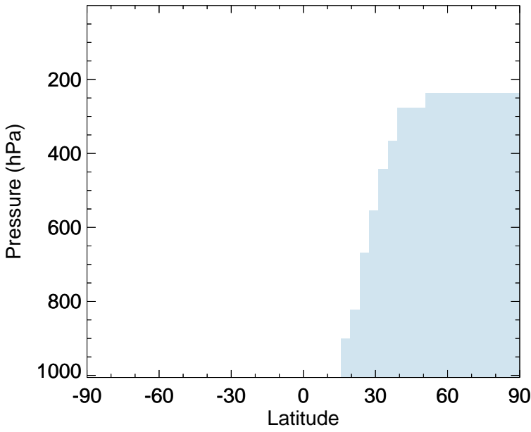
v11-02d - v11-02c CO - Zonal mean abs diff for Apr
