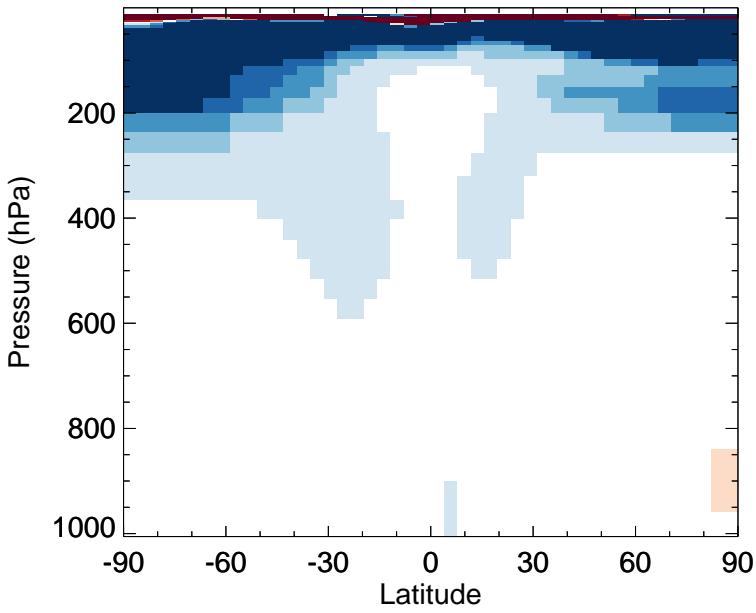
v11-02d - v11-02a O3 - Zonal mean abs diff for Apr
