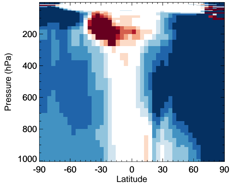
v11-02d / v11-02c RIPA - Zonal mean % diff for Apr
