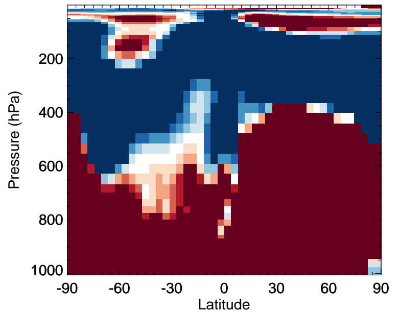
v11-02d / v11-02a Cl2 - Zonal mean % diff for Apr
