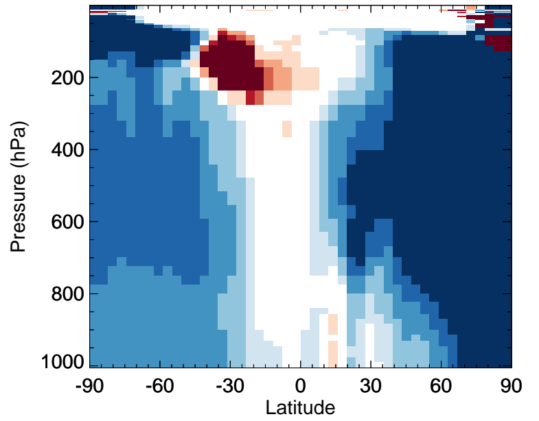
v11-02d / v11-02c RIPB - Zonal mean % diff for Apr
