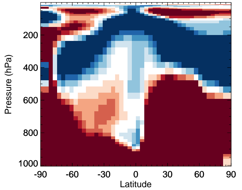
v11-02d / v11-02a Cl - Zonal mean % diff for Apr
