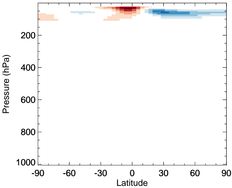
v11-02d - v11-02a OCS - Zonal mean abs diff for Apr
