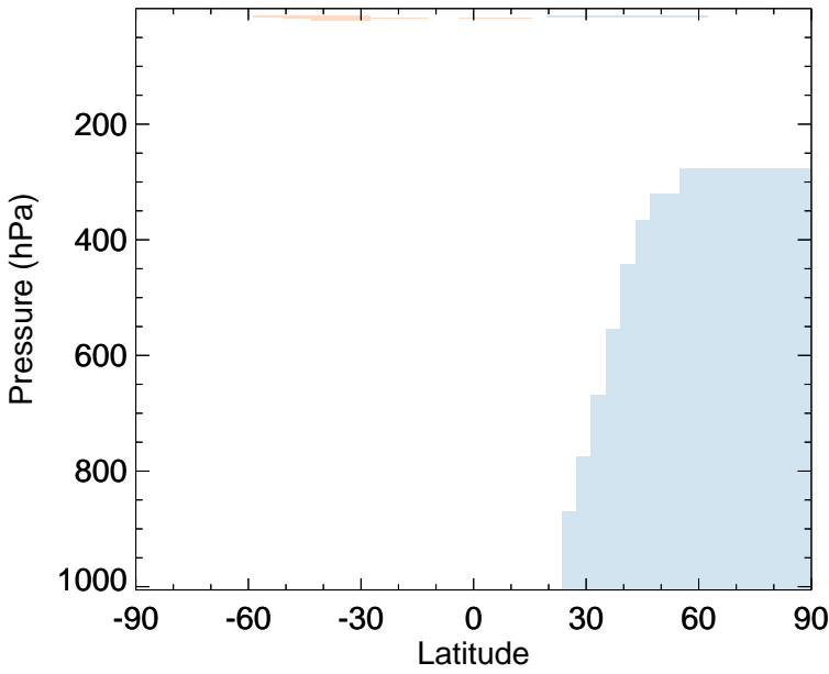
v11-02d - v11-02a CO - Zonal mean abs diff for Apr
