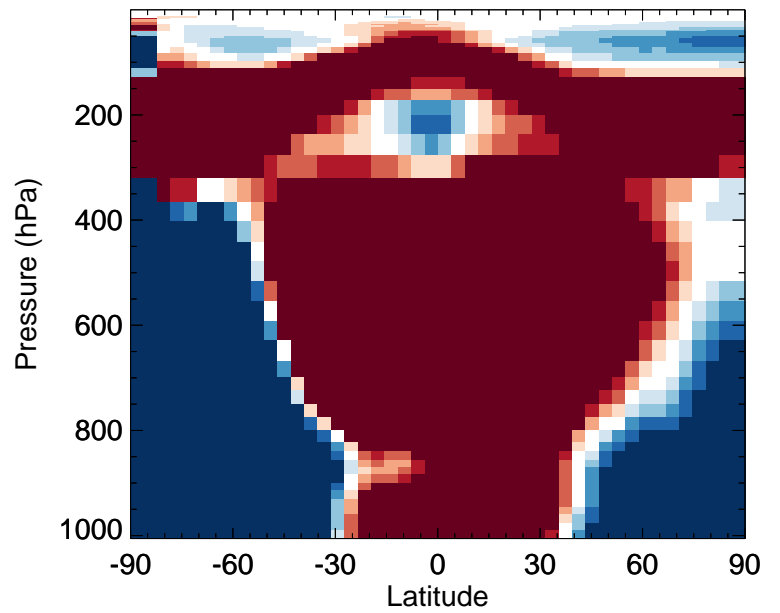
v11-02d / v11-02a BrO - Zonal mean % diff for Apr
