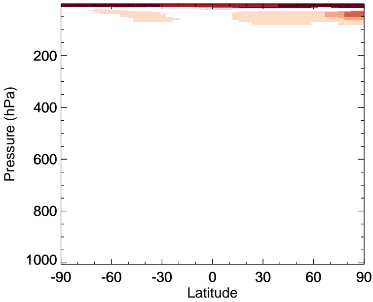
v11-02d - v11-02a NO - Zonal mean abs diff for Apr
