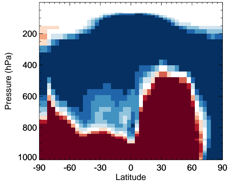
v11-02d / v11-02c ClO - Zonal mean % diff for Apr
