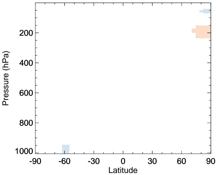
v11-02d - v11-02a BrO - Zonal mean abs diff for Apr
