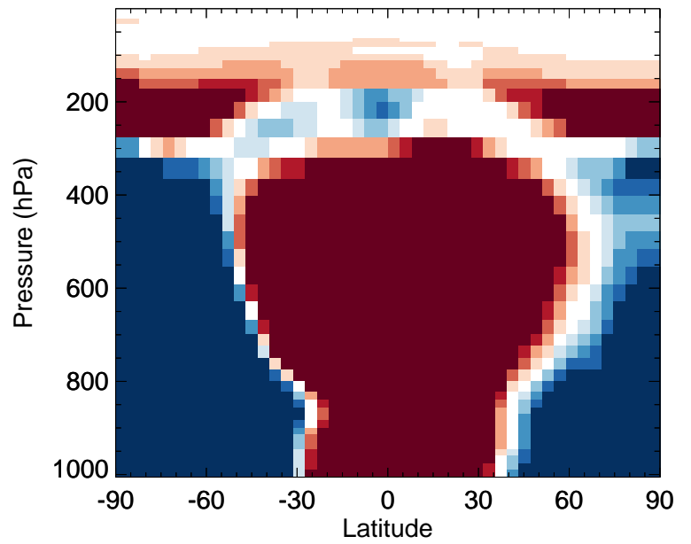
v11-02d / v11-02c BrO - Zonal mean % diff for Apr
