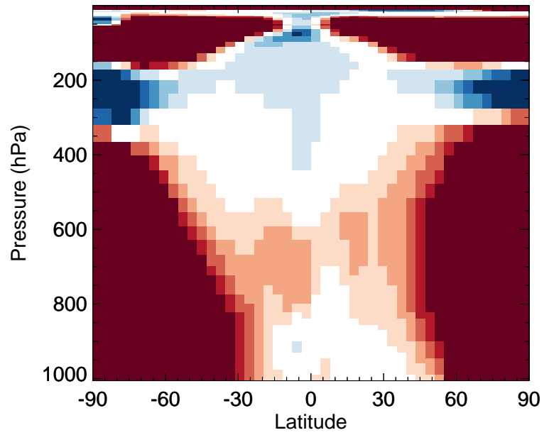
v11-02d / v11-02a NO - Zonal mean % diff for Apr
