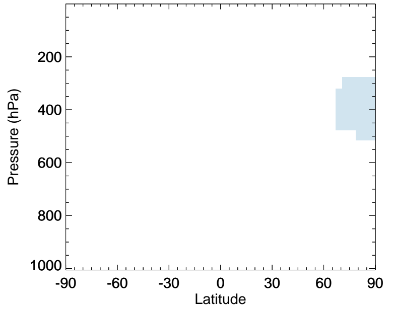
v11-02d / v11-02c CO - Zonal mean % diff for Apr
