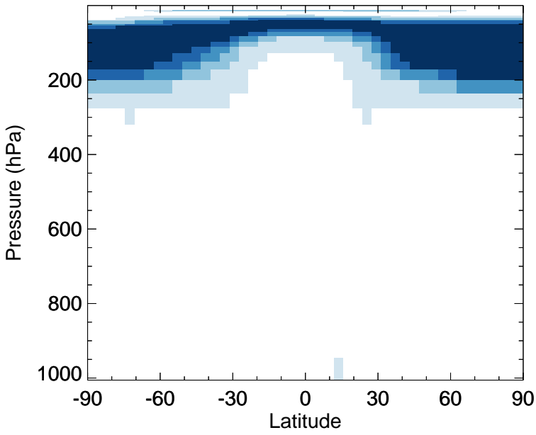
v11-02d - v11-02c O3 - Zonal mean abs diff for Apr
