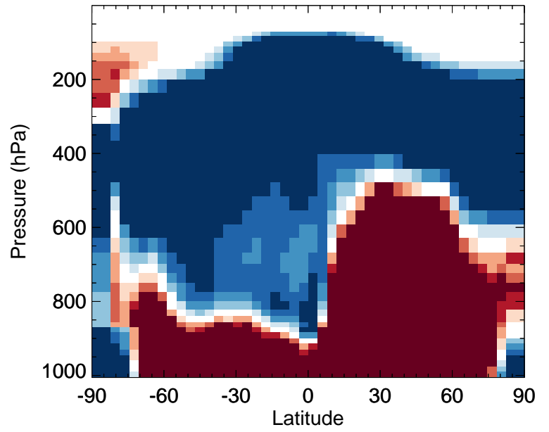
v11-02d / v11-02c Cl - Zonal mean % diff for Apr
