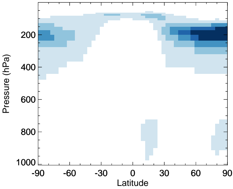
v11-02d - v11-02c HCl - Zonal mean abs diff for Apr
