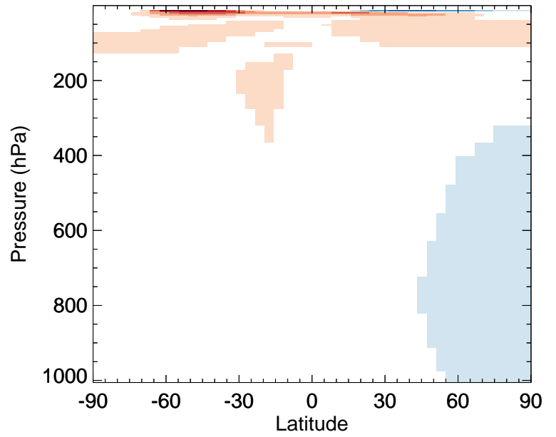
v11-02d / v11-02a CO - Zonal mean % diff for Apr
