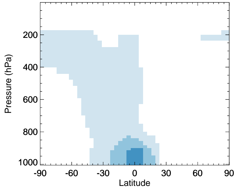
v11-02d / v11-02c O3 - Zonal mean % diff for Apr
