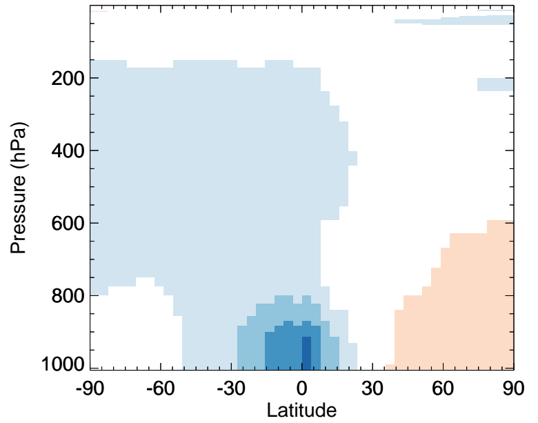
v11-02d / v11-02a O3 - Zonal mean % diff for Apr
