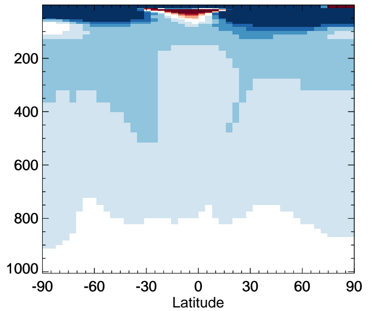
v11-02d / v11-02a CCI4 - Zonal mean % diff for Apr
