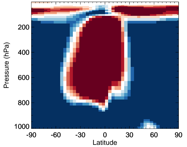
v11-02d / v11-02a HCl - Zonal mean % diff for Apr
