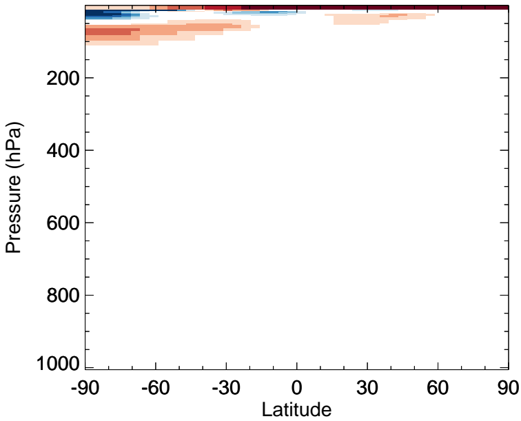
v11-02d - v11-02a NO - Zonal mean abs diff for Jan
