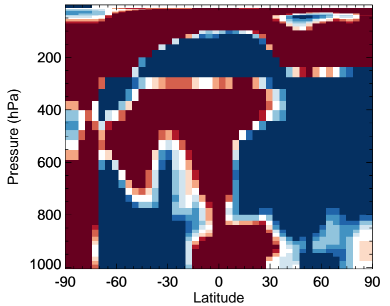
v11-02d / v11-02a Br2 - Zonal mean % diff for Jan
