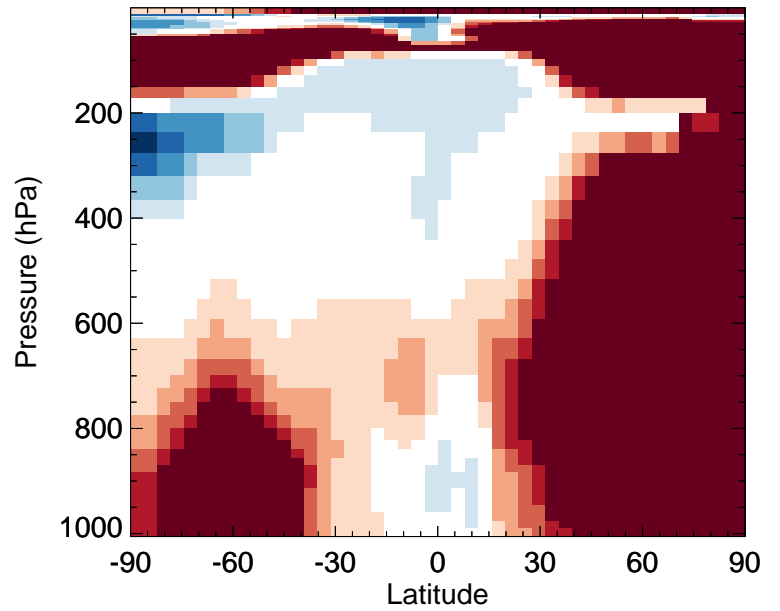
v11-02d / v11-02a NO - Zonal mean % diff for Jan
