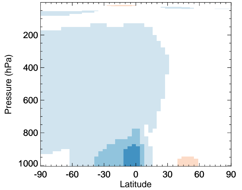
v11-02d / v11-02a O3 - Zonal mean % diff for Jan
