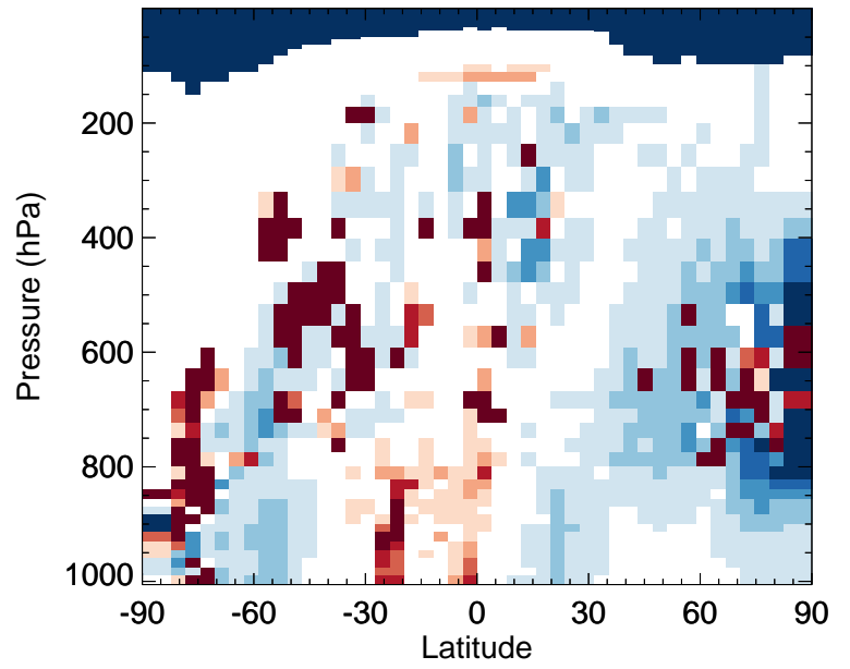
v11-02d / v11-02c NIT - Zonal mean % diff for Jan
