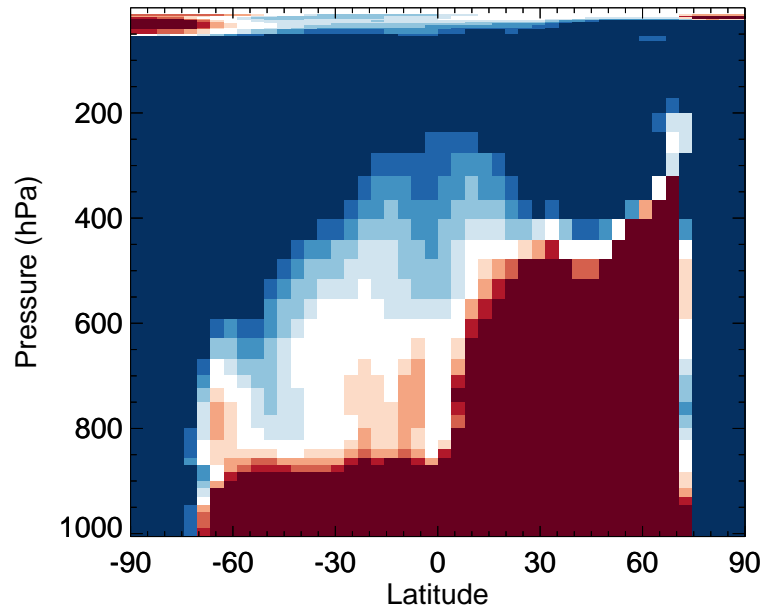
v11-02d / v11-02a ClO - Zonal mean % diff for Jan
