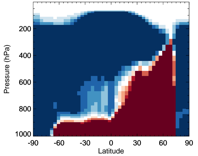
v11-02d / v11-02c ClO - Zonal mean % diff for Jan
