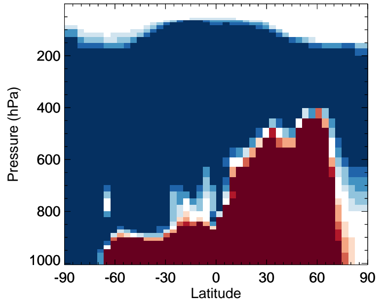
v11-02d / v11-02c Cl2 - Zonal mean % diff for Jan
