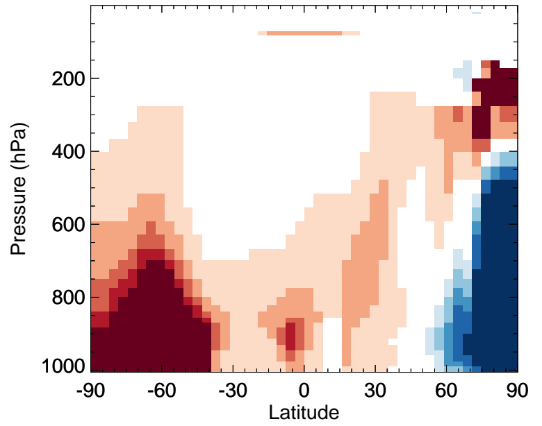
v11-02d / v11-02c NO - Zonal mean % diff for Jan
