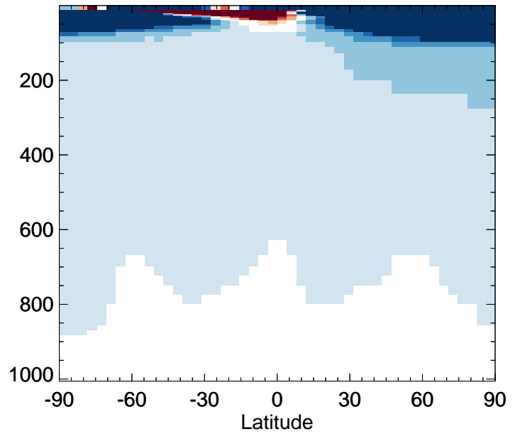
v11-02d / v11-02a CCI4 - Zonal mean % diff for Jan
