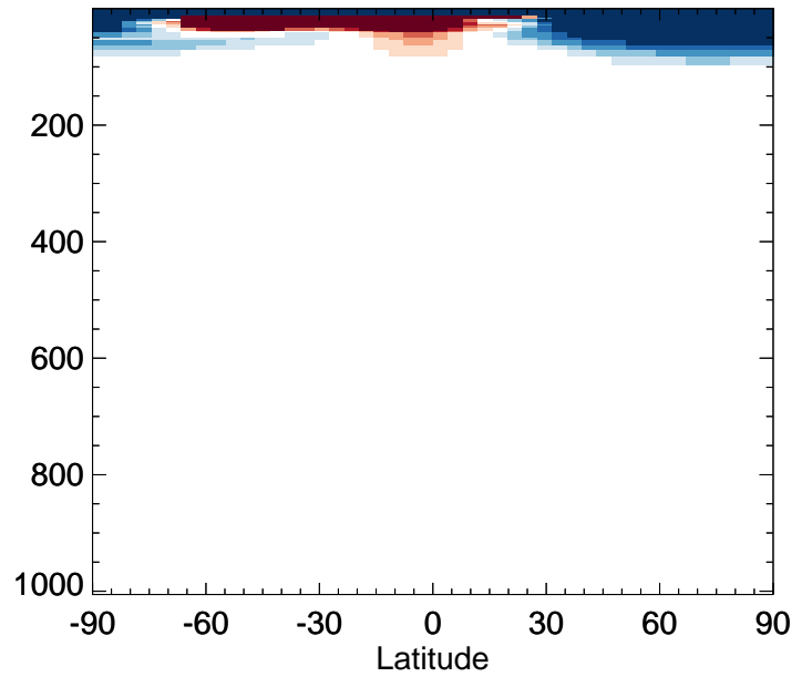
v11-02d / v11-02a OCS - Zonal mean % diff for Jan
