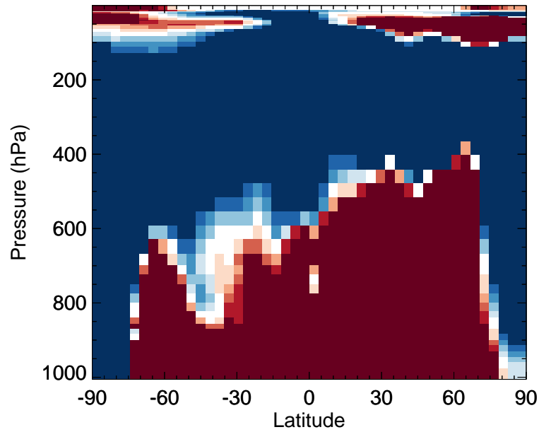
v11-02d / v11-02a Cl2 - Zonal mean % diff for Jan
