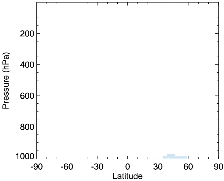
v11-02d - v11-02a NIT - Zonal mean abs diff for Jan
