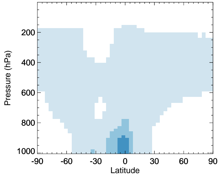
v11-02d / v11-02c O3 - Zonal mean % diff for Jan
