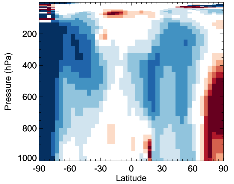
v11-02d / v11-02c ISN1 - Zonal mean % diff for Jan
