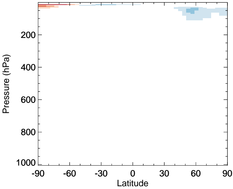
v11-02d - v11-02a ClO - Zonal mean abs diff for Jan
