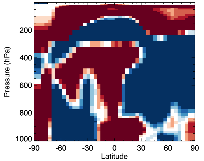
v11-02d / v11-02c Br2 - Zonal mean % diff for Jan
