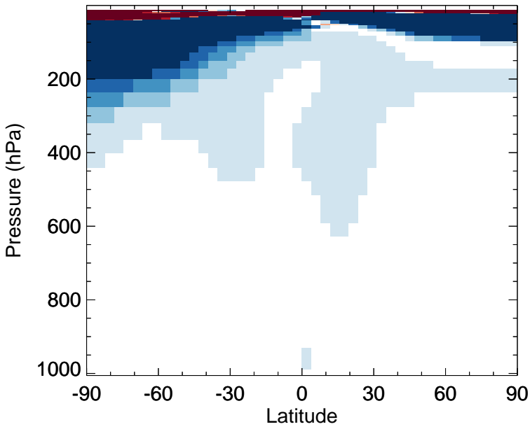
v11-02d - v11-02a O3 - Zonal mean abs diff for Jan
