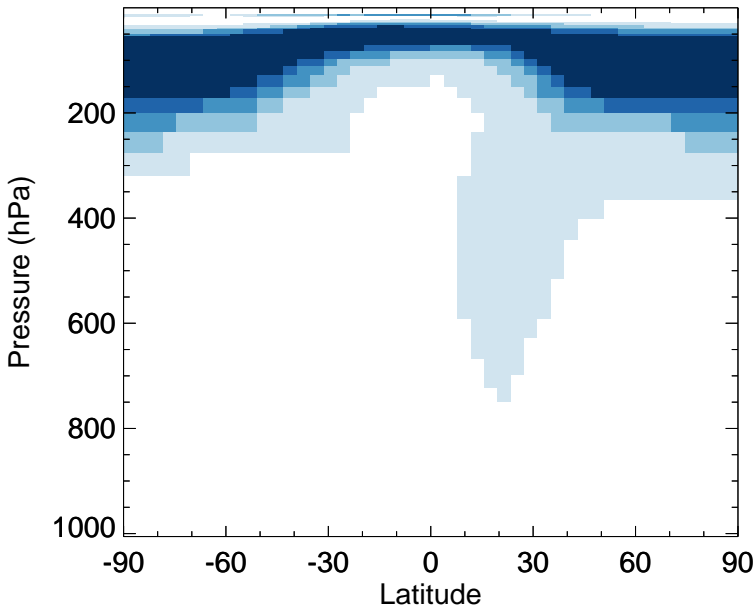
v11-02d - v11-02c O3 - Zonal mean abs diff for Jan
