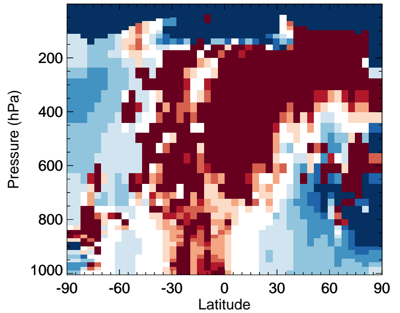
v11-02d / v11-02a NIT - Zonal mean % diff for Jan
