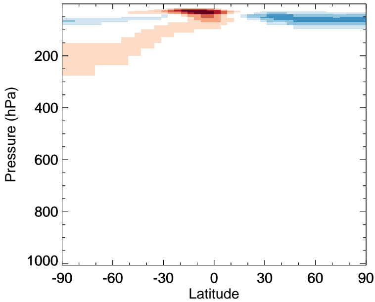
v11-02d - v11-02a OCS - Zonal mean abs diff for Jan
