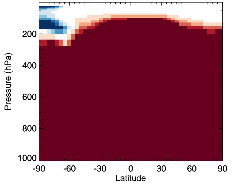
v11-02d / v11-02c BrCl - Zonal mean % diff for Jul
