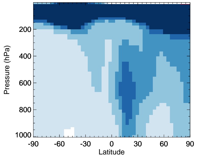
v11-02d / v11-02c C3H8 - Zonal mean % diff for Jul
