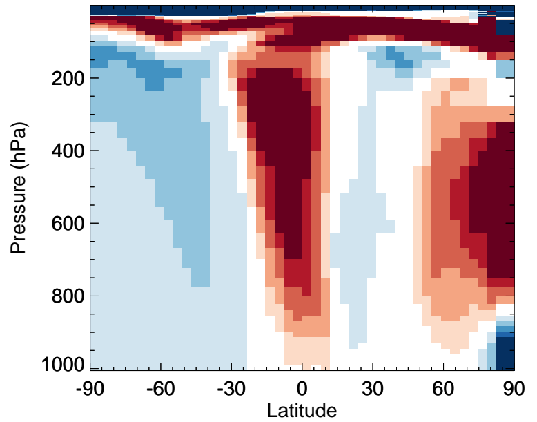
v11-02d / v11-02a XYLE - Zonal mean % diff for Jul
