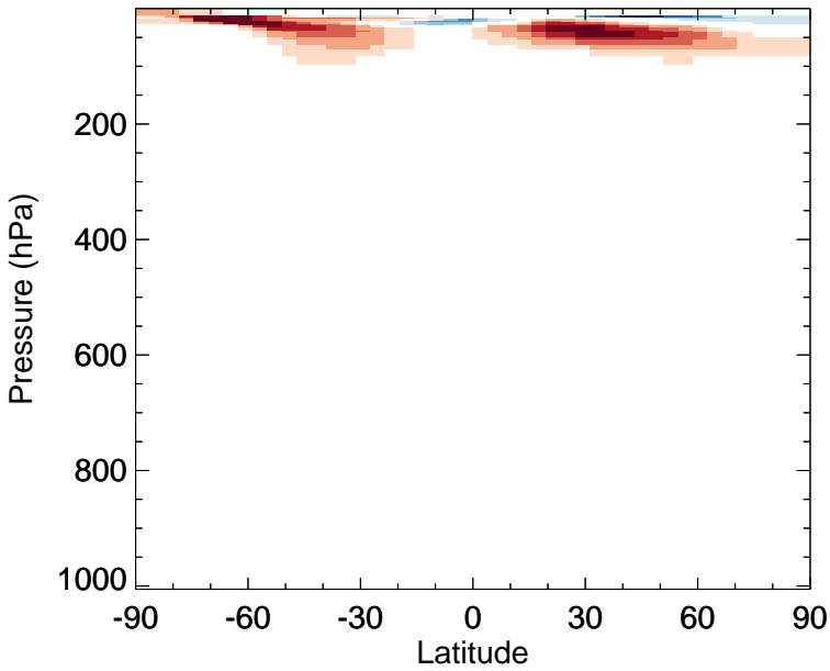
v11-02d - v11-02a NO 2 - Zonal mean abs diff for Jul
