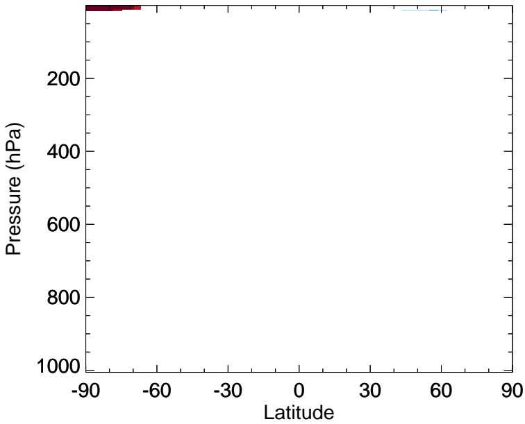
v11-02d - v11-02a NO 3 - Zonal mean abs diff for Jul
