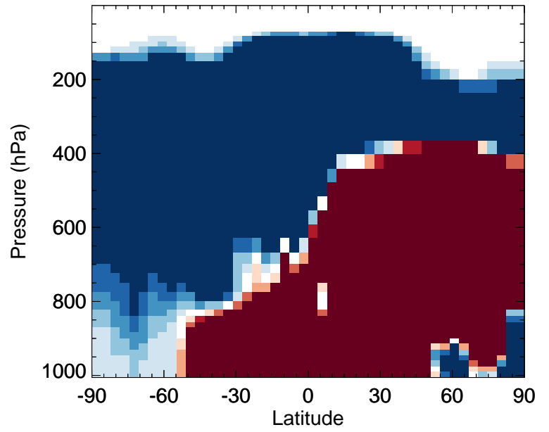
v11-02d / v11-02c Cl2 - Zonal mean % diff for Jul
