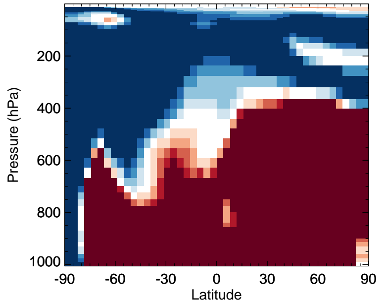
v11-02d / v11-02a ClO - Zonal mean % diff for Jul
