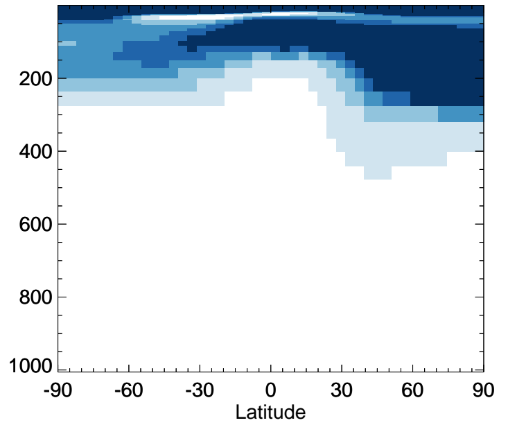
v11-02d / v11-02a SO4 - Zonal mean % diff for Jul
