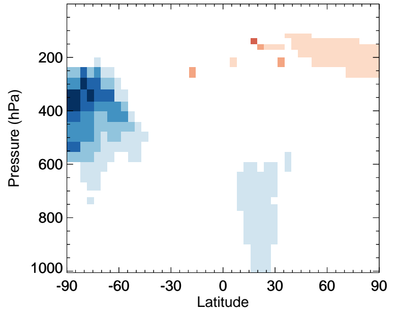
v11-02d / v11-02c NH3 - Zonal mean % diff for Jul
