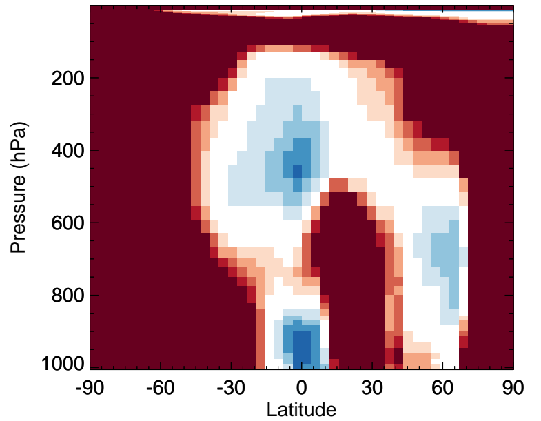
v11-02d / v11-02a N2O5 - Zonal mean % diff for Jul
