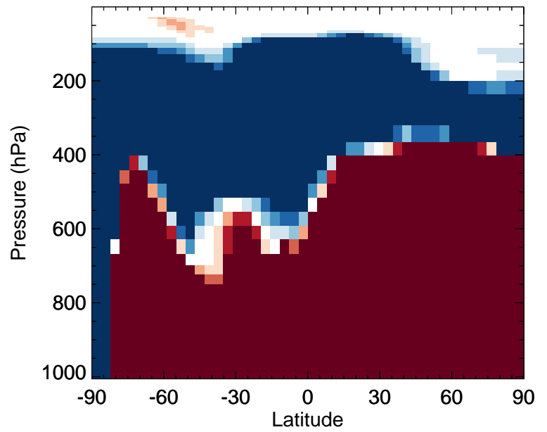
v11-02d / v11-02c Cl 2 O 2 - Zonal mean % diff for Jul
