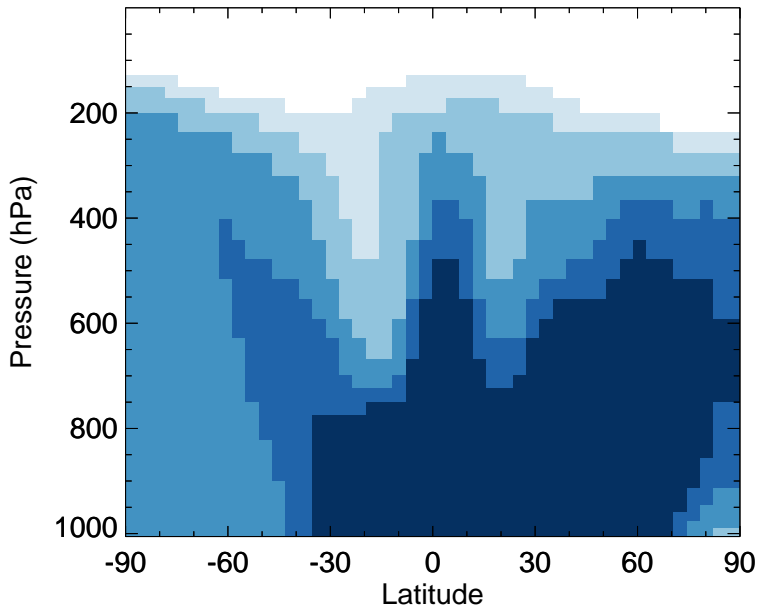
v11-02d - v11-02a R4N2 - Zonal mean abs diff for Jul
