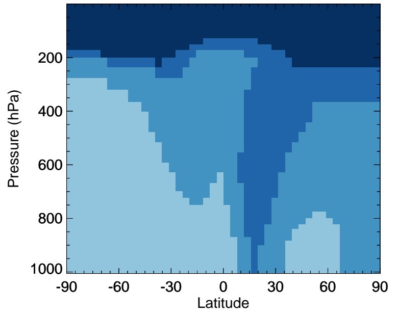
v11-02d / v11-02c C2H6 - Zonal mean % diff for Jul
