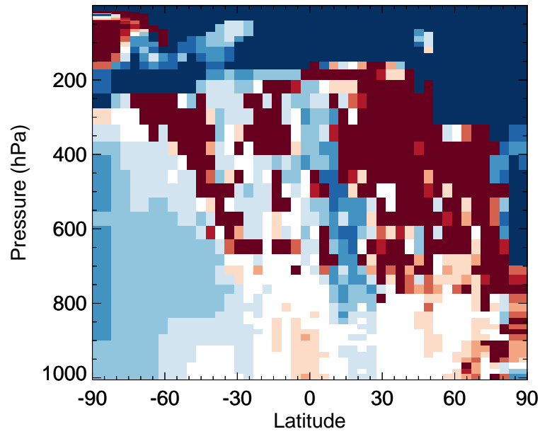
v11-02d / v11-02a NIT - Zonal mean % diff for Jul
