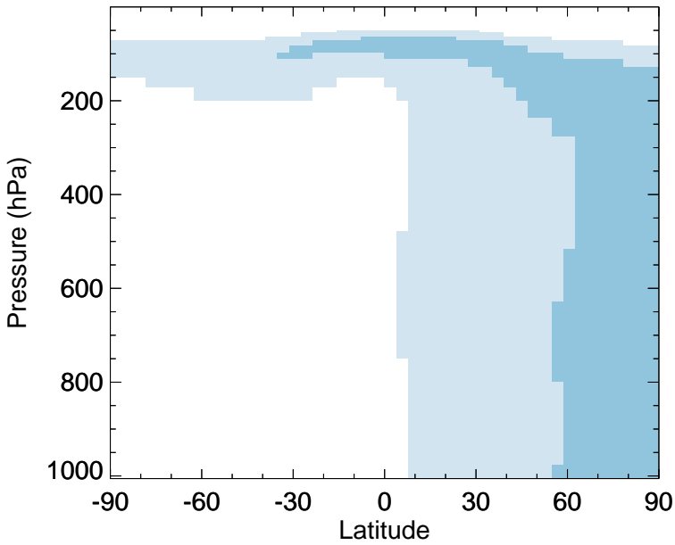
v11-02d - v11-02a C2H6 - Zonal mean abs diff for Jul
