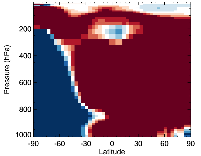
v11-02d / v11-02a BrO - Zonal mean % diff for Jul
