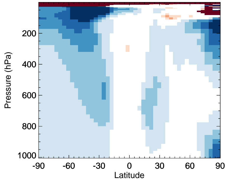
v11-02d / v11-02c XYLE - Zonal mean % diff for Jul
