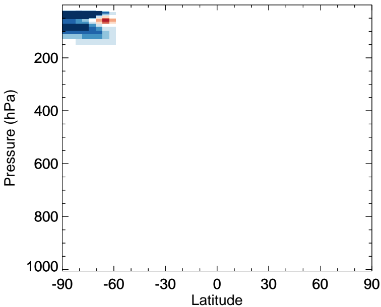
v11-02d - v11-02a Cl 2 O 2 - Zonal mean abs diff for Jul
