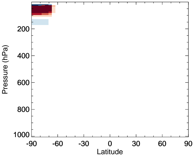
v11-02d - v11-02a Cl2 - Zonal mean abs diff for Jul
