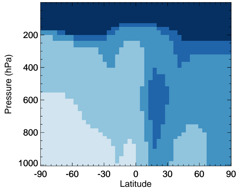
v11-02d / v11-02a C2H6 - Zonal mean % diff for Jul
