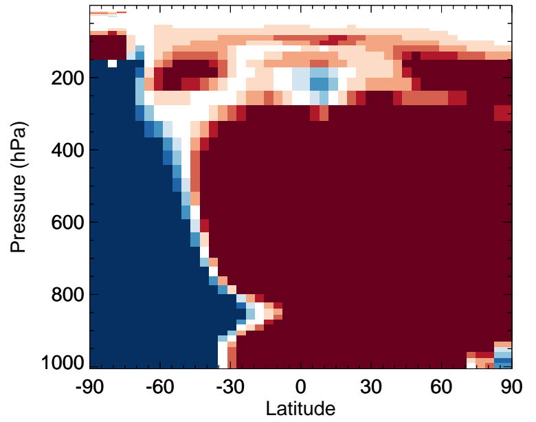
v11-02d / v11-02c Br - Zonal mean % diff for Jul
