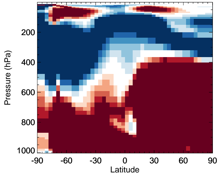
v11-02d / v11-02a Cl - Zonal mean % diff for Jul
