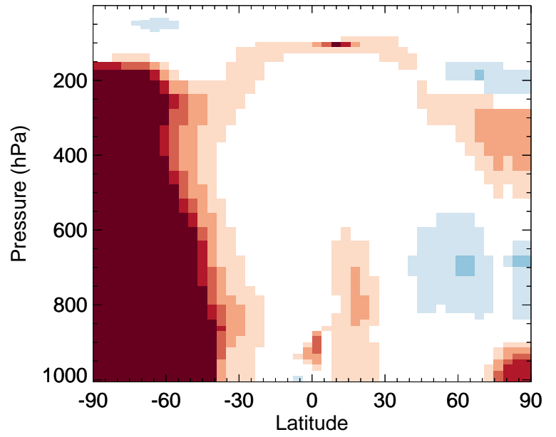
v11-02d / v11-02c NO 2 - Zonal mean % diff for Jul
