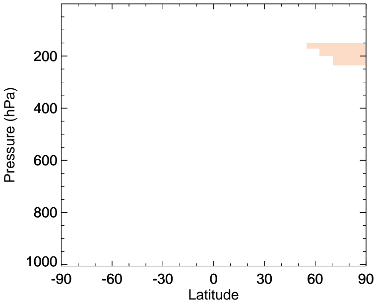
v11-02d - v11-02a BrO - Zonal mean abs diff for Jul
