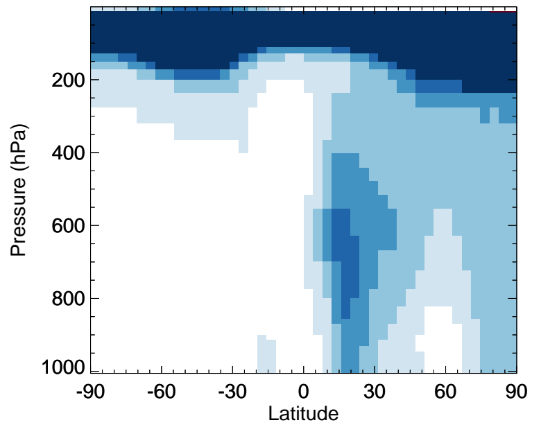
v11-02d / v11-02a C3H8 - Zonal mean % diff for Jul
