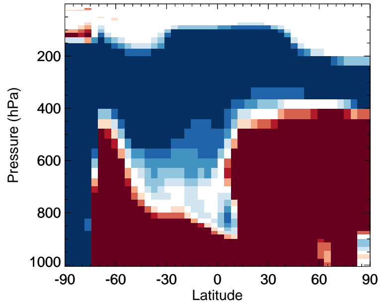
v11-02d / v11-02c Cl - Zonal mean % diff for Jul
