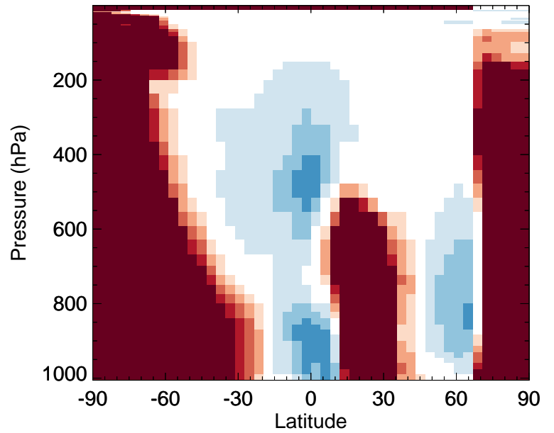
v11-02d / v11-02a NO 3 - Zonal mean % diff for Jul
