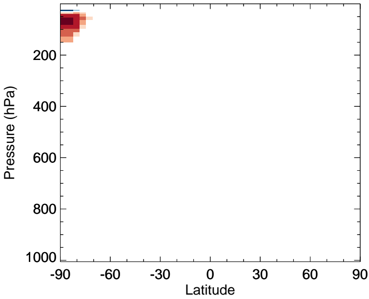
v11-02d - v11-02a NIT - Zonal mean abs diff for Jul
