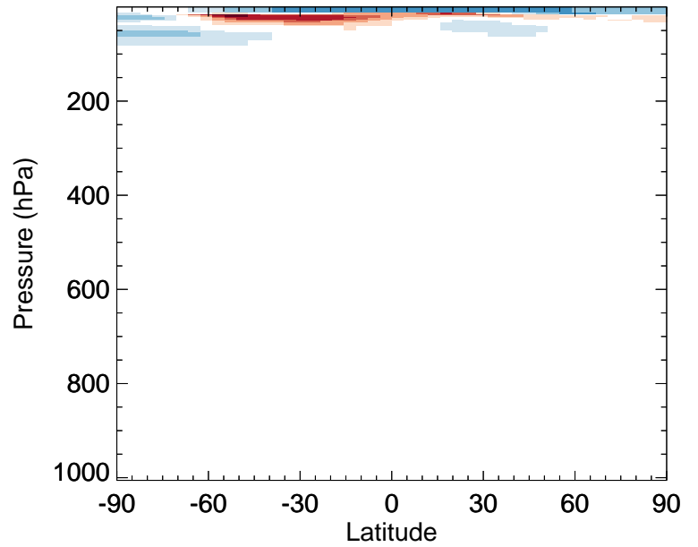
v11-02d / v11-02a CH4 - Zonal mean % diff for Jul
