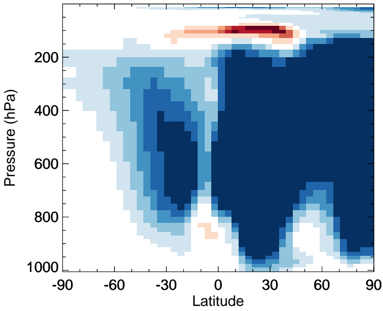
v11-02d - v11-02c CH4 - Zonal mean abs diff for Jul
