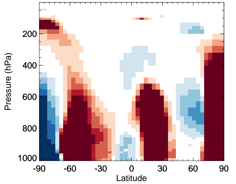
v11-02d / v11-02c N2O5 - Zonal mean % diff for Jul
