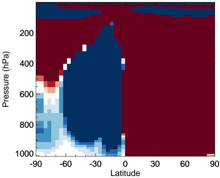
v11-02d - v11-02a CH4 - Zonal mean abs diff for Jul
