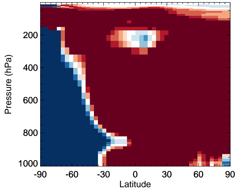
v11-02d / v11-02a Br - Zonal mean % diff for Jul
