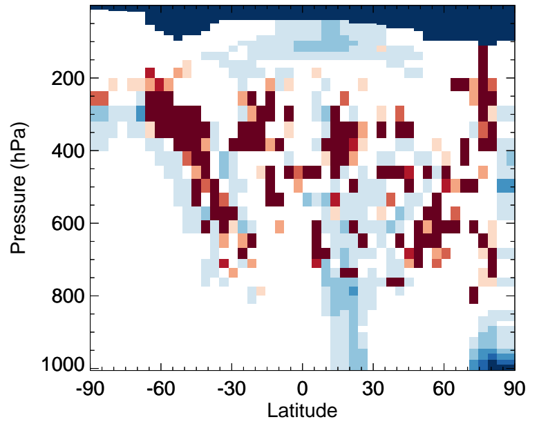
v11-02d / v11-02c NIT - Zonal mean % diff for Jul
