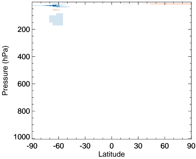
v11-02d - v11-02a ClO - Zonal mean abs diff for Jul
