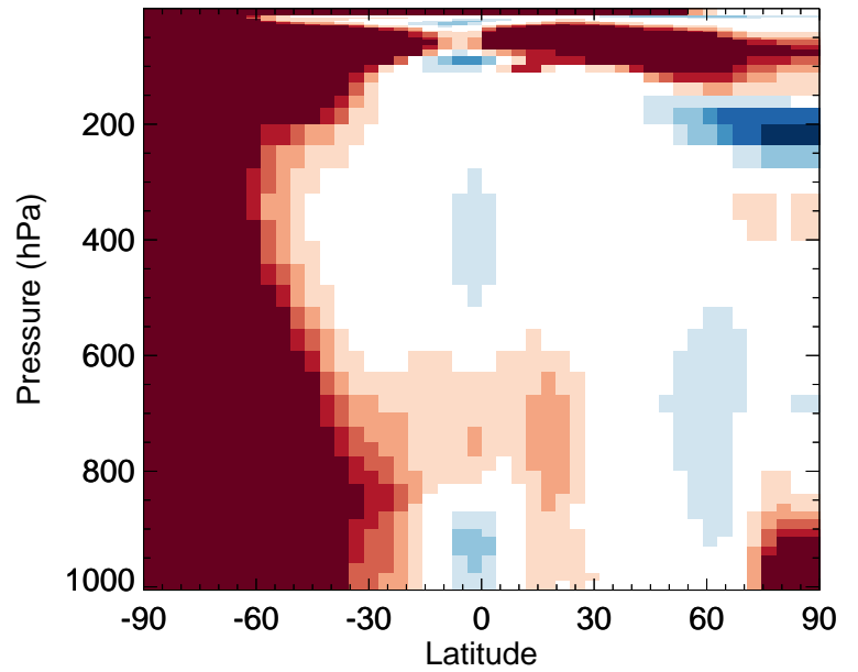
v11-02d / v11-02a NO 2 - Zonal mean % diff for Jul
