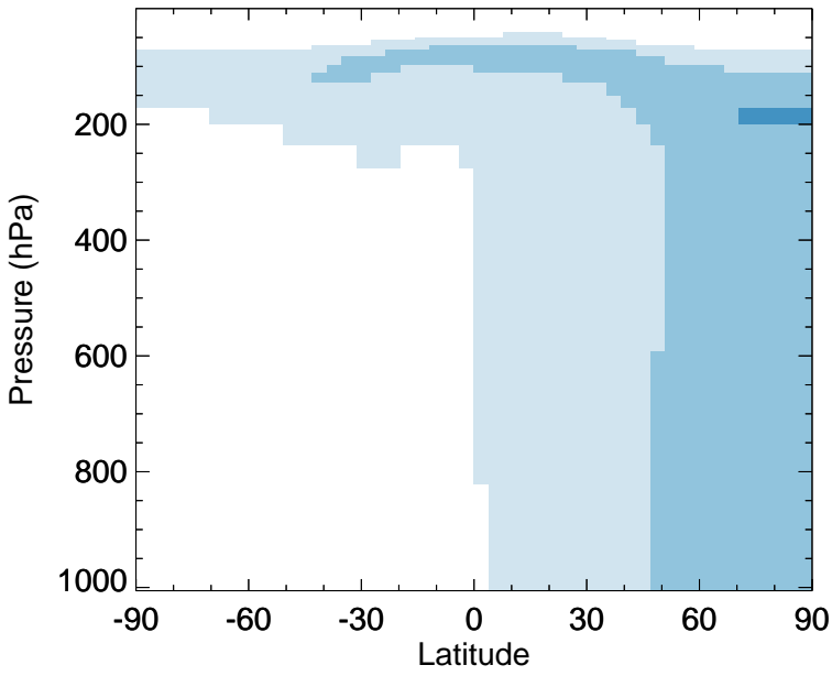
v11-02d - v11-02c C2H6 - Zonal mean abs diff for Jul
