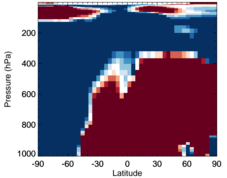
v11-02d / v11-02a Cl2 - Zonal mean % diff for Jul
