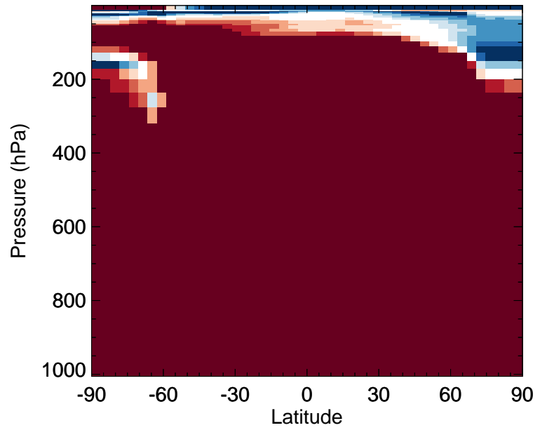
v11-02d / v11-02a BrCl - Zonal mean % diff for Jul
