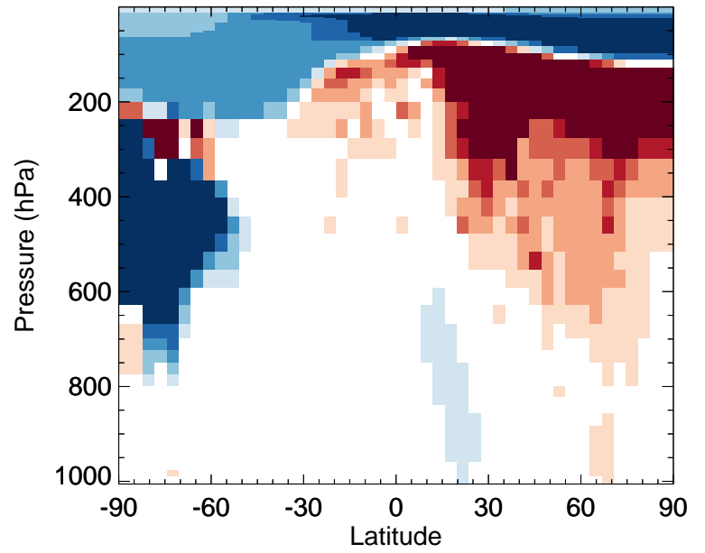
v11-02d / v11-02a NH3 - Zonal mean % diff for Jul
