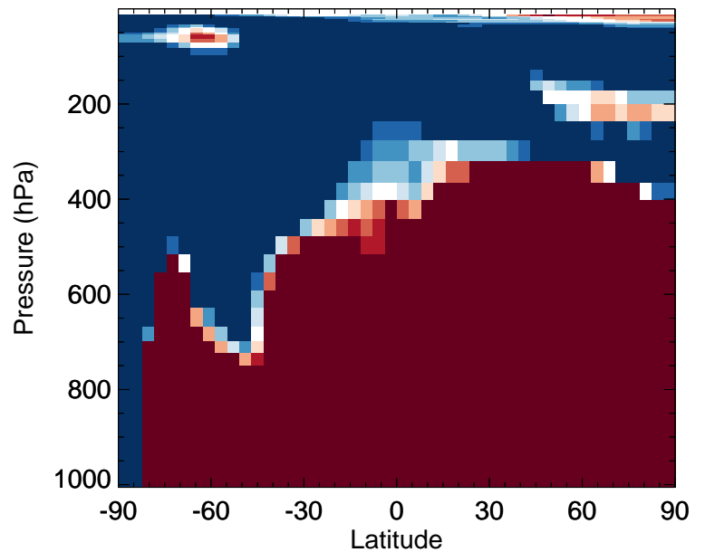
v11-02d / v11-02a Cl 2 O 2 - Zonal mean % diff for Jul
