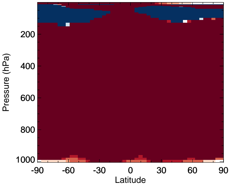
v11-02d - v11-02a N2O - Zonal mean abs diff for Jul
