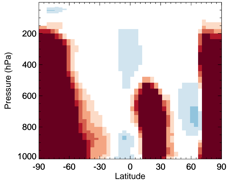
v11-02d / v11-02c NO 3 - Zonal mean % diff for Jul
