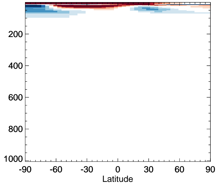
v11-02d / v11-02a N2O - Zonal mean % diff for Jul
