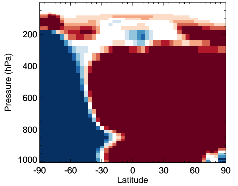
v11-02d / v11-02c BrO - Zonal mean % diff for Jul
