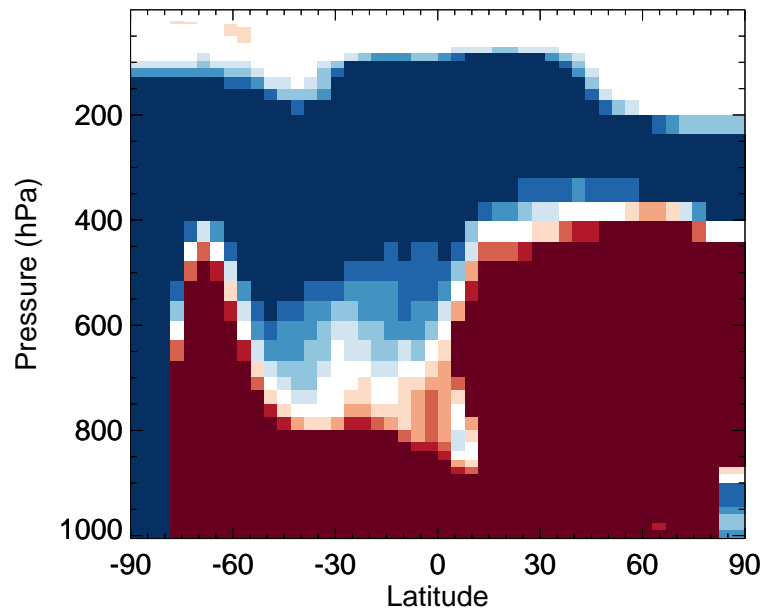
v11-02d / v11-02c ClO - Zonal mean % diff for Jul
