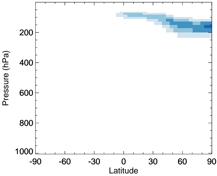
v11-02d - v11-02a SO4 - Zonal mean abs diff for Jul
