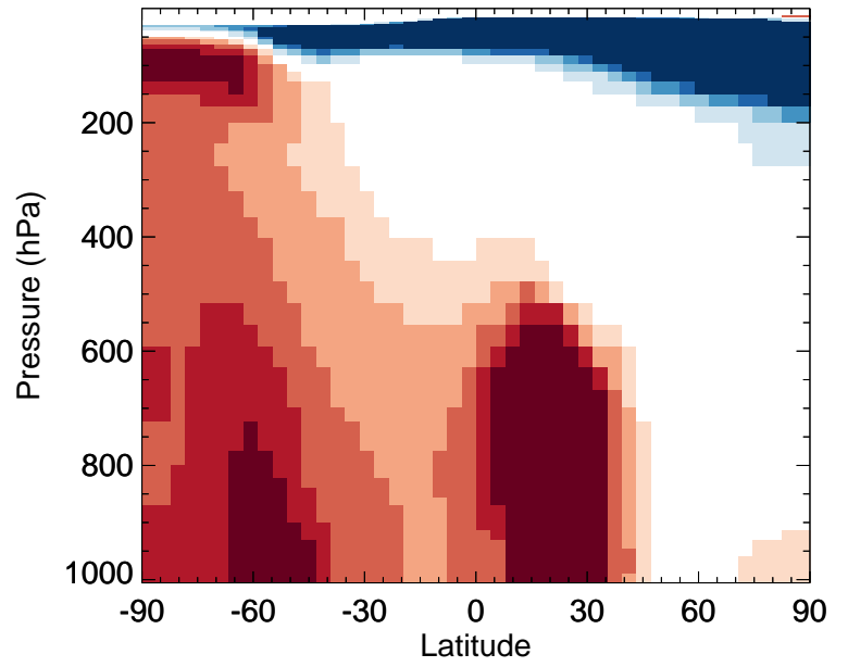
v11-02d / v11-02c R4N2 - Zonal mean % diff for Jul
