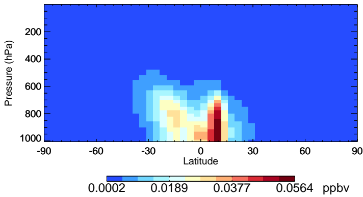
v11-02d SOAIE - Species Zonal Mean for Oct
