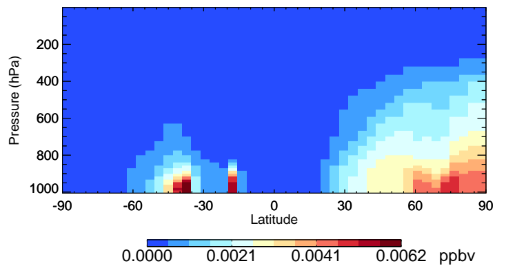
v11-02d RCHO - Species Curtain @ -180.000 for Oct
