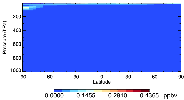
v11-02d CIO - Species Zonal Mean for Oct
