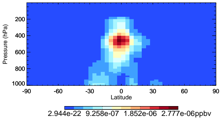
v11-02d ISN1OG - Species Zonal Mean for Oct
