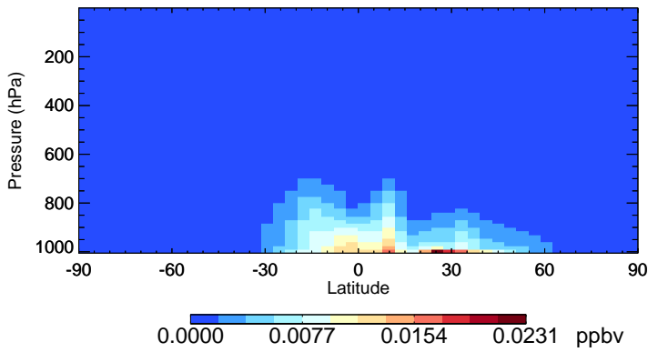
v11-02d GLYX - Species Zonal Mean for Oct
