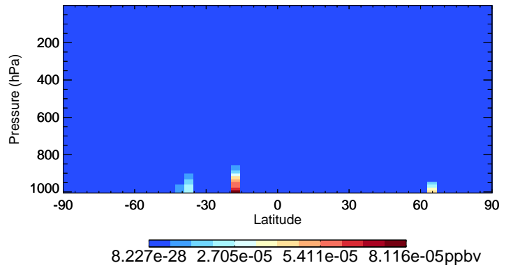
v11-02a LIMO - Species Curtain @ -180.000 for Oct
