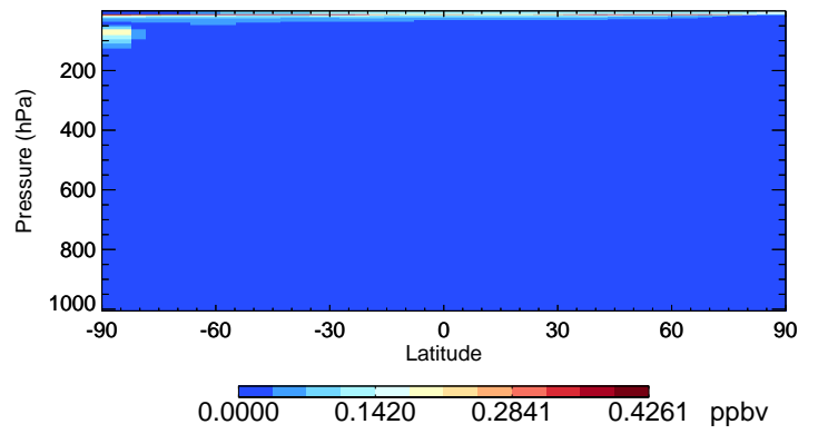
v11-02c CIO - Species Curtain @ -180.000 for Oct
