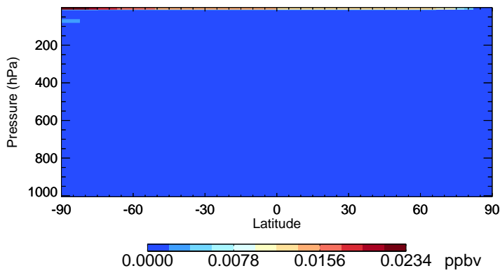
v11-02d Br - Species Zonal Mean for Oct
