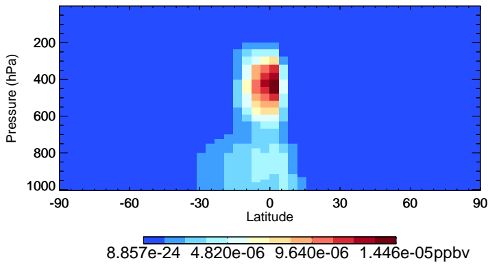
v11-02d LVOC - Species Zonal Mean for Oct
