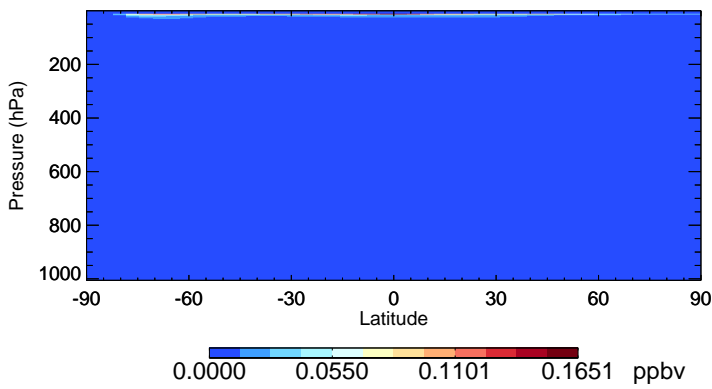
v11-02d NO3 - Species Zonal Mean for Oct
