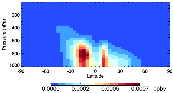
v11-02d ISN10A - Species Zonal Mean for Oct
