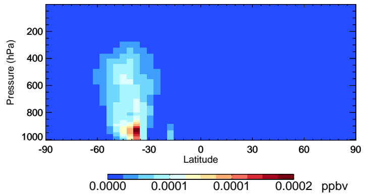
v11-02d IEPOXD - Species Curtain @ -180.000 for Oct
