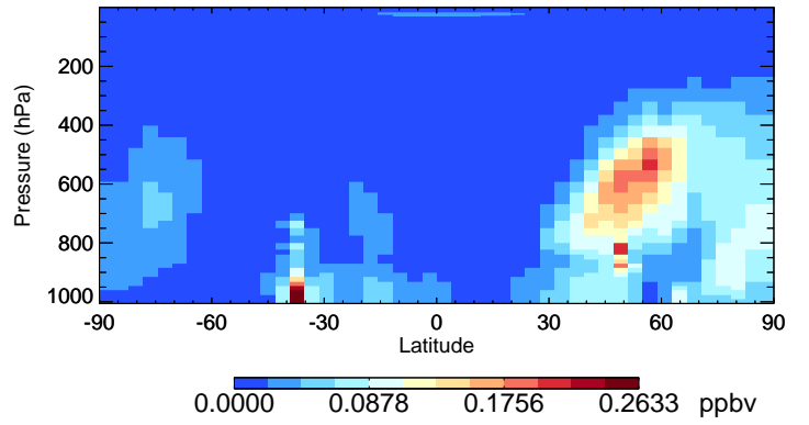
v11-02c SO2 - Species Curtain @ -180.000 for Oct
