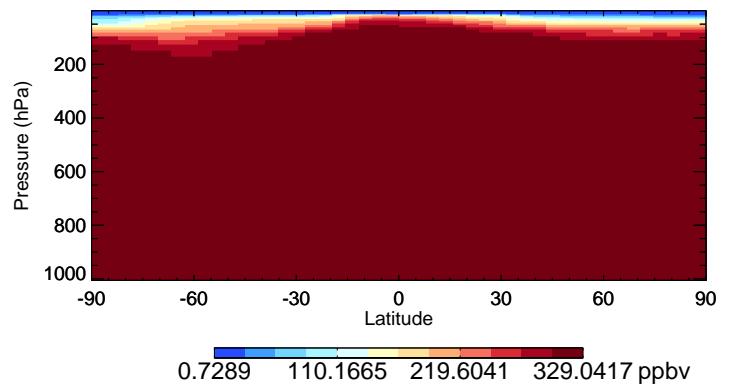
v11-02d N2O - Species Curtain @ -180.000 for Oct
