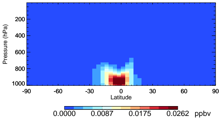
v11-02d RIPB - Species Zonal Mean for Oct
