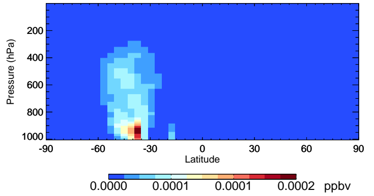
v11-02c IEPOXD - Species Curtain @ -180.000 for Oct
