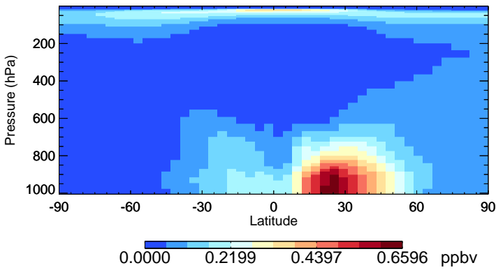
v11-02d SO4 - Species Zonal Mean for Oct
