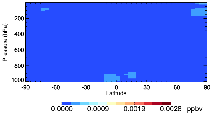
v11-02d Br2 - Species Zonal Mean for Oct
