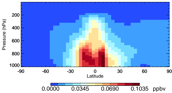
v11-02d MAP - Species Zonal Mean for Oct
