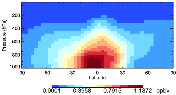
v11-02d MP - Species Zonal Mean for Oct
