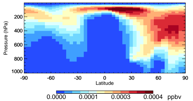
ASOA1 - Species Curtain @ -180.000 for Oct
