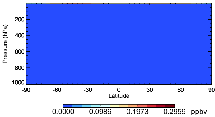
v11-02d CI - Species Zonal Mean for Oct
