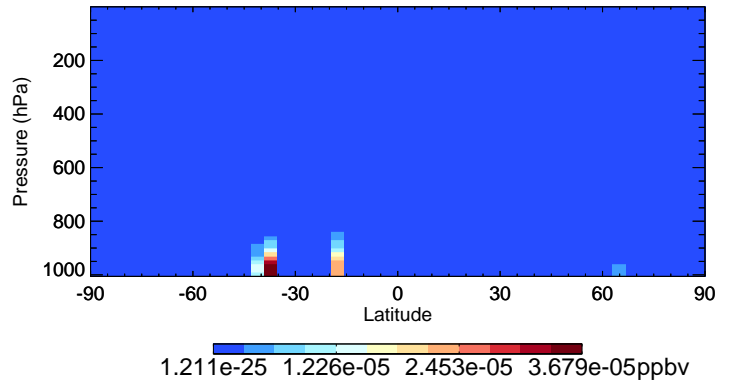
v11-02c MONITU - Species Curtain @ -180.000 for Oct
