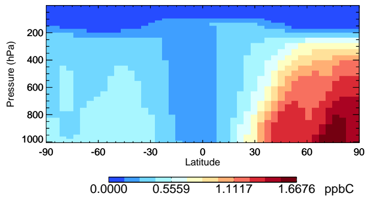
v11-02d C2H6 - Species Curtain @ -180.000 for Oct
