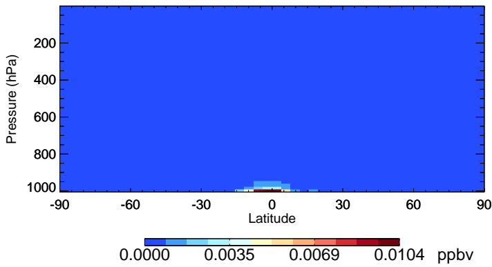
v11-02d LIMO - Species Zonal Mean for Oct
