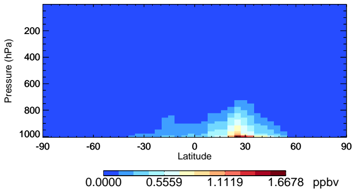
v11-02d NH3 - Species Zonal Mean for Oct
