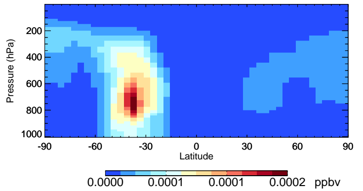
v11-02d ISN10A - Species Curtain @ -180.000 for Oct
