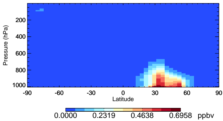
v11-02d NIT - Species Zonal Mean for Oct
