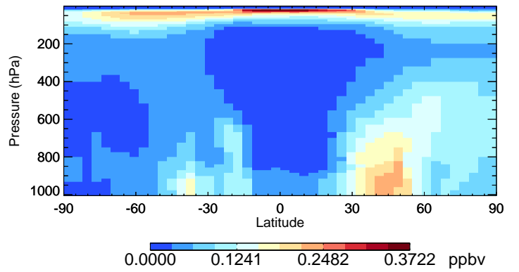
v11-02d SO4 - Species Curtain @ -180.000 for Oct
