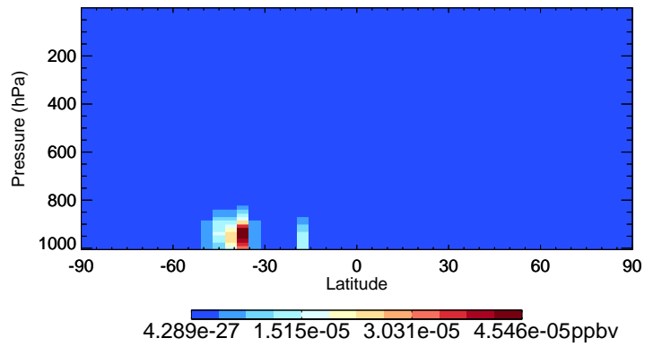
v11-02d RIPD - Species Curtain @ -180.000 for Oct
