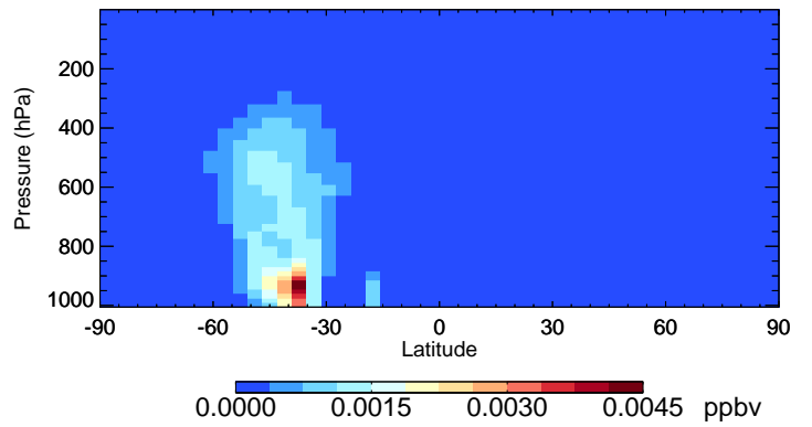
v11-02d IEPOXA - Species Curtain @ -180.000 for Oct
