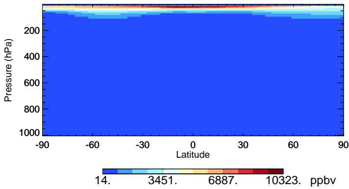
v11-02d O3 - Species Zonal Mean for Oct
