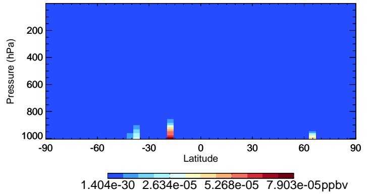
v11-02c LIMO - Species Curtain @ -180.000 for Oct
