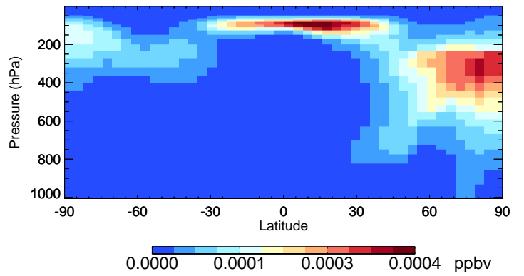
v11-02d ASOA2 - Species Curtain @ -180.000 for Oct
