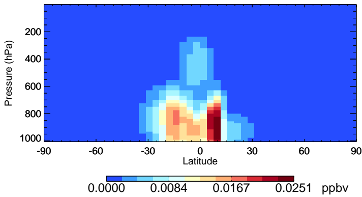
v11-02d HC187 - Species Zonal Mean for Oct
