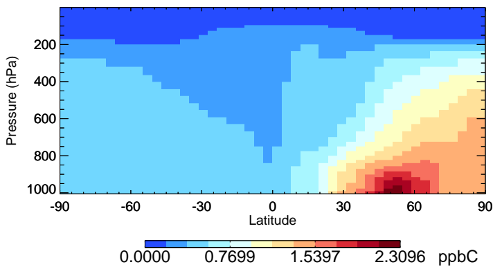
v11-02d C2H6 - Species Zonal Mean for Oct
