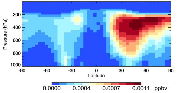
v11-02c R4N2 - Species Curtain @ -180.000 for Oct
