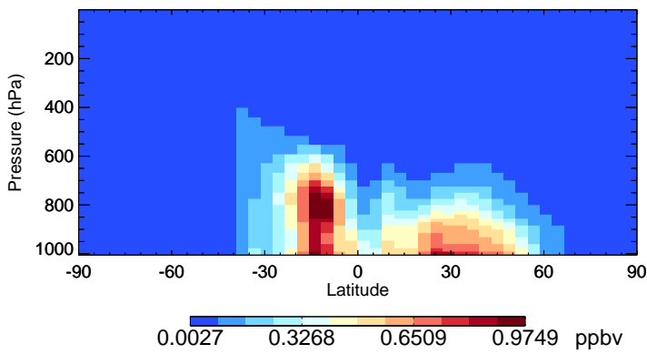
v11-02d OCPI - Species Zonal Mean for Oct
