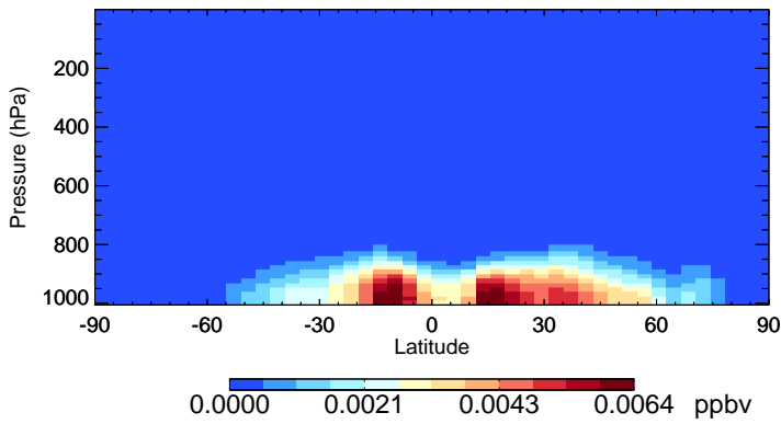
v11-02d NITs - Species Zonal Mean for Oct
