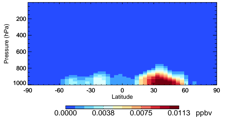
v11-02a NITs - Species Curtain @ -180.000 for Oct
