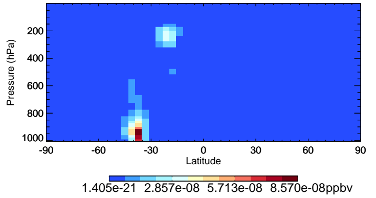
v11-02c ISN1OG - Species Curtain @ -180.000 for Oct
