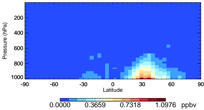
v11-02d SO2 - Species Zonal Mean for Oct
