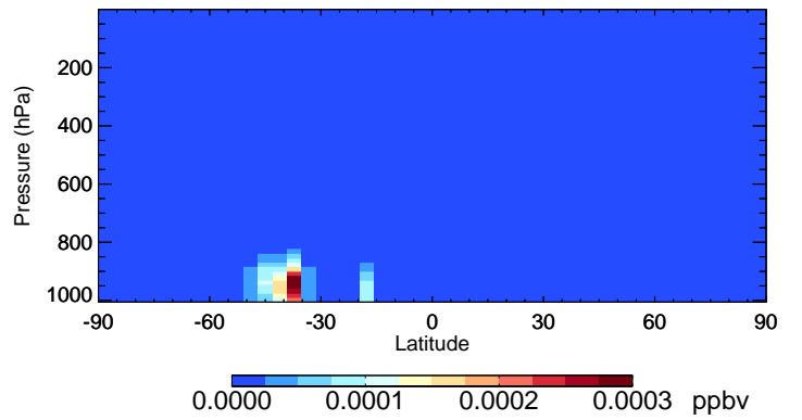
v11-02d RIPB - Species Curtain @ -180.000 for Oct
