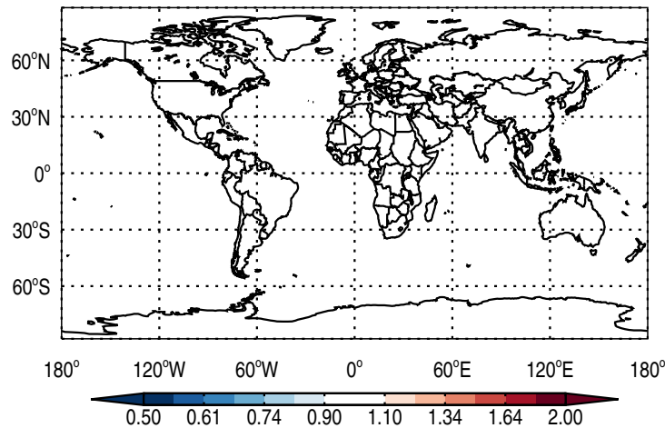
Ratio @ 500 hPa for Pb
