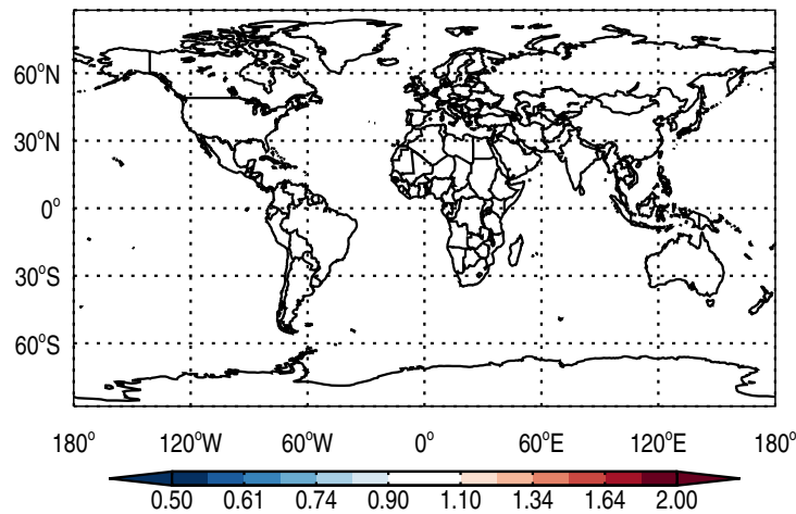
Ratio @ 500 hPa for Rn
