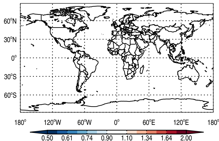
Ratio @ 500 hPa for Be7
