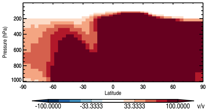
Zonal mean abs diff: Rn
