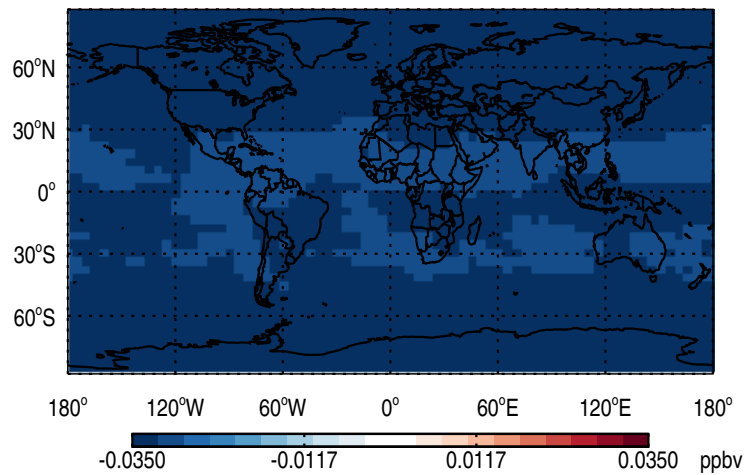
Abs Diff @ 500 hPa - PASV
