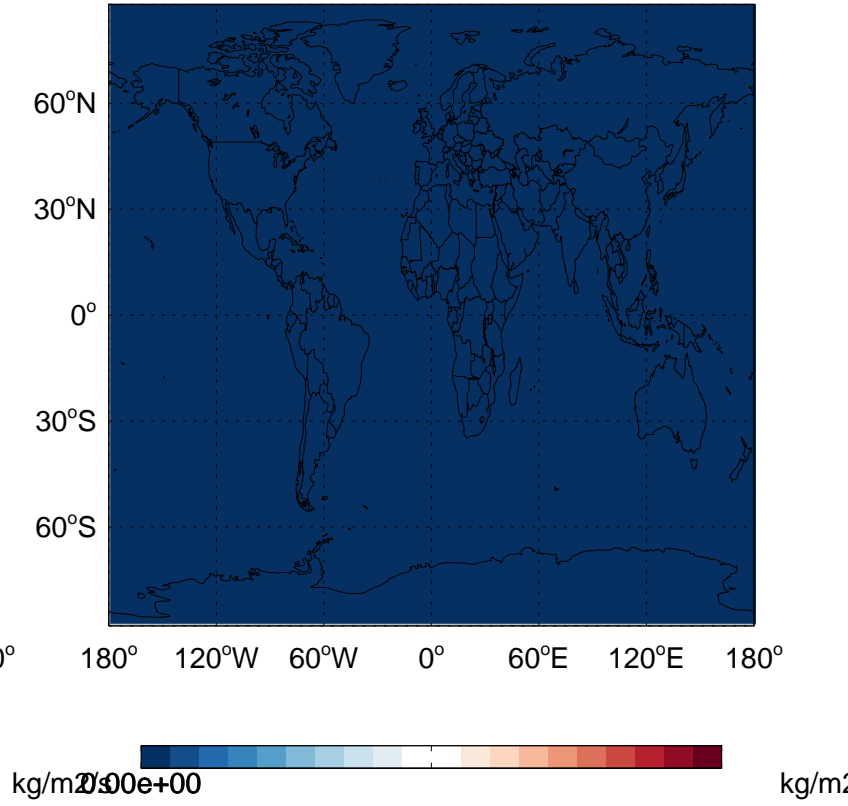
v11-02e-Run0 - v11-02d-Run1 CH 2 Br 2 biogenic emissions for Apr
