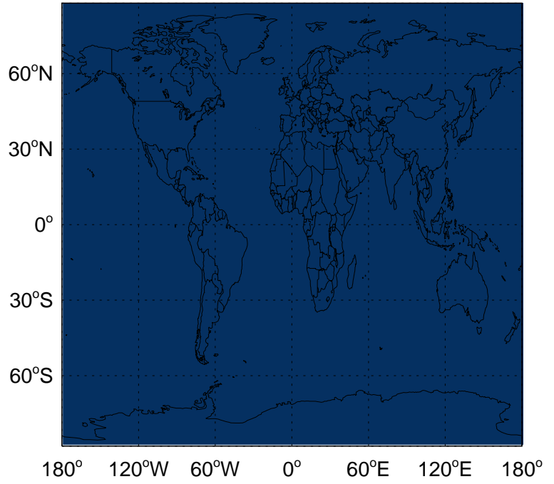
v11-02e-Run0 - v11-02d-Run1 CHBr3 biogenic emissions for Jul
