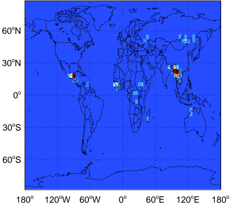
ALK4 biomass emissions for Apr
