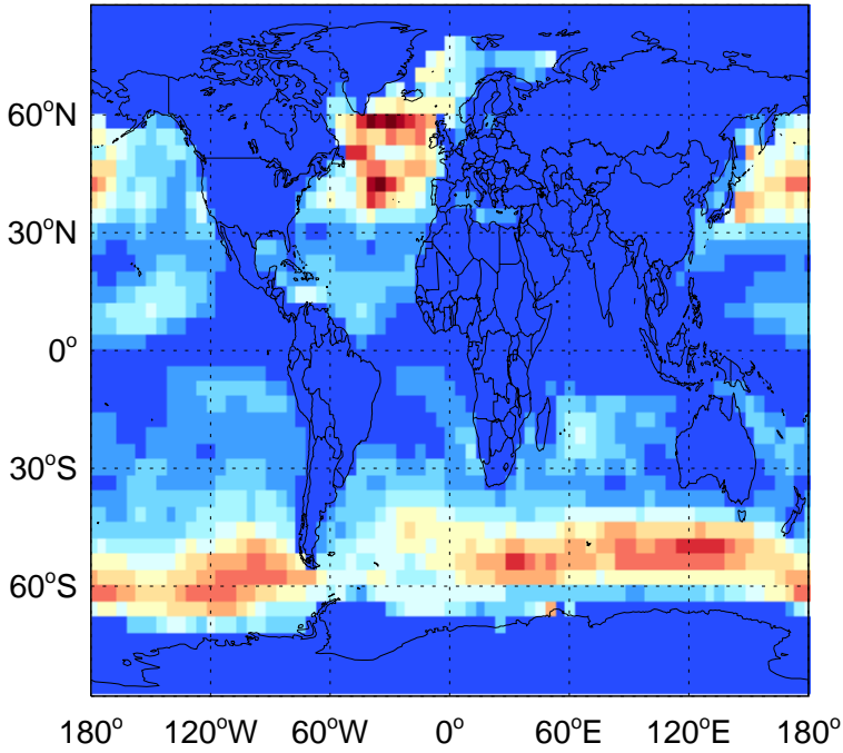
Br2 biogenic emissions for Apr
