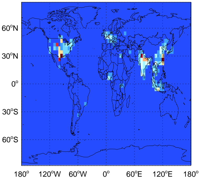
CH 2 O column anth+biof emissions for Oct
