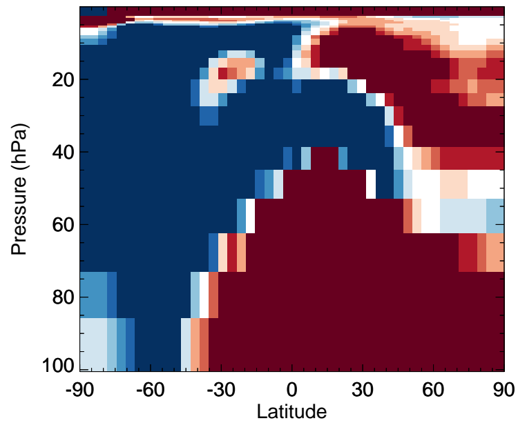
OCIO - Strat zonal mean % diff for Jul
