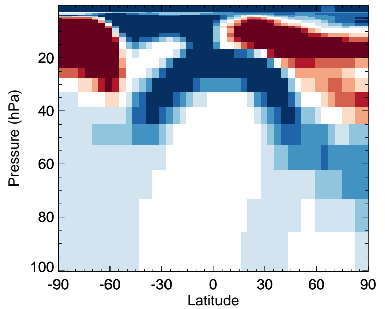
MP - Strat zonal mean % diff for Jul
