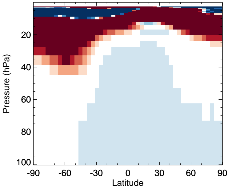
O3 - Strat zonal mean abs diff for Jul
