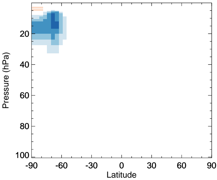
OCIO - Strat zonal mean abs diff for Jul
