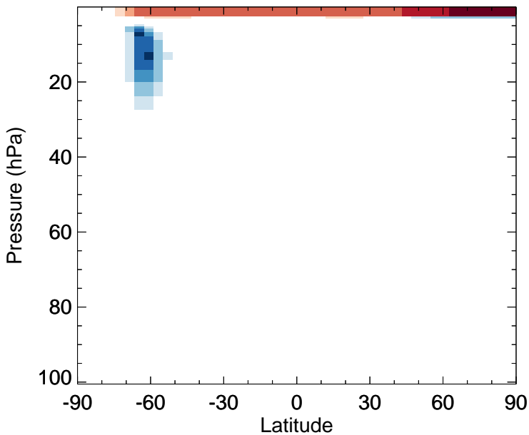
v11-02e-Run0 - v11-02c-Run0 ClO - Strat zonal mean abs diff for Jul
