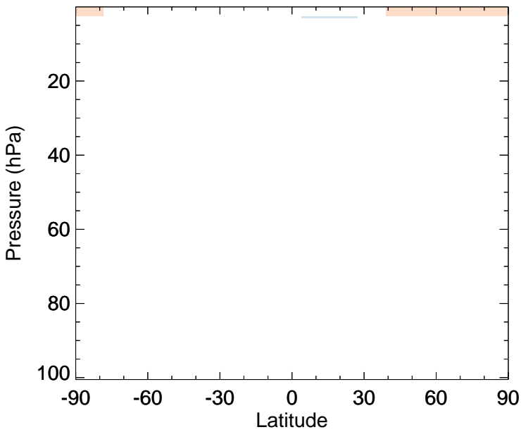
v11-02e-Run0 - v11-02c-Run0 CO - Strat zonal mean abs diff for Jul
