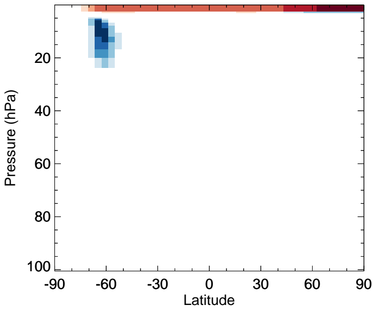
v11-02e-Run0 - v11-02d-Run1 ClO - Strat zonal mean abs diff for Jul
