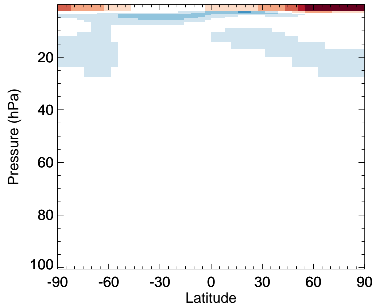
v11-02e-Run0 / v11-02c-Run0 CO - Strat zonal mean % diff for Jul
