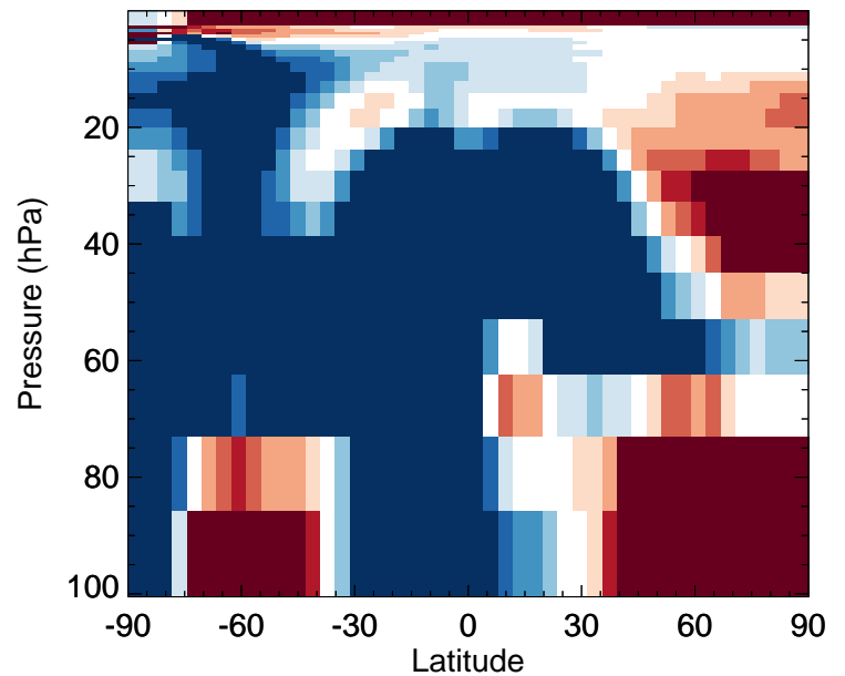
v11-02e-Run0 / v11-02c-Run0 ClO - Strat zonal mean % diff for Jul
