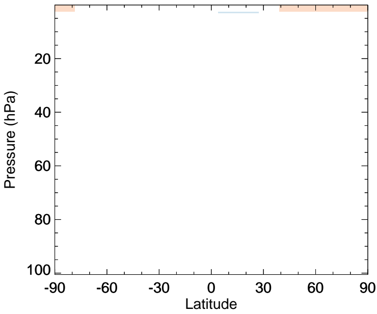
v11-02e-Run0 - v11-02d-Run1 CO - Strat zonal mean abs diff for Jul
