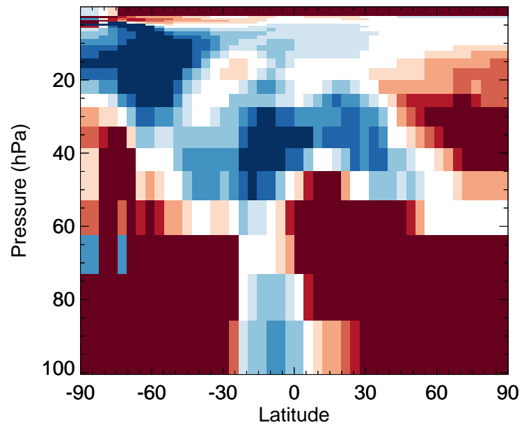
v11-02e-Run0 / v11-02d-Run1 ClO - Strat zonal mean % diff for Jul
