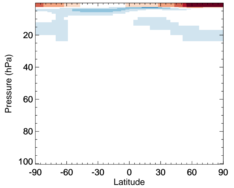
v11-02e-Run0 / v11-02d-Run1 CO - Strat zonal mean % diff for Jul
