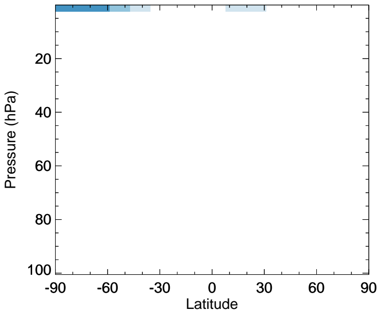
MP - Strat zonal mean abs diff for Jul
