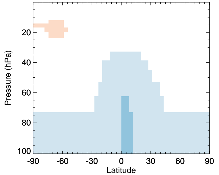
O3 - Strat zonal mean % diff for Jul
