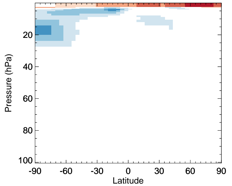
CO - Strat zonal mean % diff for Oct
