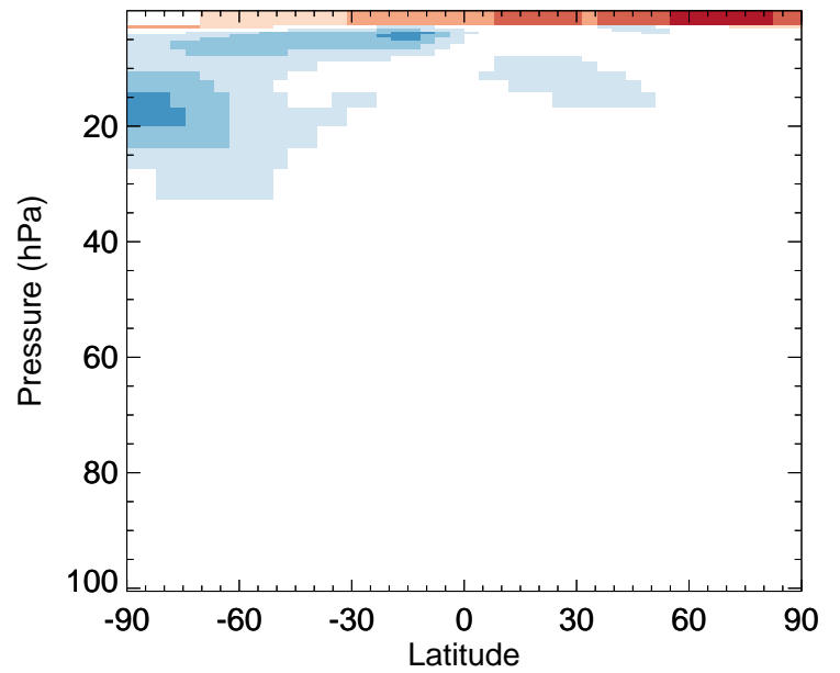
CO - Strat zonal mean % diff for Oct
