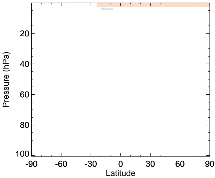
CO - Strat zonal mean abs diff for Oct
