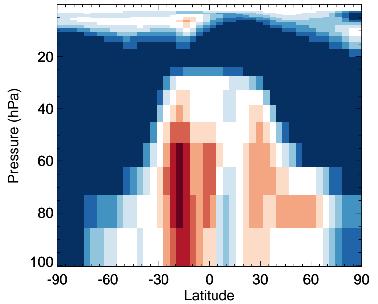
BrNO3 - Strat zonal mean % diff for Oct
