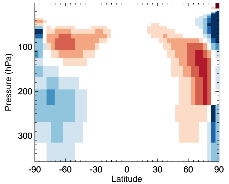
OH - Strat zonal mean % diff for Oct
