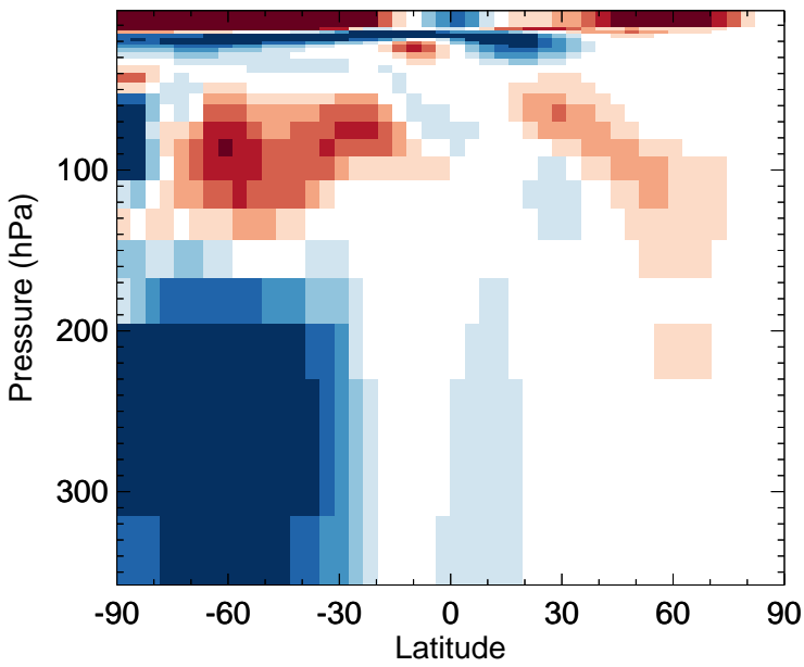
OH - Strat zonal mean abs diff for Oct
