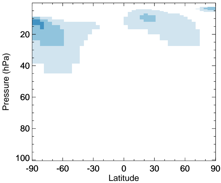
BrNO3 - Strat zonal mean abs diff for Oct
