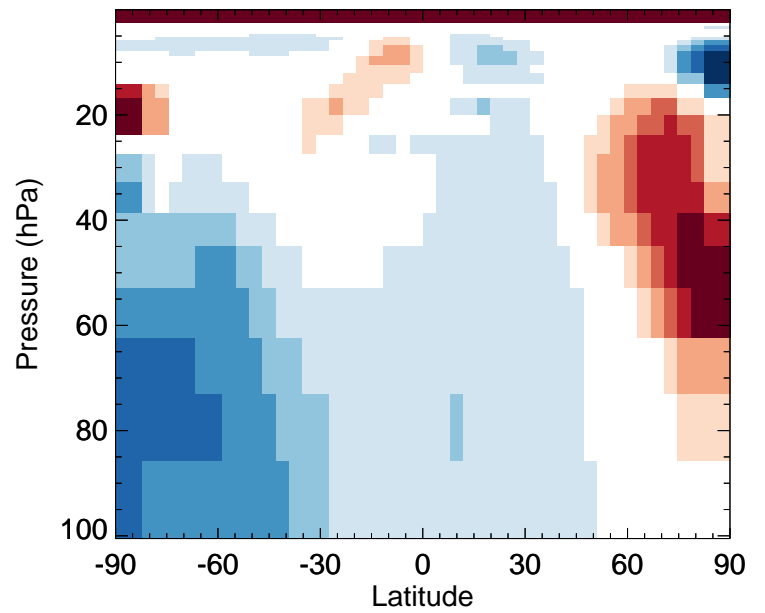
HNO 4 - Strat zonal mean % diff for Oct
