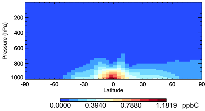
v11-02c-Run0 ALD2 - Species Zonal Mean for Oct
