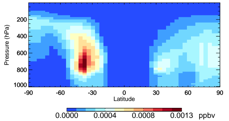
v11-02e-Run0 SOAME - Species Curtain @ -180.000 for Oct
