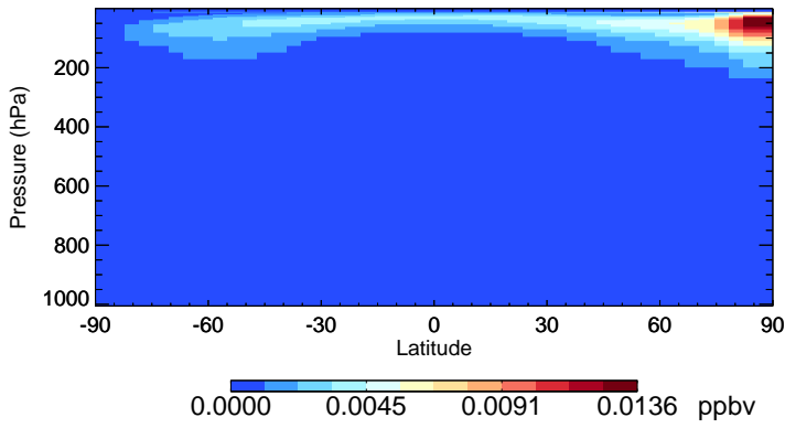
v11-02c-Run0 BrCl - Species Zonal Mean for Oct
