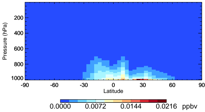
v11-02c-Run0 GLYX - Species Zonal Mean for Oct
