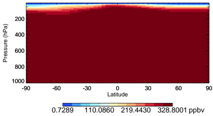
v11-02c-Run0 N2O - Species Zonal Mean for Oct
