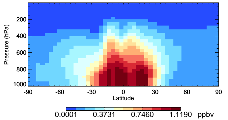
v11-02e-Run0 MP - Species Curtain @ -180.000 for Oct
