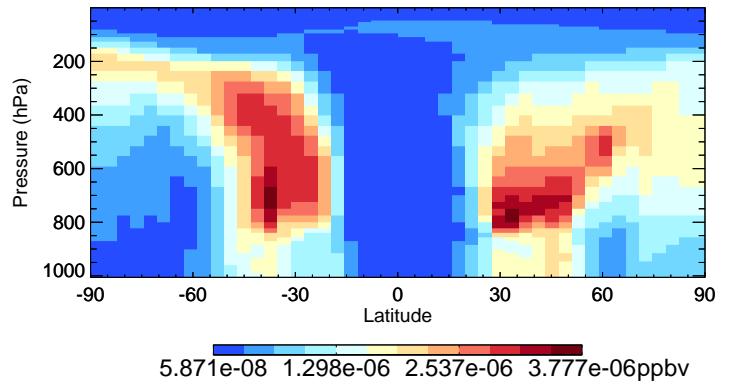
v11-02c-Run0 SOAMG - Species Curtain @ -180.000 for Oct
