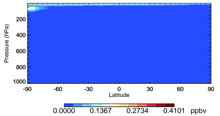
v11-02e-Run0 ClO - Species Curtain @ -180.000 for Oct
