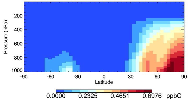
v11-02d-Run1 ALK4 - Species Curtain @ -180.000 for Oct
