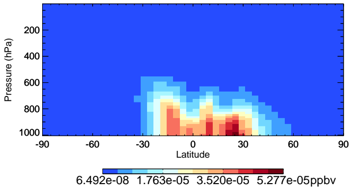
v11-02c-Run0 SOAMG - Species Zonal Mean for Oct
