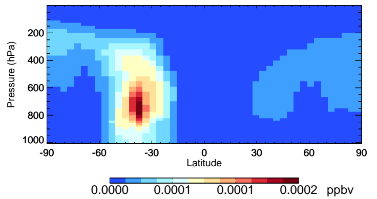
v11-02e-Run0 ISN10A - Species Curtain @ -180.000 for Oct
