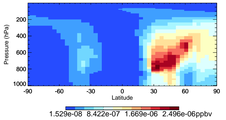
v11-02d-Run1 SOAMG - Species Curtain @ -180.000 for Oct
