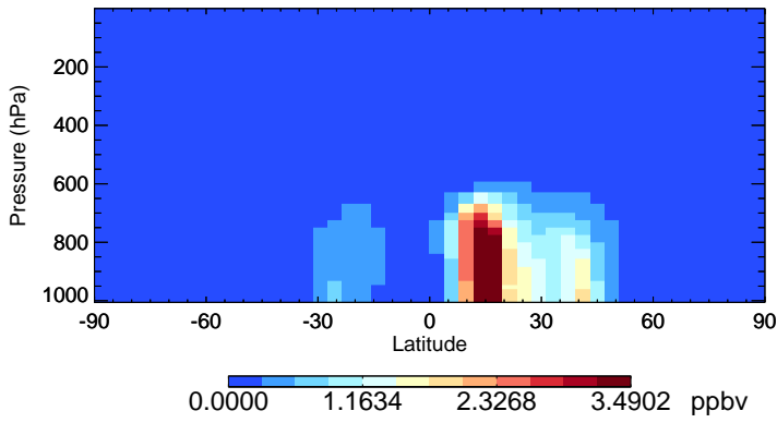
v11-02c-Run0 DST1 - Species Zonal Mean for Oct
