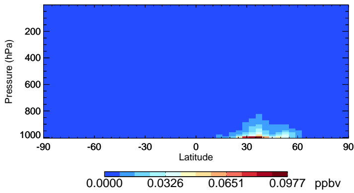
v11-02c-Run0 HNO 2 - Species Zonal Mean for Oct
