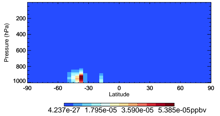
v11-02c-Run0 RIPD - Species Curtain @ -180.000 for Oct
