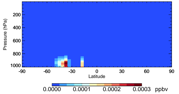
v11-02d-Run1 HPALD - Species Curtain @ -180.000 for Oct
