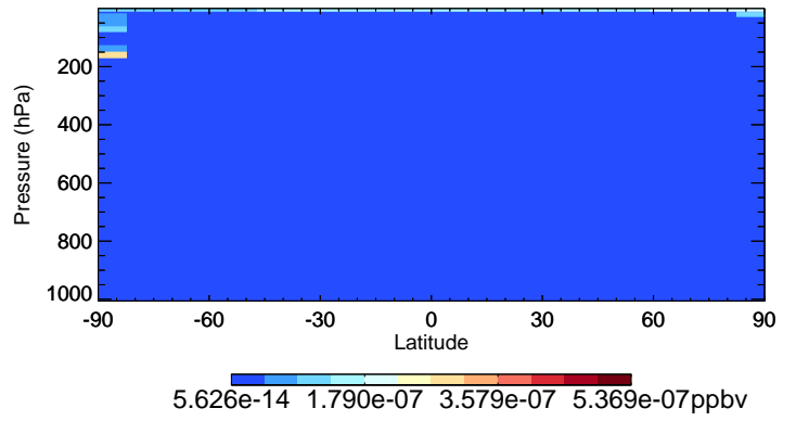
v11-02c-Run0 ClNO 2 - Species Curtain @ -180.000 for Oct
