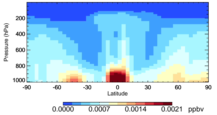
v11-02c-Run0 CHBr3 - Species Curtain @ -180.000 for Oct
