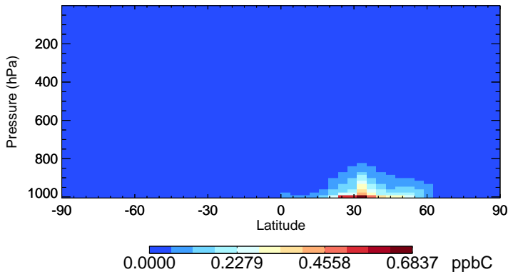
v11-02c-Run0 XYLE - Species Zonal Mean for Oct
