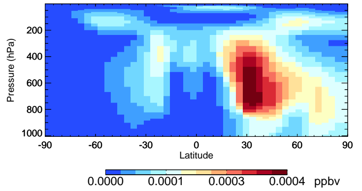
v11-02c-Run0 ASOG1 - Species Curtain @ -180.000 for Oct
