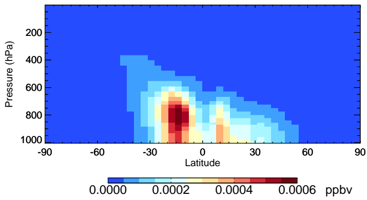
v11-02c-Run0 ISN10A - Species Zonal Mean for Oct
