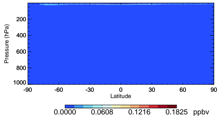
v11-02c-Run0 NO3 - Species Curtain @ -180.000 for Oct
