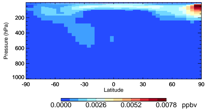
v11-02e-Run0 HOBr - Species Curtain @ -180.000 for Oct
