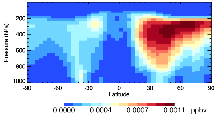
v11-02c-Run0 R4N2 - Species Curtain @ -180.000 for Oct
