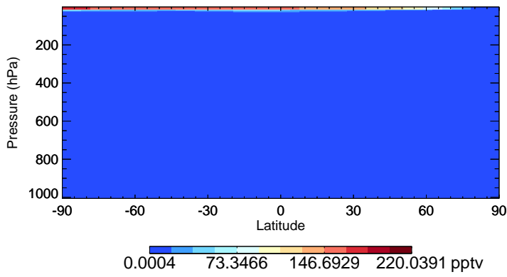
v11-02c-Run0 HO2 - Species Zonal Mean for Oct
