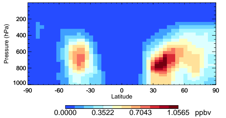
v11-02e-Run0 DST1 - Species Curtain @ -180.000 for Oct
