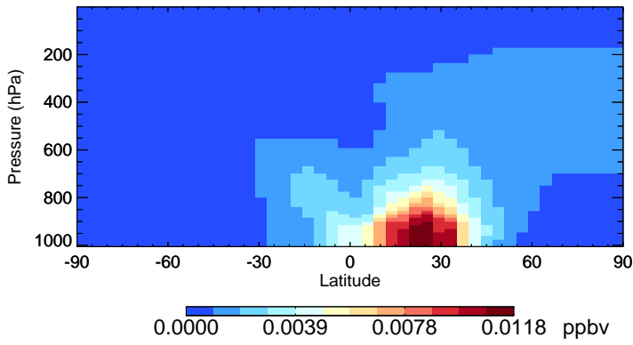
v11-02c-Run0 ASOAN - Species Zonal Mean for Oct
