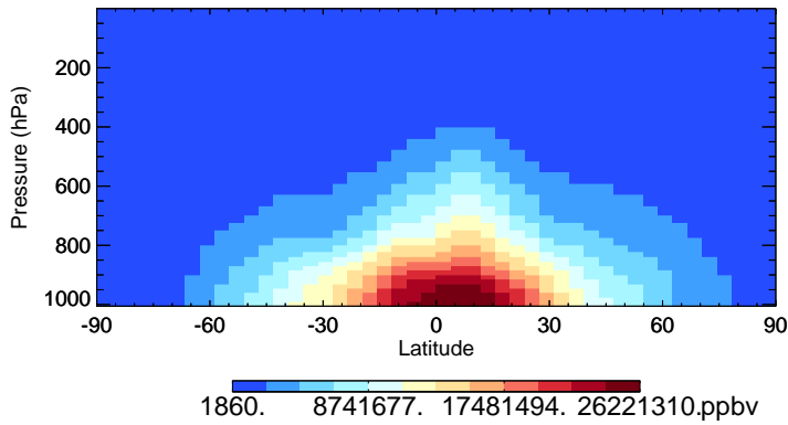
v11-02c-Run0 H2O - Species Zonal Mean for Oct
