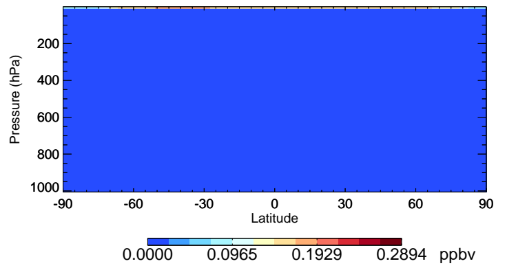
v11-02d-Run1 CI - Species Curtain @ -180.000 for Oct
