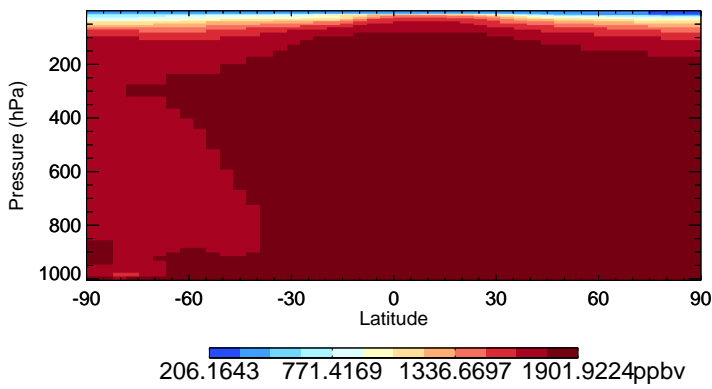
v11-02e-Run0 CH4 - Species Zonal Mean for Oct
