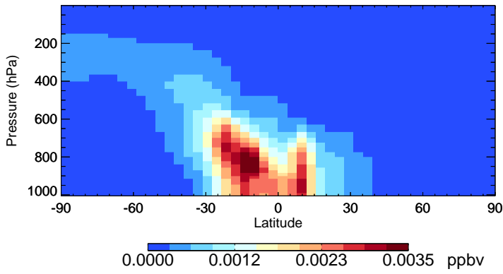
v11-02c-Run0 SOAME - Species Zonal Mean for Oct
