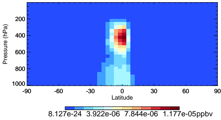
v11-02c-Run0 LVOC - Species Zonal Mean for Oct
