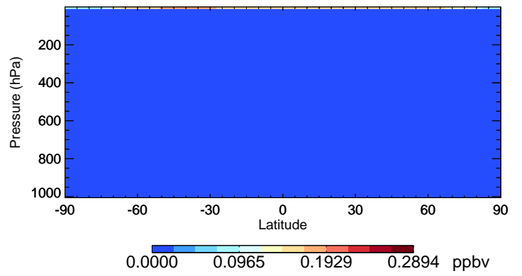
v11-02c-Run0 CI - Species Curtain @ -180.000 for Oct
