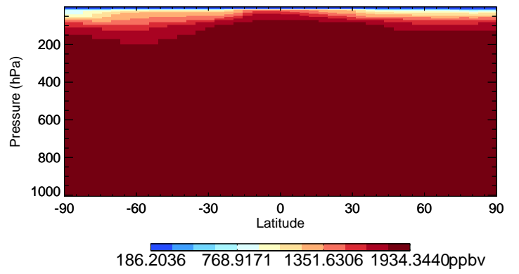
v11-02d-Run1 CH4 - Species Curtain @ -180.000 for Oct
