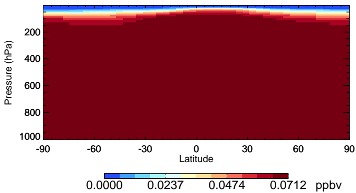
v11-02e-Run0 CFC113 - Species Zonal Mean for Oct
