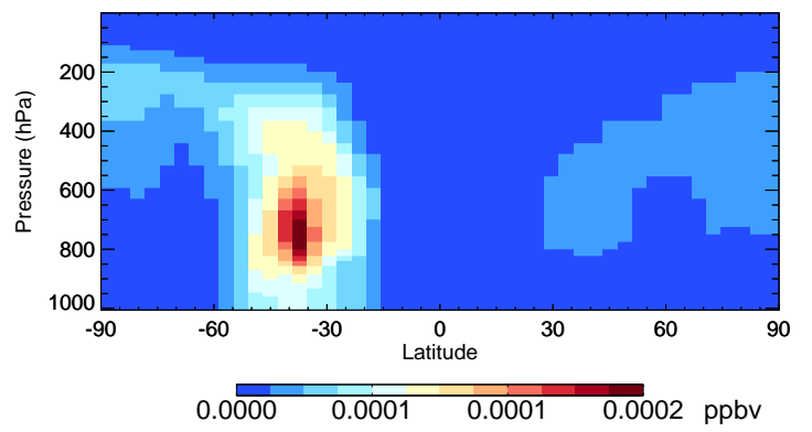
v11-02d-Run1 ISN10A - Species Curtain @ -180.000 for Oct
