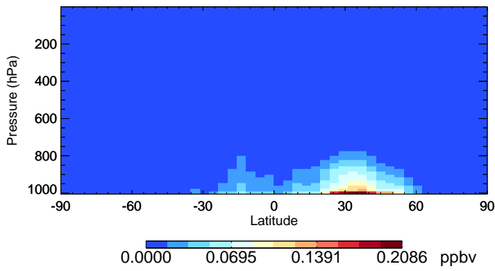
v11-02d-Run1 BCPO - Species Zonal Mean for Oct
