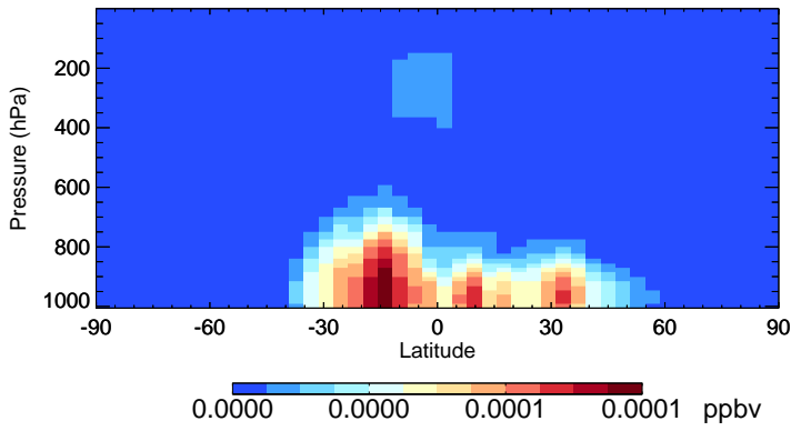
v11-02c-Run0 MACRN - Species Zonal Mean for Oct
