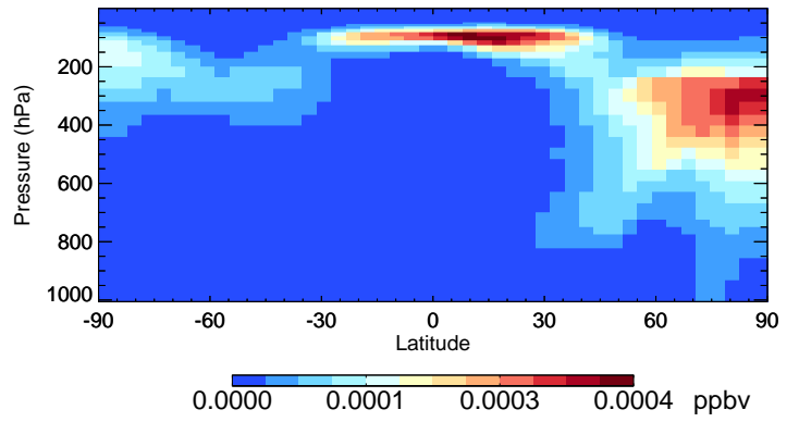
v11-02c-Run0 ASOA2 - Species Curtain @ -180.000 for Oct
