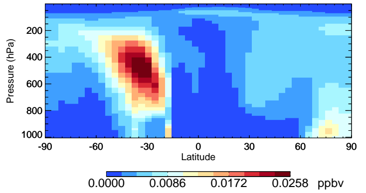
v11-02c-Run0 TSOG3 - Species Curtain @ -180.000 for Oct
