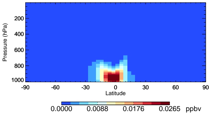
v11-02e-Run0 RIPB - Species Zonal Mean for Oct
