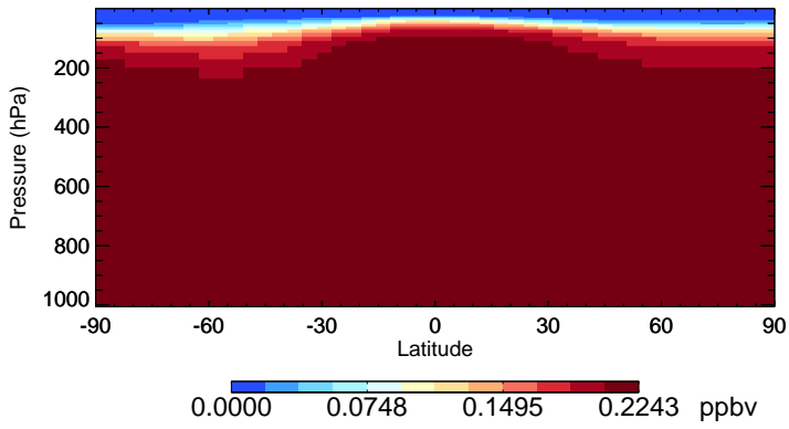
v11-02c-Run0 CFC11 - Species Zonal Mean for Oct
