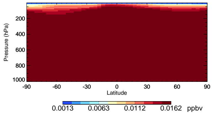
v11-02d-Run1 CFC114 - Species Curtain @ -180.000 for Oct
