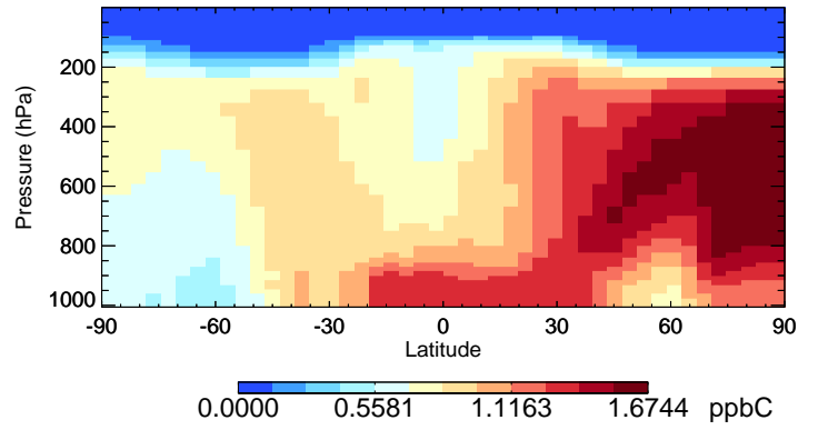
v11-02d-Run1 ACET - Species Curtain @ -180.000 for Oct
