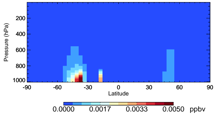
v11-02c-Run0 SOAP - Species Curtain @ -180.000 for Oct
