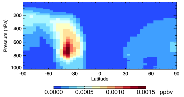
v11-02c-Run0 SOAME - Species Curtain @ -180.000 for Oct
