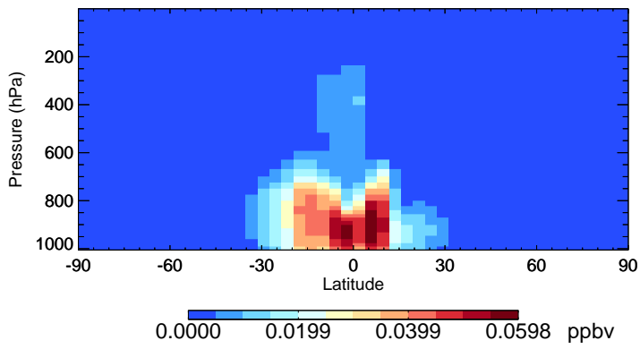
v11-02c-Run0 IEPOXA - Species Zonal Mean for Oct
