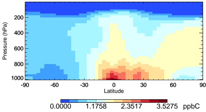
v11-02d-Run1 ACET - Species Zonal Mean for Oct
