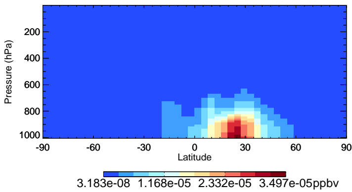
v11-02e-Run0 SOAMG - Species Zonal Mean for Oct
