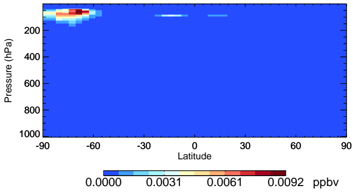
v11-02c-Run0 Cl2 - Species Zonal Mean for Oct
