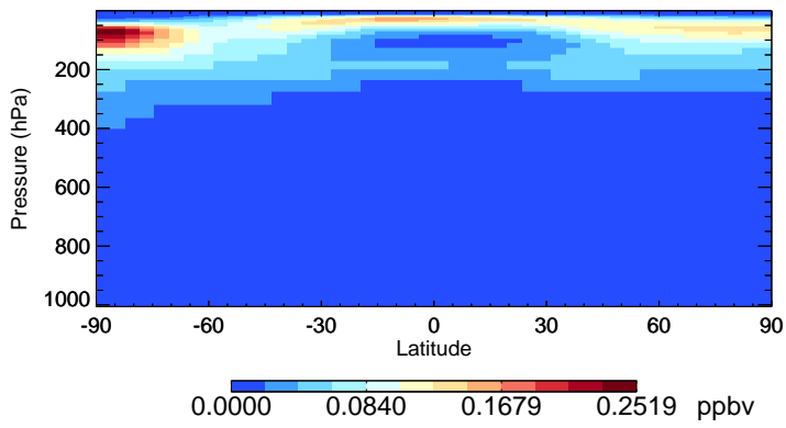
v11-02c-Run0 MPN - Species Zonal Mean for Oct
