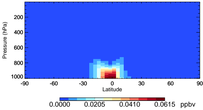
v11-02d-Run1 HPALD - Species Zonal Mean for Oct
