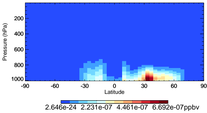
v11-02d-Run1 NPMN - Species Zonal Mean for Oct
