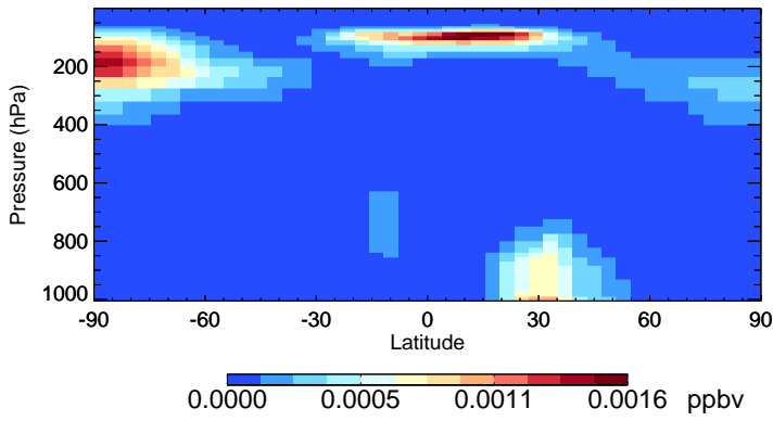
v11-02c-Run0 ASOA3 - Species Zonal Mean for Oct
