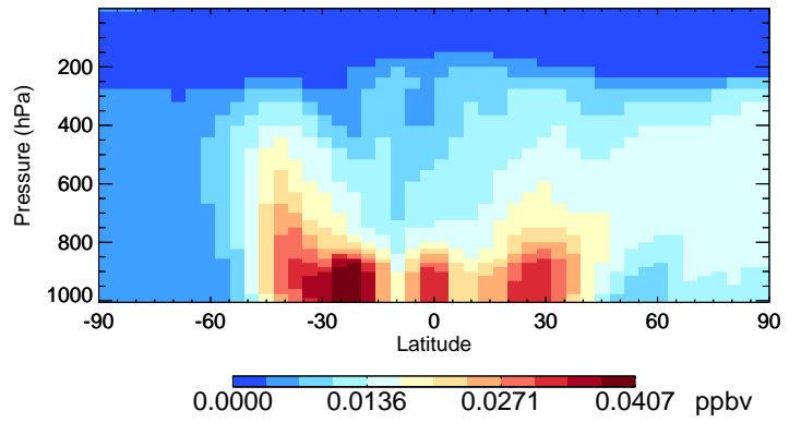
v11-02c-Run0 MAP - Species Curtain @ -180.000 for Oct
