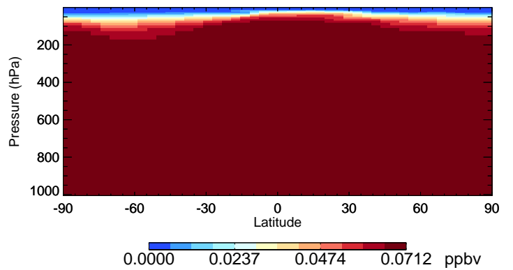
v11-02e-Run0 CFC113 - Species Curtain @ -180.000 for Oct
