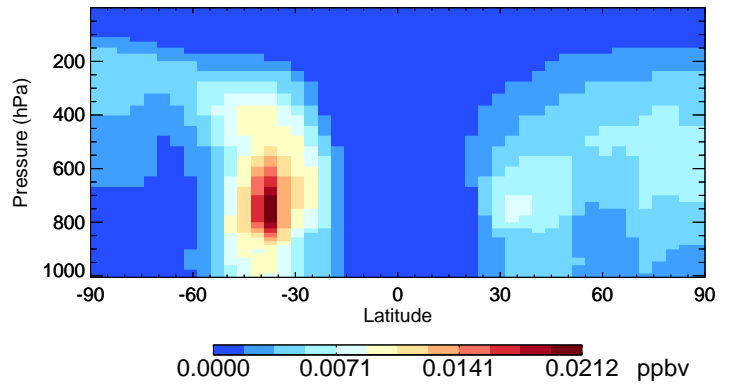
v11-02c-Run0 INDIOL - Species Curtain @ -180.000 for Oct
