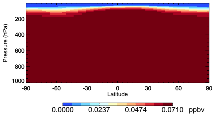
v11-02e-Run0 CCI4 - Species Zonal Mean for Oct
