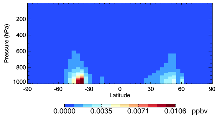
v11-02c-Run0 BCPO - Species Curtain @ -180.000 for Oct
