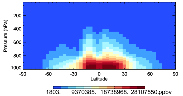
v11-02e-Run0 H2O - Species Curtain @ -180.000 for Oct
