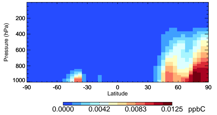
v11-02c-Run0 XYLE - Species Curtain @ -180.000 for Oct
