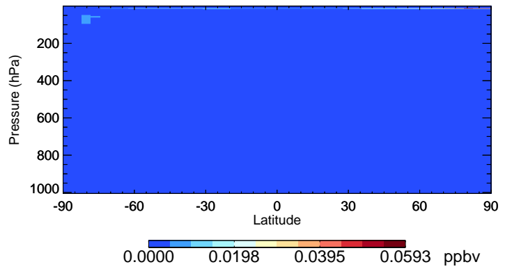
v11-02e-Run0 OCIO - Species Curtain @ -180.000 for Oct
