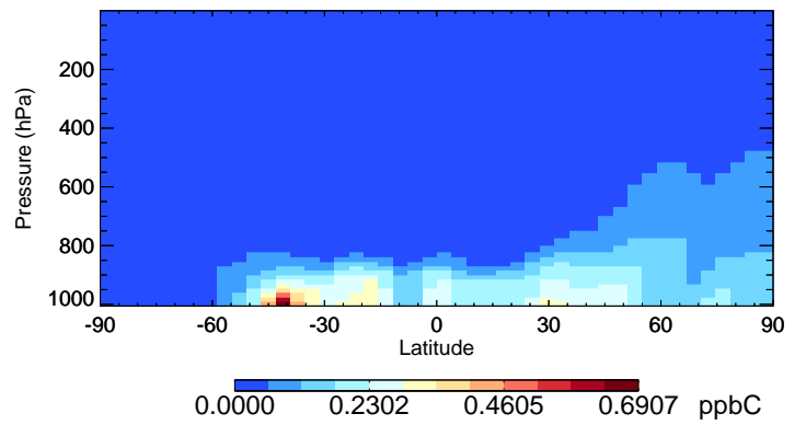
v11-02d-Run1 ALD2 - Species Curtain @ -180.000 for Oct
