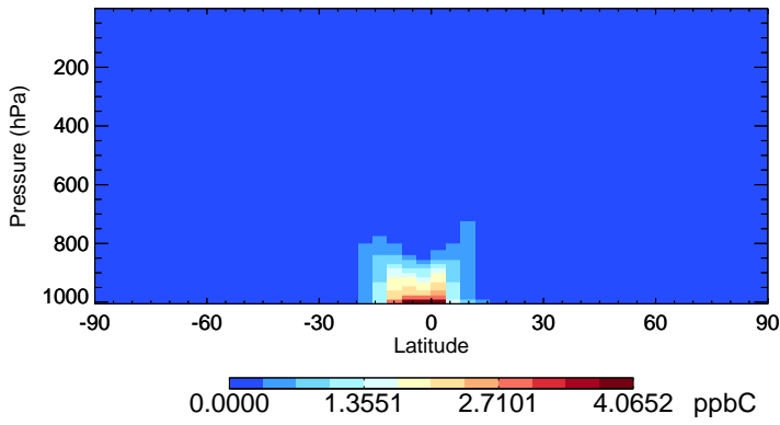
v11-02c-Run0 ISOP - Species Zonal Mean for Oct
