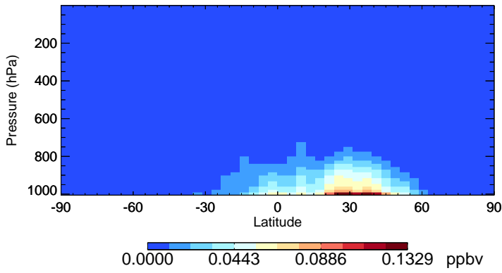
v11-02c-Run0 SOAP - Species Zonal Mean for Oct
