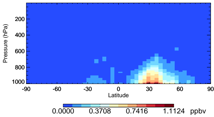
v11-02c-Run0 SO2 - Species Zonal Mean for Oct
