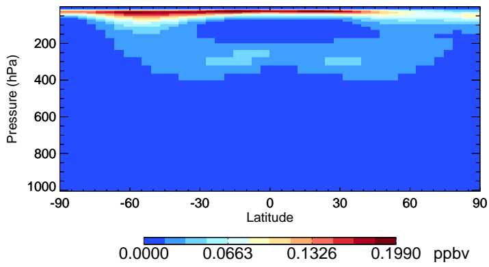
v11-02d-Run1 HNO4 - Species Zonal Mean for Oct
