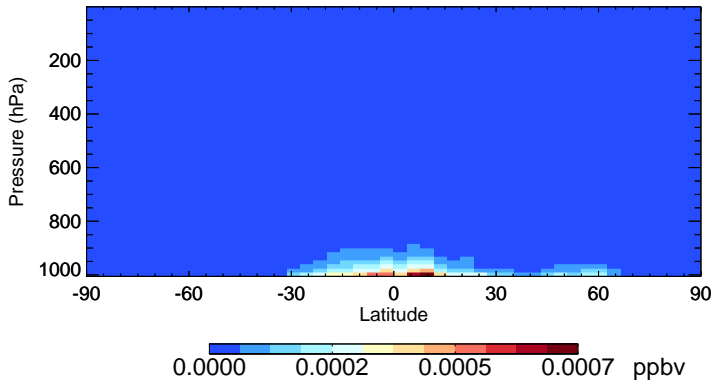
v11-02d-Run1 MONITU - Species Zonal Mean for Oct
