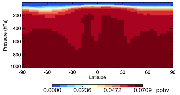
v11-02c-Run0 CCI4 - Species Curtain @ -180.000 for Oct
