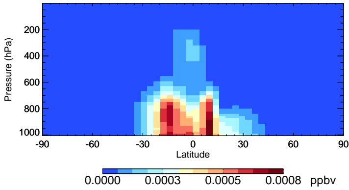
v11-02d-Run1 HCOOH - Species Zonal Mean for Oct
