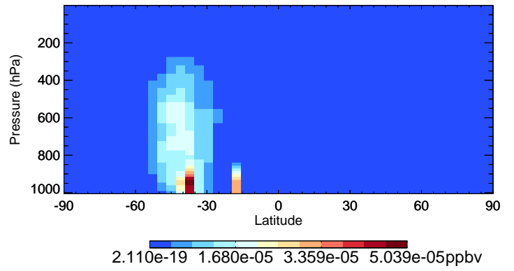
v11-02c-Run0 HCOOH - Species Curtain @ -180.000 for Oct
