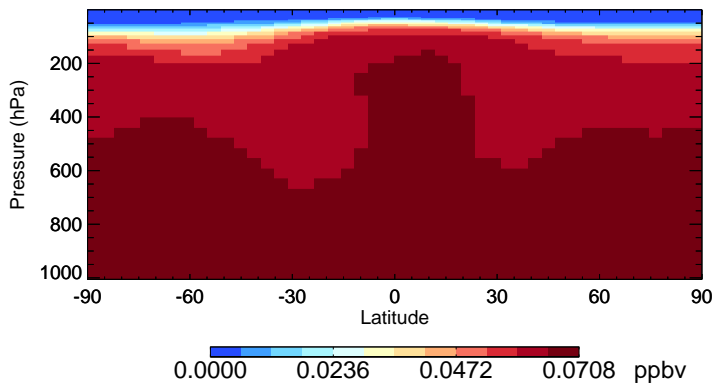
v11-02c-Run0 CCI4 - Species Zonal Mean for Oct
