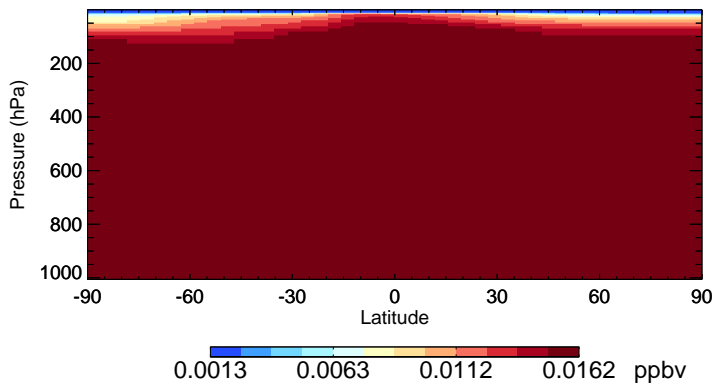
v11-02c-Run0 CFC114 - Species Zonal Mean for Oct
