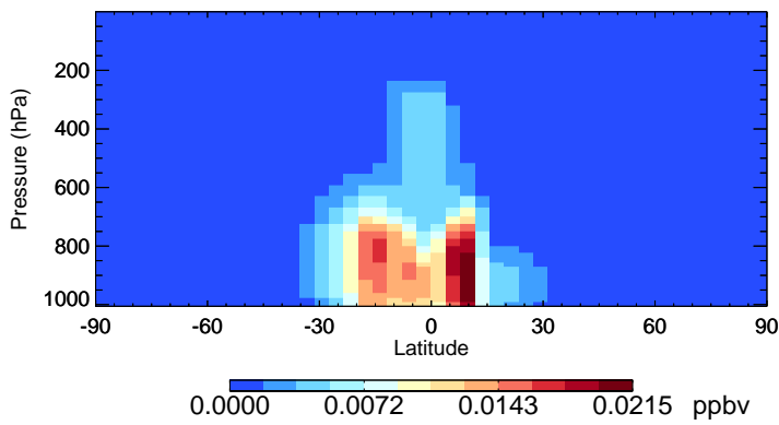
v11-02e-Run0 HC187 - Species Zonal Mean for Oct
