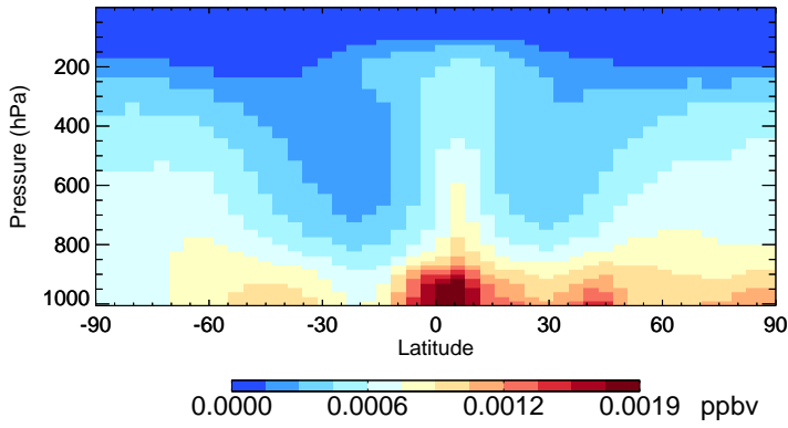
v11-02d-Run1 CHBr3 - Species Zonal Mean for Oct
