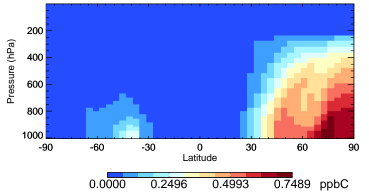
v11-02c-Run0 ALK4 - Species Curtain @ -180.000 for Oct
