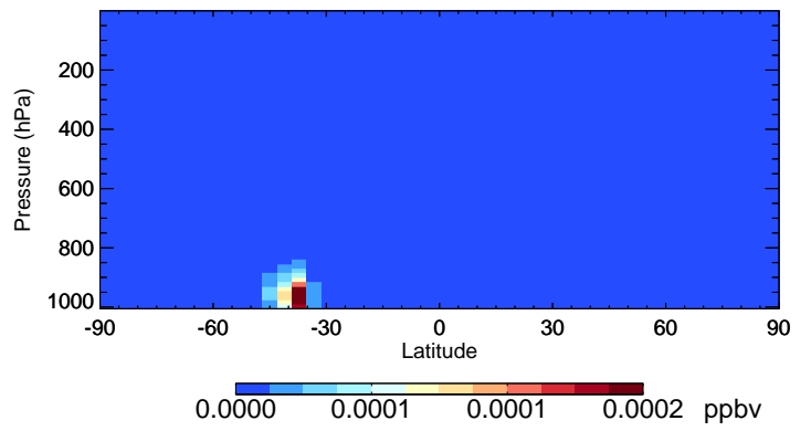
v11-02c-Run0 ISN1 - Species Curtain @ -180.000 for Oct
