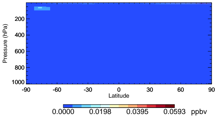
v11-02e-Run0 OCIO - Species Zonal Mean for Oct
