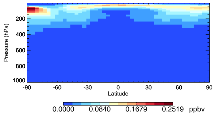
v11-02c-Run0 MPN - Species Curtain @ -180.000 for Oct
