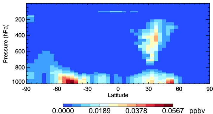
v11-02c-Run0 NIT - Species Curtain @ -180.000 for Oct
