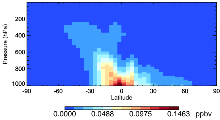
v11-02c-Run0 TSOG3 - Species Zonal Mean for Oct
