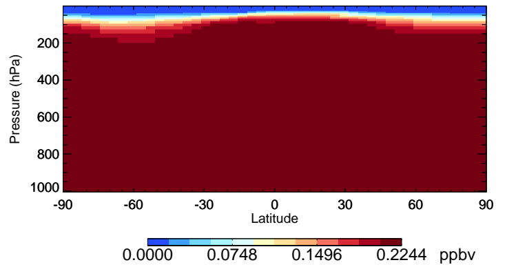
v11-02e-Run0 CFC11 - Species Curtain @ -180.000 for Oct
