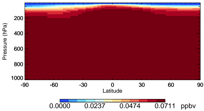
v11-02d-Run1 CFC113 - Species Zonal Mean for Oct
