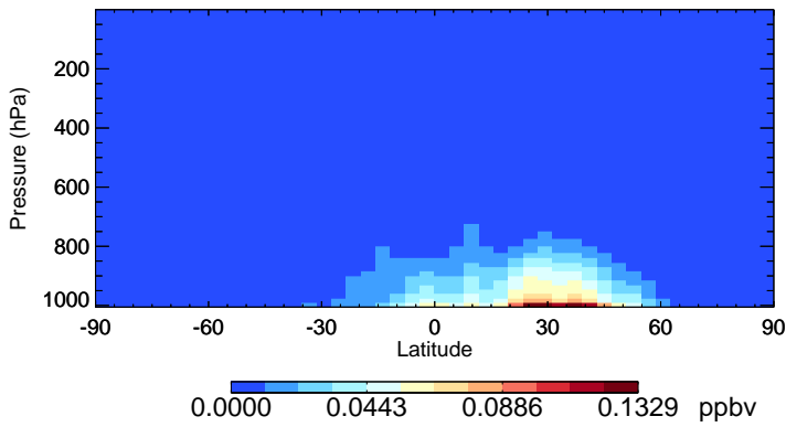
v11-02e-Run0 SOAP - Species Zonal Mean for Oct
