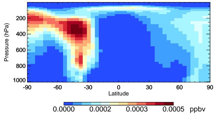
v11-02c-Run0 TSOA1 - Species Curtain @ -180.000 for Oct
