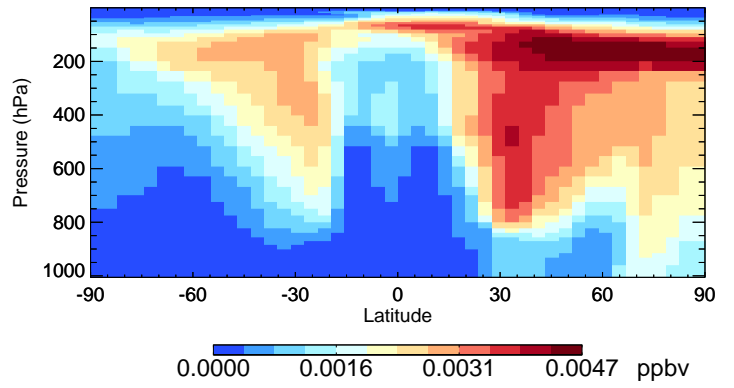
v11-02c-Run0 ASOG3 - Species Curtain @ -180.000 for Oct
