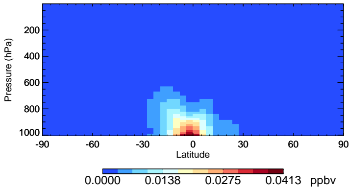
v11-02c-Run0 TSOA0 - Species Zonal Mean for Oct
