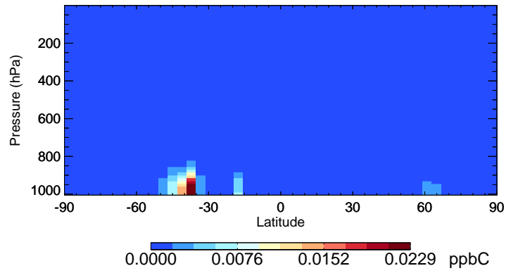
v11-02c-Run0 ISOP - Species Curtain @ -180.000 for Oct
