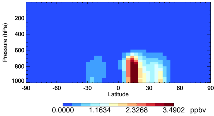
v11-02d-Run1 DST1 - Species Zonal Mean for Oct
