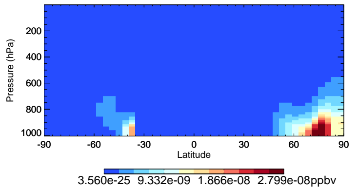
v11-02d-Run1 NPMN - Species Curtain @ -180.000 for Oct
