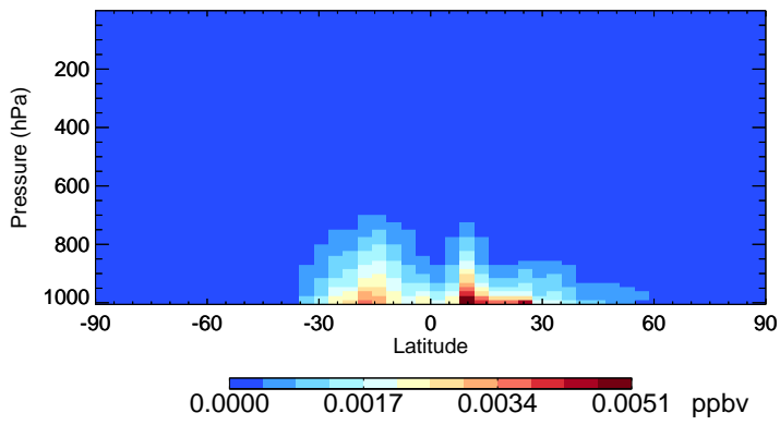
v11-02c-Run0 ISN1 - Species Zonal Mean for Oct
