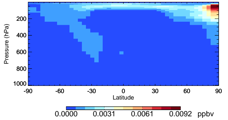
v11-02d-Run1 HOBr - Species Curtain @ -180.000 for Oct
