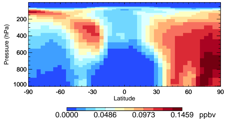
v11-02c-Run0 PAN - Species Curtain @ -180.000 for Oct
