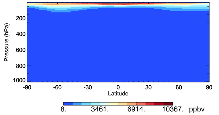
v11-02c-Run0 O3 - Species Curtain @ -180.000 for Oct
