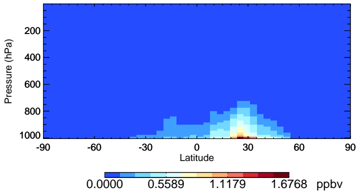
v11-02c-Run0 NH3 - Species Zonal Mean for Oct
