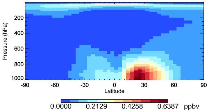
v11-02c-Run0 SO4 - Species Zonal Mean for Oct
