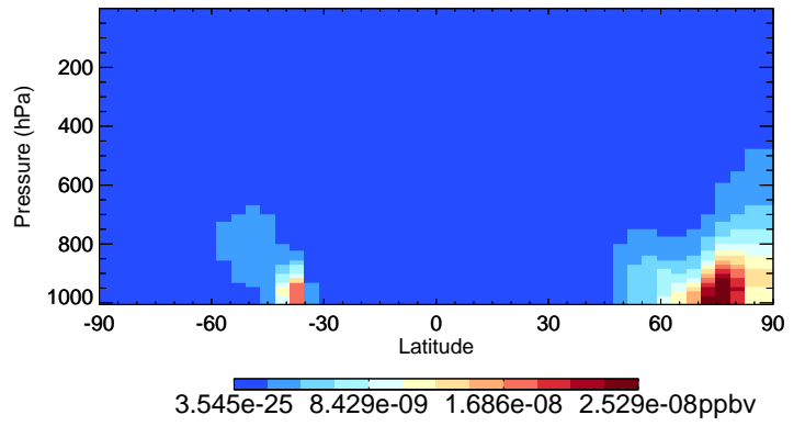
v11-02c-Run0 NPMN - Species Curtain @ -180.000 for Oct
