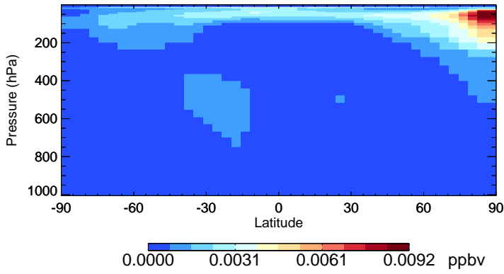
v11-02d-Run1 HOBr - Species Zonal Mean for Oct
