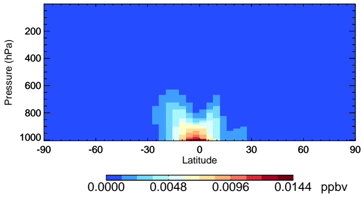
v11-02c-Run0 TSOA1 - Species Zonal Mean for Oct
