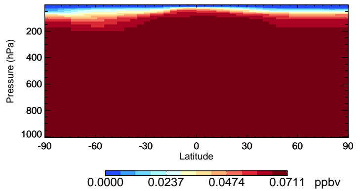
v11-02d-Run1 CFC113 - Species Curtain @ -180.000 for Oct
