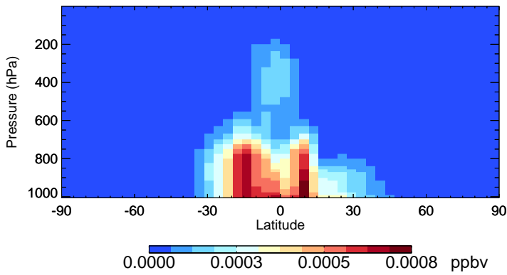
v11-02e-Run0 HCOOH - Species Zonal Mean for Oct
