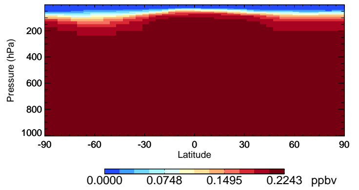
v11-02d-Run1 CFC11 - Species Curtain @ -180.000 for Oct
