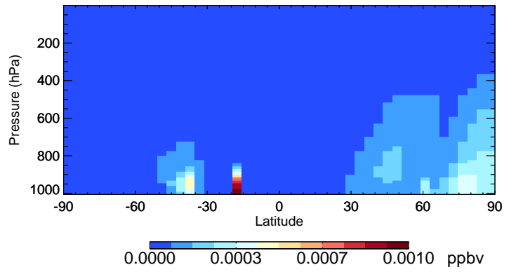
v11-02c-Run0 GLYX - Species Curtain @ -180.000 for Oct
