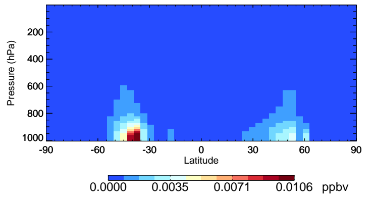
v11-02d-Run1 BCPO - Species Curtain @ -180.000 for Oct
