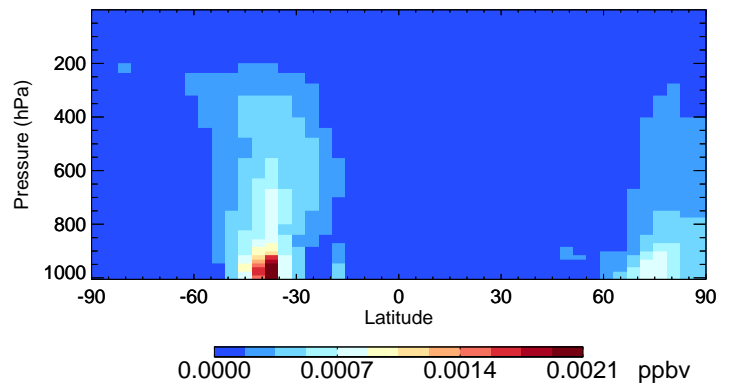
v11-02d-Run1 MONITA - Species Curtain @ -180.000 for Oct
