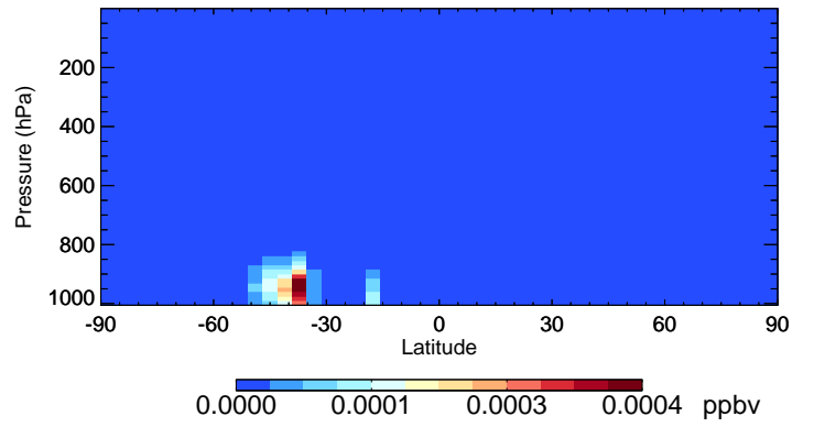
v11-02c-Run0 RIPB - Species Curtain @ -180.000 for Oct
