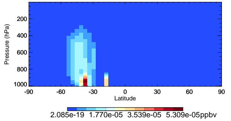
v11-02d-Run1 HCOOH - Species Curtain @ -180.000 for Oct
