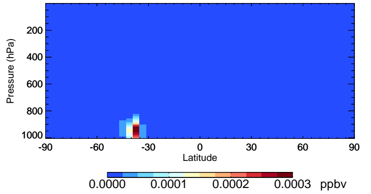
v11-02d-Run1 ISOPNB - Species Curtain @ -180.000 for Oct
