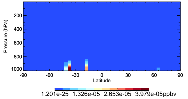
v11-02d-Run1 MONITU - Species Curtain @ -180.000 for Oct
