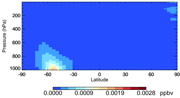
v11-02c-Run0 Br2 - Species Zonal Mean for Oct
