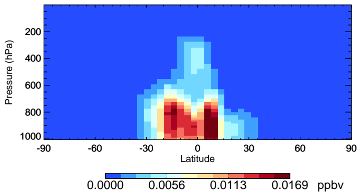
v11-02c-Run0 HC187 - Species Zonal Mean for Oct
