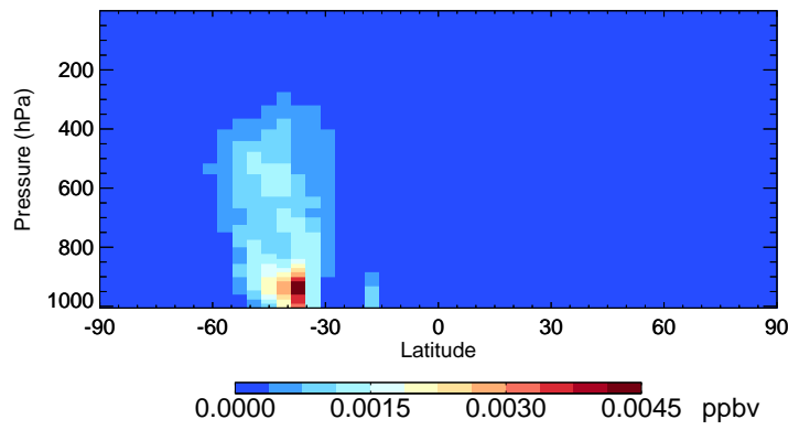
v11-02c-Run0 IEPOXA - Species Curtain @ -180.000 for Oct
