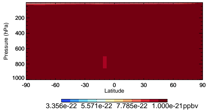
v11-02e-Run0 HCFC123 - Species Curtain @ -180.000 for Oct
