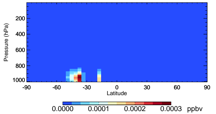
v11-02e-Run0 HPALD - Species Curtain @ -180.000 for Oct
