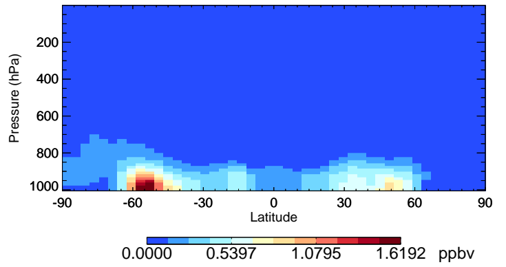
v11-02c-Run0 SALA - Species Curtain @ -180.000 for Oct
