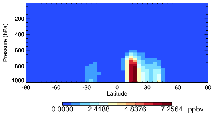
v11-02c-Run0 DST2 - Species Zonal Mean for Oct
