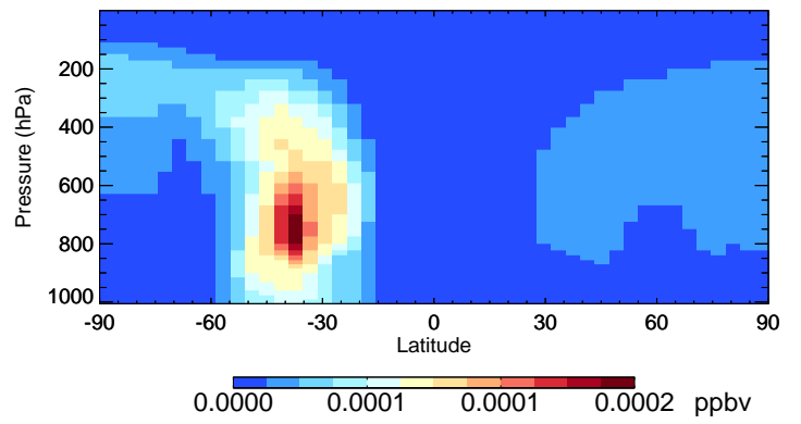
v11-02c-Run0 ISN10A - Species Curtain @ -180.000 for Oct
