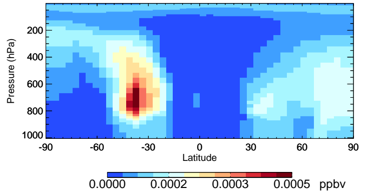
v11-02d-Run1 SOAME - Species Curtain @ -180.000 for Oct
