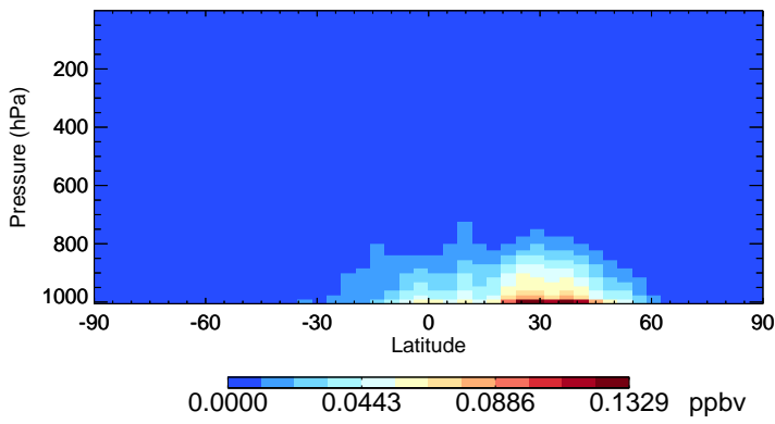
v11-02d-Run1 SOAP - Species Zonal Mean for Oct
