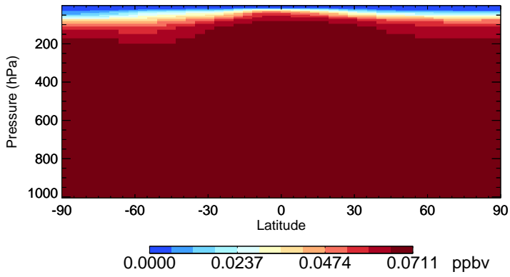
v11-02c-Run0 CFC113 - Species Zonal Mean for Oct
