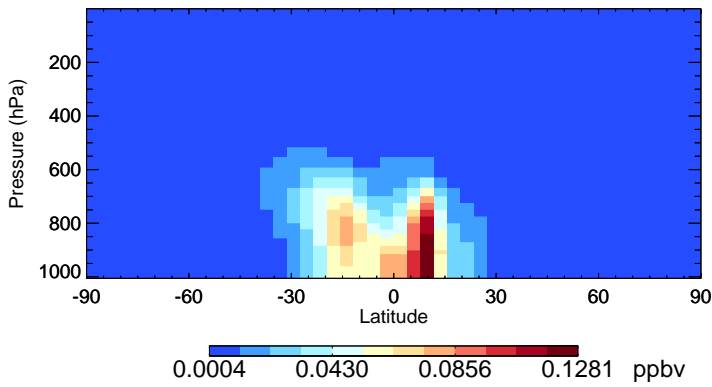
v11-02e-Run0 SOAIE - Species Zonal Mean for Oct
