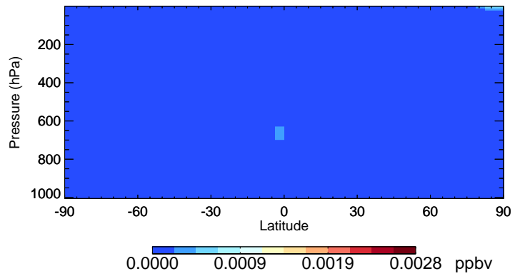
v11-02e-Run0 Br2 - Species Curtain @ -180.000 for Oct
