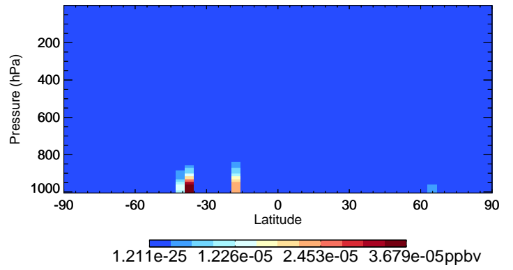
v11-02c-Run0 MONITU - Species Curtain @ -180.000 for Oct
