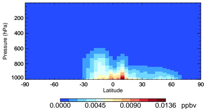
v11-02d-Run1 MONITA - Species Zonal Mean for Oct
