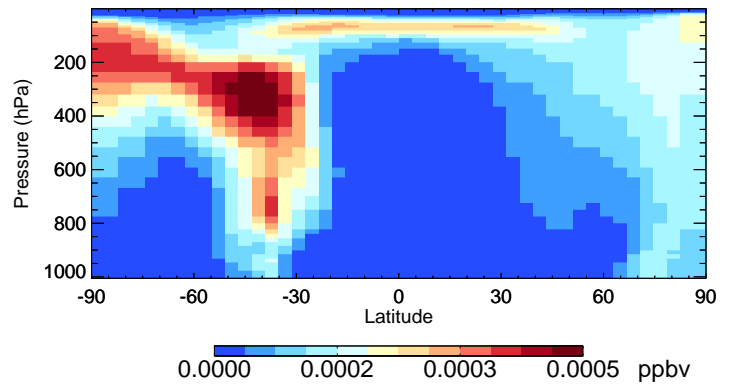
v11-02e-Run0 TSOA1 - Species Curtain @ -180.000 for Oct
