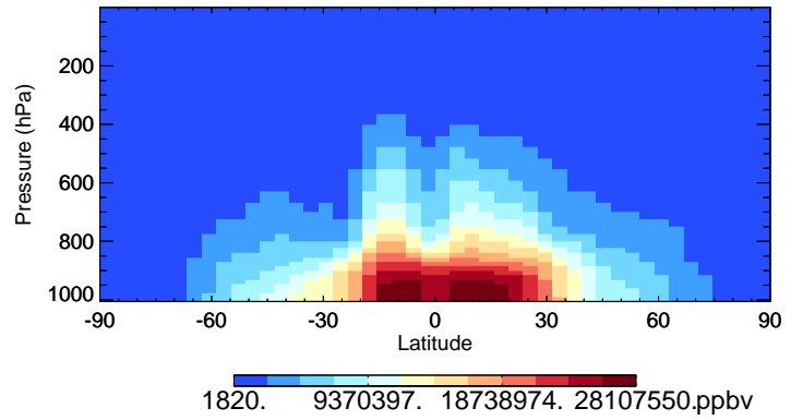
v11-02d-Run1 H2O - Species Curtain @ -180.000 for Oct
