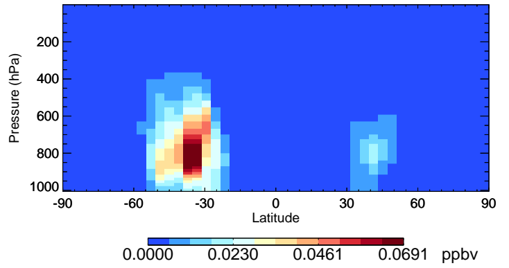
v11-02d-Run1 DST4 - Species Curtain @ -180.000 for Oct
