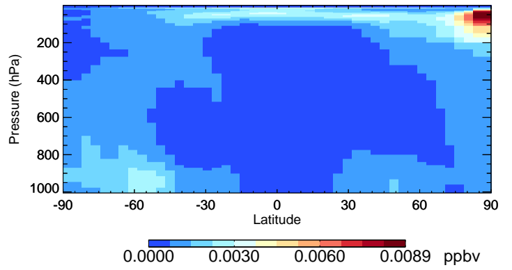
v11-02c-Run0 HOBr - Species Curtain @ -180.000 for Oct
