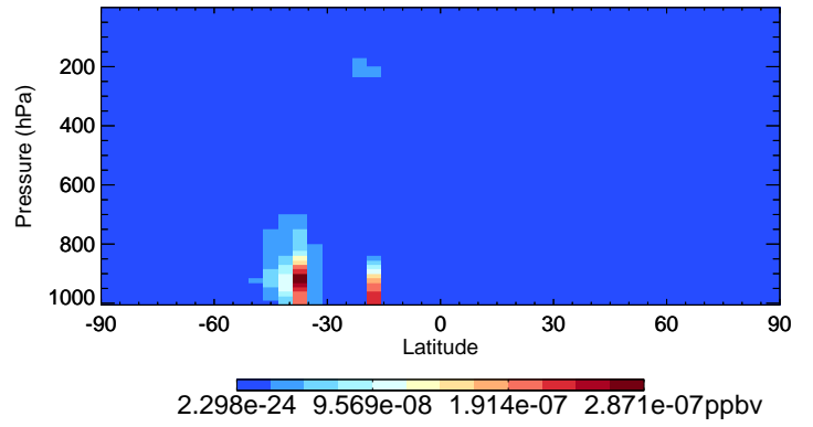
v11-02d-Run1 LVOC - Species Curtain @ -180.000 for Oct
