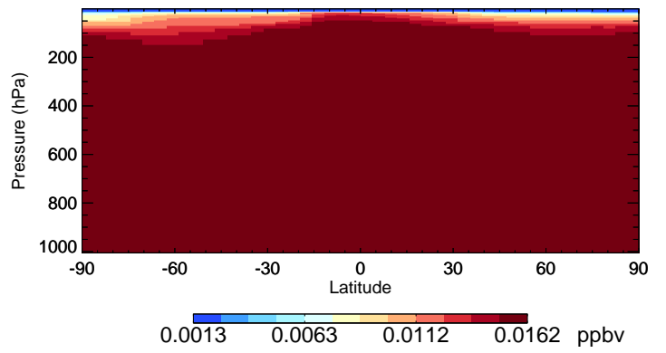
v11-02c-Run0 CFC114 - Species Curtain @ -180.000 for Oct
