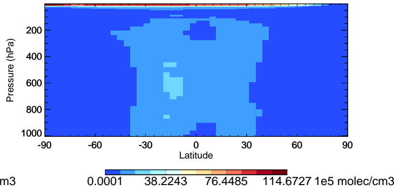
v11-02c-Run0 OH - Species Curtain @ -180.000 for Oct
