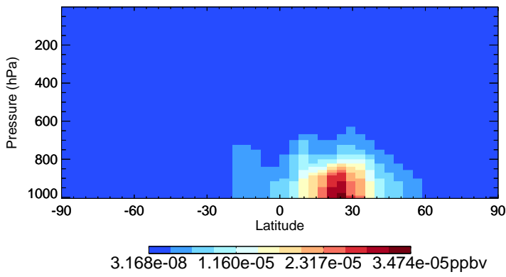
v11-02d-Run1 SOAMG - Species Zonal Mean for Oct
