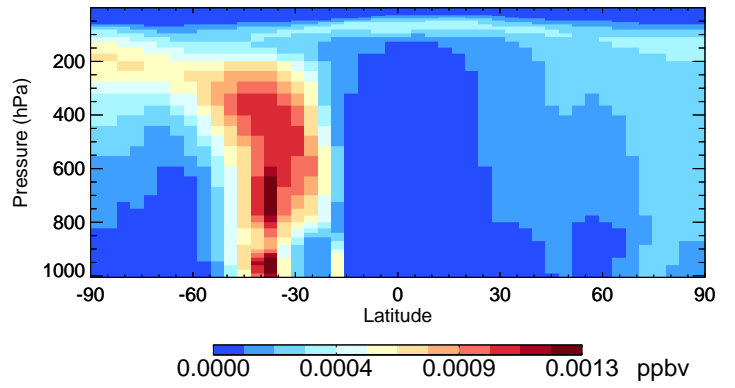
v11-02c-Run0 TSOA0 - Species Curtain @ -180.000 for Oct
