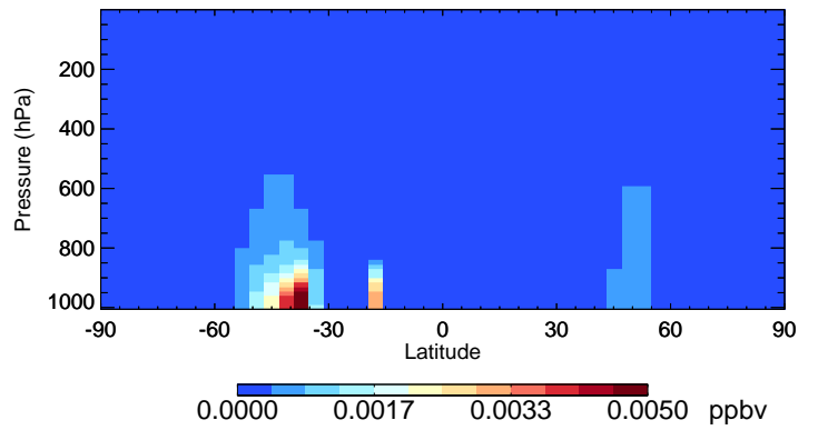
v11-02e-Run0 SOAP - Species Curtain @ -180.000 for Oct
