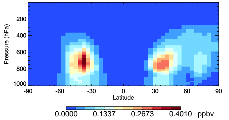
v11-02c-Run0 DST1 - Species Curtain @ -180.000 for Oct
