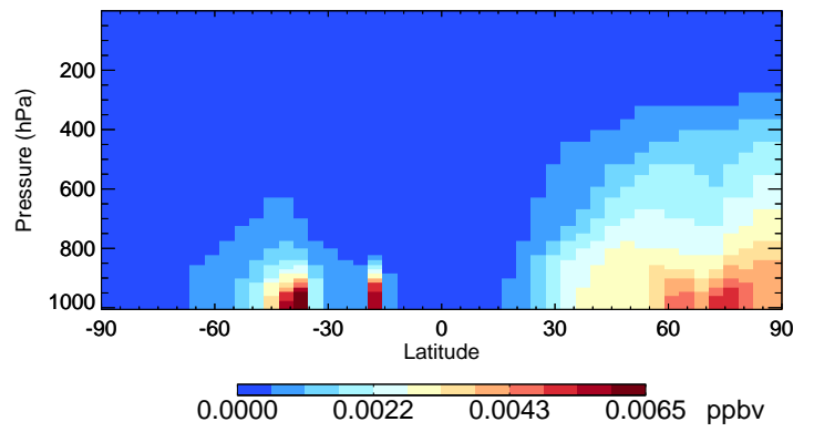
v11-02c-Run0 RCHO - Species Curtain @ -180.000 for Oct
