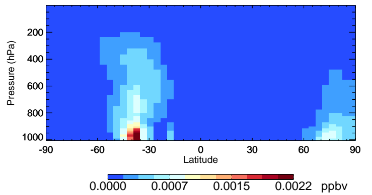
v11-02e-Run0 MONITA - Species Curtain @ -180.000 for Oct
