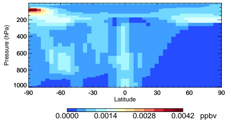
v11-02c-Run0 HBr - Species Curtain @ -180.000 for Oct
