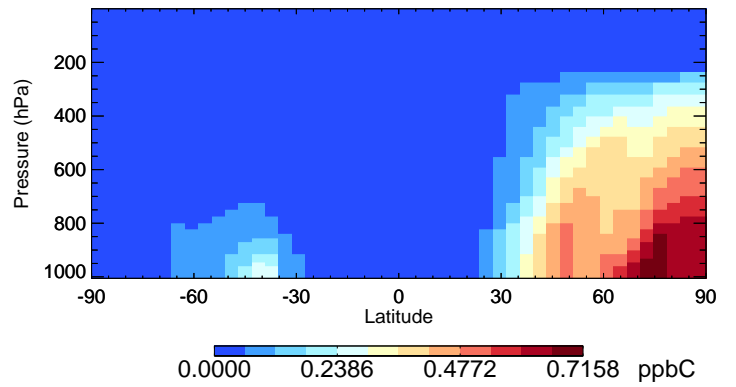
v11-02e-Run0 ALK4 - Species Curtain @ -180.000 for Oct
