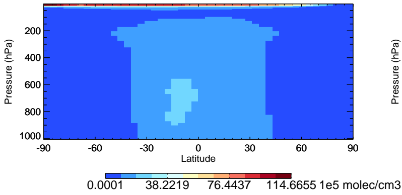
v11-02c-Run0 OH - Species Zonal Mean for Oct
