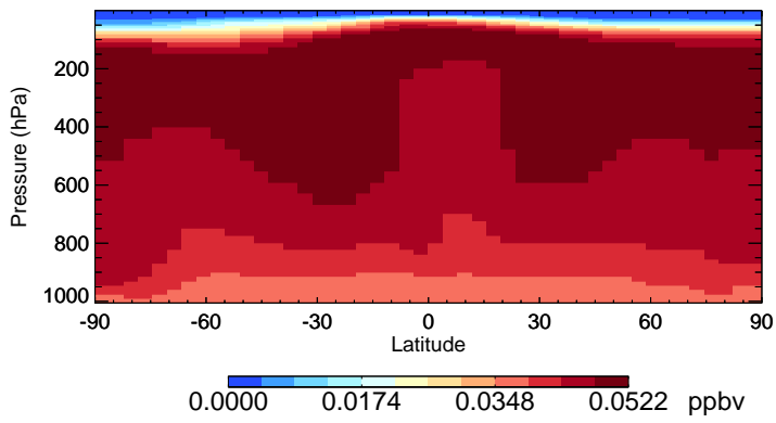
v11-02c-Run0 HCFC141b - Species Zonal Mean for Oct
