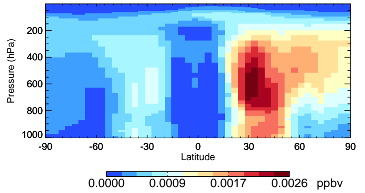
v11-02c-Run0 ASOAN - Species Curtain @ -180.000 for Oct
