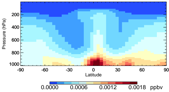
v11-02c-Run0 CHBr3 - Species Zonal Mean for Oct
