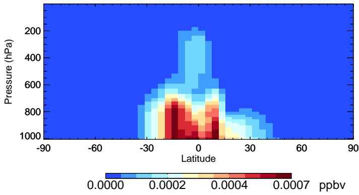
v11-02c-Run0 HCOOH - Species Zonal Mean for Oct
