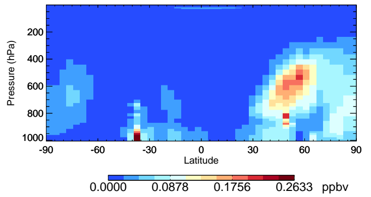
v11-02c-Run0 SO2 - Species Curtain @ -180.000 for Oct
