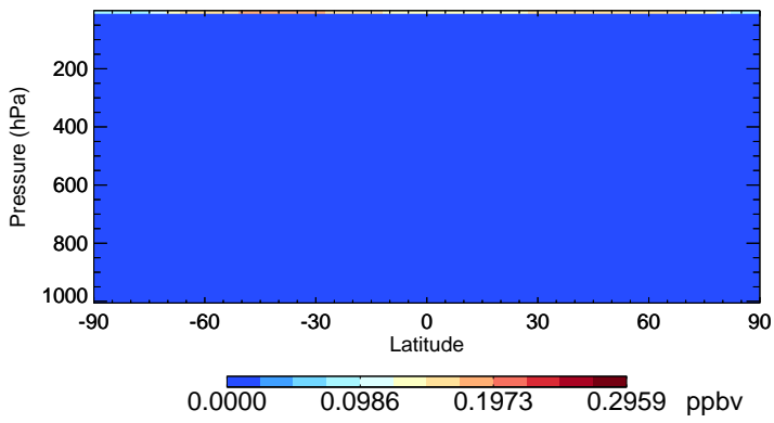
v11-02c-Run0 CI - Species Zonal Mean for Oct
