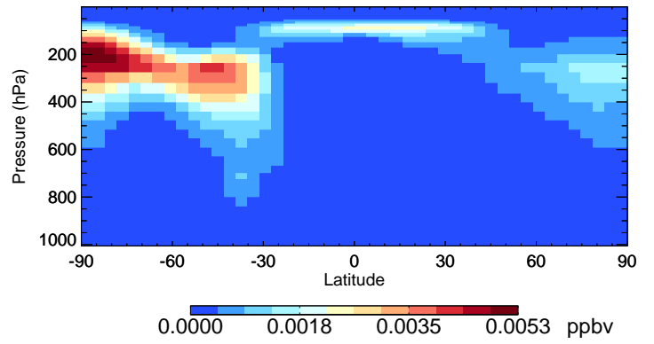
v11-02c-Run0 TSOA2 - Species Curtain @ -180.000 for Oct
