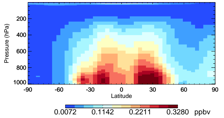
v11-02c-Run0 CH2O - Species Curtain @ -180.000 for Oct
