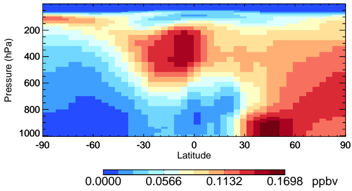
v11-02c-Run0 PAN - Species Zonal Mean for Oct
