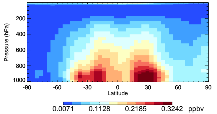
v11-02e-Run0 CH2O - Species Curtain @ -180.000 for Oct
