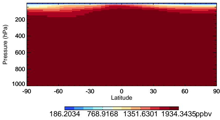
v11-02d-Run1 CH4 - Species Zonal Mean for Oct
