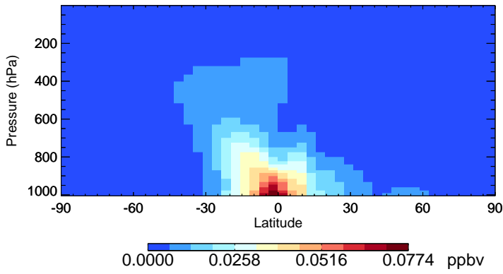
v11-02c-Run0 TSOG2 - Species Zonal Mean for Oct
