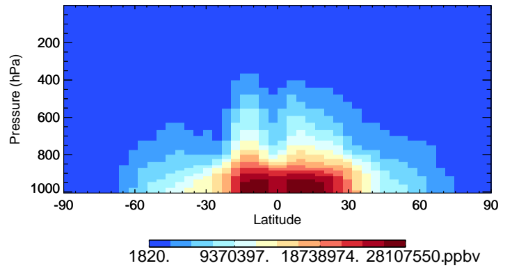
v11-02c-Run0 H2O - Species Curtain @ -180.000 for Oct
