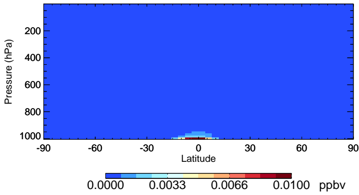
v11-02c-Run0 LIMO - Species Zonal Mean for Oct
