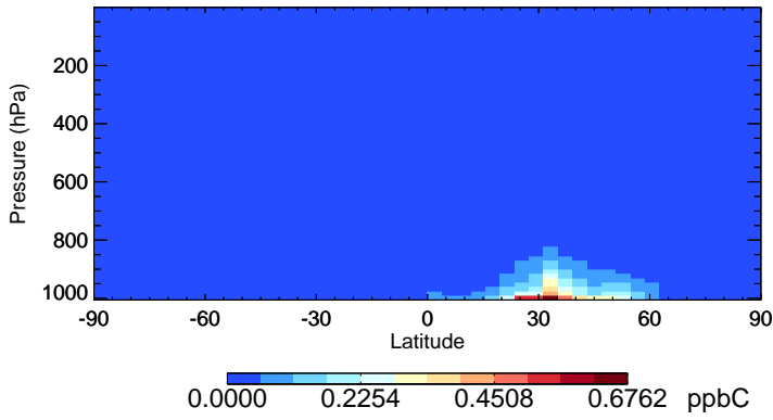
v11-02d-Run1 XYLE - Species Zonal Mean for Oct
