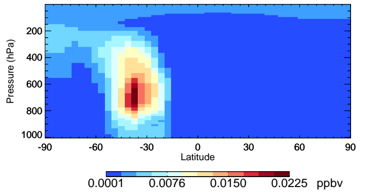
v11-02e-Run0 SOAIE - Species Curtain @ -180.000 for Oct
