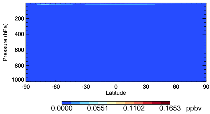
v11-02c-Run0 NO3 - Species Zonal Mean for Oct
