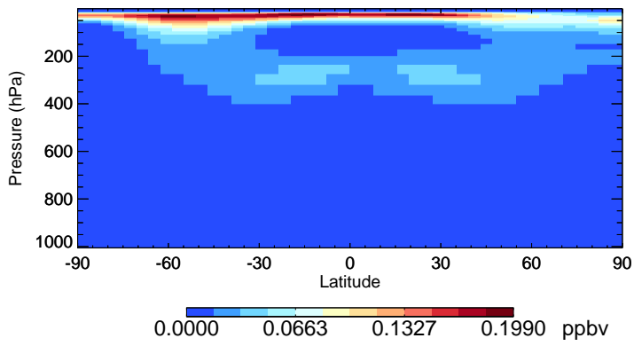
v11-02c-Run0 HNO4 - Species Zonal Mean for Oct
