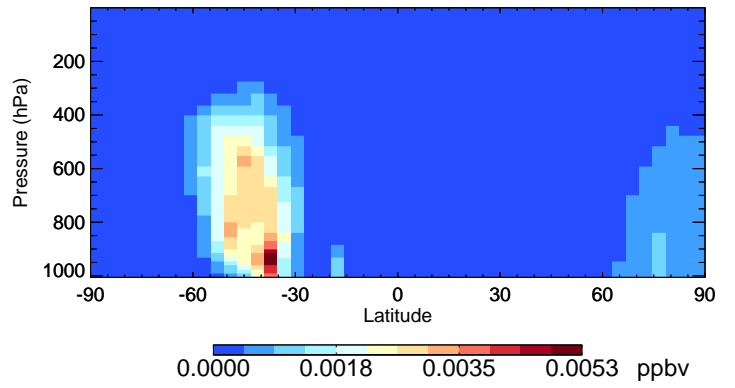
v11-02c-Run0 GLYC - Species Curtain @ -180.000 for Oct
