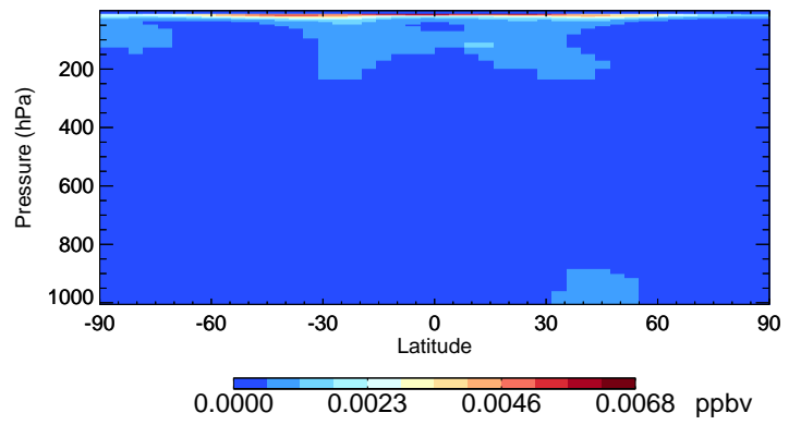
v11-02c-Run0 HNO 2 - Species Curtain @ -180.000 for Oct
