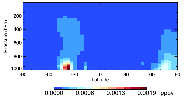
v11-02c-Run0 MONITA - Species Curtain @ -180.000 for Oct
