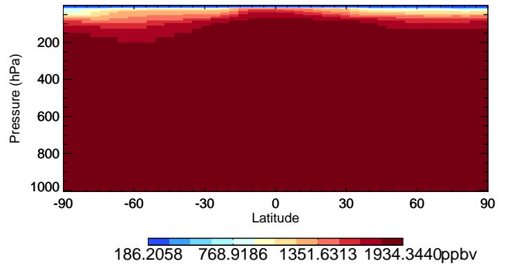
v11-02c-Run0 CH4 - Species Curtain @ -180.000 for Oct
