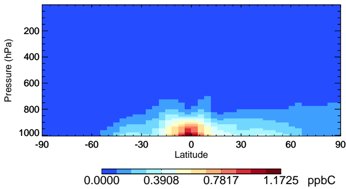
v11-02d-Run1 ALD2 - Species Zonal Mean for Oct
