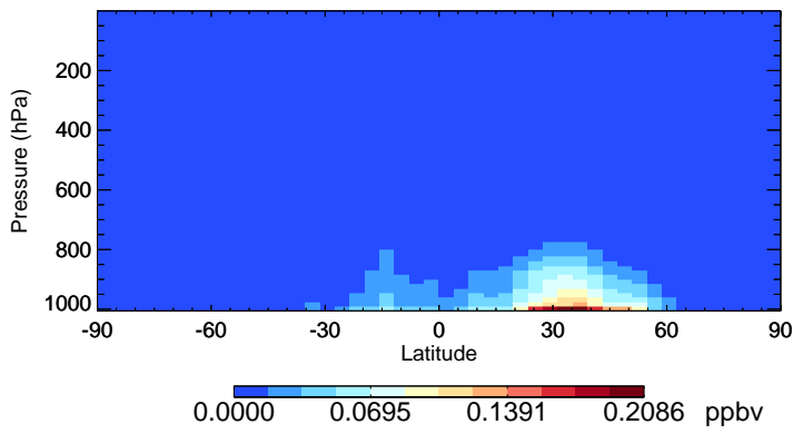
v11-02c-Run0 BCPO - Species Zonal Mean for Oct
