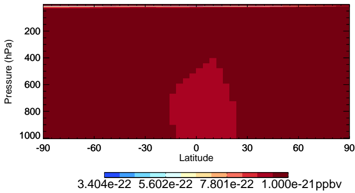
v11-02e-Run0 HCFC123 - Species Zonal Mean for Oct
