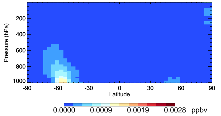
v11-02c-Run0 Br2 - Species Curtain @ -180.000 for Oct
