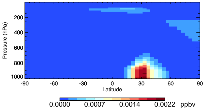
v11-02c-Run0 ASOA2 - Species Zonal Mean for Oct
