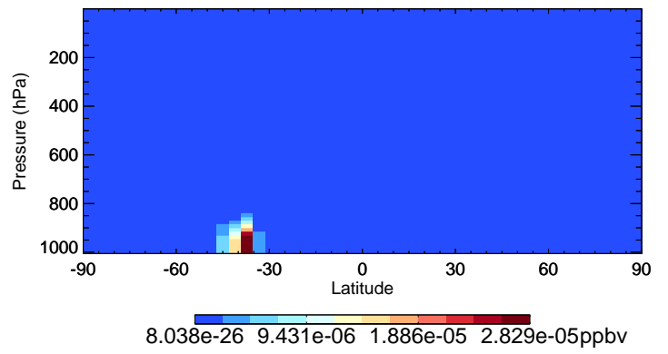
v11-02c-Run0 MOBA - Species Curtain @ -180.000 for Oct
