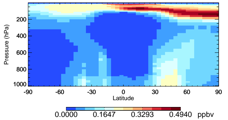
v11-02e-Run0 SO4 - Species Curtain @ -180.000 for Oct
