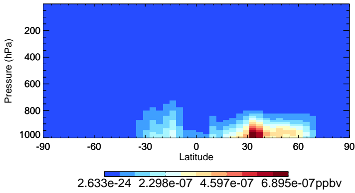
v11-02c-Run0 NPMN - Species Zonal Mean for Oct
