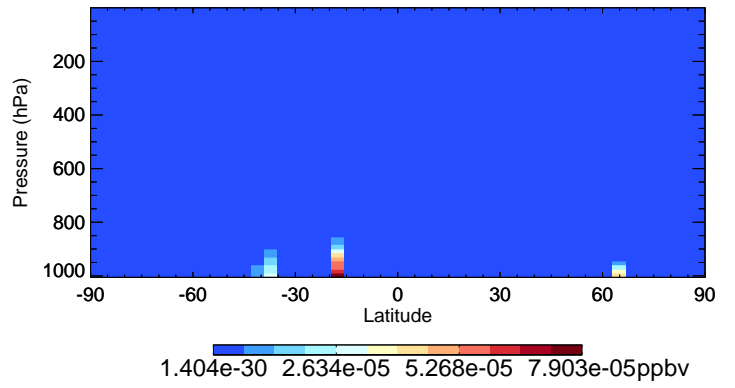
v11-02c-Run0 LIMO - Species Curtain @ -180.000 for Oct
