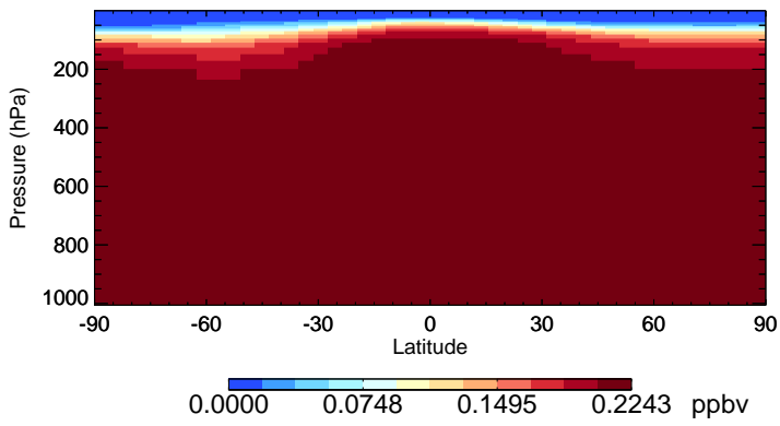
v11-02d-Run1 CFC11 - Species Zonal Mean for Oct
