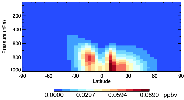
v11-02c-Run0 INDIOL - Species Zonal Mean for Oct
