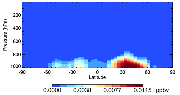
v11-02c-Run0 NITs - Species Curtain @ -180.000 for Oct
