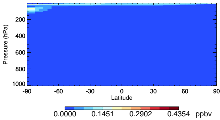
v11-02c-Run0 ClO - Species Zonal Mean for Oct
