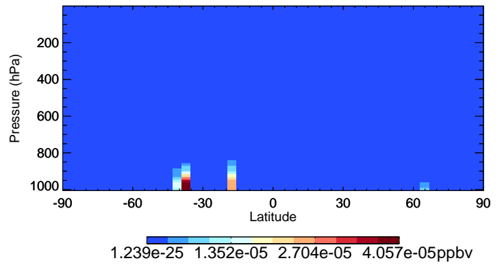
v11-02e-Run0 MONITU - Species Curtain @ -180.000 for Oct
