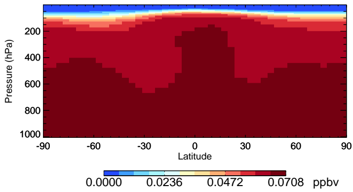
v11-02d-Run1 CCI4 - Species Zonal Mean for Oct
