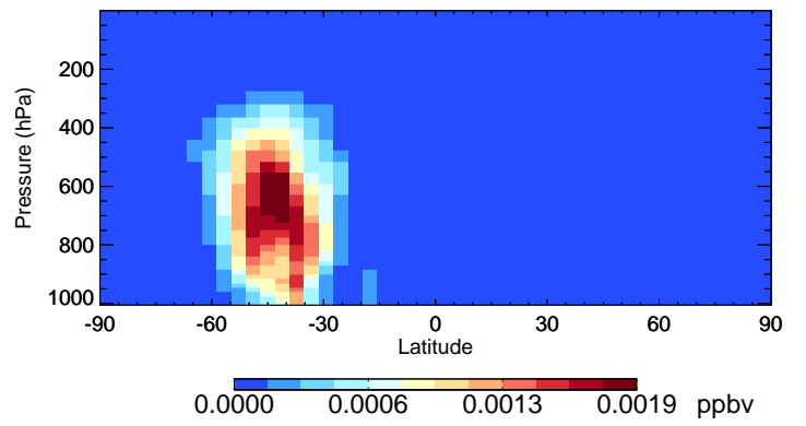
v11-02d-Run1 HC187 - Species Curtain @ -180.000 for Oct
