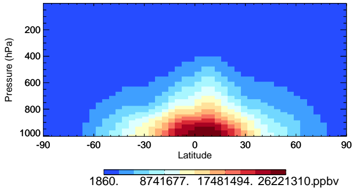
v11-02d-Run1 H2O - Species Zonal Mean for Oct
