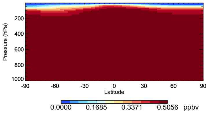
v11-02c-Run0 CFC12 - Species Zonal Mean for Oct
