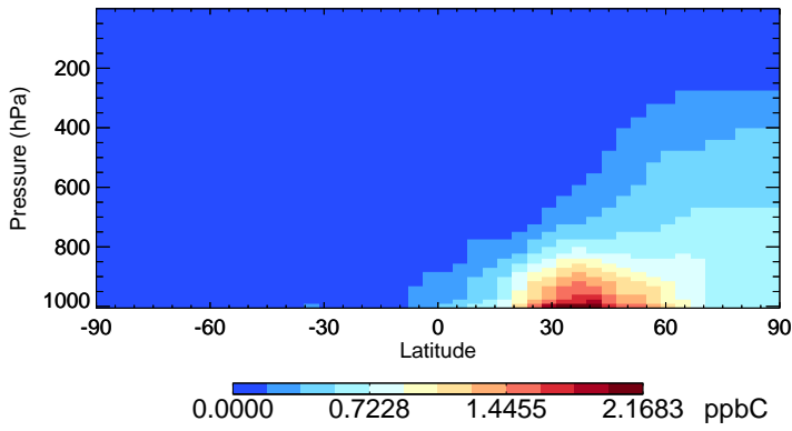
v11-02c-Run0 ALK4 - Species Zonal Mean for Oct
