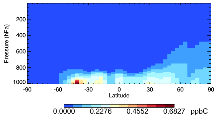
v11-02e-Run0 ALD2 - Species Curtain @ -180.000 for Oct
