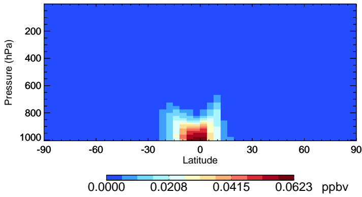
v11-02c-Run0 HPALD - Species Zonal Mean for Oct
