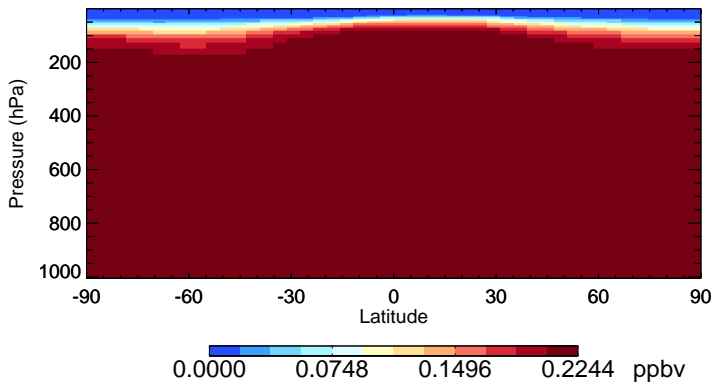
v11-02e-Run0 CFC11 - Species Zonal Mean for Oct
