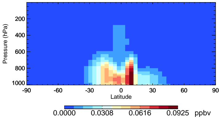
v11-02c-Run0 HAC - Species Zonal Mean for Oct
