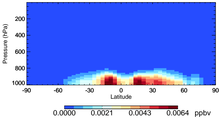
v11-02c-Run0 NITs - Species Zonal Mean for Oct
