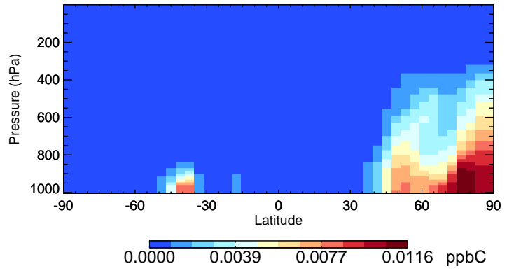
v11-02d-Run1 XYLE - Species Curtain @ -180.000 for Oct
