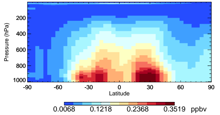
v11-02d-Run1 CH2O - Species Curtain @ -180.000 for Oct
