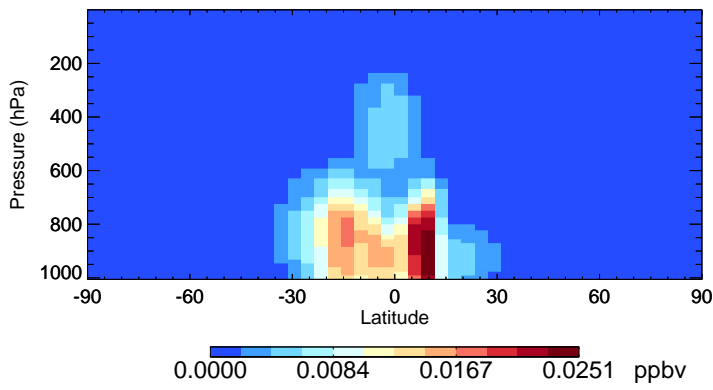
v11-02d-Run1 HC187 - Species Zonal Mean for Oct
