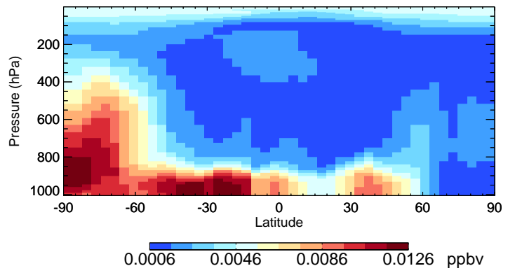
v11-02c-Run0 MSA - Species Curtain @ -180.000 for Oct
