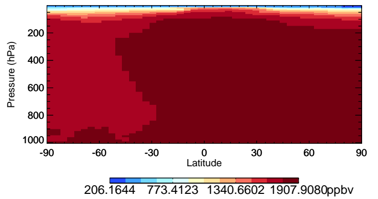
v11-02e-Run0 CH4 - Species Curtain @ -180.000 for Oct
