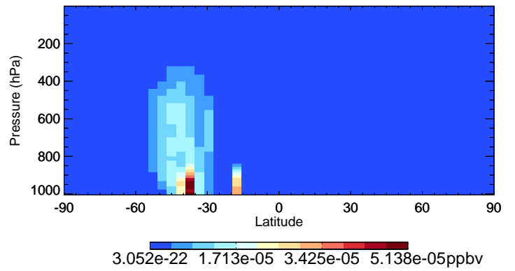
v11-02e-Run0 HCOOH - Species Curtain @ -180.000 for Oct
