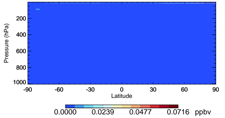
v11-02d-Run1 OCIO - Species Curtain @ -180.000 for Oct
