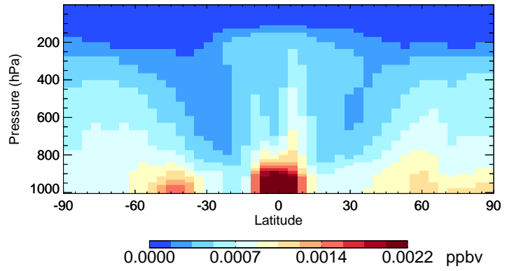
v11-02d-Run1 CHBr3 - Species Curtain @ -180.000 for Oct
