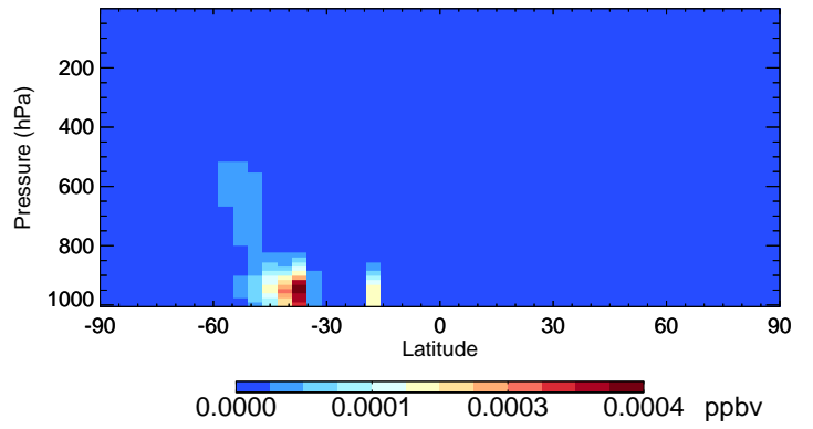
v11-02c-Run0 HPALD - Species Curtain @ -180.000 for Oct
