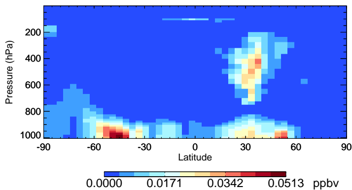
v11-02d-Run1 NIT - Species Curtain @ -180.000 for Oct
