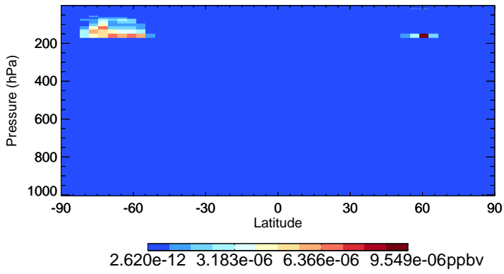
v11-02c-Run0 ClNO 2 - Species Zonal Mean for Oct
