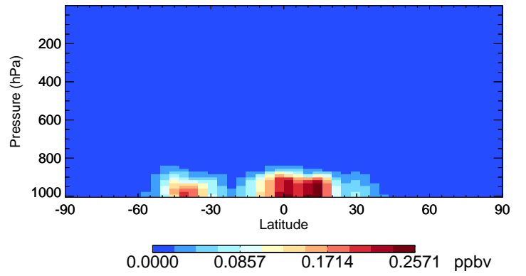
v11-02c-Run0 NH3 - Species Curtain @ -180.000 for Oct
