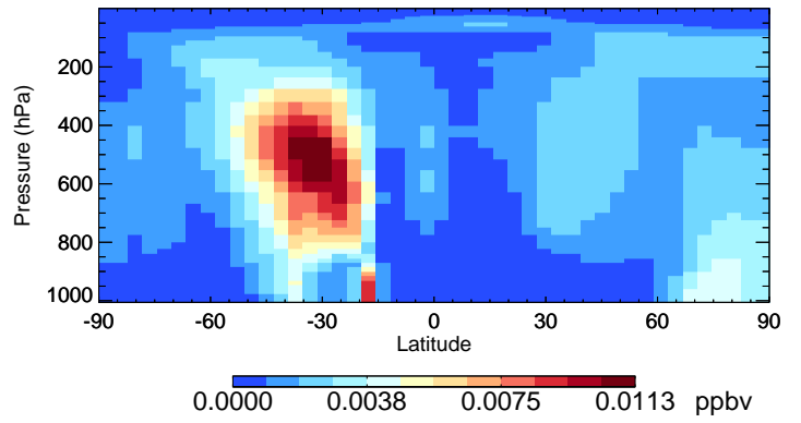
v11-02c-Run0 TSOG2 - Species Curtain @ -180.000 for Oct
