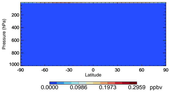
v11-02d-Run1 CI - Species Zonal Mean for Oct
