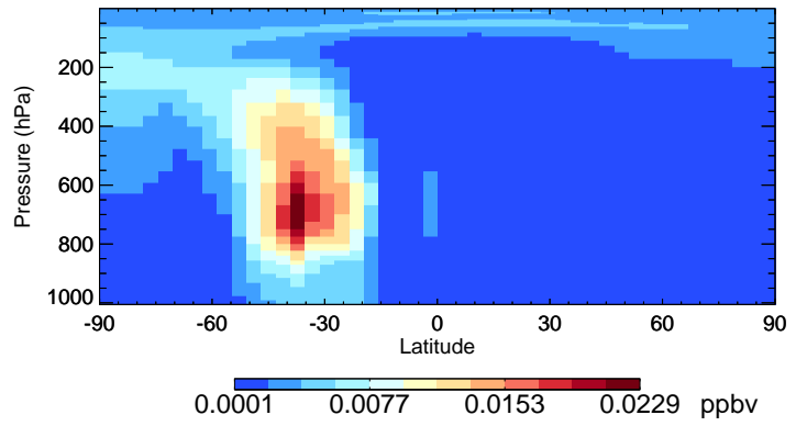
v11-02c-Run0 SOAIE - Species Curtain @ -180.000 for Oct
