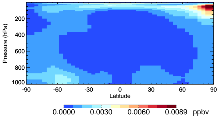
v11-02c-Run0 HOBr - Species Zonal Mean for Oct
