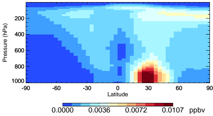
v11-02c-Run0 ASOG3 - Species Zonal Mean for Oct
