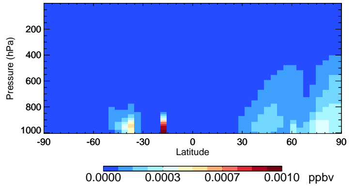
v11-02d-Run1 GLYX - Species Curtain @ -180.000 for Oct
