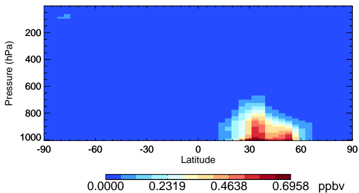
v11-02d-Run1 NIT - Species Zonal Mean for Oct
