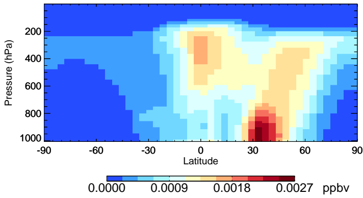
v11-02c-Run0 R4N2 - Species Zonal Mean for Oct
