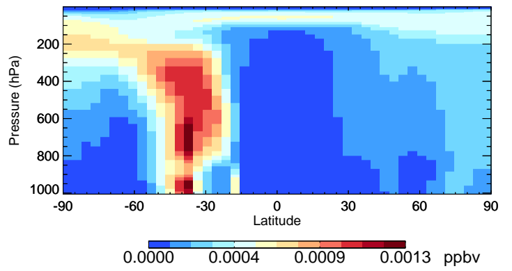
v11-02d-Run1 TSOA0 - Species Curtain @ -180.000 for Oct
