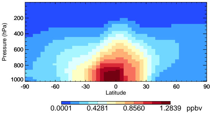
v11-02c-Run0 MP - Species Zonal Mean for Oct
