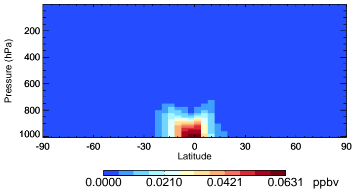
v11-02e-Run0 HPALD - Species Zonal Mean for Oct
