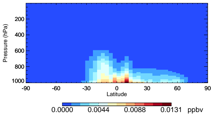
v11-02e-Run0 MONITA - Species Zonal Mean for Oct
