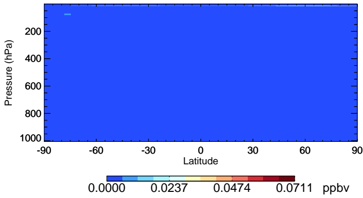
v11-02c-Run0 OCIO - Species Zonal Mean for Oct
