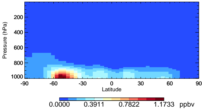
v11-02d-Run1 SALA - Species Zonal Mean for Oct
