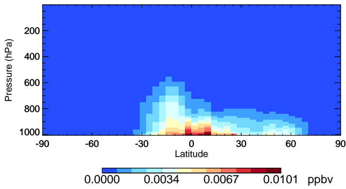
v11-02c-Run0 MONITA - Species Zonal Mean for Oct
