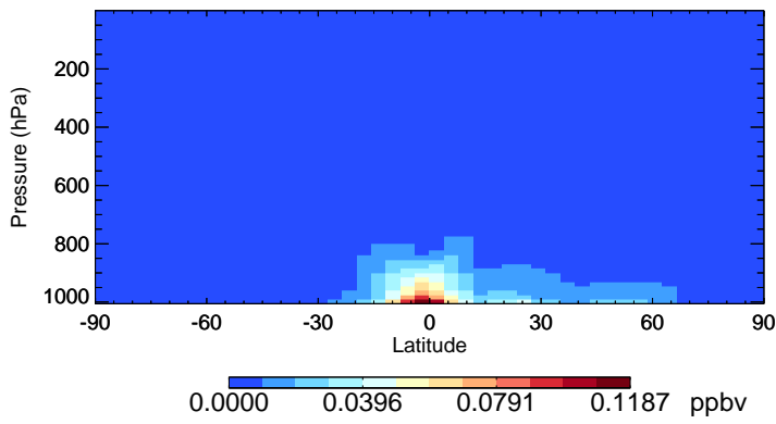
v11-02c-Run0 RCHO - Species Zonal Mean for Oct
