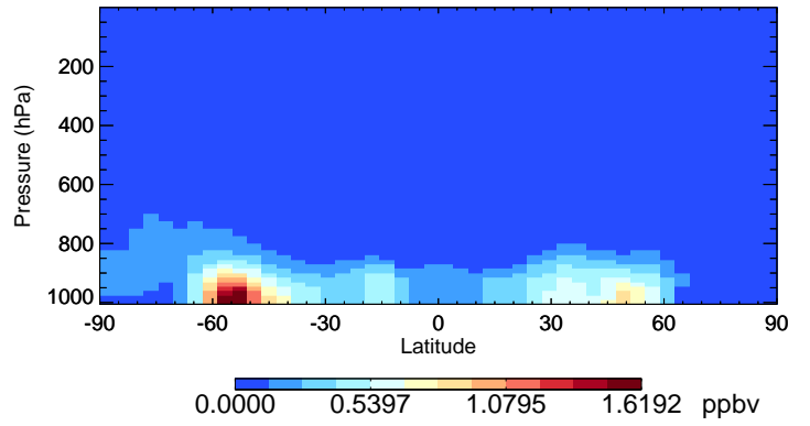
v11-02d-Run1 SALA - Species Curtain @ -180.000 for Oct
