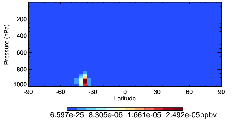
v11-02c-Run0 MACRN - Species Curtain @ -180.000 for Oct
