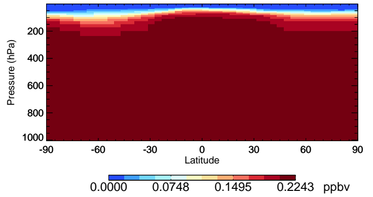
v11-02c-Run0 CFC11 - Species Curtain @ -180.000 for Oct
