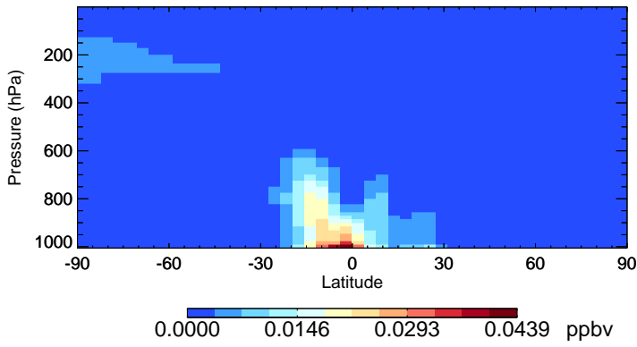
v11-02c-Run0 TSOA2 - Species Zonal Mean for Oct
