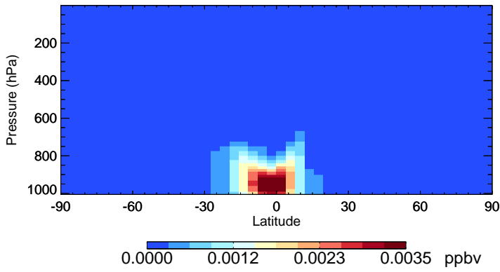
v11-02c-Run0 RIPD - Species Zonal Mean for Oct
