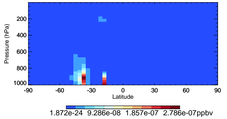
v11-02c-Run0 LVOC - Species Curtain @ -180.000 for Oct
