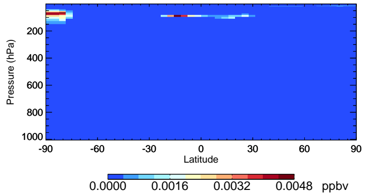
v11-02c-Run0 Cl2 - Species Curtain @ -180.000 for Oct
