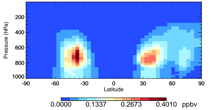
v11-02d-Run1 DST1 - Species Curtain @ -180.000 for Oct
