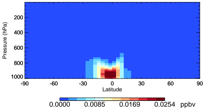
v11-02c-Run0 RIPB - Species Zonal Mean for Oct
