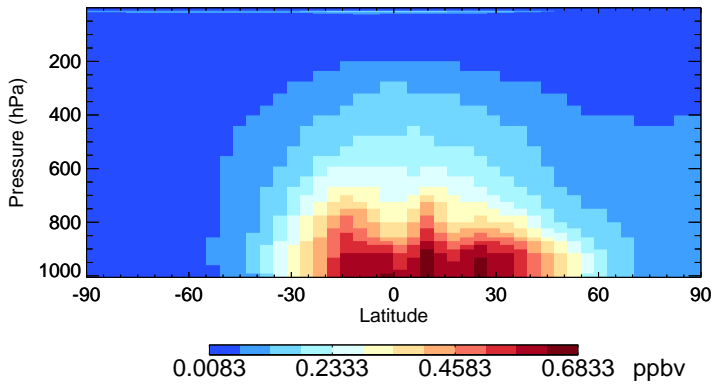
v11-02c-Run0 CH2O - Species Zonal Mean for Oct
