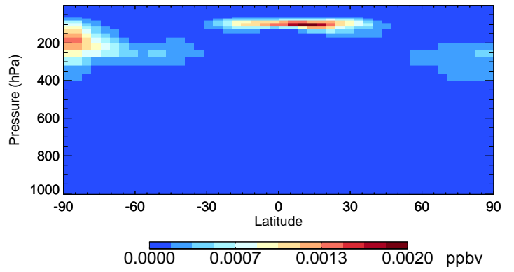
v11-02c-Run0 ASOA3 - Species Curtain @ -180.000 for Oct
