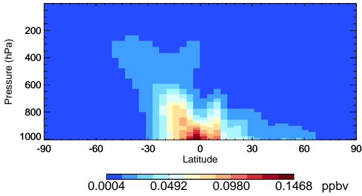
v11-02d-Run1 TSOG3 - Species Zonal Mean for Oct
