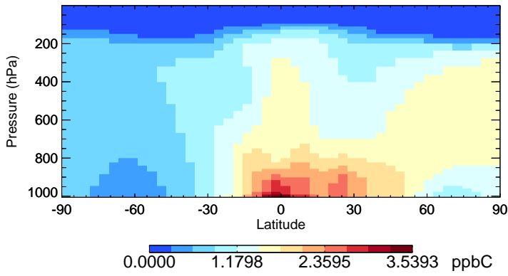
v11-02c-Run0 ACET - Species Zonal Mean for Oct
