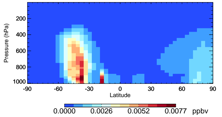
v11-02c-Run0 HAC - Species Curtain @ -180.000 for Oct
