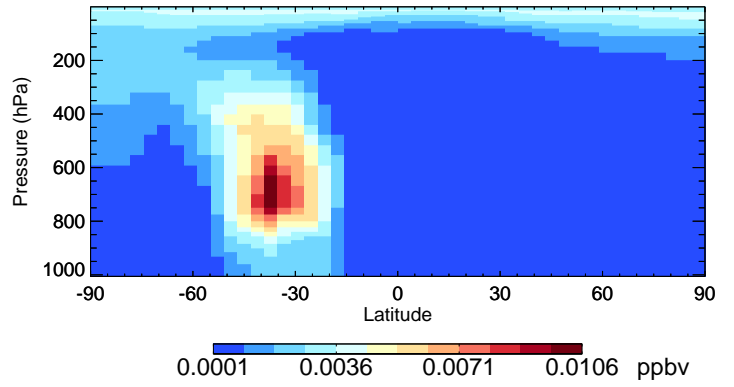
v11-02d-Run1 SOAIE - Species Curtain @ -180.000 for Oct
