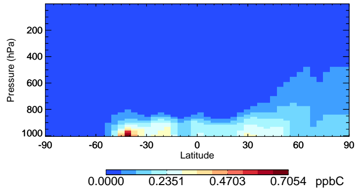
v11-02c-Run0 ALD2 - Species Curtain @ -180.000 for Oct
