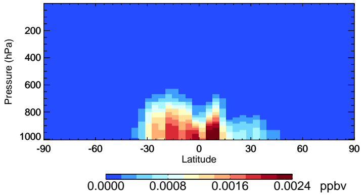
v11-02d-Run1 ISOPNB - Species Zonal Mean for Oct
