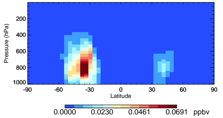
v11-02c-Run0 DST4 - Species Curtain @ -180.000 for Oct
