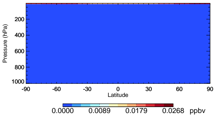
v11-02e-Run0 CI - Species Zonal Mean for Oct
