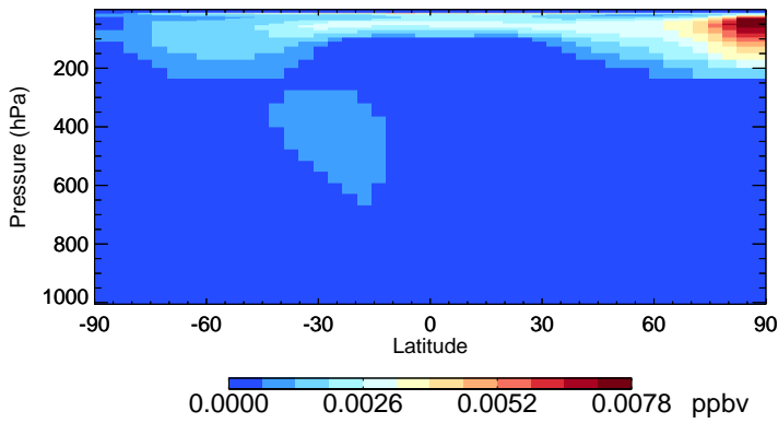
v11-02e-Run0 HOBr - Species Zonal Mean for Oct
