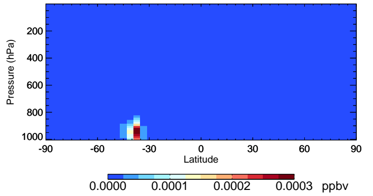
v11-02c-Run0 ISOPNB - Species Curtain @ -180.000 for Oct
