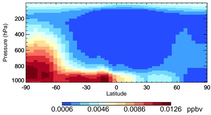
v11-02c-Run0 MSA - Species Zonal Mean for Oct
