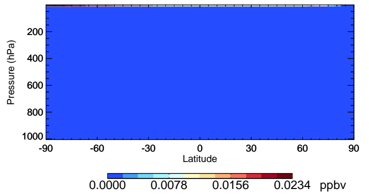
v11-02c-Run0 Br - Species Curtain @ -180.000 for Oct
