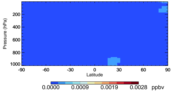
v11-02d-Run1 Br2 - Species Curtain @ -180.000 for Oct
