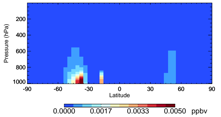
v11-02d-Run1 SOAP - Species Curtain @ -180.000 for Oct
