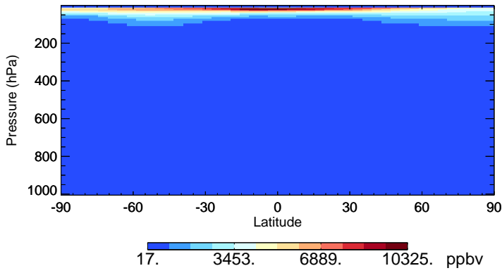
v11-02c-Run0 O3 - Species Zonal Mean for Oct
