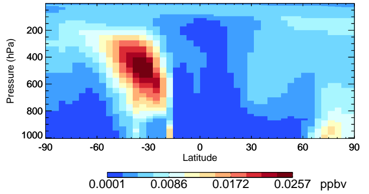
v11-02d-Run1 TSOG3 - Species Curtain @ -180.000 for Oct
