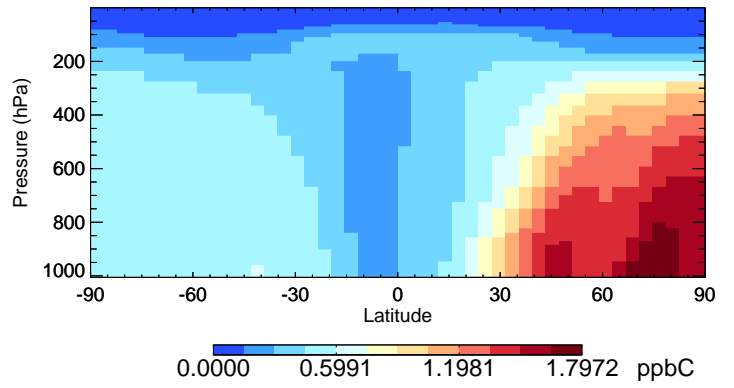
v11-02c-Run0 C2H6 - Species Curtain @ -180.000 for Oct
