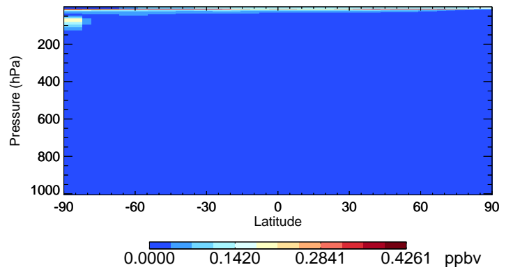
v11-02c-Run0 ClO - Species Curtain @ -180.000 for Oct
