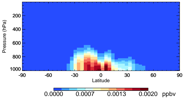
v11-02c-Run0 ISOPNB - Species Zonal Mean for Oct
