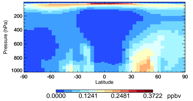
v11-02c-Run0 SO4 - Species Curtain @ -180.000 for Oct
