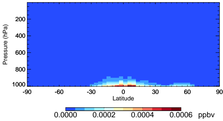
v11-02c-Run0 MONITU - Species Zonal Mean for Oct
