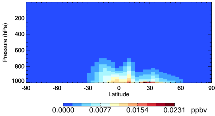
v11-02d-Run1 GLYX - Species Zonal Mean for Oct
