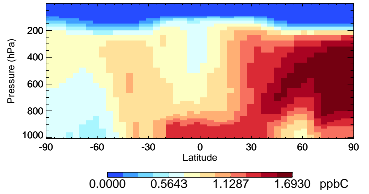
v11-02c-Run0 ACET - Species Curtain @ -180.000 for Oct
