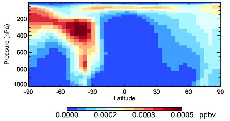
v11-02d-Run1 TSOA1 - Species Curtain @ -180.000 for Oct
