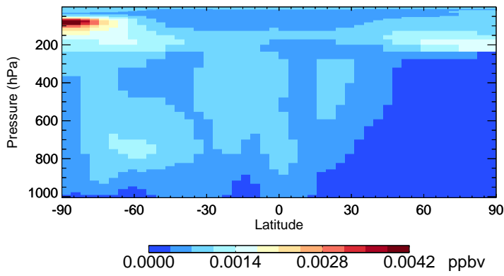
v11-02c-Run0 HBr - Species Zonal Mean for Oct
