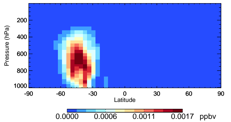
v11-02e-Run0 HC187 - Species Curtain @ -180.000 for Oct
