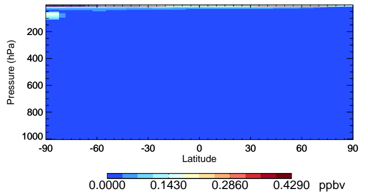
v11-02d-Run1 ClO - Species Curtain @ -180.000 for Oct
