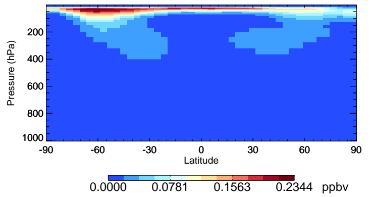
v11-02c-Run0 HNO4 - Species Curtain @ -180.000 for Oct
