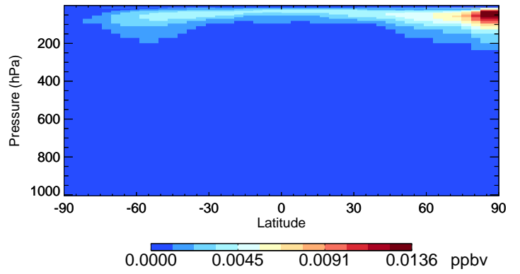
v11-02c-Run0 BrCl - Species Curtain @ -180.000 for Oct
