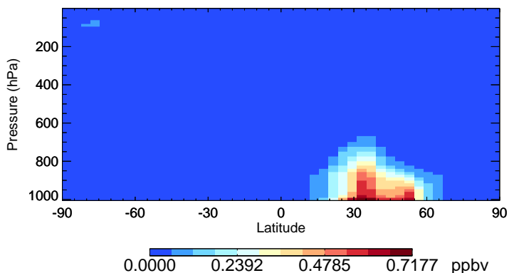
v11-02c-Run0 NIT - Species Zonal Mean for Oct
