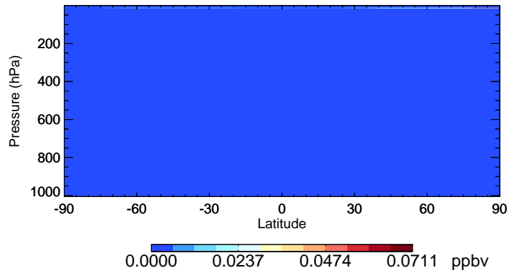
v11-02c-Run0 OCIO - Species Curtain @ -180.000 for Oct
