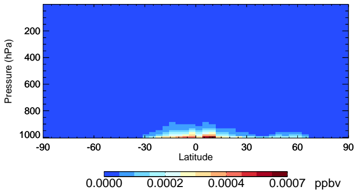
v11-02e-Run0 MONITU - Species Zonal Mean for Oct
