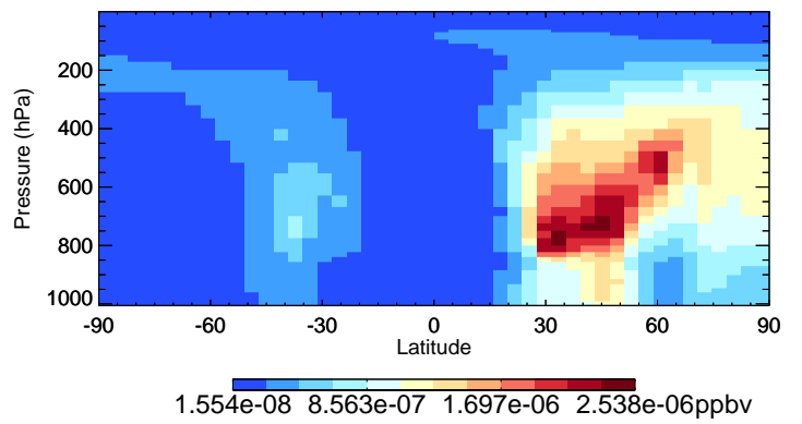
v11-02e-Run0 SOAMG - Species Curtain @ -180.000 for Oct
