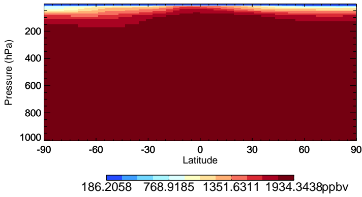
v11-02c-Run0 CH4 - Species Zonal Mean for Oct
