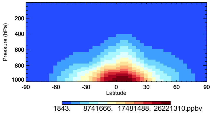
v11-02e-Run0 H2O - Species Zonal Mean for Oct
