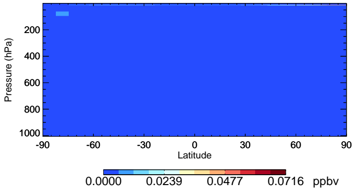
v11-02d-Run1 OCIO - Species Zonal Mean for Oct
