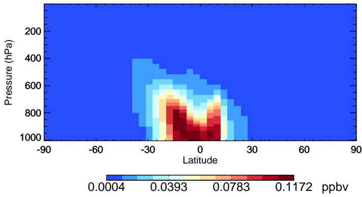
v11-02c-Run0 SOAIE - Species Zonal Mean for Oct
