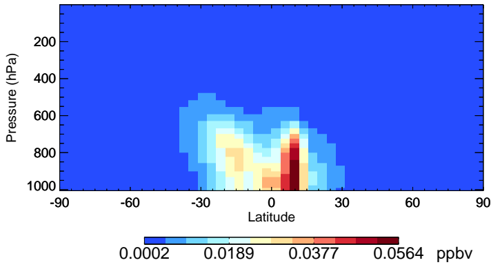
v11-02d-Run1 SOAIE - Species Zonal Mean for Oct
