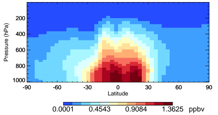
v11-02c-Run0 MP - Species Curtain @ -180.000 for Oct
