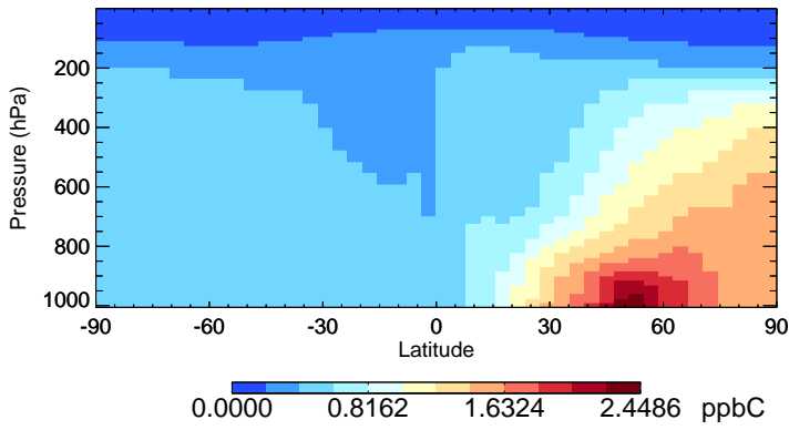
v11-02c-Run0 C2H6 - Species Zonal Mean for Oct
