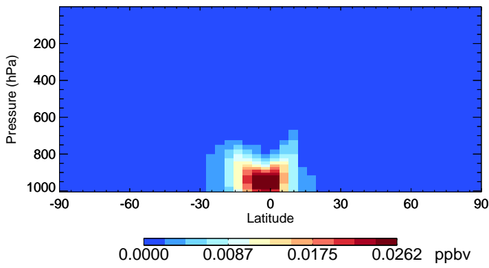
v11-02d-Run1 RIPB - Species Zonal Mean for Oct
