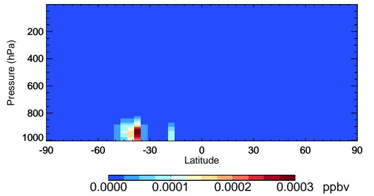
v11-02e-Run0 RIPB - Species Curtain @ -180.000 for Oct
