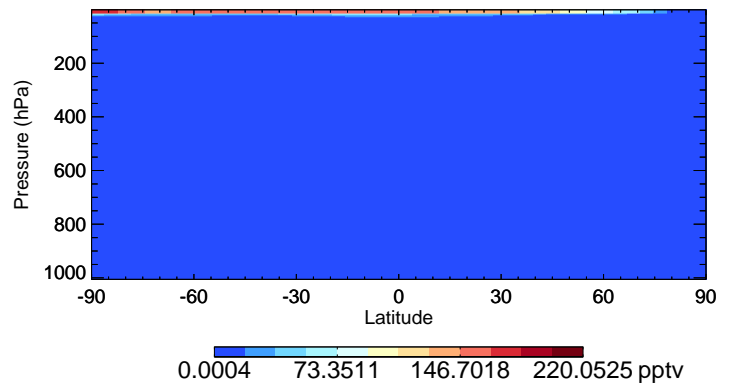
v11-02c-Run0 HO2 - Species Curtain @ -180.000 for Oct
