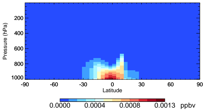
v11-02c-Run0 MOBA - Species Zonal Mean for Oct
