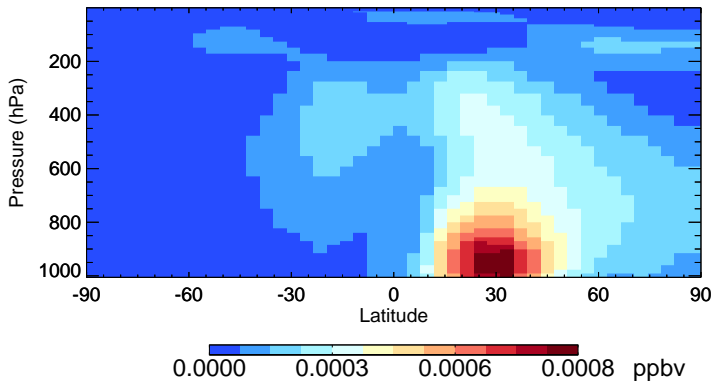
v11-02c-Run0 ASOG1 - Species Zonal Mean for Oct
