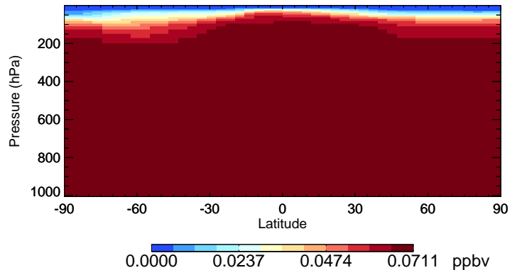
v11-02c-Run0 CFC113 - Species Curtain @ -180.000 for Oct
