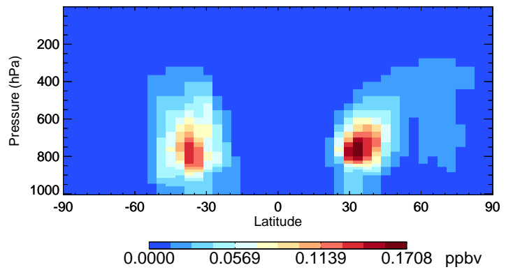
v11-02c-Run0 DST2 - Species Curtain @ -180.000 for Oct
