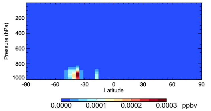
v11-02d-Run1 RIPB - Species Curtain @ -180.000 for Oct
