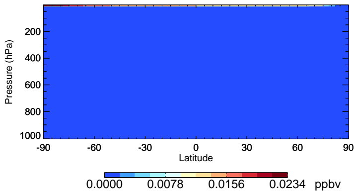
v11-02c-Run0 Br - Species Zonal Mean for Oct
