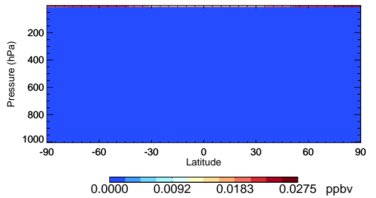
v11-02e-Run0 CI - Species Curtain @ -180.000 for Oct
