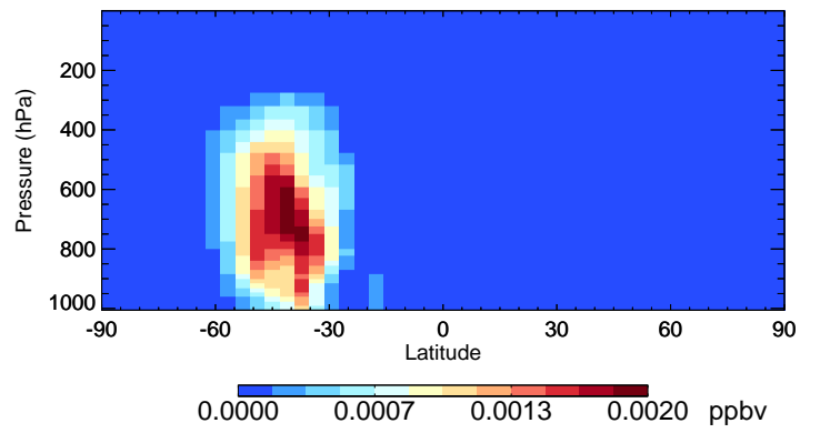
v11-02c-Run0 HC187 - Species Curtain @ -180.000 for Oct
