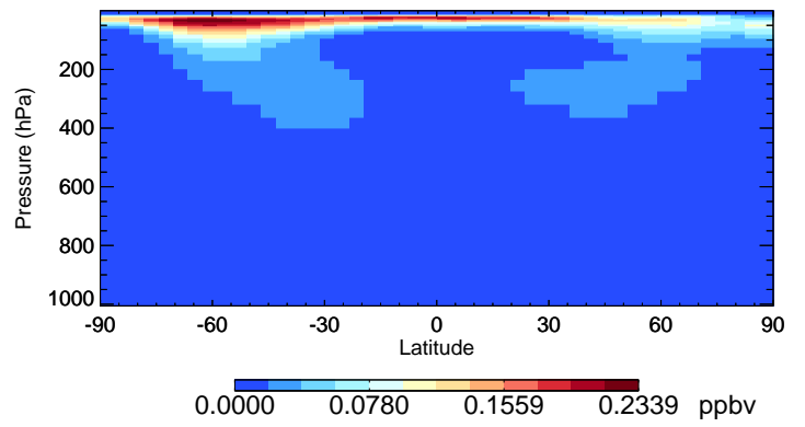
v11-02d-Run1 HNO4 - Species Curtain @ -180.000 for Oct
