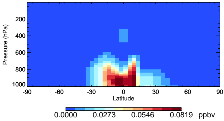
v11-02c-Run0 GLYC - Species Zonal Mean for Oct
