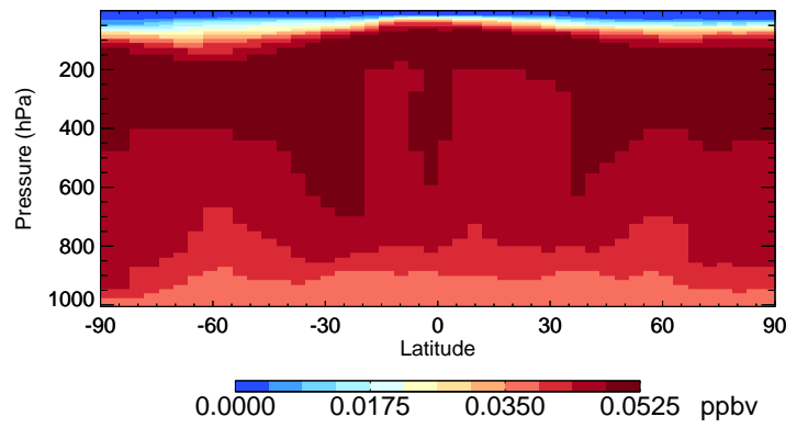
v11-02c-Run0 HCFC141b - Species Curtain @ -180.000 for Oct
