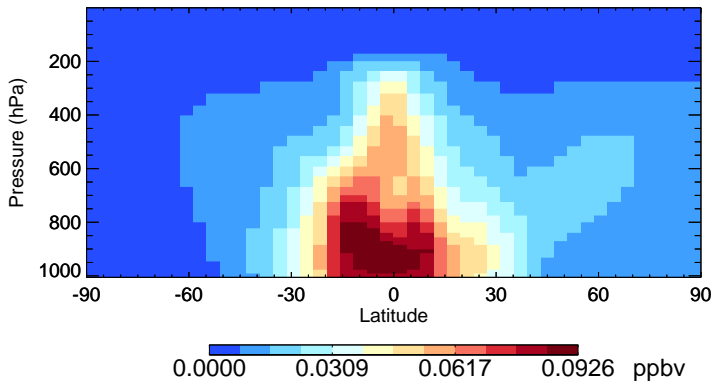
v11-02c-Run0 MAP - Species Zonal Mean for Oct
