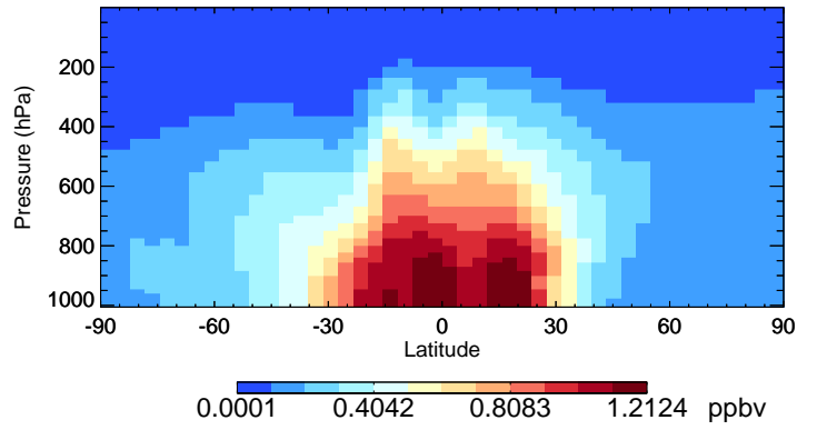
v11-02d-Run1 MP - Species Curtain @ -180.000 for Oct
