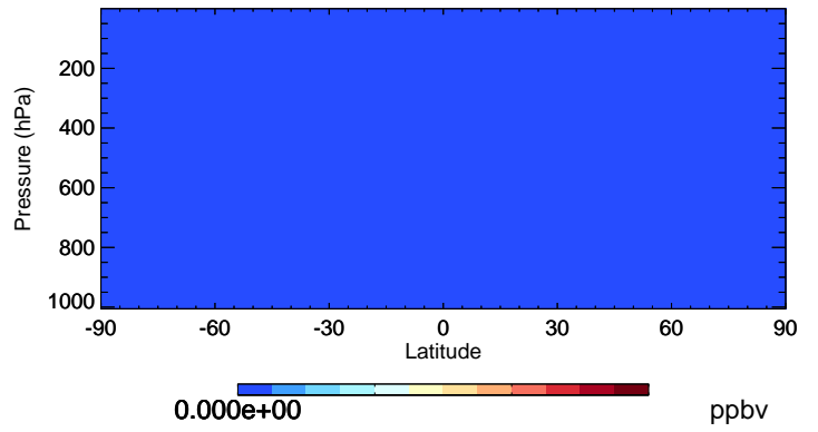
v11-02c-Run0 HCFC123 - Species Curtain @ -180.000 for Oct
