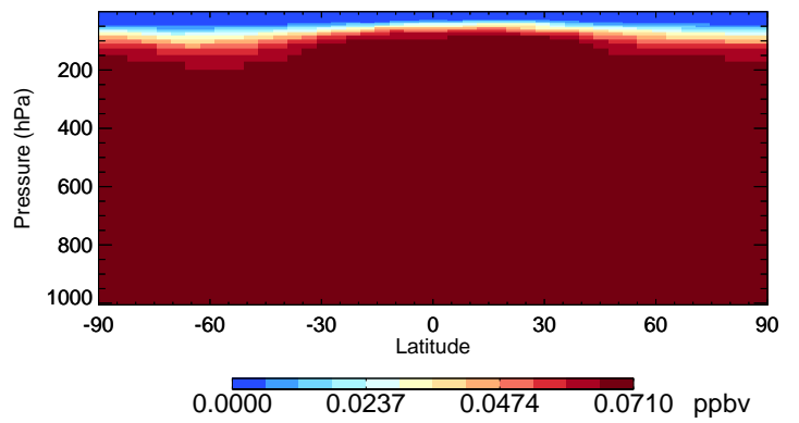
v11-02e-Run0 CCI4 - Species Curtain @ -180.000 for Oct
