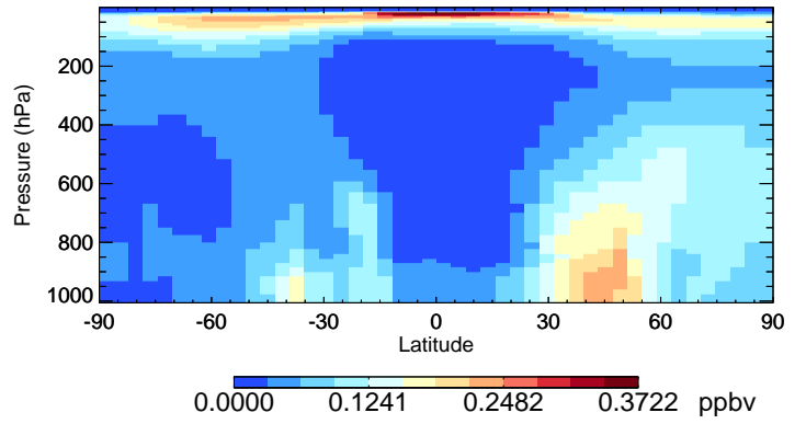
v11-02d-Run1 SO4 - Species Curtain @ -180.000 for Oct
