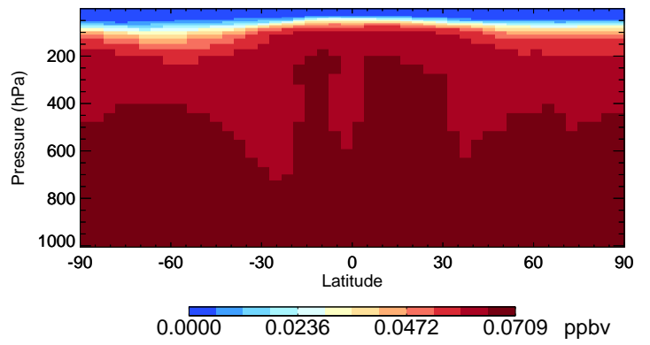
v11-02d-Run1 CCI4 - Species Curtain @ -180.000 for Oct
