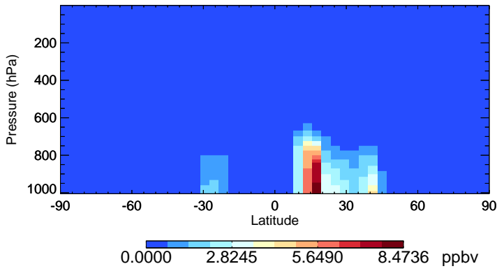
v11-02c-Run0 DST4 - Species Zonal Mean for Oct
