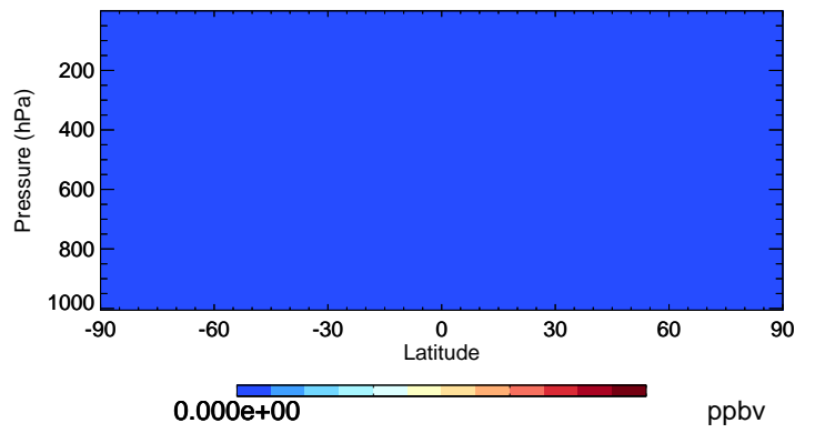
v11-02d-Run1 HCFC123 - Species Curtain @ -180.000 for Oct
