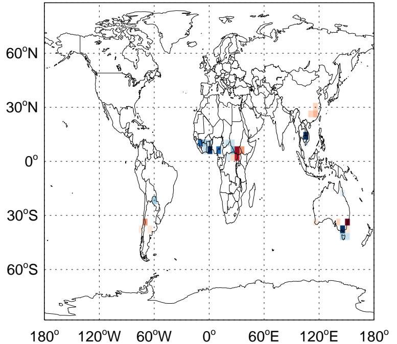
ALK4 biomass emissions for Jan
