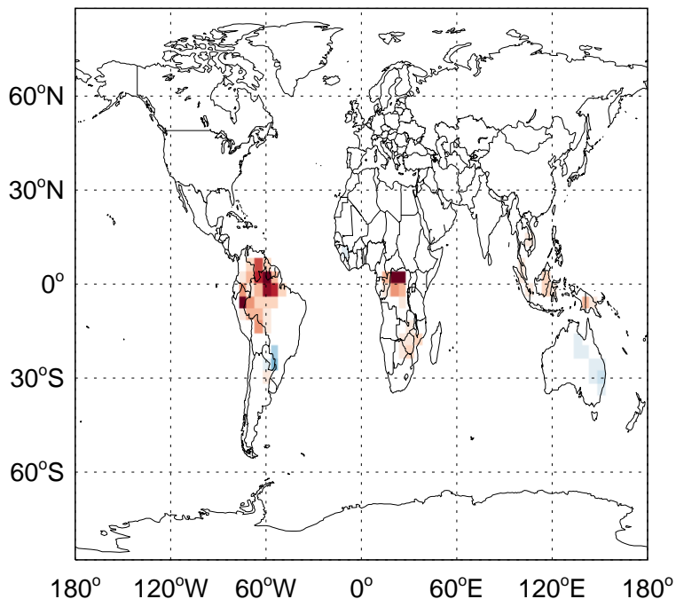
v11-02e-Run1 - v11-02e-Run0 CO from MONOT emissions for Jan
