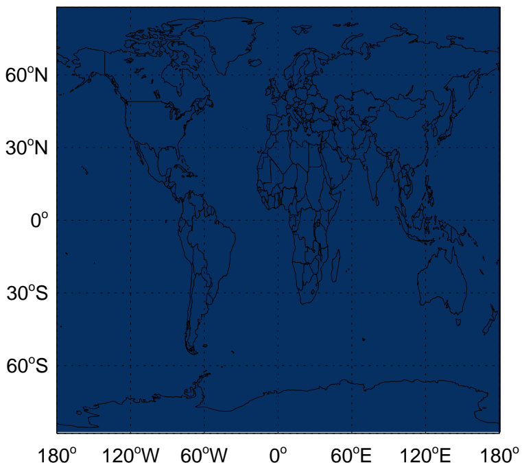
v11-02e-Run1 - v11-02d-Run1 CO ship emissions for Jan
