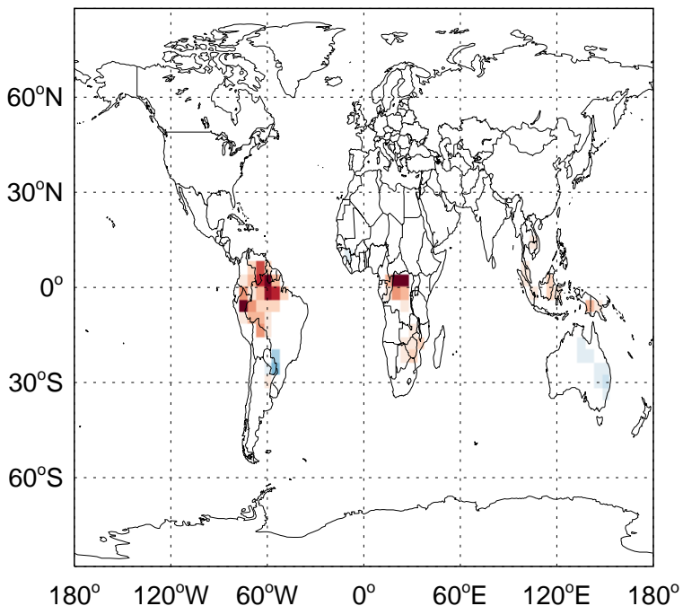
v11-02e-Run1 - v11-02d-Run1 CO from MONOT emissions for Jan
