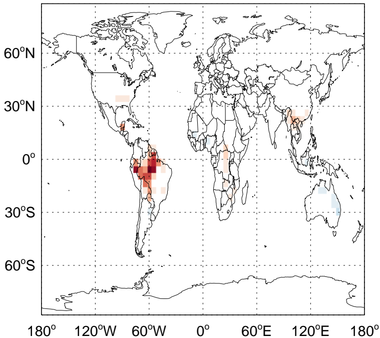
v11-02e-Run1 - v11-02d-Run1 CO from MONOT emissions for Oct
