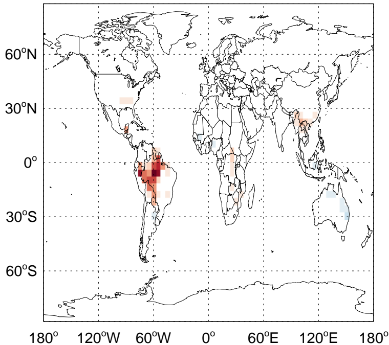
v11-02e-Run1 - v11-02e-Run0 CO from MONOT emissions for Oct
