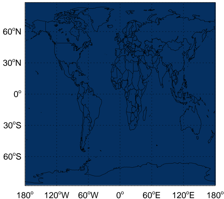
v11-02e-Run1 - v11-02e-Run0 CO ship emissions for Oct
