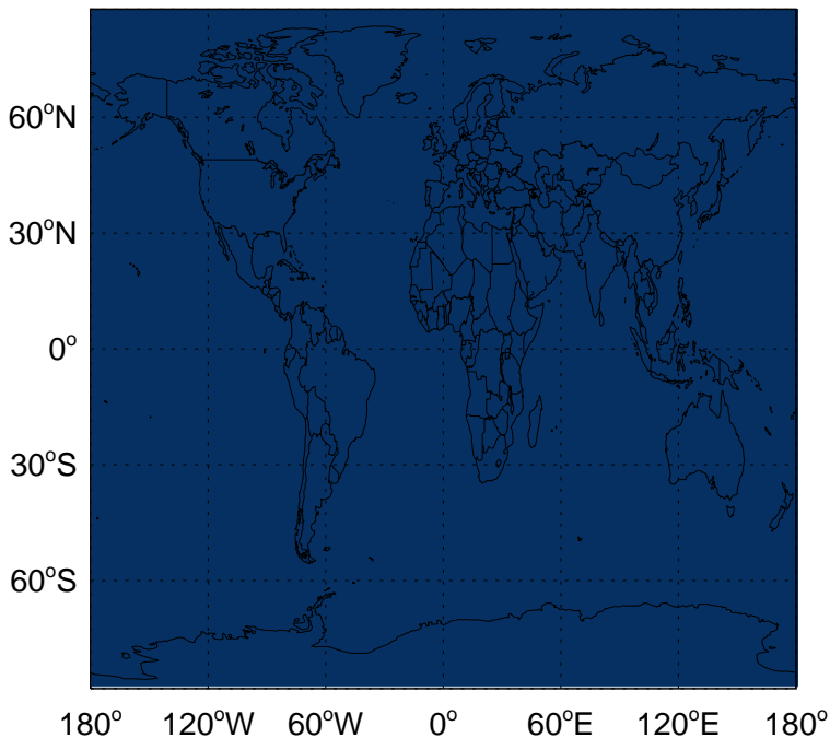
v11-02e-Run1 - v11-02d-Run1 CO ship emissions for Oct
