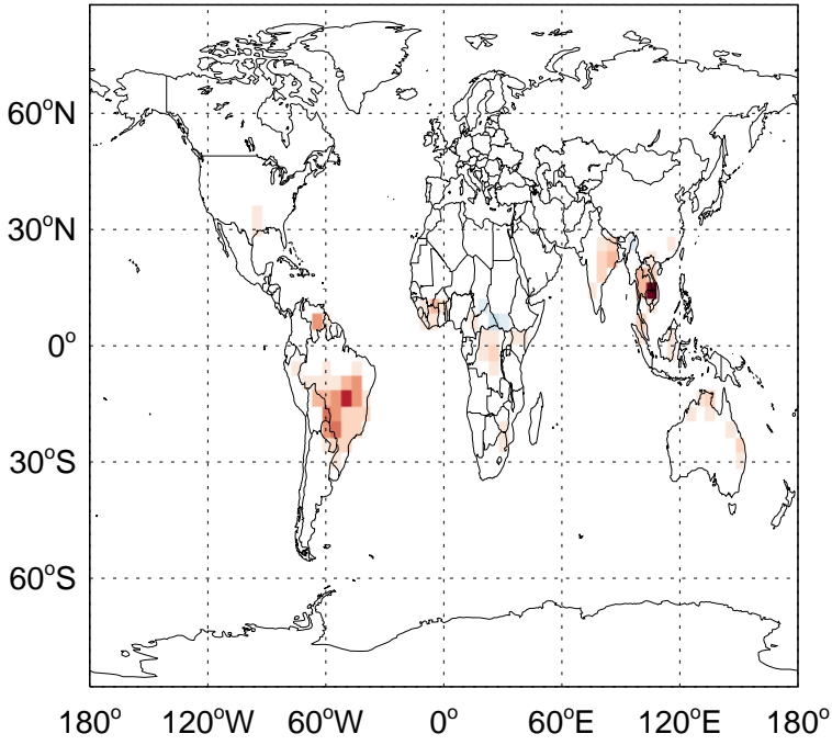
v11-02e-Run1 - v11-02d-Run1 PRPE biogenic emissions for Apr
