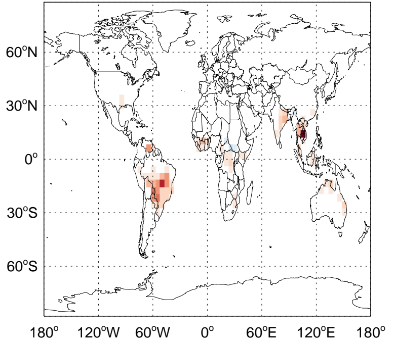
v11-02e-Run1 - v11-02e-Run0 PRPE biogenic emissions for Apr
