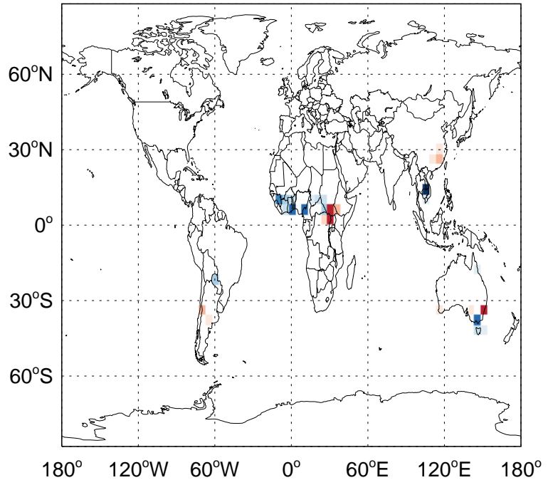
v11-02e-Run1 - v11-02e-Run0 SO2 biomass emissions for Jan
