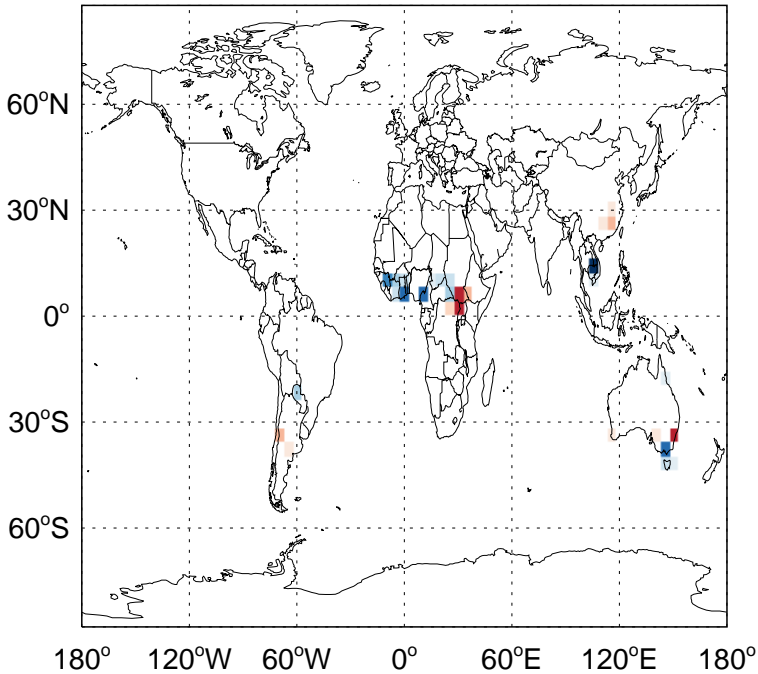
v11-02e-Run1 - v11-02d-Run1 SO2 biomass emissions for Jan
