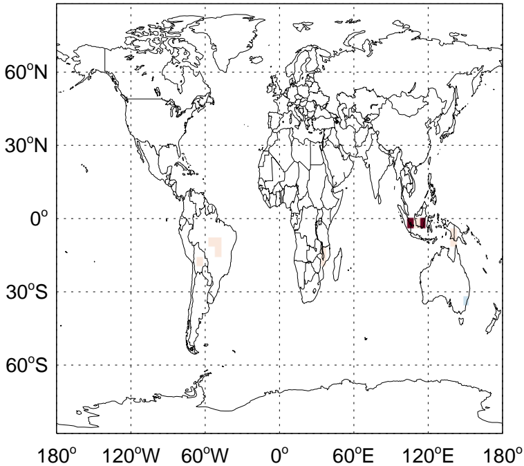
v11-02e-Run1 - v11-02d-Run1 SO2 biomass emissions for Oct
