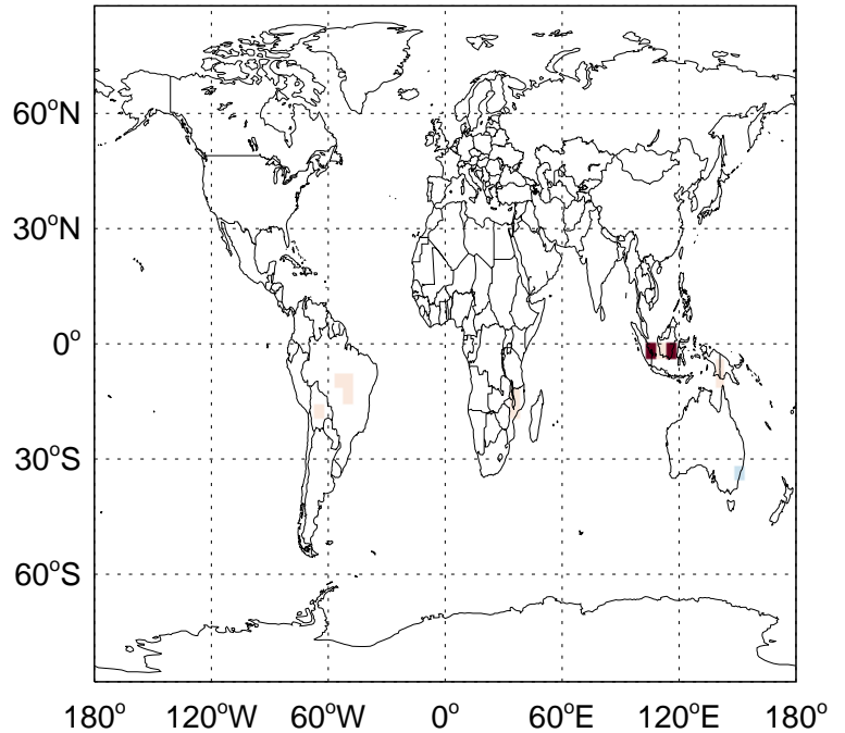
v11-02e-Run1 - v11-02e-Run0 SO2 biomass emissions for Oct
