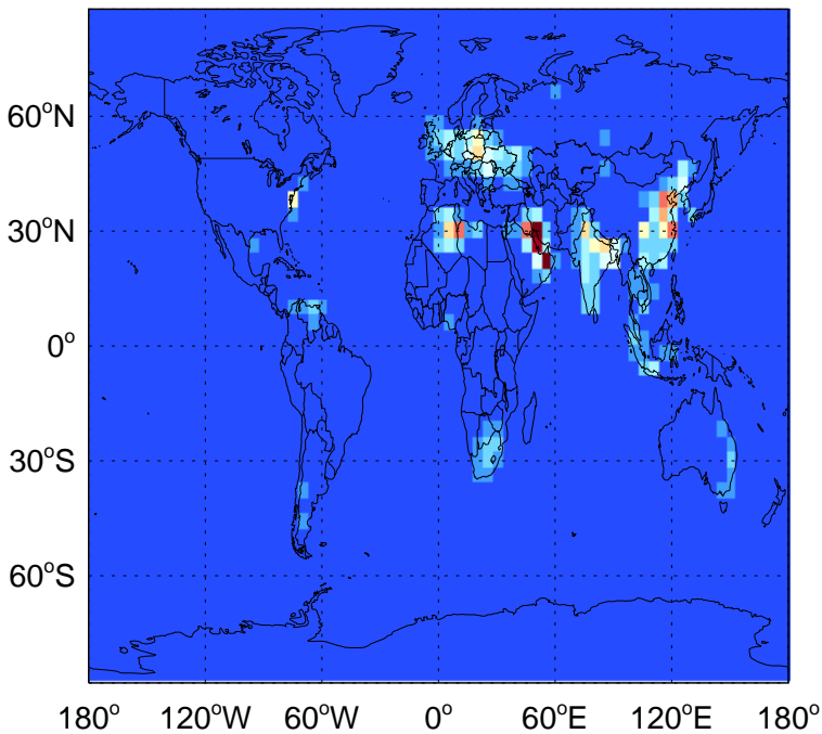
C3H8 column anth+biofl emissions for Oct
