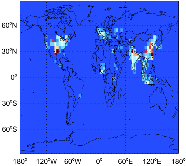
CH2O column anth+biof emissions for Jan
