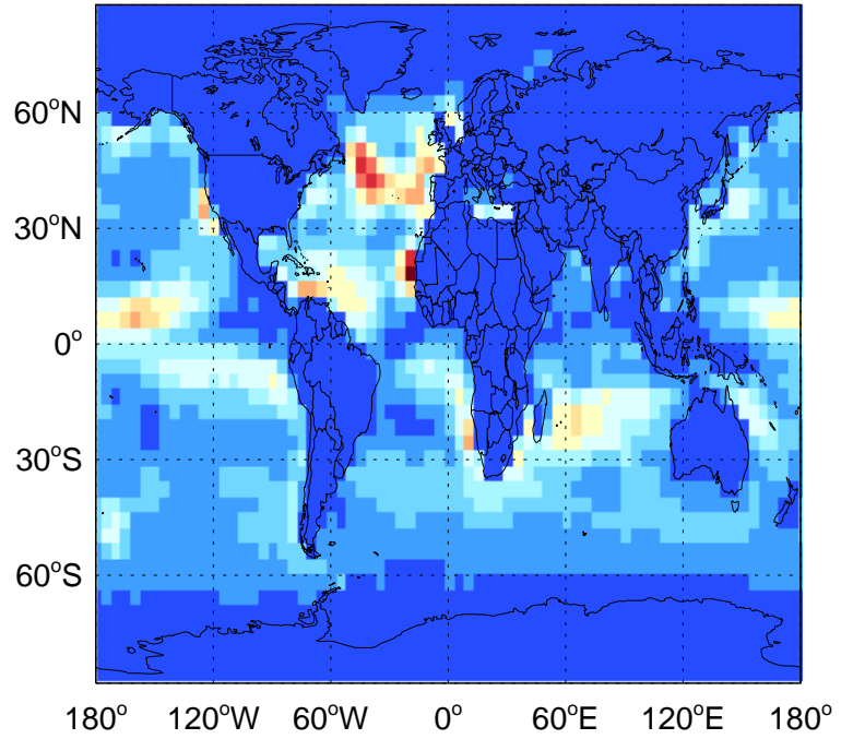
DMS biogenic emissions for Apr
