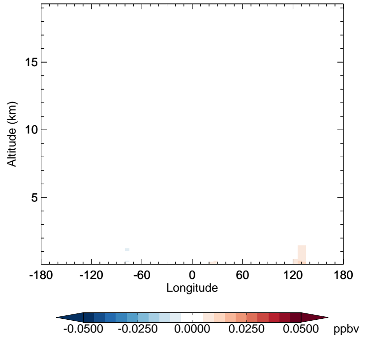
v11-02e-Run1 - v11-02e-Run0 RCHO - Diff along 42N for Apr
