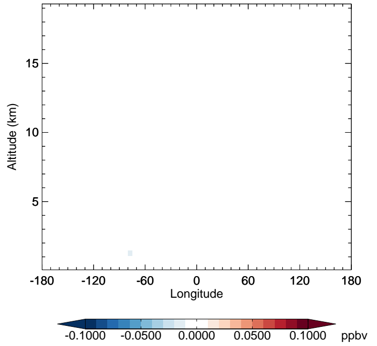
v11-02e-Run1 - v11-02e-Run0 IMAE - Diff along 42N for Apr
