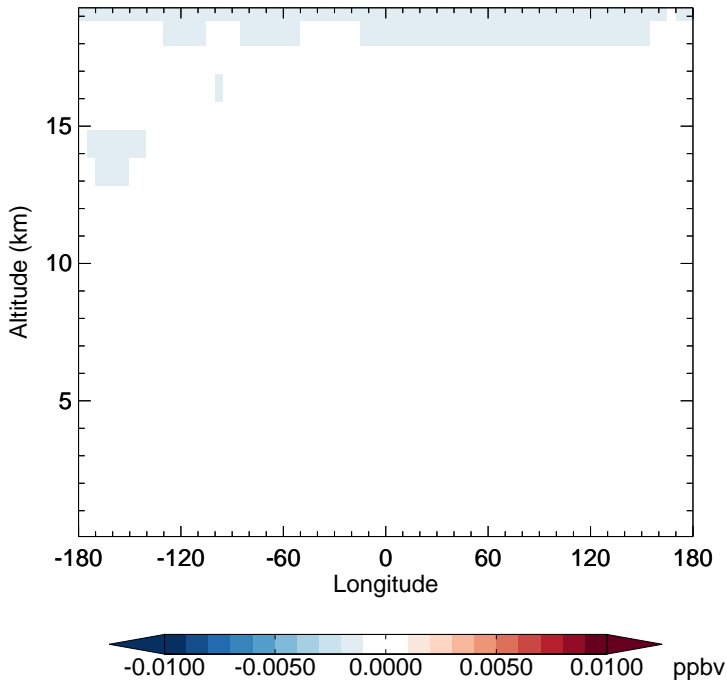
v11-02e-Run1 - v11-02d-Run1 BrNO3 - Diff along 15S for Apr
