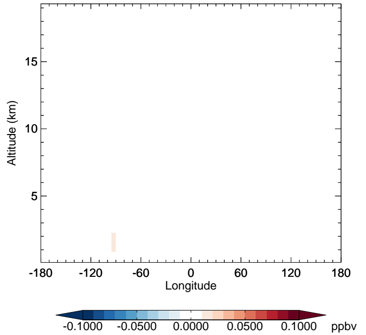
v11-02e-Run1 - v11-02d-Run1 SOAIE - Diff along 42N for Apr
