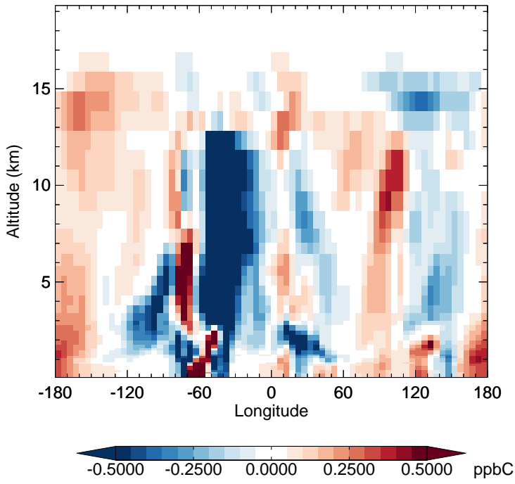
v11-02e-Run1 - v11-02e-Run0 ACET - Diff along 15S for Apr
