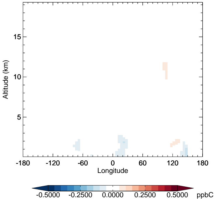
v11-02e-Run1 - v11-02e-Run0 C3H8 - Diff along 15S for Apr
