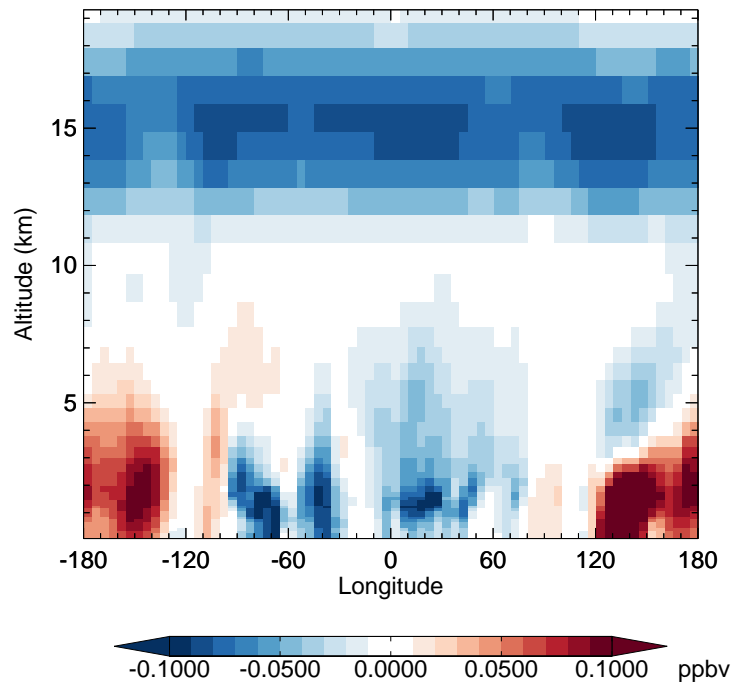
v11-02e-Run1 - v11-02d-Run1 PAN - Diff along 42N for Apr
