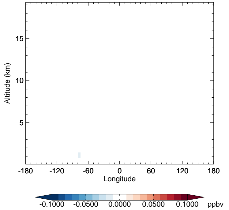
v11-02e-Run1 - v11-02e-Run0 IONITA - Diff along 42N for Apr
