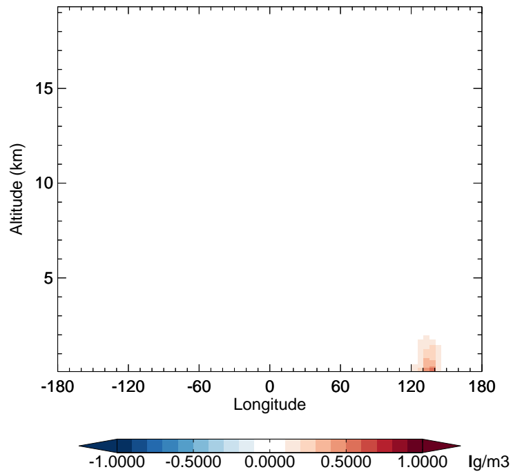
v11-02e-Run1 - v11-02d-Run1 OCPO - Diff along 42N for Apr
