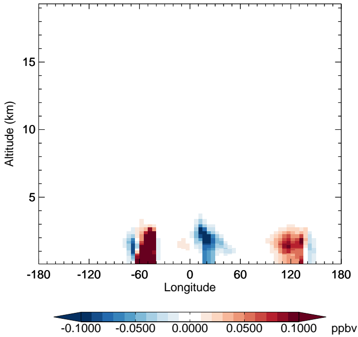
v11-02e-Run1 - v11-02d-Run1 TSOG3 - Diff along 15S for Apr
