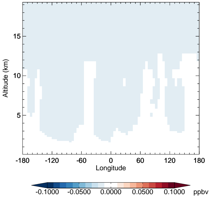
v11-02e-Run1 - v11-02d-Run1 HCFC141b - Diff along 15S for Apr
