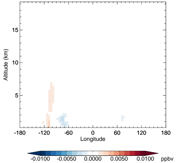
v11-02e-Run1 - v11-02d-Run1 R4N2 - Diff along 42N for Apr
