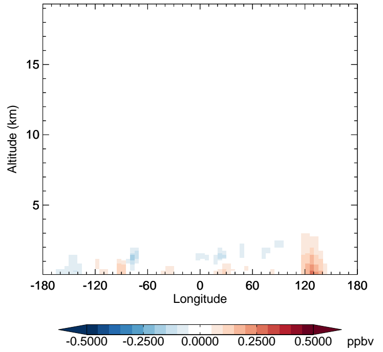
v11-02e-Run1 - v11-02e-Run0 CH 2 O - Diff along 42N for Apr
