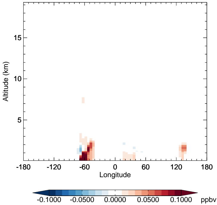
v11-02e-Run1 - v11-02d-Run1 HPALD - Diff along 15S for Apr
