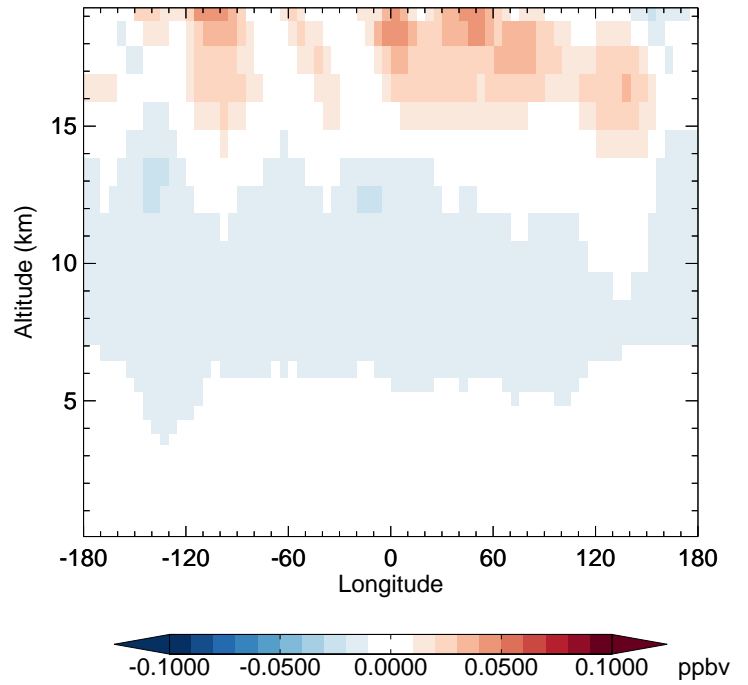
v11-02e-Run1 - v11-02d-Run1 OCS - Diff along 42N for Apr
