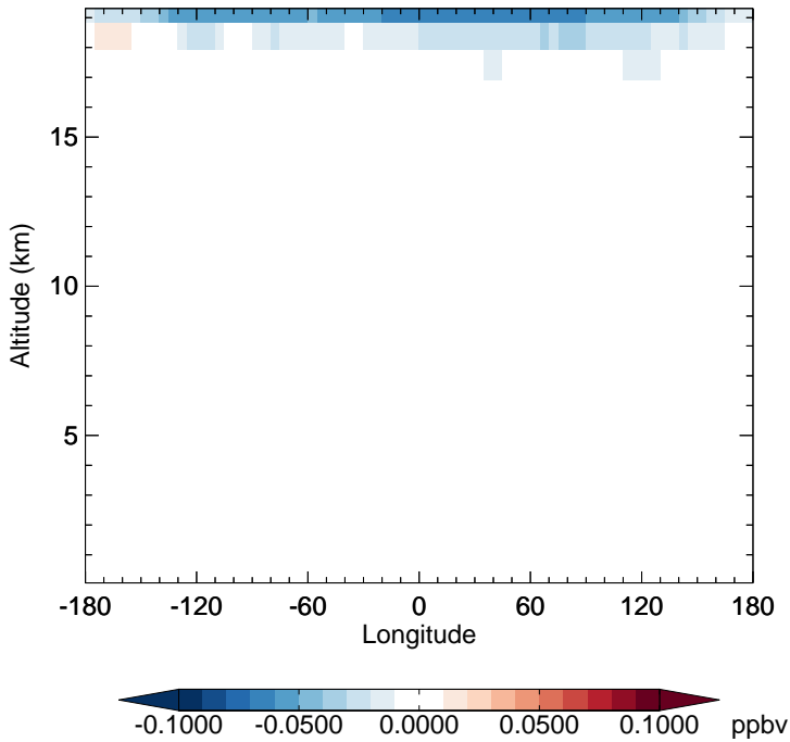
v11-02e-Run1 - v11-02d-Run1 CINO3 - Diff along 15S for Apr
