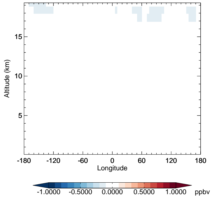
v11-02e-Run1 - v11-02d-Run1 NO - Diff along 42N for Apr
