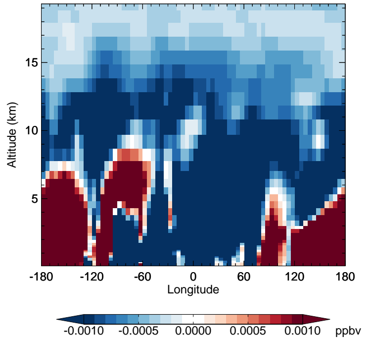
v11-02e-Run1 - v11-02e-Run0 PPN - Diff along 42N for Apr
