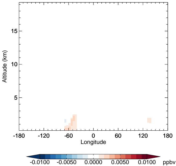
v11-02e-Run1 - v11-02d-Run1 MOBA - Diff along 15S for Apr
