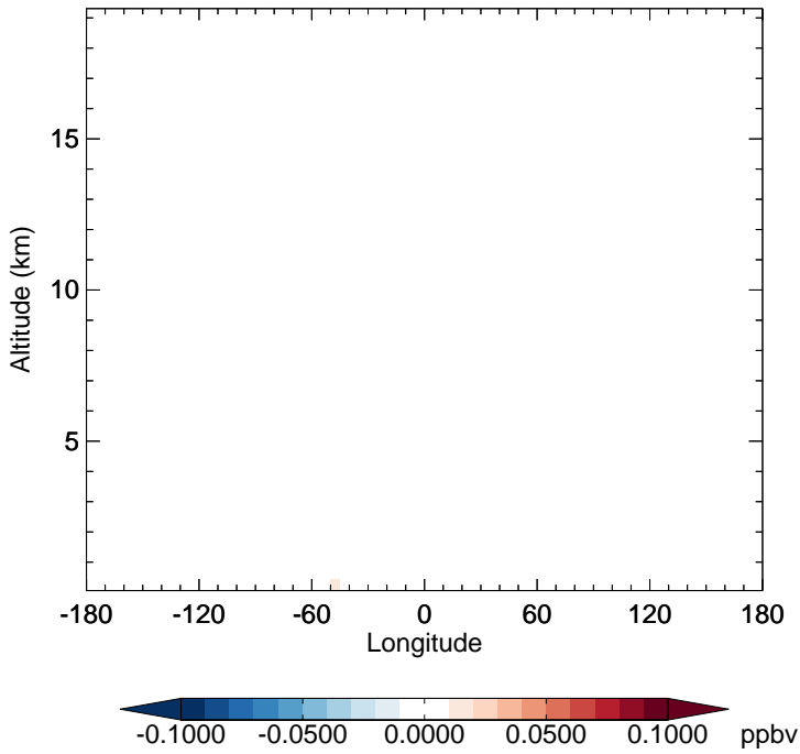
v11-02e-Run1 - v11-02d-Run1 ISN1 - Diff along 15S for Apr
