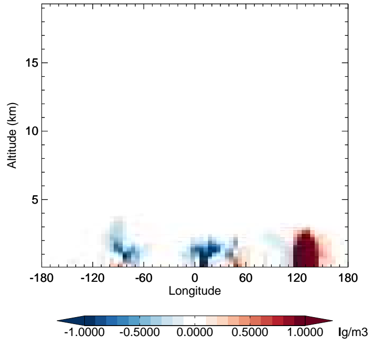
v11-02e-Run1 - v11-02d-Run1 NIT - Diff along 42N for Apr
