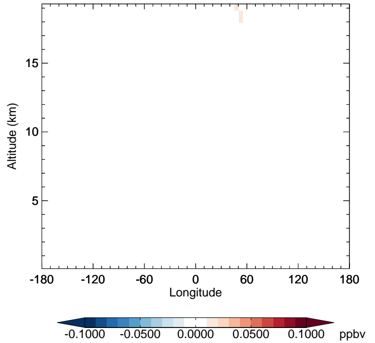
v11-02e-Run1 - v11-02d-Run1 CCI4 - Diff along 42N for Apr
