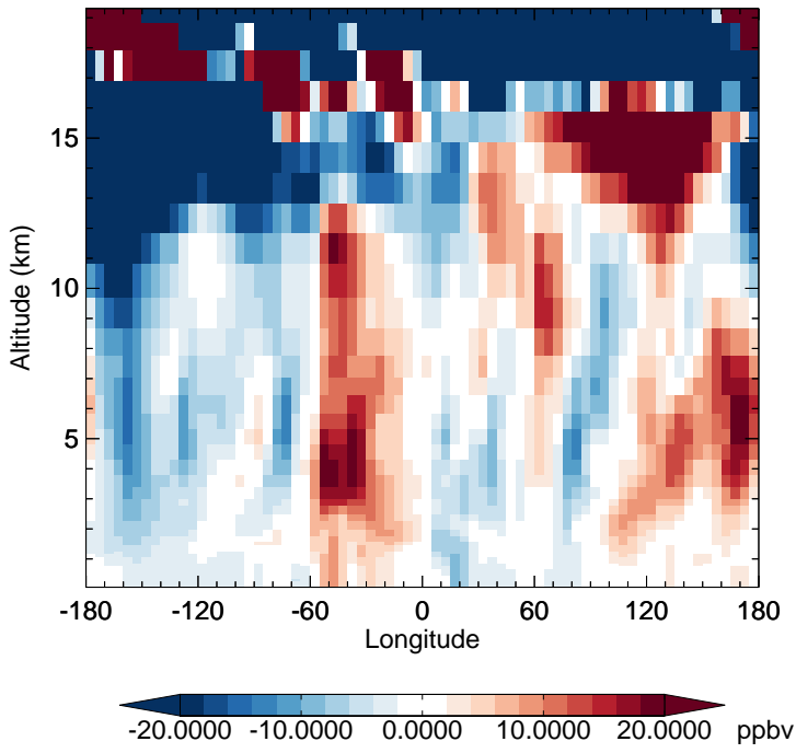
v11-02e-Run1 - v11-02e-Run0 O3 - Diff along 15S for Apr
