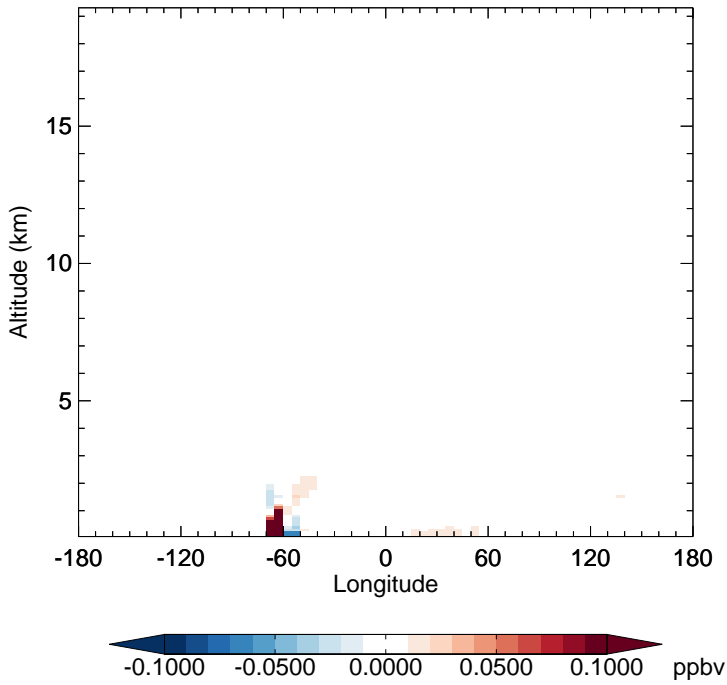
v11-02e-Run1 - v11-02d-Run1 MTPA - Diff along 15S for Apr
