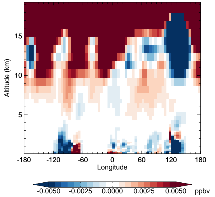
v11-02e-Run1 - v11-02e-Run0 N2O5 - Diff along 42N for Apr
