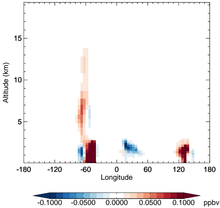
v11-02e-Run1 - v11-02d-Run1 GLYC - Diff along 15S for Apr
