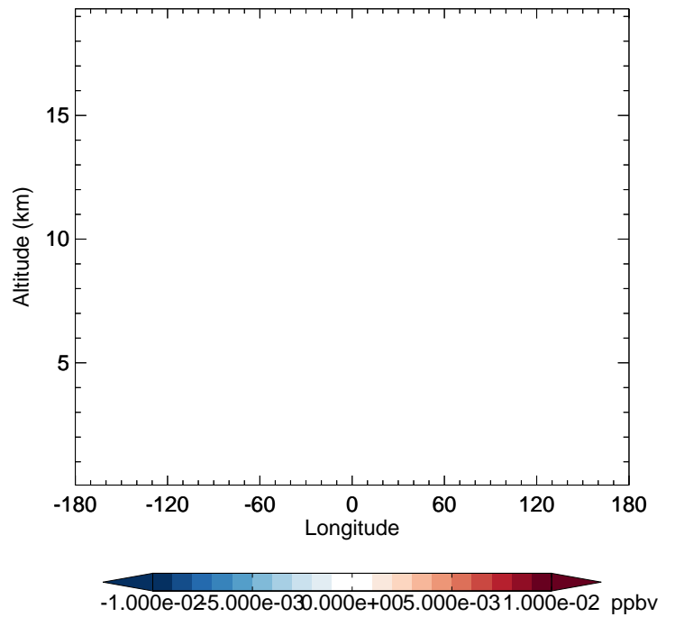
v11-02e-Run1 - v11-02d-Run1 MOBA - Diff along 42N for Apr
