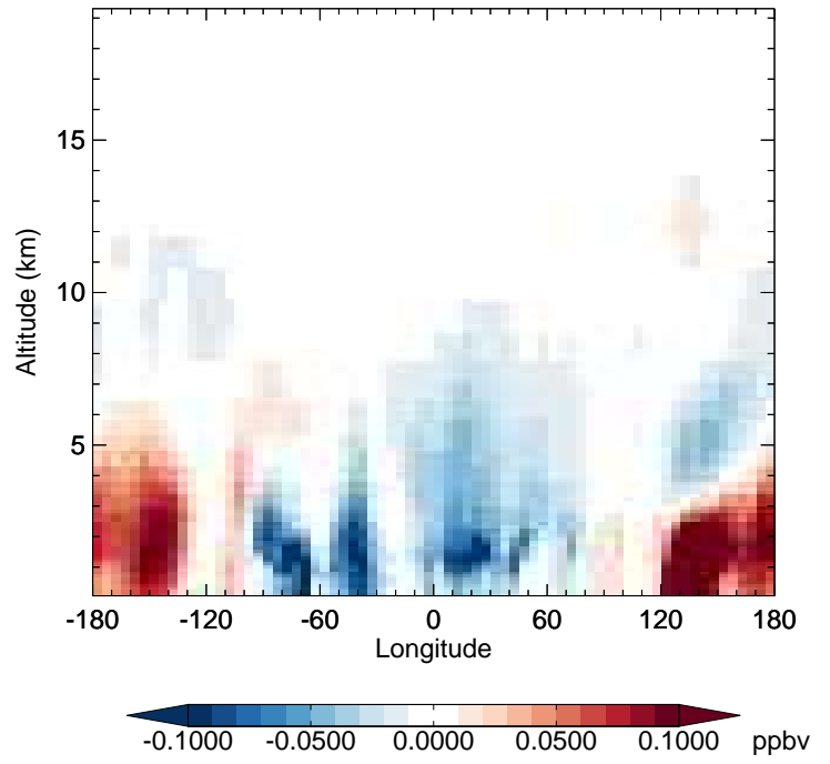
v11-02e-Run1 - v11-02e-Run0 PAN - Diff along 42N for Apr
