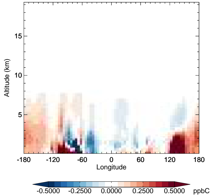
v11-02e-Run1 - v11-02d-Run1 ALK4 - Diff along 42N for Apr
