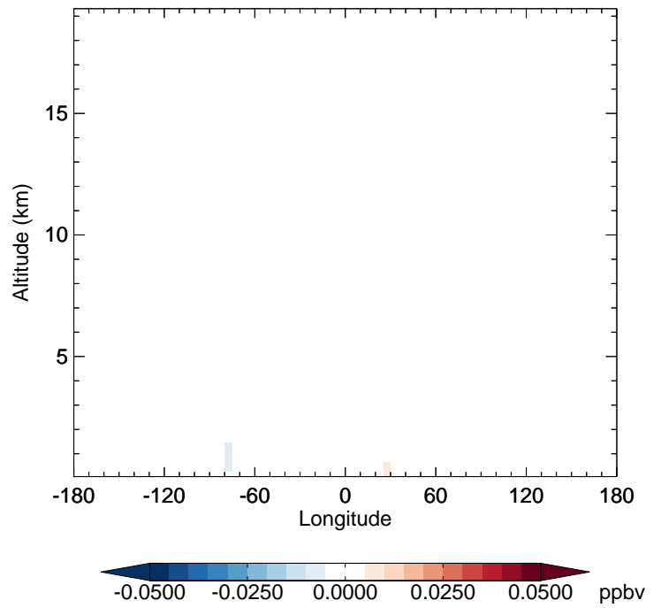
v11-02e-Run1 - v11-02d-Run1 MACR - Diff along 42N for Apr
