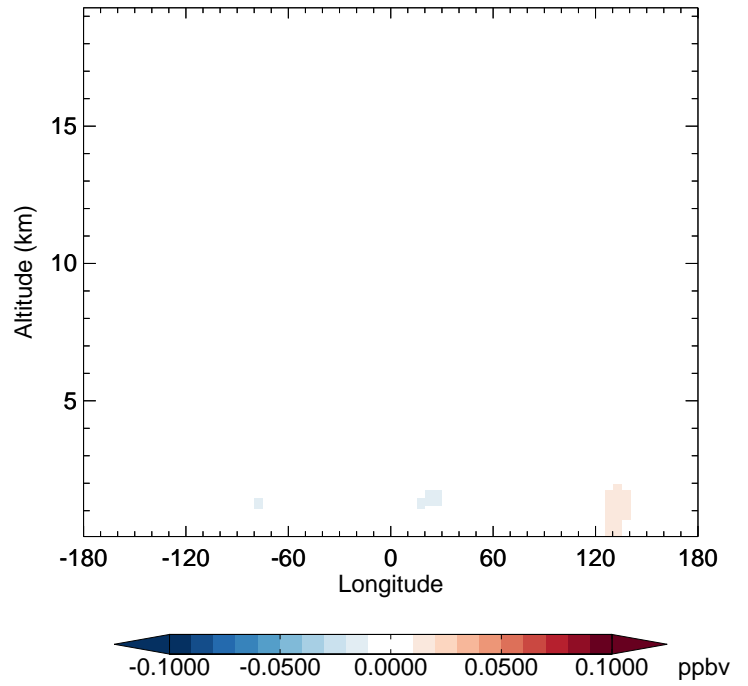
v11-02e-Run1 - v11-02e-Run0 TSOG3 - Diff along 42N for Apr
