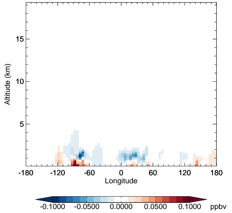
v11-02e-Run1 - v11-02e-Run0 EOH - Diff along 42N for Apr
