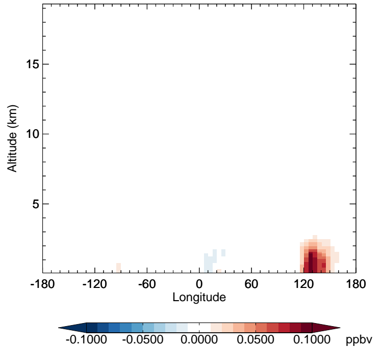
v11-02e-Run1 - v11-02e-Run0 SOAGX - Diff along 42N for Apr
