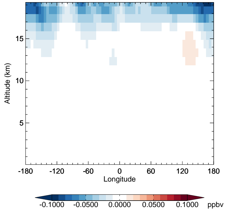
v11-02e-Run1 - v11-02e-Run0 OCS - Diff along 42N for Apr
