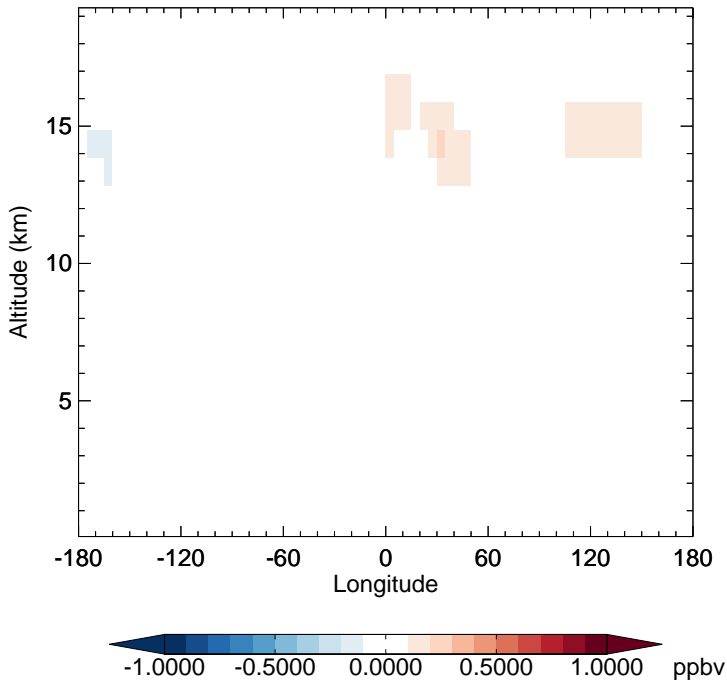
v11-02e-Run1 - v11-02e-Run0 NO - Diff along 15S for Apr
