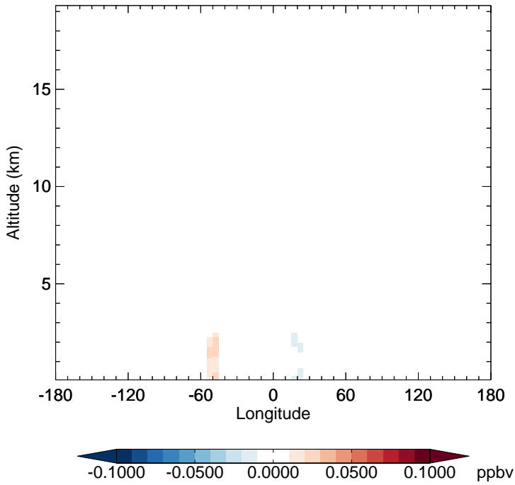
v11-02e-Run1 - v11-02d-Run1 MONITA - Diff along 15S for Apr
