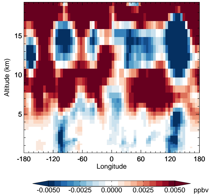
v11-02e-Run1 - v11-02e-Run0 HNO 4 - Diff along 42N for Apr
