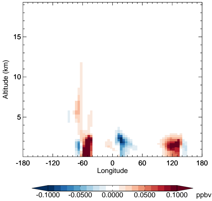
v11-02e-Run1 - v11-02e-Run0 ISO3 - Diff along 15S for Apr
