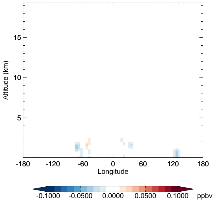
v11-02e-Run1 - v11-02d-Run1 TOLU - Diff along 15S for Apr
