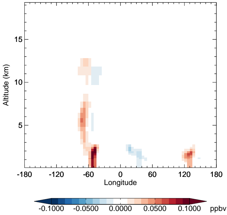
v11-02e-Run1 - v11-02e-Run0 HC187 - Diff along 15S for Apr
