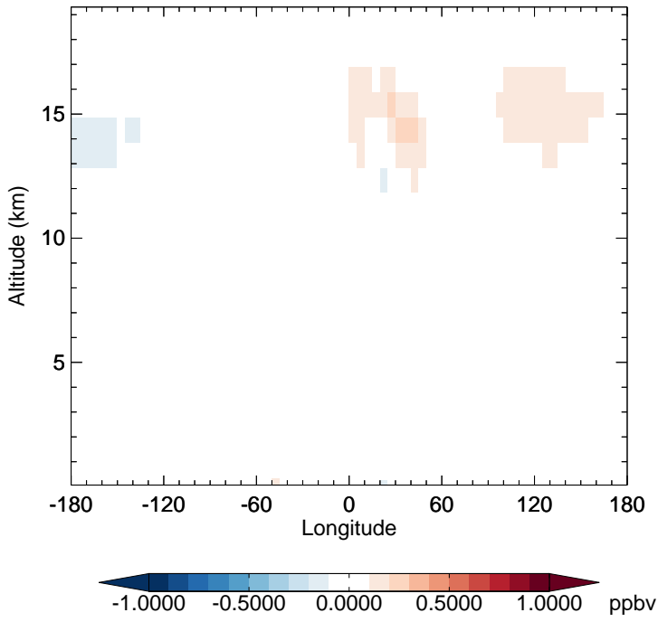
v11-02e-Run1 - v11-02e-Run0 NO2 - Diff along 15S for Apr
