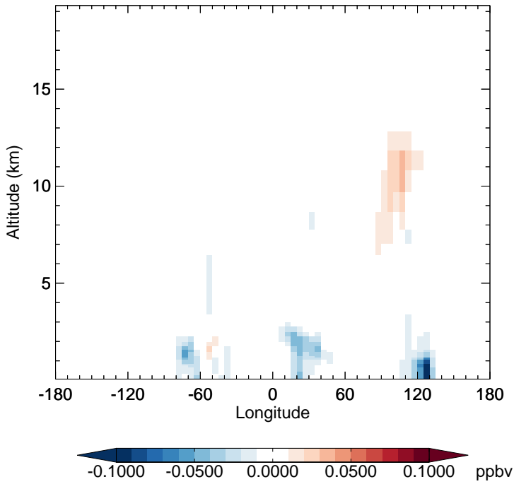
v11-02e-Run1 - v11-02d-Run1 BENZ - Diff along 15S for Apr
