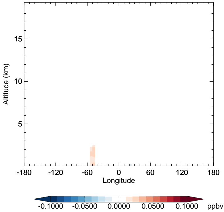
v11-02e-Run1 - v11-02e-Run0 MONITA - Diff along 15S for Apr
