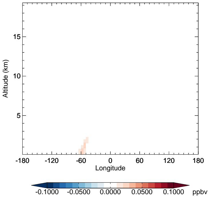
v11-02e-Run1 - v11-02d-Run1 TSOA1 - Diff along 15S for Apr
