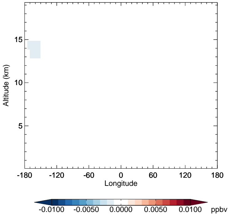
v11-02e-Run1 - v11-02e-Run0 BrNO3 - Diff along 15S for Apr
