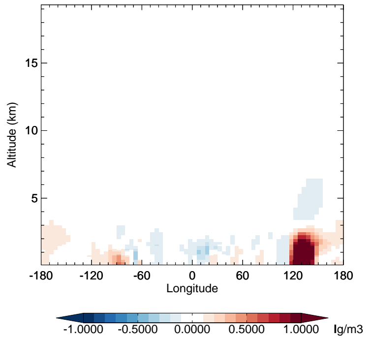
v11-02e-Run1 - v11-02d-Run1 SOAS - Diff along 42N for Apr
