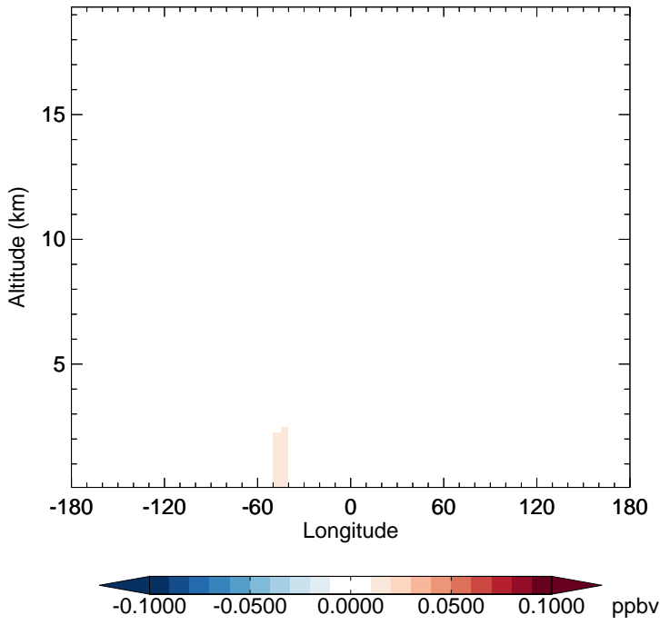
v11-02e-Run1 - v11-02e-Run0 ISOPNB - Diff along 15S for Apr
