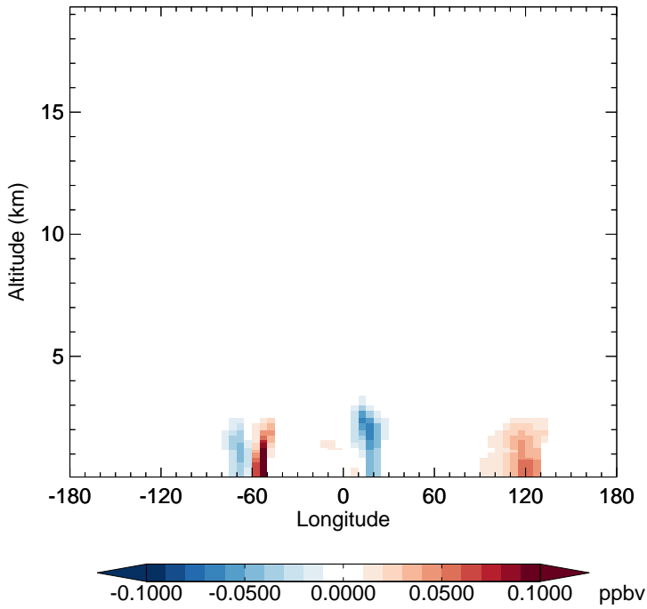
v11-02e-Run1 - v11-02d-Run1 INDIOL - Diff along 15S for Apr
