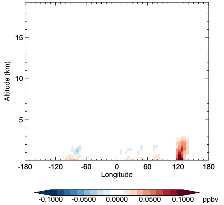
v11-02e-Run1 - v11-02e-Run0 SOAP - Diff along 42N for Apr
