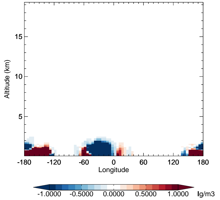
v11-02e-Run1 - v11-02e-Run0 SALC - Diff along 42N for Apr
