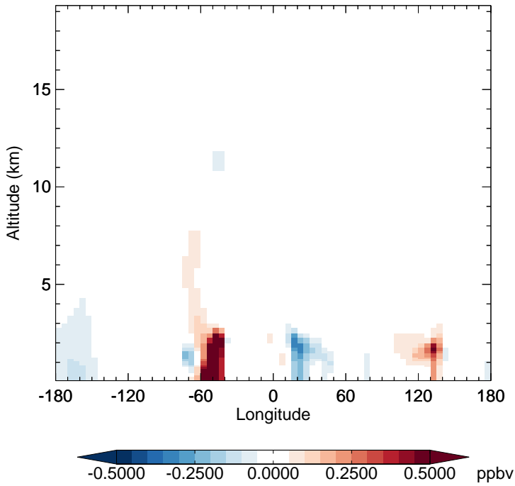
v11-02e-Run1 - v11-02d-Run1 CH 2 O - Diff along 15S for Apr
