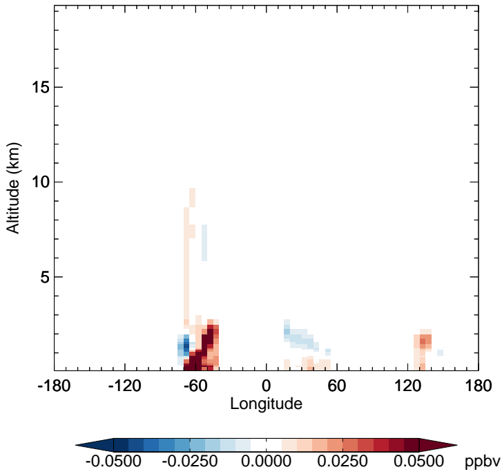
v11-02e-Run1 - v11-02e-Run0 RCHO - Diff along 15S for Apr
