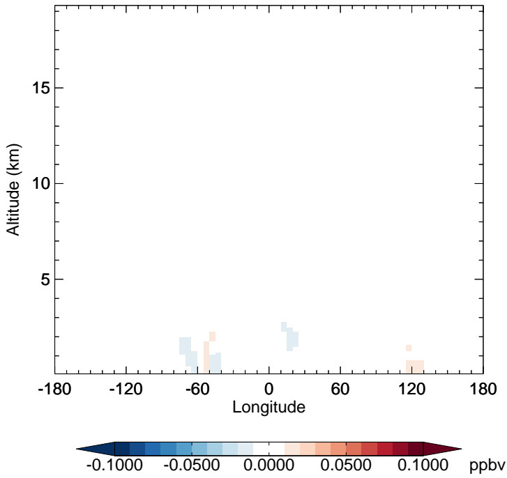
v11-02e-Run1 - v11-02e-Run0 SOAGX - Diff along 15S for Apr
