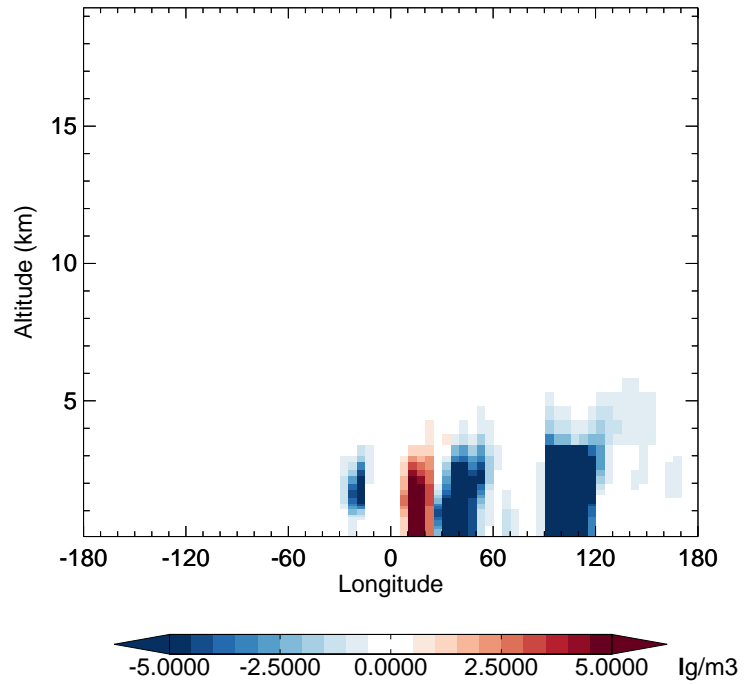
v11-02e-Run1 - v11-02d-Run1 DST2 - Diff along 42N for Apr
