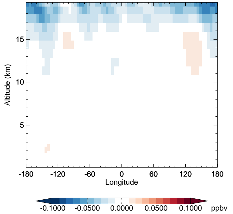
v11-02e-Run1 - v11-02e-Run0 CH3Cl - Diff along 42N for Apr
