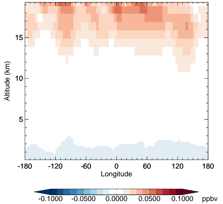
v11-02e-Run1 - v11-02d-Run1 CFC12 - Diff along 42N for Apr
