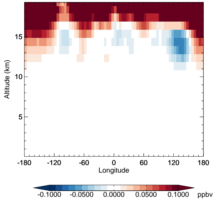
v11-02e-Run1 - v11-02e-Run0 CINO3 - Diff along 42N for Apr
