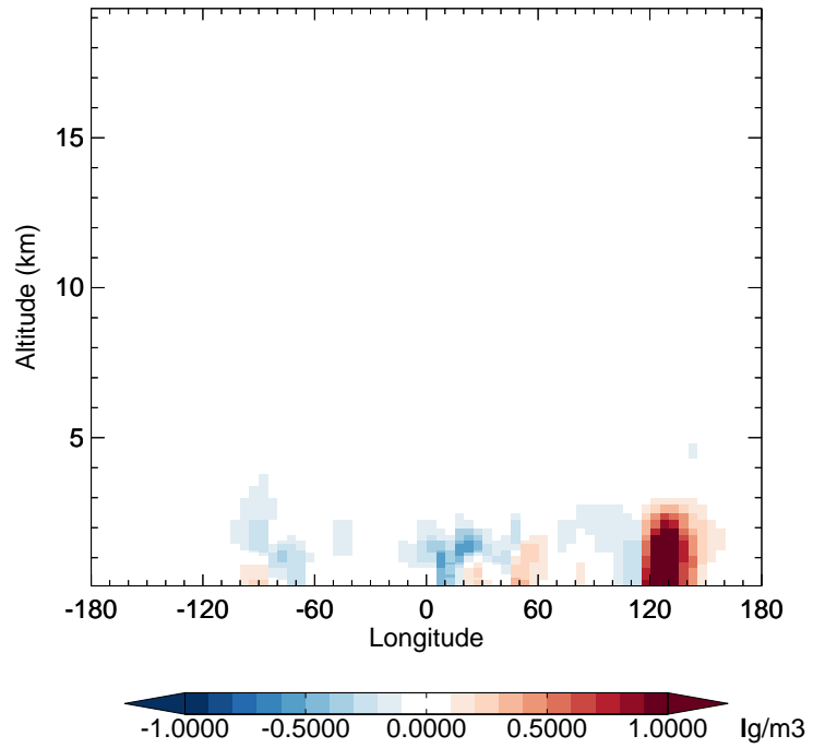
v11-02e-Run1 - v11-02d-Run1 NH4 - Diff along 42N for Apr
