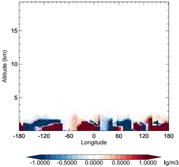
v11-02e-Run1 - v11-02d-Run1 SALC - Diff along 15S for Apr
