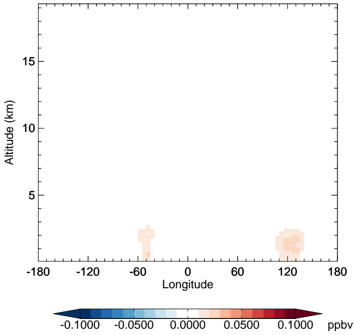
v11-02e-Run1 - v11-02e-Run0 ISOG1 - Diff along 15S for Apr
