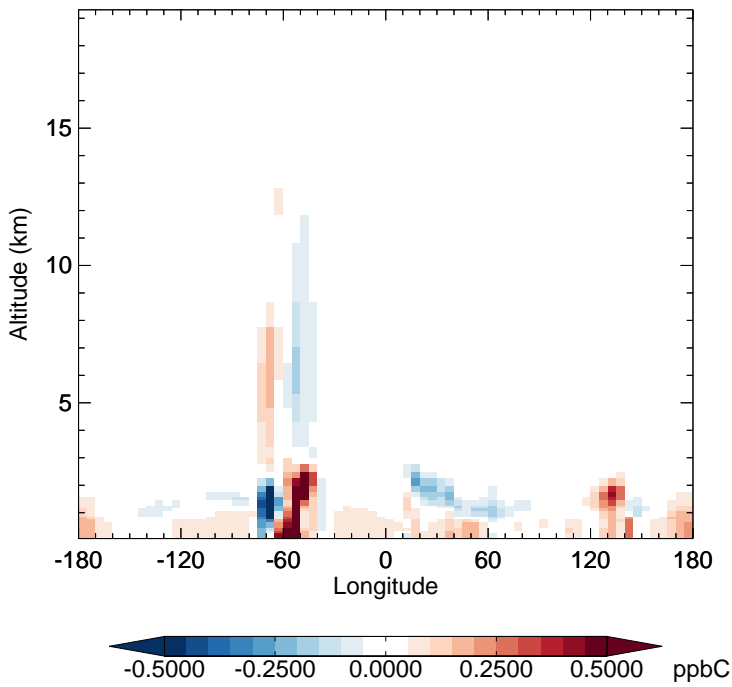
v11-02e-Run1 - v11-02d-Run1 ALD2 - Diff along 15S for Apr
