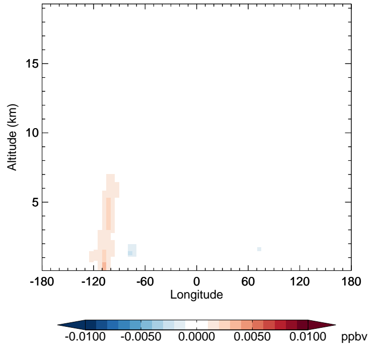
v11-02e-Run1 - v11-02e-Run0 R4N2 - Diff along 42N for Apr
