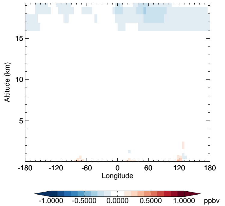
v11-02e-Run1 - v11-02d-Run1 NO2 - Diff along 42N for Apr
