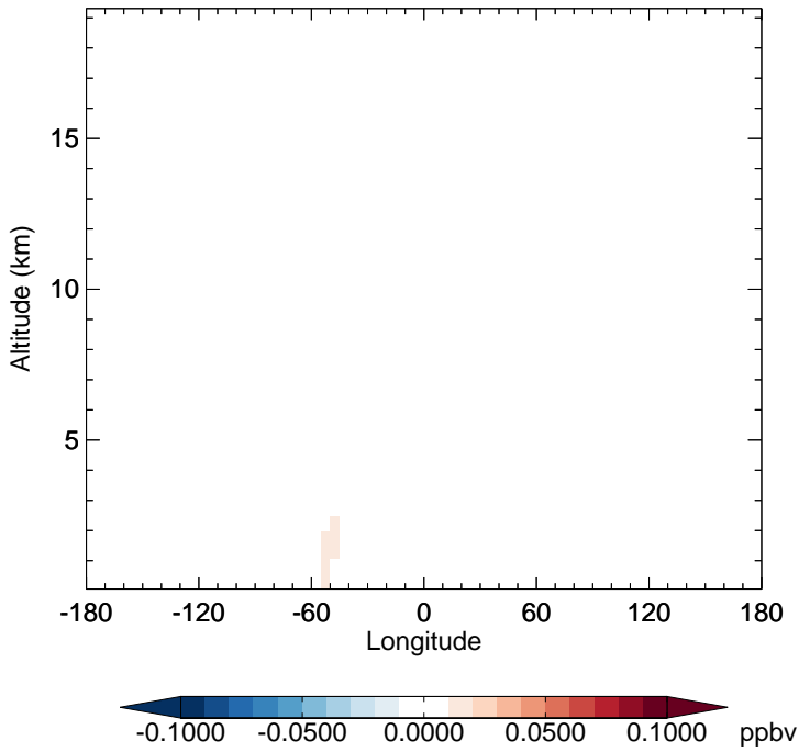
v11-02e-Run1 - v11-02d-Run1 IEPOXD - Diff along 15S for Apr
