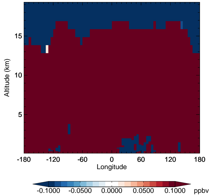
v11-02e-Run1 - v11-02e-Run0 CH4 - Diff along 42N for Apr
