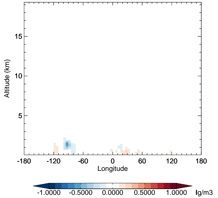
v11-02e-Run1 - v11-02e-Run0 NH3 - Diff along 42N for Apr
