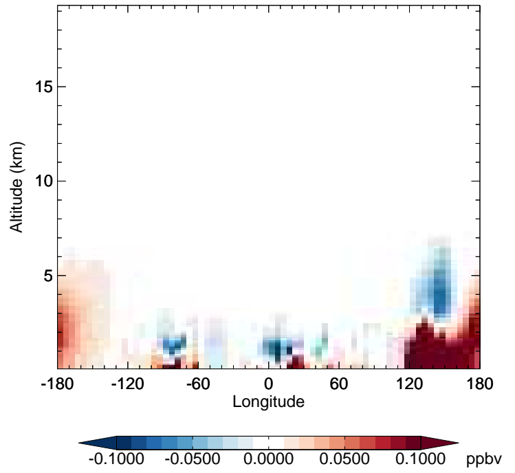
v11-02e-Run1 - v11-02e-Run0 TOLU - Diff along 42N for Apr
