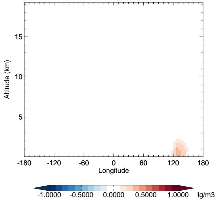
v11-02e-Run1 - v11-02d-Run1 BCPI - Diff along 42N for Apr
