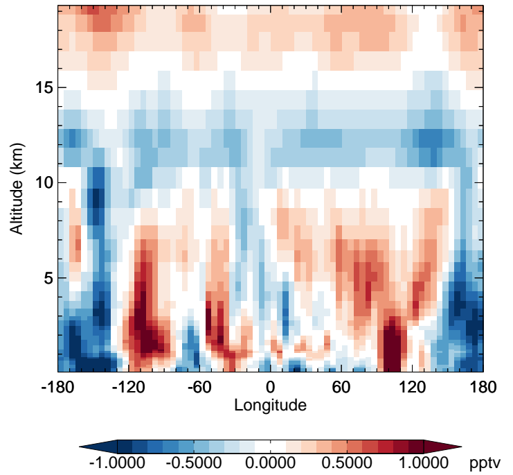
v11-02e-Run1 - v11-02d-Run1 HO2 - Diff along 42N for Apr
