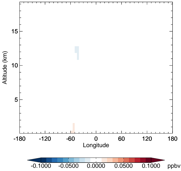
v11-02e-Run1 - v11-02e-Run0 ISOA3 - Diff along 15S for Apr
