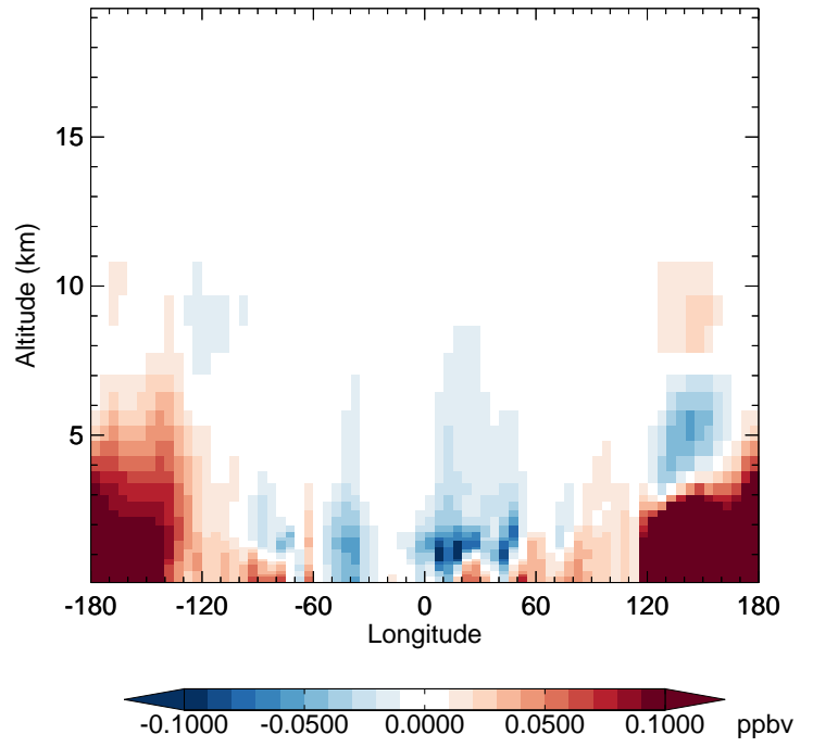
v11-02e-Run1 - v11-02e-Run0 BENZ - Diff along 42N for Apr
