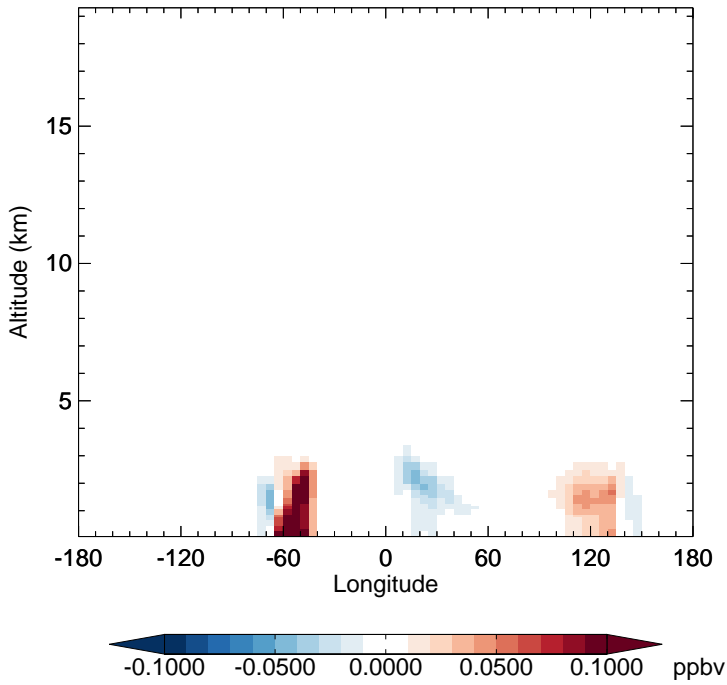
v11-02e-Run1 - v11-02d-Run1 TSOG2 - Diff along 15S for Apr
