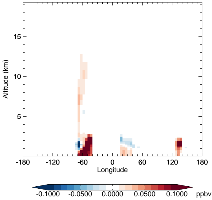
v11-02e-Run1 - v11-02e-Run0 RIPA - Diff along 15S for Apr
