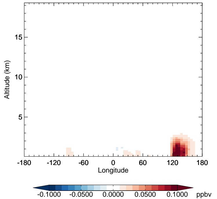
v11-02e-Run1 - v11-02d-Run1 SOAGX - Diff along 42N for Apr
