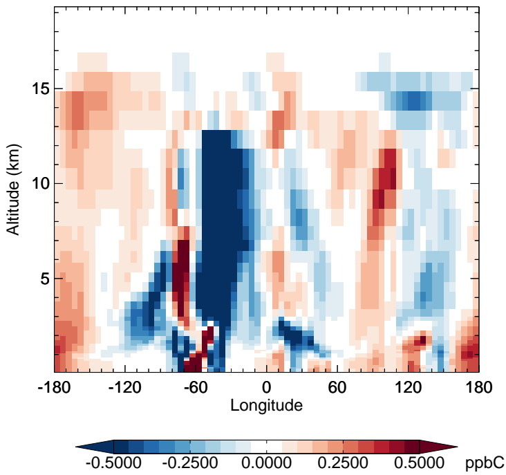
v11-02e-Run1 - v11-02d-Run1 ACET - Diff along 15S for Apr
