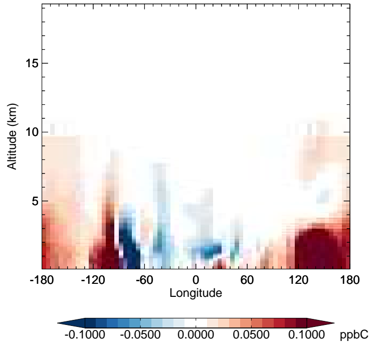
v11-02e-Run1 - v11-02e-Run0 MEK - Diff along 42N for Apr
