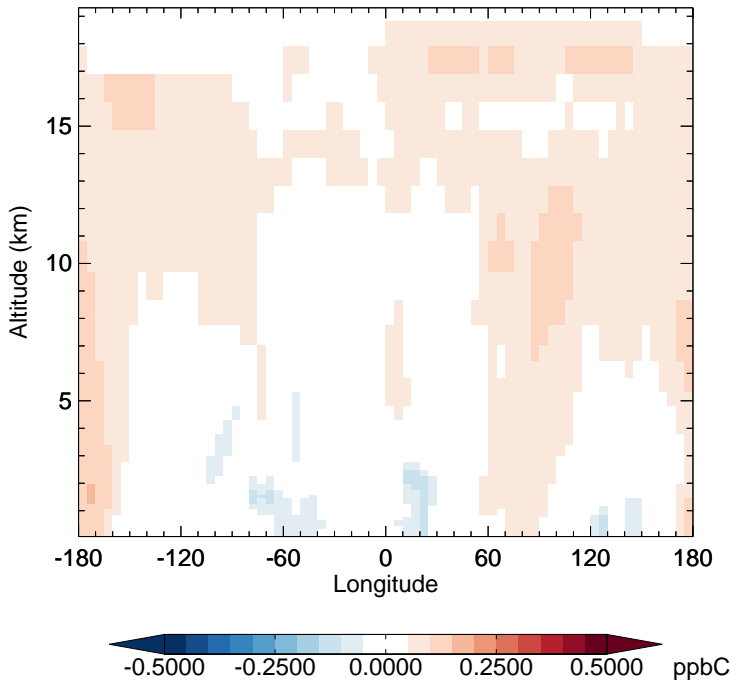
v11-02e-Run1 - v11-02d-Run1 C2H6 - Diff along 15S for Apr
