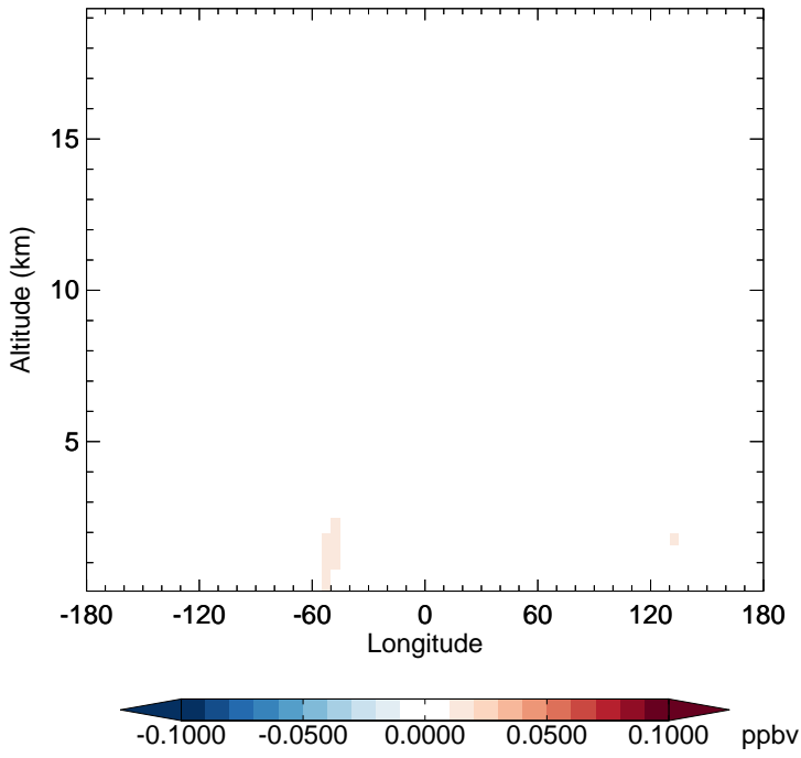
v11-02e-Run1 - v11-02e-Run0 IEPOXD - Diff along 15S for Apr
