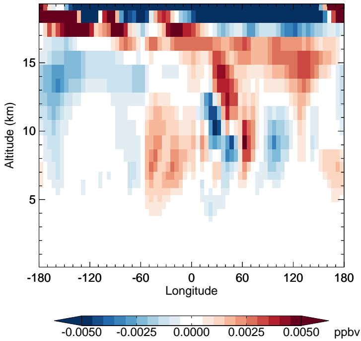
v11-02e-Run1 - v11-02d-Run1 N2O5 - Diff along 15S for Apr
