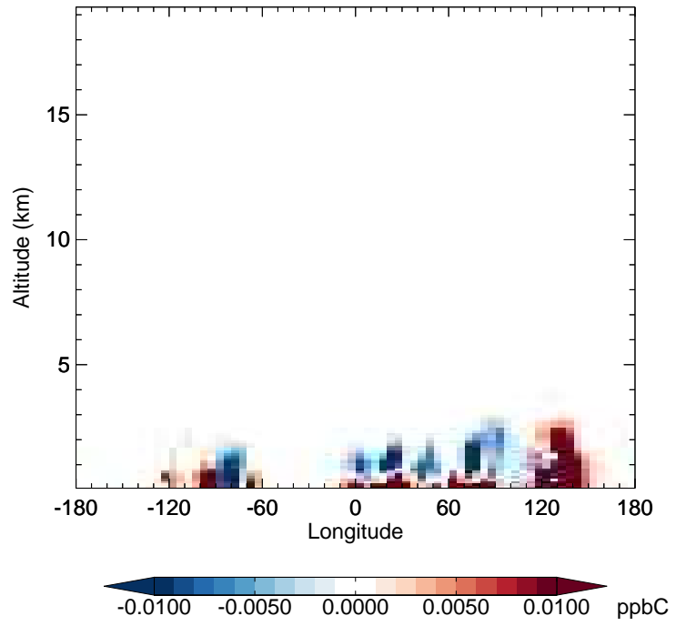
v11-02e-Run1 - v11-02e-Run0 PRPE - Diff along 42N for Apr
