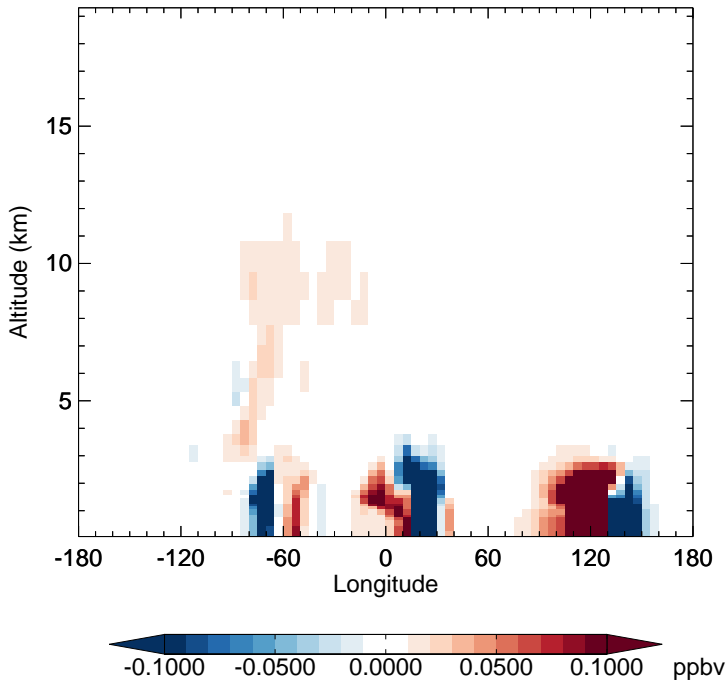
v11-02e-Run1 - v11-02e-Run0 SOAIE - Diff along 15S for Apr
