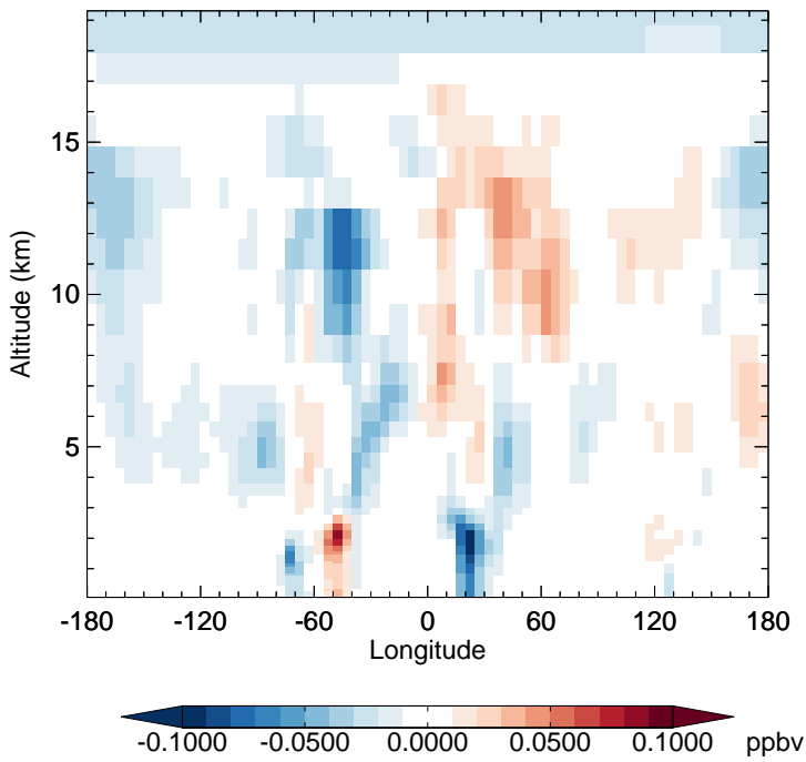
v11-02e-Run1 - v11-02d-Run1 PAN - Diff along 15S for Apr
