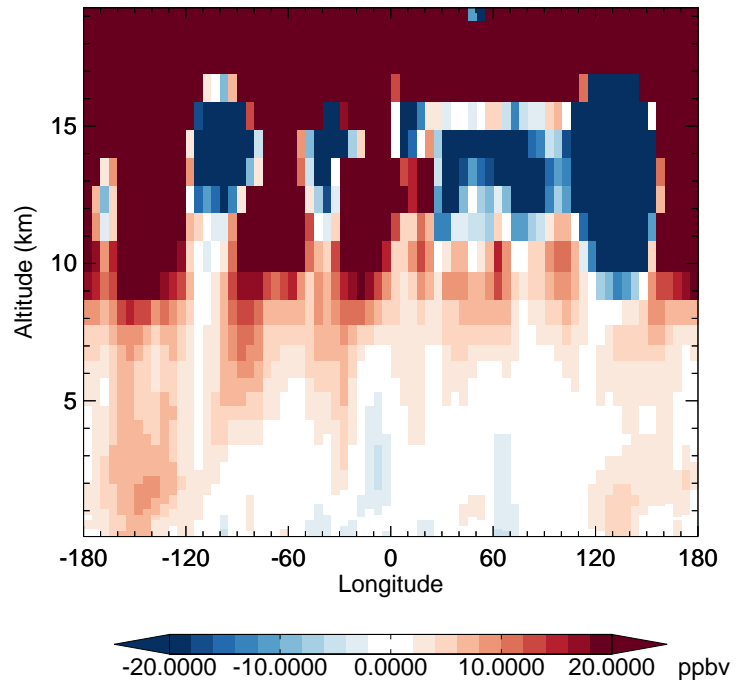
v11-02e-Run1 - v11-02e-Run0 O3 - Diff along 42N for Apr
