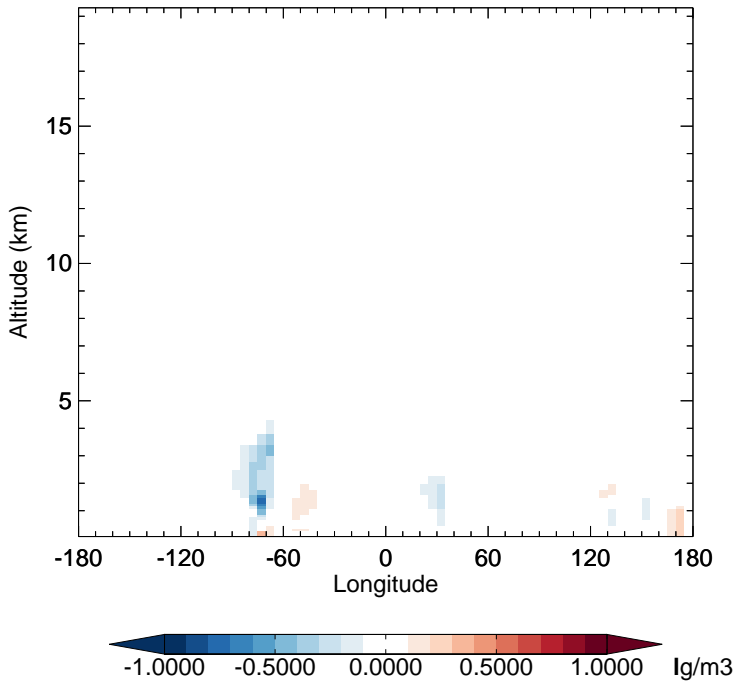
v11-02e-Run1 - v11-02e-Run0 SO 2 - Diff along 15S for Apr
