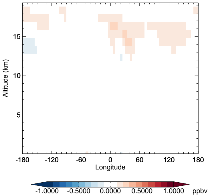
v11-02e-Run1 - v11-02d-Run1 NO2 - Diff along 15S for Apr
