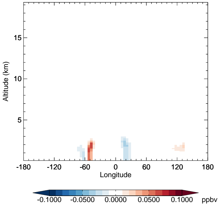
v11-02e-Run1 - v11-02d-Run1 IONITA - Diff along 15S for Apr
