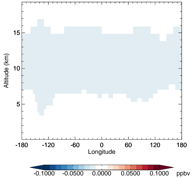
v11-02e-Run1 - v11-02d-Run1 HCFC141b - Diff along 42N for Apr
