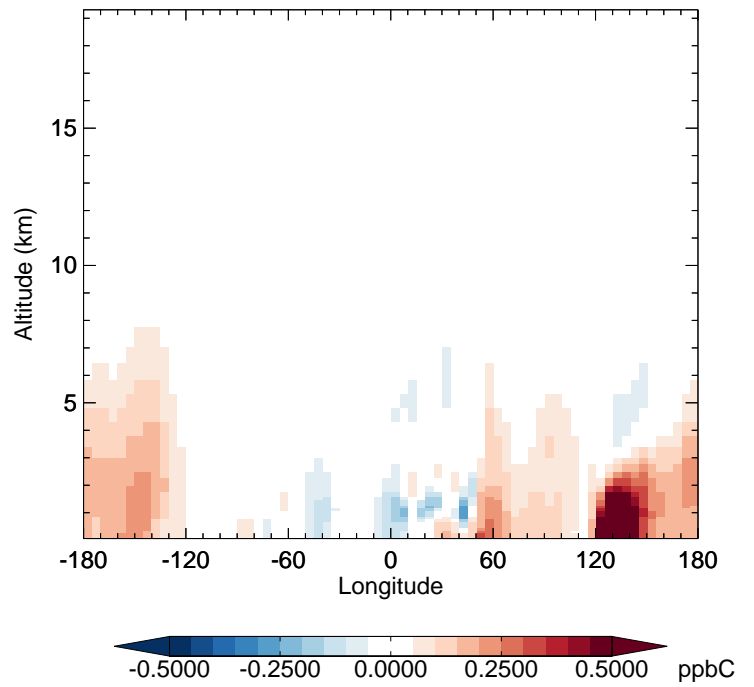
v11-02e-Run1 - v11-02d-Run1 C3H8 - Diff along 42N for Apr
