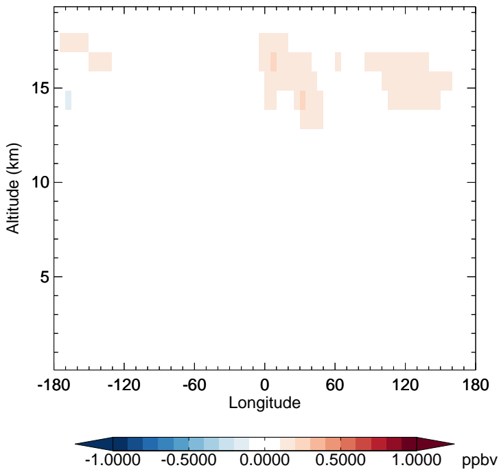
v11-02e-Run1 - v11-02d-Run1 NO - Diff along 15S for Apr
