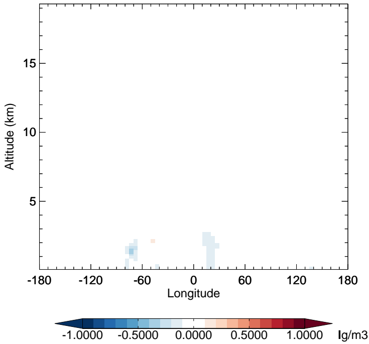
v11-02e-Run1 - v11-02d-Run1 NH4 - Diff along 15S for Apr
