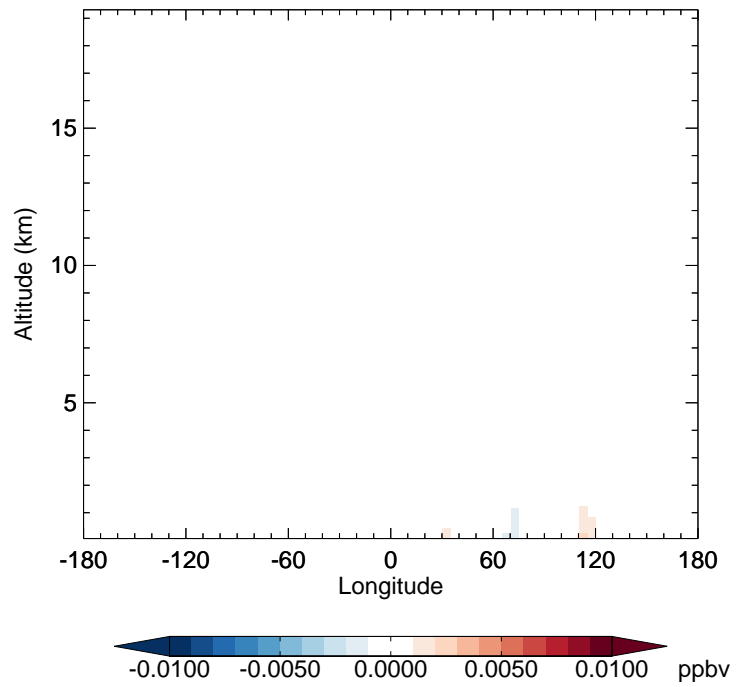
v11-02e-Run1 - v11-02d-Run1 NO3 - Diff along 42N for Apr
