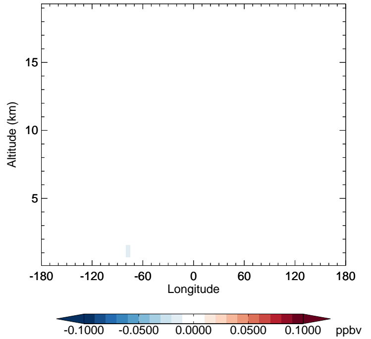
v11-02e-Run1 - v11-02d-Run1 GLYC - Diff along 42N for Apr
