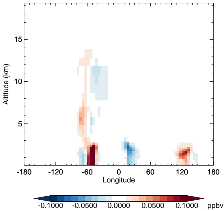
v11-02e-Run1 - v11-02d-Run1 IMAE - Diff along 15S for Apr
