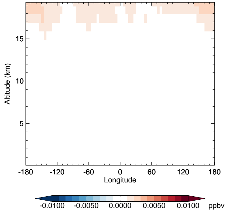
v11-02e-Run1 - v11-02e-Run0 BrNO3 - Diff along 42N for Apr
