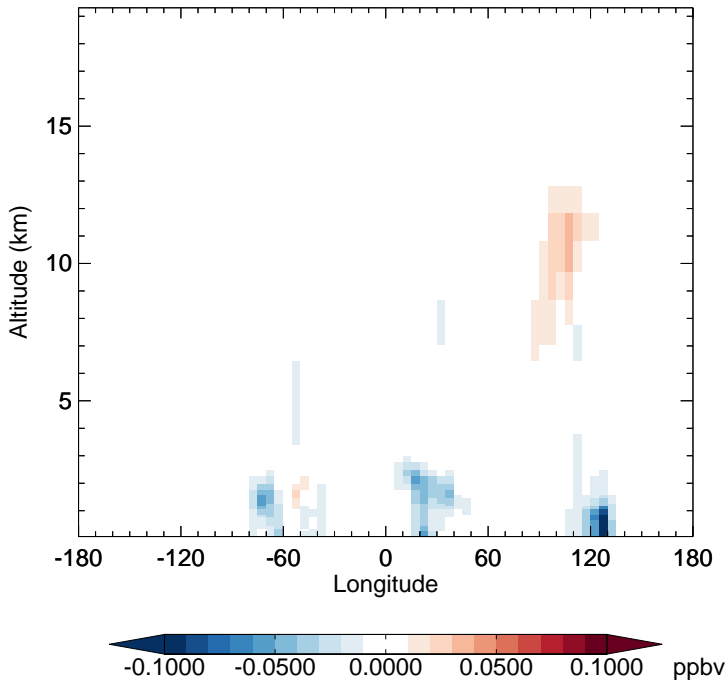
v11-02e-Run1 - v11-02e-Run0 BENZ - Diff along 15S for Apr
