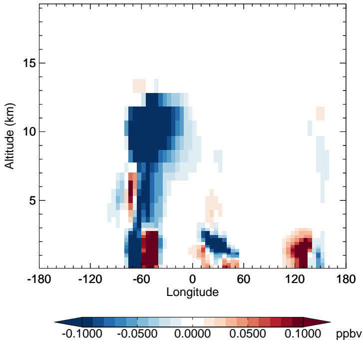
v11-02e-Run1 - v11-02e-Run0 EOH - Diff along 15S for Apr
