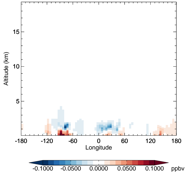
v11-02e-Run1 - v11-02d-Run1 EOH - Diff along 42N for Apr
