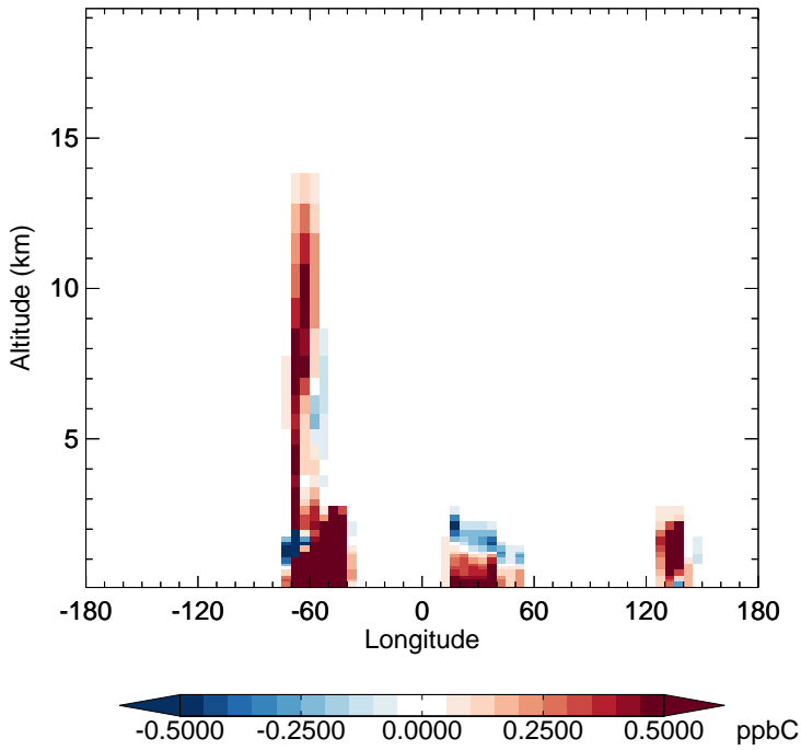
v11-02e-Run1 - v11-02d-Run1 ISOP - Diff along 15S for Apr
