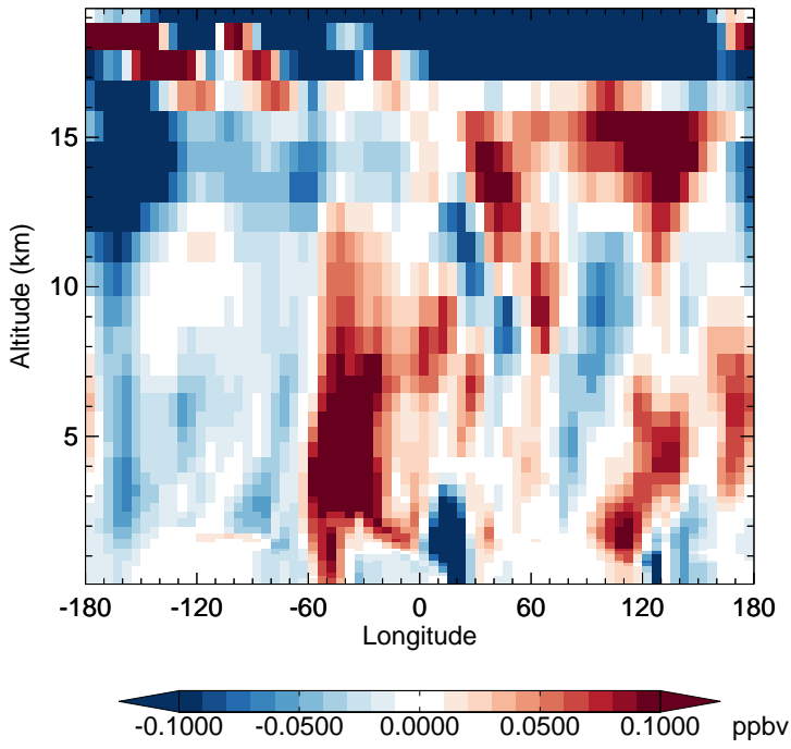
v11-02e-Run1 - v11-02e-Run0 HNO 3 - Diff along 15S for Apr
