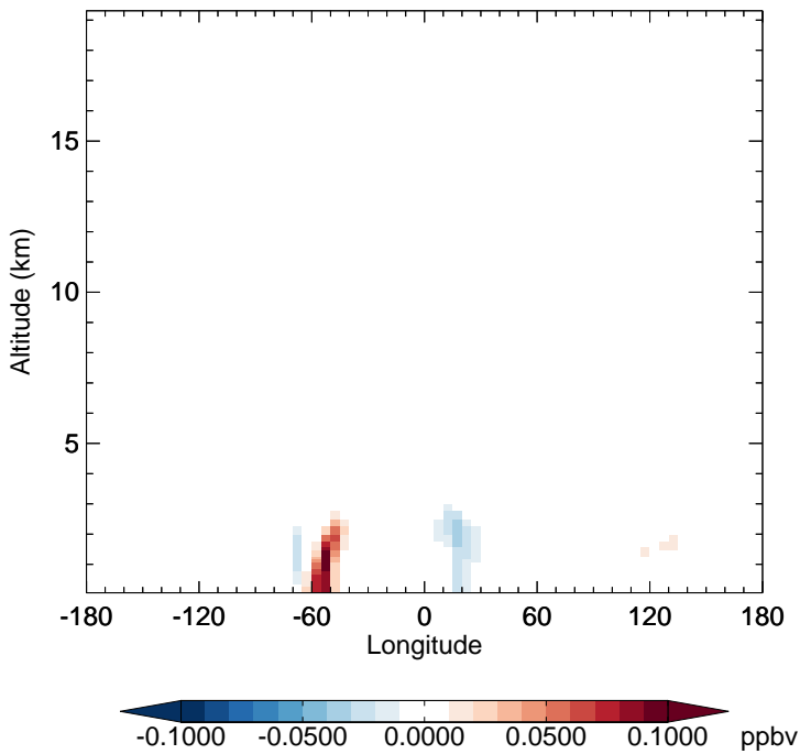
v11-02e-Run1 - v11-02d-Run1 ISOA1 - Diff along 15S for Apr
