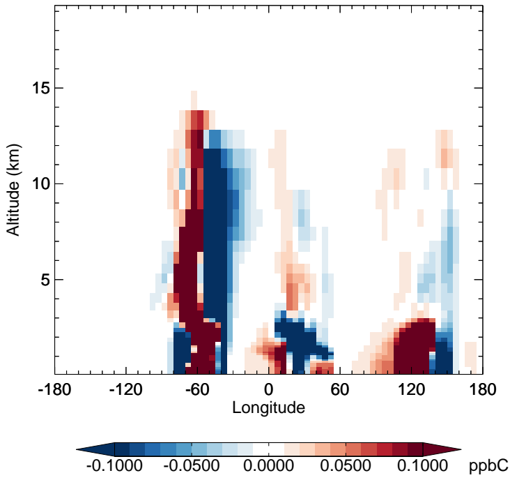
v11-02e-Run1 - v11-02e-Run0 MEK - Diff along 15S for Apr
