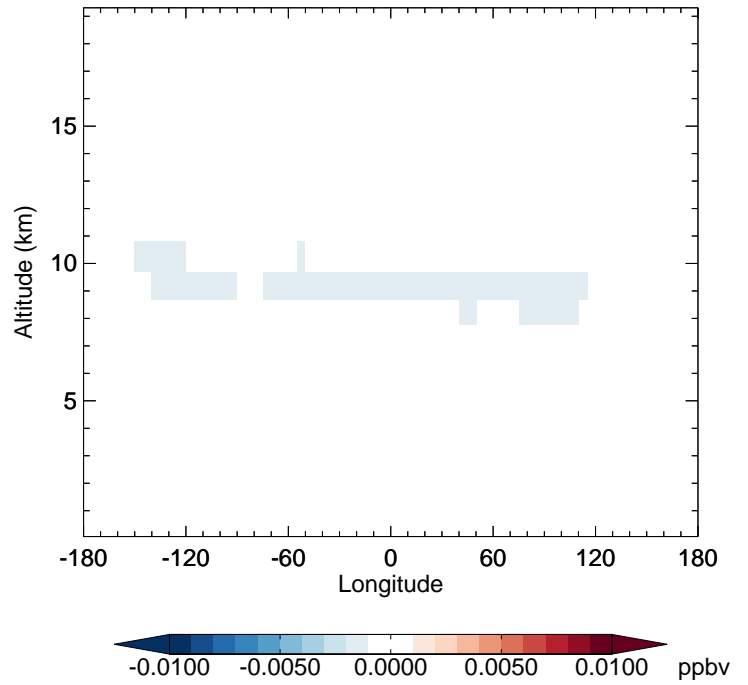
v11-02e-Run1 - v11-02d-Run1 HBr - Diff along 42N for Apr
