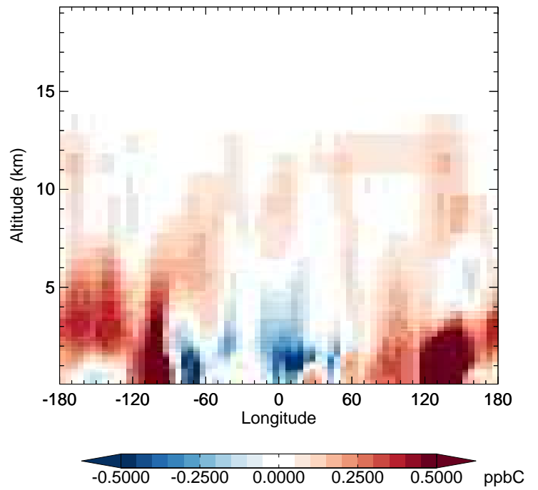
v11-02e-Run1 - v11-02d-Run1 ACET - Diff along 42N for Apr
