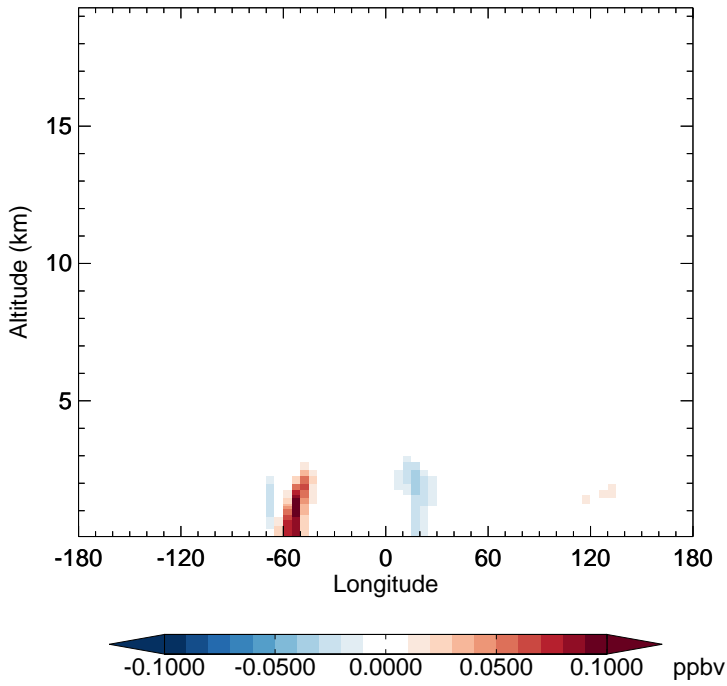
v11-02e-Run1 - v11-02e-Run0 ISOA1 - Diff along 15S for Apr
