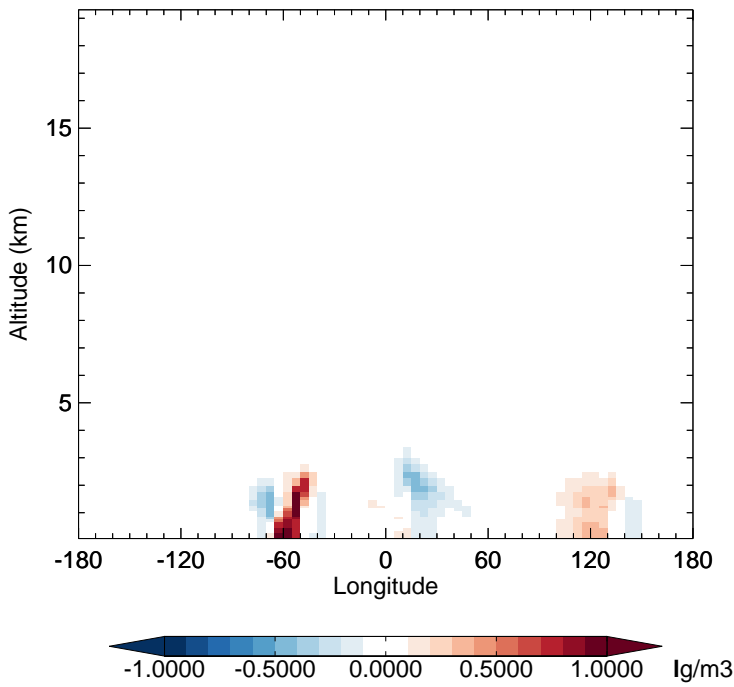
v11-02e-Run1 - v11-02d-Run1 SOAS - Diff along 15S for Apr
