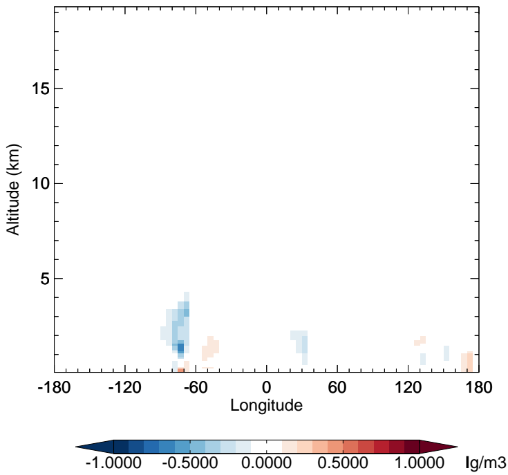
v11-02e-Run1 - v11-02d-Run1 SO 2 - Diff along 15S for Apr
