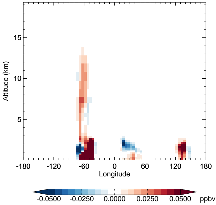
v11-02e-Run1 - v11-02e-Run0 MACR - Diff along 15S for Apr
