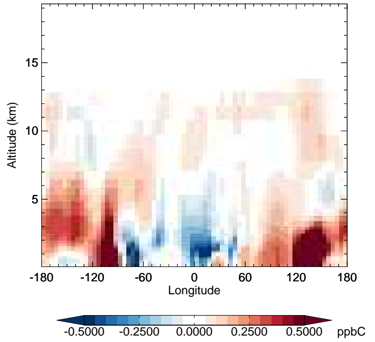
v11-02e-Run1 - v11-02e-Run0 ACET - Diff along 42N for Apr
