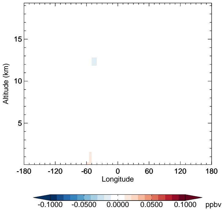
v11-02e-Run1 - v11-02d-Run1 ISOA3 - Diff along 15S for Apr
