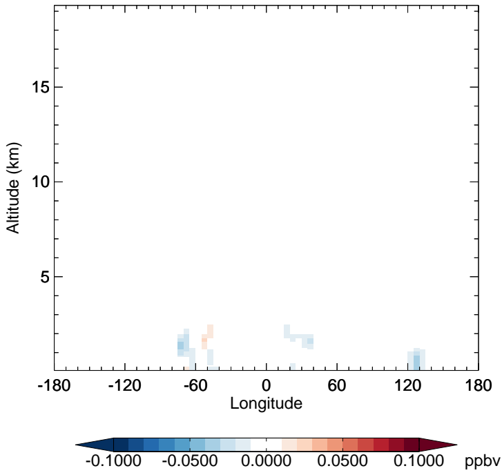
v11-02e-Run1 - v11-02e-Run0 TOLU - Diff along 15S for Apr
