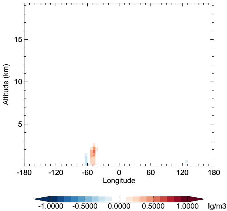
v11-02e-Run1 - v11-02d-Run1 NH3 - Diff along 15S for Apr
