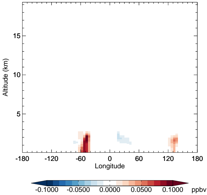
v11-02e-Run1 - v11-02e-Run0 MGLY - Diff along 15S for Apr
