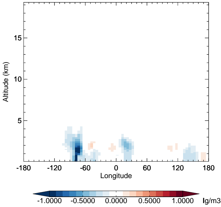
v11-02e-Run1 - v11-02e-Run0 SO4 - Diff along 15S for Apr
