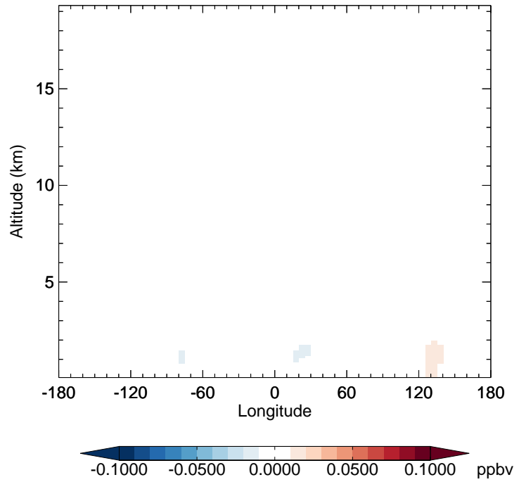
v11-02e-Run1 - v11-02d-Run1 TSOG3 - Diff along 42N for Apr
