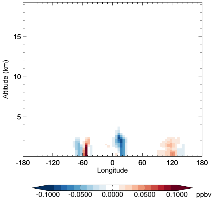
v11-02e-Run1 - v11-02e-Run0 INDIOL - Diff along 15S for Apr
