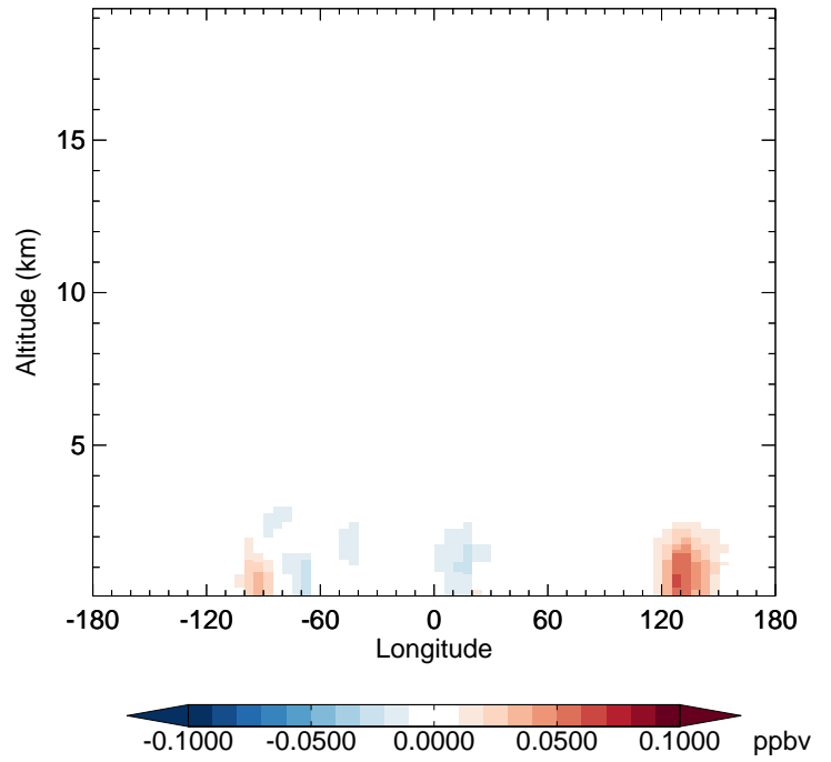
v11-02e-Run1 - v11-02e-Run0 INDIOL - Diff along 42N for Apr
