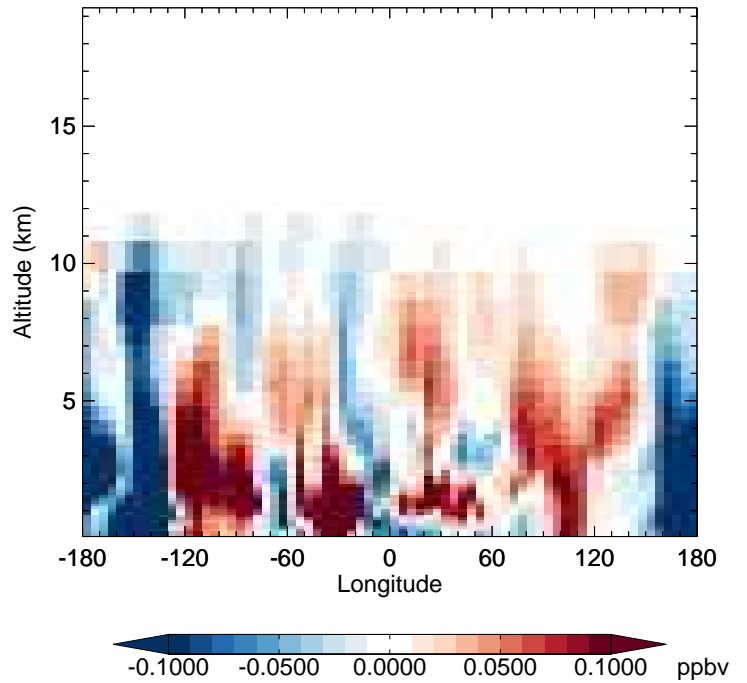
v11-02e-Run1 - v11-02d-Run1 H2O2 - Diff along 42N for Apr
