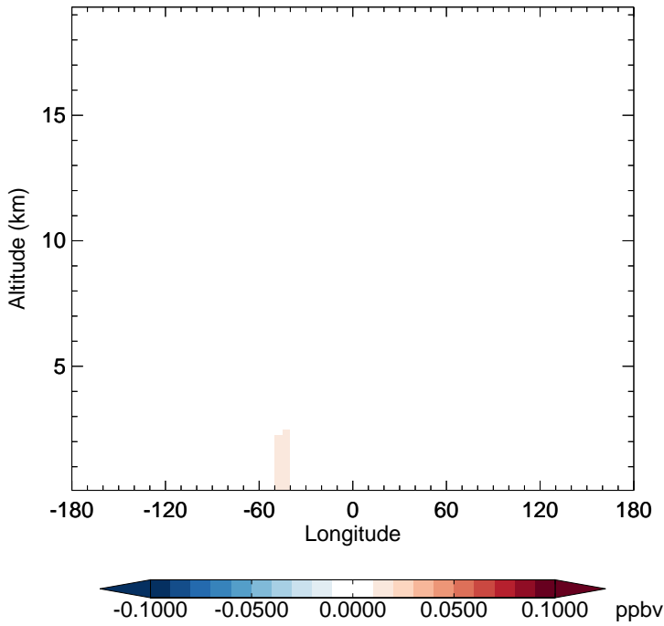
v11-02e-Run1 - v11-02d-Run1 ISOPNB - Diff along 15S for Apr
