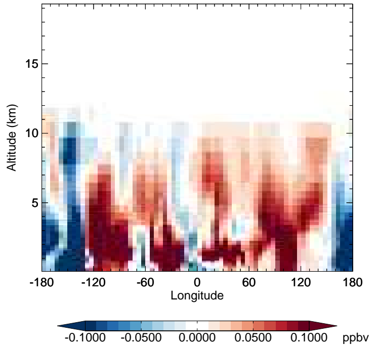
v11-02e-Run1 - v11-02e-Run0 H2O2 - Diff along 42N for Apr
