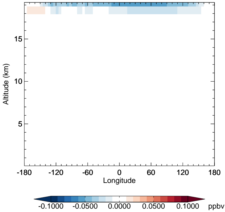
v11-02e-Run1 - v11-02e-Run0 CINO3 - Diff along 15S for Apr
