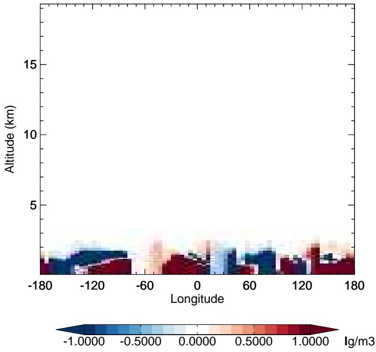
v11-02e-Run1 - v11-02e-Run0 SALC - Diff along 15S for Apr
