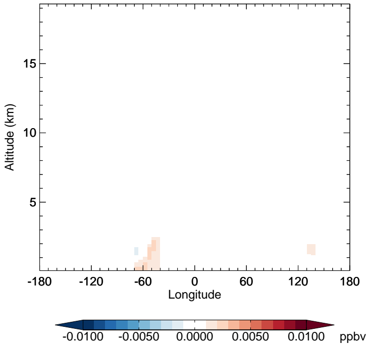
v11-02e-Run1 - v11-02e-Run0 MOBA - Diff along 15S for Apr
