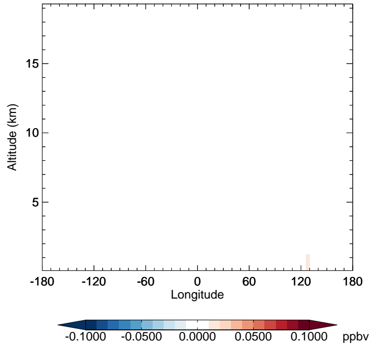
v11-02e-Run1 - v11-02e-Run0 ASOG3 - Diff along 42N for Apr
