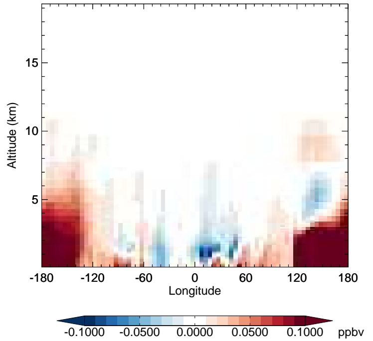
v11-02e-Run1 - v11-02d-Run1 BENZ - Diff along 42N for Apr
