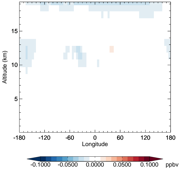
v11-02e-Run1 - v11-02d-Run1 MPN - Diff along 15S for Apr
