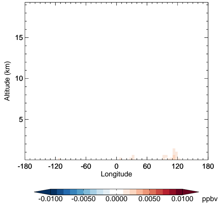
v11-02e-Run1 - v11-02e-Run0 NO3 - Diff along 42N for Apr
