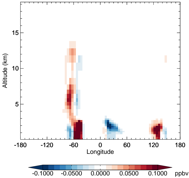
v11-02e-Run1 - v11-02d-Run1 HAC - Diff along 15S for Apr
