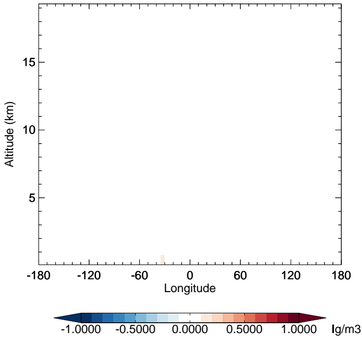
v11-02e-Run1 - v11-02d-Run1 NIT - Diff along 15S for Apr
