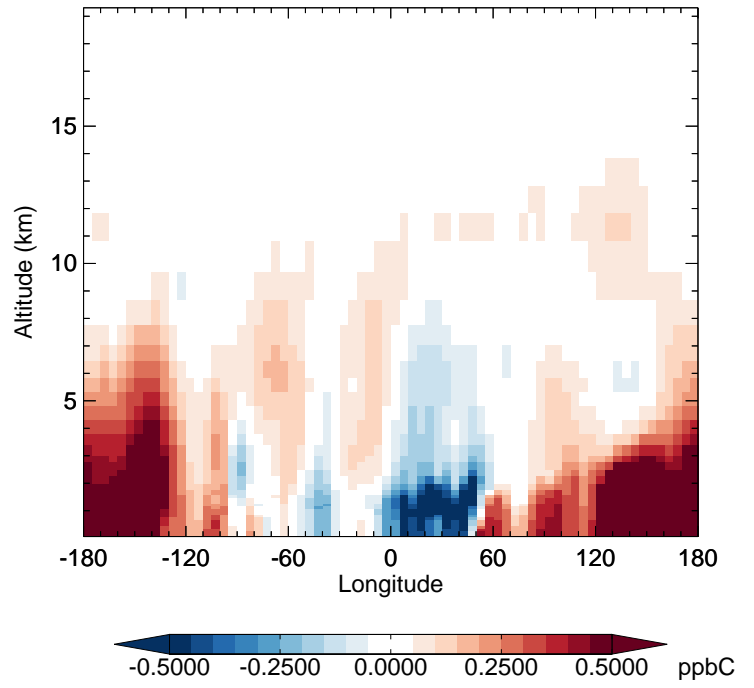
v11-02e-Run1 - v11-02e-Run0 C2H6 - Diff along 42N for Apr
