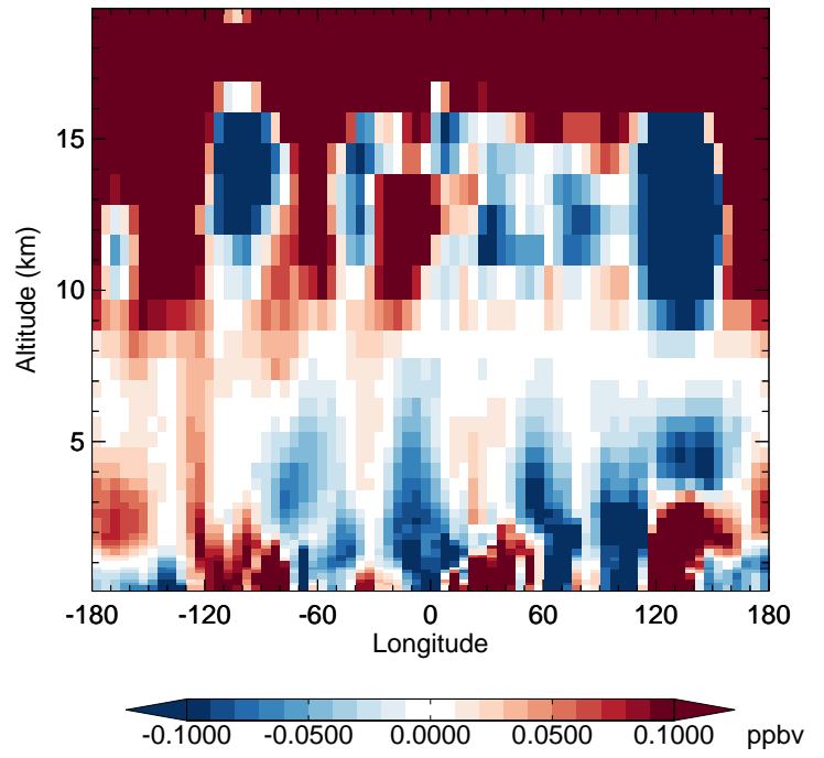
v11-02e-Run1 - v11-02e-Run0 HNO 3 - Diff along 42N for Apr
