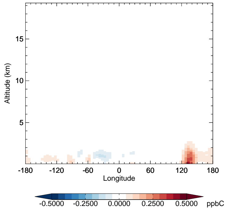
v11-02e-Run1 - v11-02d-Run1 ALD2 - Diff along 42N for Apr
