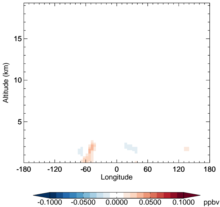
v11-02e-Run1 - v11-02d-Run1 SOAP - Diff along 15S for Apr
