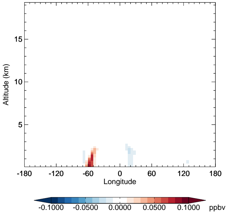
v11-02e-Run1 - v11-02d-Run1 TSOA2 - Diff along 15S for Apr
