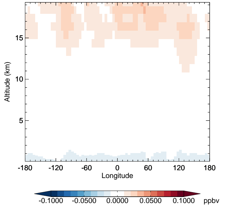
v11-02e-Run1 - v11-02d-Run1 CFC11 - Diff along 42N for Apr
