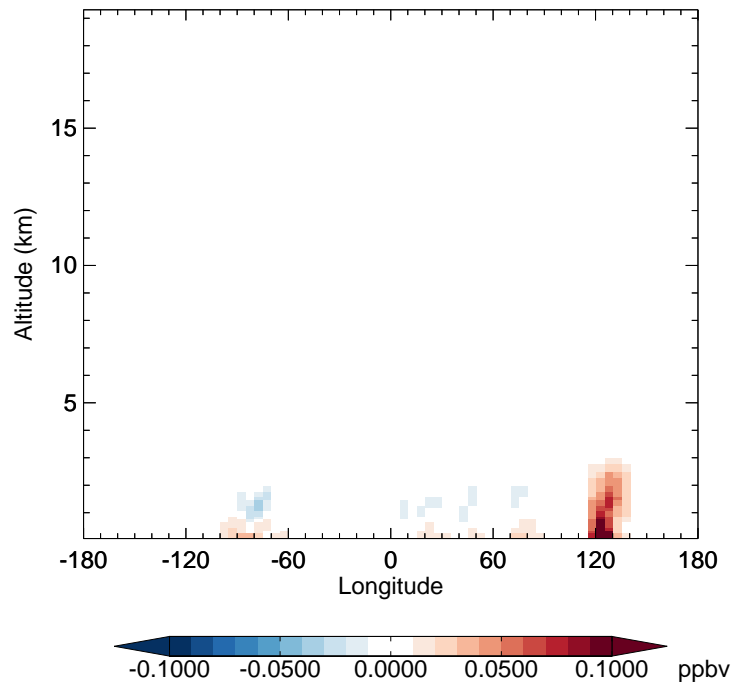
v11-02e-Run1 - v11-02d-Run1 SOAP - Diff along 42N for Apr
