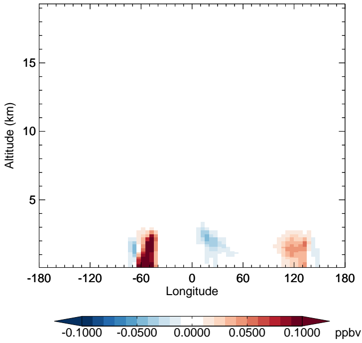
v11-02e-Run1 - v11-02e-Run0 TSOG2 - Diff along 15S for Apr
