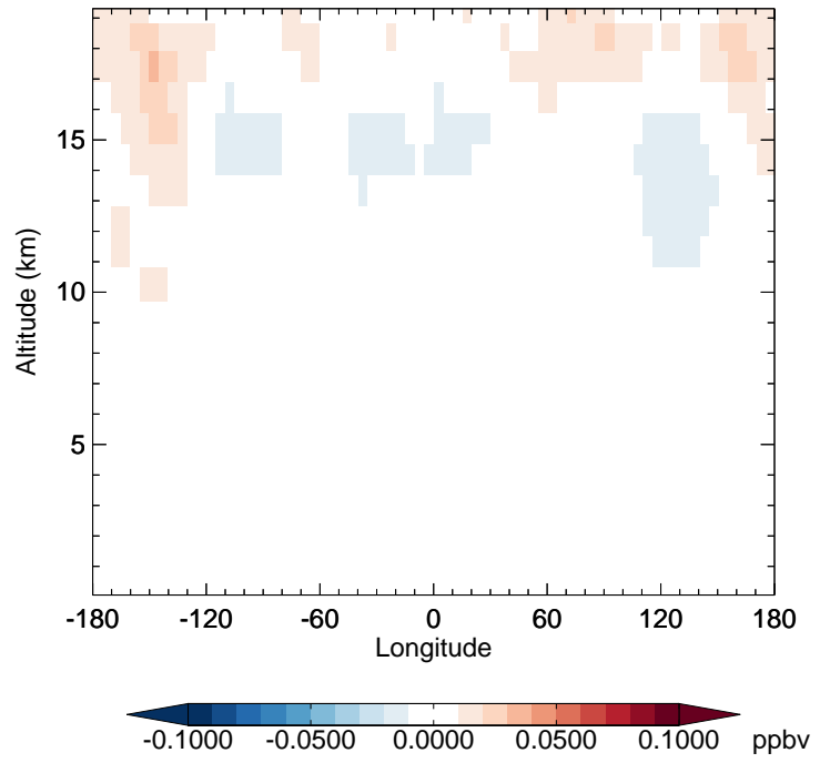
v11-02e-Run1 - v11-02e-Run0 MPN - Diff along 42N for Apr
