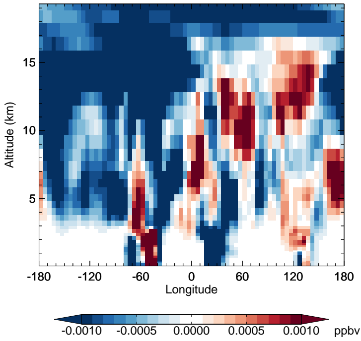
v11-02e-Run1 - v11-02e-Run0 PPN - Diff along 15S for Apr
