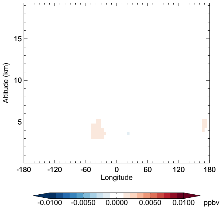
v11-02e-Run1 - v11-02d-Run1 NO3 - Diff along 15S for Apr
