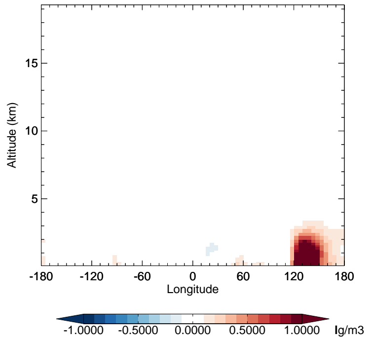
v11-02e-Run1 - v11-02d-Run1 OCPI - Diff along 42N for Apr
