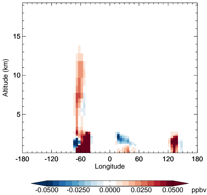
v11-02e-Run1 - v11-02d-Run1 MACR - Diff along 15S for Apr
