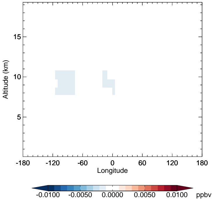
v11-02e-Run1 - v11-02d-Run1 HBr - Diff along 15S for Apr
