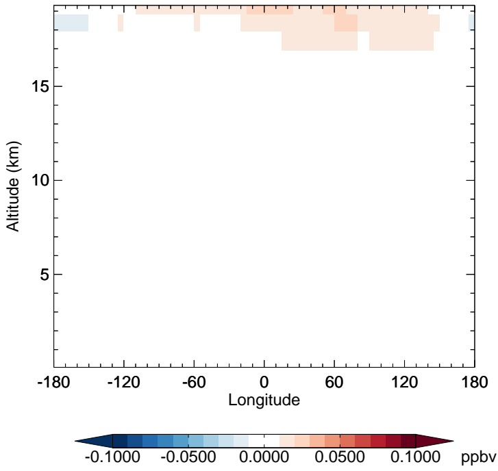
v11-02e-Run1 - v11-02e-Run0 OCS - Diff along 15S for Apr
