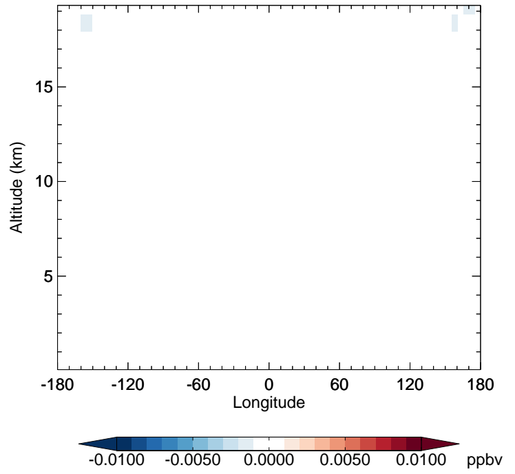
v11-02e-Run1 - v11-02e-Run0 CH3Br - Diff along 42N for Apr
