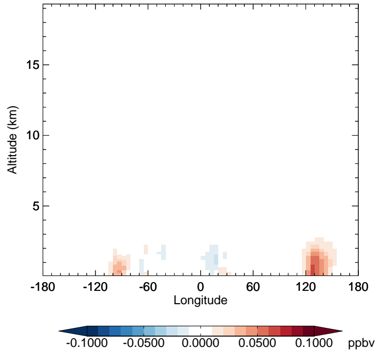
v11-02e-Run1 - v11-02d-Run1 INDIOL - Diff along 42N for Apr
