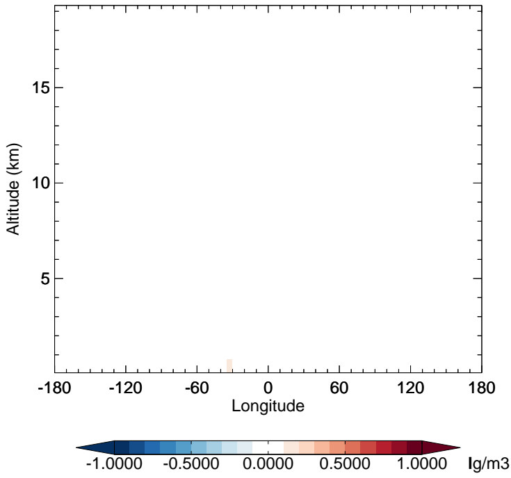
v11-02e-Run1 - v11-02e-Run0 NIT - Diff along 15S for Apr
