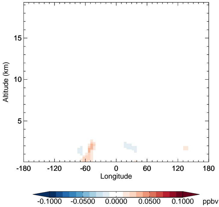
v11-02e-Run1 - v11-02e-Run0 SOAP - Diff along 15S for Apr
