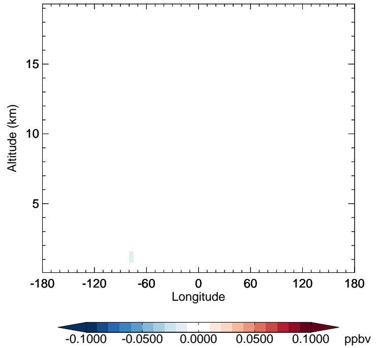
v11-02e-Run1 - v11-02d-Run1 IONITA - Diff along 42N for Apr
