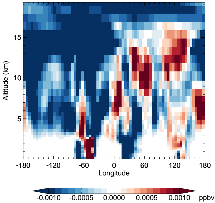
v11-02e-Run1 - v11-02d-Run1 PPN - Diff along 15S for Apr
