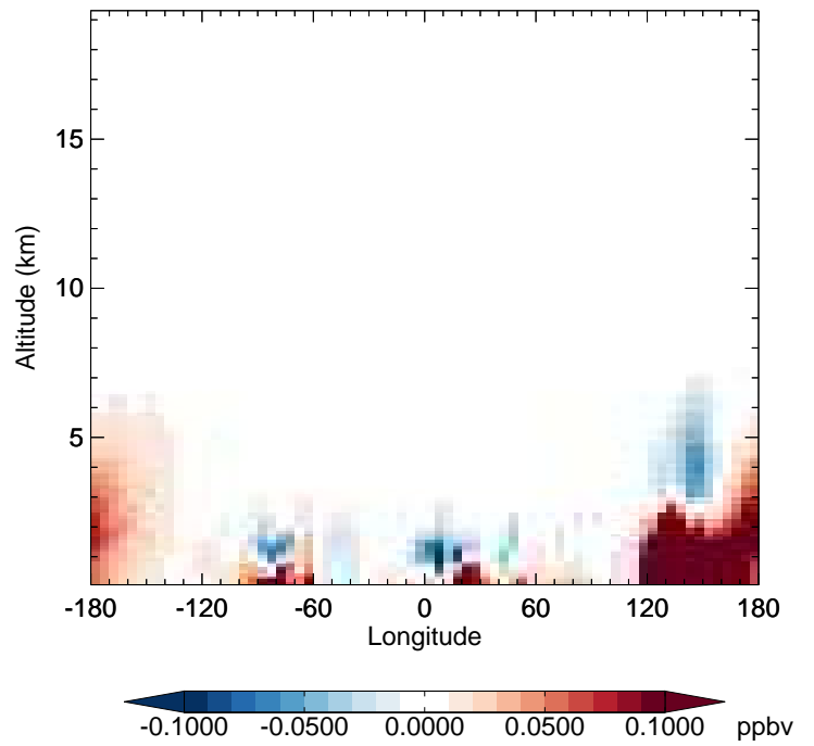
v11-02e-Run1 - v11-02d-Run1 TOLU - Diff along 42N for Apr
