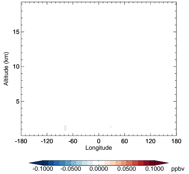
v11-02e-Run1 - v11-02e-Run0 HAC - Diff along 42N for Apr
