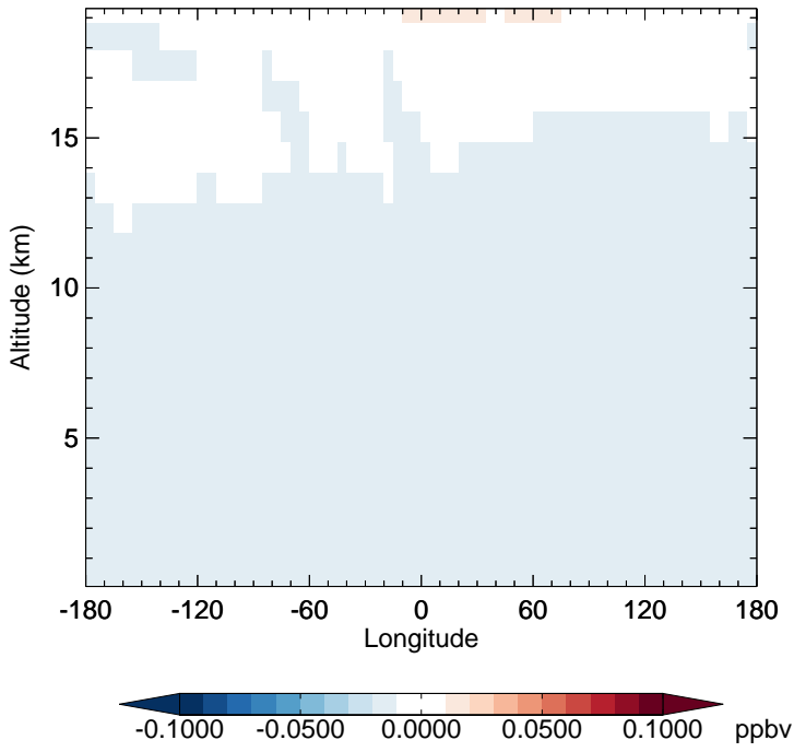
v11-02e-Run1 - v11-02e-Run0 CFC11 - Diff along 15S for Apr
