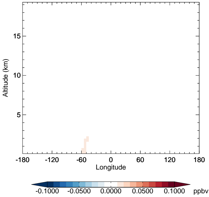
v11-02e-Run1 - v11-02e-Run0 LVOCOA - Diff along 15S for Apr
