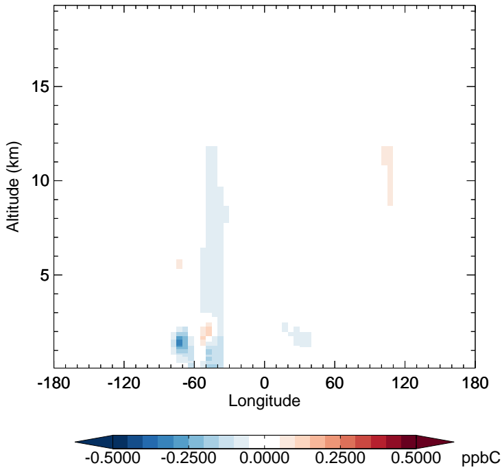
v11-02e-Run1 - v11-02e-Run0 ALK4 - Diff along 15S for Apr
