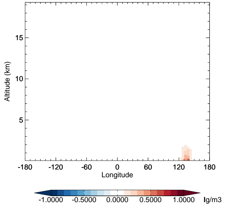
v11-02e-Run1 - v11-02e-Run0 OCPO - Diff along 42N for Apr
