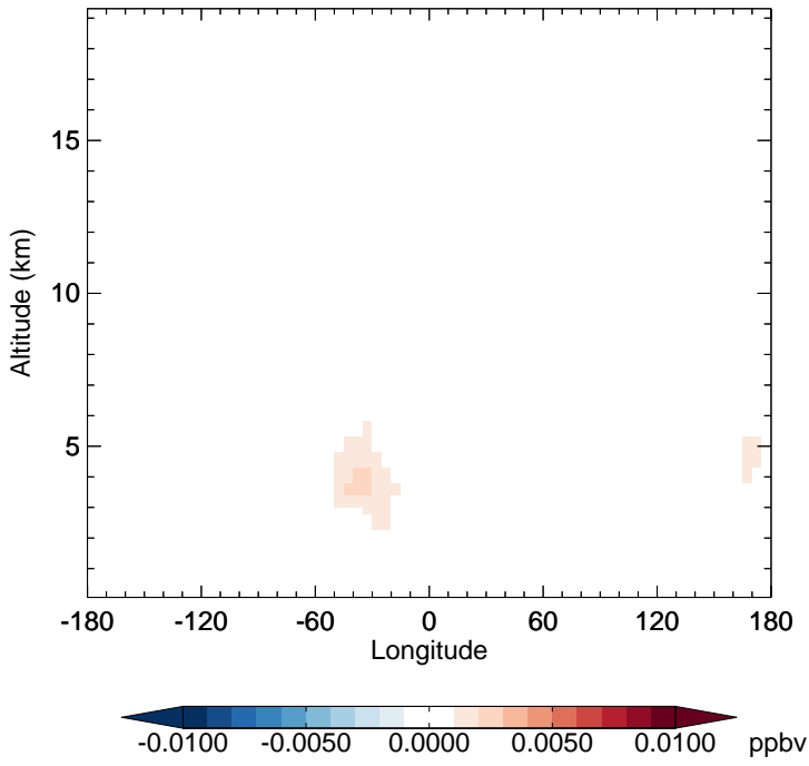
v11-02e-Run1 - v11-02e-Run0 NO3 - Diff along 15S for Apr
