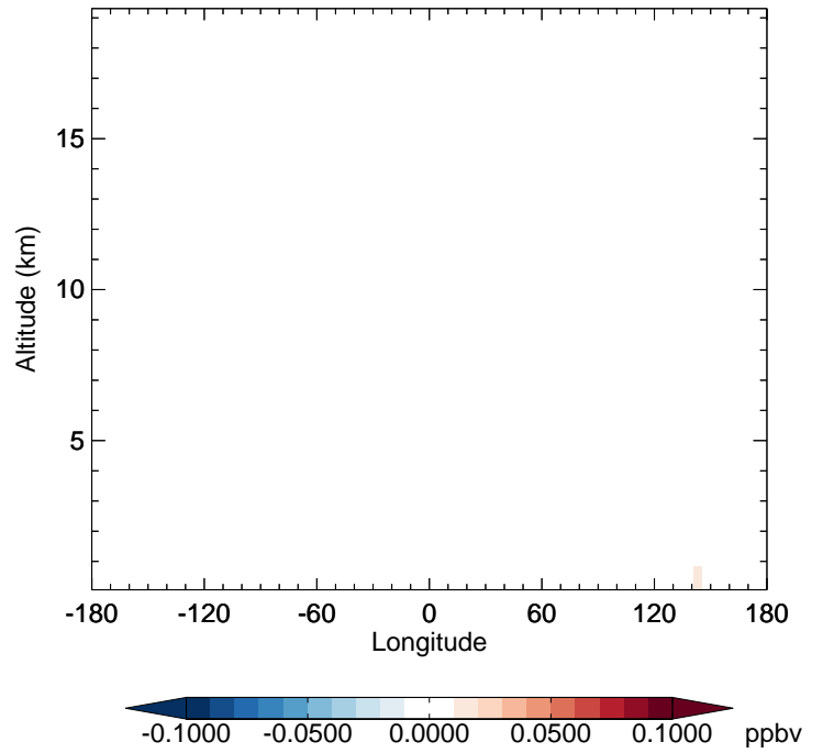
v11-02e-Run1 - v11-02d-Run1 ASOAN - Diff along 42N for Apr
