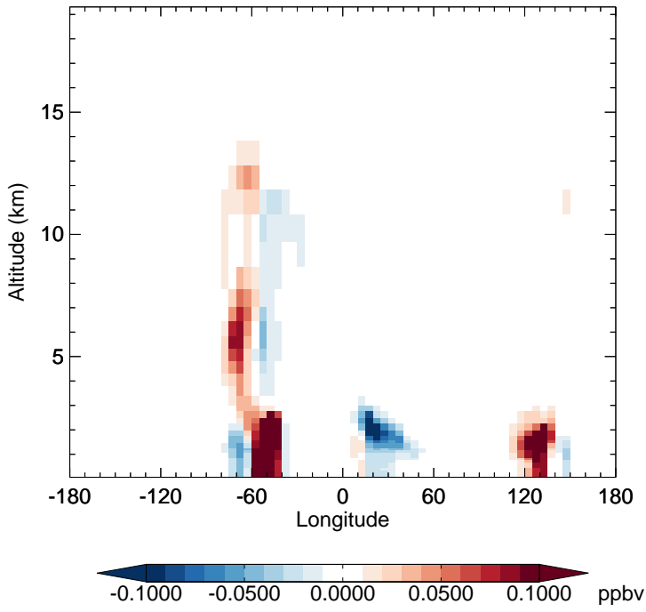
v11-02e-Run1 - v11-02e-Run0 HAC - Diff along 15S for Apr
