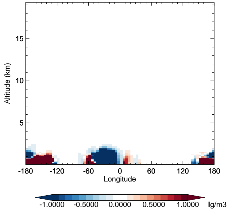
v11-02e-Run1 - v11-02d-Run1 SALC - Diff along 42N for Apr
