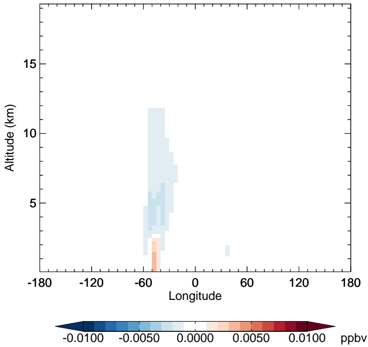
v11-02e-Run1 - v11-02d-Run1 R4N2 - Diff along 15S for Apr
