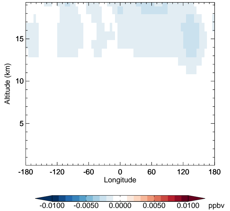
v11-02e-Run1 - v11-02d-Run1 BrNO3 - Diff along 42N for Apr
