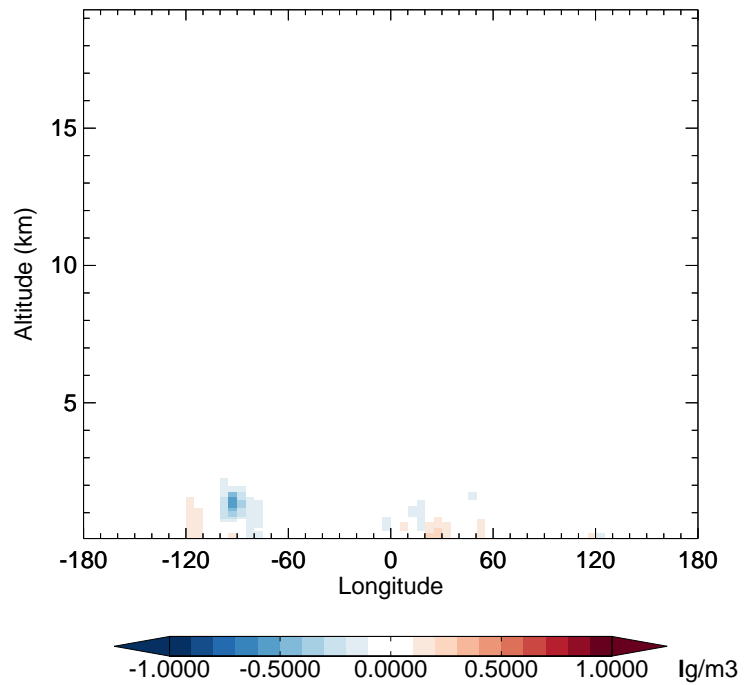
v11-02e-Run1 - v11-02d-Run1 NH3 - Diff along 42N for Apr
