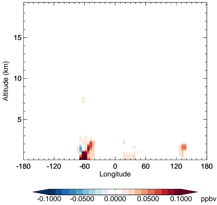
v11-02e-Run1 - v11-02e-Run0 HPALD - Diff along 15S for Apr
