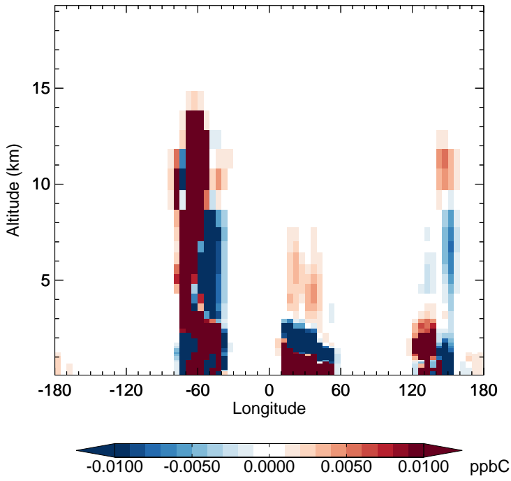
v11-02e-Run1 - v11-02e-Run0 PRPE - Diff along 15S for Apr
