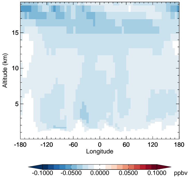
v11-02e-Run1 - v11-02d-Run1 CH3Cl - Diff along 15S for Apr
