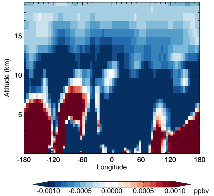
v11-02e-Run1 - v11-02d-Run1 PPN - Diff along 42N for Apr
