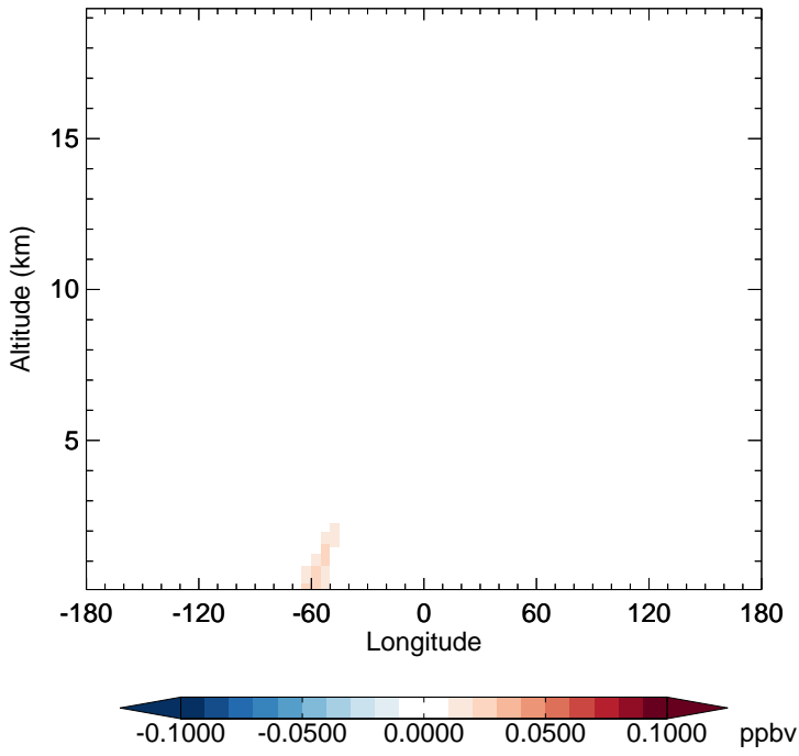
v11-02e-Run1 - v11-02e-Run0 TSOA1 - Diff along 15S for Apr
