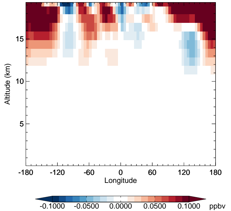
v11-02e-Run1 - v11-02d-Run1 CINO3 - Diff along 42N for Apr
