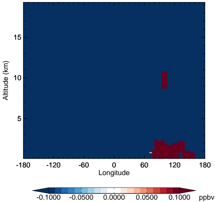
v11-02e-Run1 - v11-02d-Run1 CH4 - Diff along 15S for Apr
