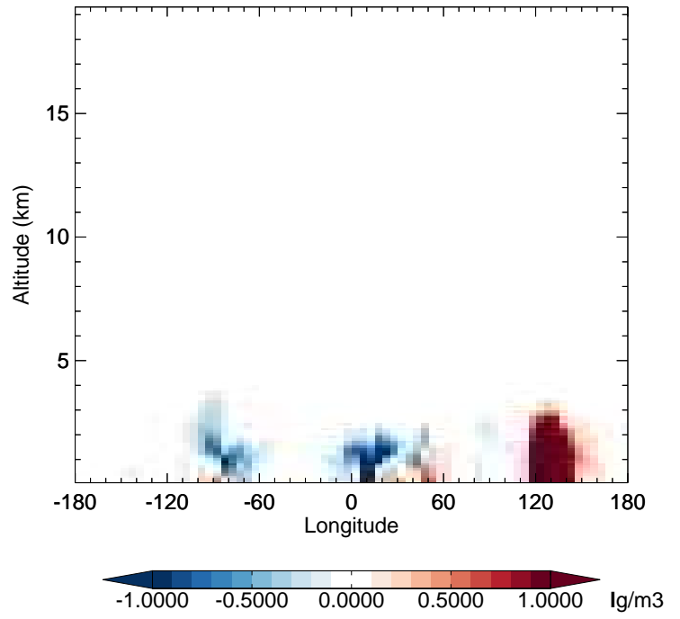
v11-02e-Run1 - v11-02e-Run0 NIT - Diff along 42N for Apr
