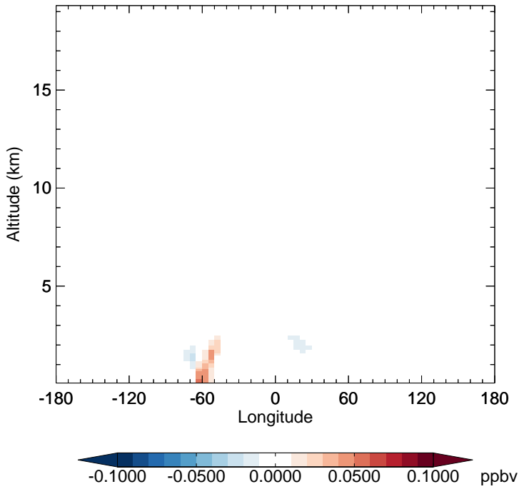
v11-02e-Run1 - v11-02d-Run1 TSOA0 - Diff along 15S for Apr
