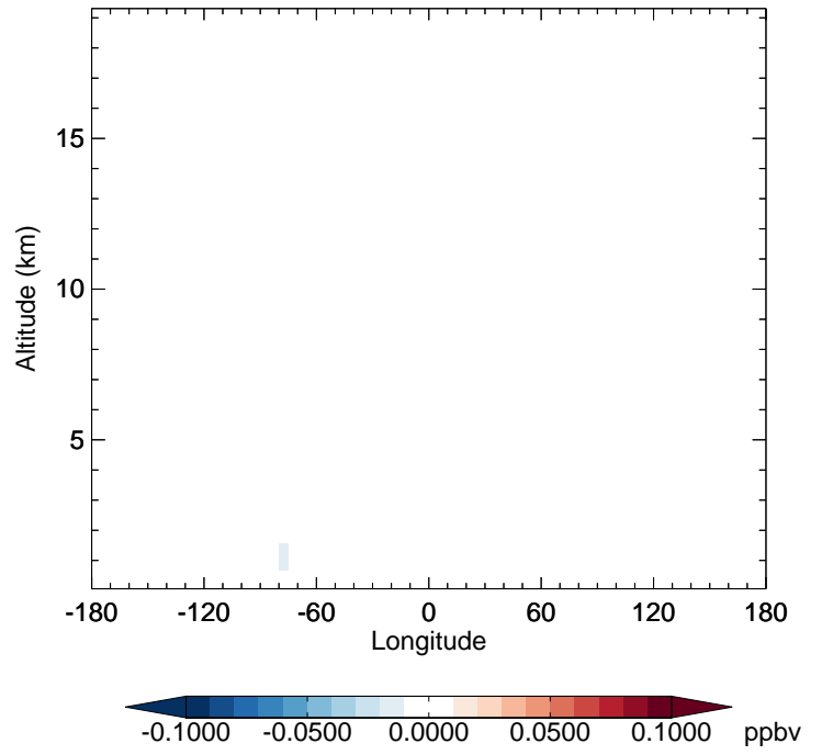
v11-02e-Run1 - v11-02e-Run0 GLYC - Diff along 42N for Apr
