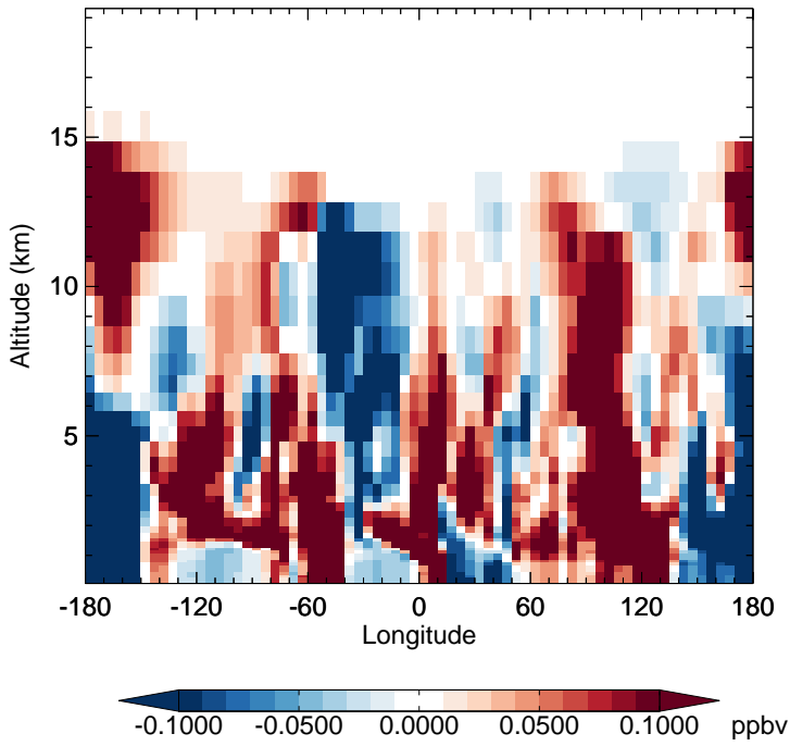
v11-02e-Run1 - v11-02e-Run0 H2O2 - Diff along 15S for Apr
