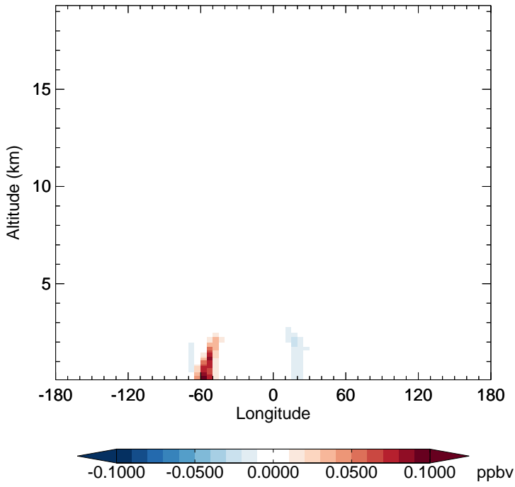
v11-02e-Run1 - v11-02e-Run0 TSOA2 - Diff along 15S for Apr
