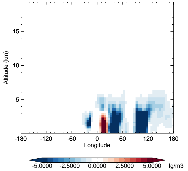
v11-02e-Run1 - v11-02e-Run0 DST2 - Diff along 42N for Apr
