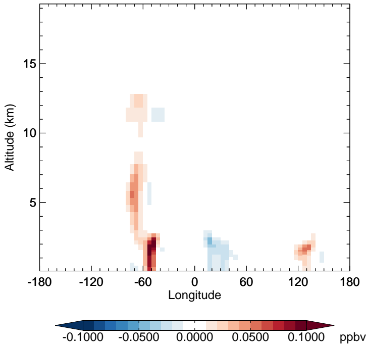
v11-02e-Run1 - v11-02d-Run1 HC187 - Diff along 15S for Apr
