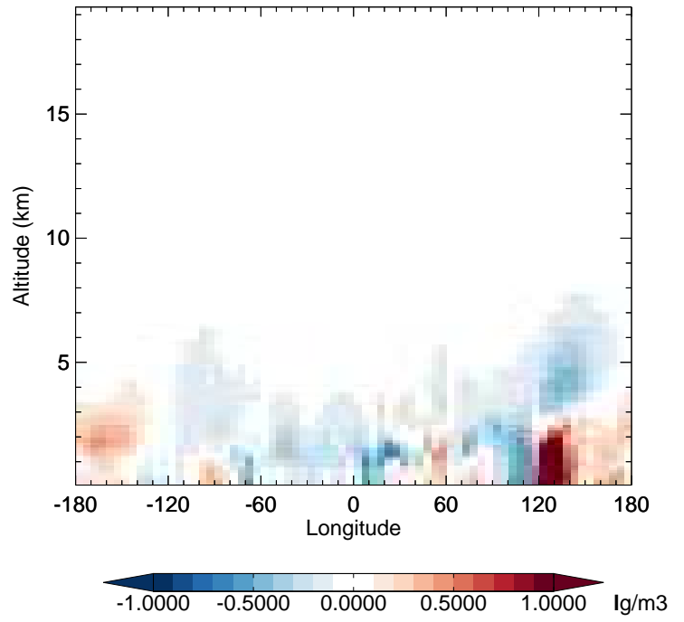
v11-02e-Run1 - v11-02e-Run0 SO4 - Diff along 42N for Apr
