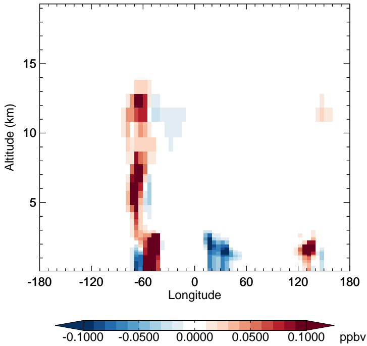
v11-02e-Run1 - v11-02d-Run1 IEPOXA - Diff along 15S for Apr
