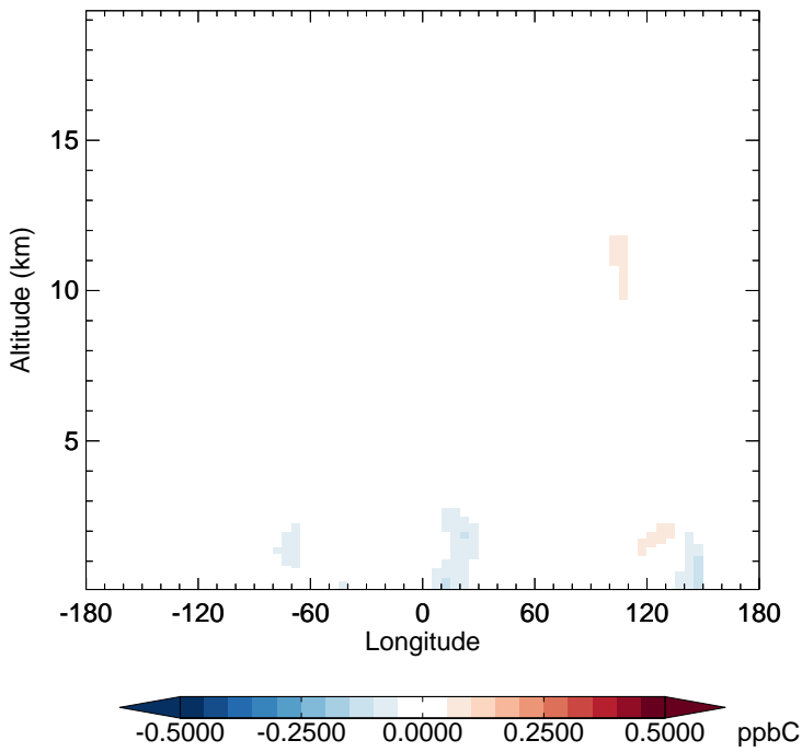
v11-02e-Run1 - v11-02d-Run1 C3H8 - Diff along 15S for Apr
