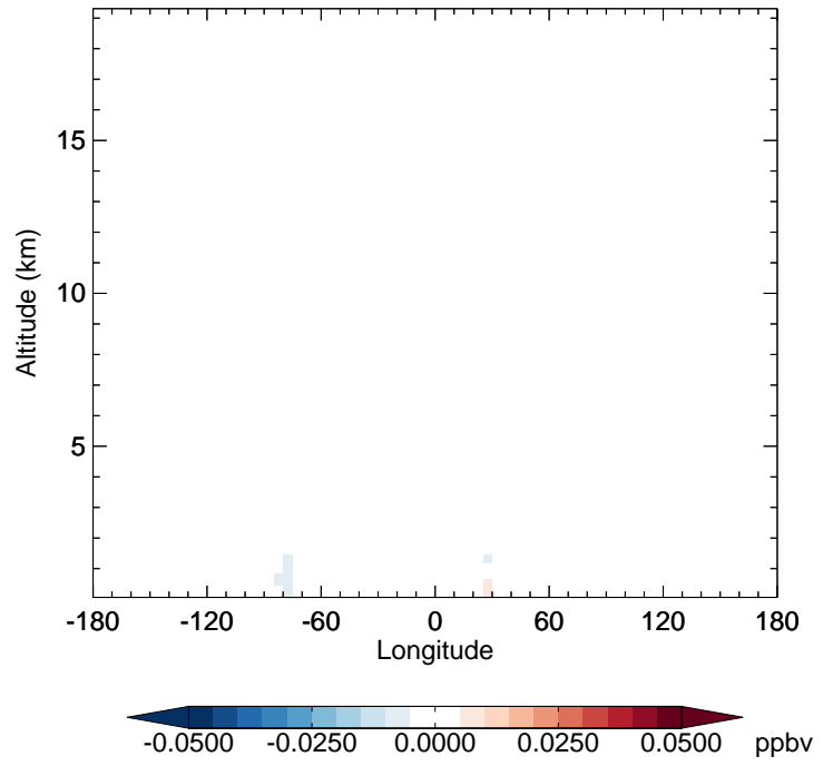
v11-02e-Run1 - v11-02e-Run0 MACR - Diff along 42N for Apr
