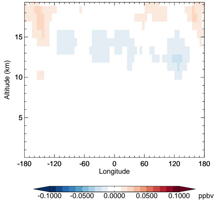
v11-02e-Run1 - v11-02d-Run1 MPN - Diff along 42N for Apr
