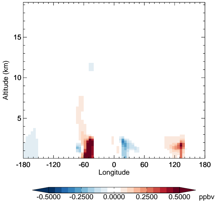
v11-02e-Run1 - v11-02e-Run0 CH 2 O - Diff along 15S for Apr
