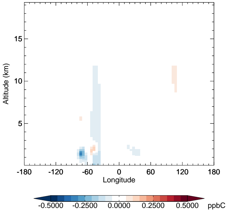
v11-02e-Run1 - v11-02d-Run1 ALK4 - Diff along 15S for Apr
