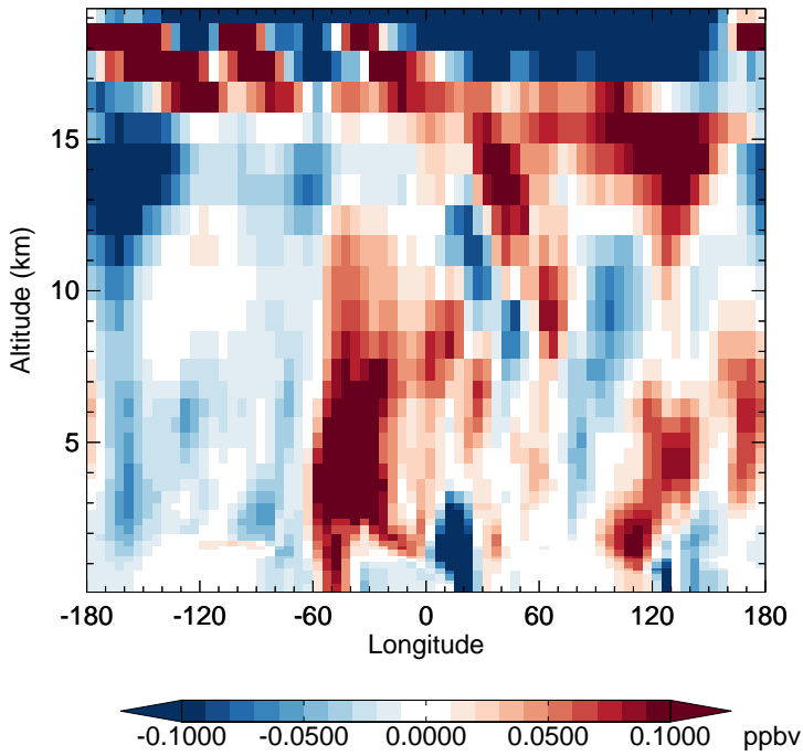
v11-02e-Run1 - v11-02d-Run1 HNO 3 - Diff along 15S for Apr
