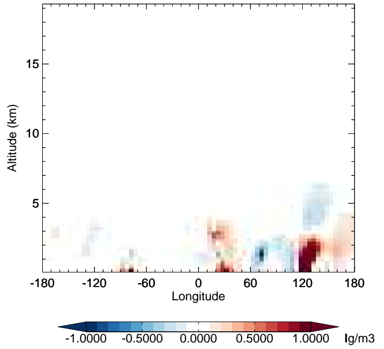
v11-02e-Run1 - v11-02e-Run0 SO 2 - Diff along 42N for Apr
