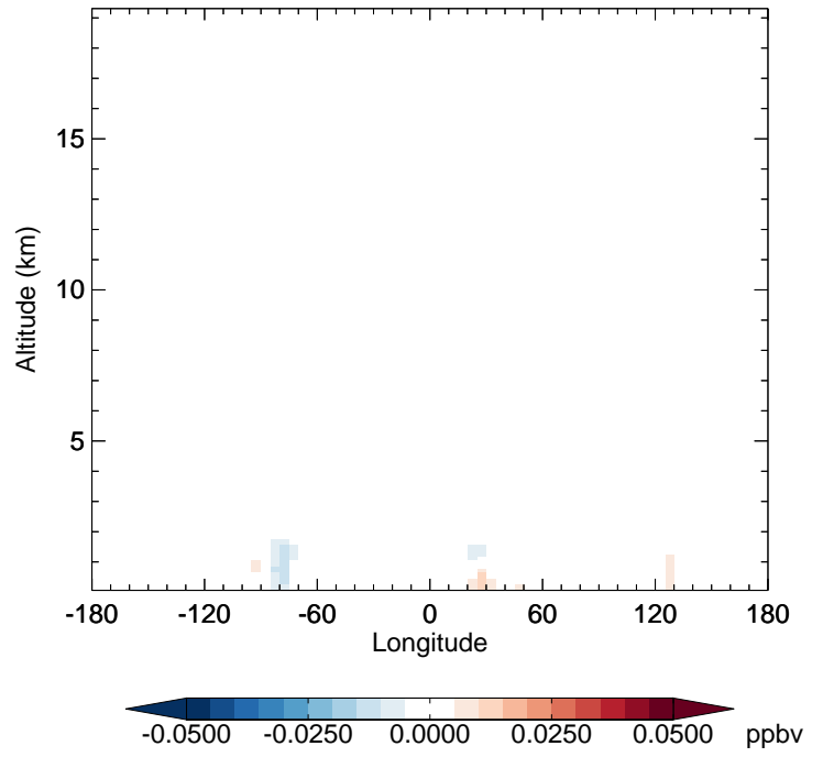
v11-02e-Run1 - v11-02e-Run0 MVK - Diff along 42N for Apr
