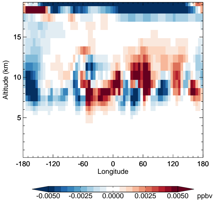
v11-02e-Run1 - v11-02e-Run0 HNO 4 - Diff along 15S for Apr
