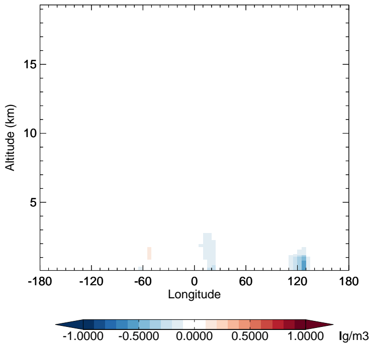
v11-02e-Run1 - v11-02d-Run1 OCPI - Diff along 15S for Apr
