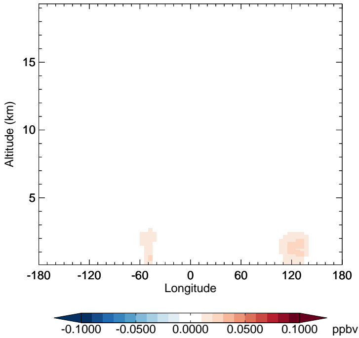
v11-02e-Run1 - v11-02d-Run1 ISOG1 - Diff along 15S for Apr
