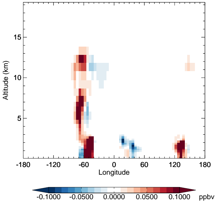
v11-02e-Run1 - v11-02e-Run0 IEPOXA - Diff along 15S for Apr
