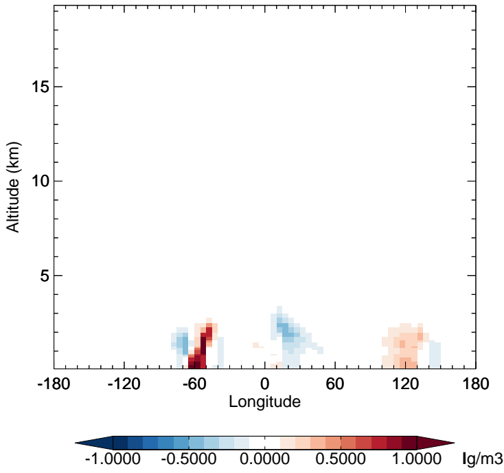
v11-02e-Run1 - v11-02e-Run0 SOAS - Diff along 15S for Apr
