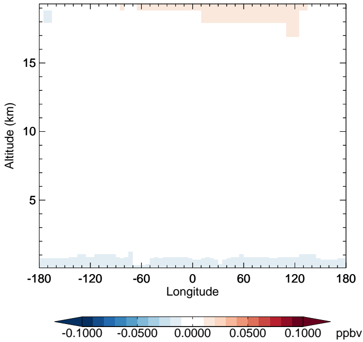
v11-02e-Run1 - v11-02d-Run1 CFC11 - Diff along 15S for Apr
