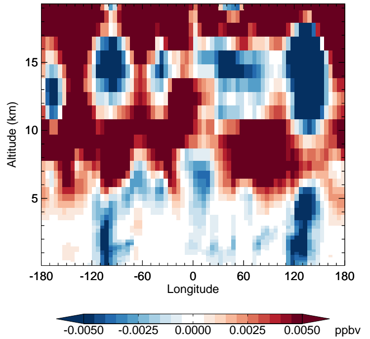
v11-02e-Run1 - v11-02d-Run1 HNO 4 - Diff along 42N for Apr
