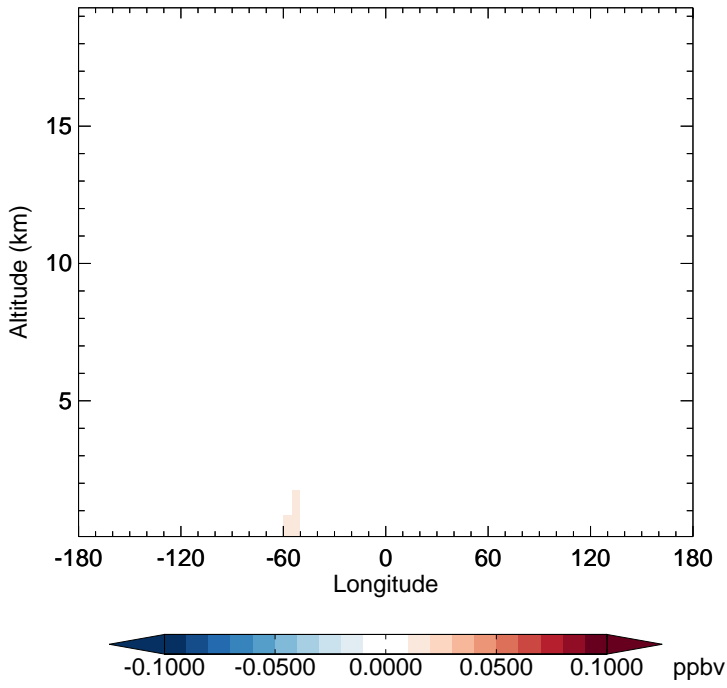
v11-02e-Run1 - v11-02e-Run0 TSOA3 - Diff along 15S for Apr
