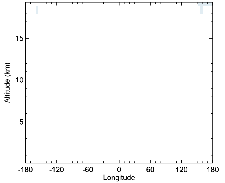
v11-02e-Run1 - v11-02e-Run0 HCFC22 - Diff along 42N for Apr
