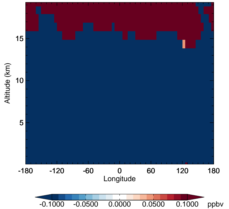
v11-02e-Run1 - v11-02d-Run1 CH4 - Diff along 42N for Apr
