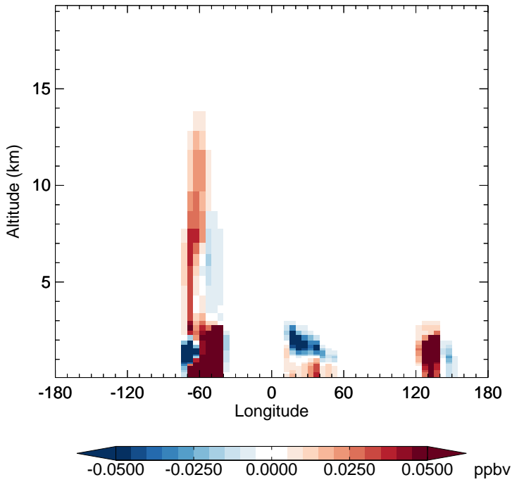
v11-02e-Run1 - v11-02d-Run1 MVK - Diff along 15S for Apr
