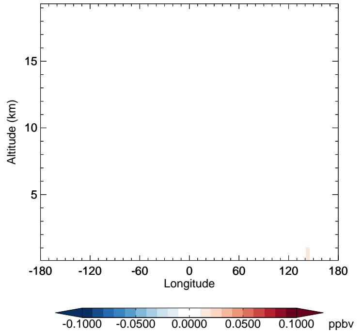
v11-02e-Run1 - v11-02e-Run0 ASOAN - Diff along 42N for Apr
