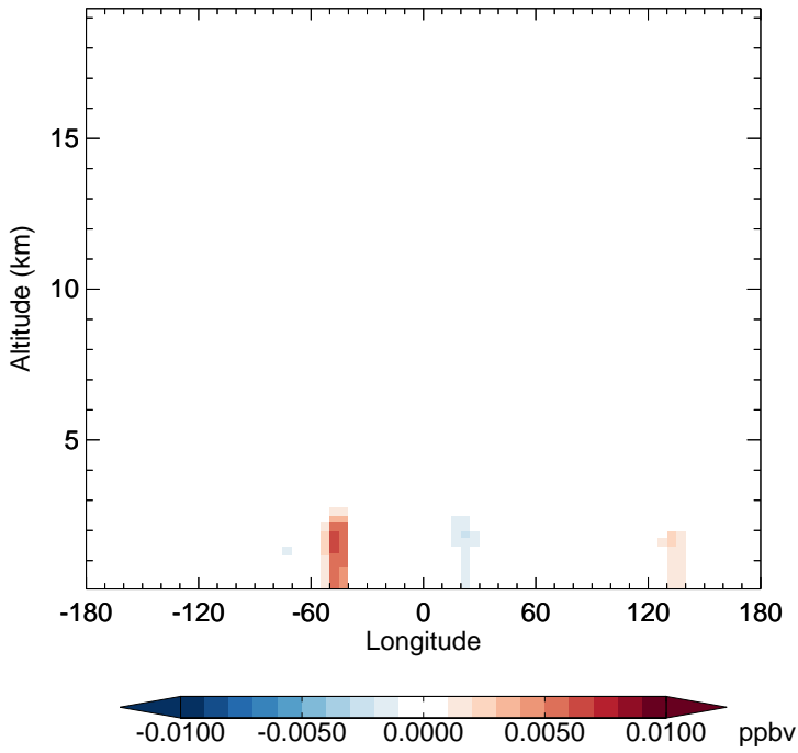
v11-02e-Run1 - v11-02e-Run0 MVKN - Diff along 15S for Apr
