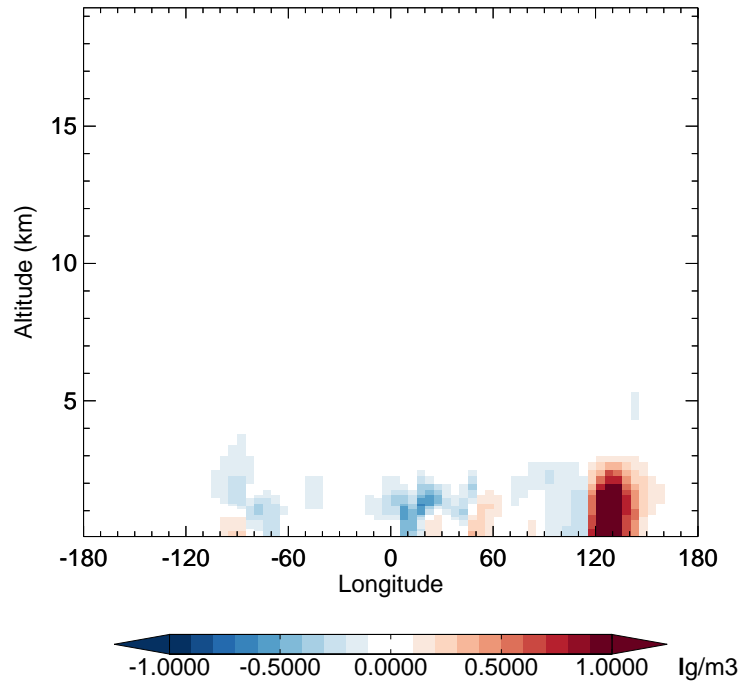
v11-02e-Run1 - v11-02e-Run0 NH4 - Diff along 42N for Apr
