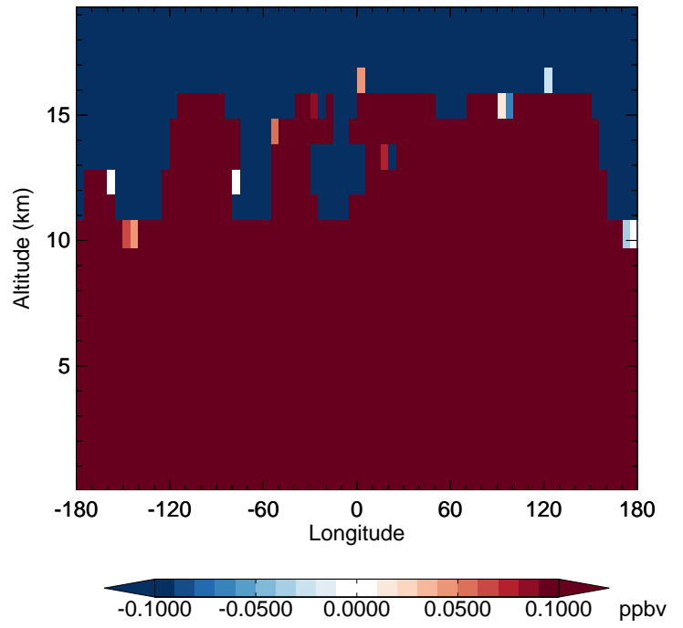
v11-02e-Run1 - v11-02e-Run0 N2O - Diff along 42N for Apr
