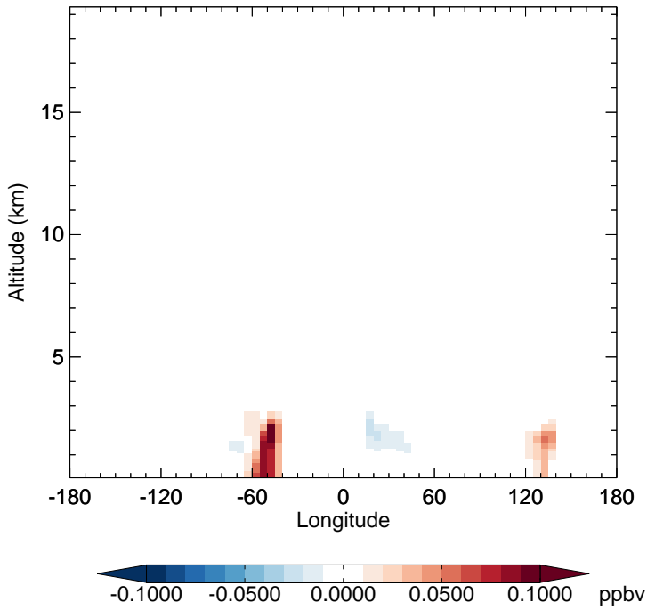
v11-02e-Run1 - v11-02d-Run1 MGLY - Diff along 15S for Apr
