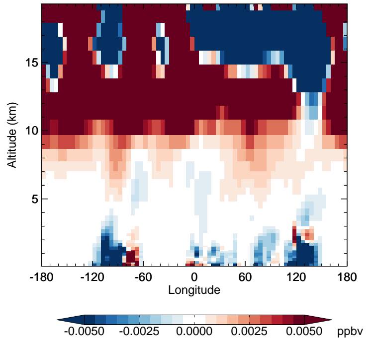
v11-02e-Run1 - v11-02d-Run1 N2O5 - Diff along 42N for Apr
