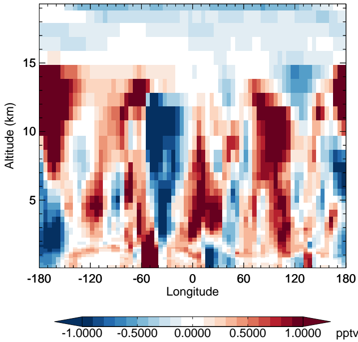
v11-02e-Run1 - v11-02d-Run1 HO2 - Diff along 15S for Apr
