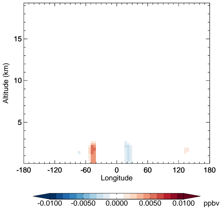
v11-02e-Run1 - v11-02d-Run1 MVKN - Diff along 15S for Apr
