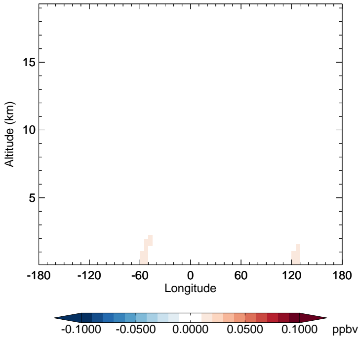
v11-02e-Run1 - v11-02d-Run1 LVOCOA - Diff along 15S for Apr
