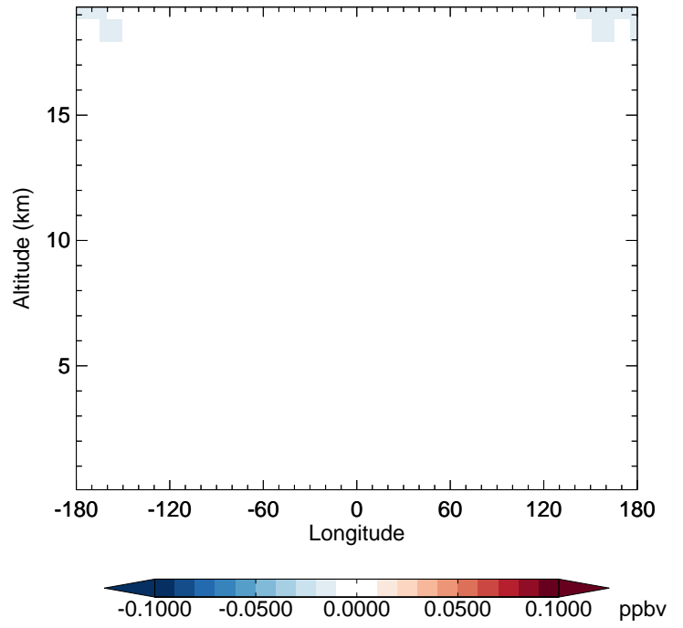
v11-02e-Run1 - v11-02e-Run0 CFC113 - Diff along 42N for Apr
