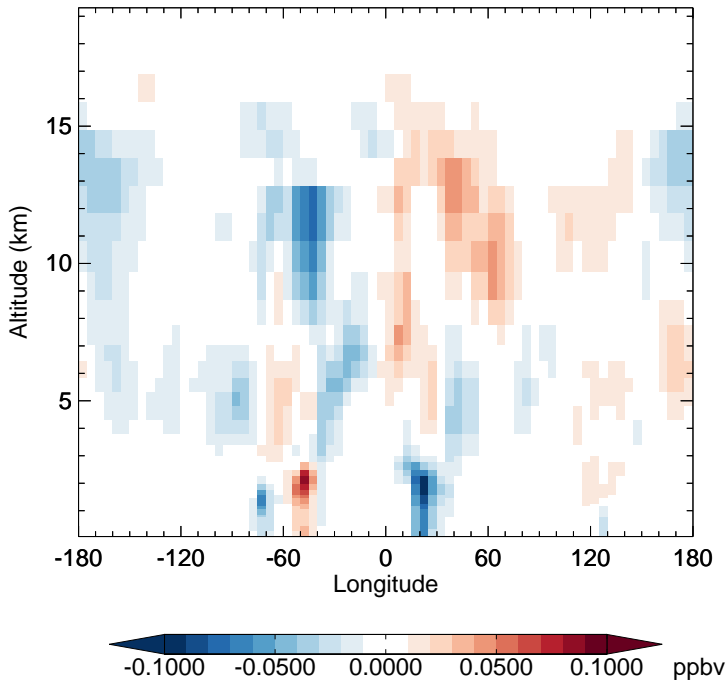
v11-02e-Run1 - v11-02e-Run0 PAN - Diff along 15S for Apr
