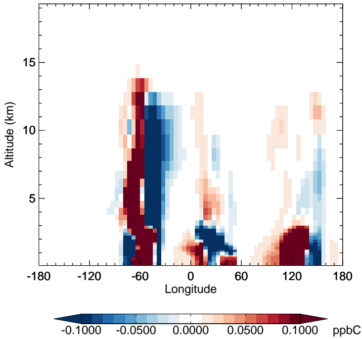
v11-02e-Run1 - v11-02d-Run1 MEK - Diff along 15S for Apr
