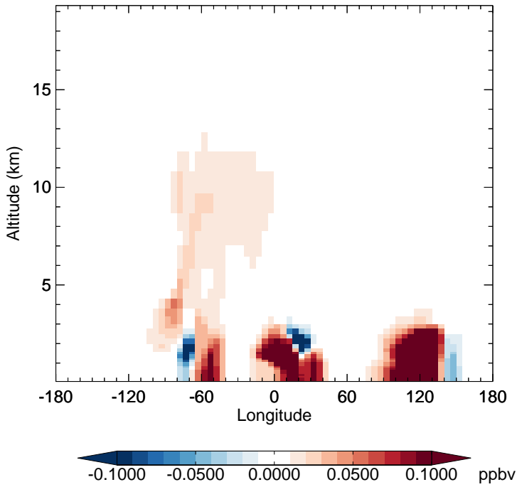
v11-02e-Run1 - v11-02d-Run1 SOAIE - Diff along 15S for Apr
