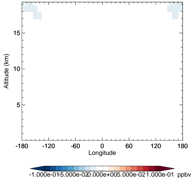
v11-02e-Run1 - v11-02e-Run0 CCI4 - Diff along 42N for Apr
