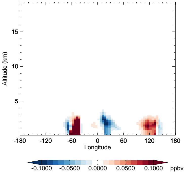
v11-02e-Run1 - v11-02e-Run0 TSOG3 - Diff along 15S for Apr
