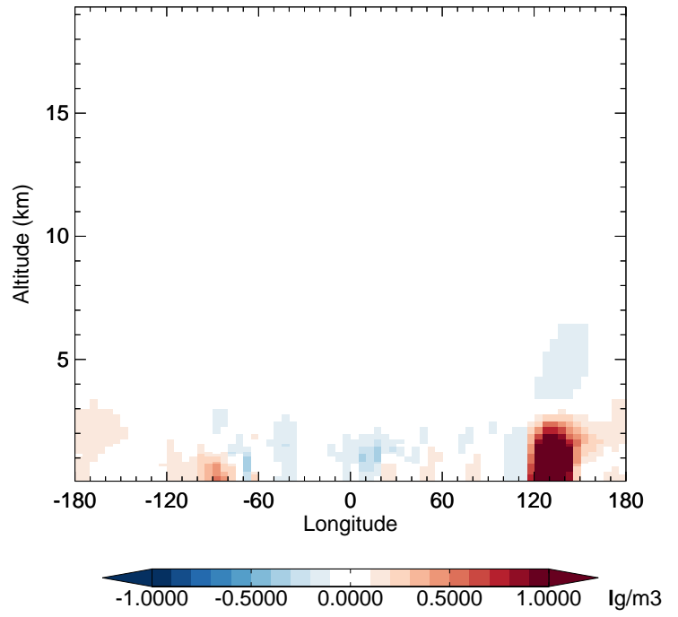
v11-02e-Run1 - v11-02e-Run0 SOAS - Diff along 42N for Apr
