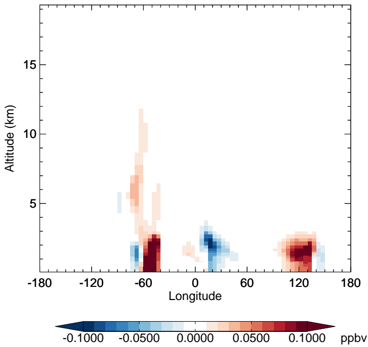
v11-02e-Run1 - v11-02d-Run1 ISO3 - Diff along 15S for Apr
