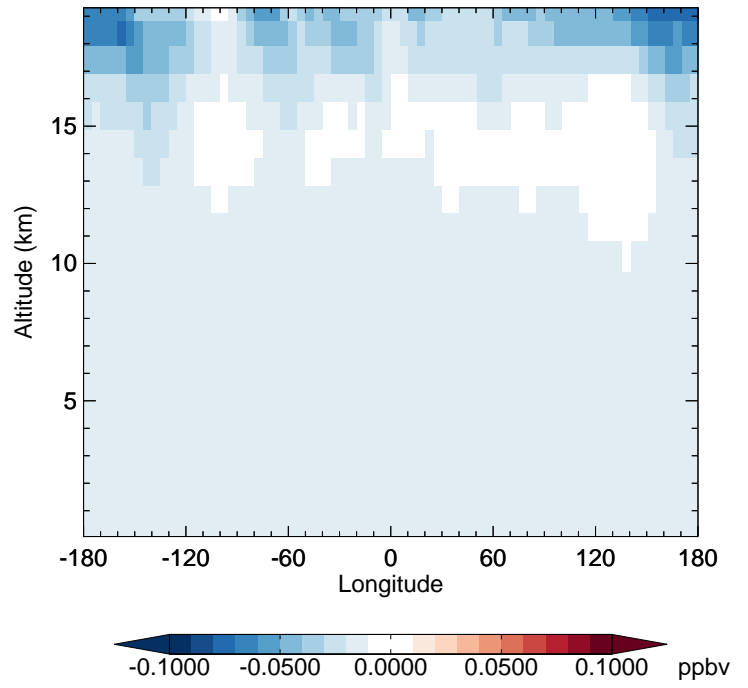
v11-02e-Run1 - v11-02e-Run0 CFC12 - Diff along 42N for Apr
