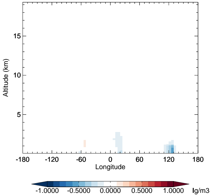
v11-02e-Run1 - v11-02e-Run0 OCPI - Diff along 15S for Apr
