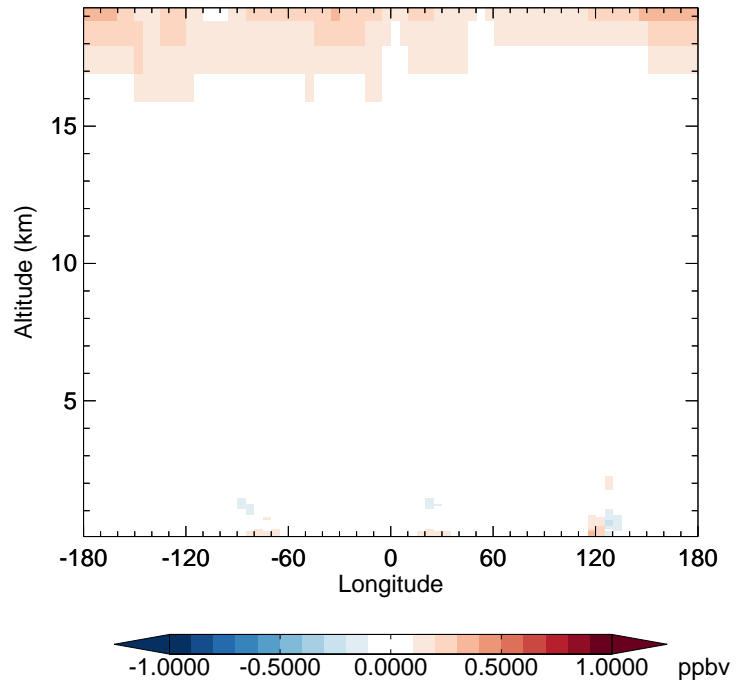
v11-02e-Run1 - v11-02e-Run0 NO2 - Diff along 42N for Apr
