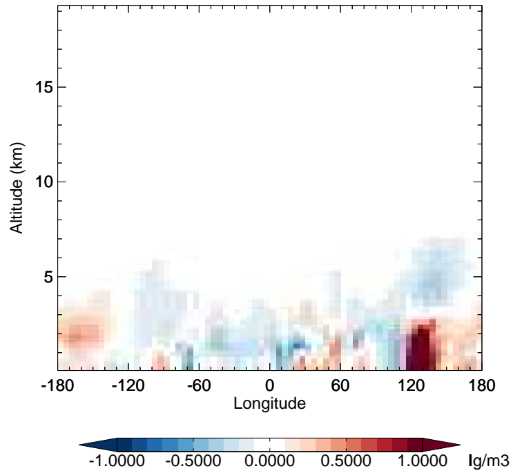
v11-02e-Run1 - v11-02d-Run1 SO4 - Diff along 42N for Apr
