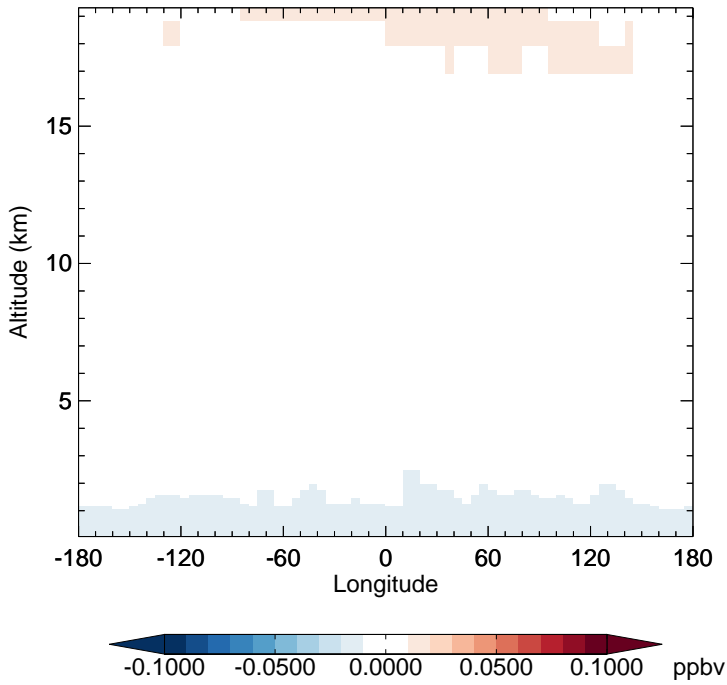
v11-02e-Run1 - v11-02d-Run1 CFC12 - Diff along 15S for Apr
