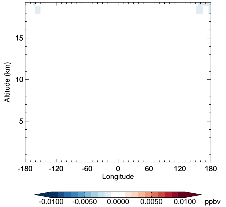
v11-02e-Run1 - v11-02d-Run1 CH3Br - Diff along 42N for Apr
