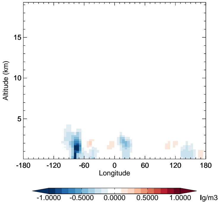
v11-02e-Run1 - v11-02d-Run1 SO4 - Diff along 15S for Apr
