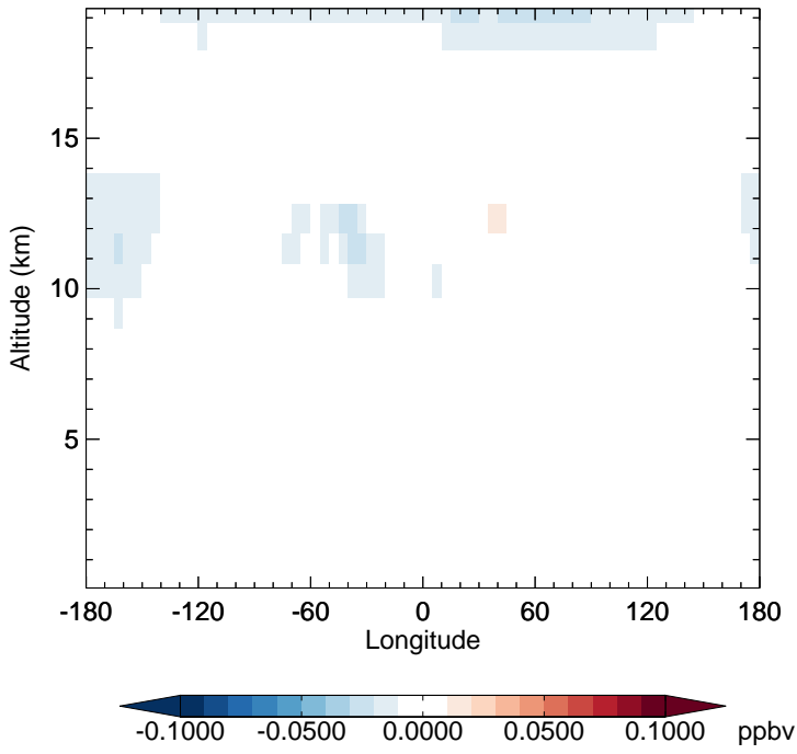
v11-02e-Run1 - v11-02e-Run0 MPN - Diff along 15S for Apr
