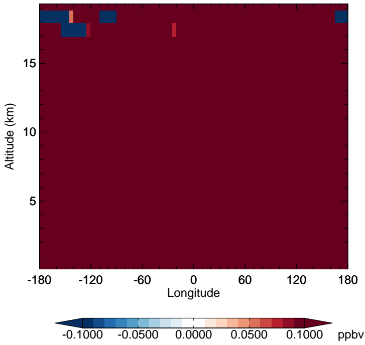
v11-02e-Run1 - v11-02e-Run0 N2O - Diff along 15S for Apr
