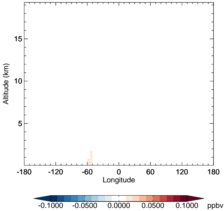
v11-02e-Run1 - v11-02d-Run1 TSOA3 - Diff along 15S for Apr
