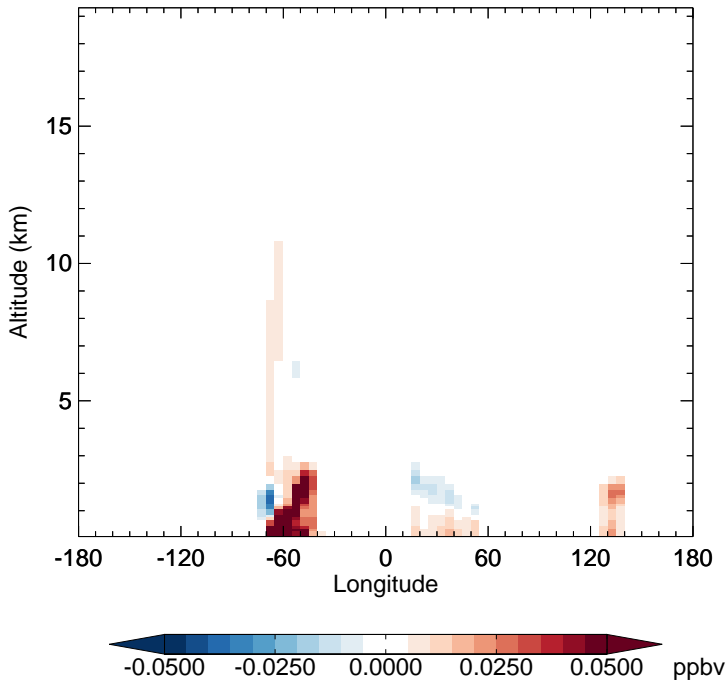
v11-02e-Run1 - v11-02d-Run1 RCHO - Diff along 15S for Apr
