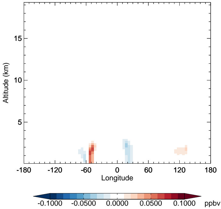
v11-02e-Run1 - v11-02e-Run0 IONITA - Diff along 15S for Apr
