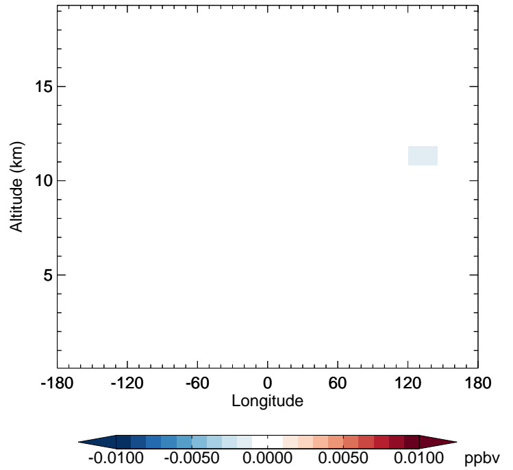
v11-02e-Run1 - v11-02d-Run1 HOBr - Diff along 42N for Apr
