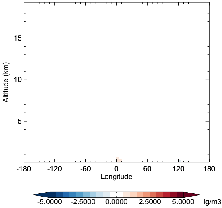
v11-02e-Run1 - v11-02e-Run0 DST2 - Diff along 15S for Apr
