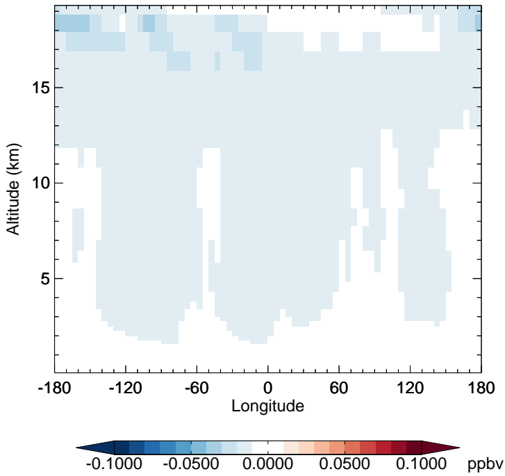
v11-02e-Run1 - v11-02d-Run1 OCS - Diff along 15S for Apr
