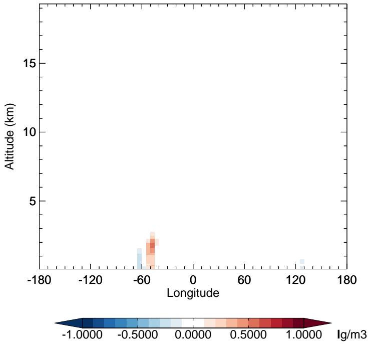
v11-02e-Run1 - v11-02e-Run0 NH3 - Diff along 15S for Apr
