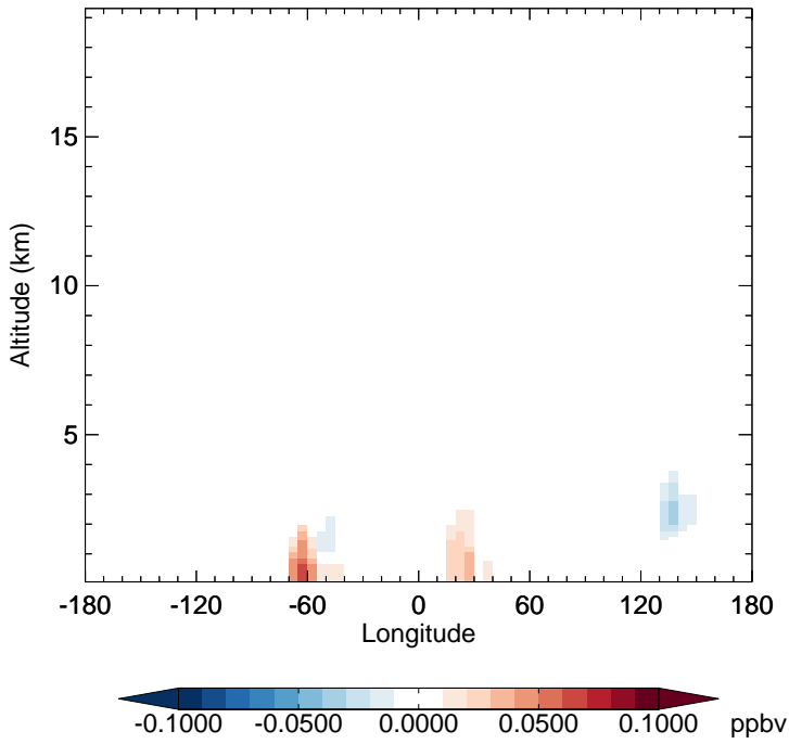
v11-02e-Run1 - v11-02e-Run0 ISOA1 - Diff along 15S for Jan
