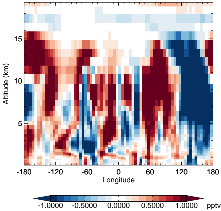
v11-02e-Run1 - v11-02d-Run1 HO2 - Diff along 15S for Jan
