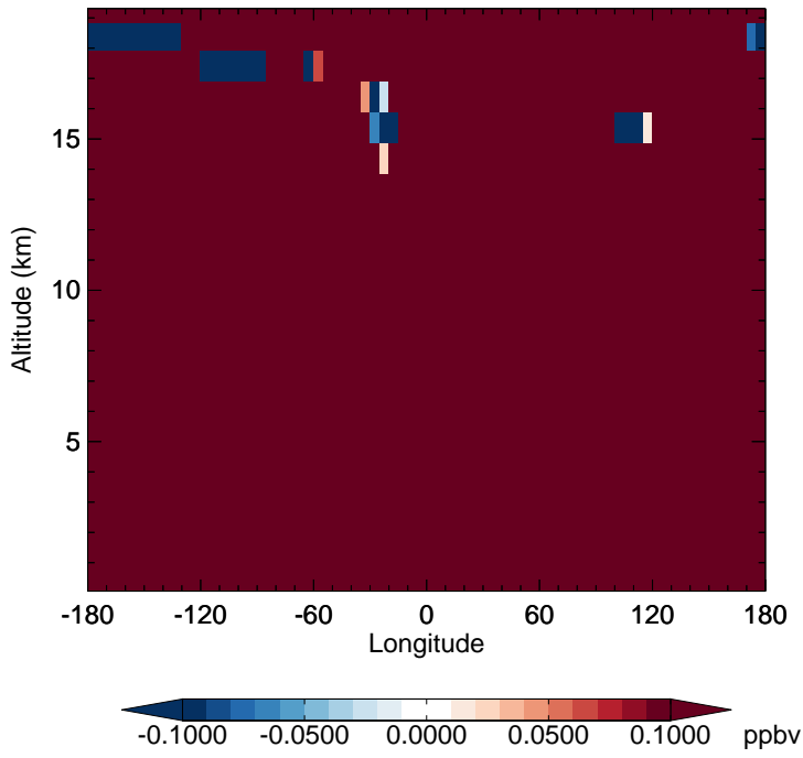
v11-02e-Run1 - v11-02e-Run0 N2O - Diff along 15S for Jan
