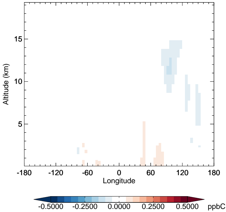
v11-02e-Run1 - v11-02d-Run1 C3H8 - Diff along 15S for Jan
