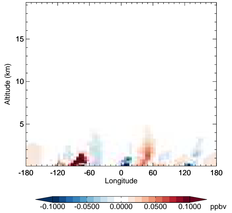
v11-02e-Run1 - v11-02e-Run0 EOH - Diff along 42N for Jan
