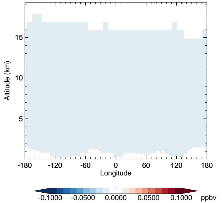
v11-02e-Run1 - v11-02d-Run1 HCFC22 - Diff along 42N for Jan
