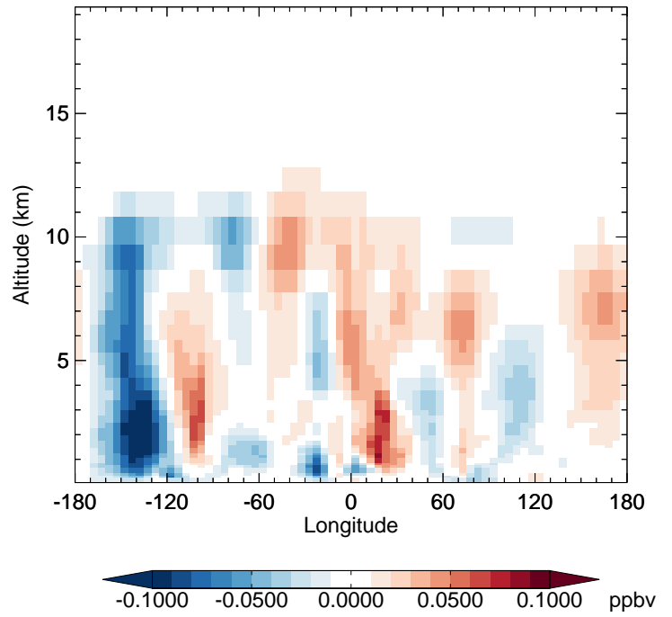
v11-02e-Run1 - v11-02e-Run0 H2O2 - Diff along 42N for Jan
