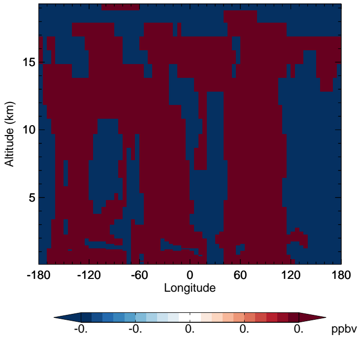
v11-02e-Run1 - v11-02e-Run0 H2O - Diff along 15S for Jan
