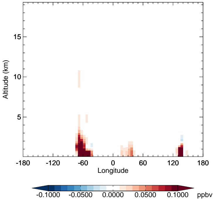
v11-02e-Run1 - v11-02d-Run1 HPALD - Diff along 15S for Jan
