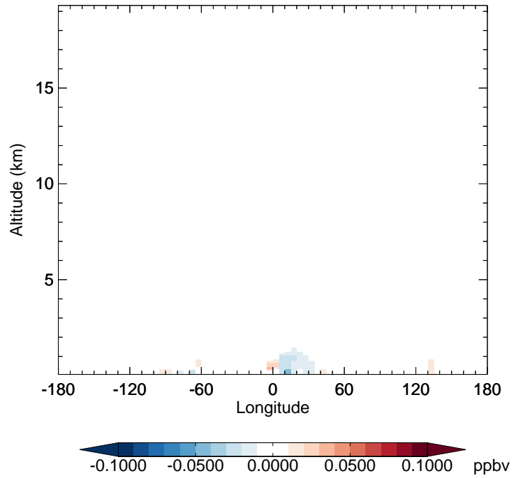
v11-02e-Run1 - v11-02d-Run1 CINO2 - Diff along 42N for Jan
