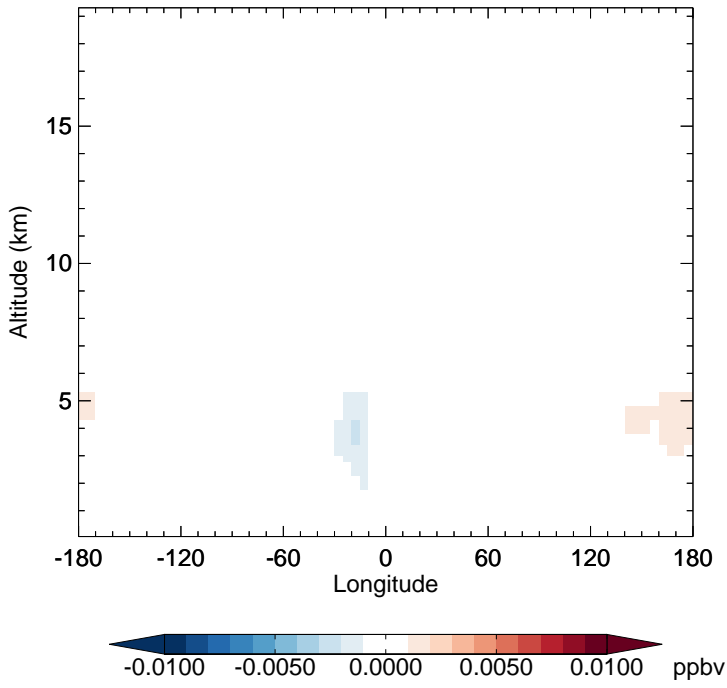
v11-02e-Run1 - v11-02e-Run0 NO3 - Diff along 15S for Jan
