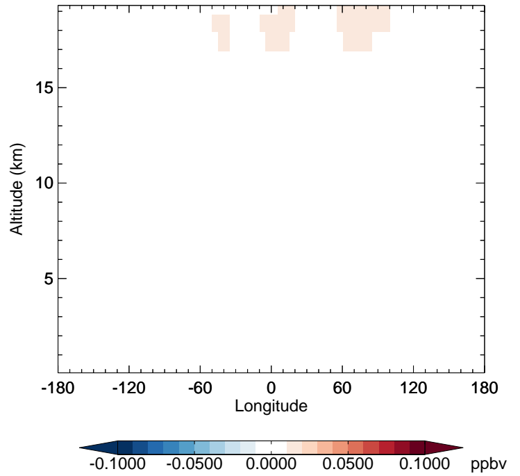
v11-02e-Run1 - v11-02d-Run1 CCI4 - Diff along 42N for Jan
