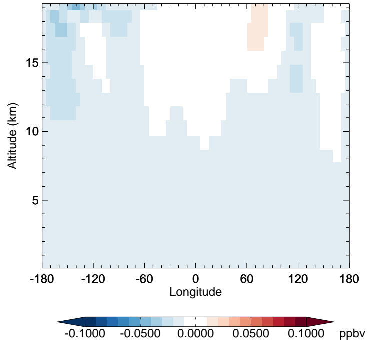
v11-02e-Run1 - v11-02e-Run0 CFC12 - Diff along 42N for Jan
