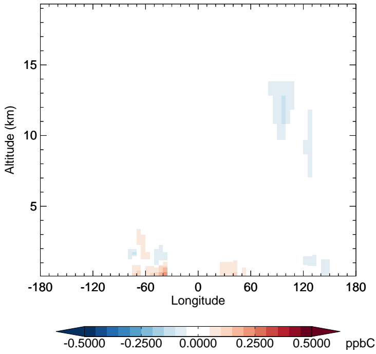
v11-02e-Run1 - v11-02e-Run0 ALK4 - Diff along 15S for Jan
