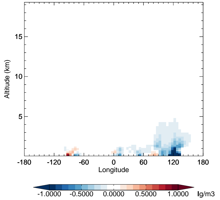
v11-02e-Run1 - v11-02e-Run0 NH4 - Diff along 42N for Jan
