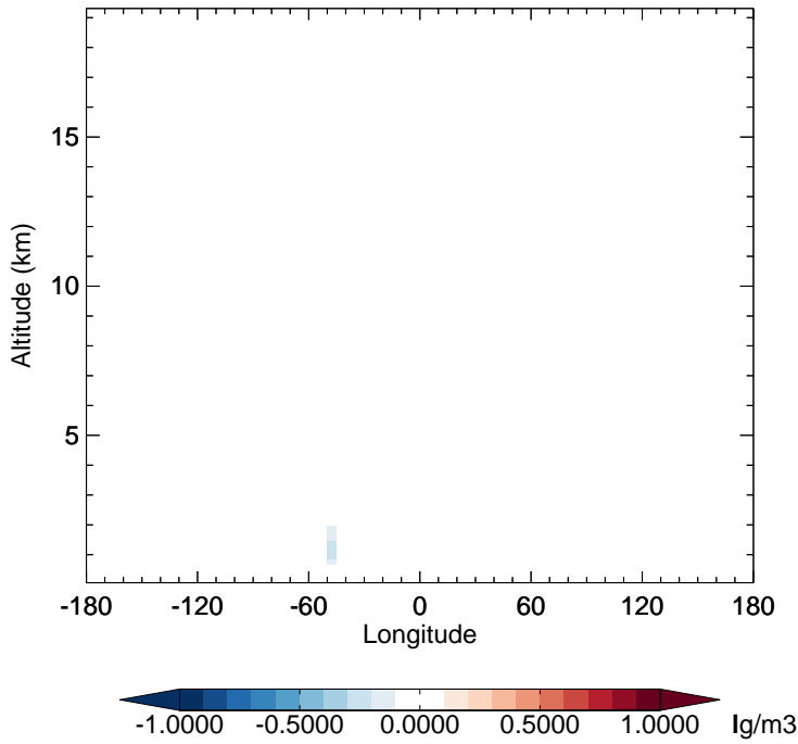
v11-02e-Run1 - v11-02d-Run1 NH3 - Diff along 15S for Jan
