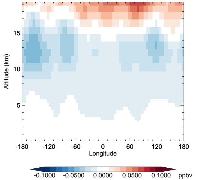
v11-02e-Run1 - v11-02d-Run1 CH3Cl - Diff along 42N for Jan
