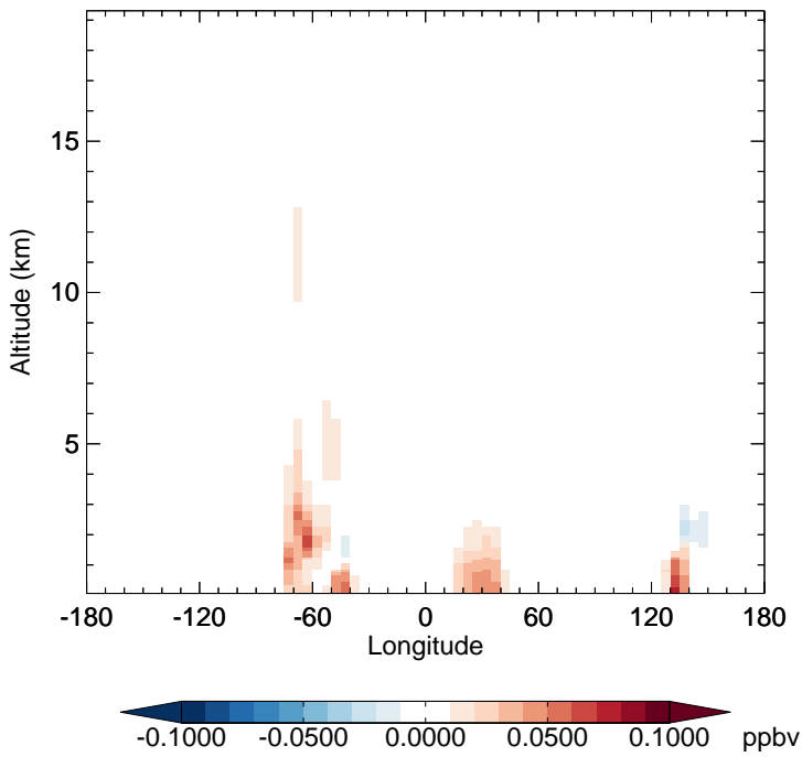
v11-02e-Run1 - v11-02d-Run1 IPMN - Diff along 15S for Jan
