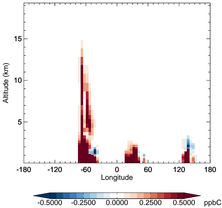
v11-02e-Run1 - v11-02d-Run1 ISOP - Diff along 15S for Jan
