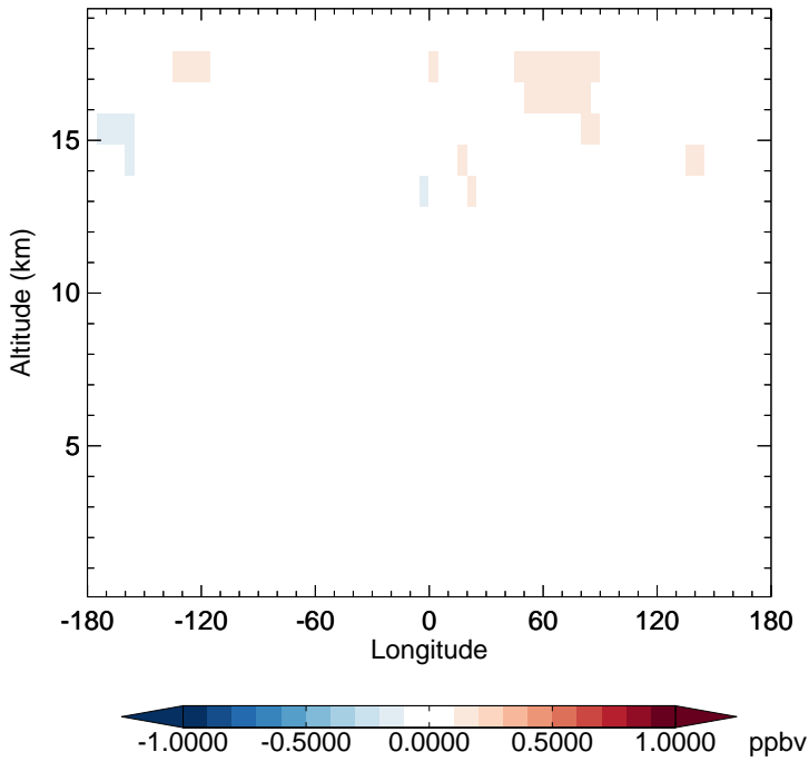
v11-02e-Run1 - v11-02d-Run1 NO - Diff along 15S for Jan
