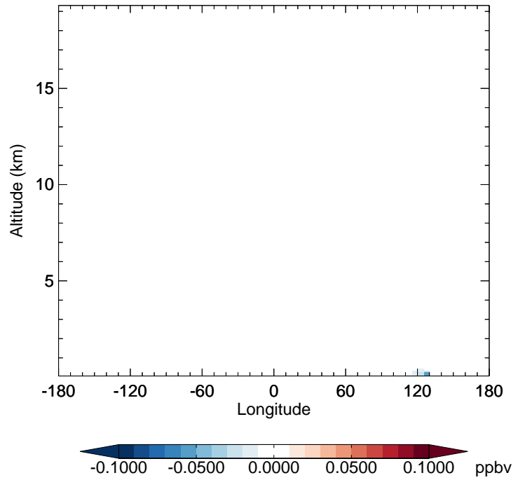
v11-02e-Run1 - v11-02d-Run1 MGLY - Diff along 42N for Jan
