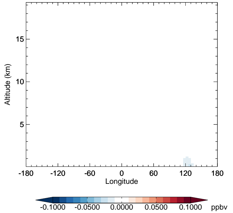
v11-02e-Run1 - v11-02e-Run0 ASOG3 - Diff along 42N for Jan
