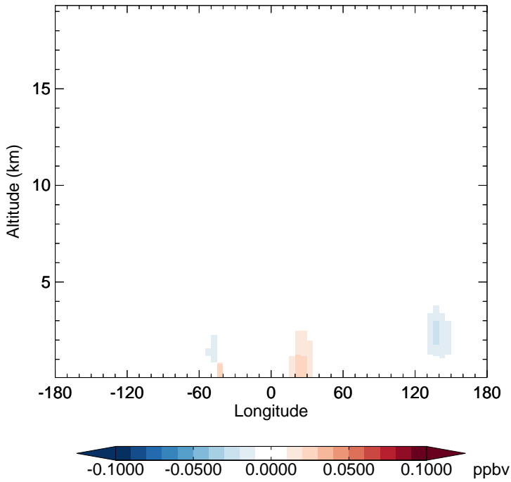
v11-02e-Run1 - v11-02d-Run1 IONITA - Diff along 15S for Jan
