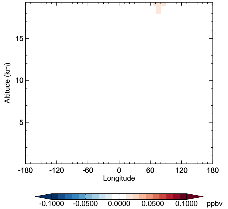
v11-02e-Run1 - v11-02d-Run1 CFC113 - Diff along 42N for Jan
