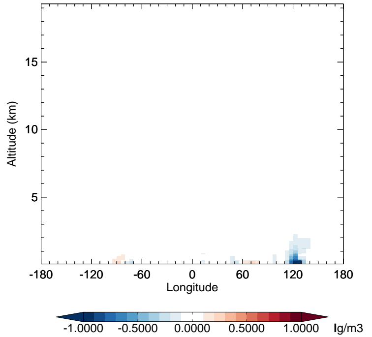
v11-02e-Run1 - v11-02d-Run1 OCPI - Diff along 42N for Jan
