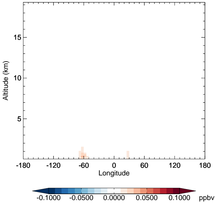
v11-02e-Run1 - v11-02d-Run1 TSOA1 - Diff along 15S for Jan
