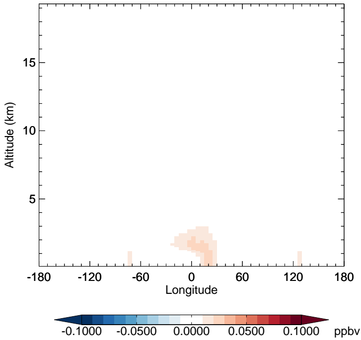
v11-02e-Run1 - v11-02d-Run1 SOAME - Diff along 15S for Jan
