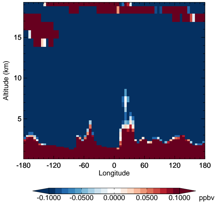
v11-02e-Run1 - v11-02d-Run1 N2O - Diff along 15S for Jan
