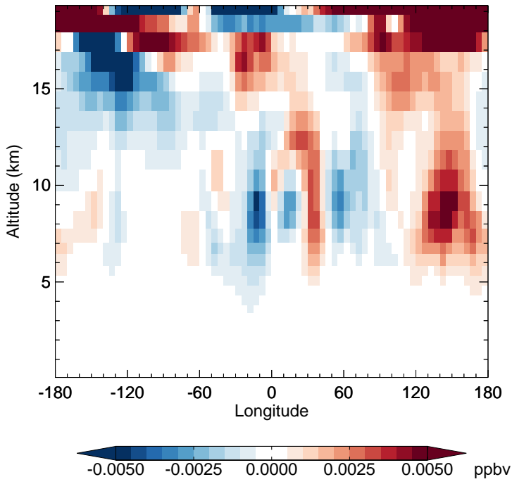
v11-02e-Run1 - v11-02e-Run0 N2O5 - Diff along 15S for Jan
