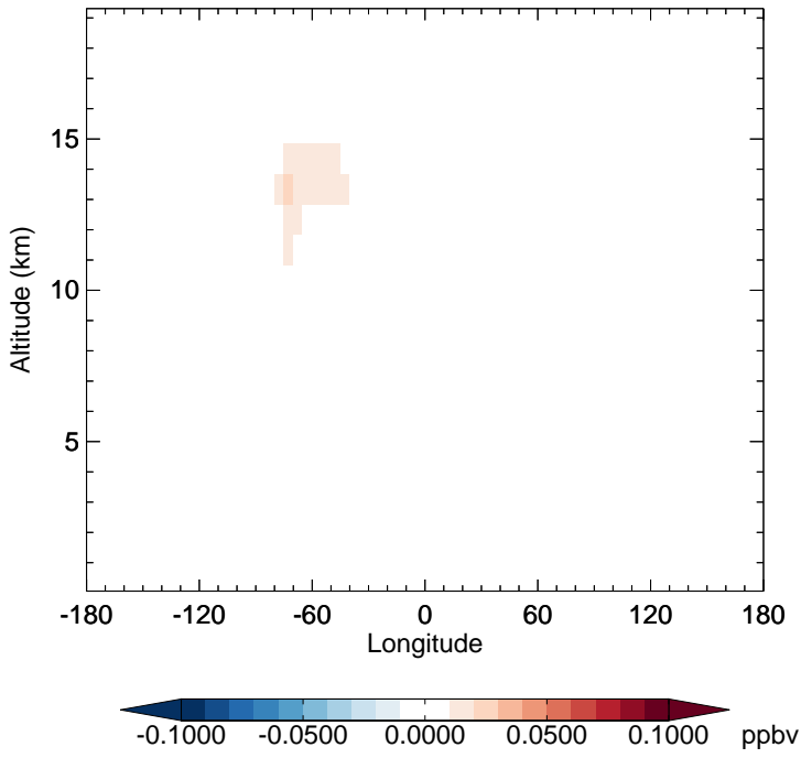
v11-02e-Run1 - v11-02e-Run0 ISOA3 - Diff along 15S for Jan
