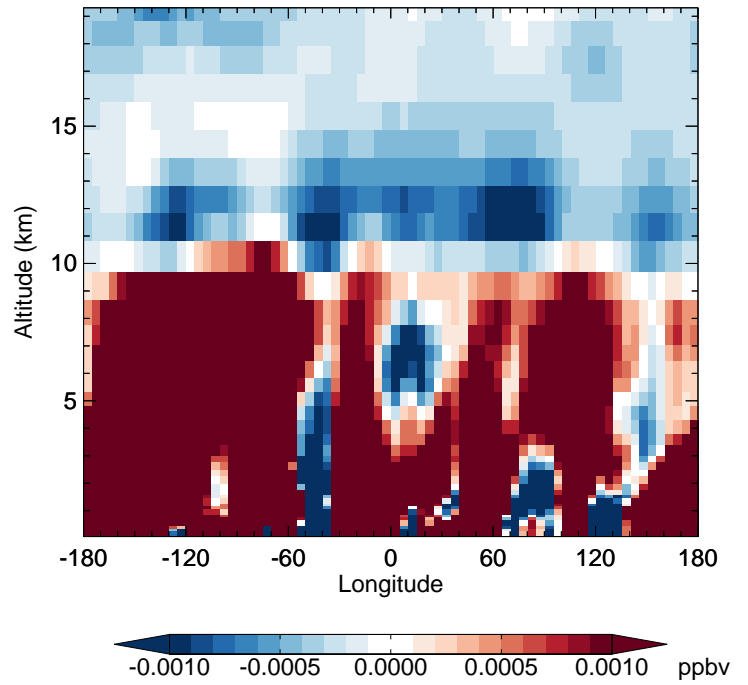
v11-02e-Run1 - v11-02d-Run1 PPN - Diff along 42N for Jan
