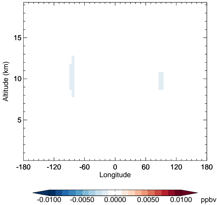
v11-02e-Run1 - v11-02d-Run1 HBr - Diff along 15S for Jan
