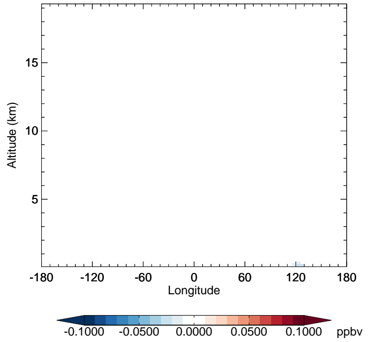
v11-02e-Run1 - v11-02e-Run0 GLYC - Diff along 42N for Jan
