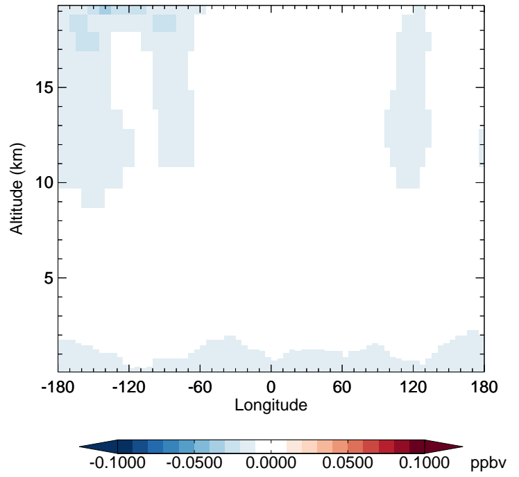
v11-02e-Run1 - v11-02e-Run0 CFC11 - Diff along 42N for Jan
