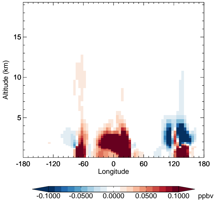
v11-02e-Run1 - v11-02e-Run0 SOAIE - Diff along 15S for Jan
