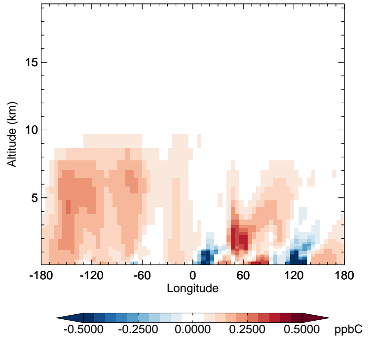
v11-02e-Run1 - v11-02d-Run1 C3H8 - Diff along 42N for Jan
