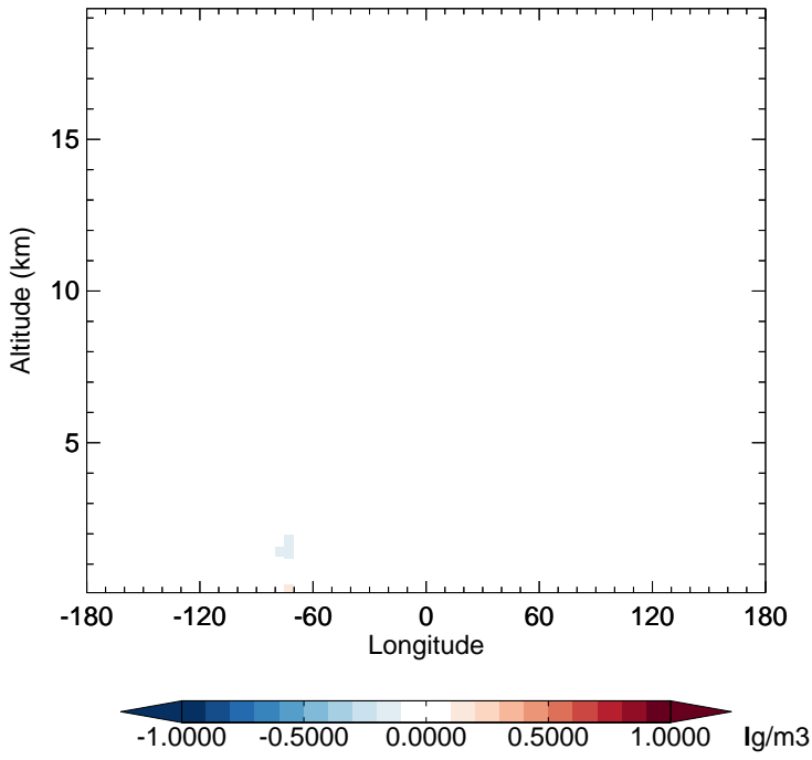
v11-02e-Run1 - v11-02e-Run0 NH4 - Diff along 15S for Jan
