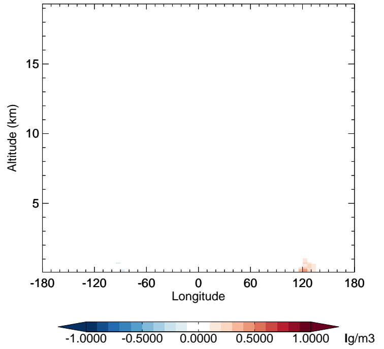
v11-02e-Run1 - v11-02e-Run0 NH3 - Diff along 42N for Jan
