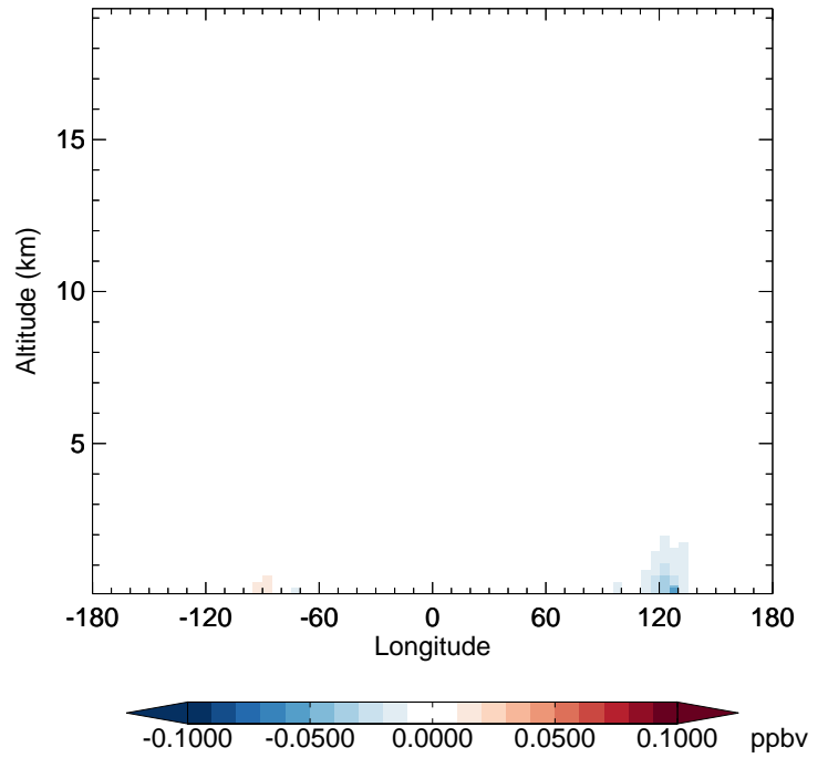
v11-02e-Run1 - v11-02d-Run1 INDIOL - Diff along 42N for Jan
