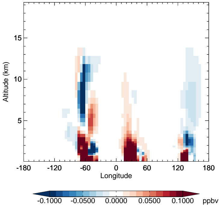
v11-02e-Run1 - v11-02e-Run0 EOH - Diff along 15S for Jan
