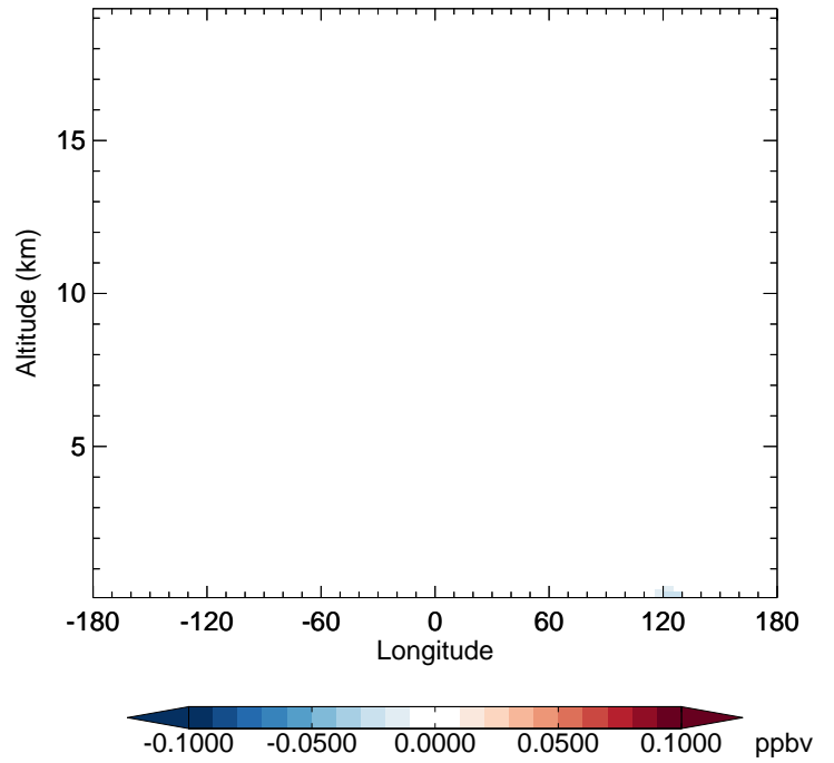
v11-02e-Run1 - v11-02d-Run1 GLYC - Diff along 42N for Jan
