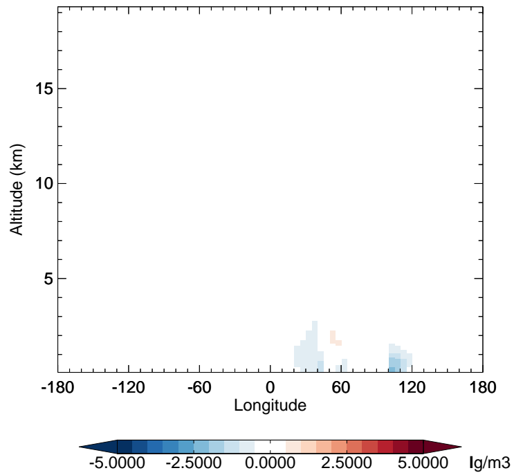
v11-02e-Run1 - v11-02d-Run1 DST2 - Diff along 42N for Jan
