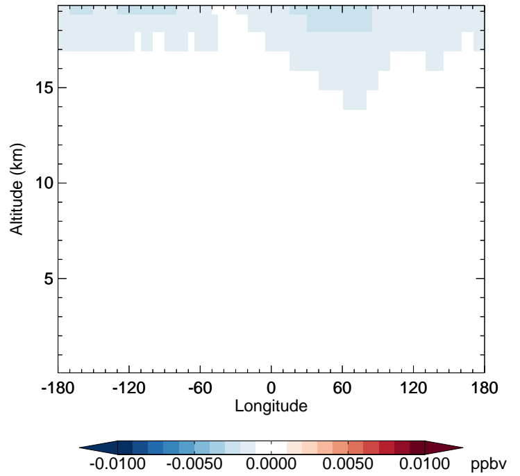
v11-02e-Run1 - v11-02d-Run1 HOBr - Diff along 42N for Jan
