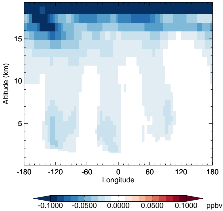
v11-02e-Run1 - v11-02d-Run1 HCl - Diff along 15S for Jan
