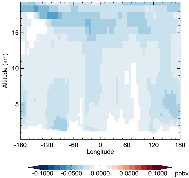
v11-02e-Run1 - v11-02d-Run1 CH3Cl - Diff along 15S for Jan
