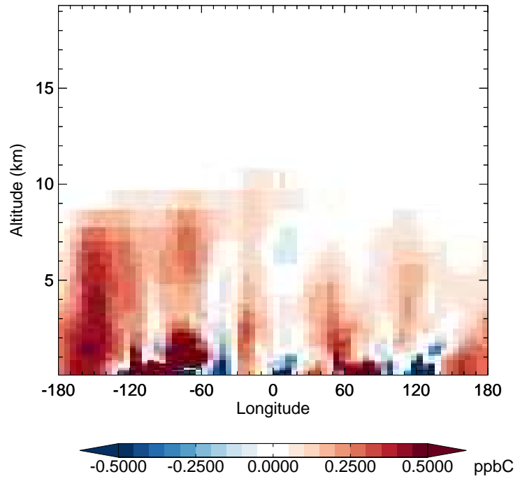
v11-02e-Run1 - v11-02e-Run0 ALK4 - Diff along 42N for Jan
