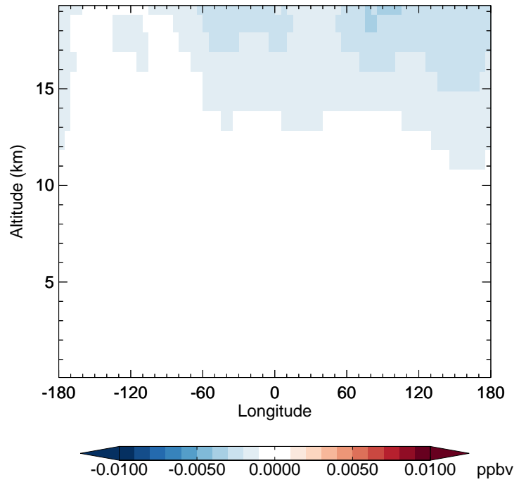
v11-02e-Run1 - v11-02d-Run1 BrNO3 - Diff along 42N for Jan
