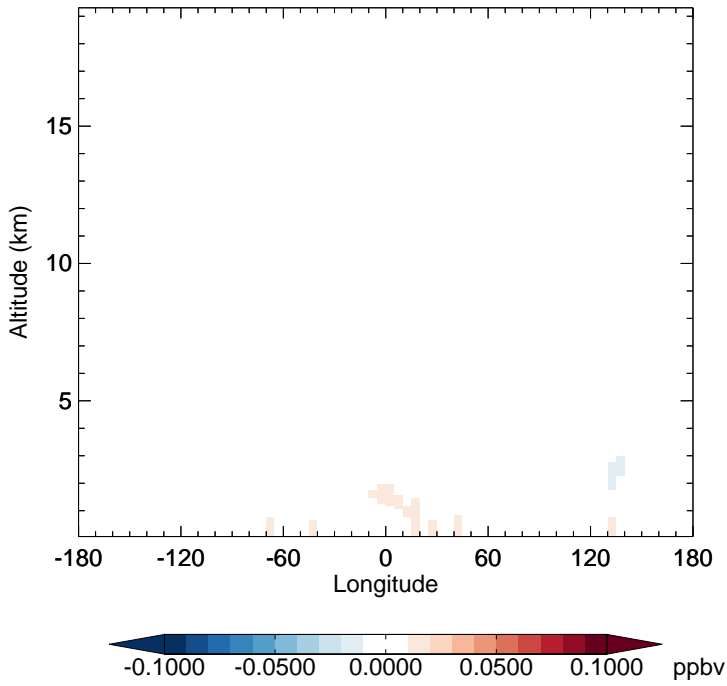
v11-02e-Run1 - v11-02e-Run0 SOAGX - Diff along 15S for Jan
