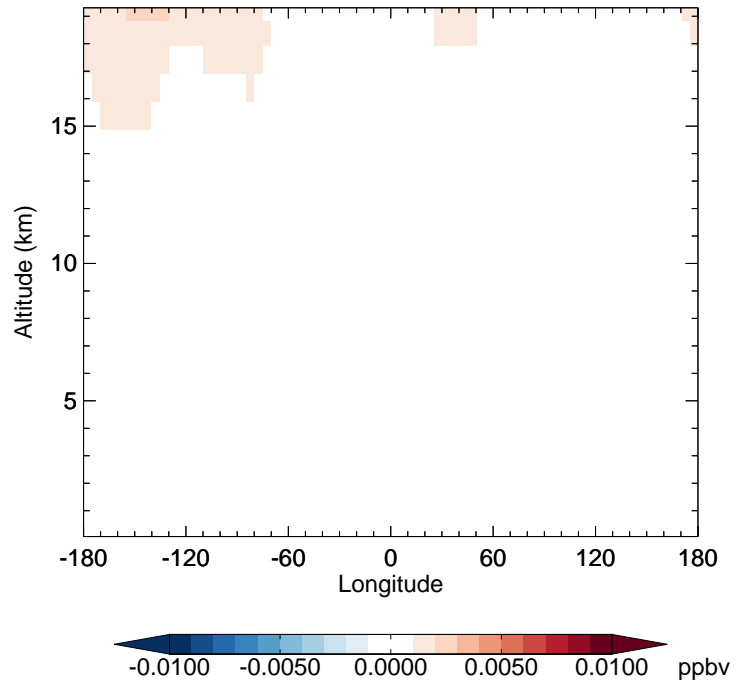
v11-02e-Run1 - v11-02e-Run0 BrNO3 - Diff along 42N for Jan
