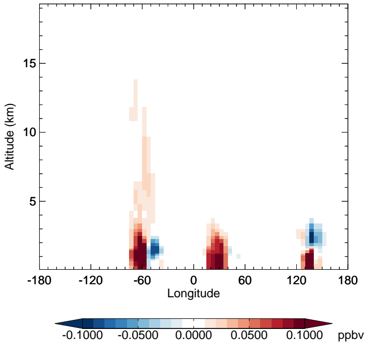
v11-02e-Run1 - v11-02d-Run1 GLYC - Diff along 15S for Jan
