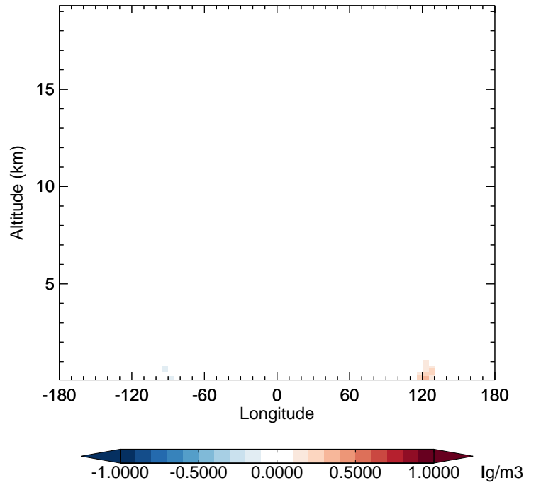
v11-02e-Run1 - v11-02d-Run1 NH3 - Diff along 42N for Jan
