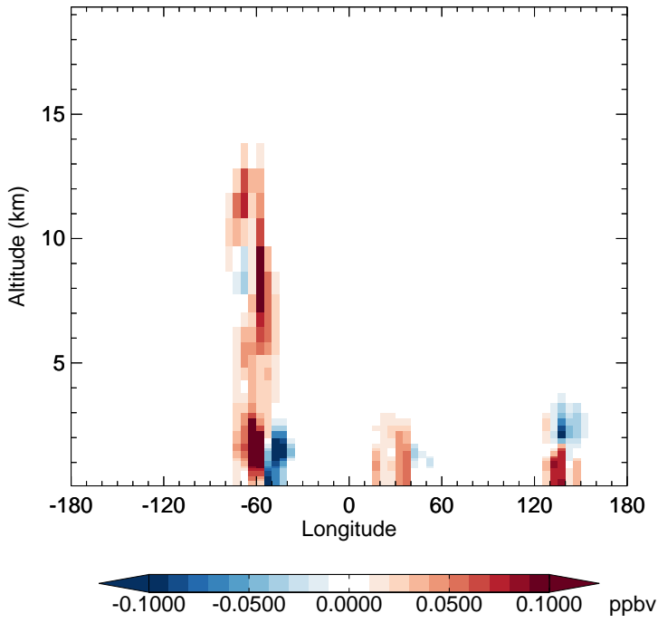
v11-02e-Run1 - v11-02e-Run0 IEPOXA - Diff along 15S for Jan
