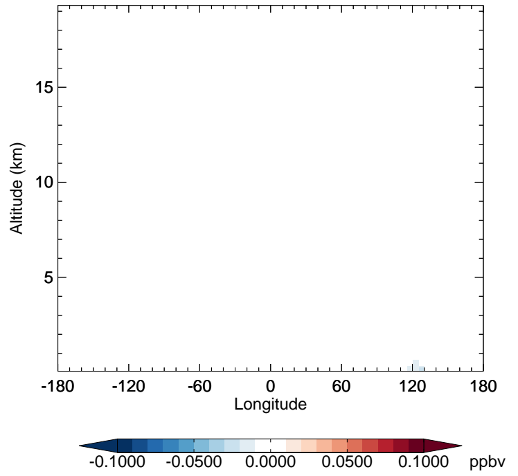
v11-02e-Run1 - v11-02e-Run0 ASOA2 - Diff along 42N for Jan
