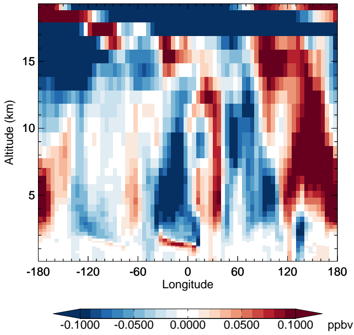
v11-02e-Run1 - v11-02e-Run0 HNO 3 - Diff along 15S for Jan
