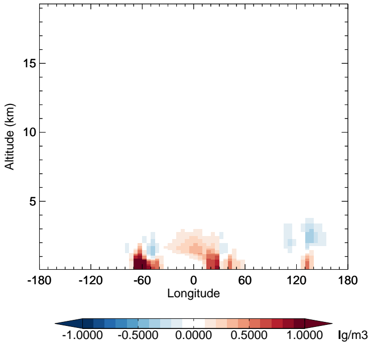
v11-02e-Run1 - v11-02d-Run1 SOAS - Diff along 15S for Jan
