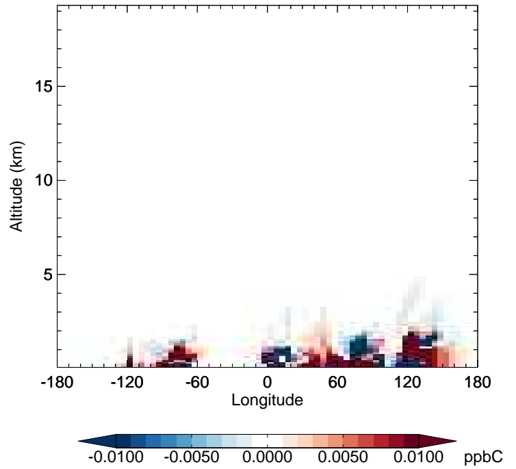
v11-02e-Run1 - v11-02d-Run1 PRPE - Diff along 42N for Jan
