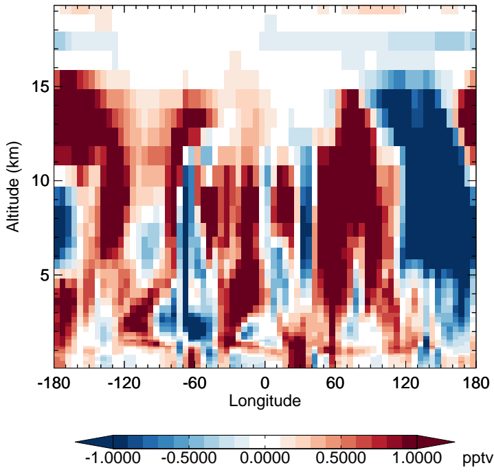
v11-02e-Run1 - v11-02e-Run0 HO2 - Diff along 15S for Jan
