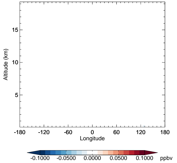
v11-02e-Run1 - v11-02e-Run0 ASOA1 - Diff along 42N for Jan
