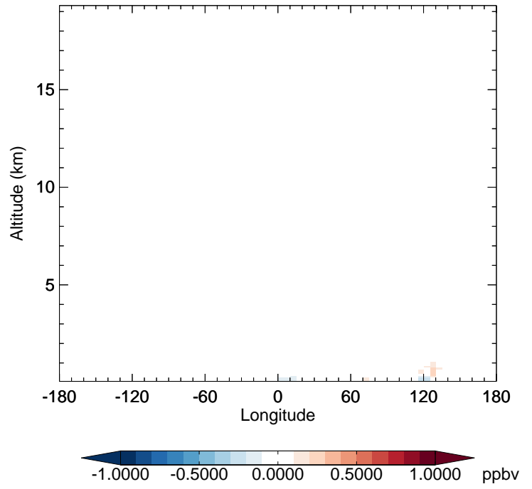
v11-02e-Run1 - v11-02e-Run0 NO - Diff along 42N for Jan
