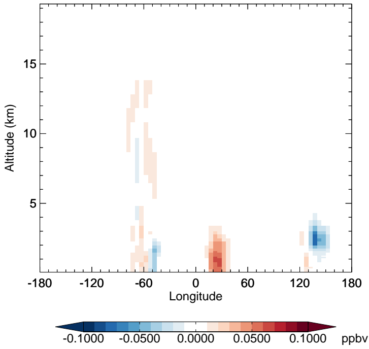
v11-02e-Run1 - v11-02e-Run0 IMAE - Diff along 15S for Jan
