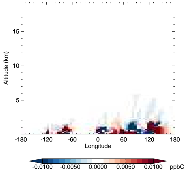
v11-02e-Run1 - v11-02e-Run0 PRPE - Diff along 42N for Jan
