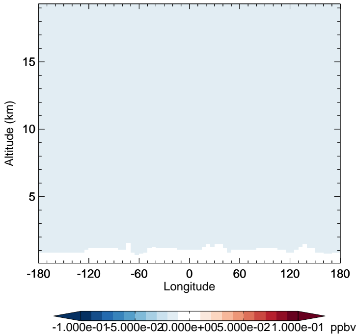
v11-02e-Run1 - v11-02d-Run1 HCFC22 - Diff along 15S for Jan
