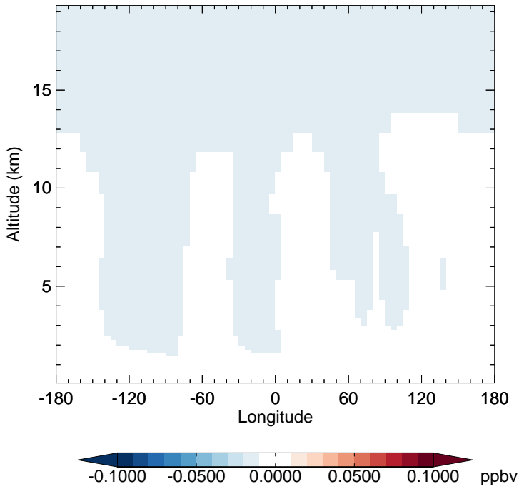
v11-02e-Run1 - v11-02d-Run1 HCFC141b - Diff along 15S for Jan
