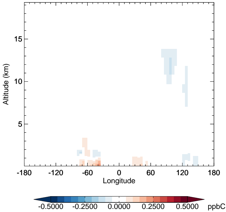
v11-02e-Run1 - v11-02d-Run1 ALK4 - Diff along 15S for Jan
