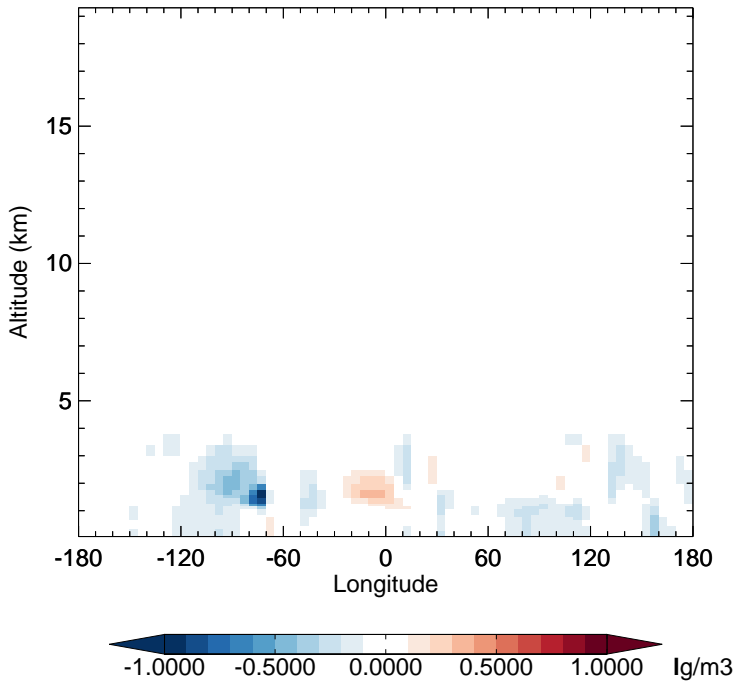
v11-02e-Run1 - v11-02e-Run0 SO4 - Diff along 15S for Jan
