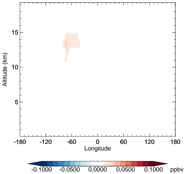
v11-02e-Run1 - v11-02d-Run1 ISOA3 - Diff along 15S for Jan
