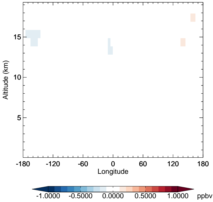
v11-02e-Run1 - v11-02e-Run0 NO - Diff along 15S for Jan
