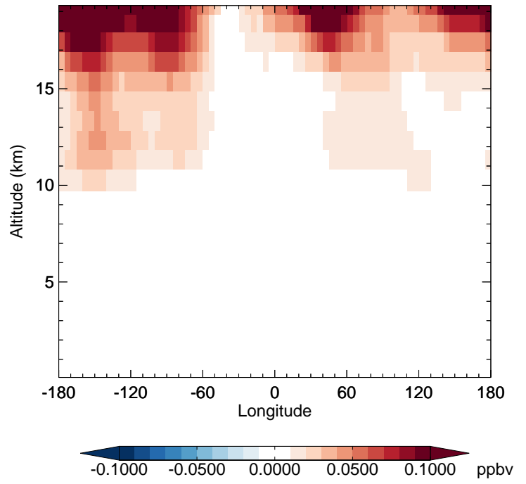
v11-02e-Run1 - v11-02e-Run0 HCl - Diff along 42N for Jan
