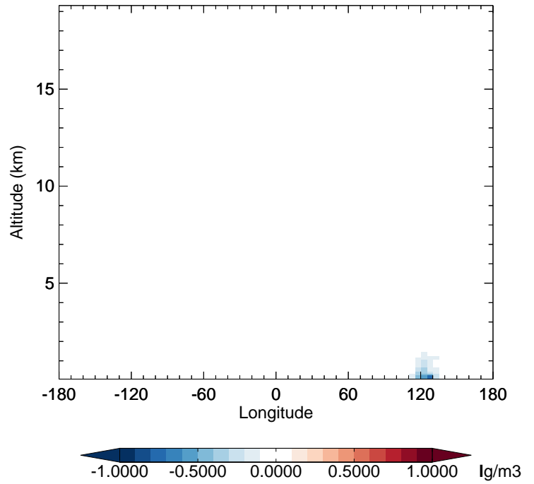
v11-02e-Run1 - v11-02d-Run1 BCPI - Diff along 42N for Jan
