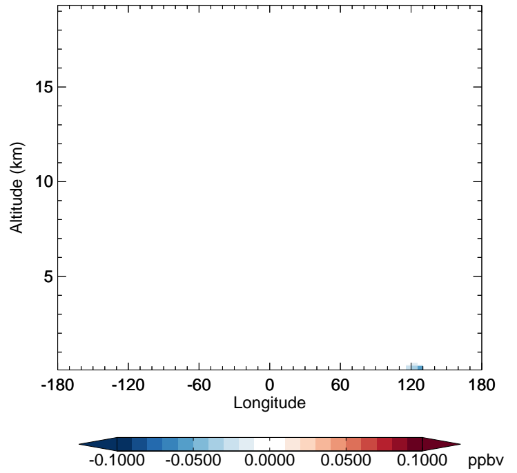
v11-02e-Run1 - v11-02e-Run0 MGLY - Diff along 42N for Jan
