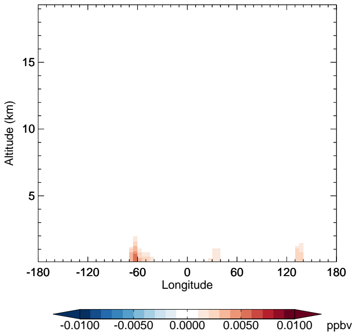
v11-02e-Run1 - v11-02d-Run1 MOBA - Diff along 15S for Jan
