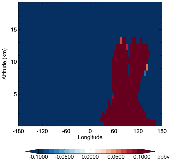
v11-02e-Run1 - v11-02d-Run1 CH4 - Diff along 15S for Jan
