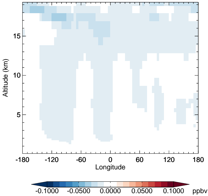
v11-02e-Run1 - v11-02d-Run1 OCS - Diff along 15S for Jan
