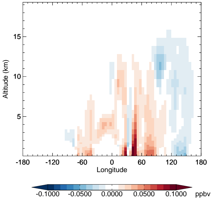
v11-02e-Run1 - v11-02e-Run0 BENZ - Diff along 15S for Jan
