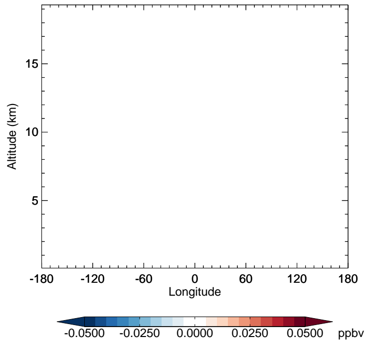
v11-02e-Run1 - v11-02d-Run1 MACR - Diff along 42N for Jan
