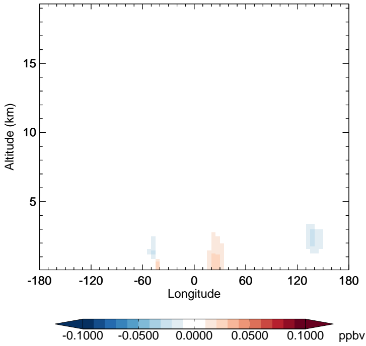
v11-02e-Run1 - v11-02e-Run0 IONITA - Diff along 15S for Jan
