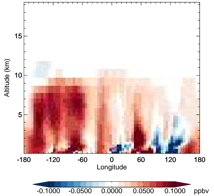
v11-02e-Run1 - v11-02d-Run1 BENZ - Diff along 42N for Jan
