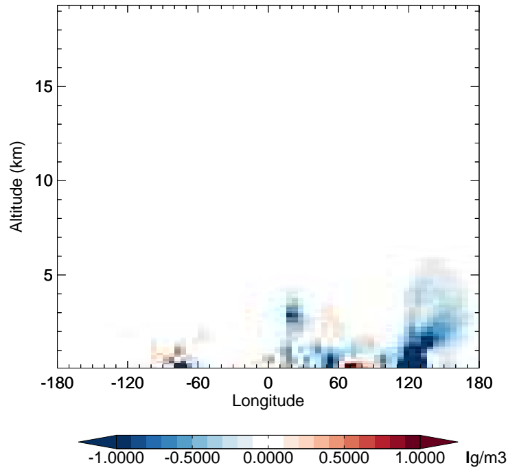
v11-02e-Run1 - v11-02e-Run0 SO 2 - Diff along 42N for Jan
