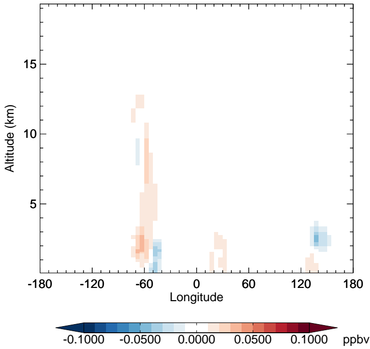
v11-02e-Run1 - v11-02e-Run0 HC187 - Diff along 15S for Jan
