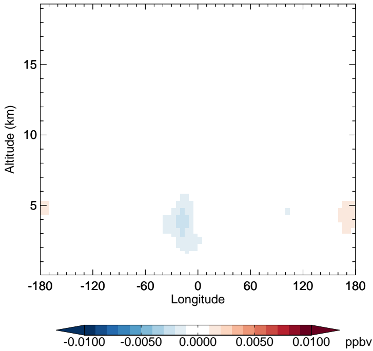
v11-02e-Run1 - v11-02d-Run1 NO3 - Diff along 15S for Jan
