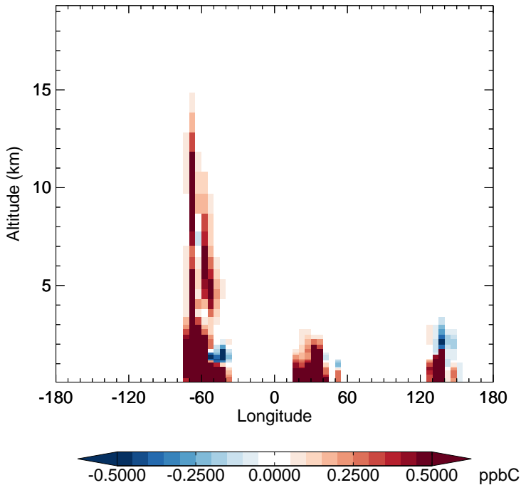
v11-02e-Run1 - v11-02e-Run0 ISOP - Diff along 15S for Jan
