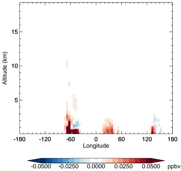
v11-02e-Run1 - v11-02e-Run0 RCHO - Diff along 15S for Jan
