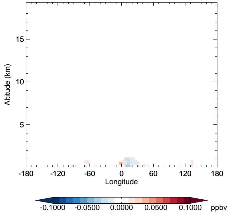
v11-02e-Run1 - v11-02e-Run0 CINO2 - Diff along 42N for Jan
