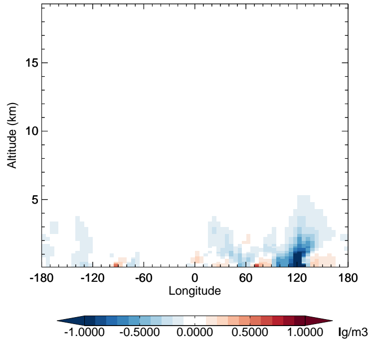
v11-02e-Run1 - v11-02d-Run1 SO4 - Diff along 42N for Jan
