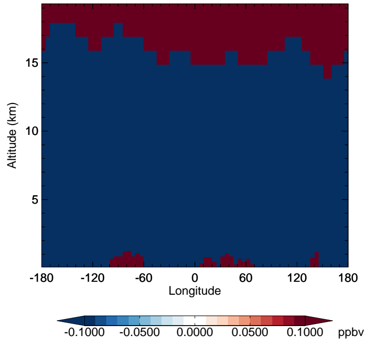
v11-02e-Run1 - v11-02d-Run1 CH4 - Diff along 42N for Jan
