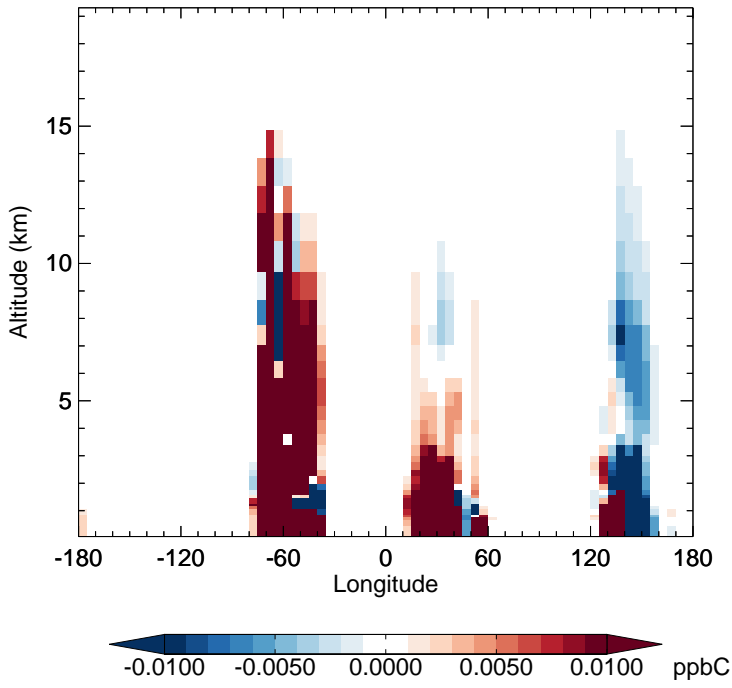
v11-02e-Run1 - v11-02e-Run0 PRPE - Diff along 15S for Jan
