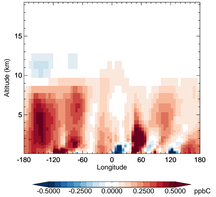
v11-02e-Run1 - v11-02e-Run0 C2H6 - Diff along 42N for Jan
