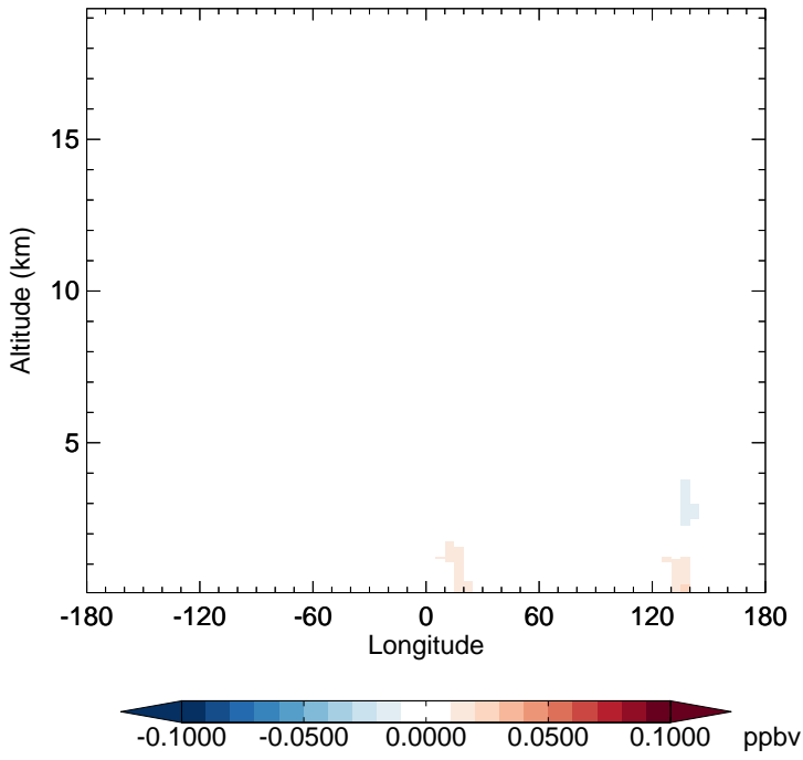
v11-02e-Run1 - v11-02e-Run0 ISOG1 - Diff along 15S for Jan
