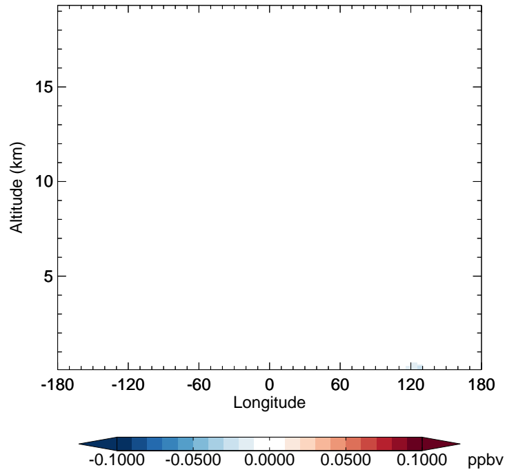
v11-02e-Run1 - v11-02d-Run1 ASOA2 - Diff along 42N for Jan
