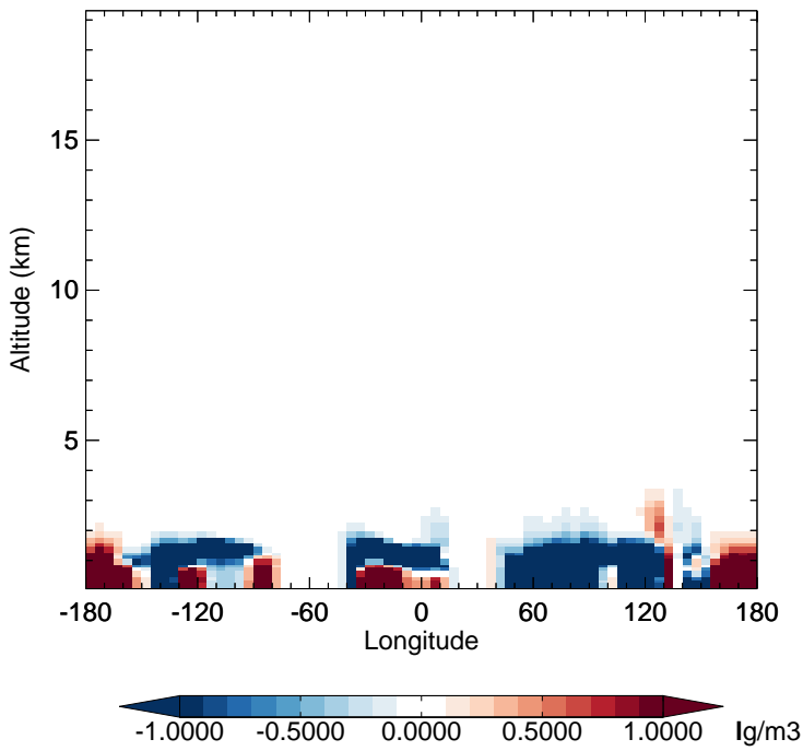
v11-02e-Run1 - v11-02d-Run1 SALC - Diff along 15S for Jan
