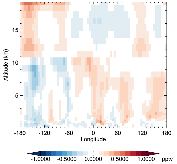
v11-02e-Run1 - v11-02e-Run0 HO2 - Diff along 42N for Jan
