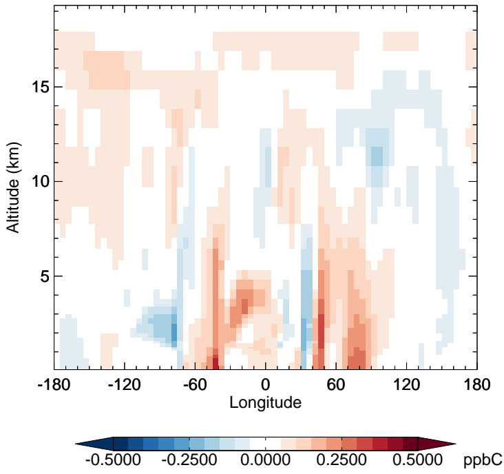
v11-02e-Run1 - v11-02e-Run0 C2H6 - Diff along 15S for Jan
