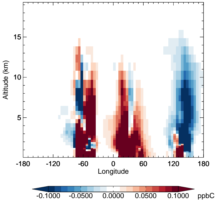
v11-02e-Run1 - v11-02d-Run1 MEK - Diff along 15S for Jan
