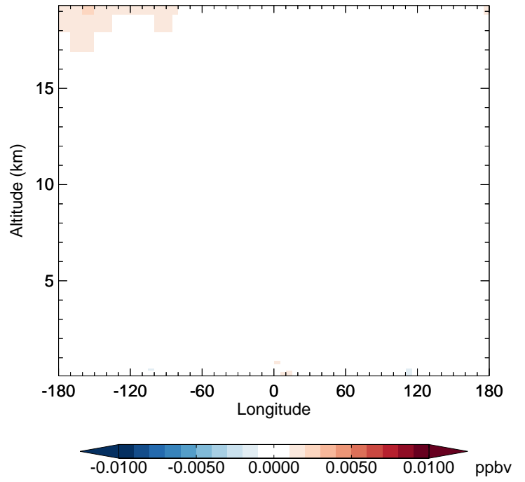
v11-02e-Run1 - v11-02e-Run0 NO3 - Diff along 42N for Jan
