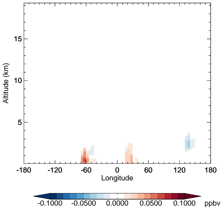
v11-02e-Run1 - v11-02d-Run1 ISOA1 - Diff along 15S for Jan
