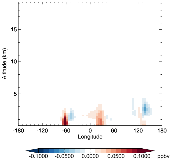
v11-02e-Run1 - v11-02e-Run0 TSOG2 - Diff along 15S for Jan
