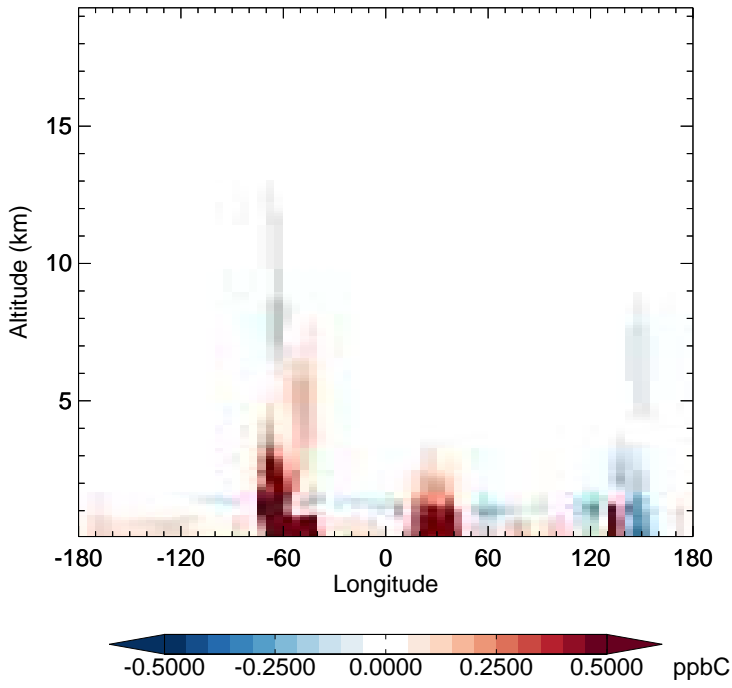
v11-02e-Run1 - v11-02e-Run0 ALD2 - Diff along 15S for Jan
