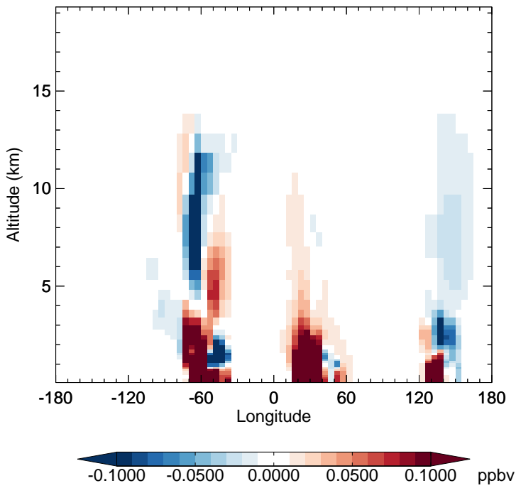
v11-02e-Run1 - v11-02d-Run1 EOH - Diff along 15S for Jan
