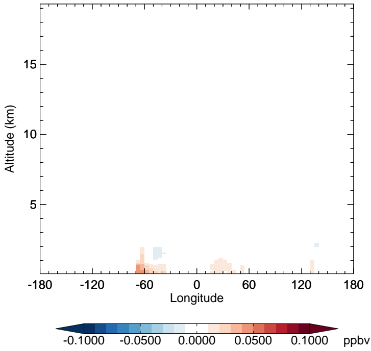
v11-02e-Run1 - v11-02e-Run0 SOAP - Diff along 15S for Jan
