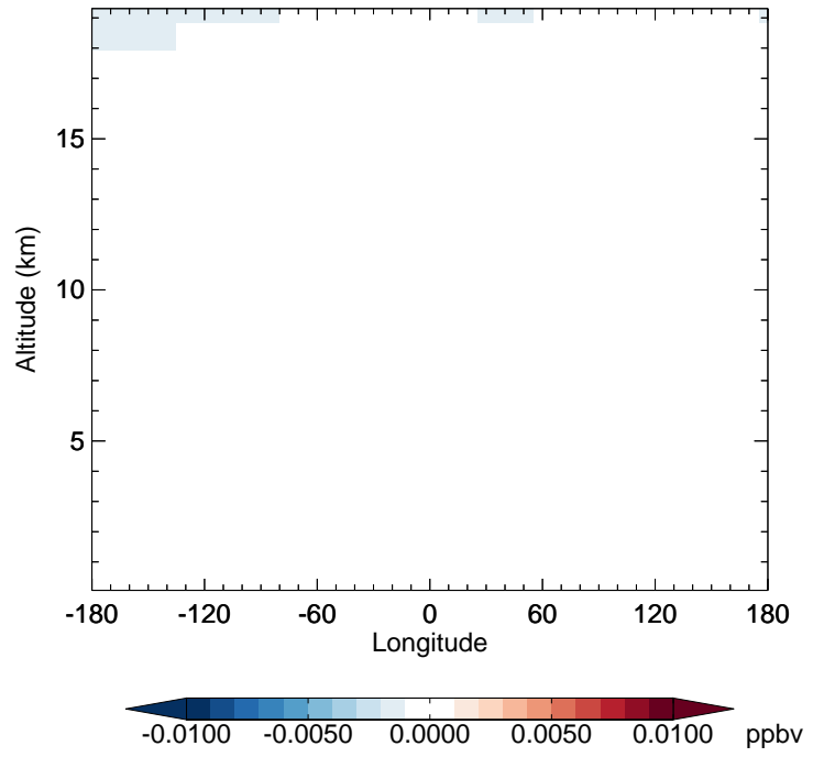
v11-02e-Run1 - v11-02e-Run0 HOBr - Diff along 42N for Jan
