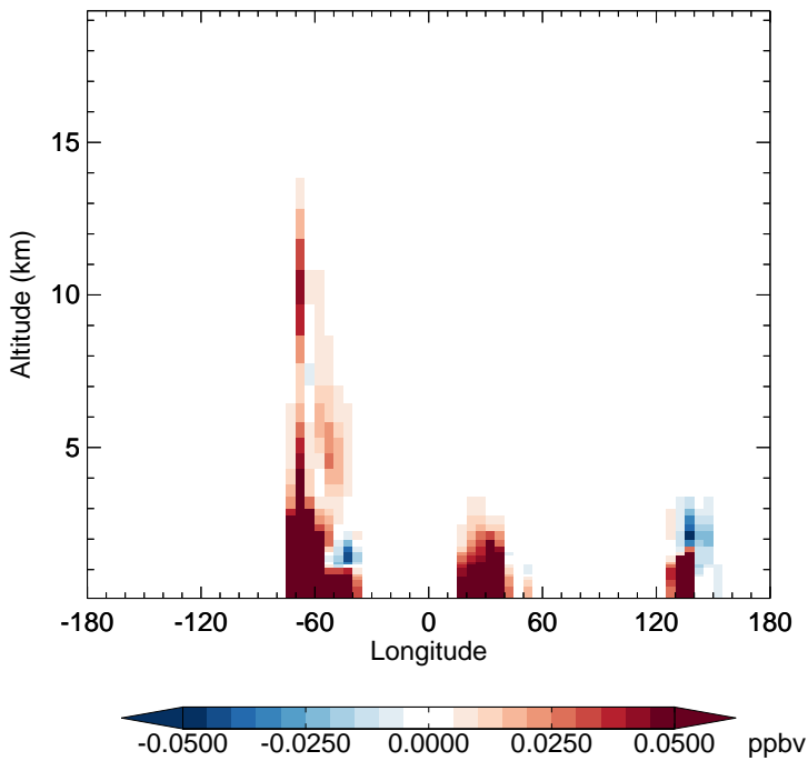
v11-02e-Run1 - v11-02d-Run1 MACR - Diff along 15S for Jan
