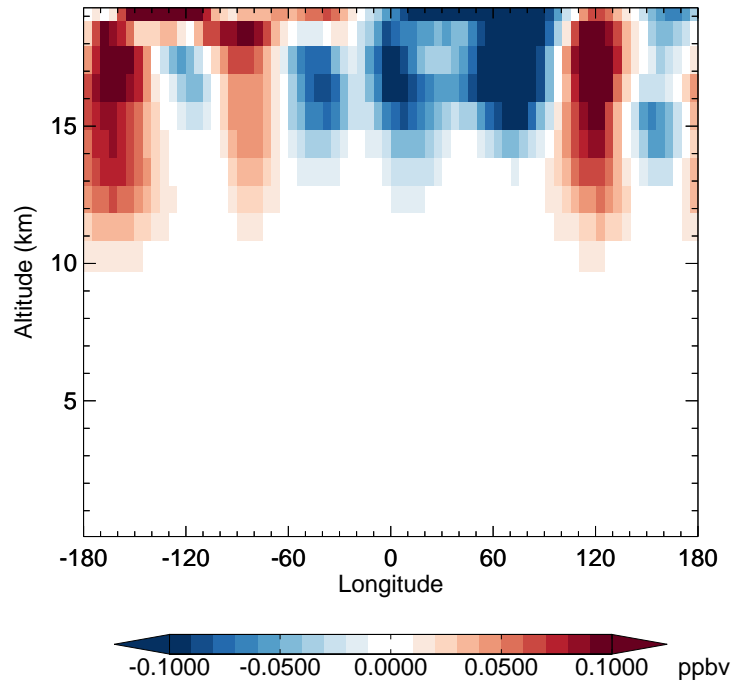
v11-02e-Run1 - v11-02e-Run0 CINO3 - Diff along 42N for Jan
