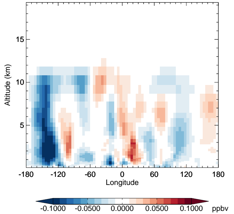
v11-02e-Run1 - v11-02d-Run1 H2O2 - Diff along 42N for Jan
