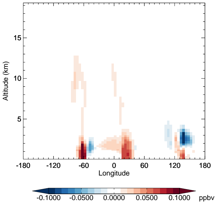
v11-02e-Run1 - v11-02d-Run1 ISO3 - Diff along 15S for Jan
