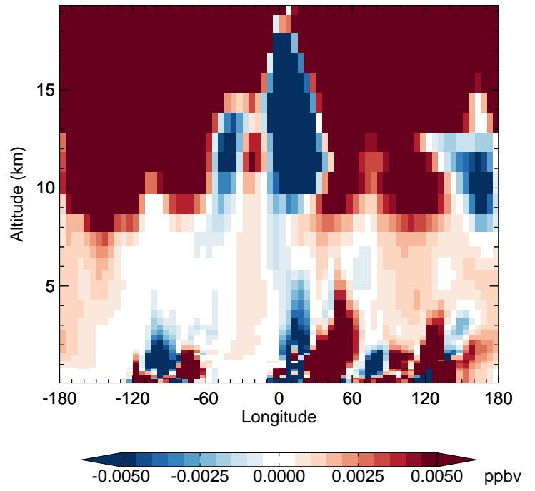
v11-02e-Run1 - v11-02e-Run0 N2O5 - Diff along 42N for Jan
