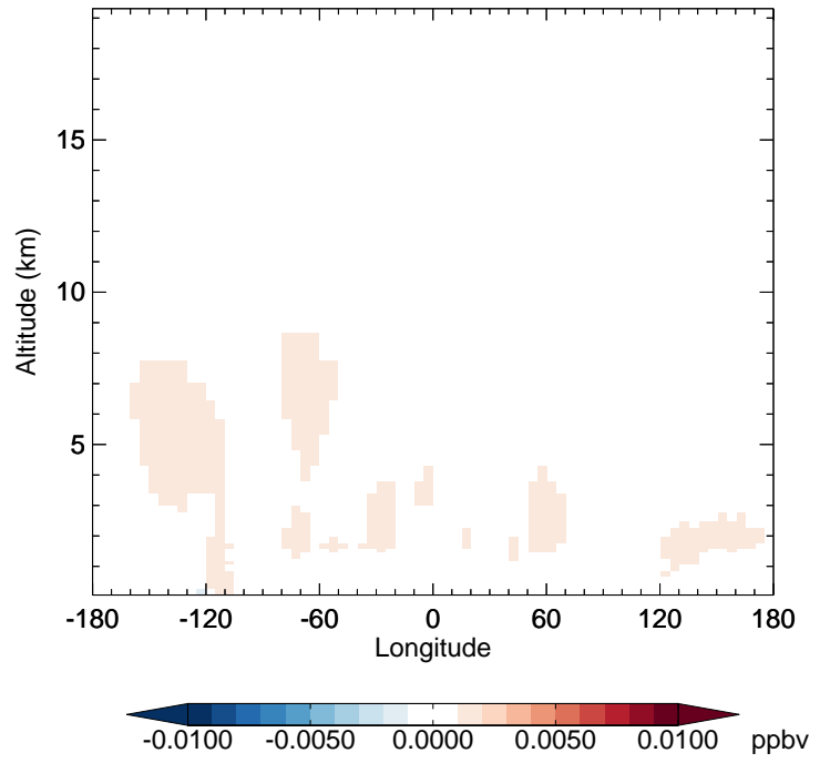
v11-02e-Run1 - v11-02e-Run0 R4N2 - Diff along 42N for Jan
