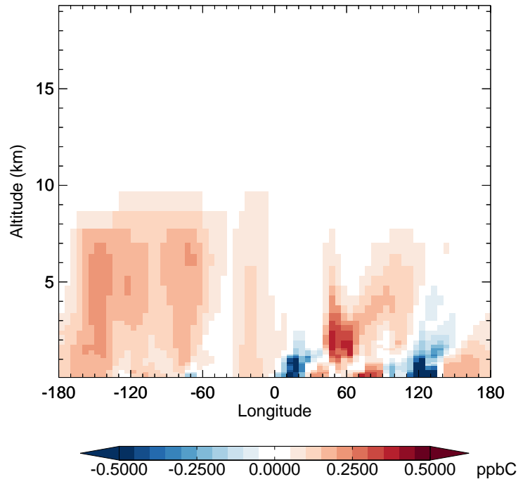
v11-02e-Run1 - v11-02e-Run0 C3H8 - Diff along 42N for Jan
