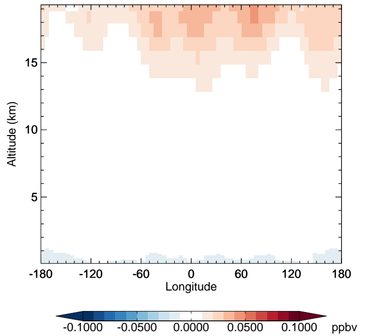
v11-02e-Run1 - v11-02d-Run1 CFC11 - Diff along 42N for Jan
