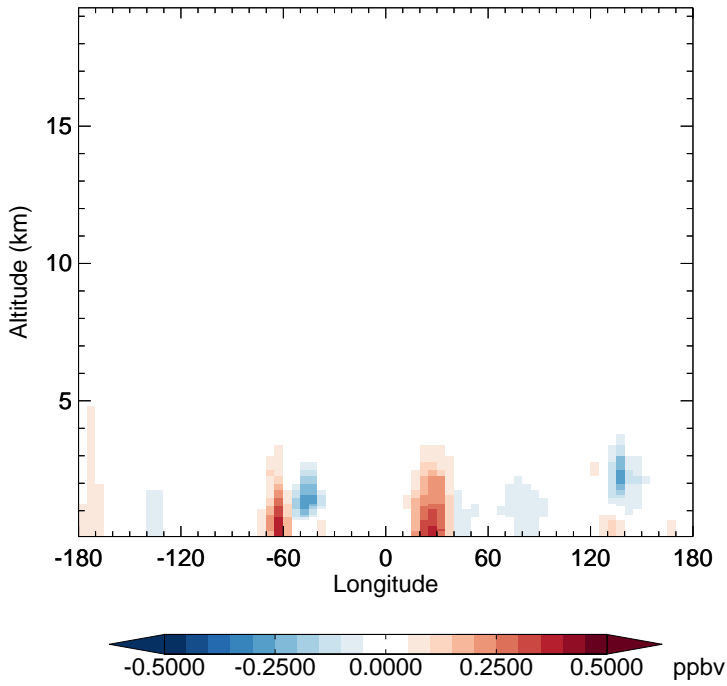
v11-02e-Run1 - v11-02e-Run0 CH 2 O - Diff along 15S for Jan
