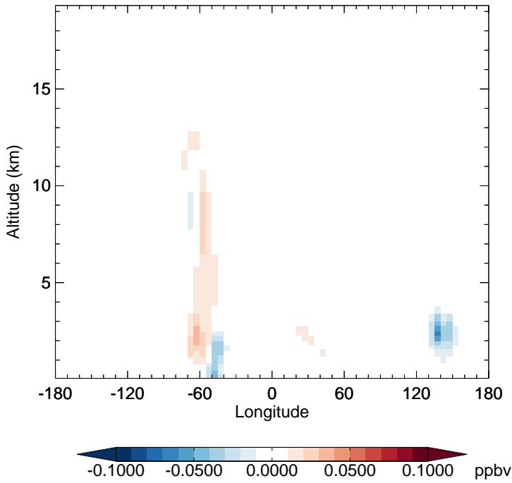
v11-02e-Run1 - v11-02d-Run1 HC187 - Diff along 15S for Jan
