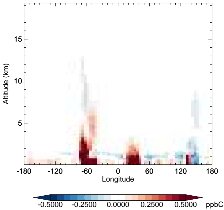
v11-02e-Run1 - v11-02d-Run1 ALD2 - Diff along 15S for Jan
