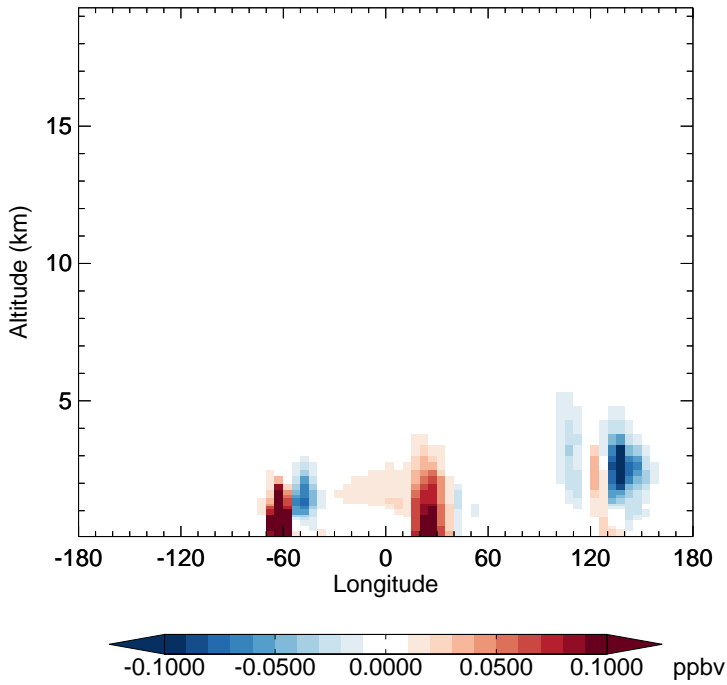
v11-02e-Run1 - v11-02d-Run1 TSOG3 - Diff along 15S for Jan
