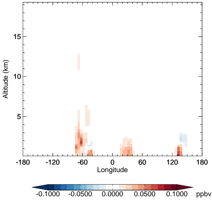
v11-02e-Run1 - v11-02e-Run0 IPMN - Diff along 15S for Jan
