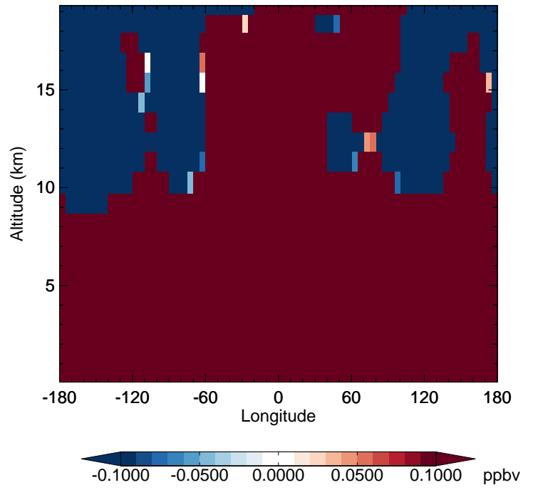
v11-02e-Run1 - v11-02e-Run0 N2O - Diff along 42N for Jan
