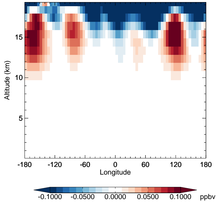
v11-02e-Run1 - v11-02d-Run1 CINO3 - Diff along 42N for Jan
