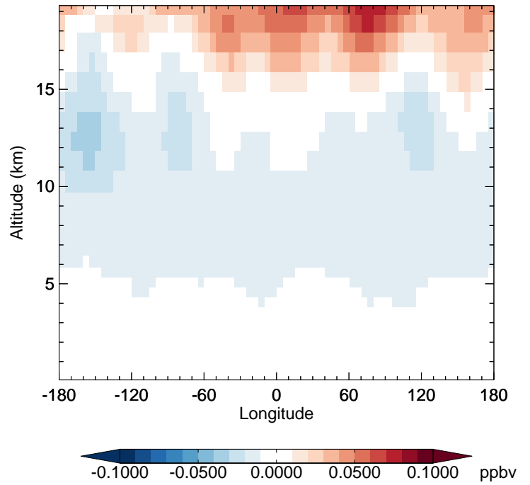
v11-02e-Run1 - v11-02d-Run1 OCS - Diff along 42N for Jan
