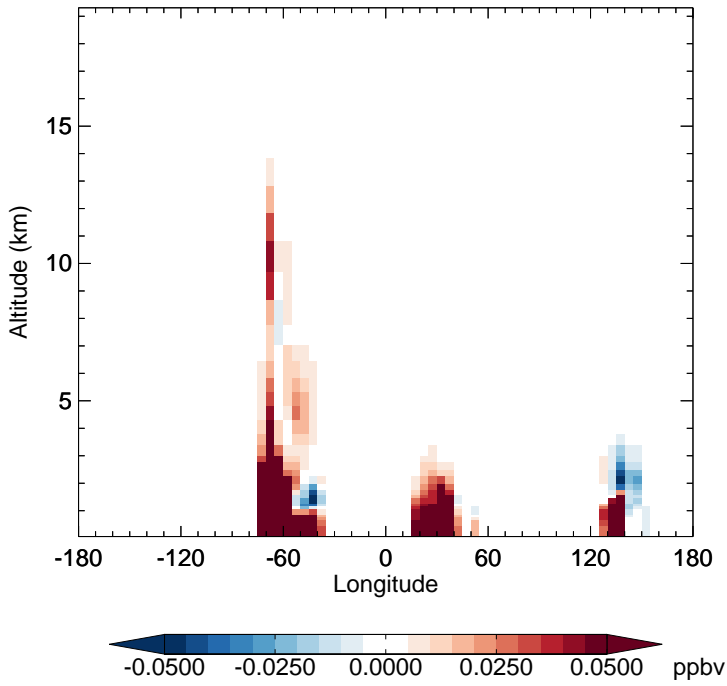
v11-02e-Run1 - v11-02e-Run0 MACR - Diff along 15S for Jan
