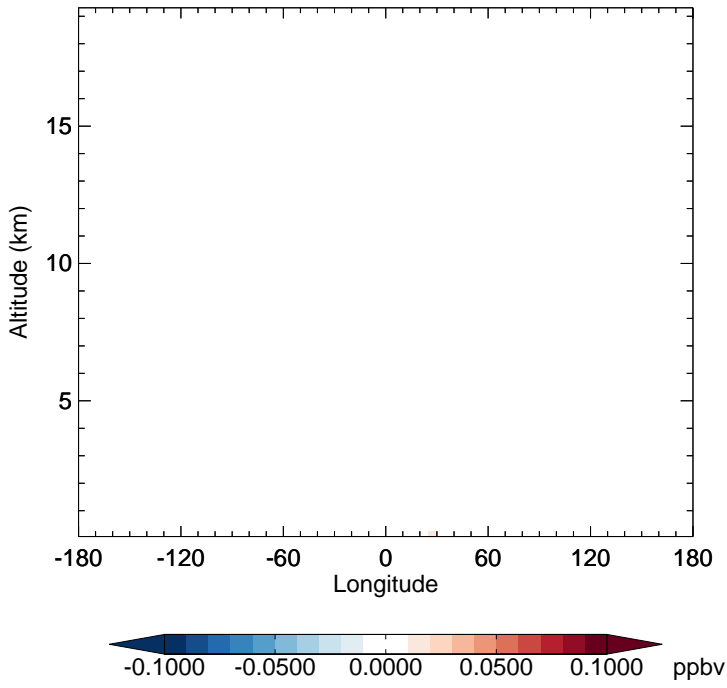
v11-02e-Run1 - v11-02e-Run0 MONITA - Diff along 15S for Jan
