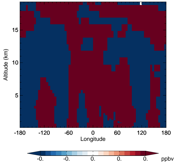
v11-02e-Run1 - v11-02d-Run1 H2O - Diff along 42N for Jan
