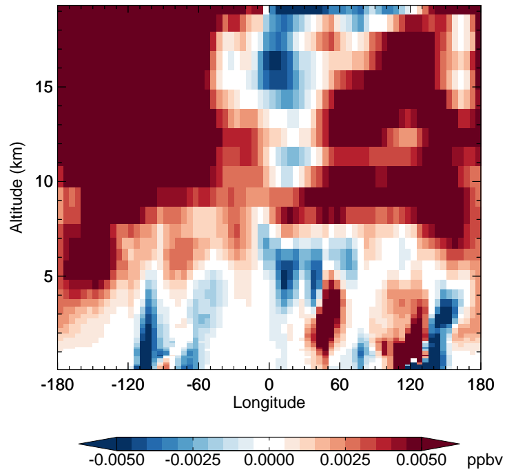
v11-02e-Run1 - v11-02d-Run1 HNO 4 - Diff along 42N for Jan
