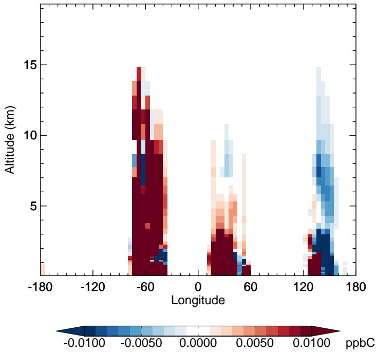
v11-02e-Run1 - v11-02d-Run1 PRPE - Diff along 15S for Jan
