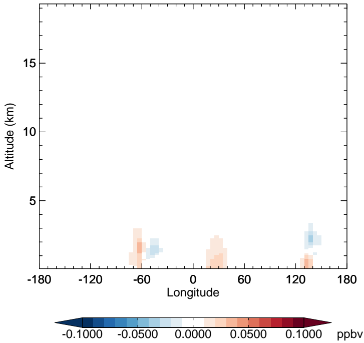
v11-02e-Run1 - v11-02d-Run1 MGLY - Diff along 15S for Jan
