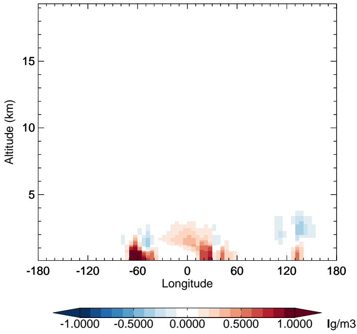
v11-02e-Run1 - v11-02e-Run0 SOAS - Diff along 15S for Jan
