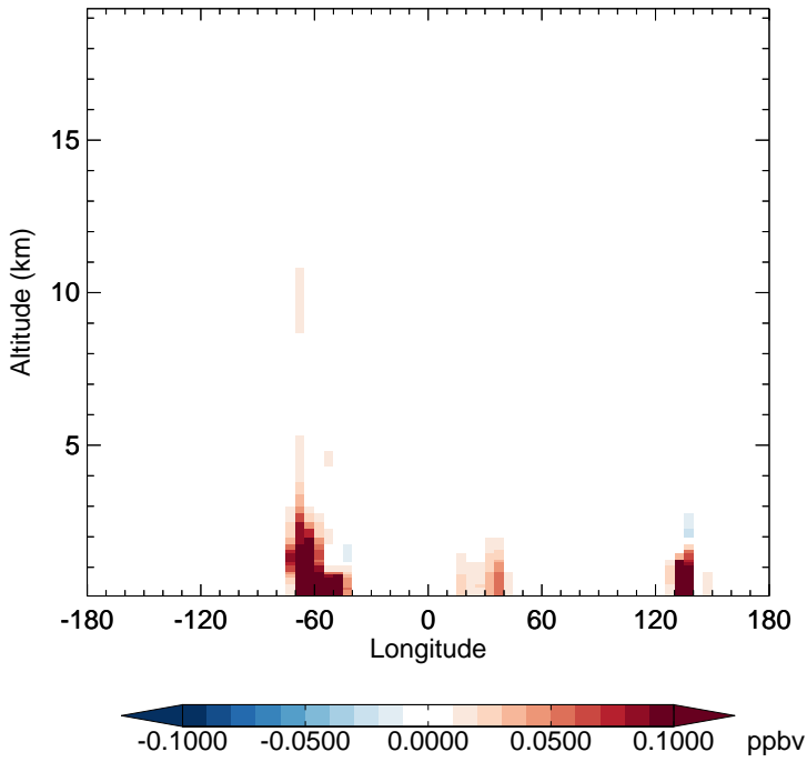
v11-02e-Run1 - v11-02e-Run0 HPALD - Diff along 15S for Jan
