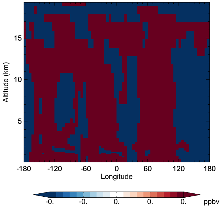
v11-02e-Run1 - v11-02d-Run1 H2O - Diff along 15S for Jan
