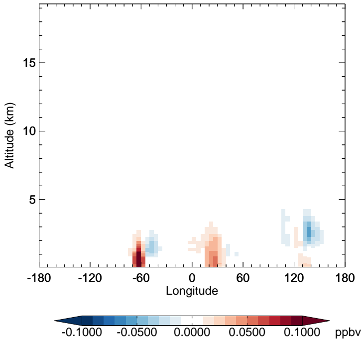
v11-02e-Run1 - v11-02d-Run1 TSOG2 - Diff along 15S for Jan
