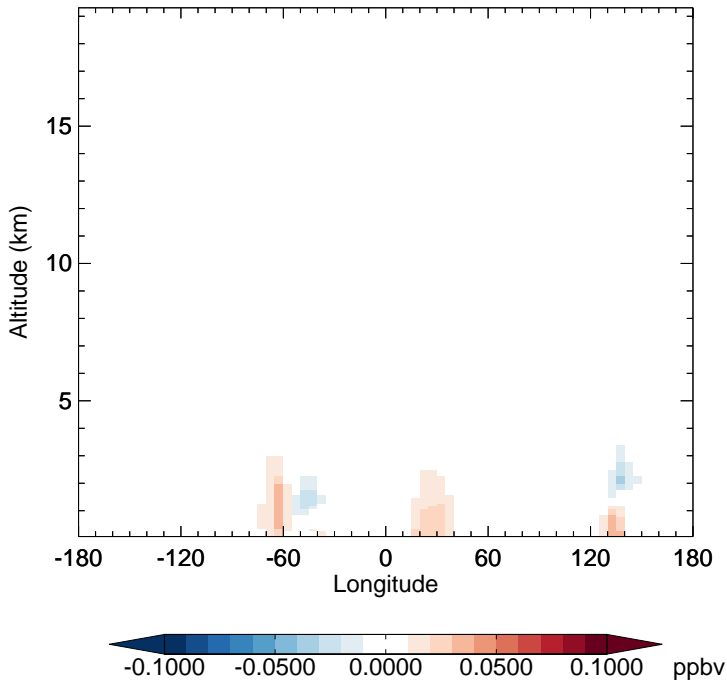
v11-02e-Run1 - v11-02e-Run0 MGLY - Diff along 15S for Jan
