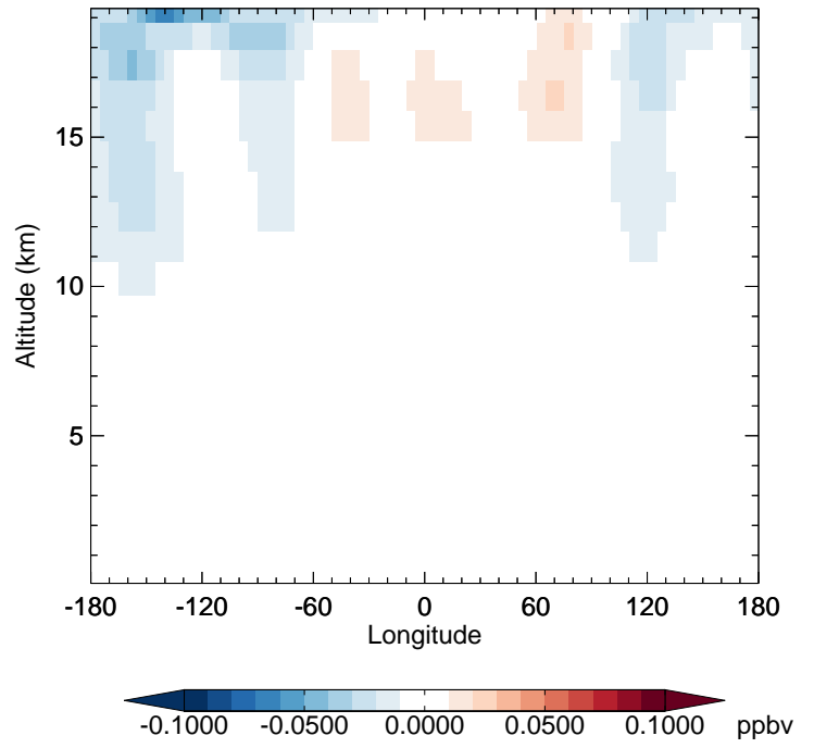
v11-02e-Run1 - v11-02e-Run0 OCS - Diff along 42N for Jan
