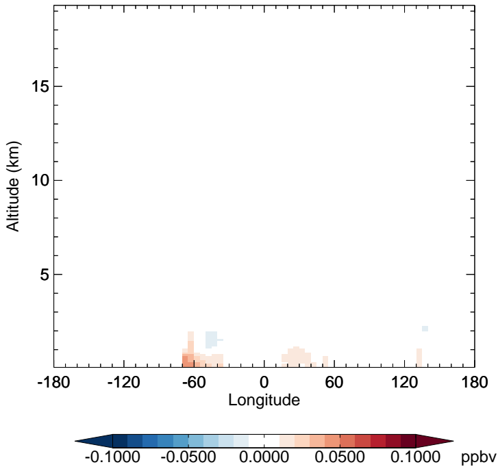
v11-02e-Run1 - v11-02d-Run1 SOAP - Diff along 15S for Jan
