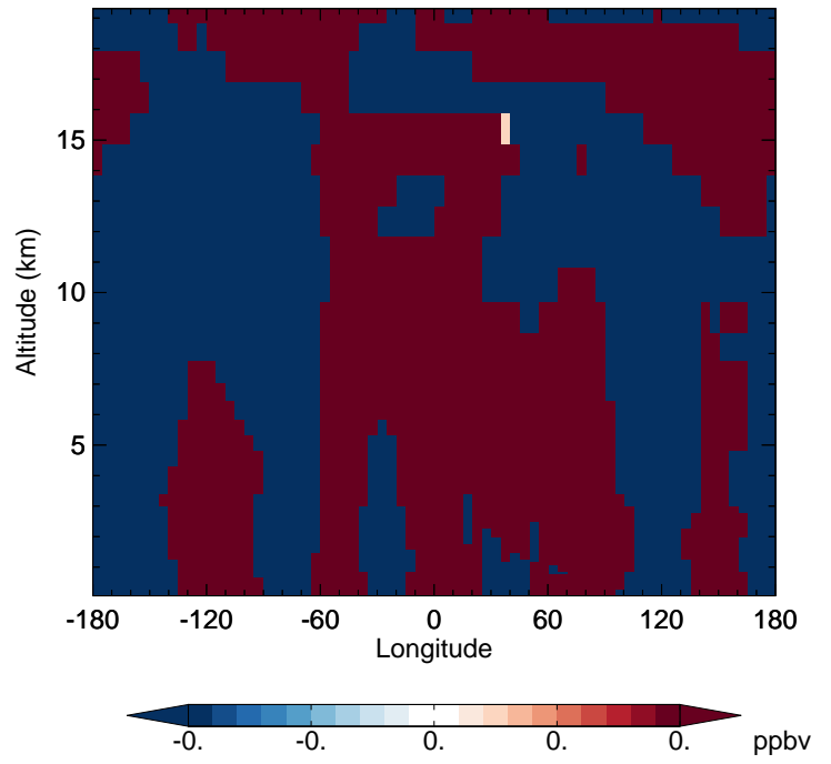
v11-02e-Run1 - v11-02e-Run0 H2O - Diff along 42N for Jan
