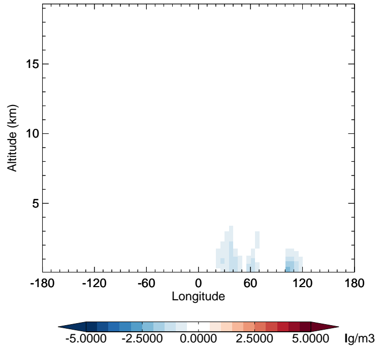
v11-02e-Run1 - v11-02e-Run0 DST2 - Diff along 42N for Jan
