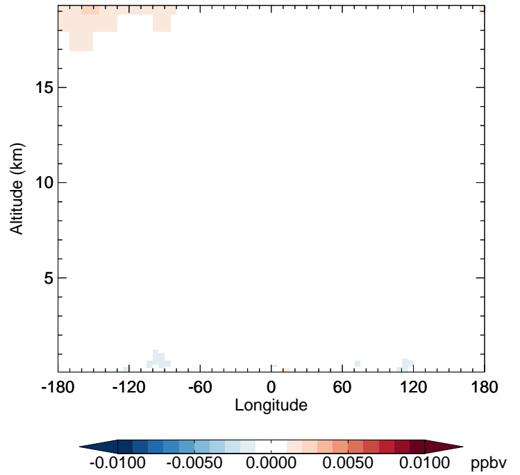
v11-02e-Run1 - v11-02d-Run1 NO3 - Diff along 42N for Jan
