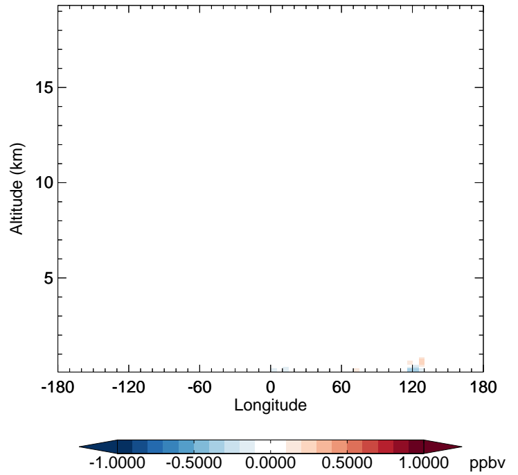
v11-02e-Run1 - v11-02d-Run1 NO - Diff along 42N for Jan
