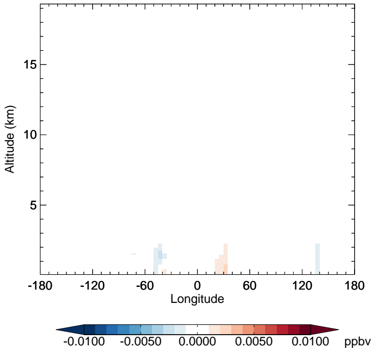
v11-02e-Run1 - v11-02e-Run0 MVKN - Diff along 15S for Jan
