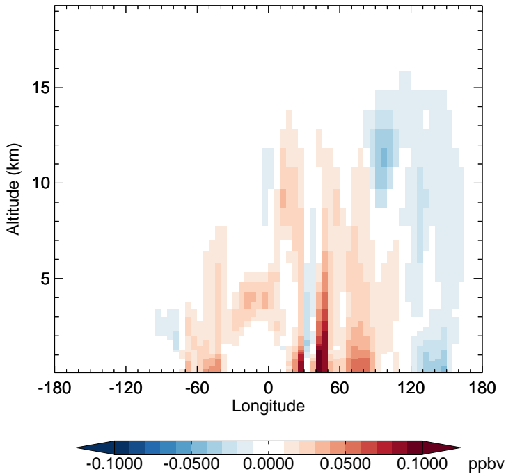
v11-02e-Run1 - v11-02d-Run1 BENZ - Diff along 15S for Jan
