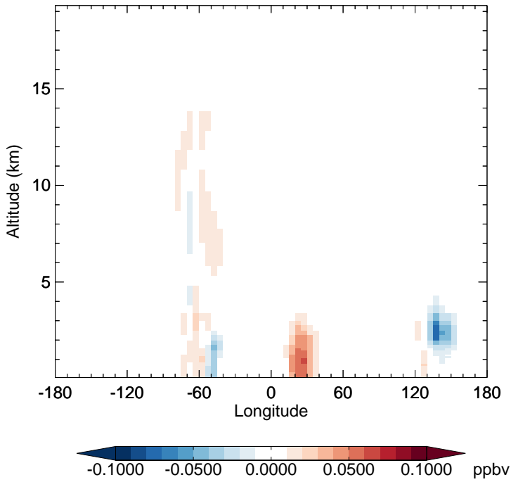
v11-02e-Run1 - v11-02d-Run1 IMAE - Diff along 15S for Jan
