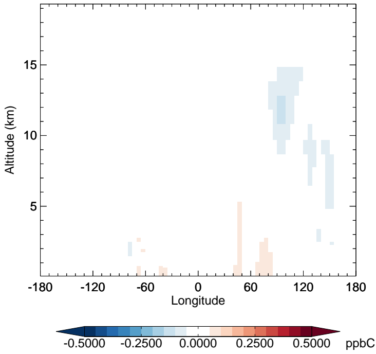
v11-02e-Run1 - v11-02e-Run0 C3H8 - Diff along 15S for Jan
