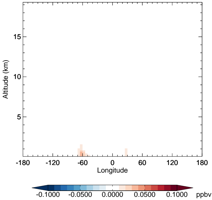
v11-02e-Run1 - v11-02e-Run0 TSOA1 - Diff along 15S for Jan
