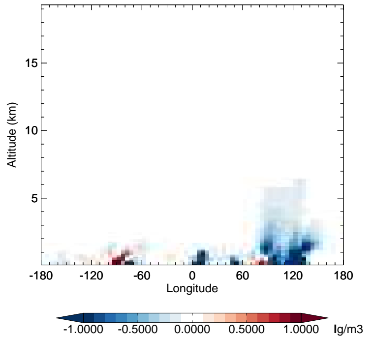
v11-02e-Run1 - v11-02d-Run1 NIT - Diff along 42N for Jan
