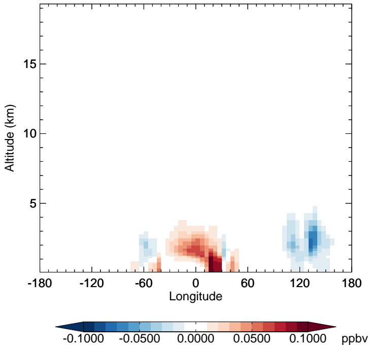
v11-02e-Run1 - v11-02e-Run0 INDIOL - Diff along 15S for Jan
