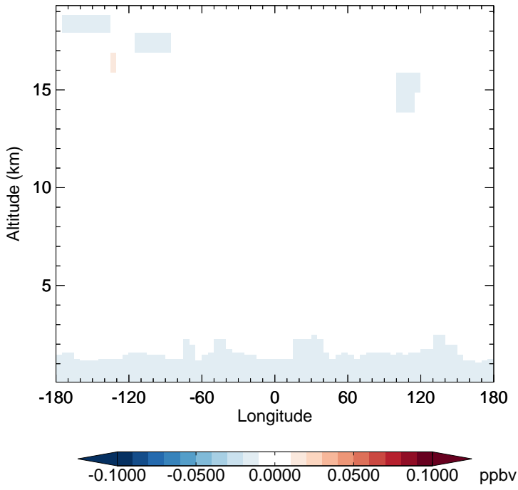
v11-02e-Run1 - v11-02e-Run0 CFC11 - Diff along 15S for Jan
