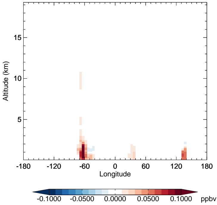
v11-02e-Run1 - v11-02e-Run0 RIPB - Diff along 15S for Jan
