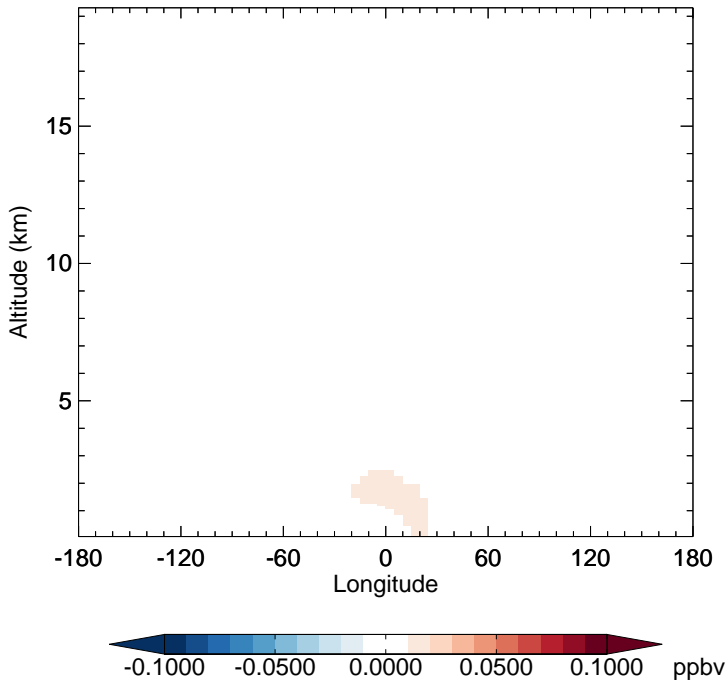
v11-02e-Run1 - v11-02e-Run0 SOAME - Diff along 15S for Jan
