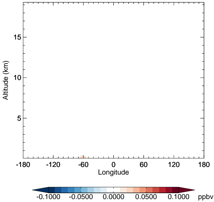
v11-02e-Run1 - v11-02d-Run1 MTPO - Diff along 15S for Jan
