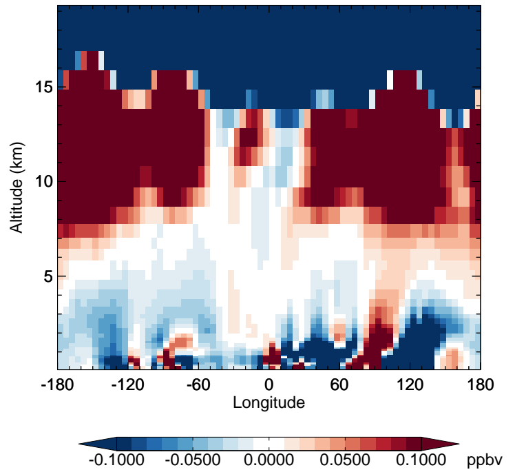
v11-02e-Run1 - v11-02d-Run1 HNO 3 - Diff along 42N for Jan
