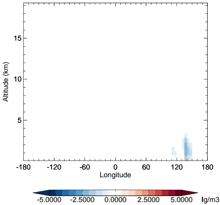
v11-02e-Run1 - v11-02d-Run1 DST2 - Diff along 15S for Jan
