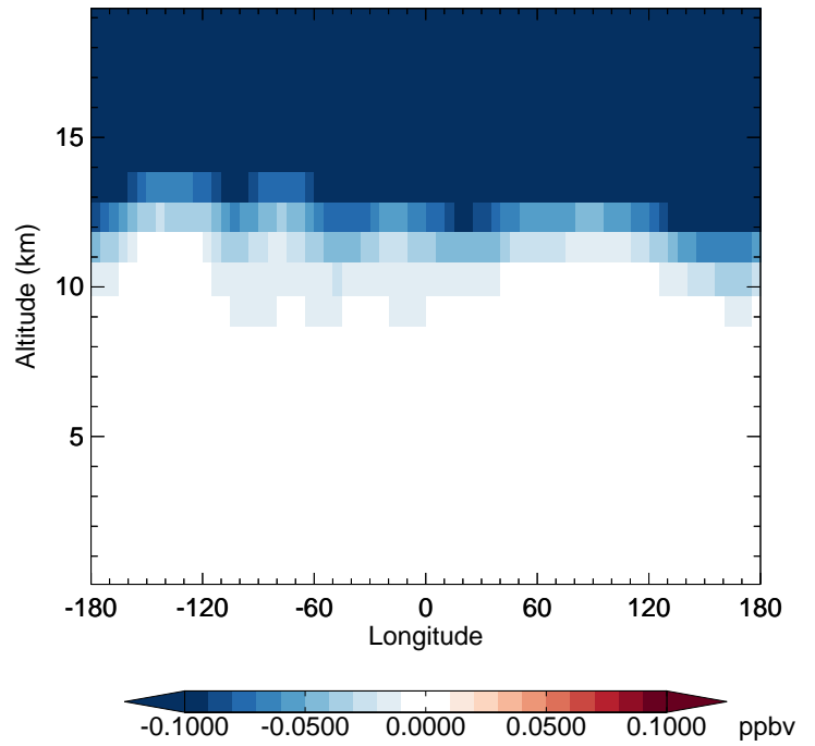
v11-02e-Run1 - v11-02d-Run1 HCl - Diff along 42N for Jan
