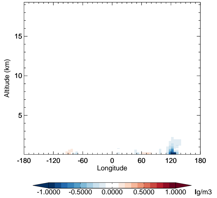
v11-02e-Run1 - v11-02e-Run0 OCPI - Diff along 42N for Jan
