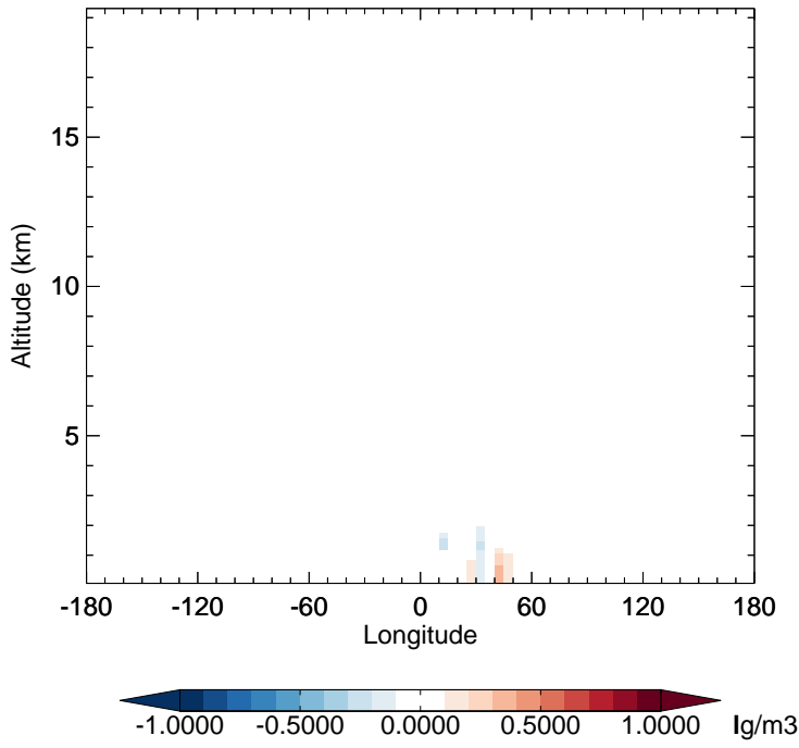
v11-02e-Run1 - v11-02e-Run0 OCPI - Diff along 15S for Jan
