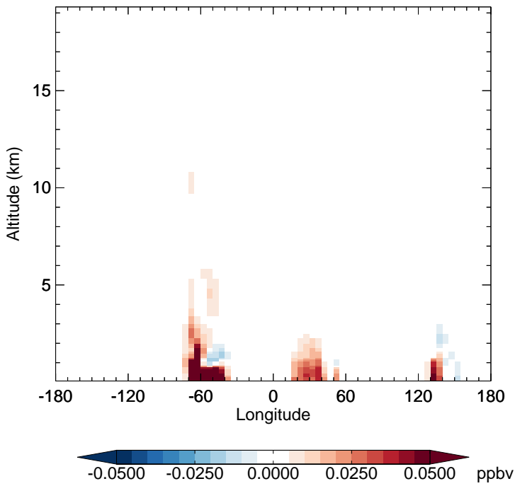
v11-02e-Run1 - v11-02d-Run1 RCHO - Diff along 15S for Jan
