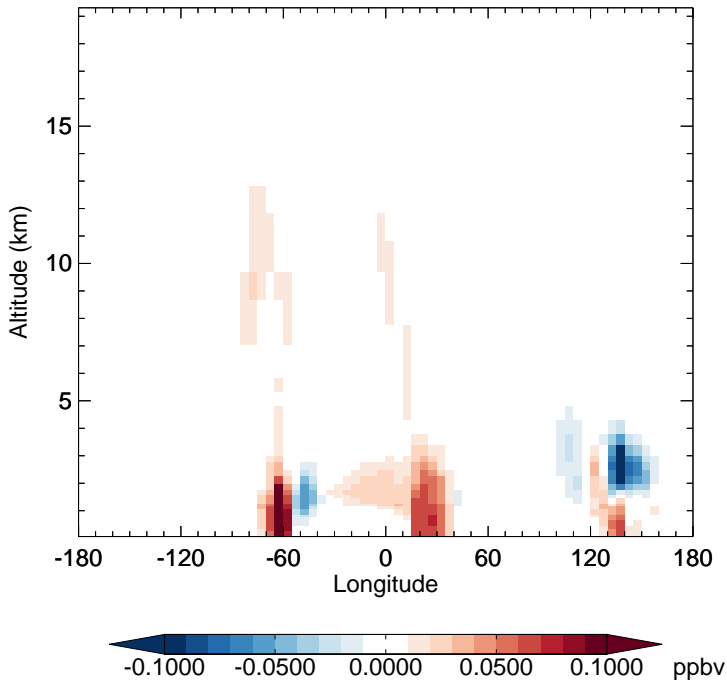
v11-02e-Run1 - v11-02e-Run0 ISO3 - Diff along 15S for Jan
