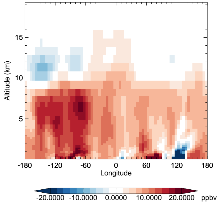
v11-02e-Run1 - v11-02d-Run1 CO - Diff along 42N for Jan
