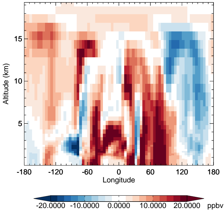
v11-02e-Run1 - v11-02e-Run0 CO - Diff along 15S for Jan
