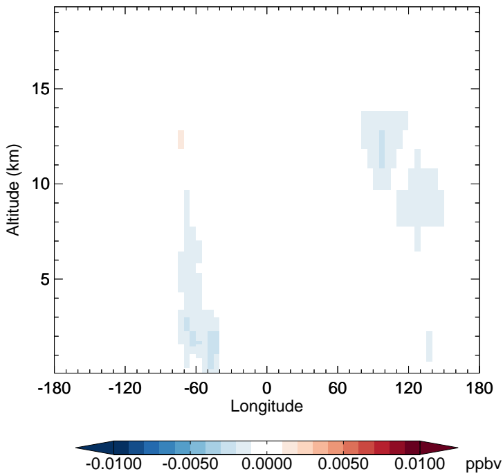
v11-02e-Run1 - v11-02d-Run1 R4N2 - Diff along 15S for Jan
