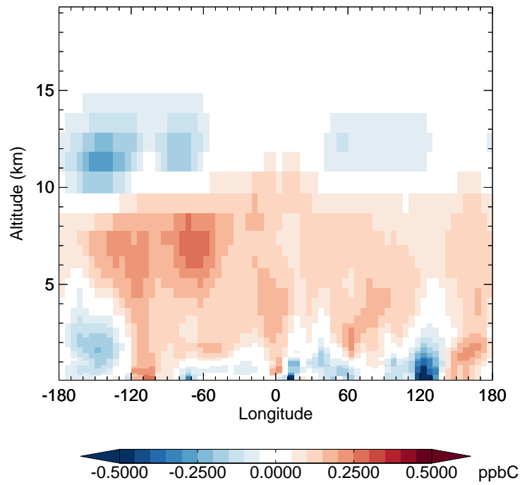
v11-02e-Run1 - v11-02d-Run1 ACET - Diff along 42N for Jan
