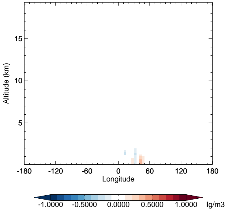
v11-02e-Run1 - v11-02d-Run1 OCPI - Diff along 15S for Jan
