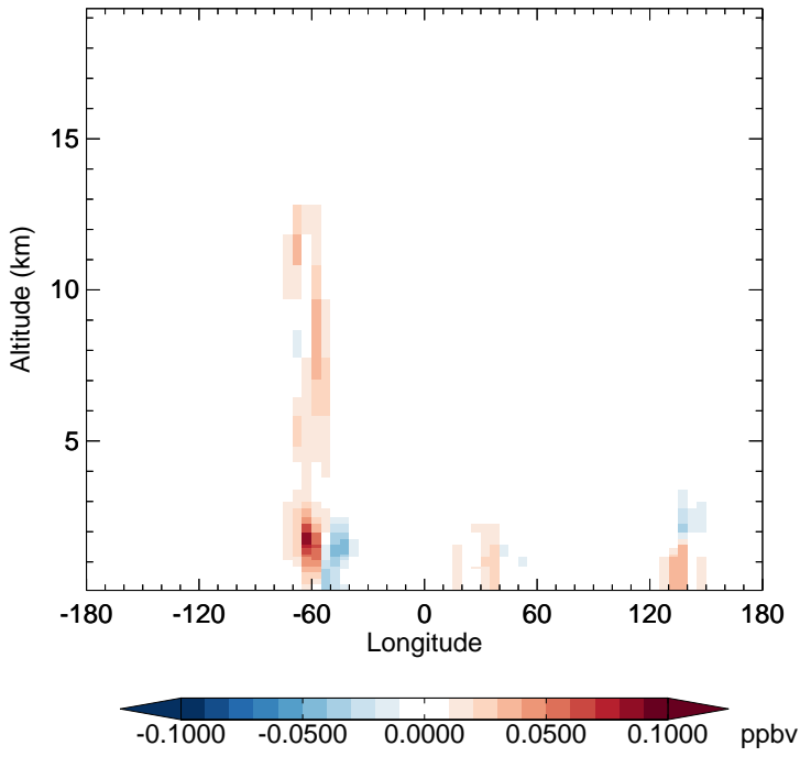
v11-02e-Run1 - v11-02e-Run0 IEPOXB - Diff along 15S for Jan
