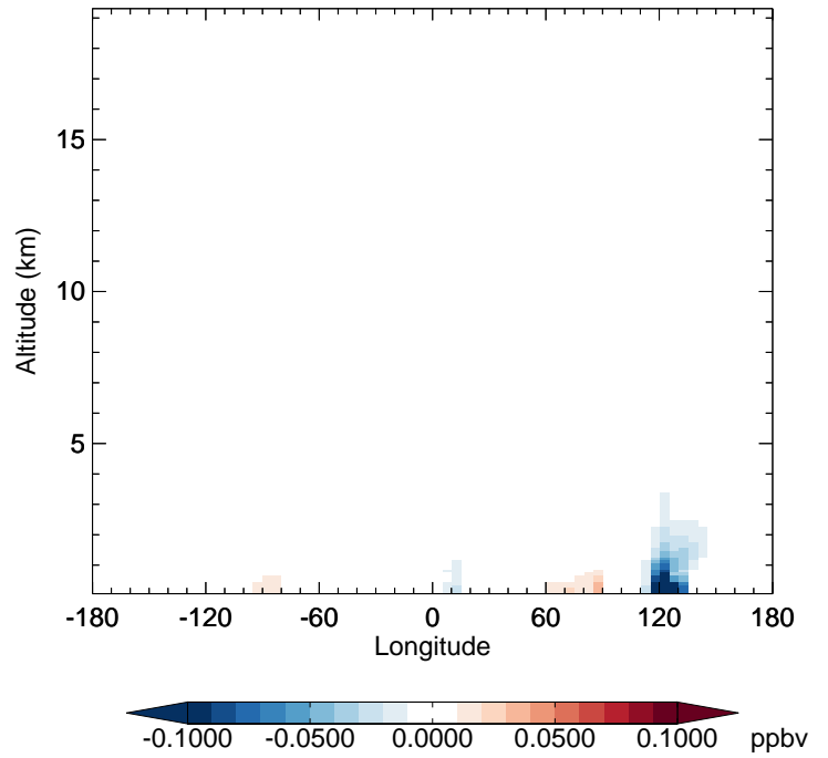
v11-02e-Run1 - v11-02d-Run1 SOAGX - Diff along 42N for Jan
