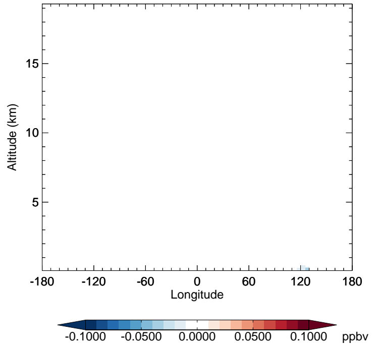
v11-02e-Run1 - v11-02e-Run0 ASOA3 - Diff along 42N for Jan
