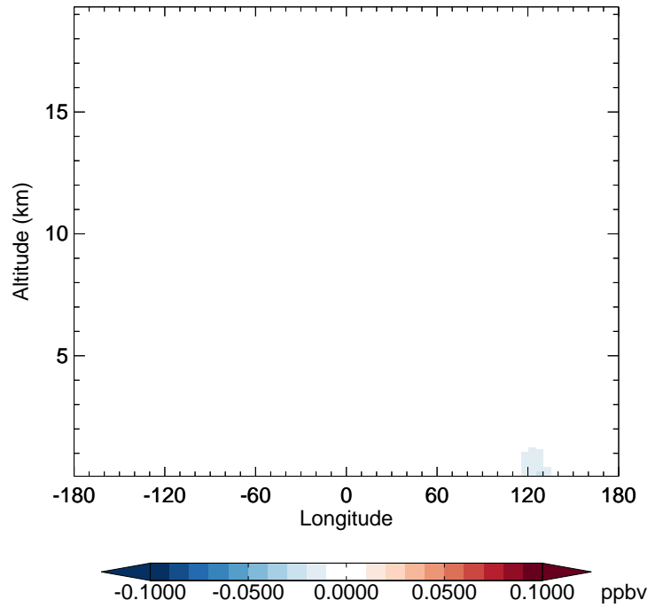
v11-02e-Run1 - v11-02d-Run1 ASOG3 - Diff along 42N for Jan
