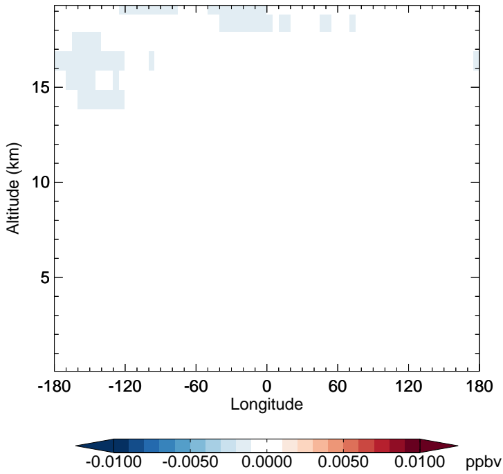
v11-02e-Run1 - v11-02d-Run1 BrNO3 - Diff along 15S for Jan
