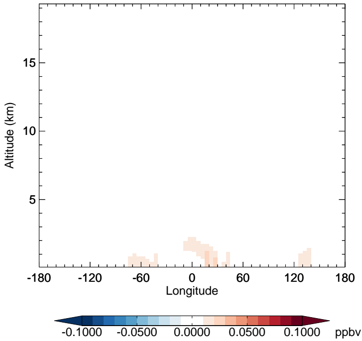
v11-02e-Run1 - v11-02d-Run1 SOAGX - Diff along 15S for Jan
