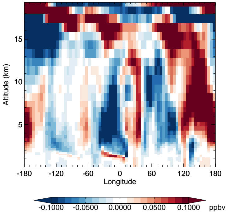
v11-02e-Run1 - v11-02d-Run1 HNO 3 - Diff along 15S for Jan
