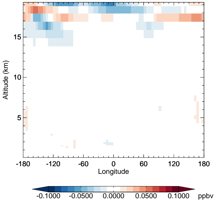
v11-02e-Run1 - v11-02e-Run0 HCl - Diff along 15S for Jan
