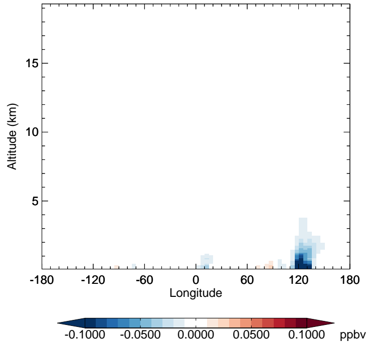
v11-02e-Run1 - v11-02e-Run0 SOAGX - Diff along 42N for Jan
