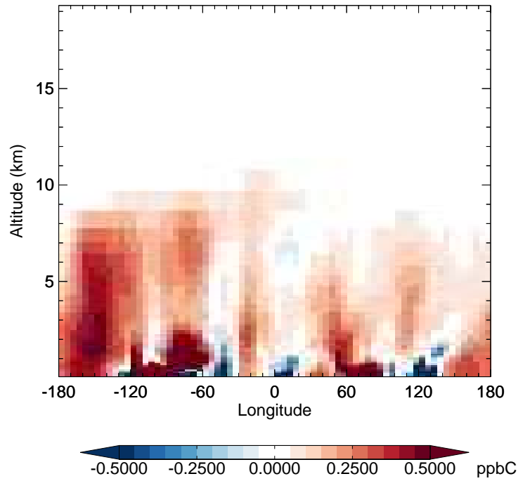
v11-02e-Run1 - v11-02d-Run1 ALK4 - Diff along 42N for Jan
