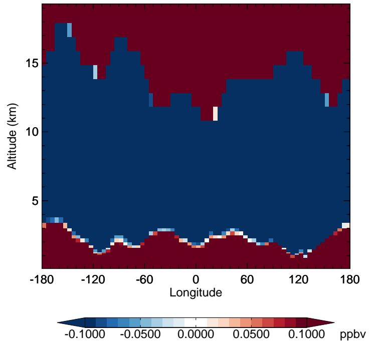
v11-02e-Run1 - v11-02d-Run1 N2O - Diff along 42N for Jan
