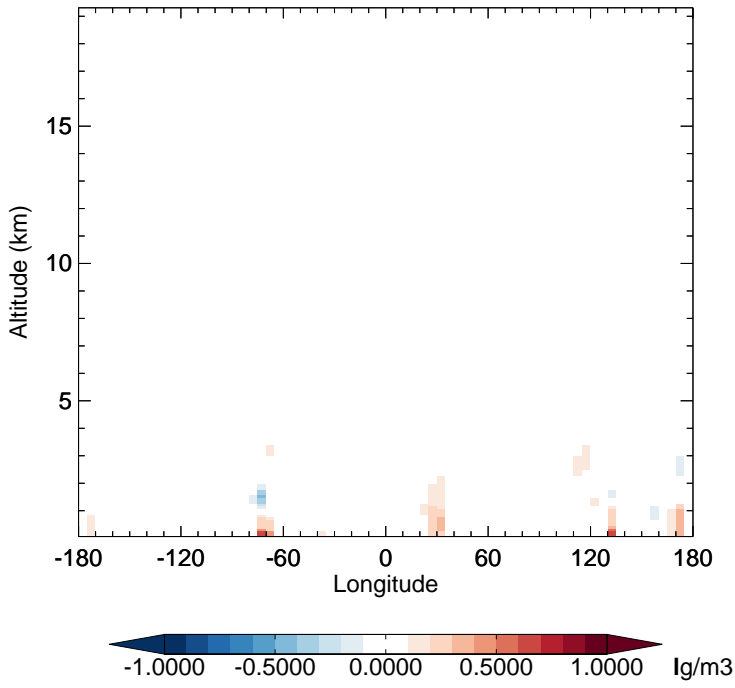
v11-02e-Run1 - v11-02e-Run0 SO 2 - Diff along 15S for Jan
