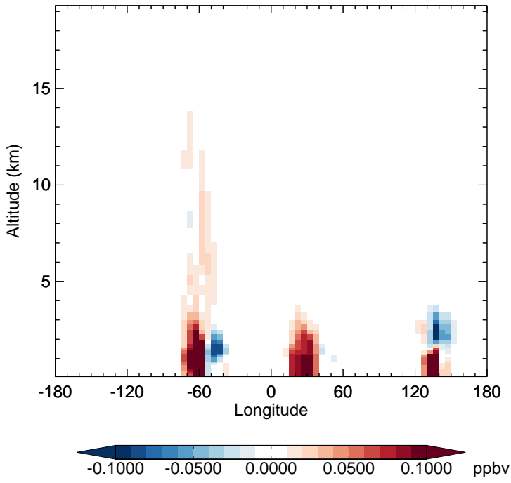
v11-02e-Run1 - v11-02e-Run0 GLYC - Diff along 15S for Jan
