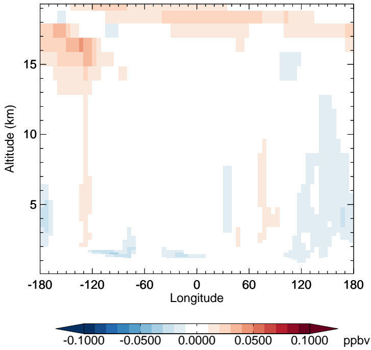
v11-02e-Run1 - v11-02e-Run0 CH3Cl - Diff along 15S for Jan
