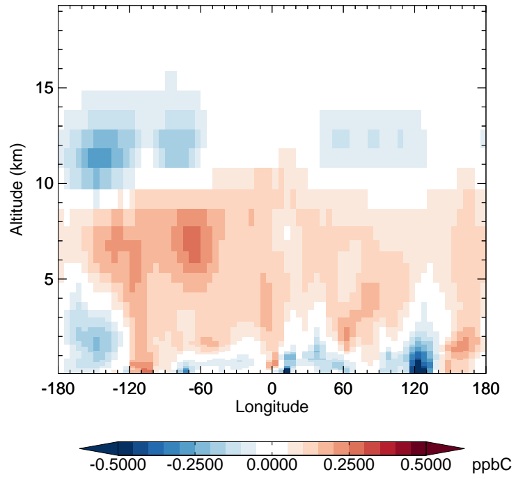
v11-02e-Run1 - v11-02e-Run0 ACET - Diff along 42N for Jan
