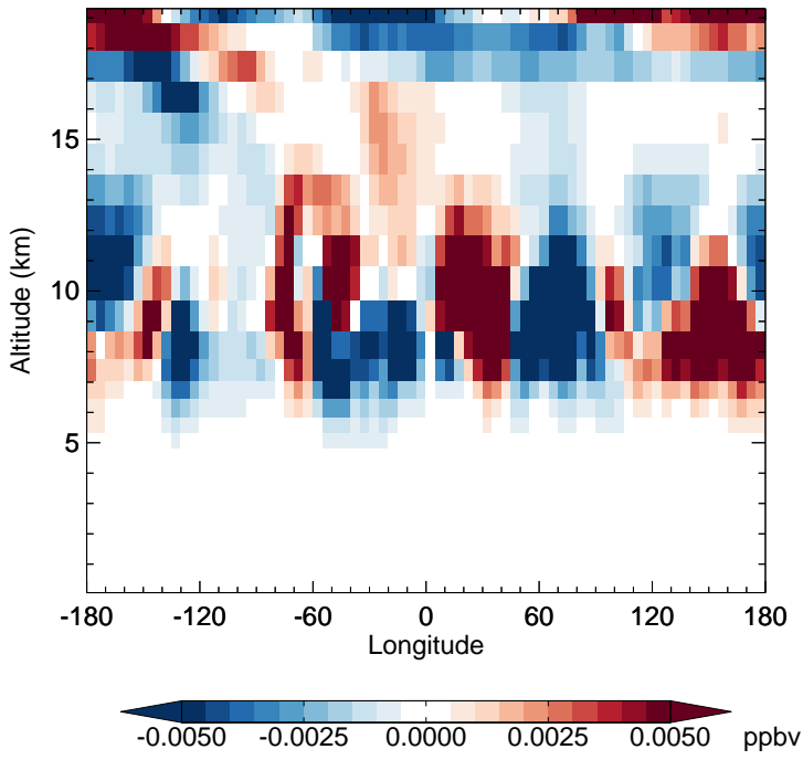
v11-02e-Run1 - v11-02e-Run0 HNO 4 - Diff along 15S for Jan
