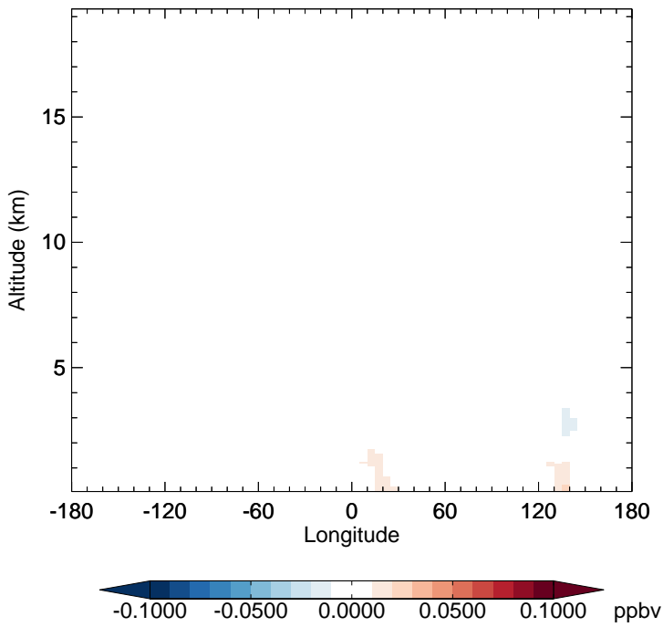
v11-02e-Run1 - v11-02d-Run1 ISOG1 - Diff along 15S for Jan
