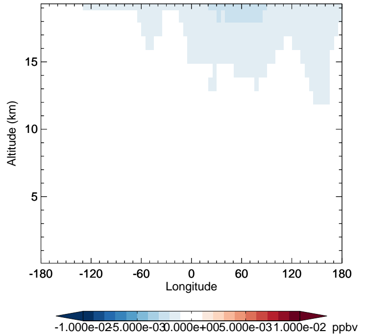
v11-02e-Run1 - v11-02d-Run1 BrO - Diff along 42N for Jan
