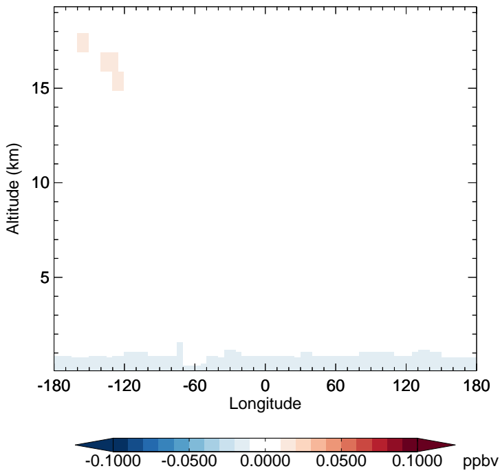
v11-02e-Run1 - v11-02d-Run1 CFC11 - Diff along 15S for Jan
