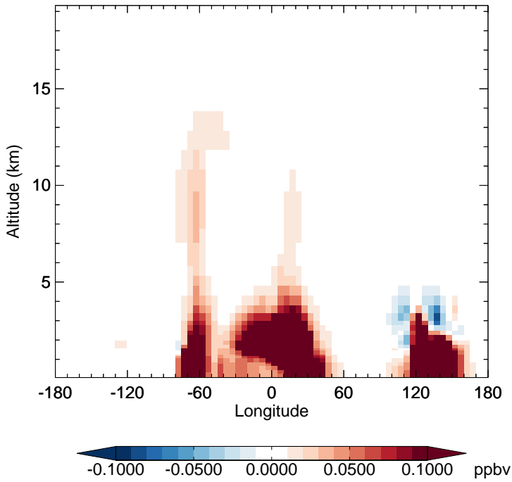
v11-02e-Run1 - v11-02d-Run1 SOAIE - Diff along 15S for Jan
