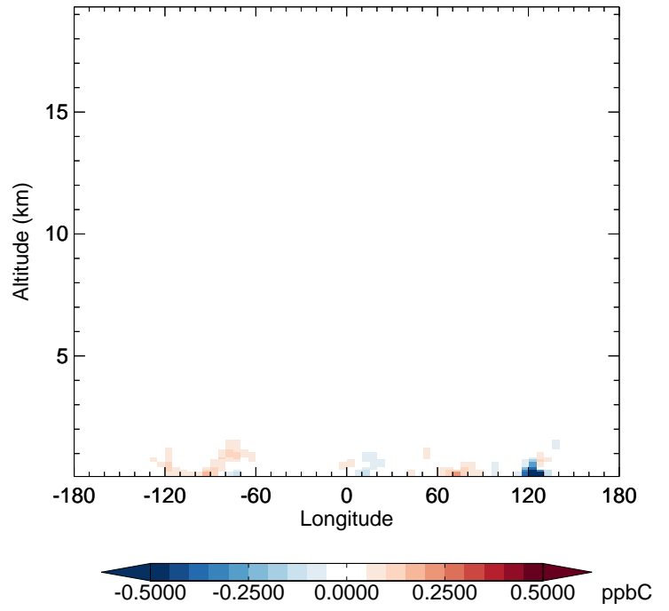
v11-02e-Run1 - v11-02e-Run0 ALD2 - Diff along 42N for Jan
