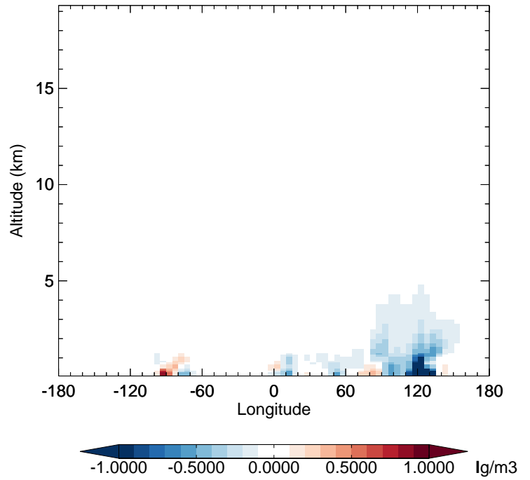
v11-02e-Run1 - v11-02d-Run1 NH4 - Diff along 42N for Jan
