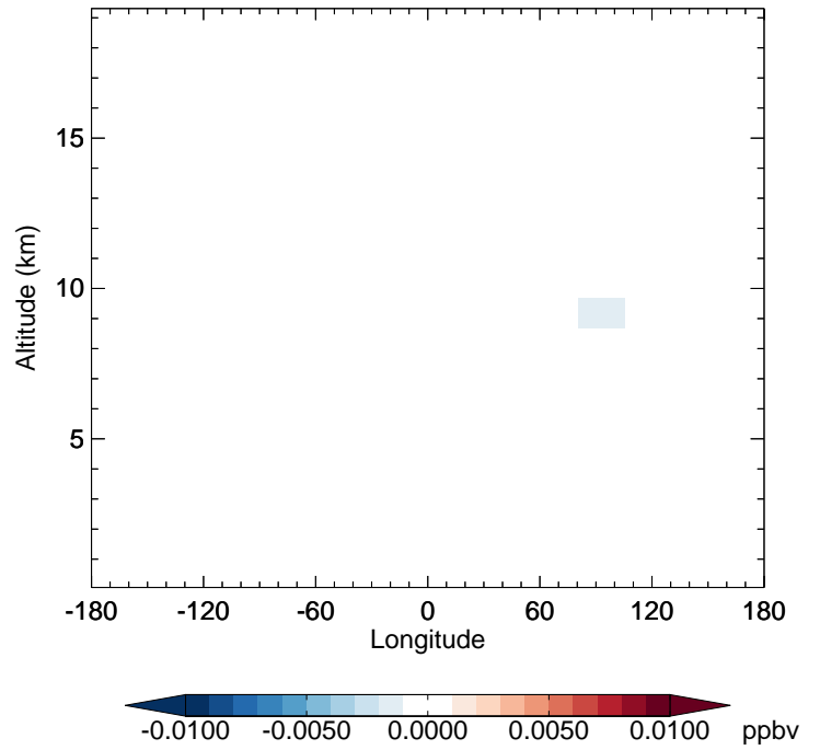
v11-02e-Run1 - v11-02d-Run1 HBr - Diff along 42N for Jan
