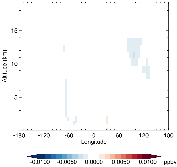
v11-02e-Run1 - v11-02e-Run0 R4N2 - Diff along 15S for Jan
