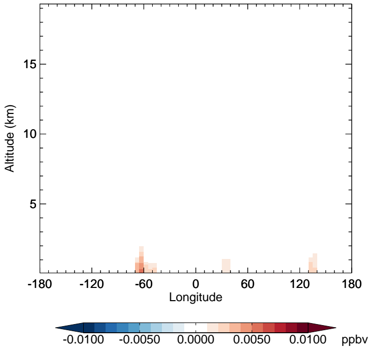
v11-02e-Run1 - v11-02e-Run0 MOBA - Diff along 15S for Jan
