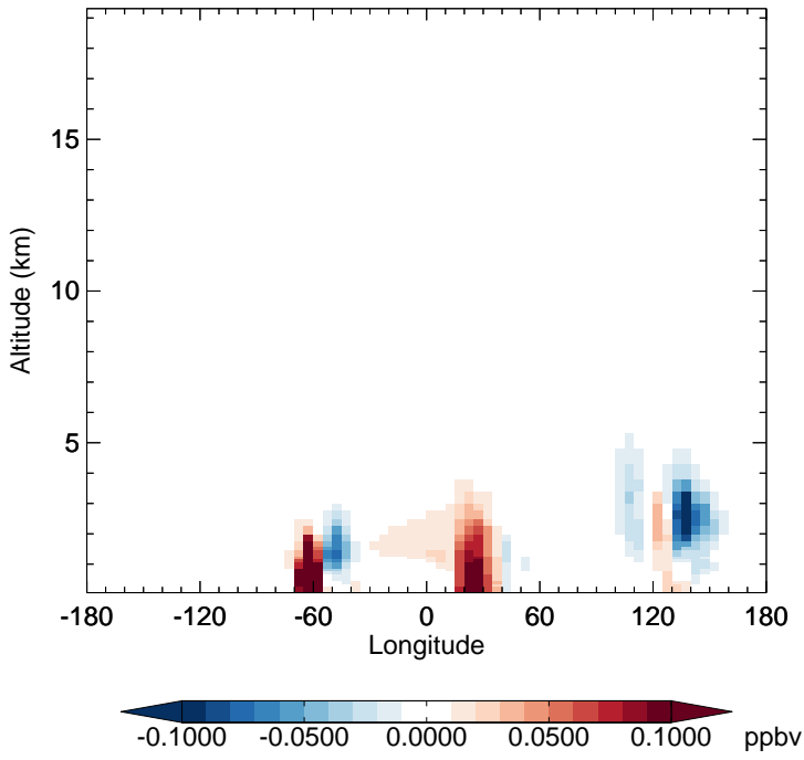
v11-02e-Run1 - v11-02e-Run0 TSOG3 - Diff along 15S for Jan
