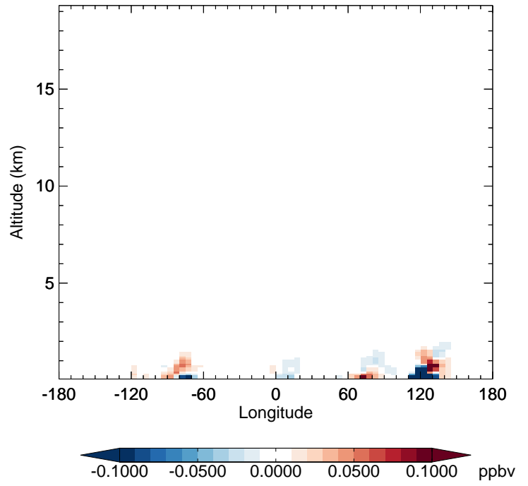
v11-02e-Run1 - v11-02e-Run0 SOAP - Diff along 42N for Jan
