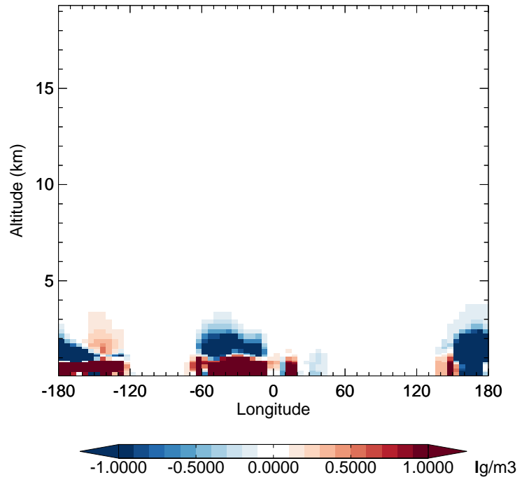
v11-02e-Run1 - v11-02e-Run0 SALC - Diff along 42N for Jan
