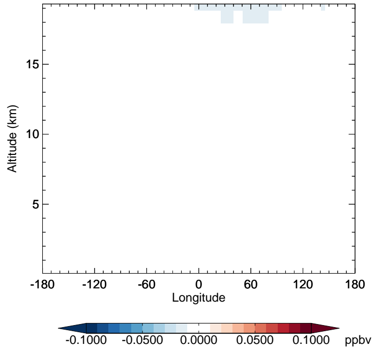
v11-02e-Run1 - v11-02d-Run1 ClO - Diff along 42N for Jan
