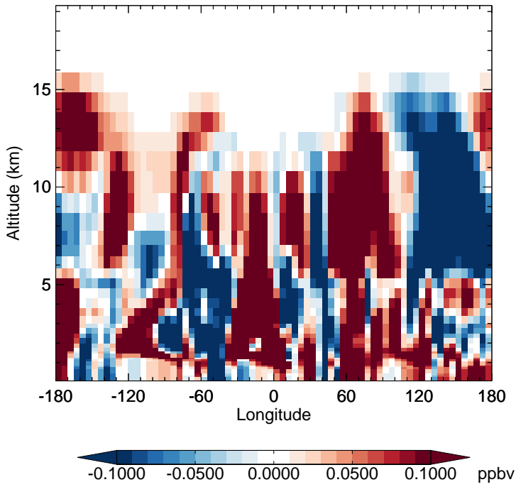
v11-02e-Run1 - v11-02e-Run0 H2O2 - Diff along 15S for Jan
