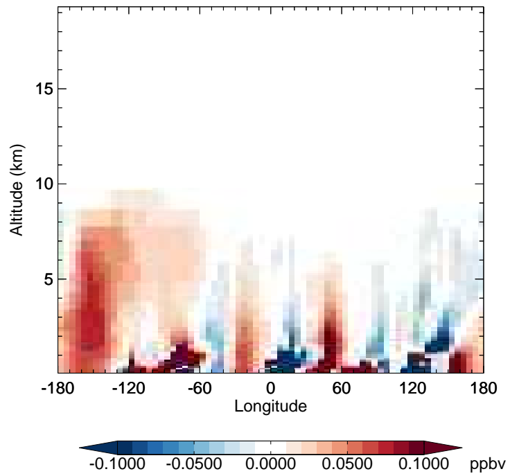
v11-02e-Run1 - v11-02d-Run1 TOLU - Diff along 42N for Jan
