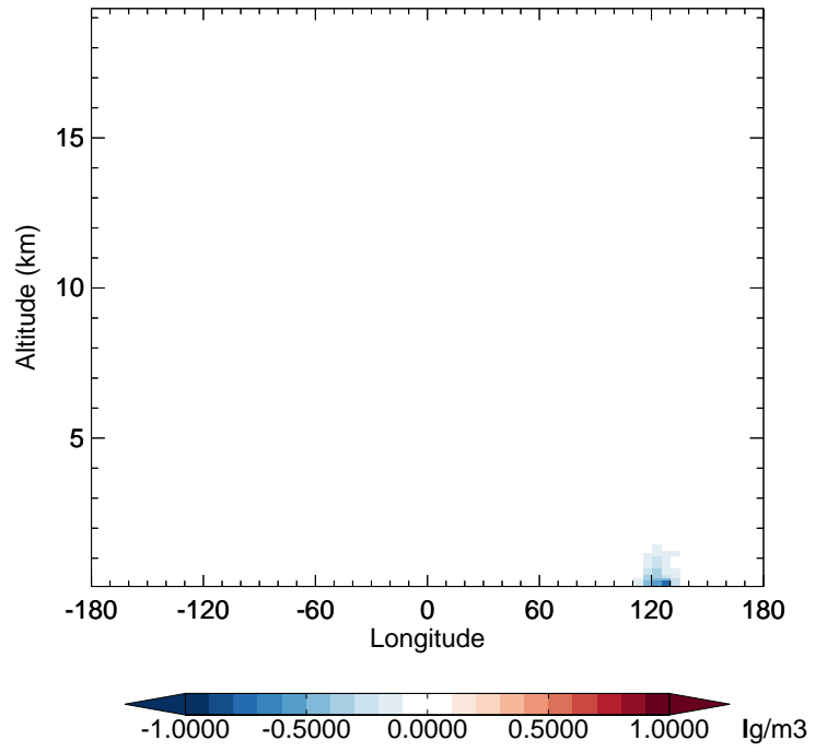
v11-02e-Run1 - v11-02e-Run0 BCPI - Diff along 42N for Jan
