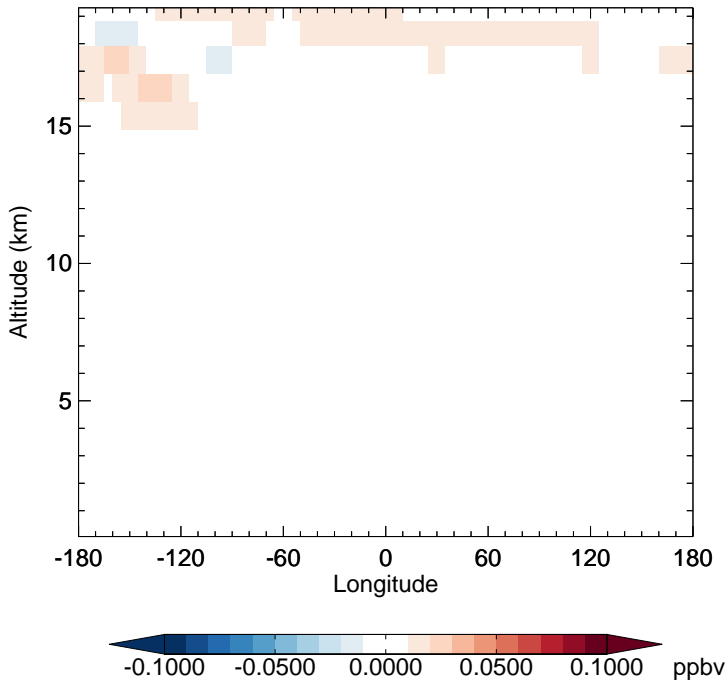
v11-02e-Run1 - v11-02e-Run0 OCS - Diff along 15S for Jan
