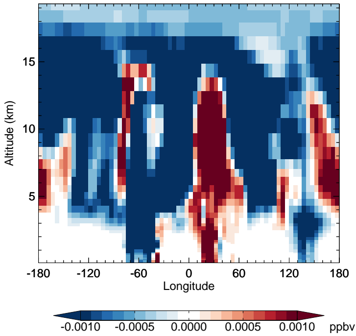
v11-02e-Run1 - v11-02e-Run0 PPN - Diff along 15S for Jan
