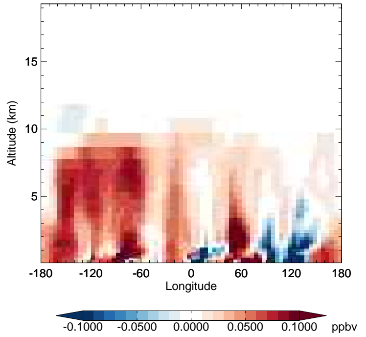
v11-02e-Run1 - v11-02e-Run0 BENZ - Diff along 42N for Jan
