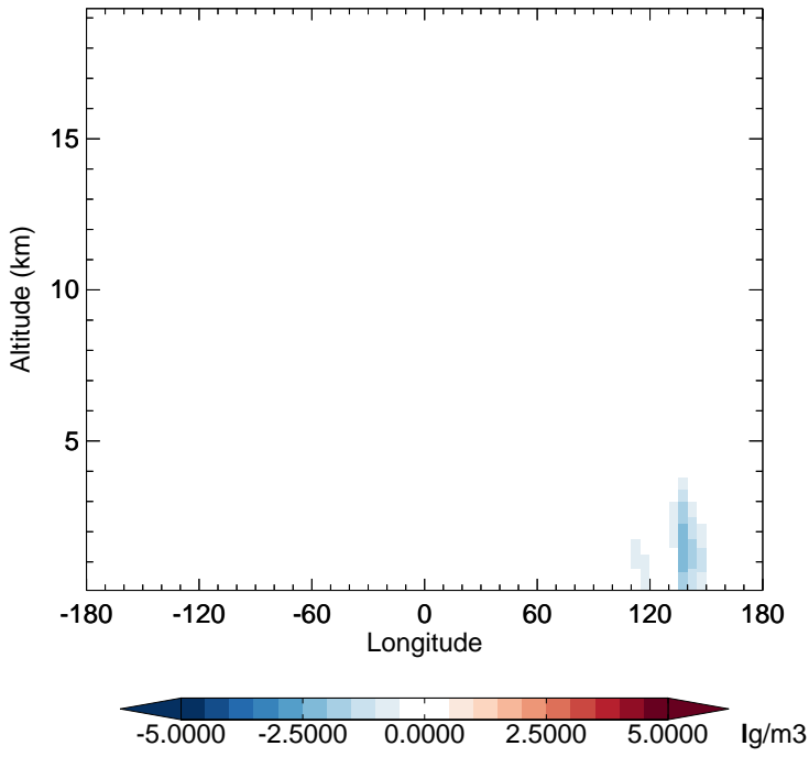
v11-02e-Run1 - v11-02e-Run0 DST2 - Diff along 15S for Jan
