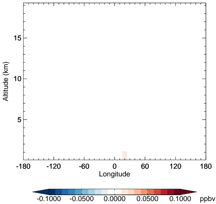
v11-02e-Run1 - v11-02d-Run1 LVOCOA - Diff along 15S for Jan
