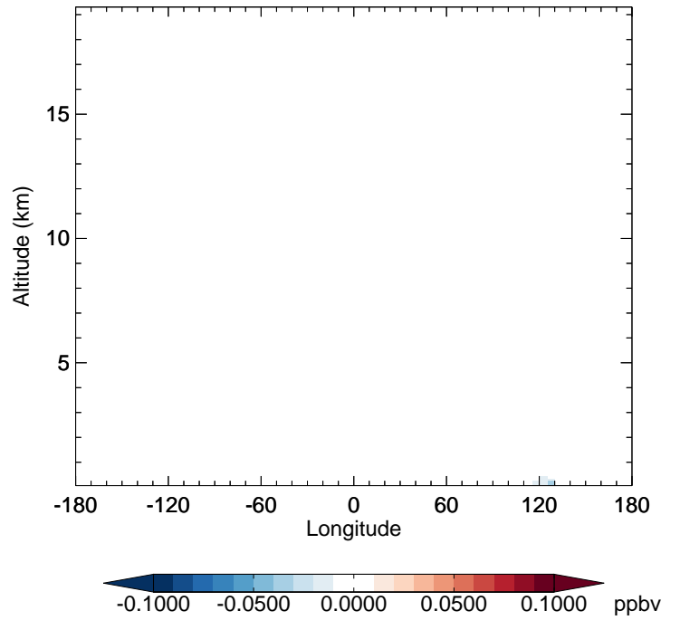
v11-02e-Run1 - v11-02d-Run1 ASOA3 - Diff along 42N for Jan
