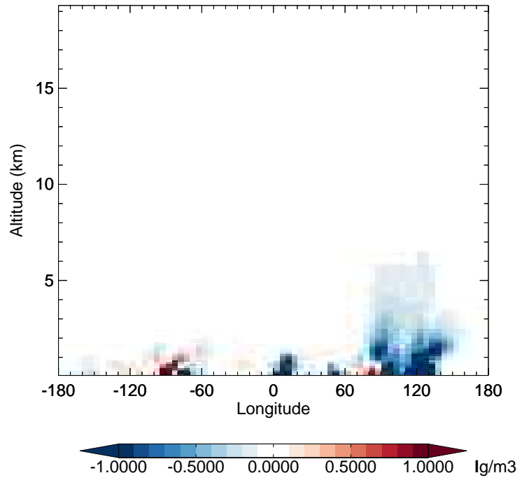
v11-02e-Run1 - v11-02e-Run0 NIT - Diff along 42N for Jan
