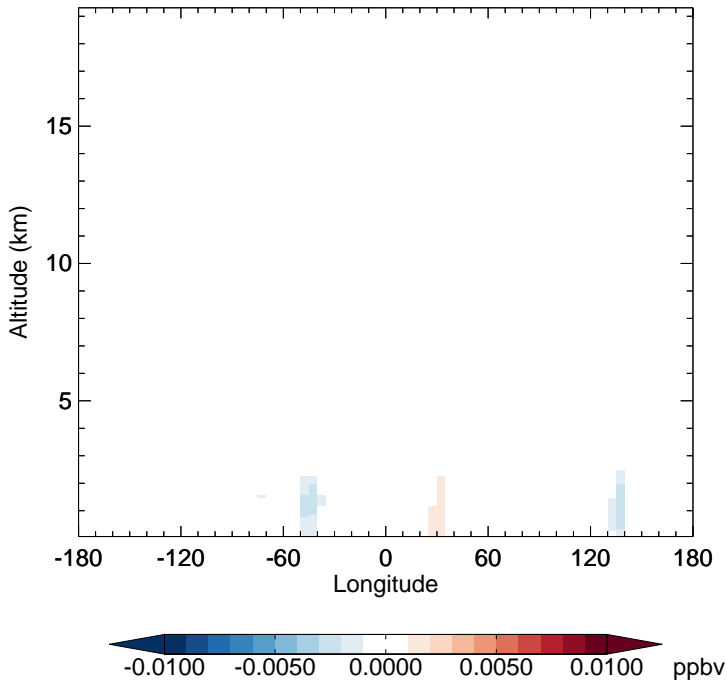
v11-02e-Run1 - v11-02d-Run1 MVKN - Diff along 15S for Jan
