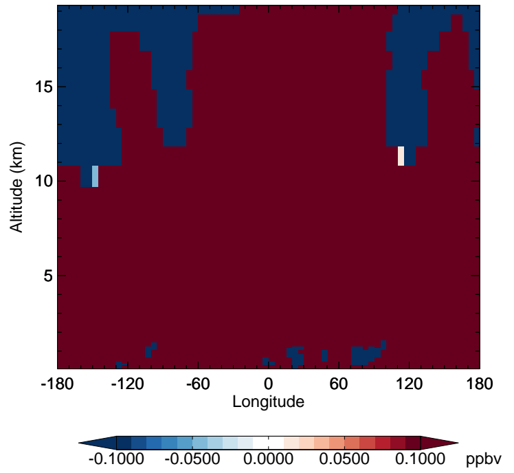
v11-02e-Run1 - v11-02e-Run0 CH4 - Diff along 42N for Jan
