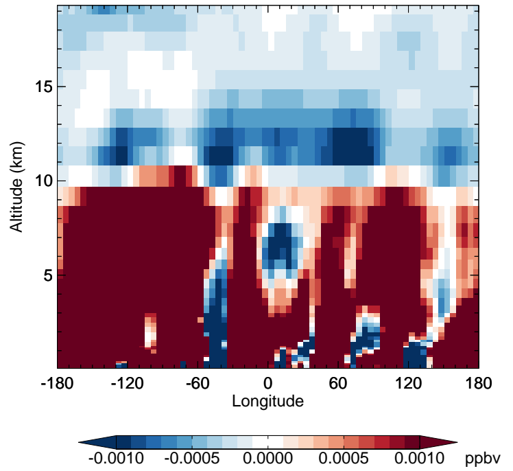
v11-02e-Run1 - v11-02e-Run0 PPN - Diff along 42N for Jan
