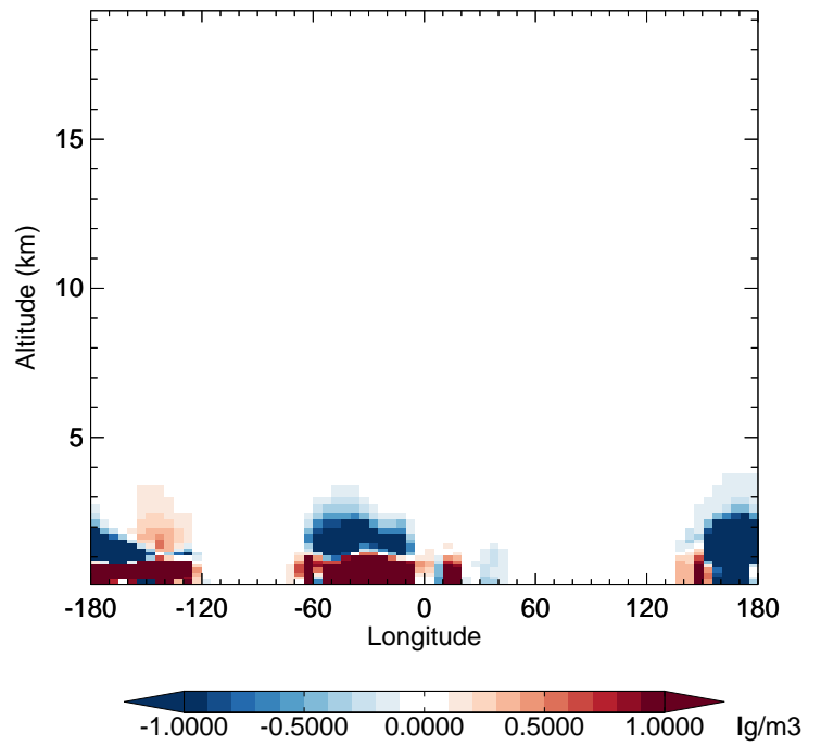
v11-02e-Run1 - v11-02d-Run1 SALC - Diff along 42N for Jan
