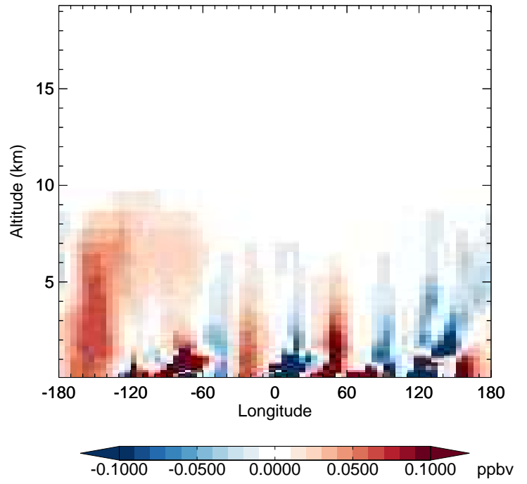
v11-02e-Run1 - v11-02e-Run0 TOLU - Diff along 42N for Jan
