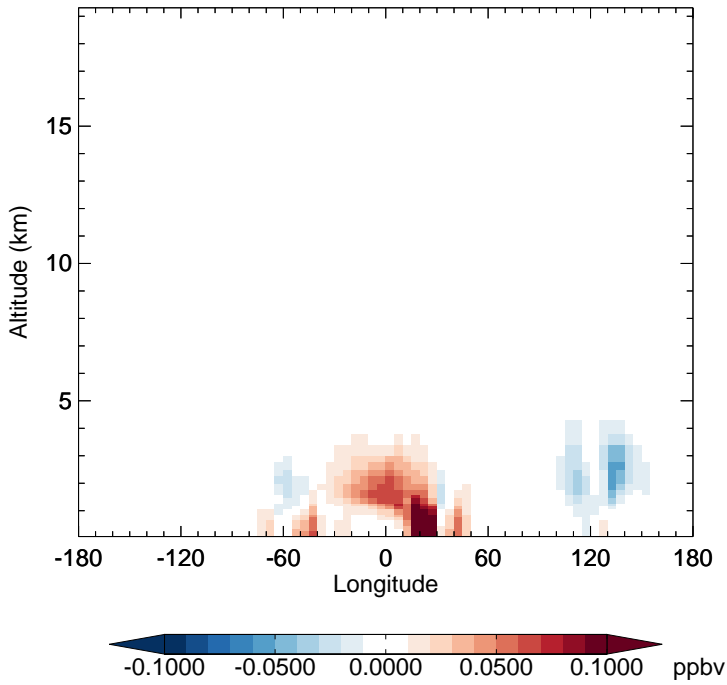
v11-02e-Run1 - v11-02d-Run1 INDIOL - Diff along 15S for Jan
