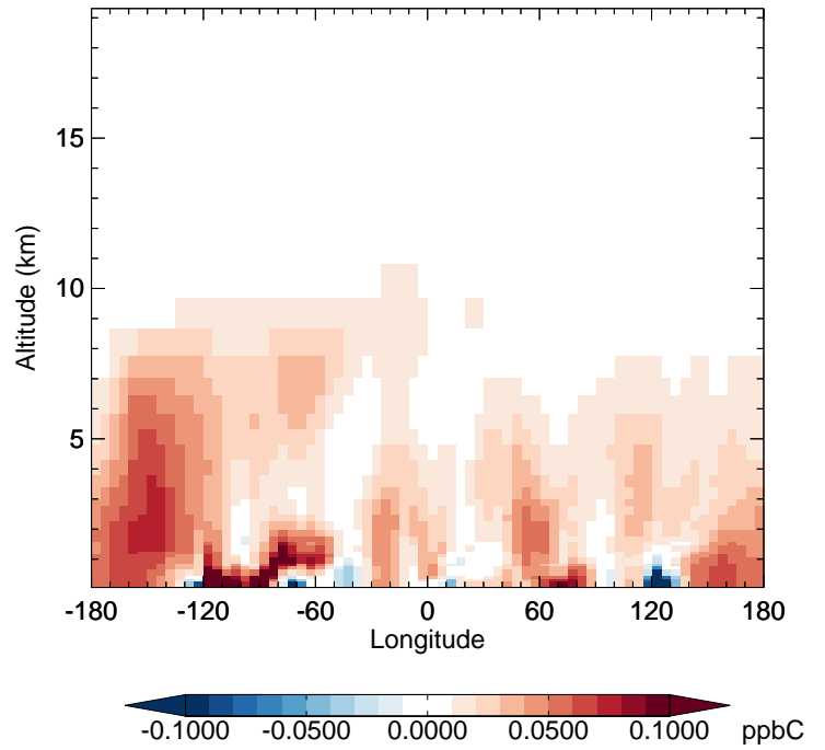
v11-02e-Run1 - v11-02d-Run1 MEK - Diff along 42N for Jan
