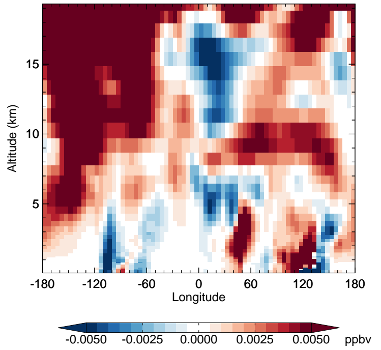
v11-02e-Run1 - v11-02e-Run0 HNO 4 - Diff along 42N for Jan
