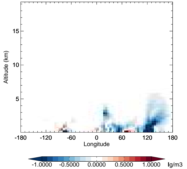
v11-02e-Run1 - v11-02d-Run1 SO 2 - Diff along 42N for Jan
