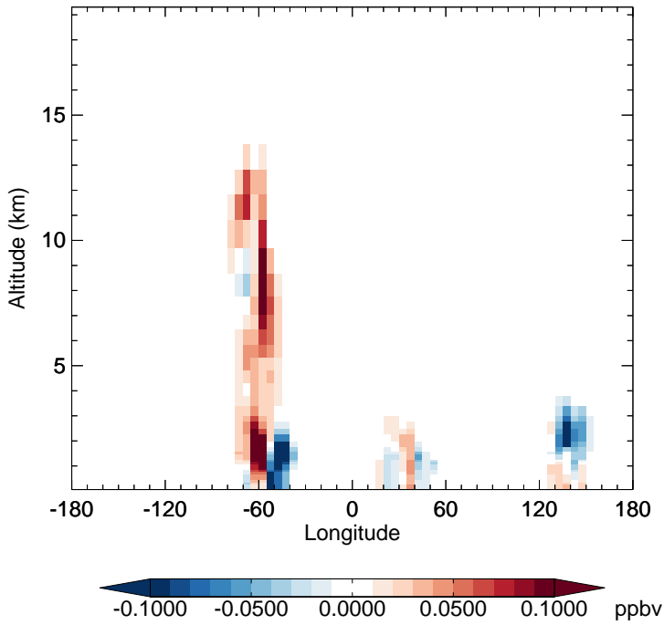
v11-02e-Run1 - v11-02d-Run1 IEPOXA - Diff along 15S for Jan
