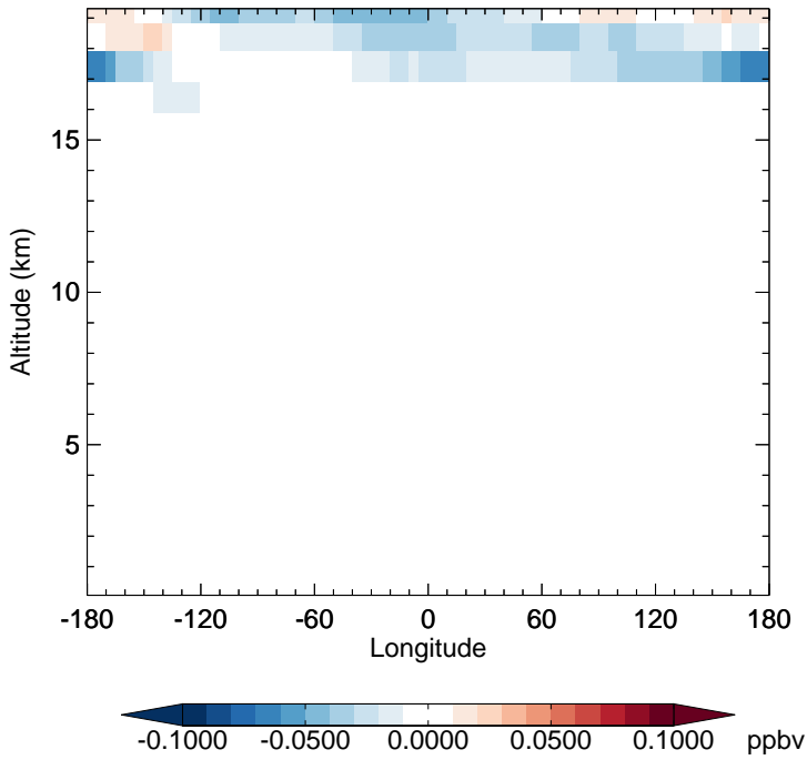
v11-02e-Run1 - v11-02d-Run1 CINO3 - Diff along 15S for Jan
