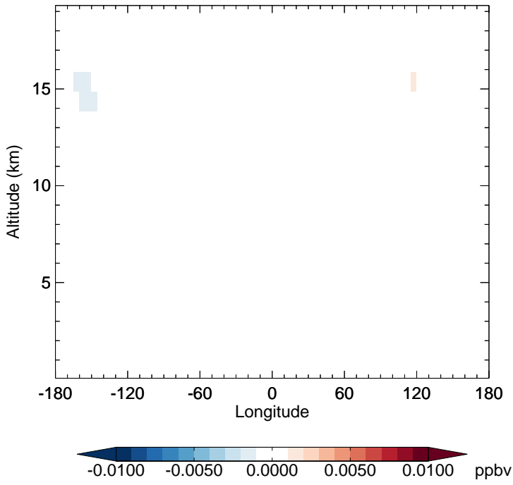
v11-02e-Run1 - v11-02e-Run0 BrNO3 - Diff along 15S for Jan
