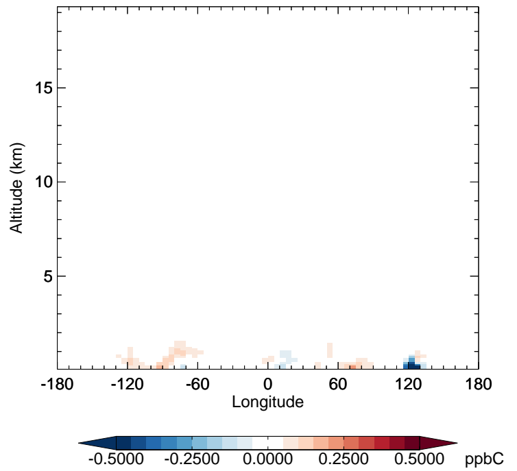
v11-02e-Run1 - v11-02d-Run1 ALD2 - Diff along 42N for Jan
