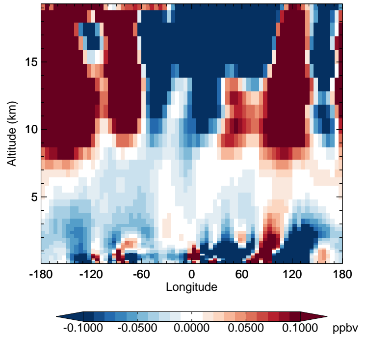
v11-02e-Run1 - v11-02e-Run0 HNO 3 - Diff along 42N for Jan
