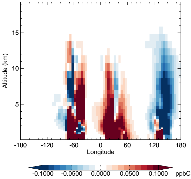
v11-02e-Run1 - v11-02e-Run0 MEK - Diff along 15S for Jan
