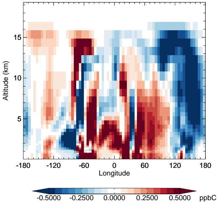
v11-02e-Run1 - v11-02e-Run0 ACET - Diff along 15S for Jan
