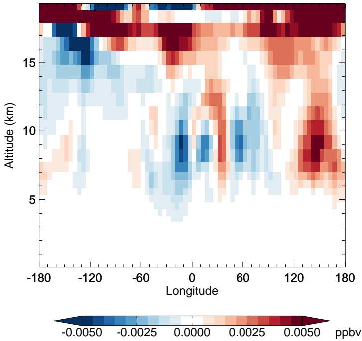
v11-02e-Run1 - v11-02d-Run1 N2O5 - Diff along 15S for Jan
