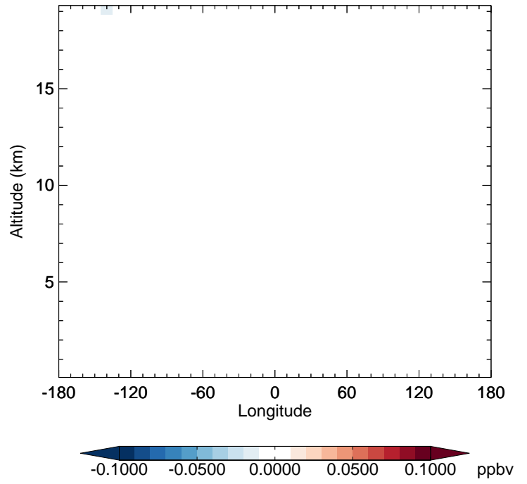
v11-02e-Run1 - v11-02e-Run0 CCI4 - Diff along 42N for Jan
