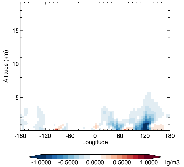
v11-02e-Run1 - v11-02e-Run0 SO4 - Diff along 42N for Jan
