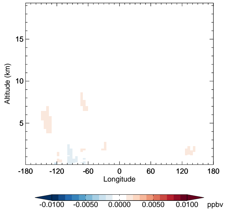
v11-02e-Run1 - v11-02d-Run1 R4N2 - Diff along 42N for Jan
