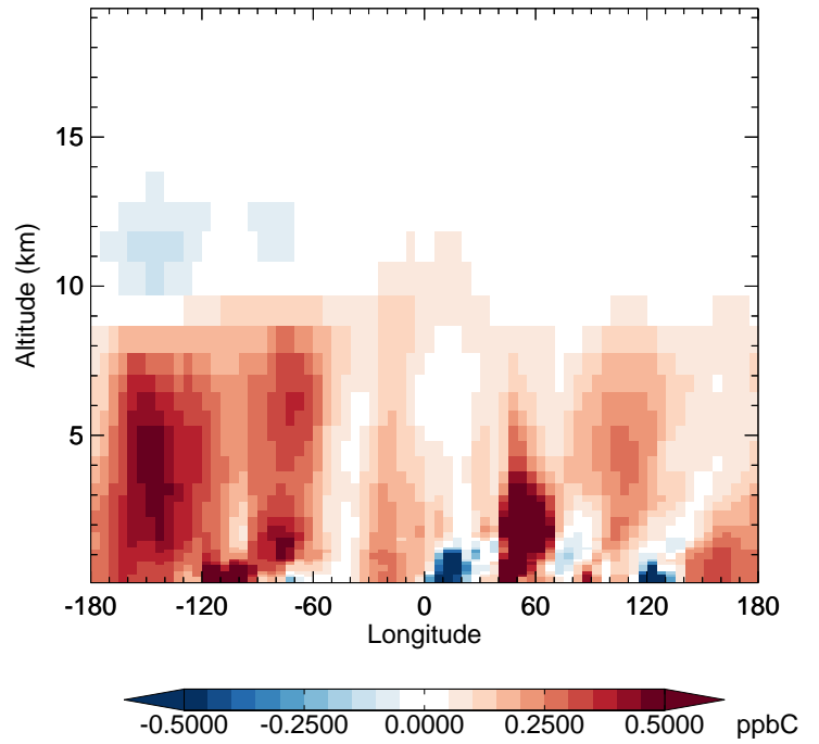
v11-02e-Run1 - v11-02d-Run1 C2H6 - Diff along 42N for Jan
