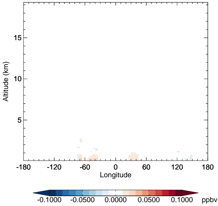
v11-02e-Run1 - v11-02e-Run0 TOLU - Diff along 15S for Jan
