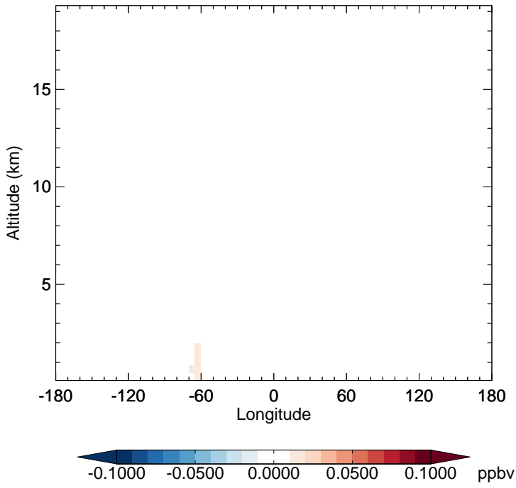
v11-02e-Run1 - v11-02e-Run0 RIPD - Diff along 15S for Jan
