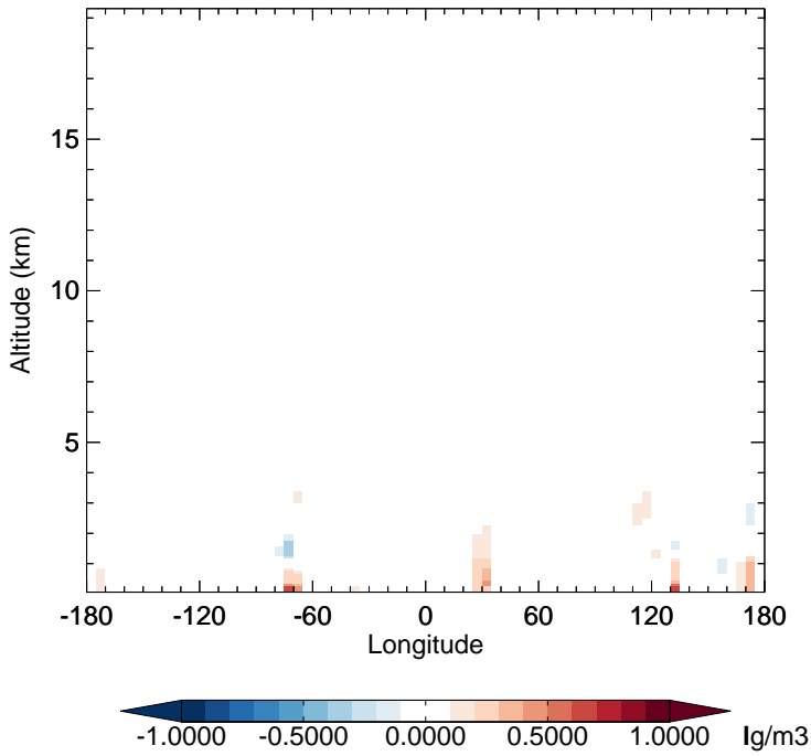
v11-02e-Run1 - v11-02d-Run1 SO 2 - Diff along 15S for Jan
