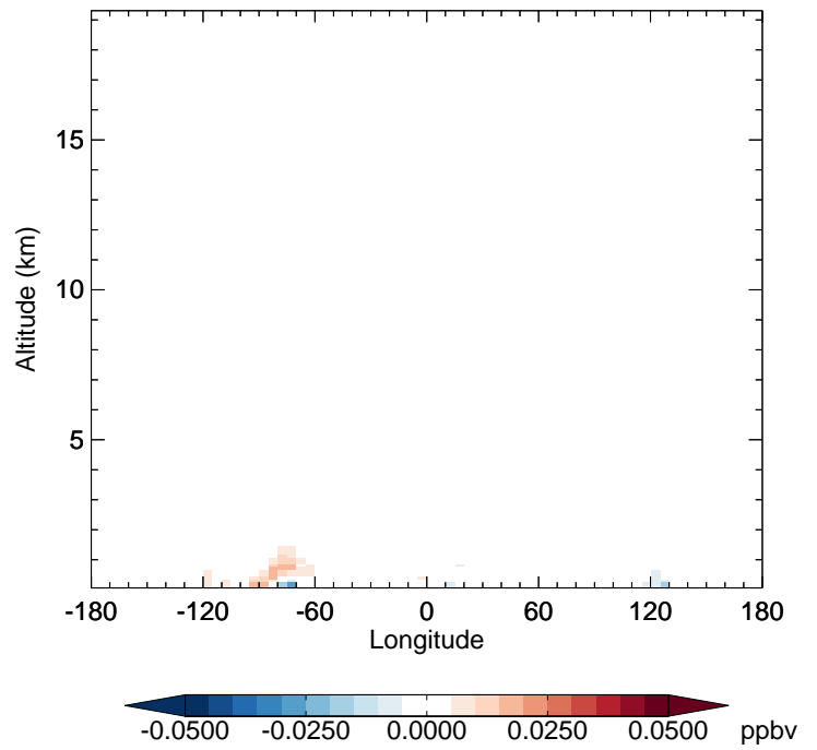
v11-02e-Run1 - v11-02d-Run1 RCHO - Diff along 42N for Jan
