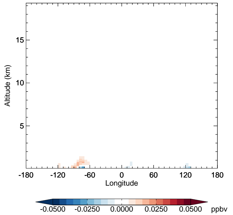
v11-02e-Run1 - v11-02e-Run0 RCHO - Diff along 42N for Jan
