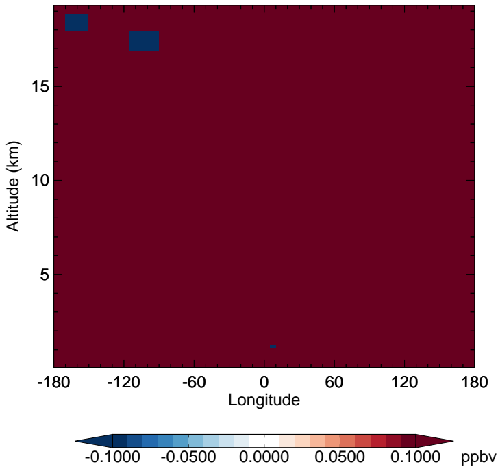
v11-02e-Run1 - v11-02e-Run0 CH4 - Diff along 15S for Jan
