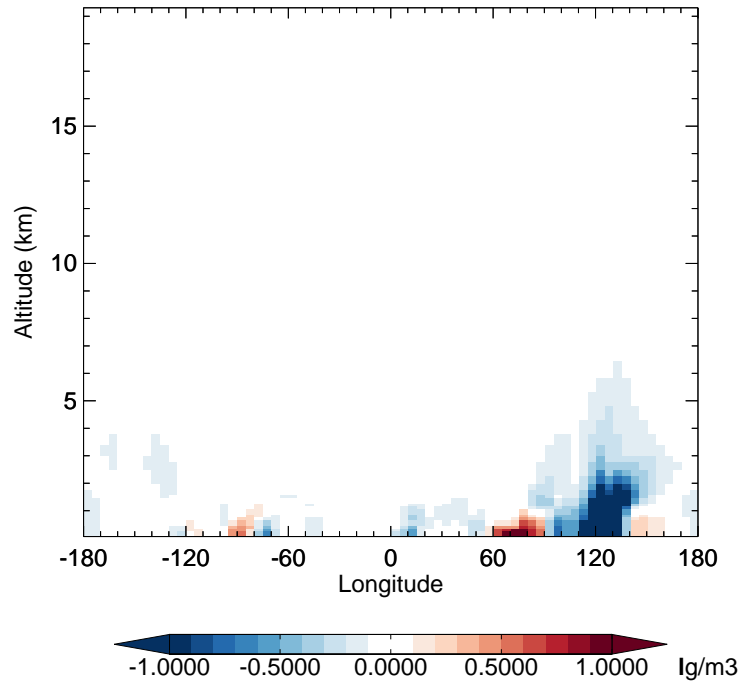
v11-02e-Run1 - v11-02e-Run0 SOAS - Diff along 42N for Jan
