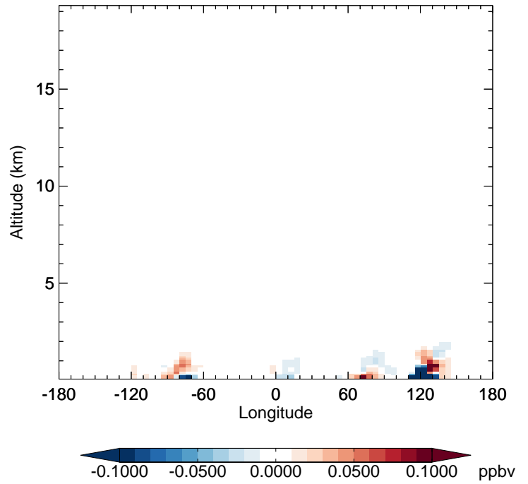
v11-02e-Run1 - v11-02d-Run1 SOAP - Diff along 42N for Jan
