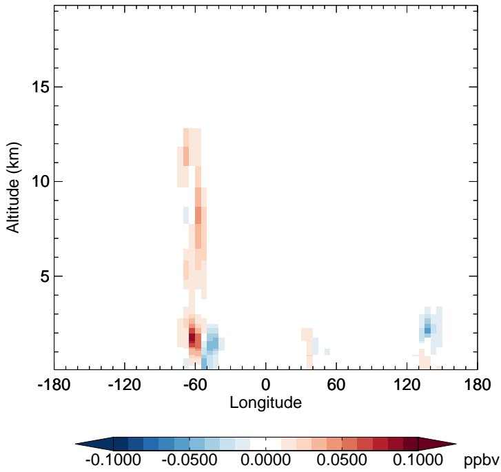
v11-02e-Run1 - v11-02d-Run1 IEPOXB - Diff along 15S for Jan
