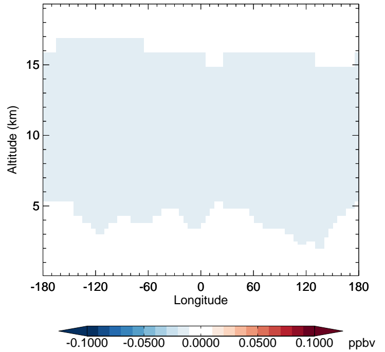
v11-02e-Run1 - v11-02d-Run1 HCFC141b - Diff along 42N for Jan
