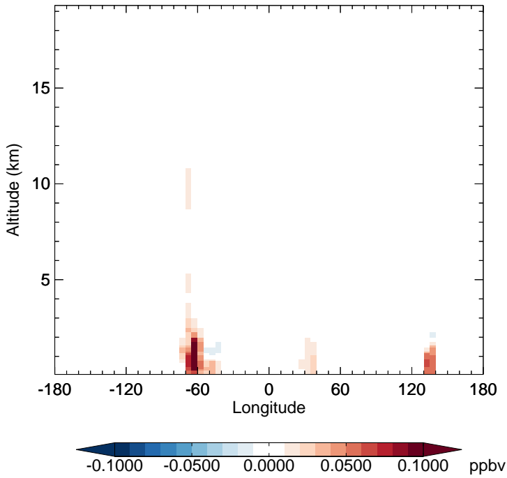
v11-02e-Run1 - v11-02d-Run1 RIPB - Diff along 15S for Jan
