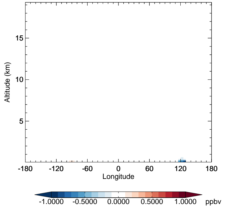
v11-02e-Run1 - v11-02d-Run1 HNO 2 - Diff along 42N for Jan
