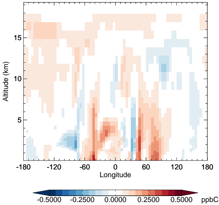
v11-02e-Run1 - v11-02d-Run1 C2H6 - Diff along 15S for Jan
