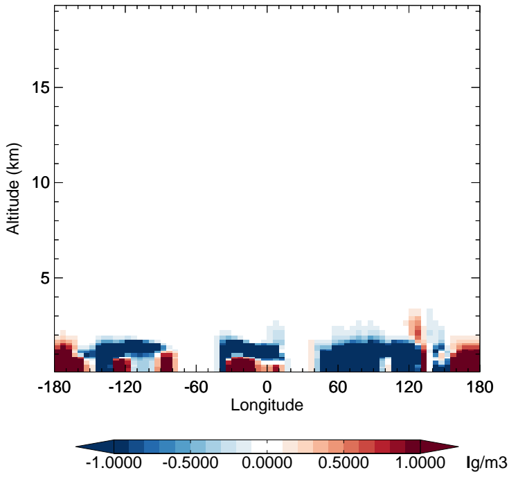
v11-02e-Run1 - v11-02e-Run0 SALC - Diff along 15S for Jan
