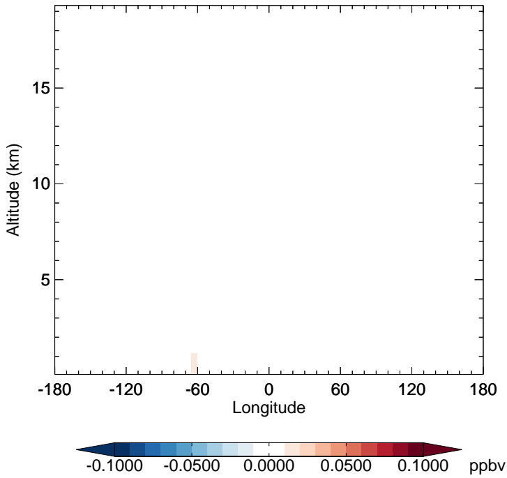
v11-02e-Run1 - v11-02d-Run1 TSOA3 - Diff along 15S for Jan
