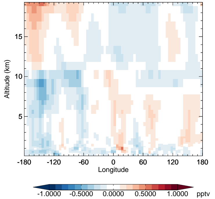
v11-02e-Run1 - v11-02d-Run1 HO2 - Diff along 42N for Jan
