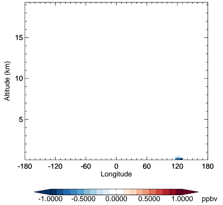
v11-02e-Run1 - v11-02e-Run0 HNO 2 - Diff along 42N for Jan
