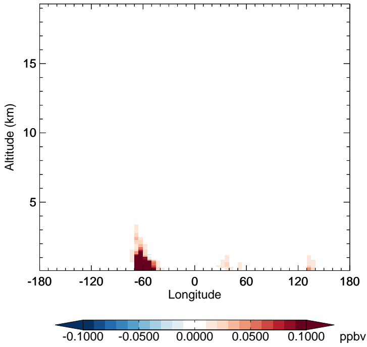
v11-02e-Run1 - v11-02e-Run0 MTPA - Diff along 15S for Jan
