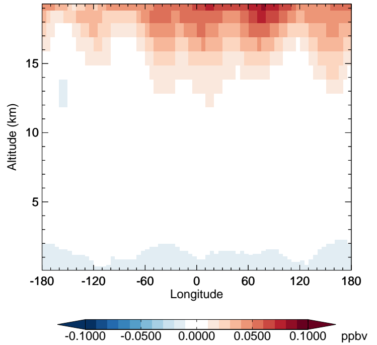
v11-02e-Run1 - v11-02d-Run1 CFC12 - Diff along 42N for Jan
