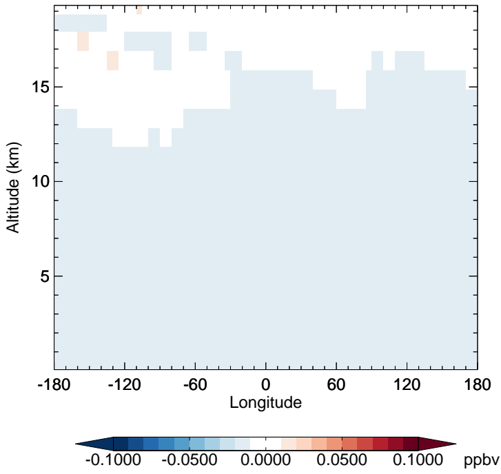
v11-02e-Run1 - v11-02e-Run0 CFC12 - Diff along 15S for Jan
