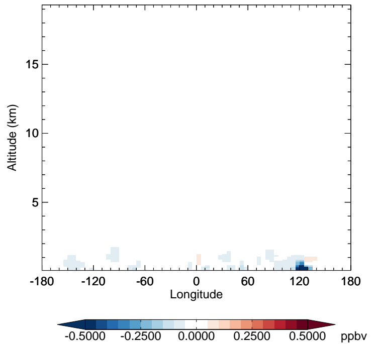
v11-02e-Run1 - v11-02d-Run1 CH 2 O - Diff along 42N for Jan
