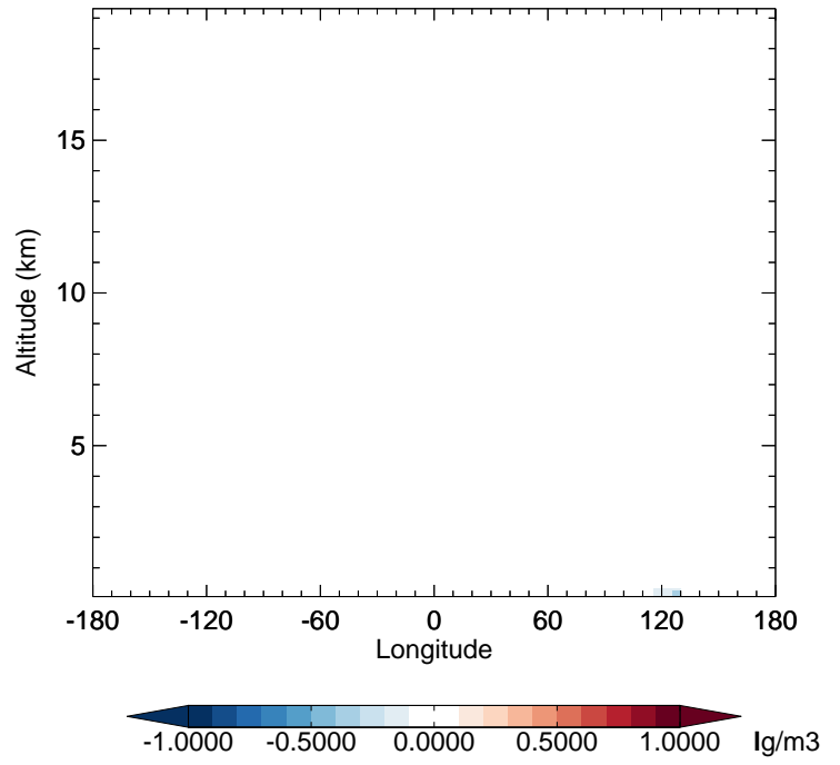
v11-02e-Run1 - v11-02e-Run0 BCPO - Diff along 42N for Jan
