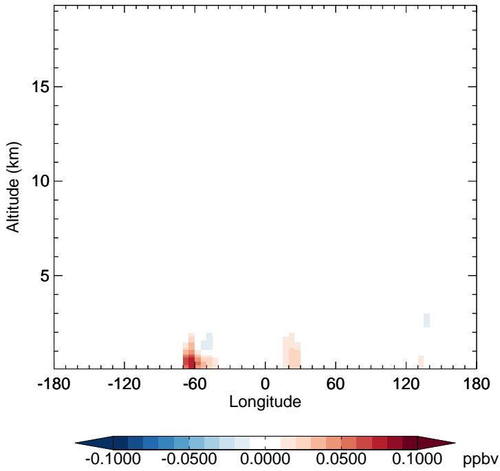
v11-02e-Run1 - v11-02d-Run1 TSOA0 - Diff along 15S for Jan
