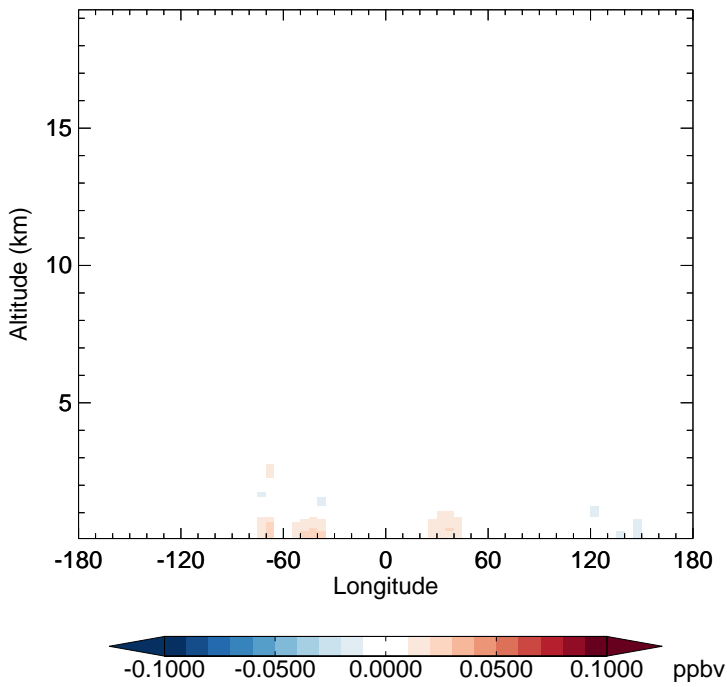
v11-02e-Run1 - v11-02d-Run1 TOLU - Diff along 15S for Jan
