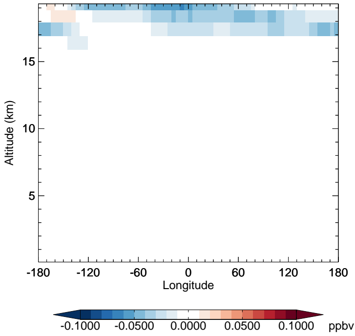
v11-02e-Run1 - v11-02e-Run0 CINO3 - Diff along 15S for Jan
