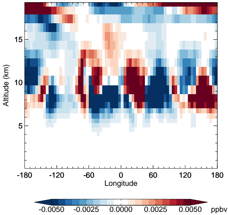
v11-02e-Run1 - v11-02d-Run1 HNO 4 - Diff along 15S for Jan
