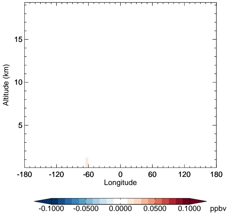
v11-02e-Run1 - v11-02e-Run0 TSOA3 - Diff along 15S for Jan
