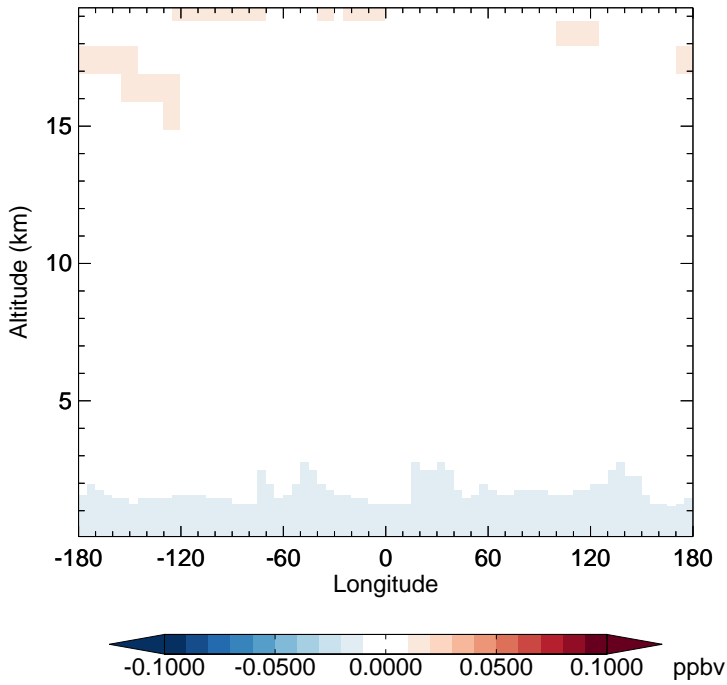
v11-02e-Run1 - v11-02d-Run1 CFC12 - Diff along 15S for Jan
