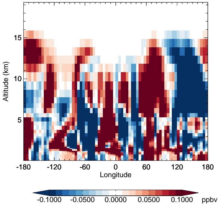
v11-02e-Run1 - v11-02d-Run1 H2O2 - Diff along 15S for Jan
