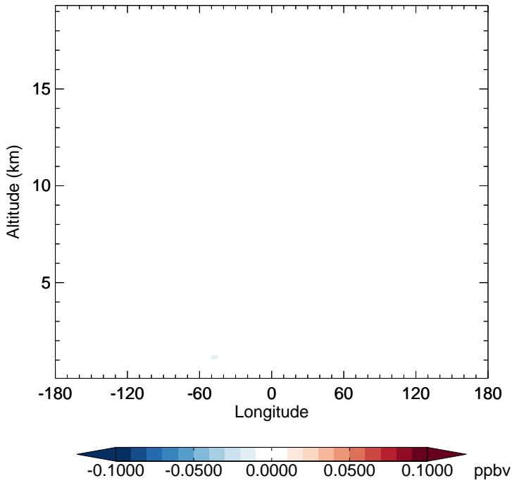
v11-02e-Run1 - v11-02d-Run1 MONITA - Diff along 15S for Jan
