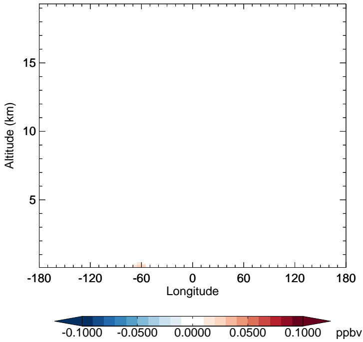
v11-02e-Run1 - v11-02e-Run0 MTPO - Diff along 15S for Jan
