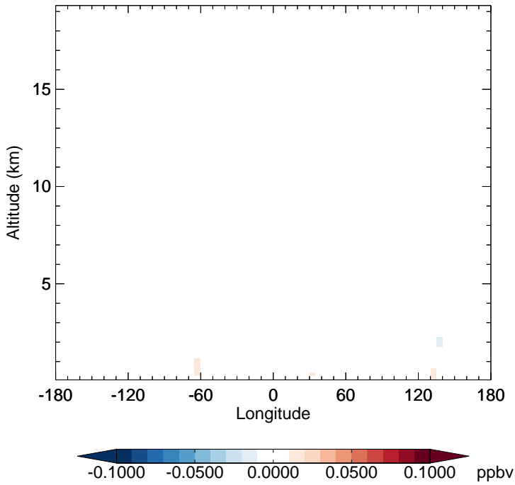
v11-02e-Run1 - v11-02d-Run1 GLYX - Diff along 15S for Jan
