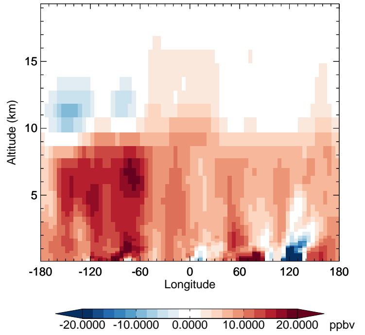
v11-02e-Run1 - v11-02e-Run0 CO - Diff along 42N for Jan
