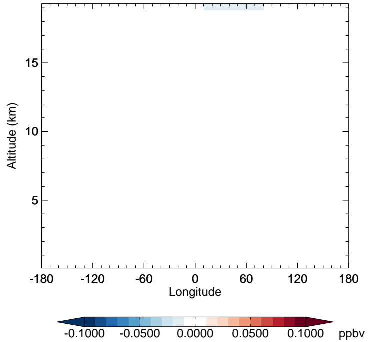
v11-02e-Run1 - v11-02d-Run1 HOCl - Diff along 42N for Jan
