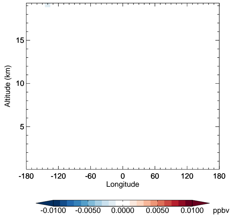
v11-02e-Run1 - v11-02d-Run1 CH3Br - Diff along 42N for Jan
