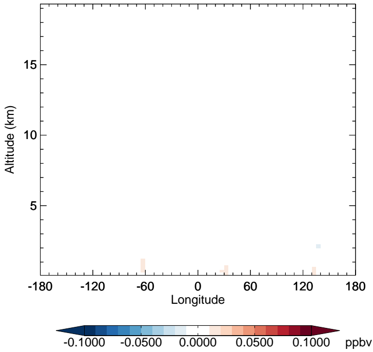
v11-02e-Run1 - v11-02e-Run0 GLYX - Diff along 15S for Jan
