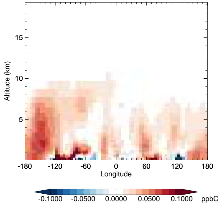
v11-02e-Run1 - v11-02e-Run0 MEK - Diff along 42N for Jan
