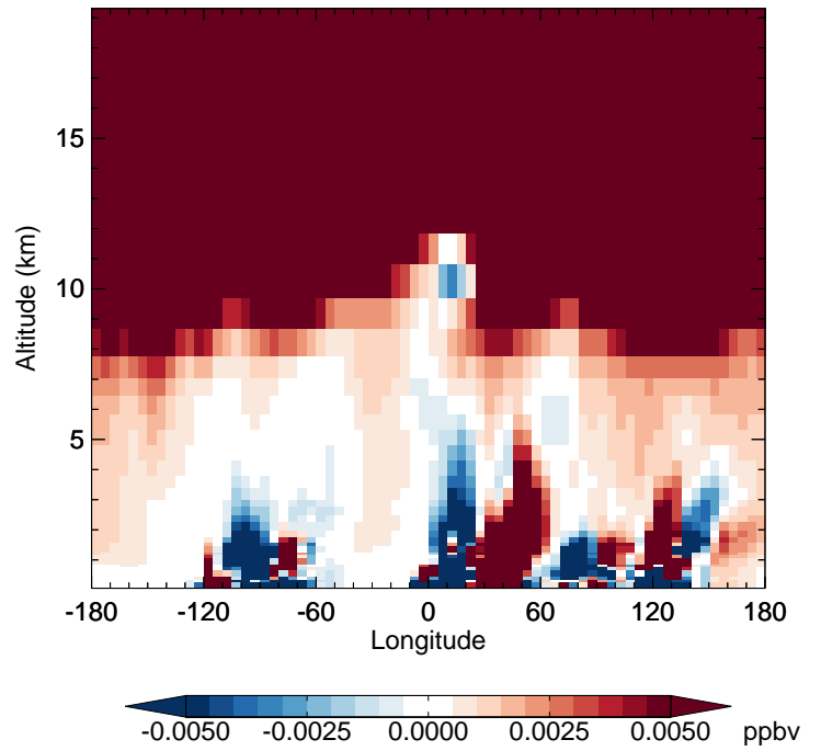
v11-02e-Run1 - v11-02d-Run1 N2O5 - Diff along 42N for Jan
