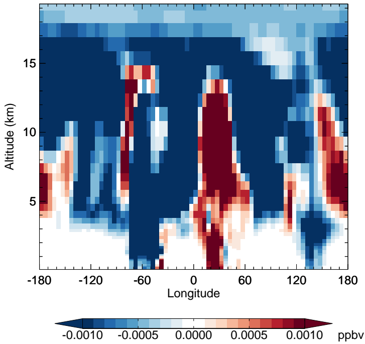
v11-02e-Run1 - v11-02d-Run1 PPN - Diff along 15S for Jan
