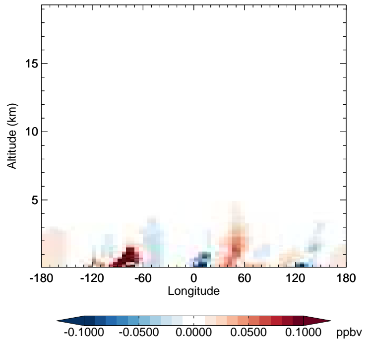
v11-02e-Run1 - v11-02d-Run1 EOH - Diff along 42N for Jan
