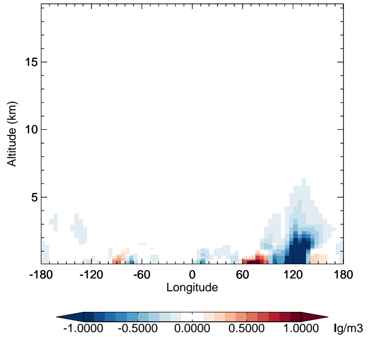
v11-02e-Run1 - v11-02d-Run1 SOAS - Diff along 42N for Jan
