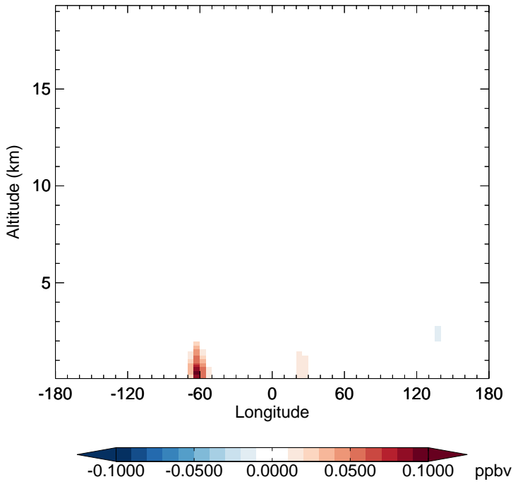
v11-02e-Run1 - v11-02e-Run0 TSOA2 - Diff along 15S for Jan
