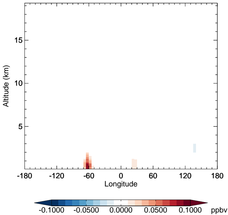
v11-02e-Run1 - v11-02d-Run1 TSOA2 - Diff along 15S for Jan
