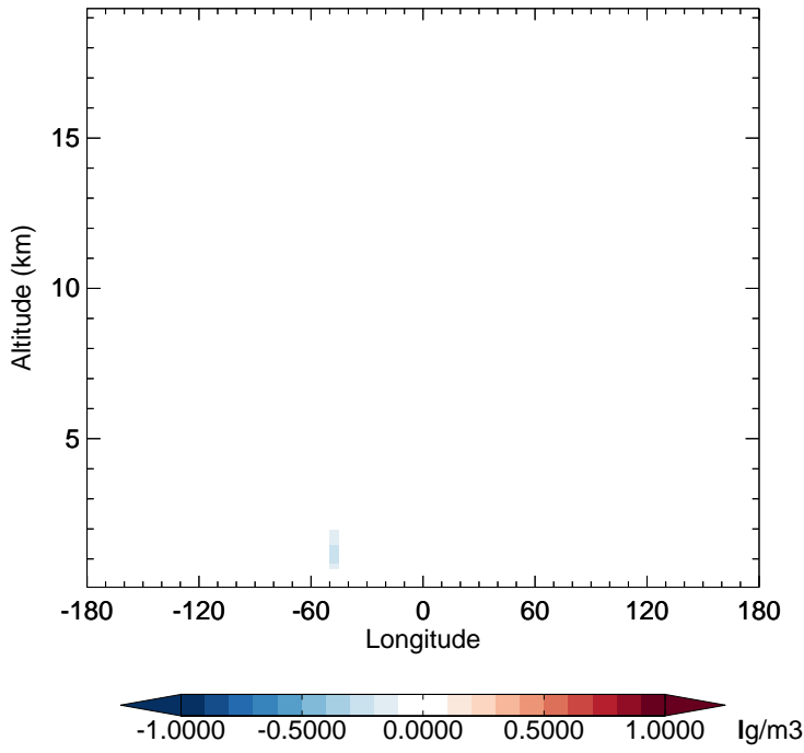
v11-02e-Run1 - v11-02e-Run0 NH3 - Diff along 15S for Jan
