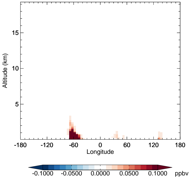
v11-02e-Run1 - v11-02d-Run1 MTPA - Diff along 15S for Jan
