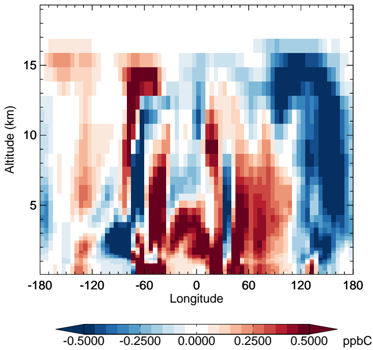
v11-02e-Run1 - v11-02d-Run1 ACET - Diff along 15S for Jan
