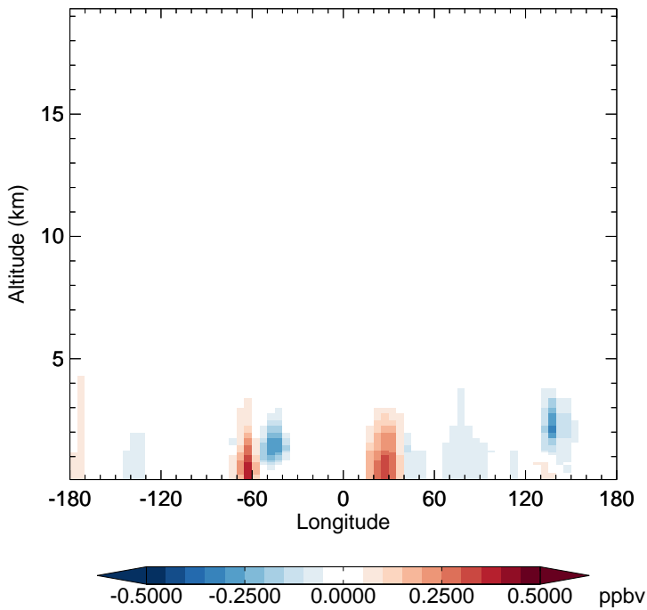
v11-02e-Run1 - v11-02d-Run1 CH 2 O - Diff along 15S for Jan
