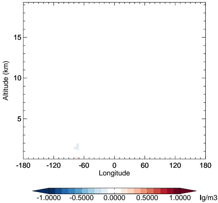
v11-02e-Run1 - v11-02d-Run1 NH4 - Diff along 15S for Jan
