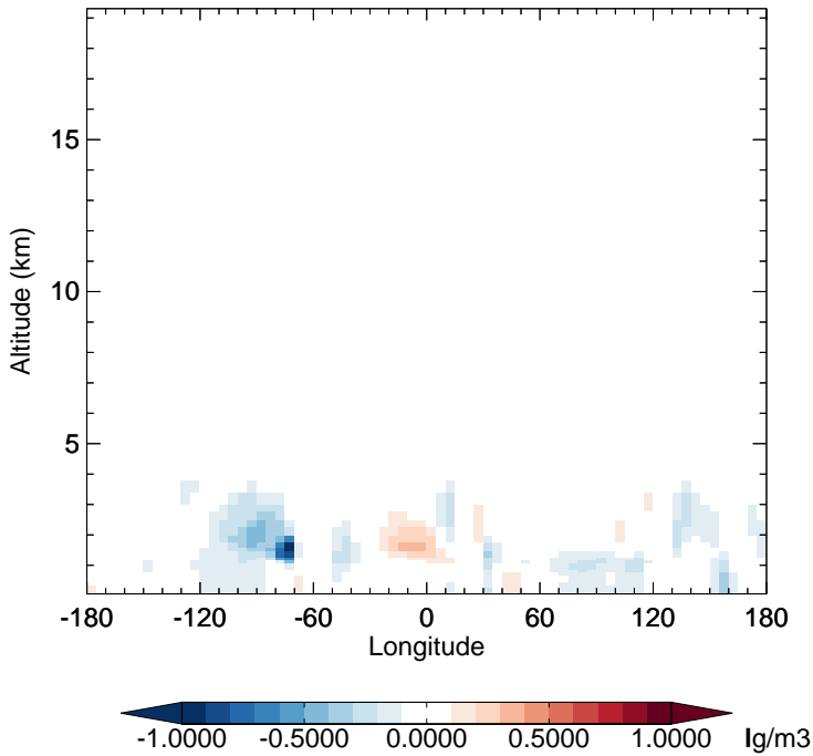
v11-02e-Run1 - v11-02d-Run1 SO4 - Diff along 15S for Jan
