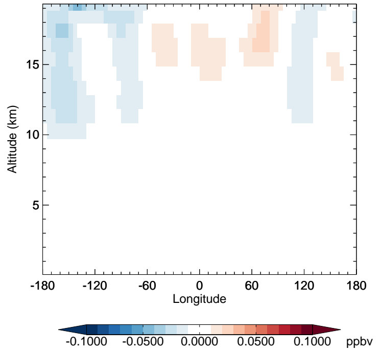
v11-02e-Run1 - v11-02e-Run0 CH3Cl - Diff along 42N for Jan
