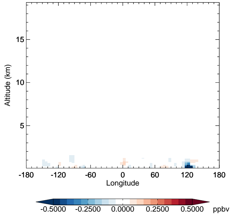
v11-02e-Run1 - v11-02e-Run0 CH 2 O - Diff along 42N for Jan
