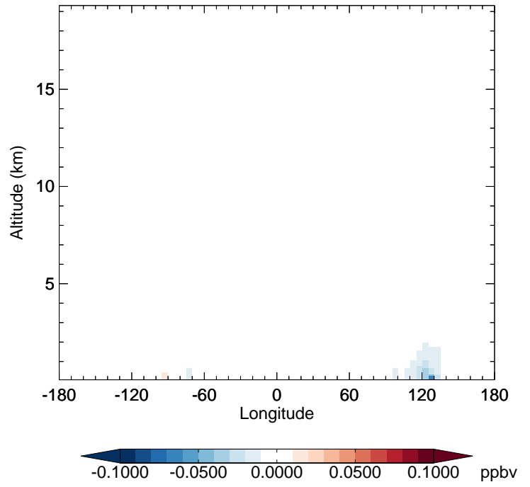
v11-02e-Run1 - v11-02e-Run0 INDIOL - Diff along 42N for Jan
