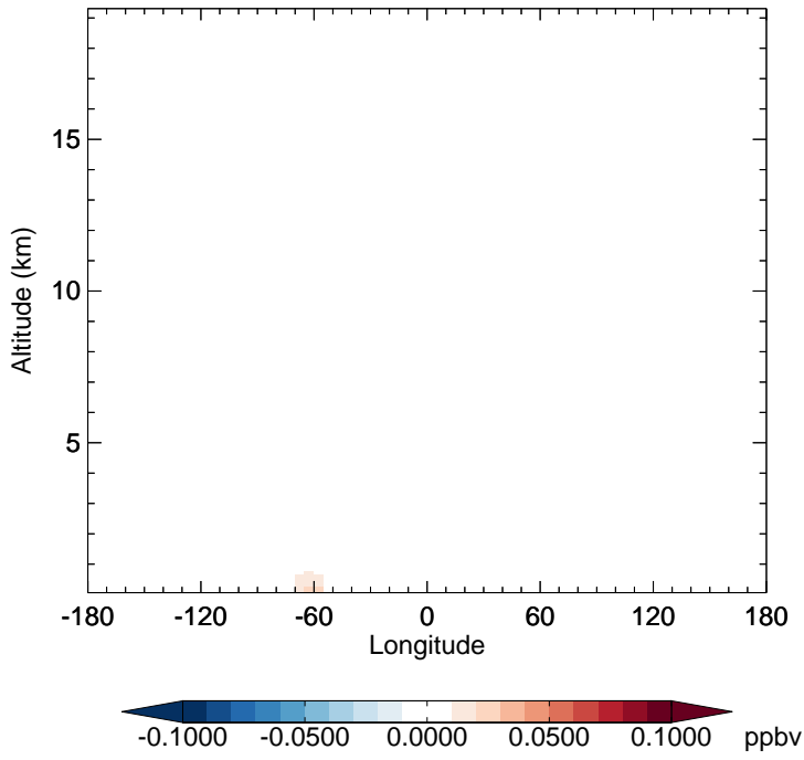
v11-02e-Run1 - v11-02e-Run0 LIMO - Diff along 15S for Jan
