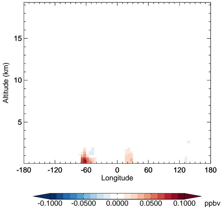
v11-02e-Run1 - v11-02e-Run0 TSOA0 - Diff along 15S for Jan
