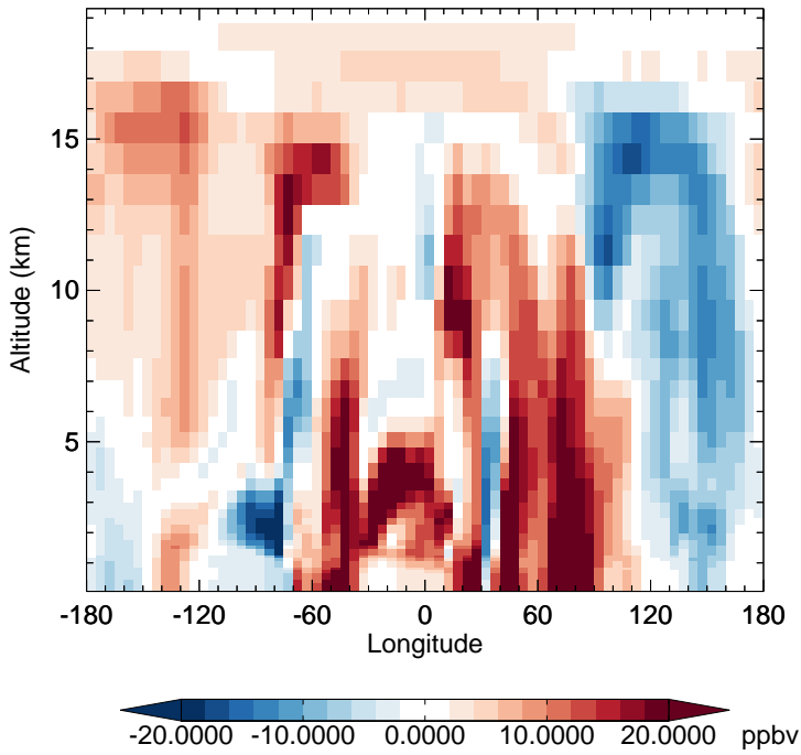
v11-02e-Run1 - v11-02d-Run1 CO - Diff along 15S for Jan
