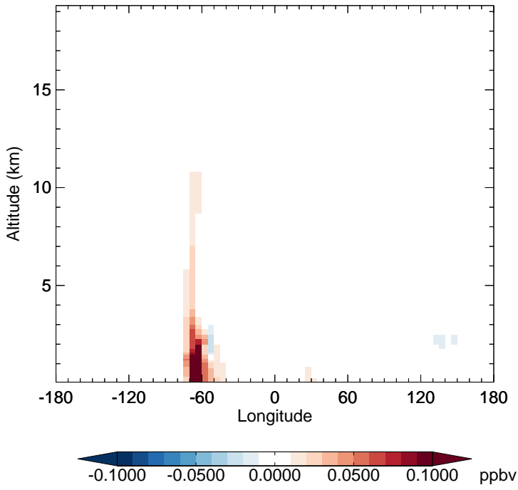
v11-02e-Run1 - v11-02e-Run0 IPMN - Diff along 15S for Oct
