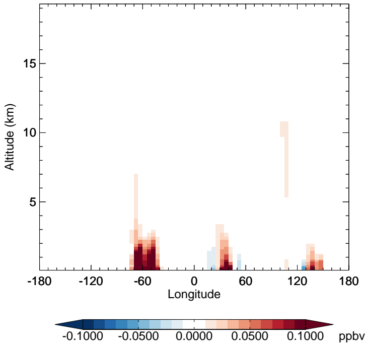
v11-02e-Run1 - v11-02d-Run1 TOLU - Diff along 15S for Oct
