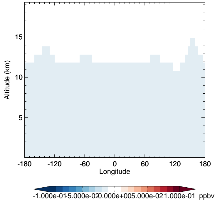
v11-02e-Run1 - v11-02e-Run0 HCFC22 - Diff along 42N for Oct
