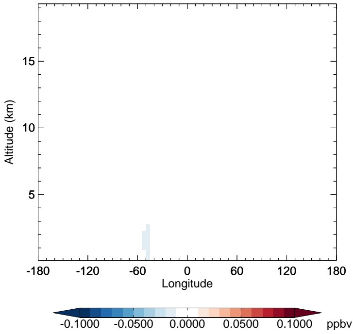
v11-02e-Run1 - v11-02e-Run0 MONITA - Diff along 15S for Oct
