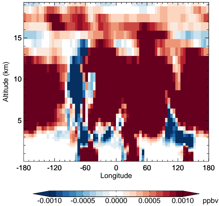
v11-02e-Run1 - v11-02d-Run1 PPN - Diff along 15S for Oct
