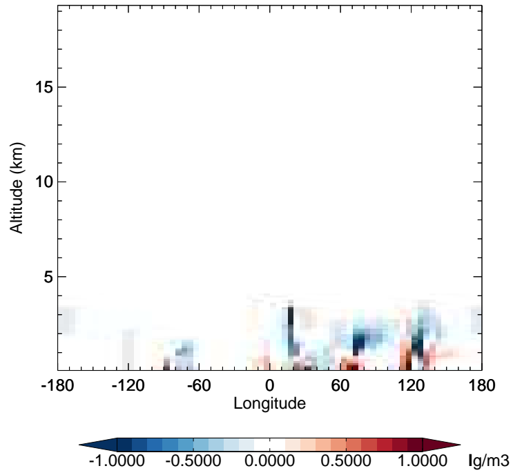
v11-02e-Run1 - v11-02e-Run0 SO 2 - Diff along 42N for Oct
