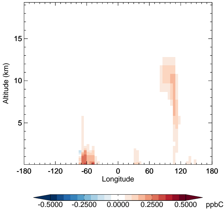
v11-02e-Run1 - v11-02d-Run1 ALK4 - Diff along 15S for Oct
