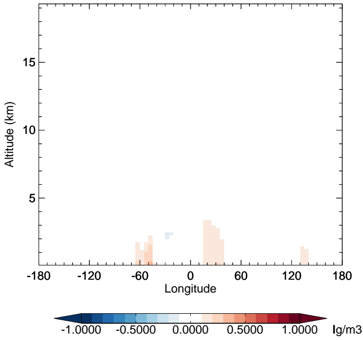
v11-02e-Run1 - v11-02e-Run0 BCPI - Diff along 15S for Oct
