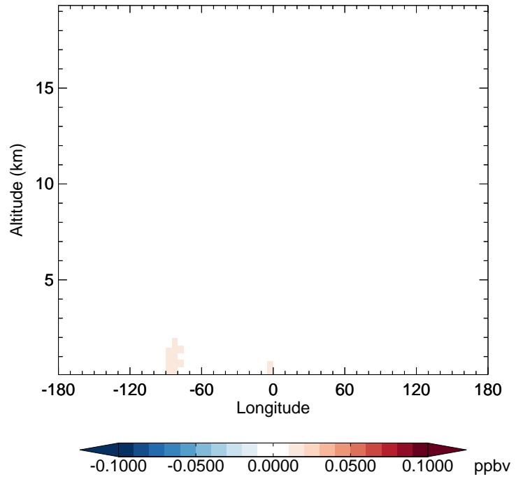
v11-02e-Run1 - v11-02e-Run0 IONITA - Diff along 42N for Oct
