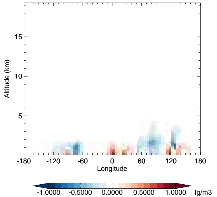
v11-02e-Run1 - v11-02d-Run1 NH4 - Diff along 42N for Oct
