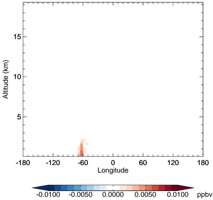
v11-02e-Run1 - v11-02e-Run0 MOBA - Diff along 15S for Oct
