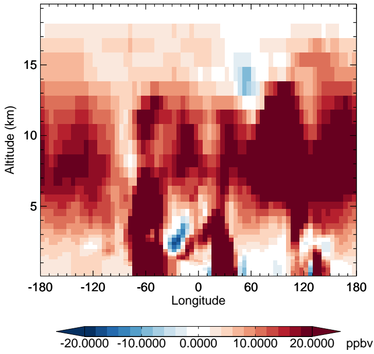
v11-02e-Run1 - v11-02e-Run0 CO - Diff along 15S for Oct
