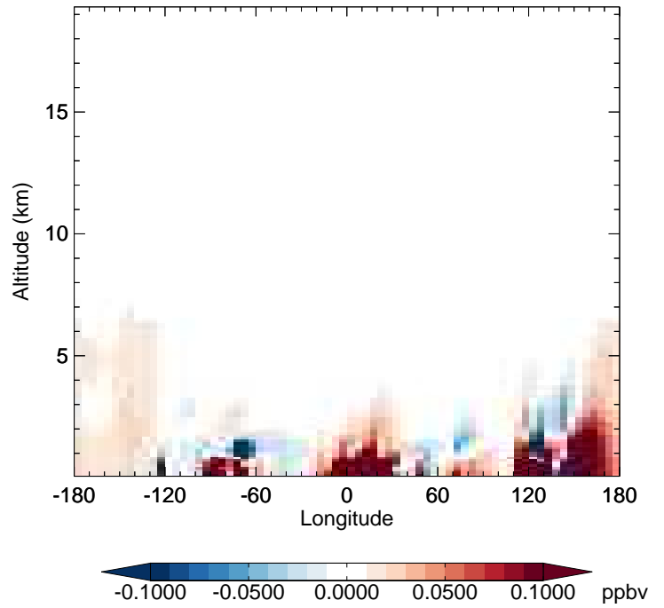
v11-02e-Run1 - v11-02d-Run1 TOLU - Diff along 42N for Oct
