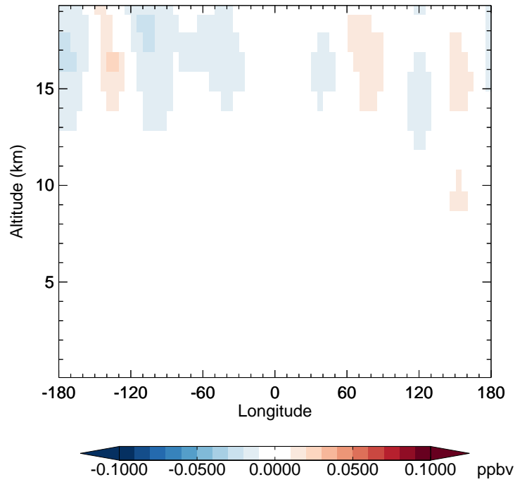
v11-02e-Run1 - v11-02d-Run1 MPN - Diff along 42N for Oct
