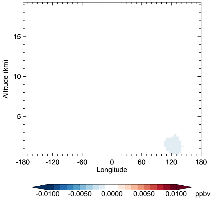
v11-02e-Run1 - v11-02d-Run1 HOBr - Diff along 15S for Oct
