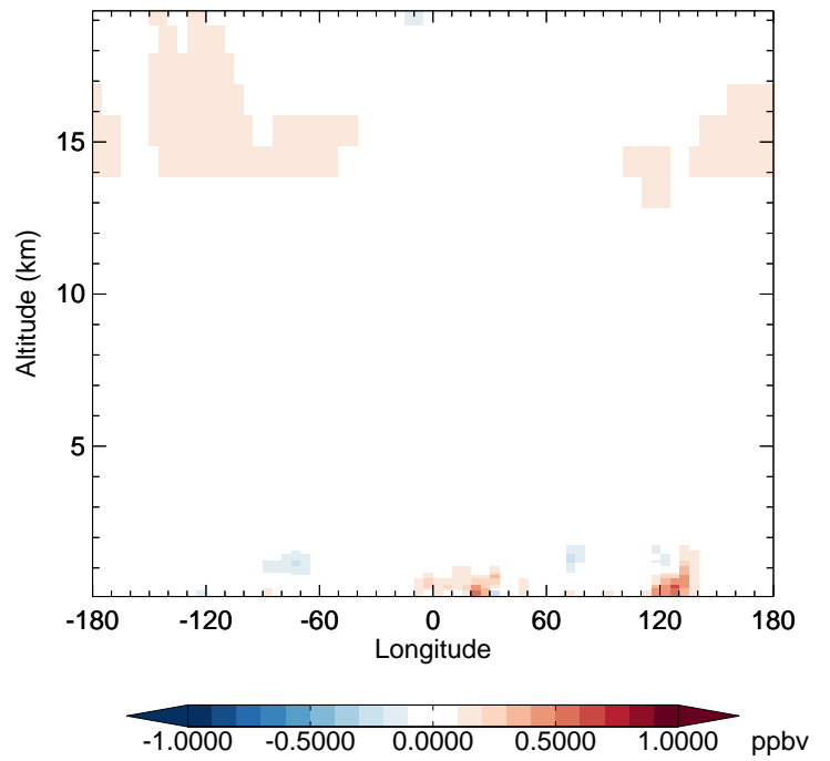
v11-02e-Run1 - v11-02d-Run1 NO 2 - Diff along 42N for Oct
