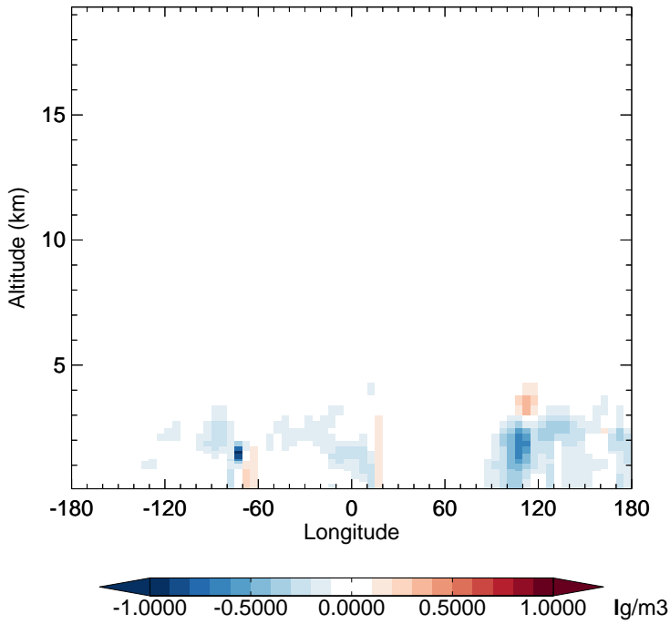
v11-02e-Run1 - v11-02d-Run1 SO4 - Diff along 15S for Oct
