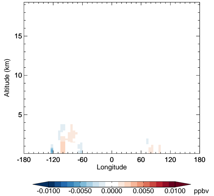
v11-02e-Run1 - v11-02d-Run1 R4N2 - Diff along 42N for Oct
