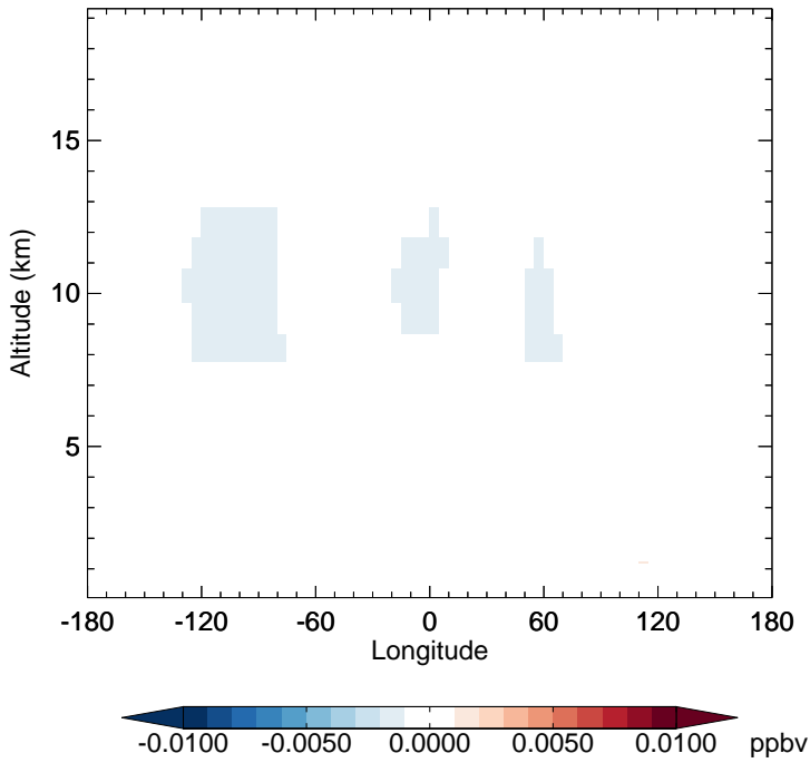
v11-02e-Run1 - v11-02d-Run1 HBr - Diff along 15S for Oct
