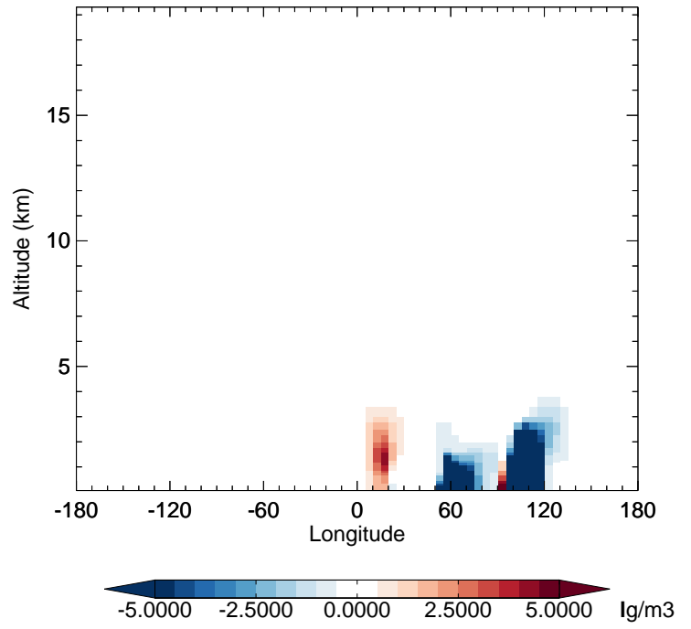
v11-02e-Run1 - v11-02e-Run0 DST4 - Diff along 42N for Oct
