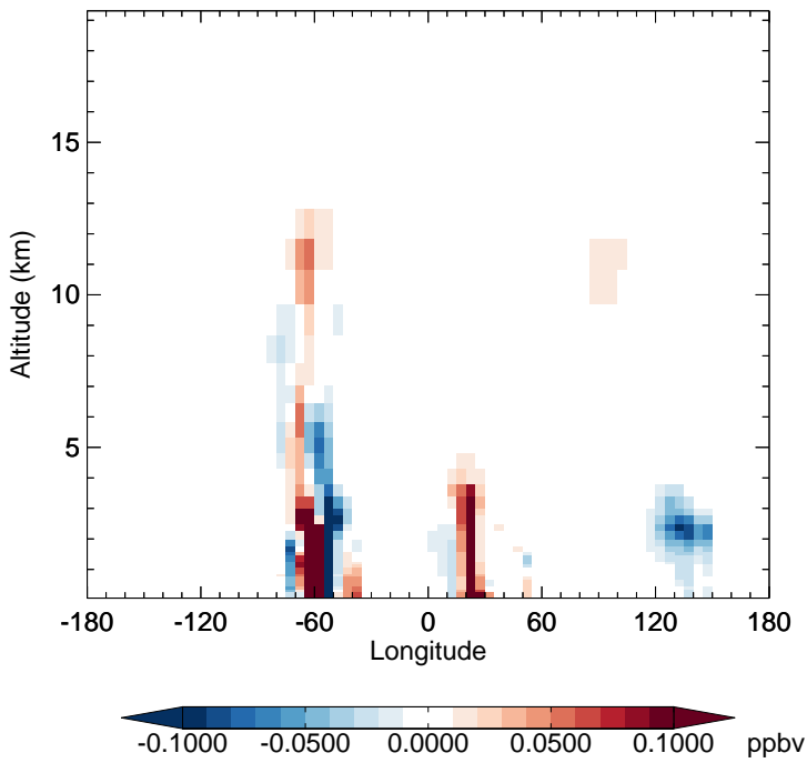
v11-02e-Run1 - v11-02d-Run1 EOH - Diff along 15S for Oct
