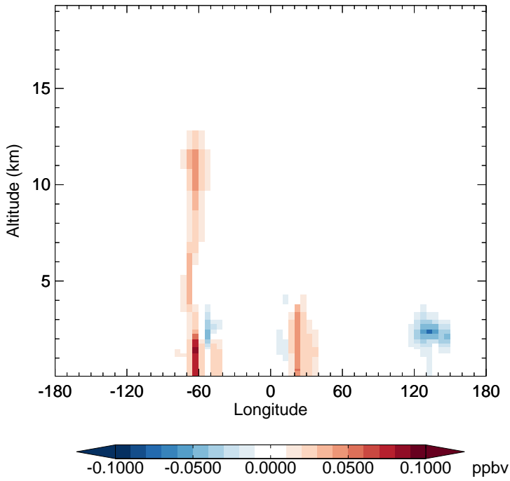
v11-02e-Run1 - v11-02e-Run0 IMAE - Diff along 15S for Oct
