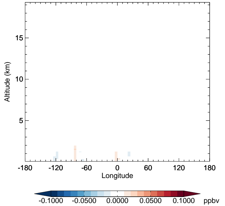
v11-02e-Run1 - v11-02d-Run1 TSOG3 - Diff along 42N for Oct
