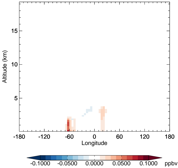
v11-02e-Run1 - v11-02e-Run0 TSOA3 - Diff along 15S for Oct
