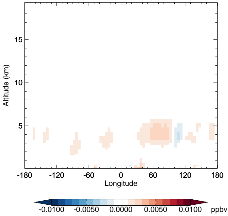
v11-02e-Run1 - v11-02e-Run0 NO3 - Diff along 15S for Oct
