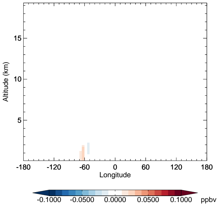
v11-02e-Run1 - v11-02d-Run1 TSOA1 - Diff along 15S for Oct
