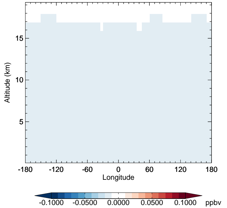
v11-02e-Run1 - v11-02d-Run1 HCFC22 - Diff along 42N for Oct
