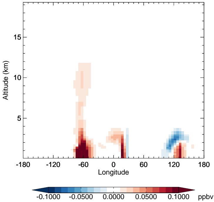
v11-02e-Run1 - v11-02d-Run1 SOAIE - Diff along 15S for Oct
