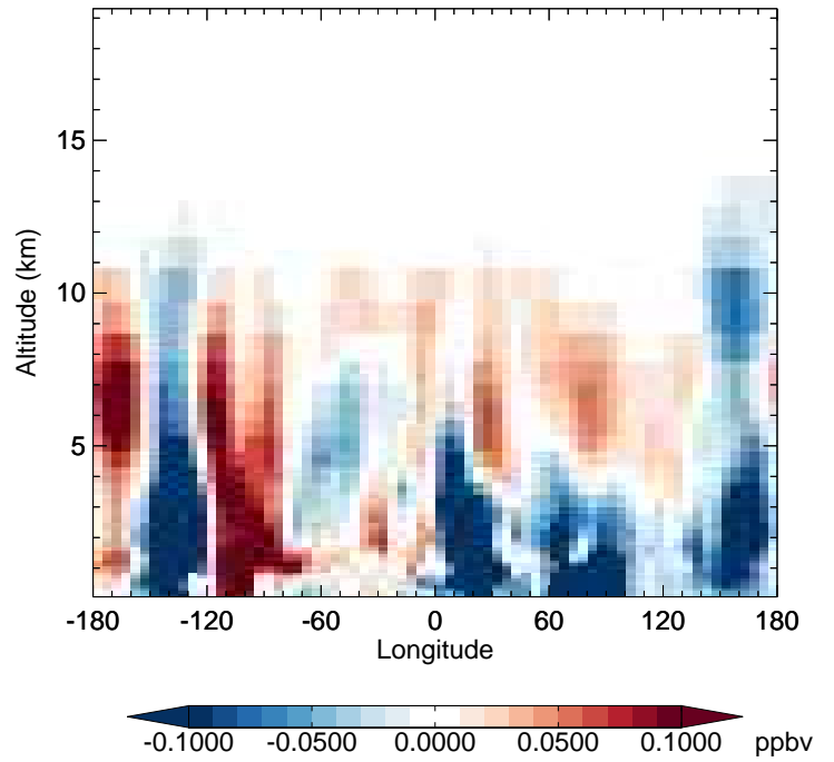
v11-02e-Run1 - v11-02d-Run1 H2O2 - Diff along 42N for Oct
