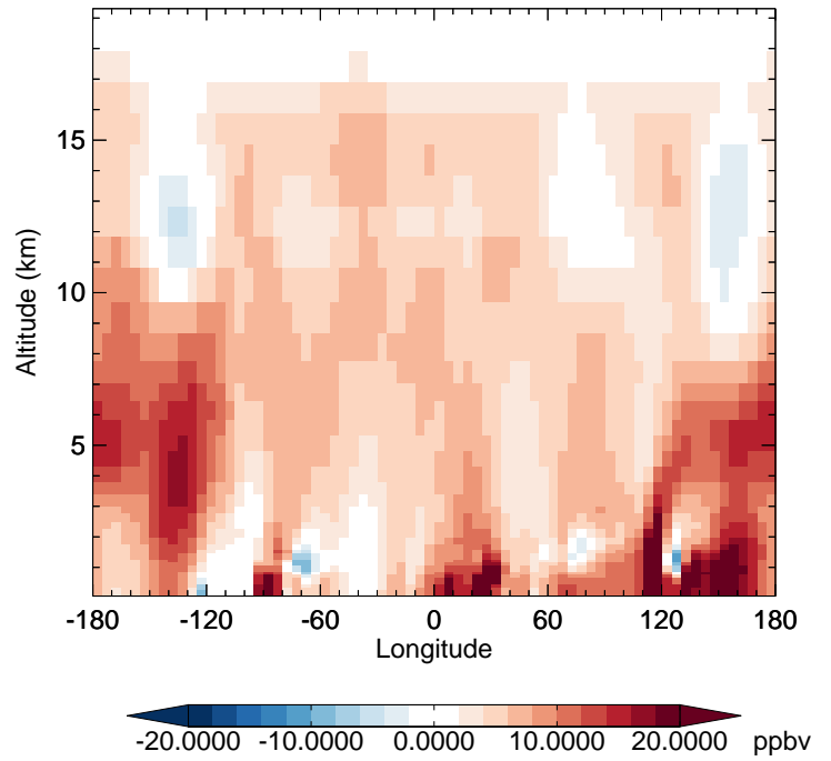
v11-02e-Run1 - v11-02d-Run1 CO - Diff along 42N for Oct
