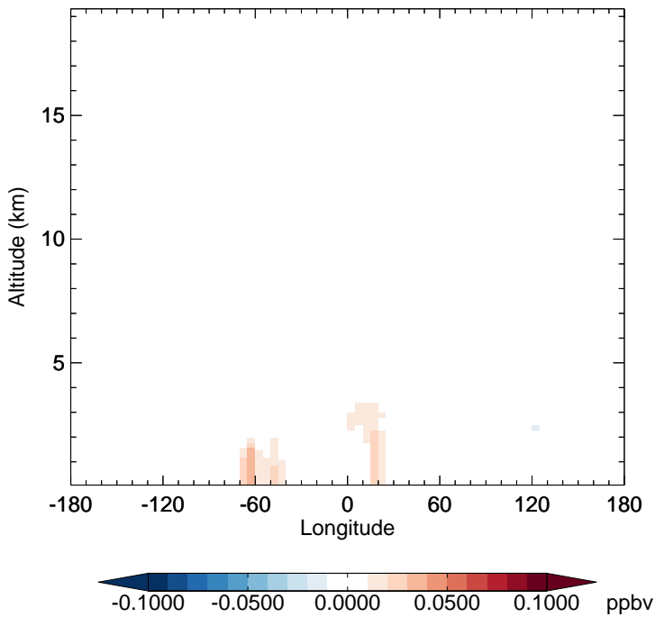
v11-02e-Run1 - v11-02d-Run1 SOAGX - Diff along 15S for Oct
