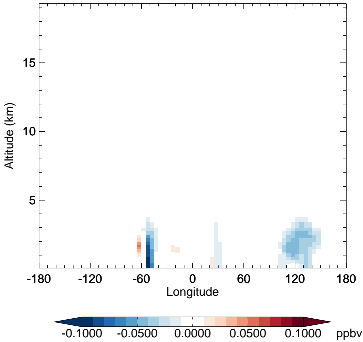
v11-02e-Run1 - v11-02d-Run1 TSOG2 - Diff along 15S for Oct
