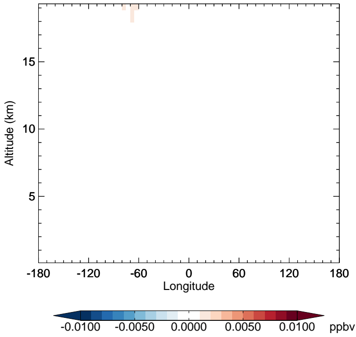
v11-02e-Run1 - v11-02e-Run0 CH3Br - Diff along 15S for Oct
