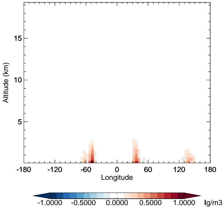
v11-02e-Run1 - v11-02e-Run0 OCPO - Diff along 15S for Oct
