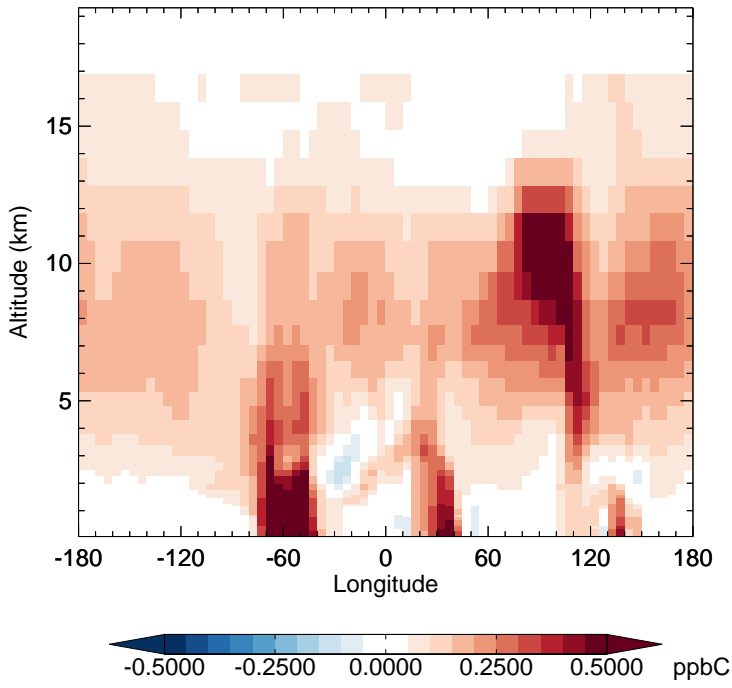
v11-02e-Run1 - v11-02e-Run0 C2H6 - Diff along 15S for Oct
