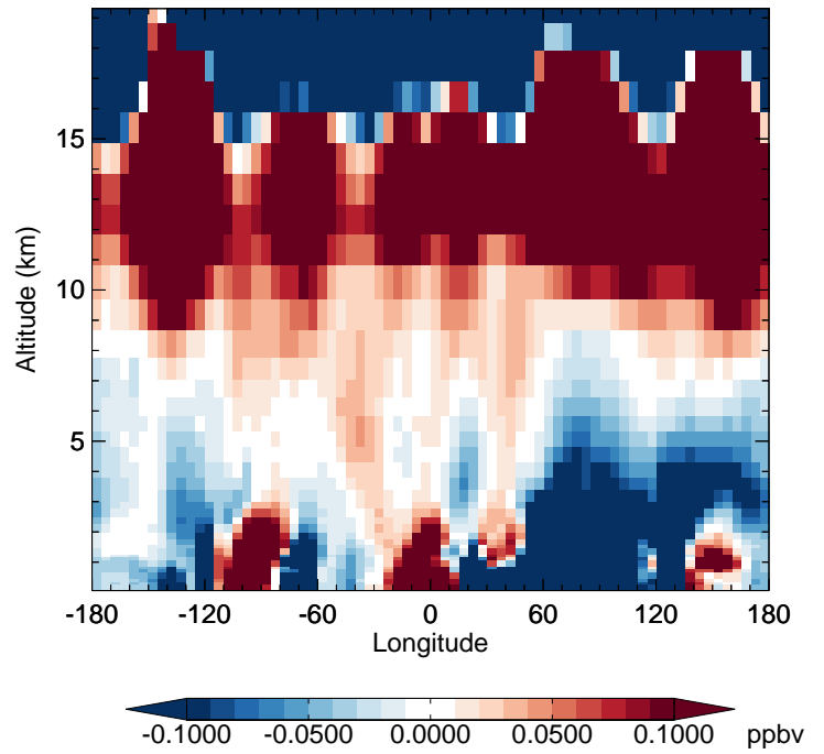
v11-02e-Run1 - v11-02d-Run1 HNO 3 - Diff along 42N for Oct
