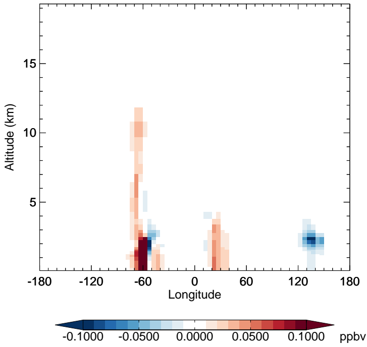
v11-02e-Run1 - v11-02e-Run0 GLYC - Diff along 15S for Oct
