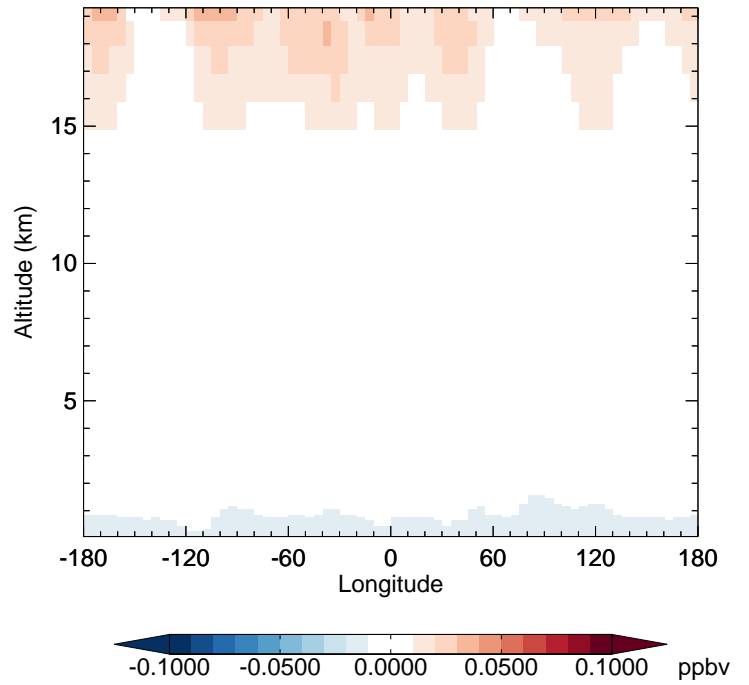
v11-02e-Run1 - v11-02d-Run1 CFC11 - Diff along 42N for Oct
