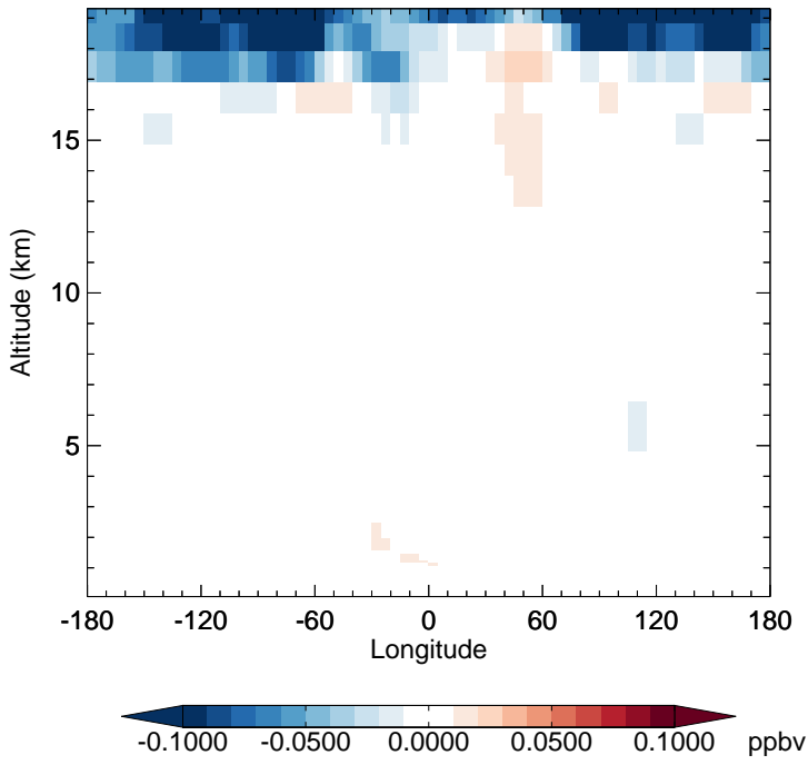
v11-02e-Run1 - v11-02e-Run0 HCl - Diff along 15S for Oct
