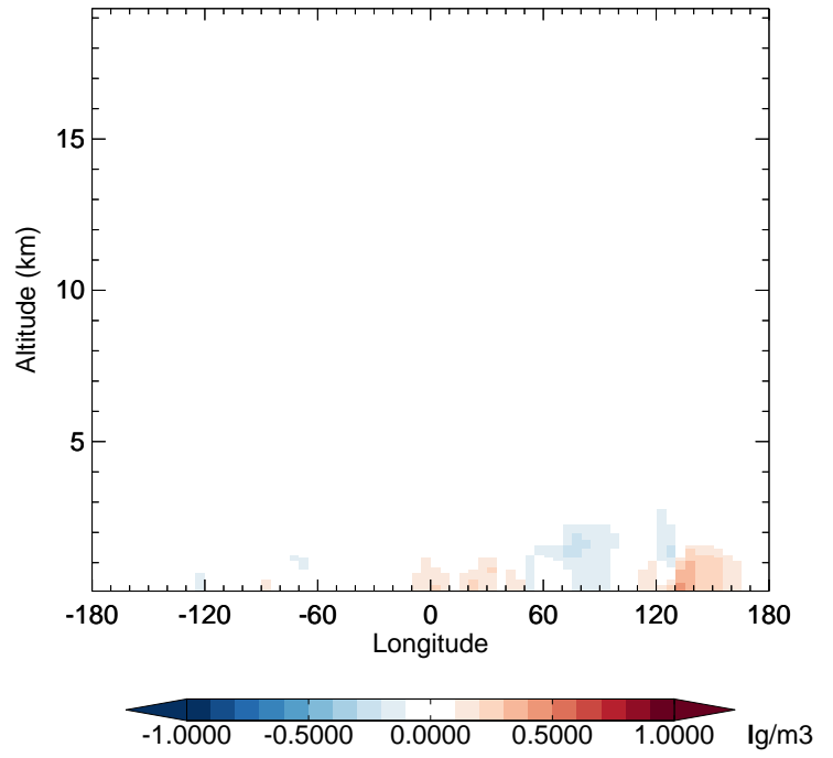
v11-02e-Run1 - v11-02e-Run0 OCPI - Diff along 42N for Oct
