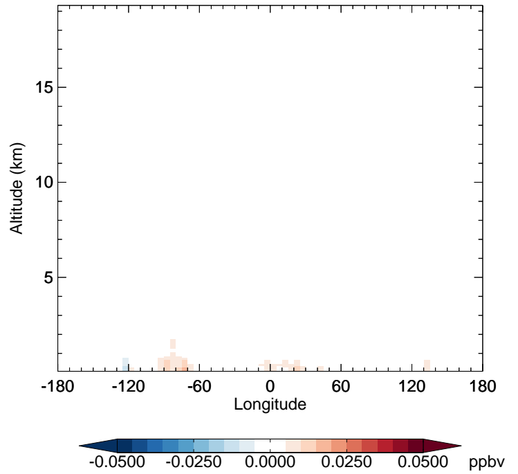
v11-02e-Run1 - v11-02d-Run1 RCHO - Diff along 42N for Oct
