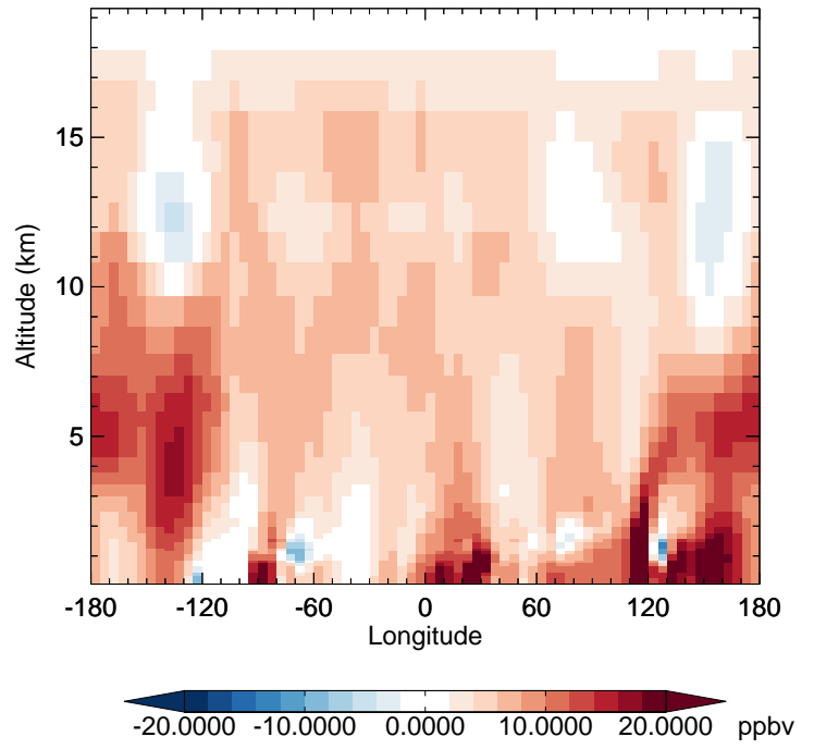
v11-02e-Run1 - v11-02e-Run0 CO - Diff along 42N for Oct
