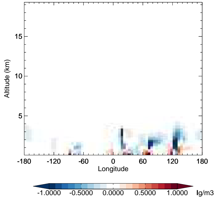
v11-02e-Run1 - v11-02d-Run1 SO 2 - Diff along 42N for Oct
