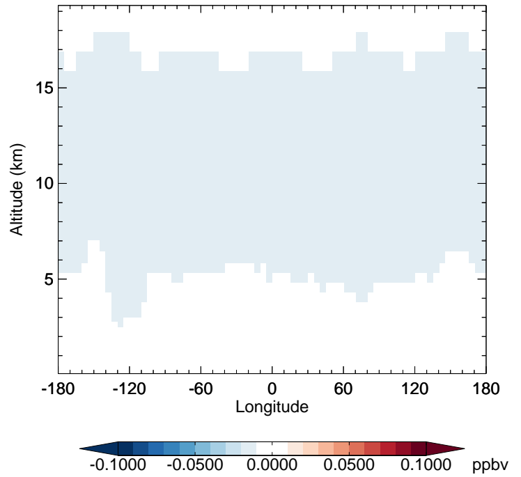
v11-02e-Run1 - v11-02d-Run1 HCFC141b - Diff along 42N for Oct
