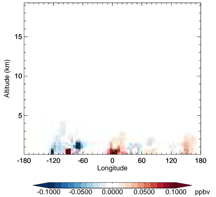
v11-02e-Run1 - v11-02d-Run1 EOH - Diff along 42N for Oct
