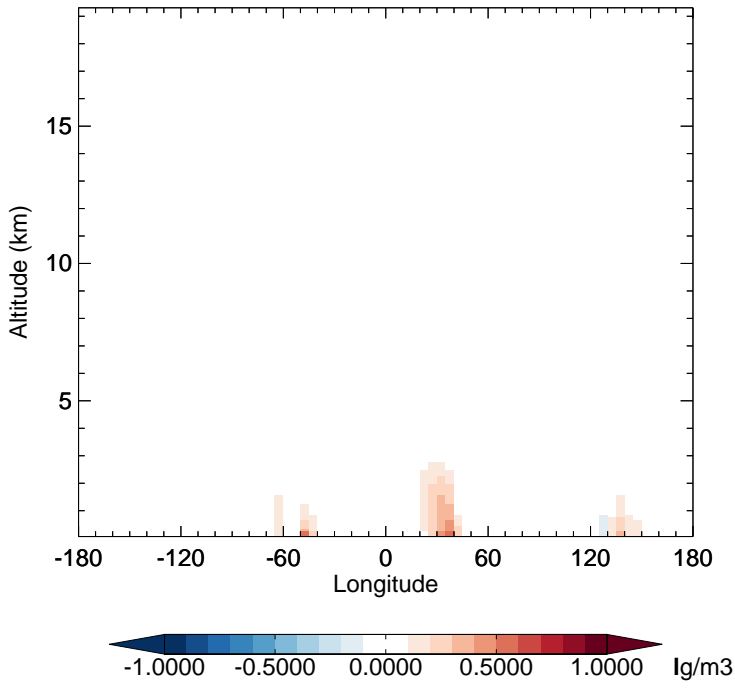
v11-02e-Run1 - v11-02e-Run0 NH3 - Diff along 15S for Oct
