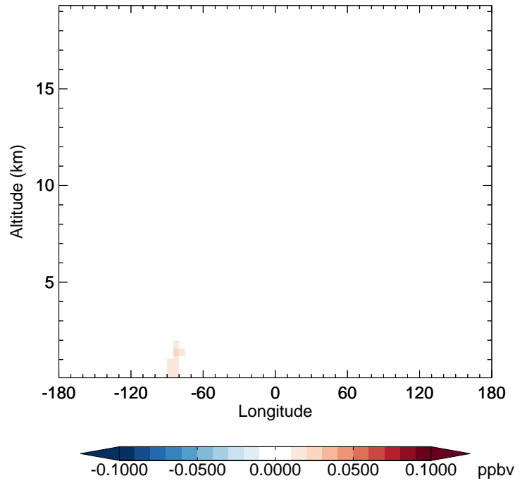
v11-02e-Run1 - v11-02e-Run0 IMAE - Diff along 42N for Oct
