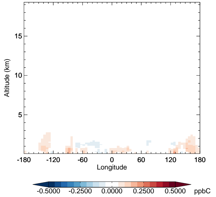
v11-02e-Run1 - v11-02e-Run0 ALD2 - Diff along 42N for Oct
