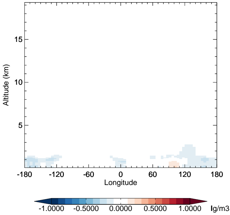
v11-02e-Run1 - v11-02e-Run0 SALA - Diff along 15S for Oct
