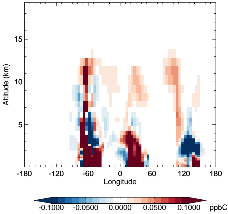
v11-02e-Run1 - v11-02e-Run0 MEK - Diff along 15S for Oct
