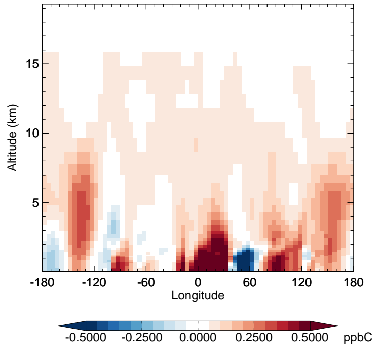
v11-02e-Run1 - v11-02e-Run0 C2H6 - Diff along 42N for Oct
