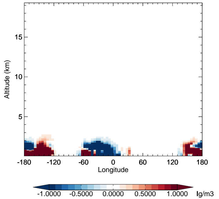
v11-02e-Run1 - v11-02d-Run1 SALC - Diff along 42N for Oct
