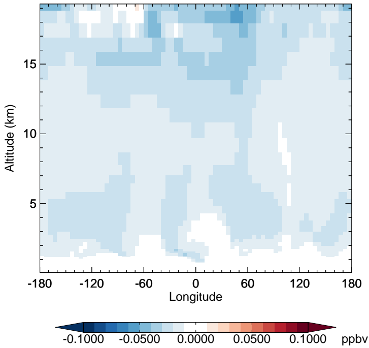
v11-02e-Run1 - v11-02d-Run1 CH3Cl - Diff along 15S for Oct
