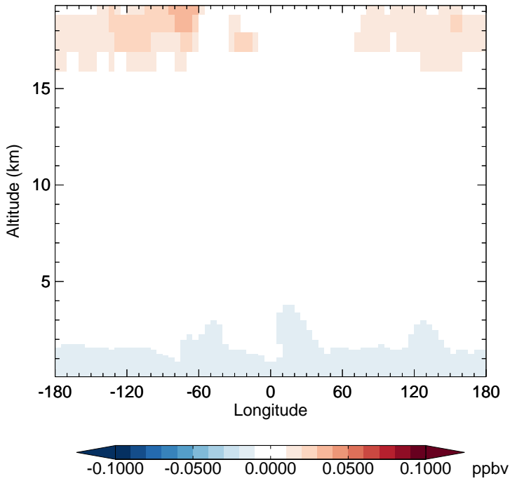
v11-02e-Run1 - v11-02d-Run1 CFC12 - Diff along 15S for Oct
