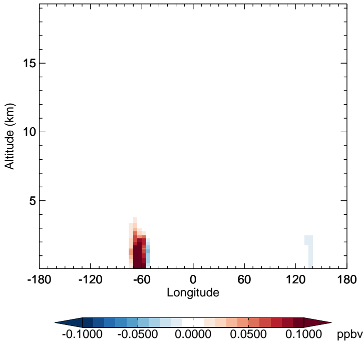
v11-02e-Run1 - v11-02d-Run1 HPALD - Diff along 15S for Oct
