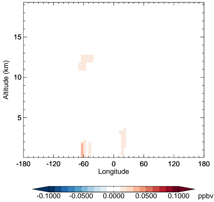
v11-02e-Run1 - v11-02e-Run0 ISOA3 - Diff along 15S for Oct
