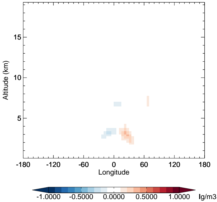
v11-02e-Run1 - v11-02d-Run1 NIT - Diff along 15S for Oct
