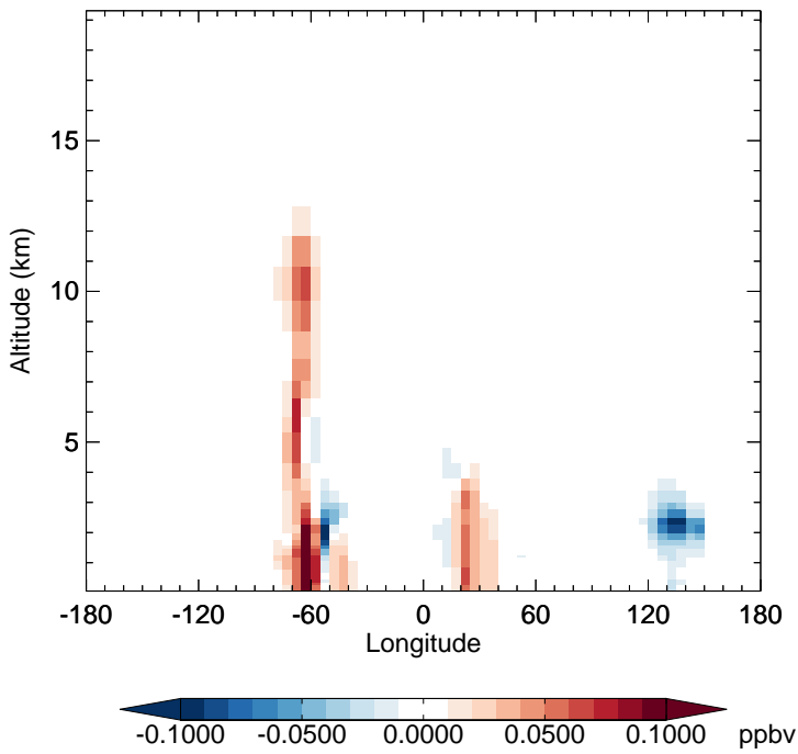
v11-02e-Run1 - v11-02d-Run1 HAC - Diff along 15S for Oct
