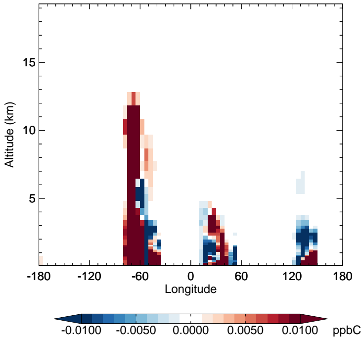
v11-02e-Run1 - v11-02d-Run1 PRPE - Diff along 15S for Oct
