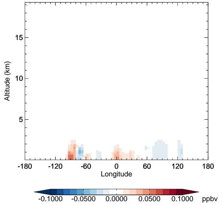
v11-02e-Run1 - v11-02e-Run0 INDIOL - Diff along 42N for Oct
