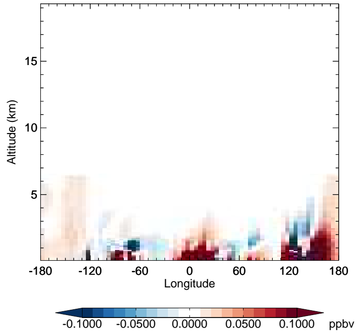
v11-02e-Run1 - v11-02e-Run0 TOLU - Diff along 42N for Oct
