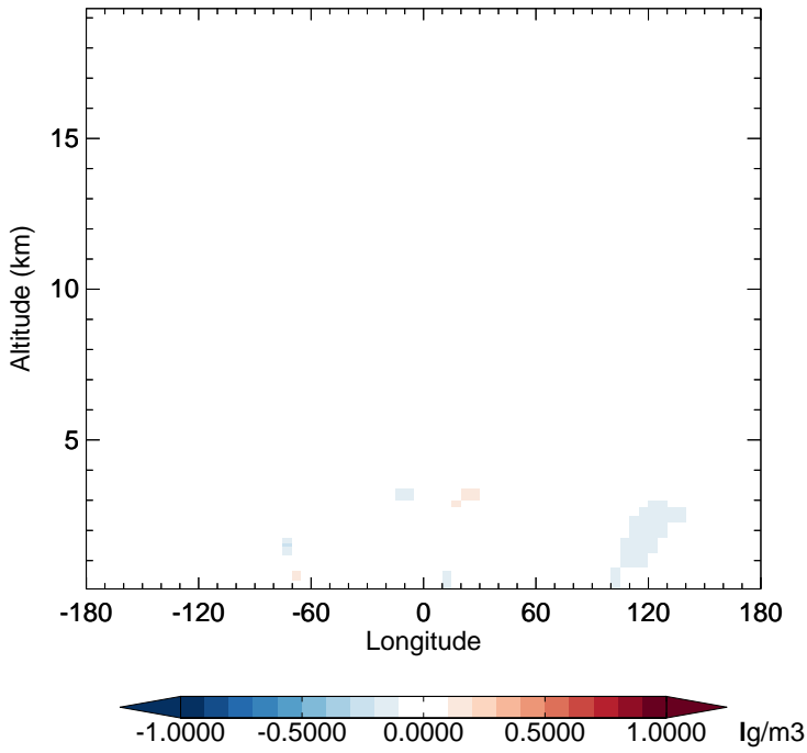
v11-02e-Run1 - v11-02e-Run0 NH4 - Diff along 15S for Oct
