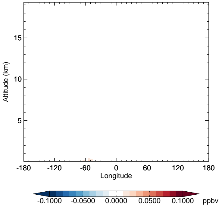
v11-02e-Run1 - v11-02e-Run0 ISN1 - Diff along 15S for Oct
