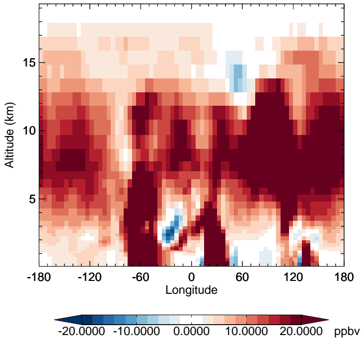
v11-02e-Run1 - v11-02d-Run1 CO - Diff along 15S for Oct
