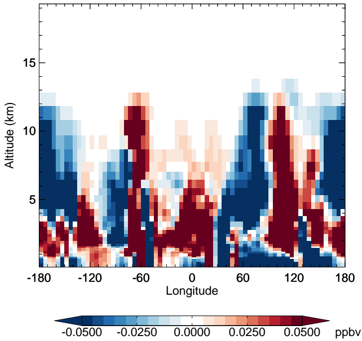
v11-02e-Run1 - v11-02d-Run1 MP - Diff along 15S for Oct
