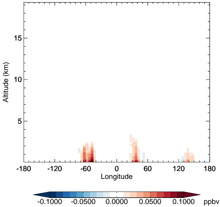
v11-02e-Run1 - v11-02d-Run1 SOAP - Diff along 15S for Oct
