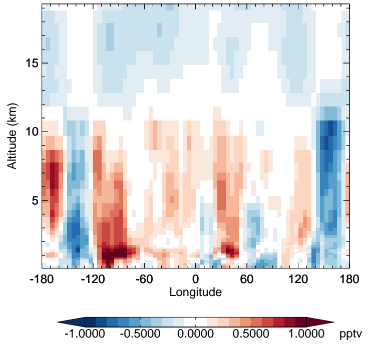
v11-02e-Run1 - v11-02e-Run0 HO2 - Diff along 42N for Oct
