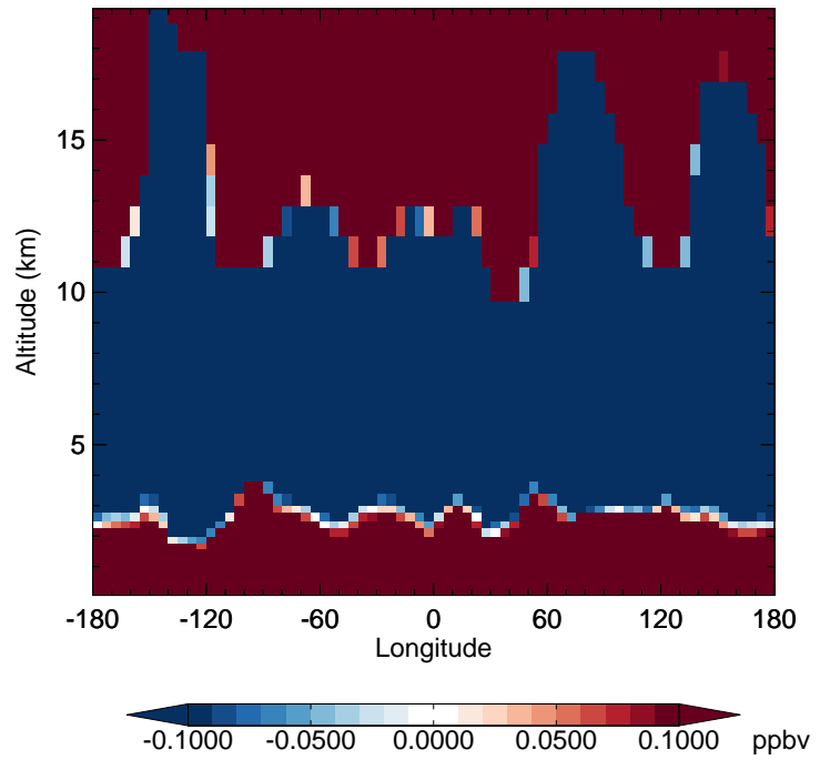
v11-02e-Run1 - v11-02d-Run1 N2O - Diff along 42N for Oct
