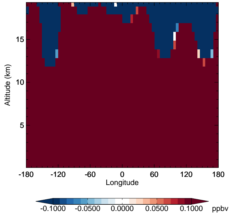
v11-02e-Run1 - v11-02e-Run0 N2O - Diff along 42N for Oct
