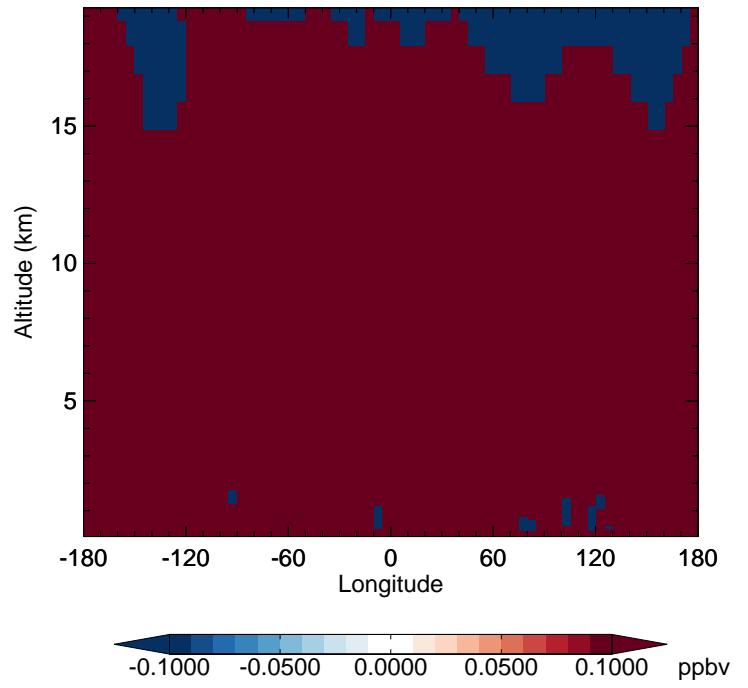
v11-02e-Run1 - v11-02e-Run0 CH4 - Diff along 42N for Oct
