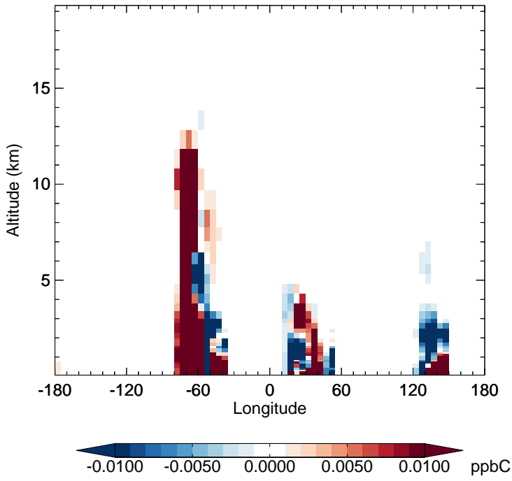
v11-02e-Run1 - v11-02e-Run0 PRPE - Diff along 15S for Oct
