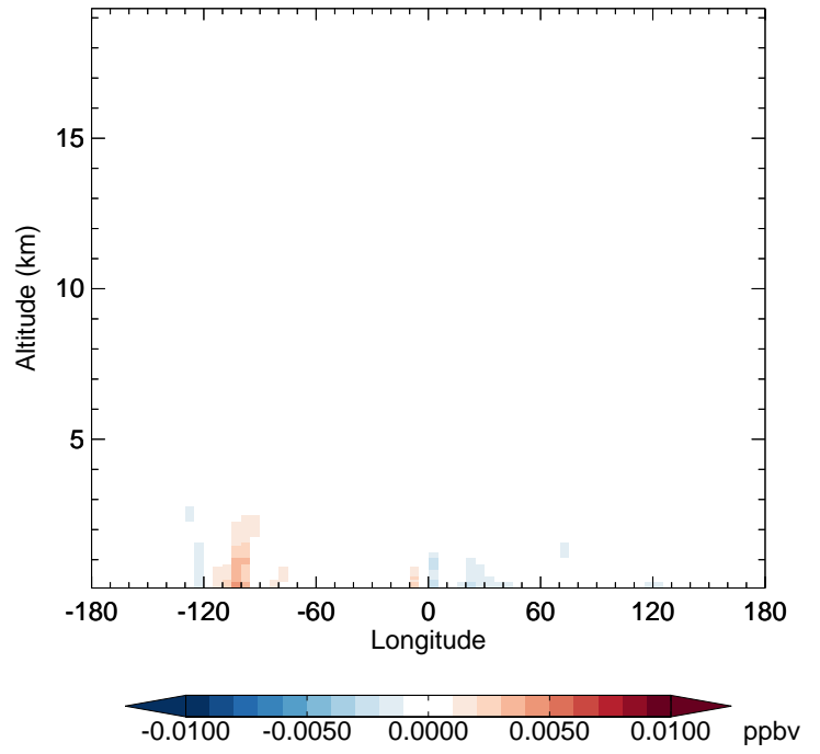
v11-02e-Run1 - v11-02e-Run0 NO3 - Diff along 42N for Oct
