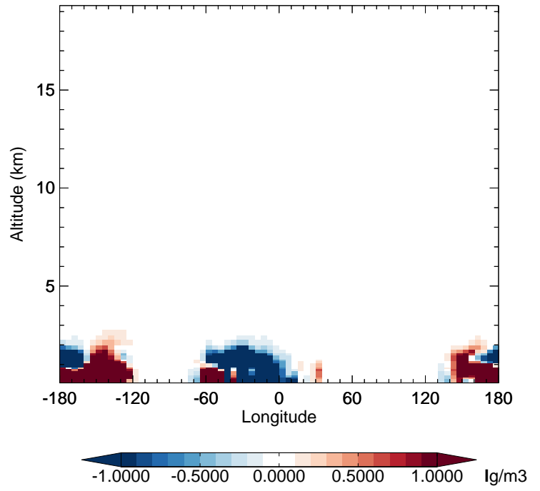
v11-02e-Run1 - v11-02e-Run0 SALC - Diff along 42N for Oct
