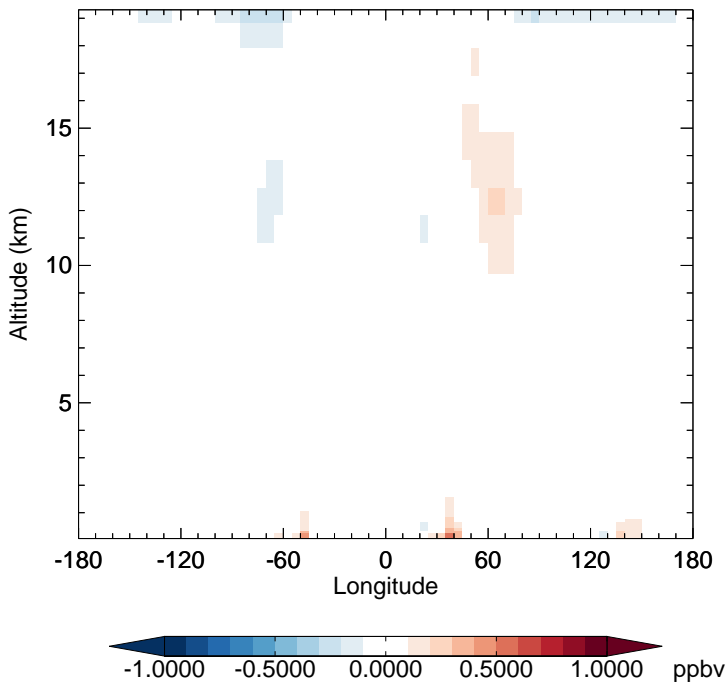
v11-02e-Run1 - v11-02e-Run0 NO 2 - Diff along 15S for Oct
