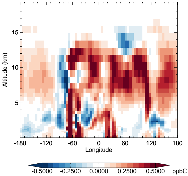
v11-02e-Run1 - v11-02e-Run0 ACET - Diff along 15S for Oct
