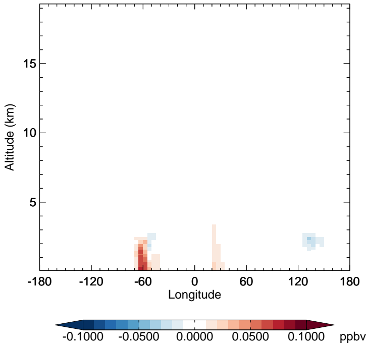
v11-02e-Run1 - v11-02e-Run0 MGLY - Diff along 15S for Oct
