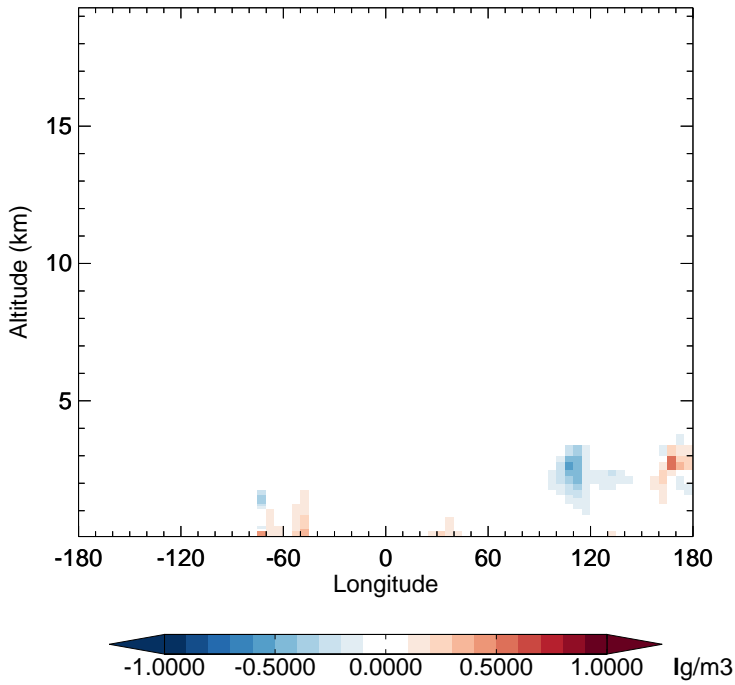
v11-02e-Run1 - v11-02d-Run1 SO 2 - Diff along 15S for Oct
