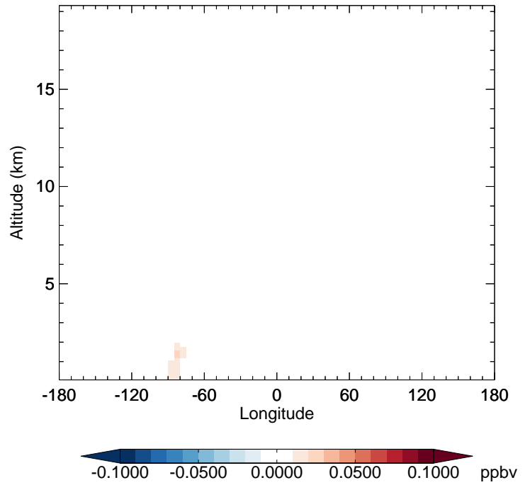
v11-02e-Run1 - v11-02d-Run1 IMAE - Diff along 42N for Oct
