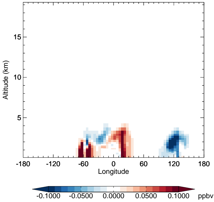
v11-02e-Run1 - v11-02e-Run0 INDIOL - Diff along 15S for Oct
