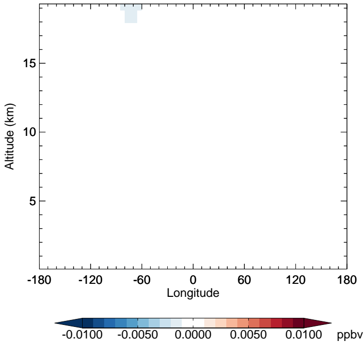
v11-02e-Run1 - v11-02e-Run0 BrNO3 - Diff along 15S for Oct
