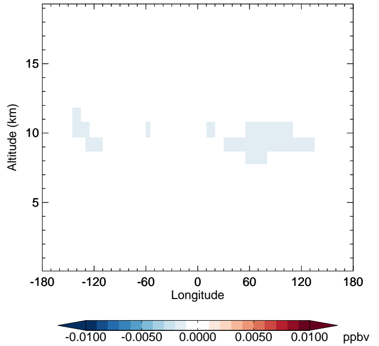
v11-02e-Run1 - v11-02d-Run1 HBr - Diff along 42N for Oct
