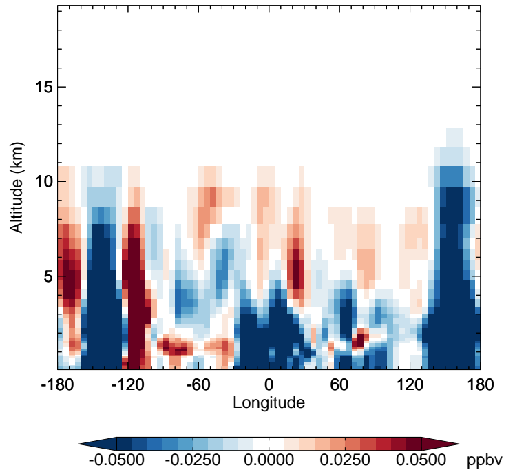
v11-02e-Run1 - v11-02d-Run1 MP - Diff along 42N for Oct
