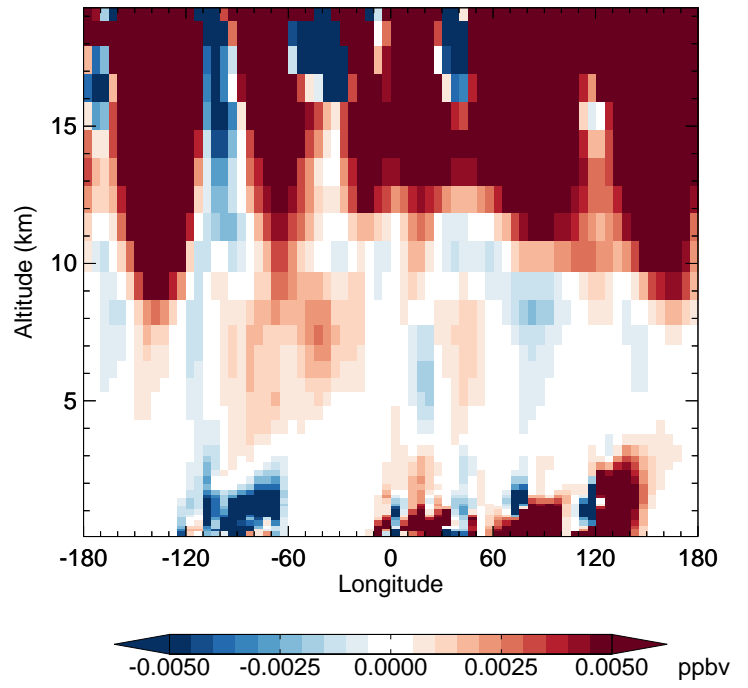
v11-02e-Run1 - v11-02e-Run0 N2O5 - Diff along 42N for Oct
