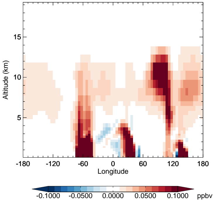
v11-02e-Run1 - v11-02d-Run1 BENZ - Diff along 15S for Oct
