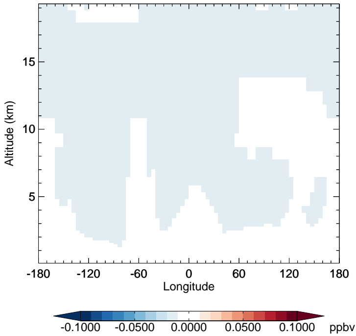
v11-02e-Run1 - v11-02d-Run1 HCFC141b - Diff along 15S for Oct
