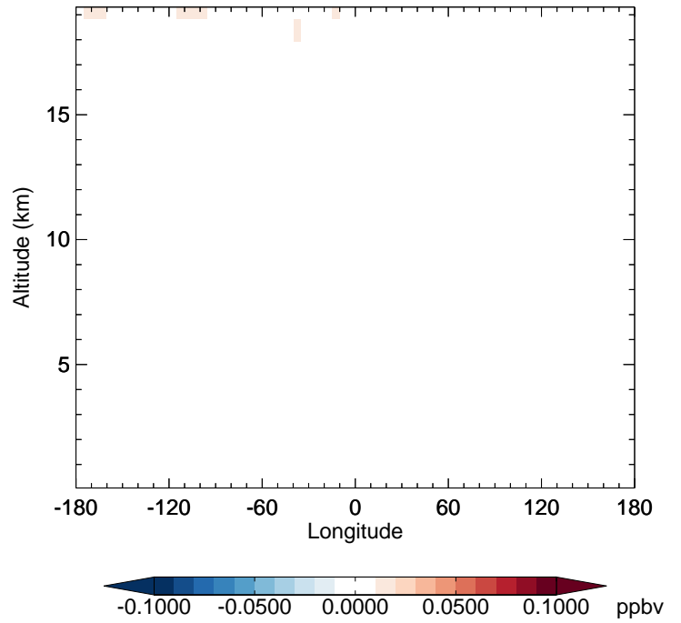
v11-02e-Run1 - v11-02d-Run1 CCI4 - Diff along 42N for Oct
