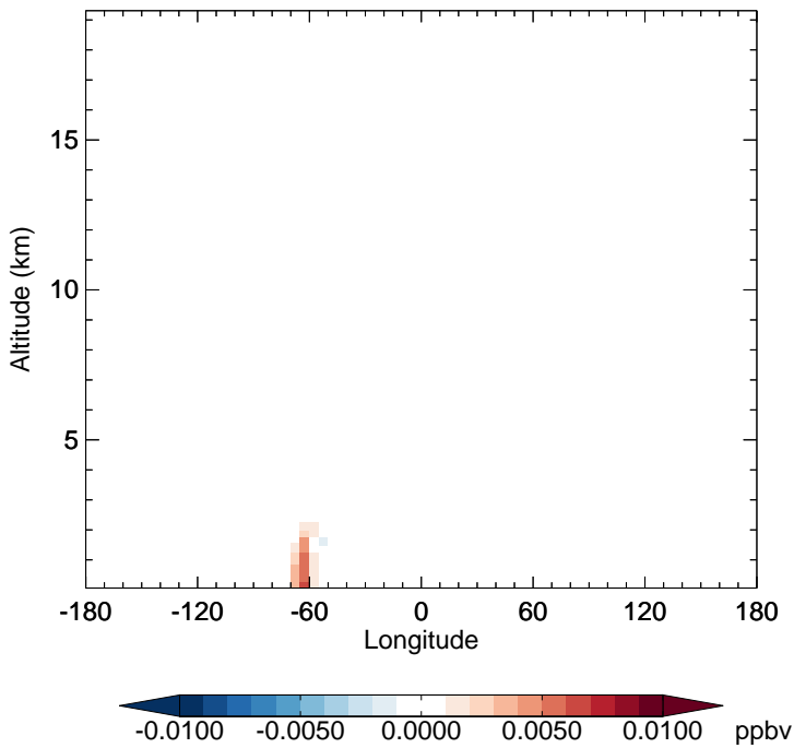
v11-02e-Run1 - v11-02d-Run1 MOBA - Diff along 15S for Oct
