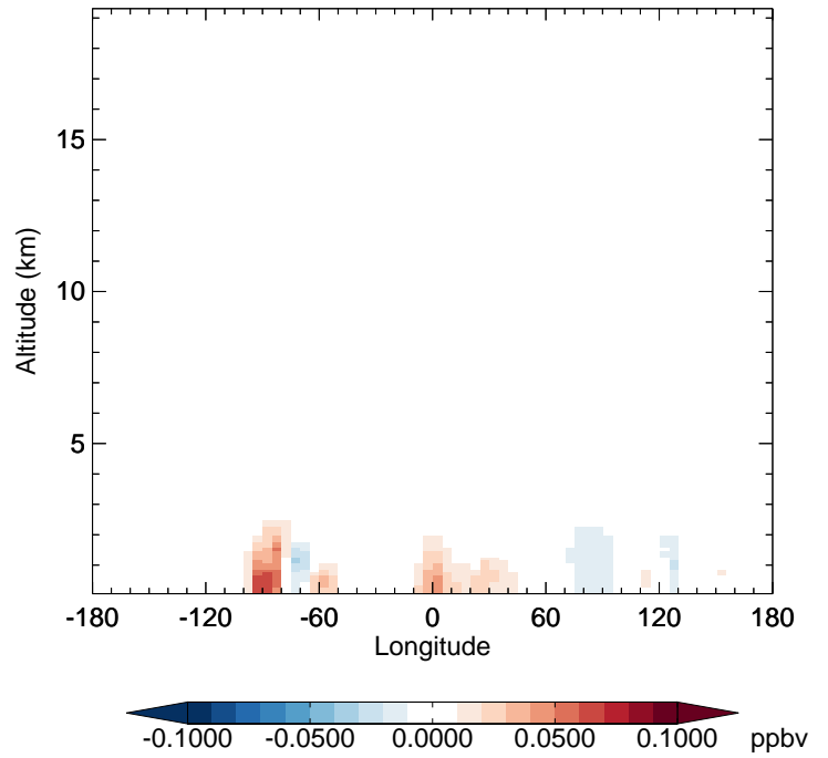
v11-02e-Run1 - v11-02d-Run1 INDIOL - Diff along 42N for Oct
