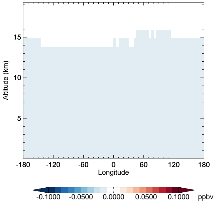
v11-02e-Run1 - v11-02e-Run0 HCFC22 - Diff along 15S for Oct
