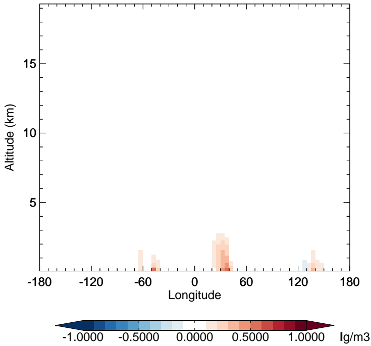
v11-02e-Run1 - v11-02d-Run1 NH3 - Diff along 15S for Oct
