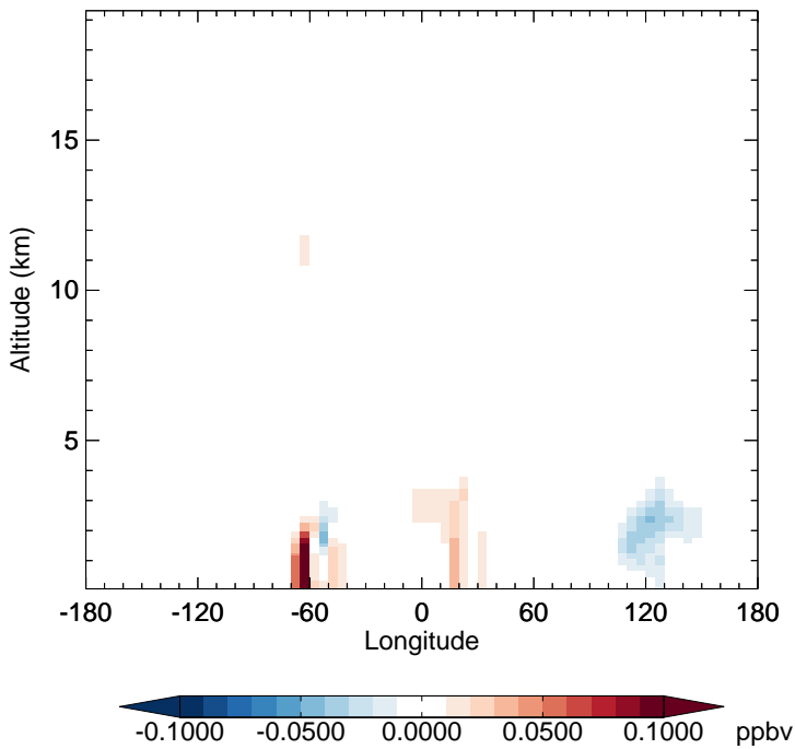
v11-02e-Run1 - v11-02d-Run1 ISOA1 - Diff along 15S for Oct
