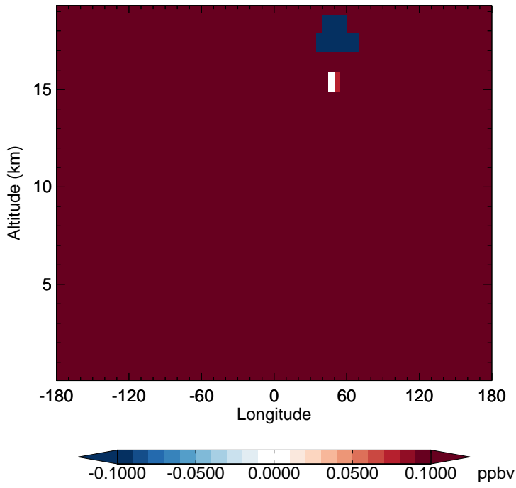
v11-02e-Run1 - v11-02e-Run0 N2O - Diff along 15S for Oct
