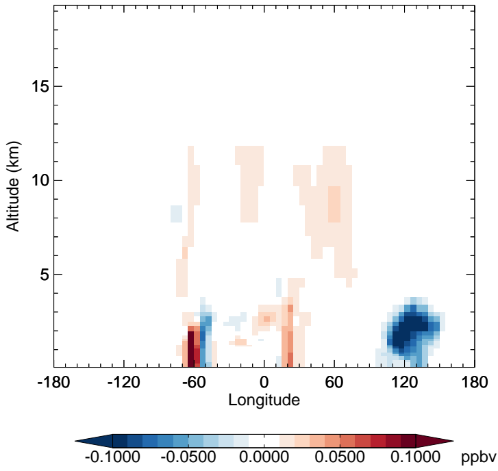
v11-02e-Run1 - v11-02e-Run0 ISO3 - Diff along 15S for Oct
