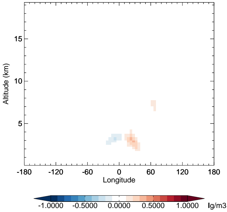
v11-02e-Run1 - v11-02e-Run0 NIT - Diff along 15S for Oct
