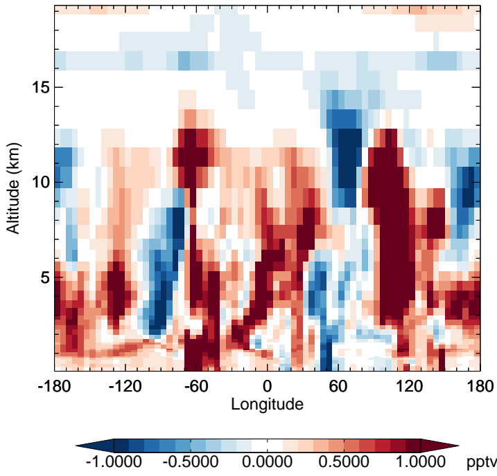
v11-02e-Run1 - v11-02e-Run0 HO2 - Diff along 15S for Oct
