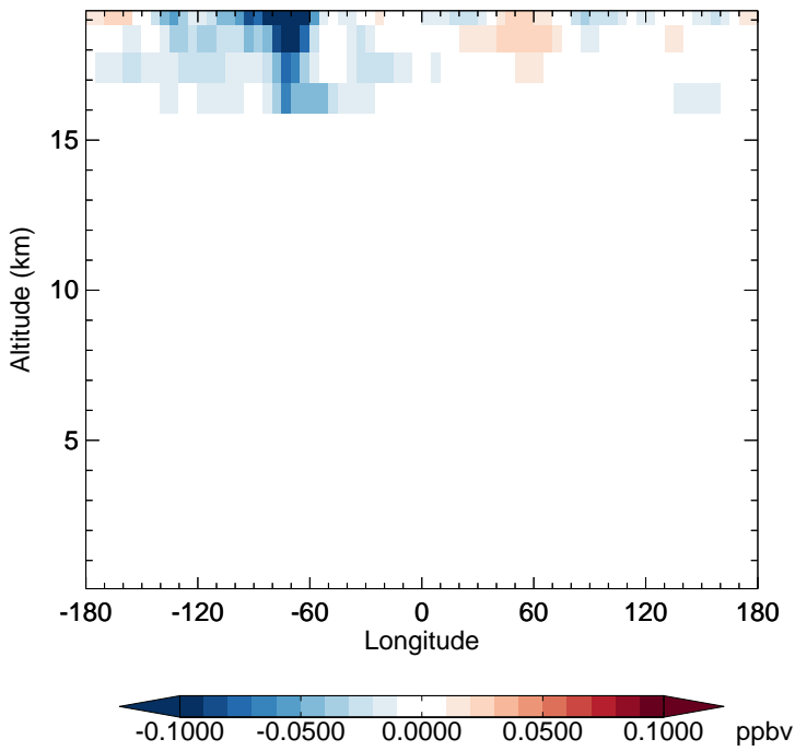
v11-02e-Run1 - v11-02d-Run1 CINO3 - Diff along 15S for Oct
