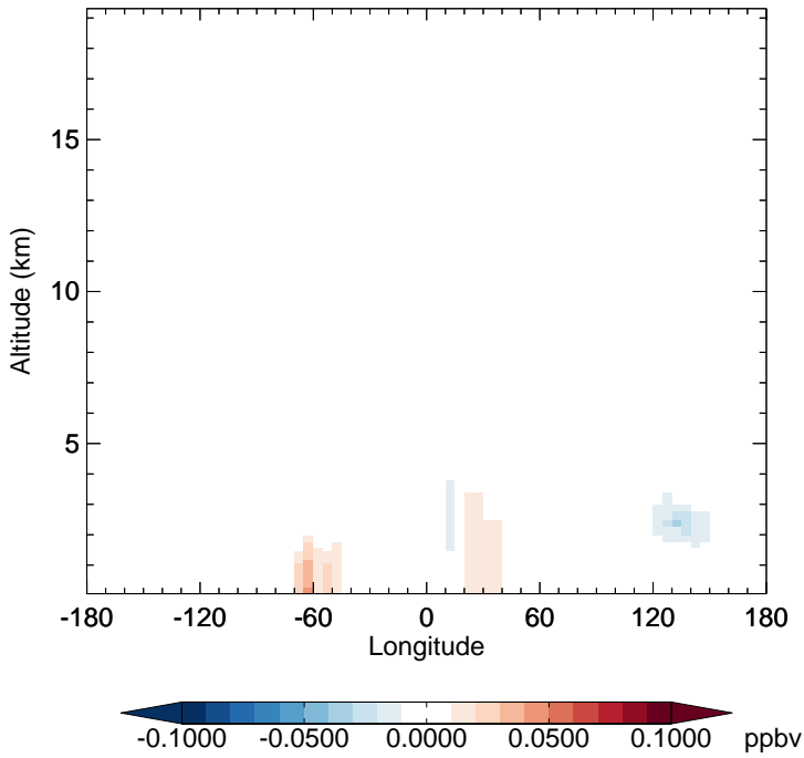
v11-02e-Run1 - v11-02d-Run1 IONITA - Diff along 15S for Oct
