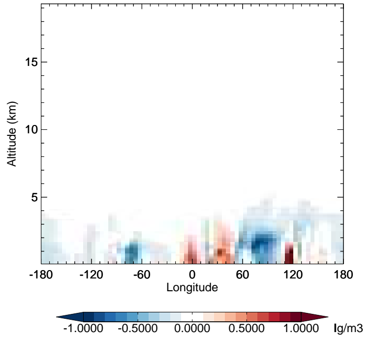
v11-02e-Run1 - v11-02d-Run1 SO4 - Diff along 42N for Oct
