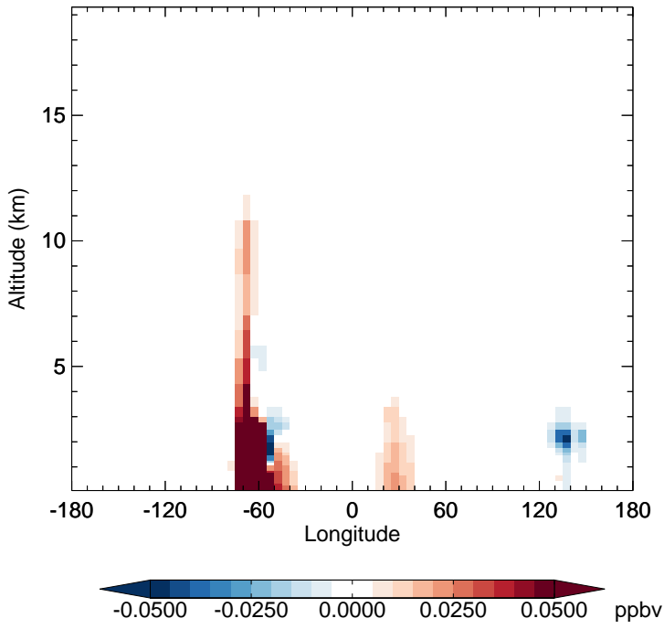
v11-02e-Run1 - v11-02e-Run0 MACR - Diff along 15S for Oct
