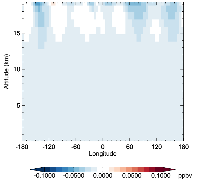
v11-02e-Run1 - v11-02e-Run0 CFC12 - Diff along 42N for Oct
