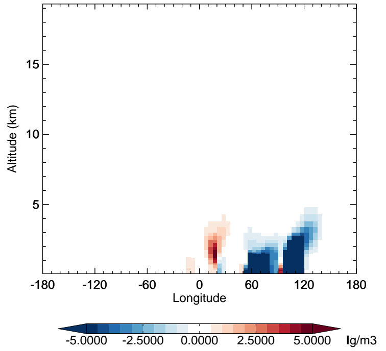
v11-02e-Run1 - v11-02e-Run0 DST3 - Diff along 42N for Oct
