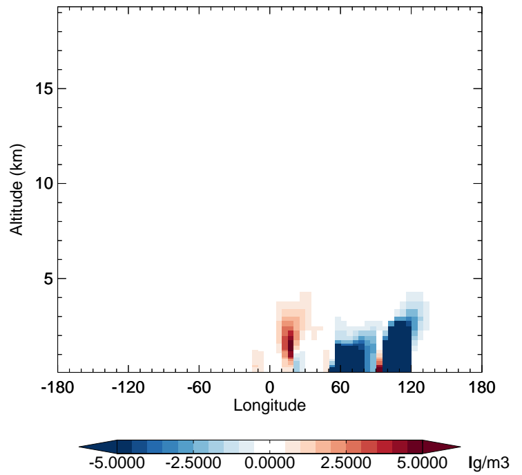
v11-02e-Run1 - v11-02d-Run1 DST3 - Diff along 42N for Oct
