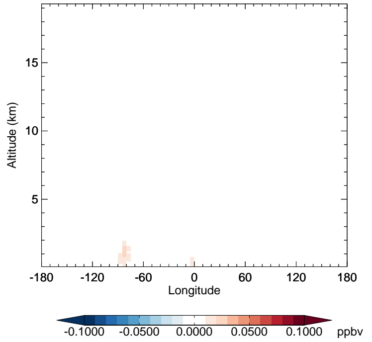
v11-02e-Run1 - v11-02e-Run0 HAC - Diff along 42N for Oct
