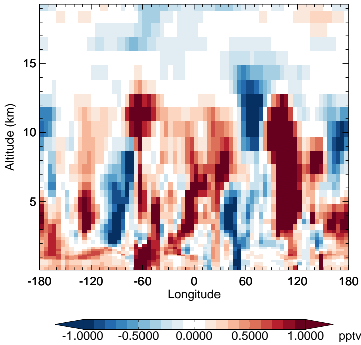
v11-02e-Run1 - v11-02d-Run1 HO2 - Diff along 15S for Oct
