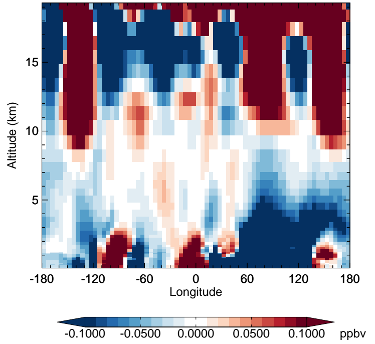
v11-02e-Run1 - v11-02e-Run0 HNO 3 - Diff along 42N for Oct
