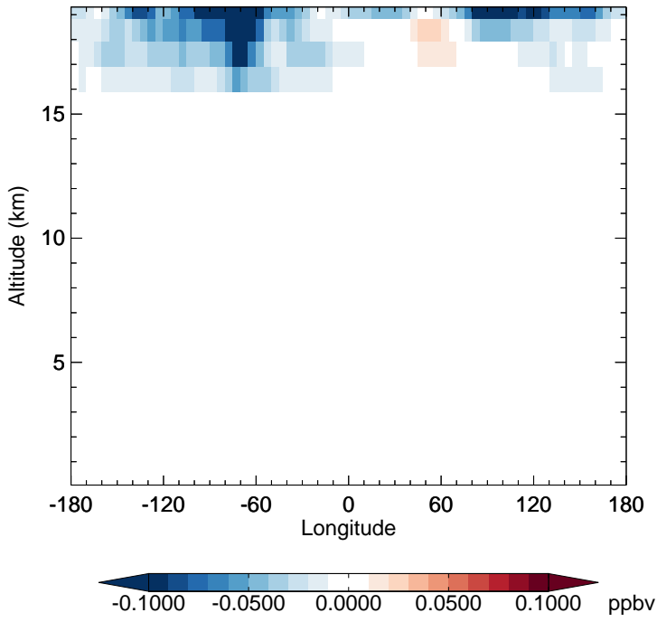
v11-02e-Run1 - v11-02e-Run0 CINO3 - Diff along 15S for Oct
