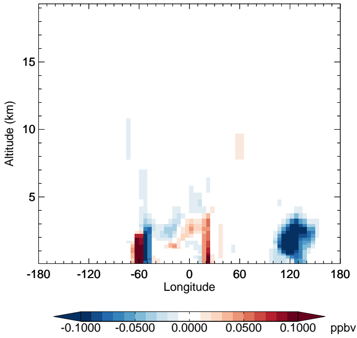
v11-02e-Run1 - v11-02e-Run0 TSOG3 - Diff along 15S for Oct
