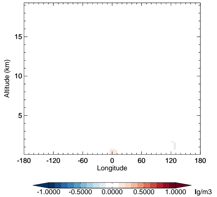
v11-02e-Run1 - v11-02d-Run1 BCPI - Diff along 42N for Oct
