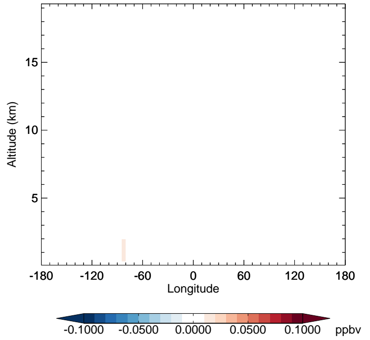
v11-02e-Run1 - v11-02e-Run0 SOAIE - Diff along 42N for Oct
