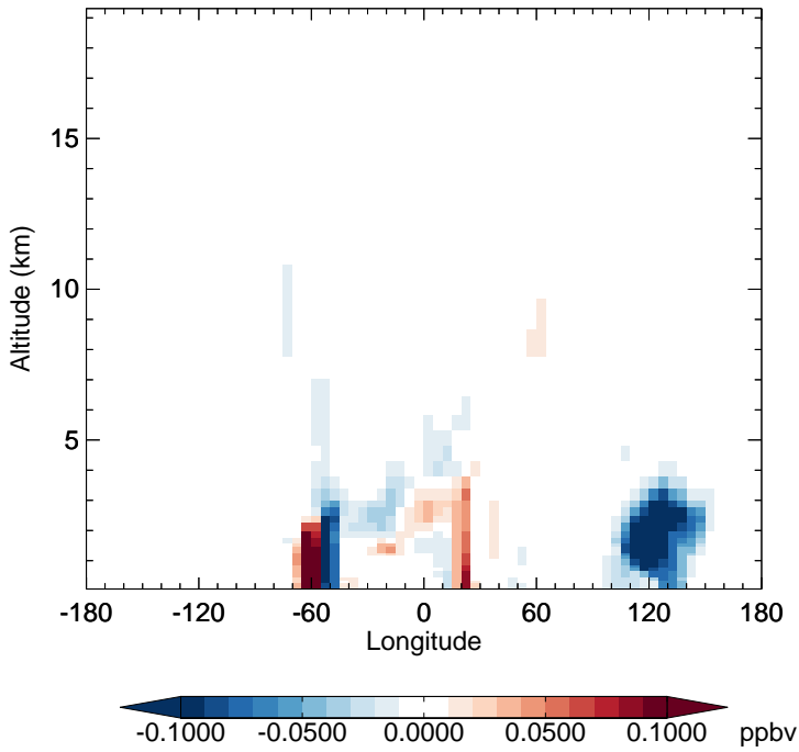
v11-02e-Run1 - v11-02d-Run1 TSOG3 - Diff along 15S for Oct
