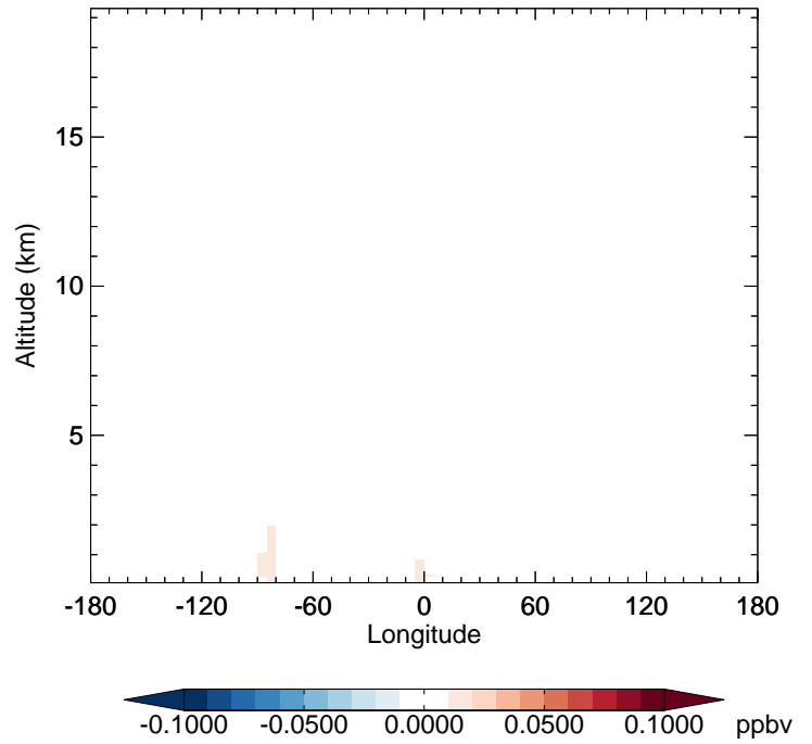
v11-02e-Run1 - v11-02d-Run1 IONITA - Diff along 42N for Oct
