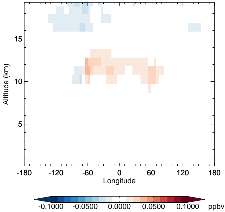
v11-02e-Run1 - v11-02d-Run1 MPN - Diff along 15S for Oct
