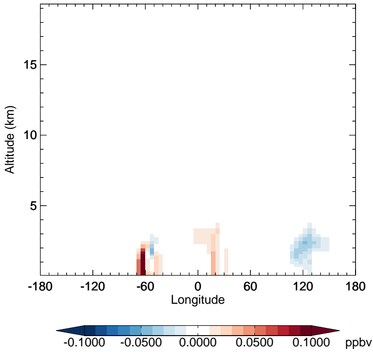
v11-02e-Run1 - v11-02e-Run0 ISOA1 - Diff along 15S for Oct
