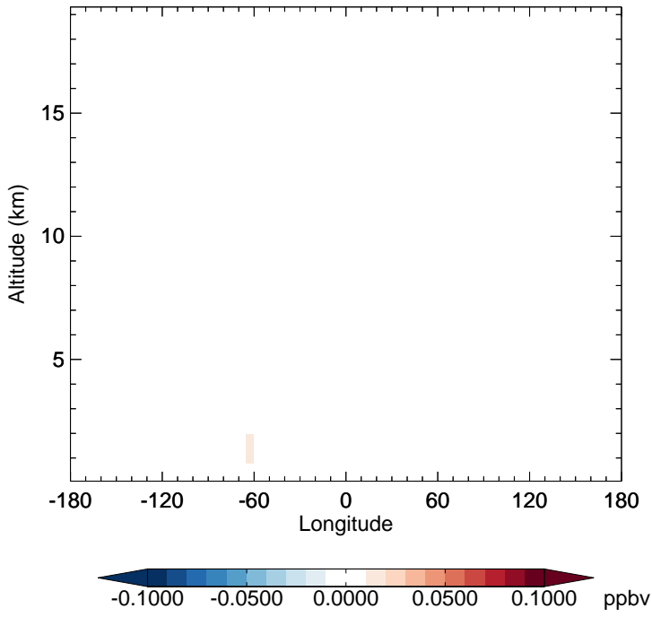
v11-02e-Run1 - v11-02e-Run0 RIPD - Diff along 15S for Oct
