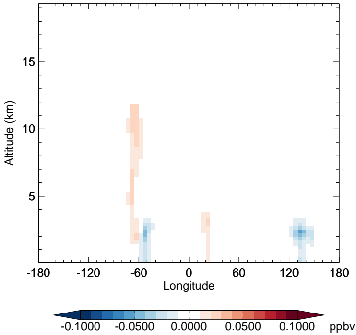
v11-02e-Run1 - v11-02d-Run1 HC187 - Diff along 15S for Oct
