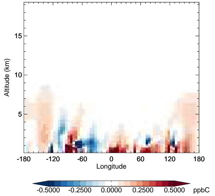
v11-02e-Run1 - v11-02e-Run0 ALK4 - Diff along 42N for Oct
