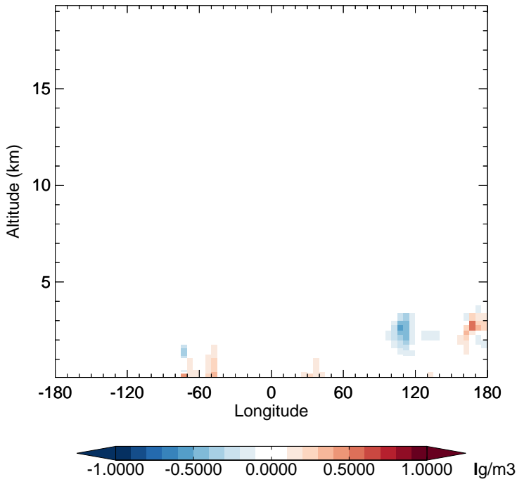
v11-02e-Run1 - v11-02e-Run0 SO 2 - Diff along 15S for Oct
