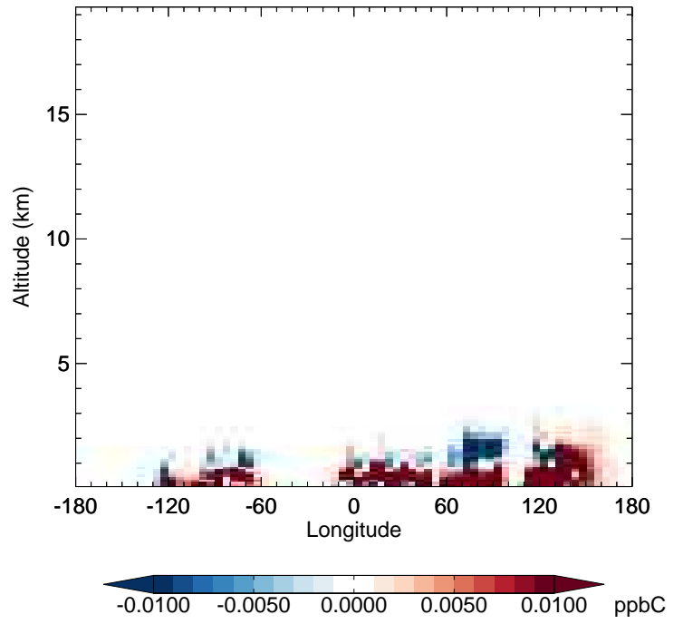
v11-02e-Run1 - v11-02e-Run0 PRPE - Diff along 42N for Oct
