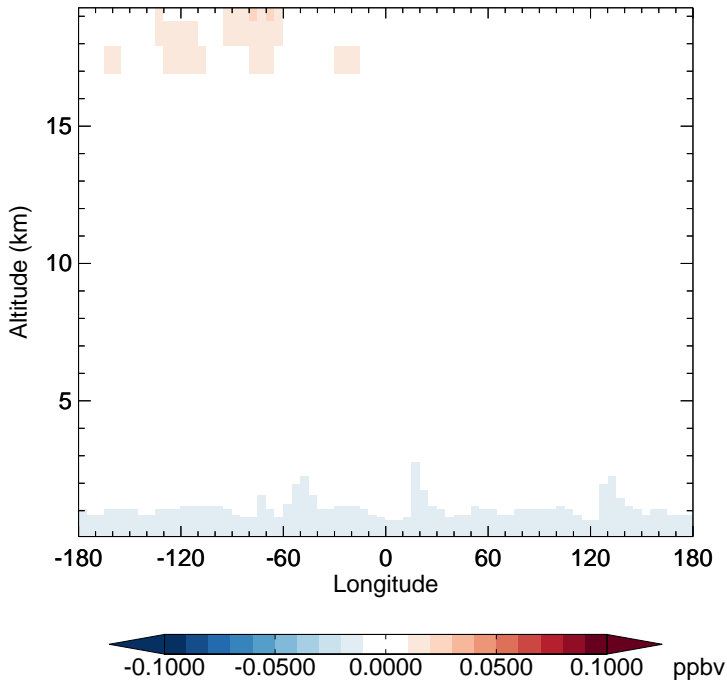
v11-02e-Run1 - v11-02d-Run1 CFC11 - Diff along 15S for Oct
