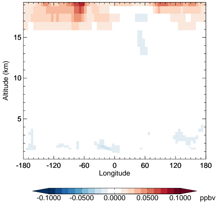
v11-02e-Run1 - v11-02e-Run0 CH3Cl - Diff along 15S for Oct
