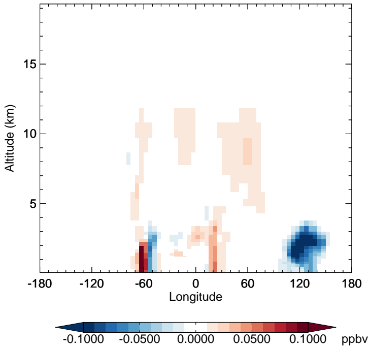
v11-02e-Run1 - v11-02d-Run1 ISO3 - Diff along 15S for Oct
