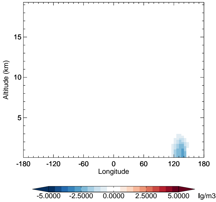
v11-02e-Run1 - v11-02e-Run0 DST4 - Diff along 15S for Oct
