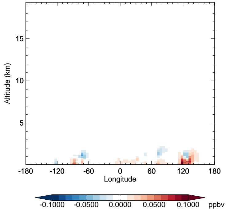
v11-02e-Run1 - v11-02e-Run0 SOAP - Diff along 42N for Oct
