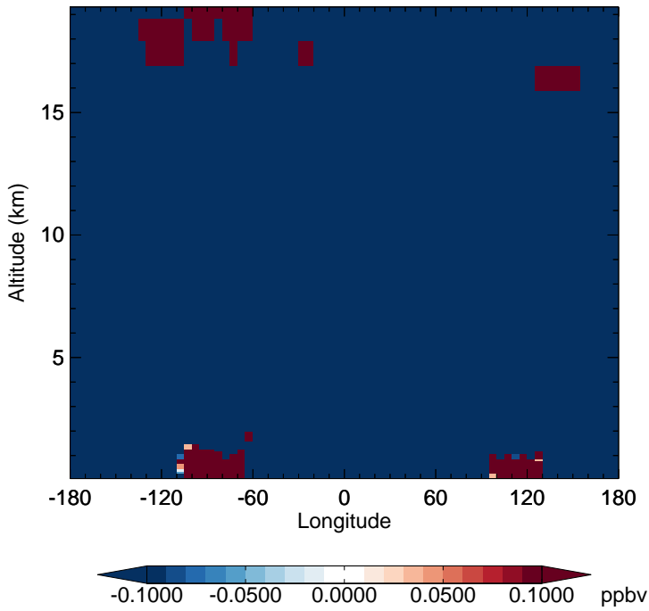
v11-02e-Run1 - v11-02d-Run1 CH4 - Diff along 15S for Oct
