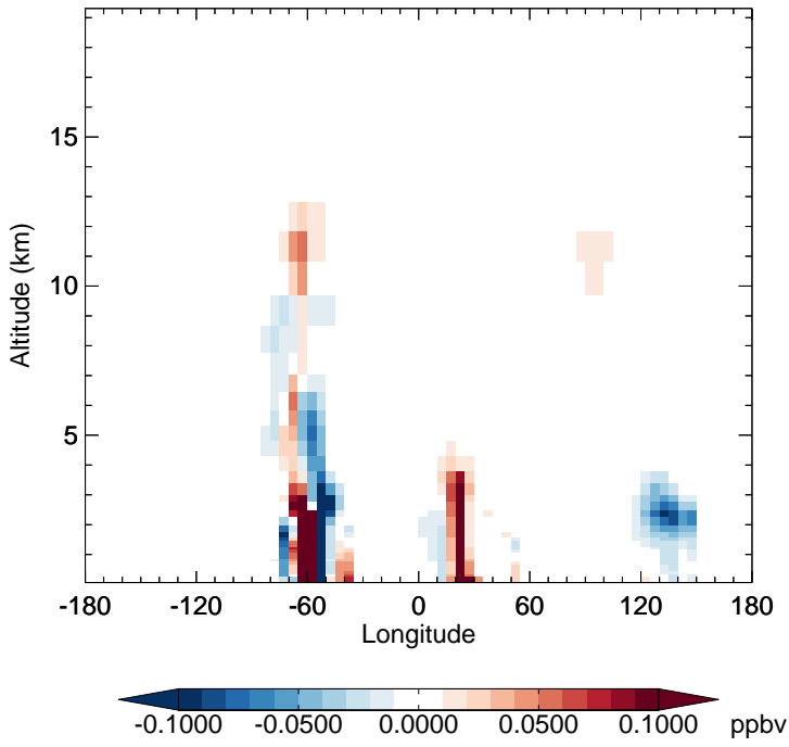
v11-02e-Run1 - v11-02e-Run0 EOH - Diff along 15S for Oct
