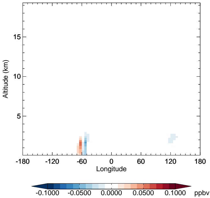
v11-02e-Run1 - v11-02d-Run1 TSOA0 - Diff along 15S for Oct
