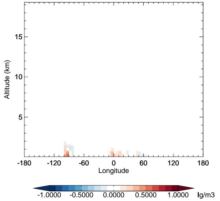
v11-02e-Run1 - v11-02e-Run0 NH3 - Diff along 42N for Oct
