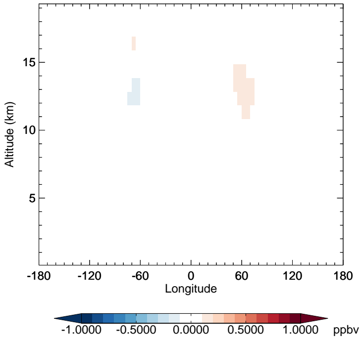
v11-02e-Run1 - v11-02e-Run0 NO - Diff along 15S for Oct
