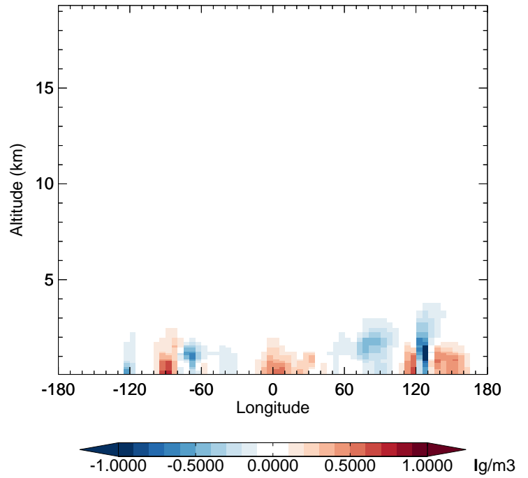
v11-02e-Run1 - v11-02d-Run1 SOAS - Diff along 42N for Oct
