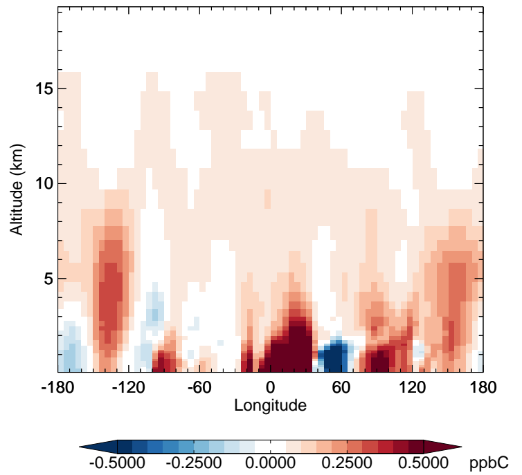
v11-02e-Run1 - v11-02d-Run1 C2H6 - Diff along 42N for Oct
