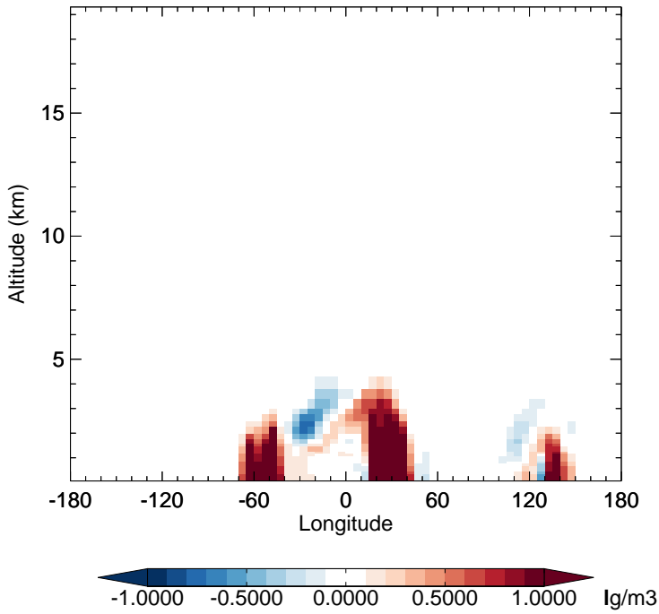
v11-02e-Run1 - v11-02d-Run1 OCPI - Diff along 15S for Oct
