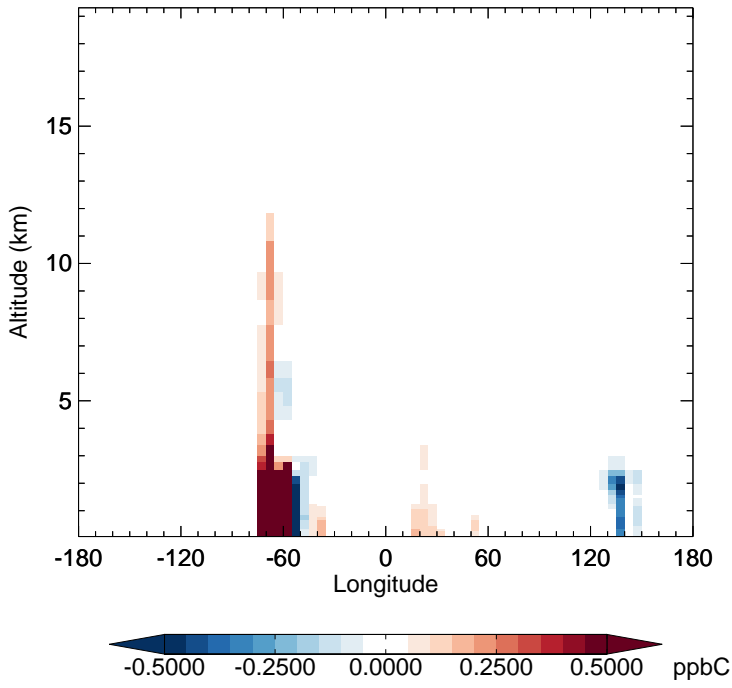
v11-02e-Run1 - v11-02e-Run0 ISOP - Diff along 15S for Oct
