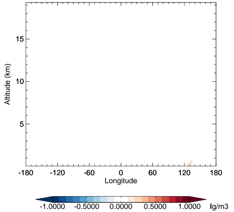
v11-02e-Run1 - v11-02d-Run1 OCPO - Diff along 42N for Oct
