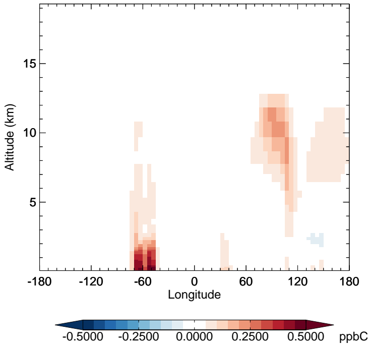
v11-02e-Run1 - v11-02e-Run0 C3H8 - Diff along 15S for Oct
