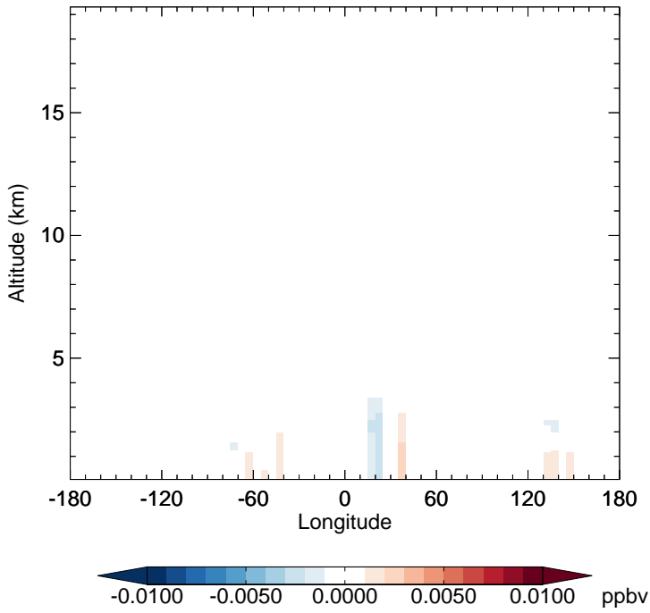
v11-02e-Run1 - v11-02e-Run0 MVKN - Diff along 15S for Oct
