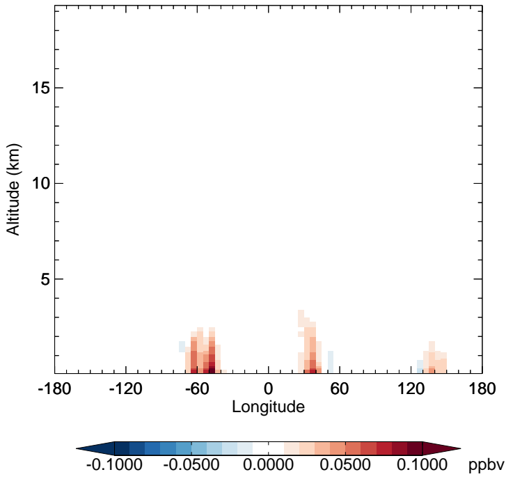
v11-02e-Run1 - v11-02e-Run0 SOAP - Diff along 15S for Oct
