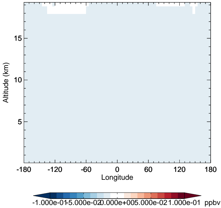
v11-02e-Run1 - v11-02d-Run1 HCFC22 - Diff along 15S for Oct
