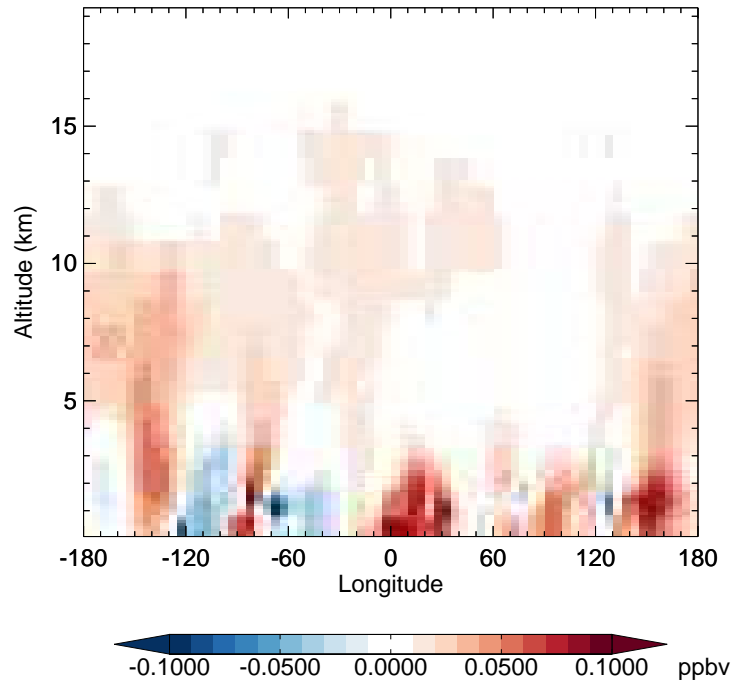
v11-02e-Run1 - v11-02e-Run0 PAN - Diff along 42N for Oct
