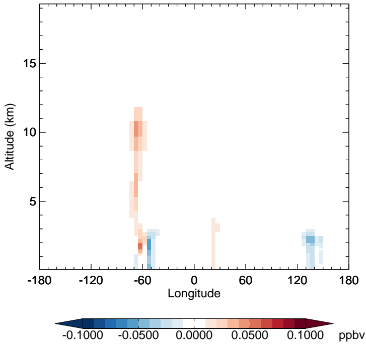
v11-02e-Run1 - v11-02d-Run1 IEPOXB - Diff along 15S for Oct
