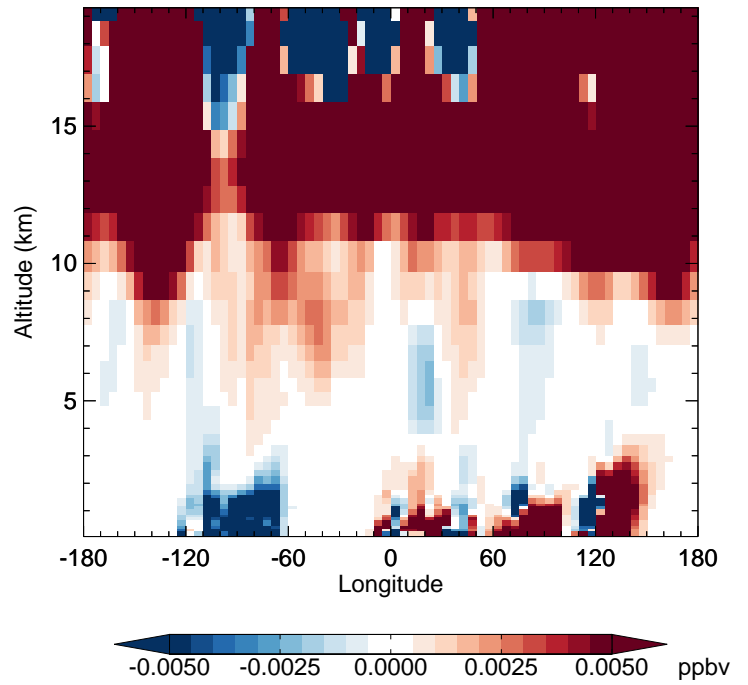
v11-02e-Run1 - v11-02d-Run1 N2O5 - Diff along 42N for Oct
