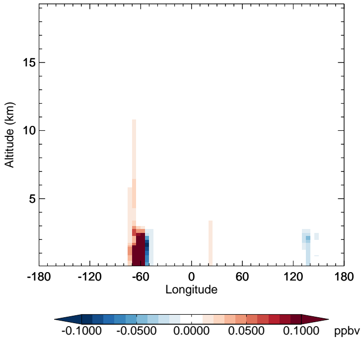
v11-02e-Run1 - v11-02e-Run0 RIPA - Diff along 15S for Oct
