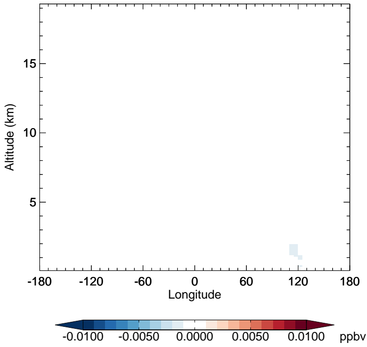
v11-02e-Run1 - v11-02e-Run0 HOBr - Diff along 15S for Oct
