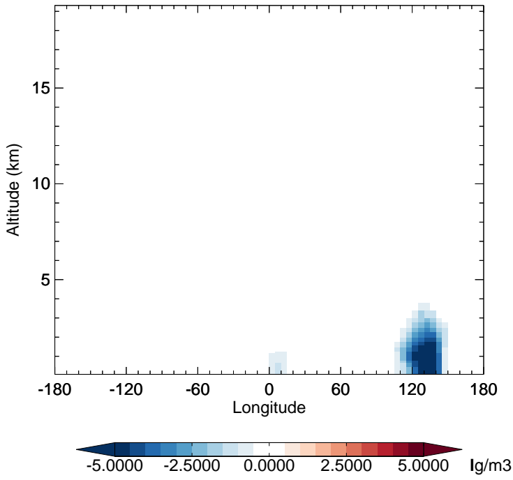
v11-02e-Run1 - v11-02e-Run0 DST3 - Diff along 15S for Oct
