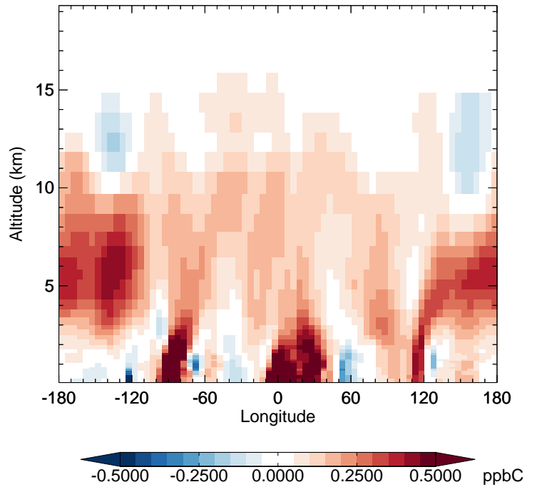
v11-02e-Run1 - v11-02d-Run1 ACET - Diff along 42N for Oct
