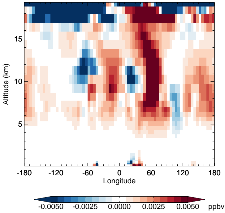
v11-02e-Run1 - v11-02e-Run0 N2O5 - Diff along 15S for Oct
