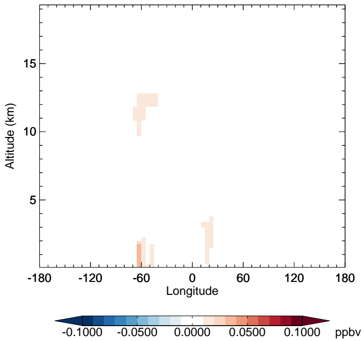
v11-02e-Run1 - v11-02d-Run1 ISOA3 - Diff along 15S for Oct
