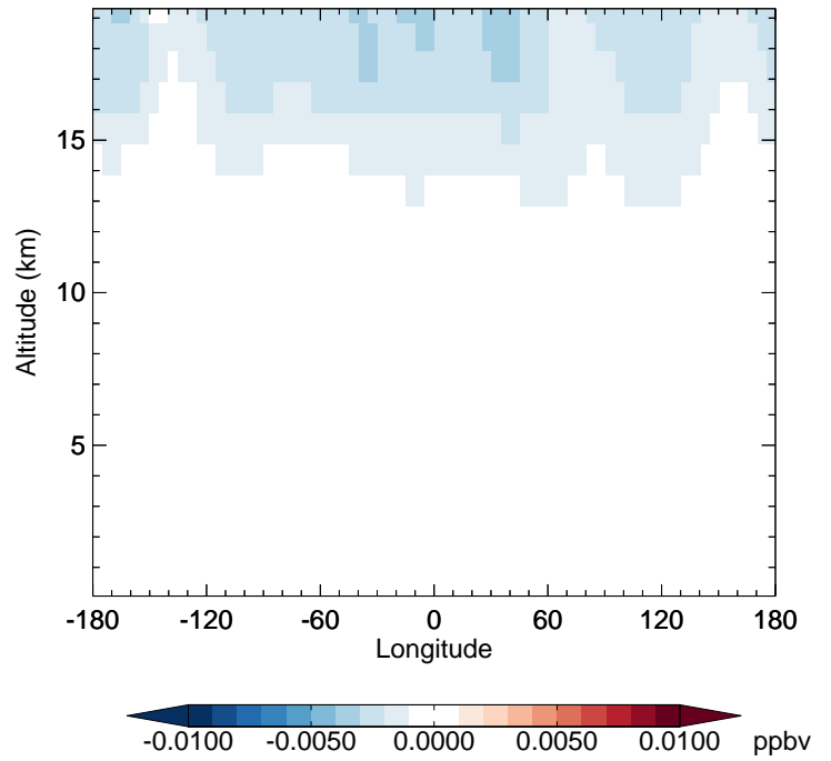
v11-02e-Run1 - v11-02d-Run1 BrNO3 - Diff along 42N for Oct
