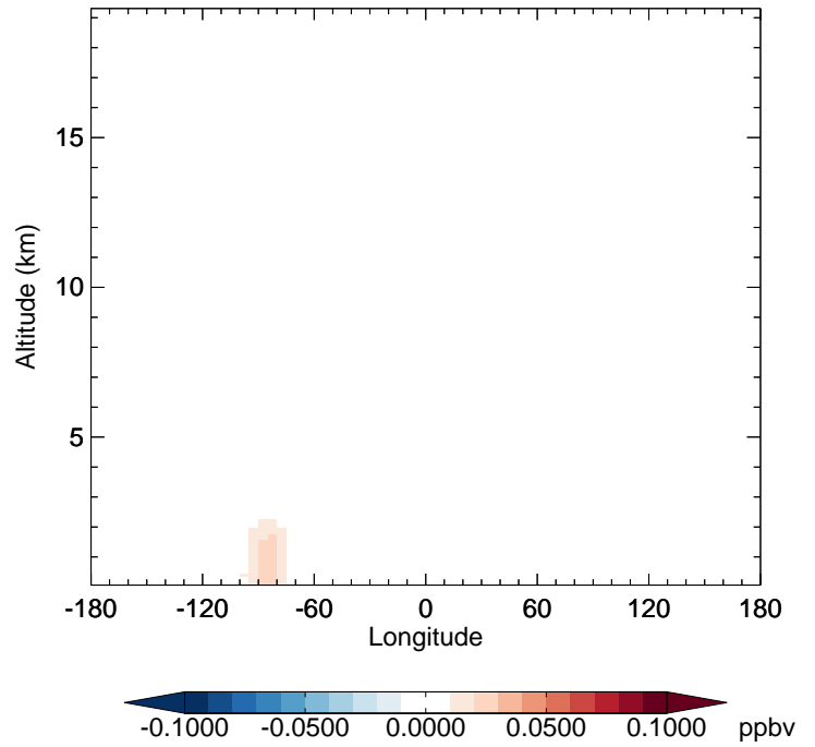
v11-02e-Run1 - v11-02d-Run1 SOAIE - Diff along 42N for Oct
