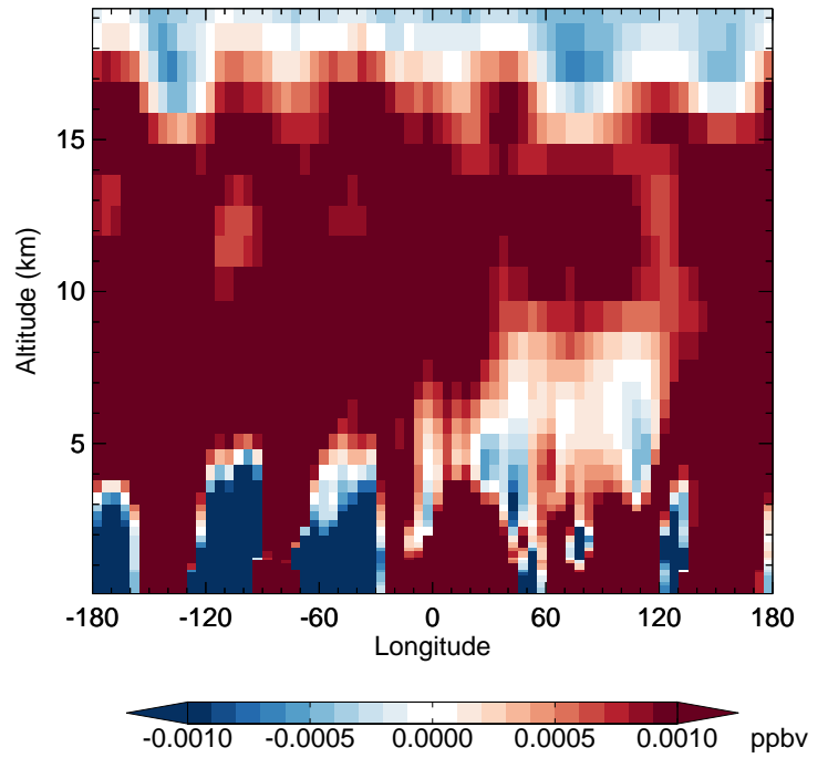
v11-02e-Run1 - v11-02d-Run1 PPN - Diff along 42N for Oct
