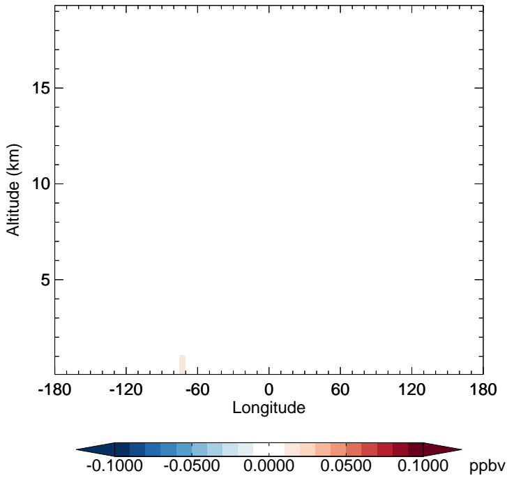
v11-02e-Run1 - v11-02d-Run1 SOAME - Diff along 15S for Oct
