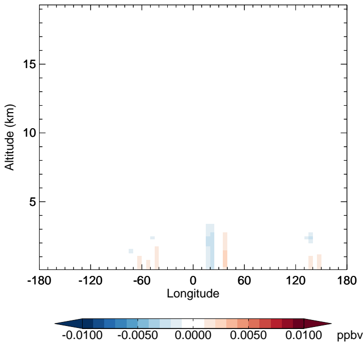
v11-02e-Run1 - v11-02d-Run1 MVKN - Diff along 15S for Oct
