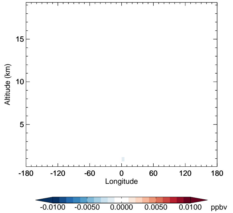
v11-02e-Run1 - v11-02e-Run0 MVKN - Diff along 42N for Oct
