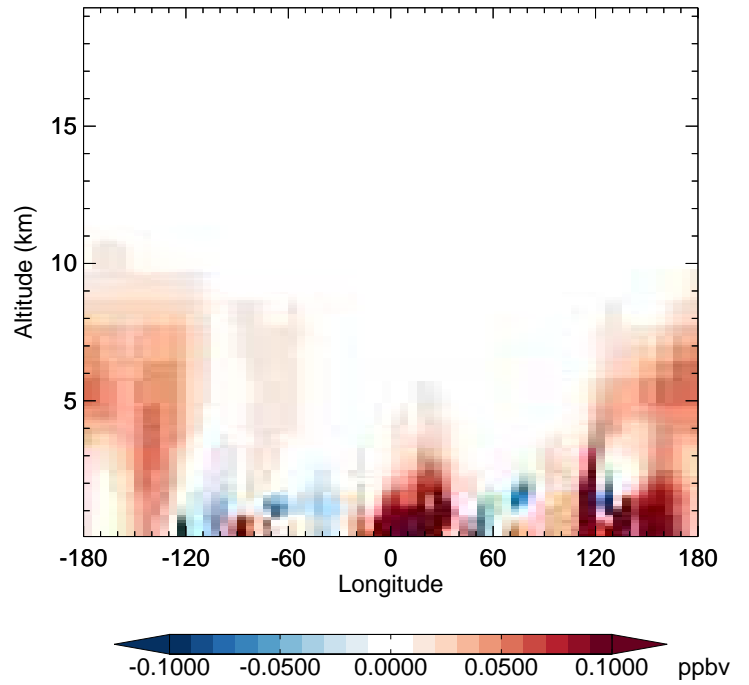
v11-02e-Run1 - v11-02d-Run1 BENZ - Diff along 42N for Oct
