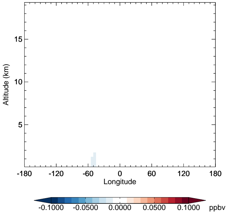
v11-02e-Run1 - v11-02e-Run0 ISOG1 - Diff along 15S for Oct
