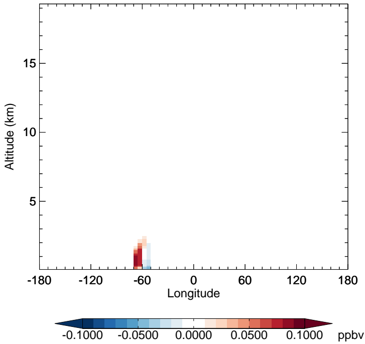
v11-02e-Run1 - v11-02d-Run1 MTPA - Diff along 15S for Oct
