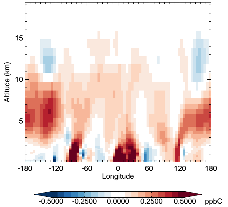
v11-02e-Run1 - v11-02e-Run0 ACET - Diff along 42N for Oct
