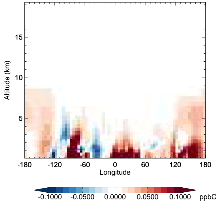
v11-02e-Run1 - v11-02e-Run0 MEK - Diff along 42N for Oct
