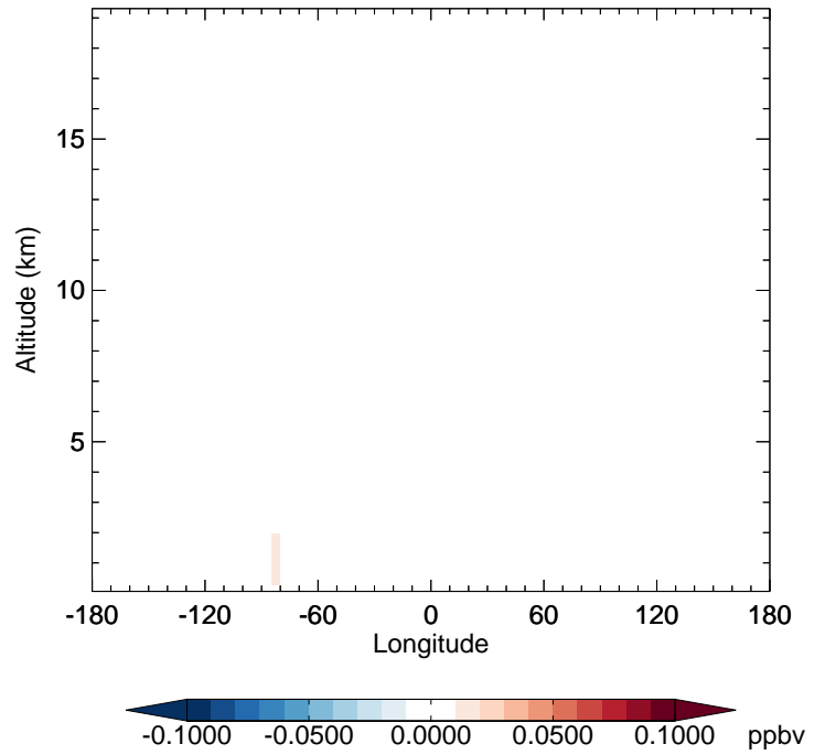
v11-02e-Run1 - v11-02d-Run1 ISO3 - Diff along 42N for Oct
