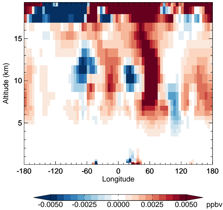
v11-02e-Run1 - v11-02d-Run1 N2O5 - Diff along 15S for Oct
