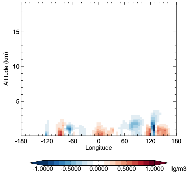
v11-02e-Run1 - v11-02e-Run0 SOAS - Diff along 42N for Oct
