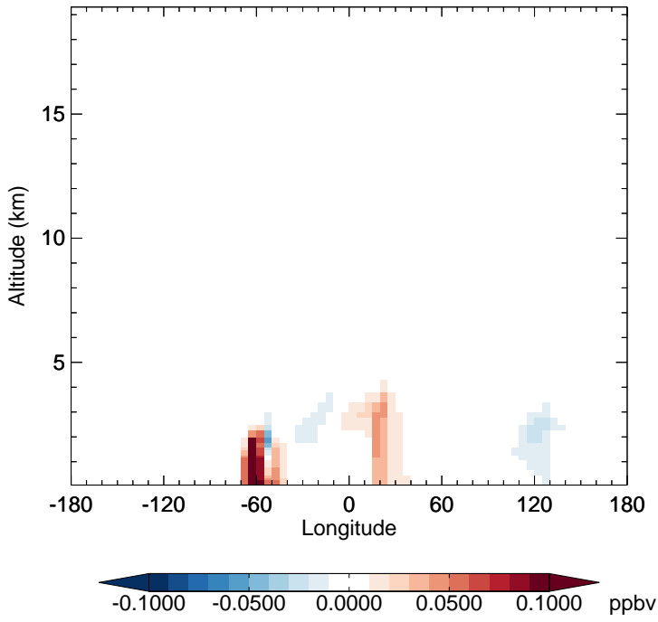
v11-02e-Run1 - v11-02e-Run0 TSOA2 - Diff along 15S for Oct
