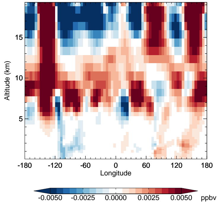
v11-02e-Run1 - v11-02d-Run1 HNO 4 - Diff along 42N for Oct
