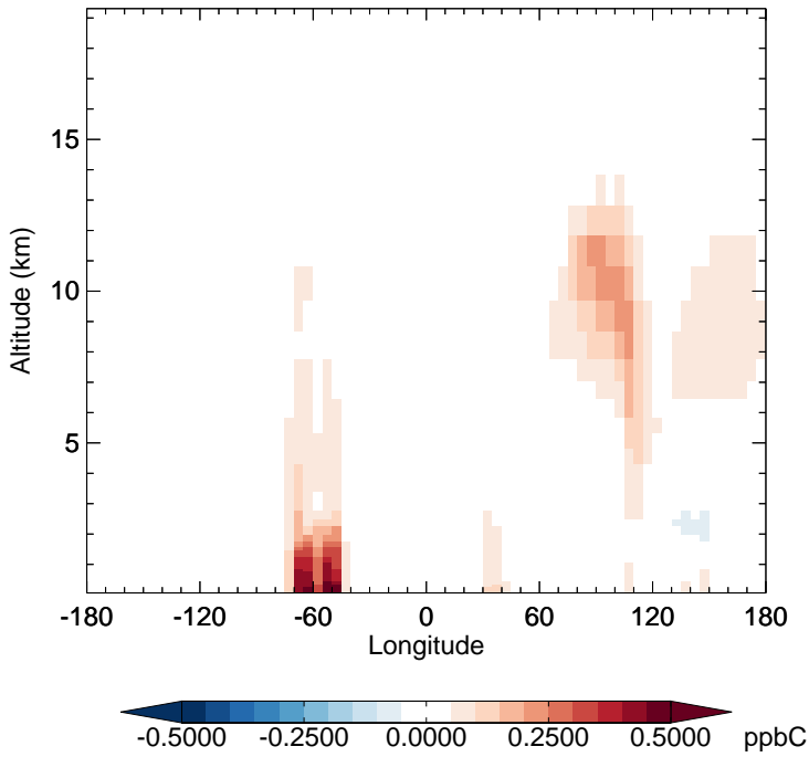
v11-02e-Run1 - v11-02d-Run1 C3H8 - Diff along 15S for Oct
