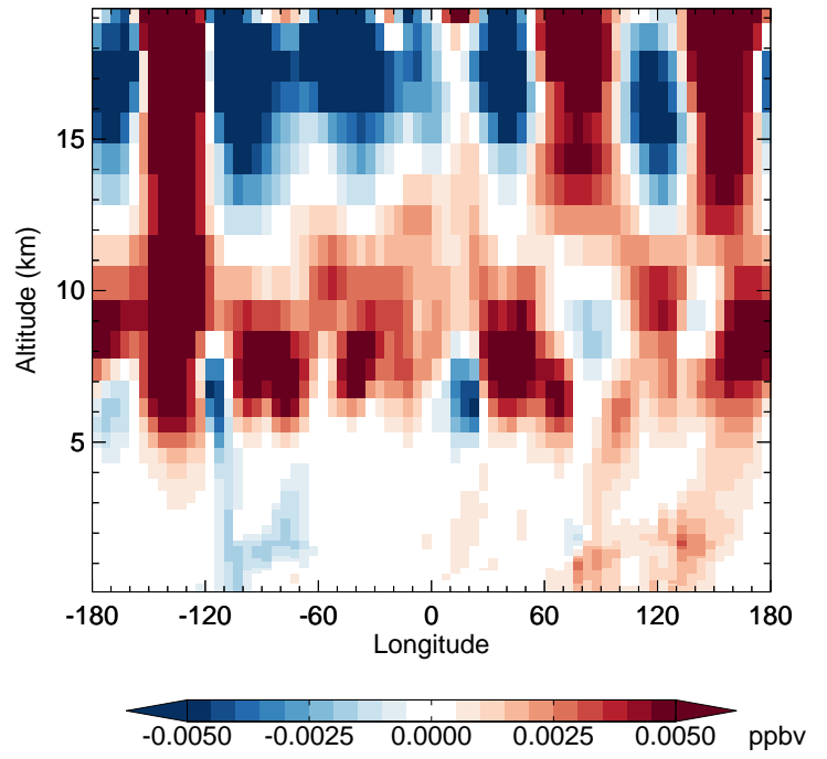
v11-02e-Run1 - v11-02e-Run0 HNO 4 - Diff along 42N for Oct
