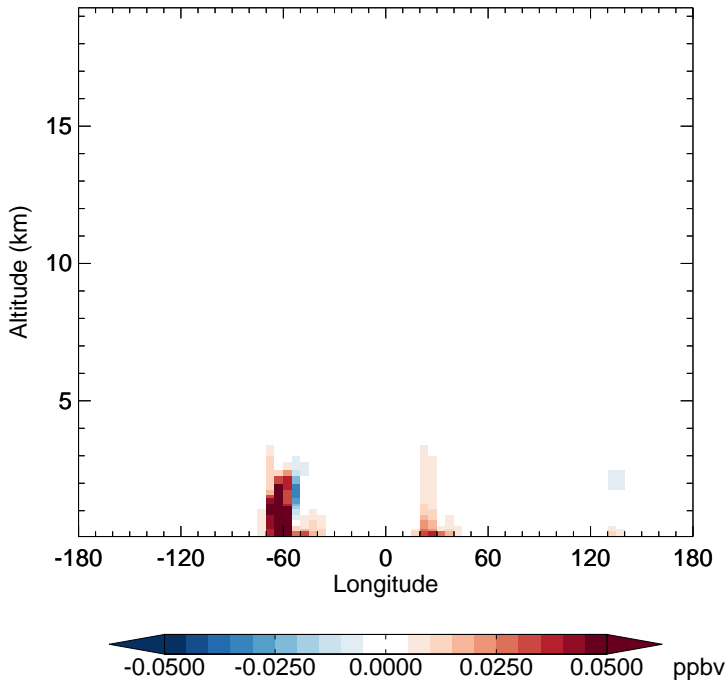
v11-02e-Run1 - v11-02d-Run1 RCHO - Diff along 15S for Oct
