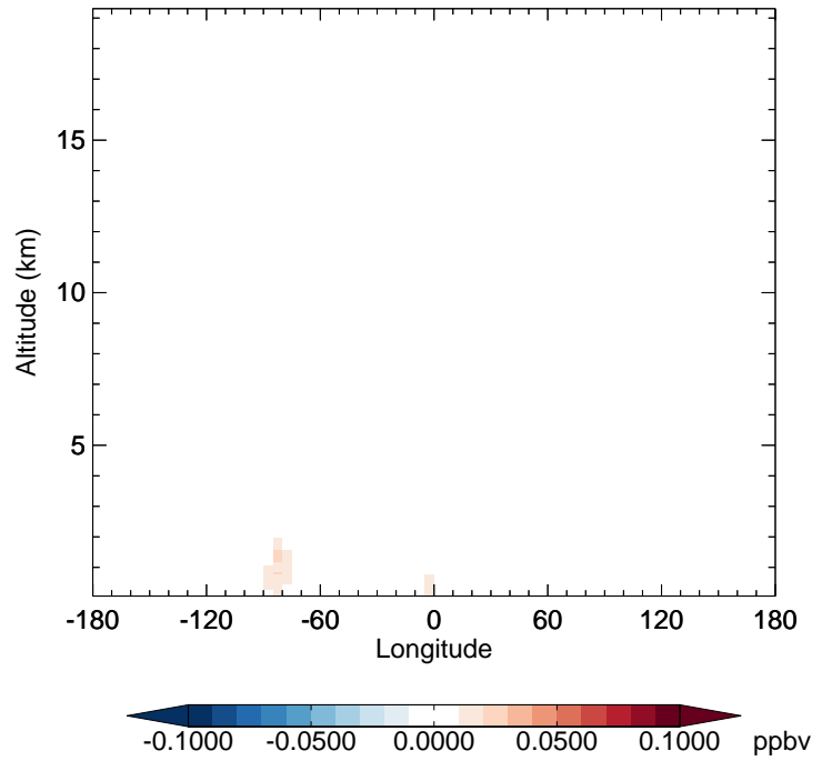
v11-02e-Run1 - v11-02d-Run1 GLYC - Diff along 42N for Oct
