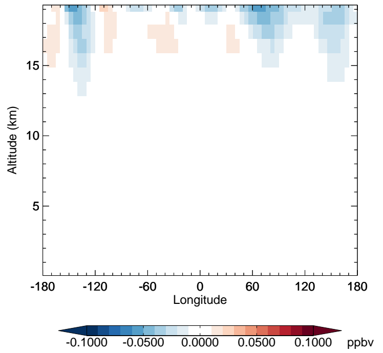
v11-02e-Run1 - v11-02e-Run0 OCS - Diff along 42N for Oct
