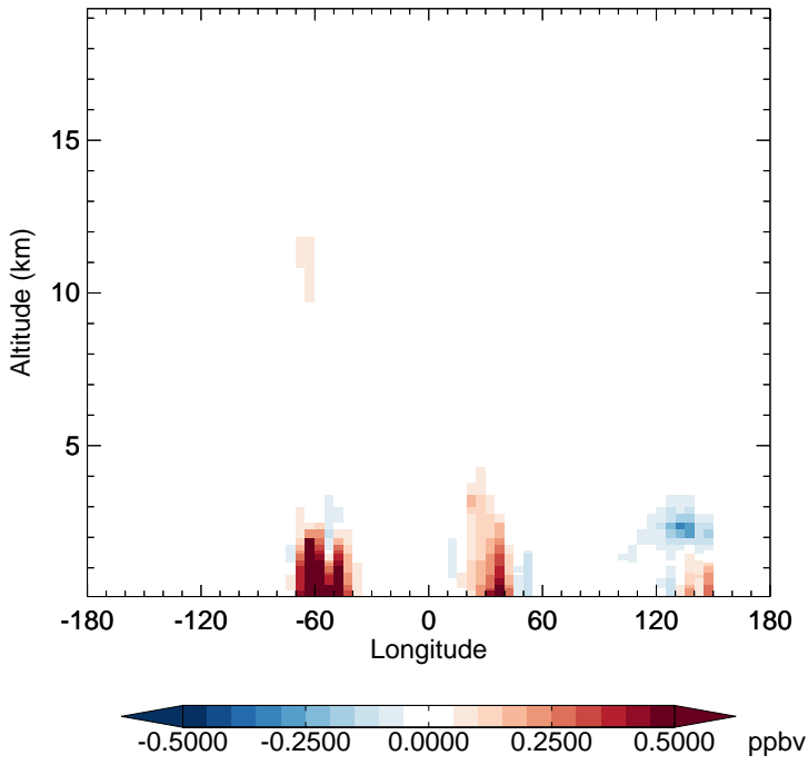
v11-02e-Run1 - v11-02e-Run0 CH 2 O - Diff along 15S for Oct
