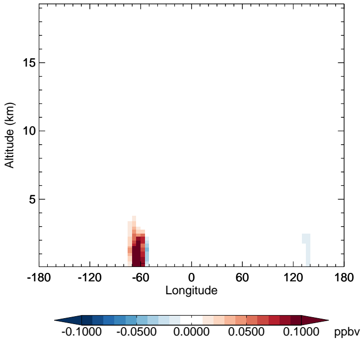
v11-02e-Run1 - v11-02e-Run0 HPALD - Diff along 15S for Oct
