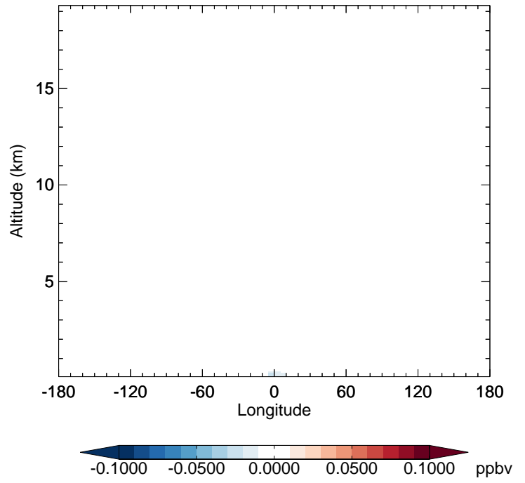
v11-02e-Run1 - v11-02e-Run0 CINO2 - Diff along 42N for Oct
