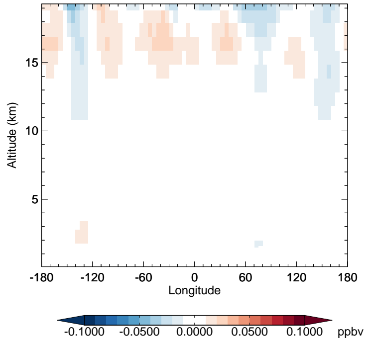
v11-02e-Run1 - v11-02e-Run0 CH3Cl - Diff along 42N for Oct
