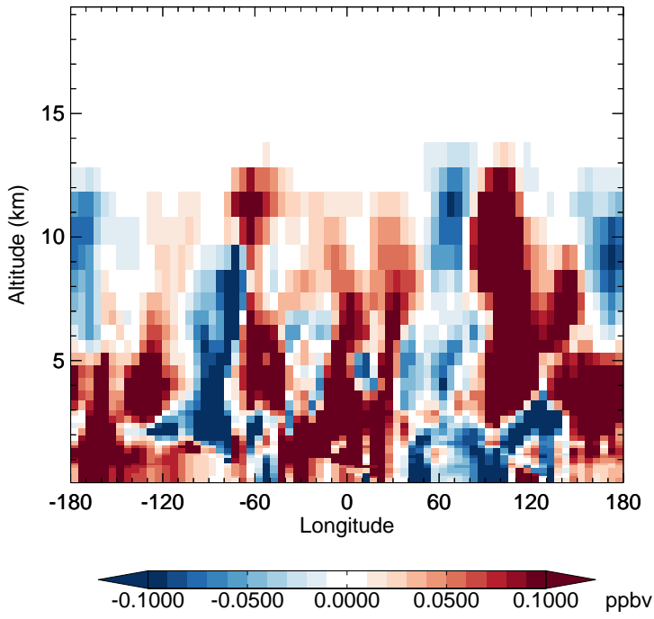
v11-02e-Run1 - v11-02e-Run0 H2O2 - Diff along 15S for Oct
