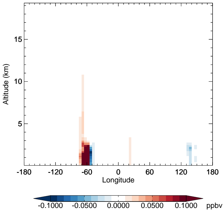
v11-02e-Run1 - v11-02d-Run1 RIPA - Diff along 15S for Oct
