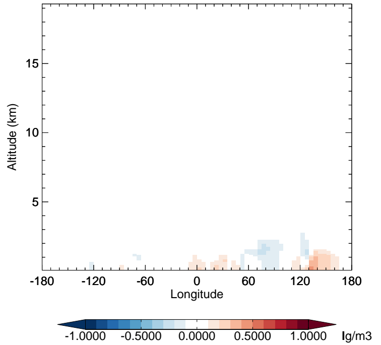
v11-02e-Run1 - v11-02d-Run1 OCPI - Diff along 42N for Oct
