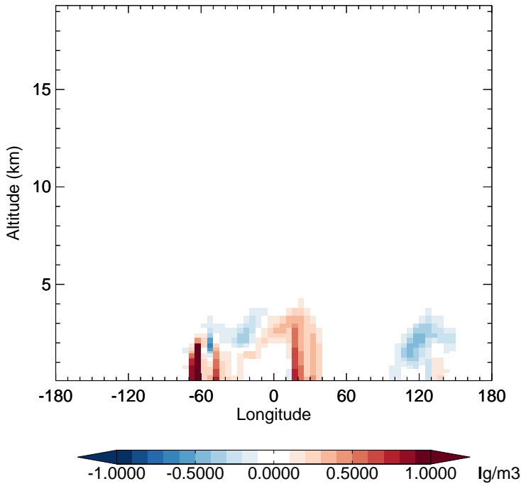
v11-02e-Run1 - v11-02d-Run1 SOAS - Diff along 15S for Oct
