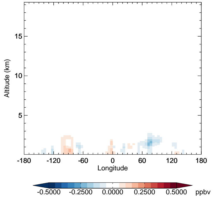
v11-02e-Run1 - v11-02e-Run0 CH 2 O - Diff along 42N for Oct
