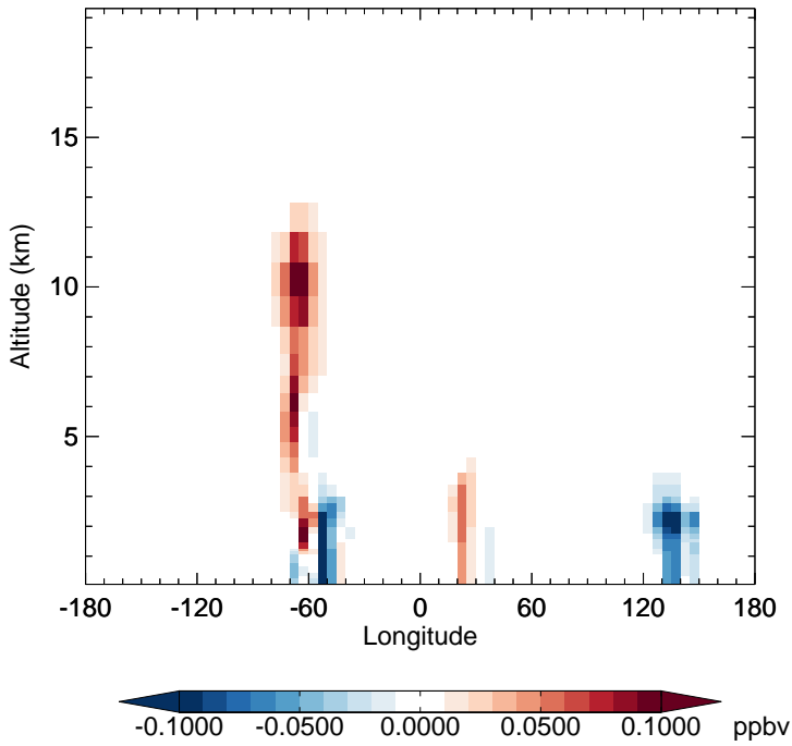
v11-02e-Run1 - v11-02d-Run1 IEPOXA - Diff along 15S for Oct
