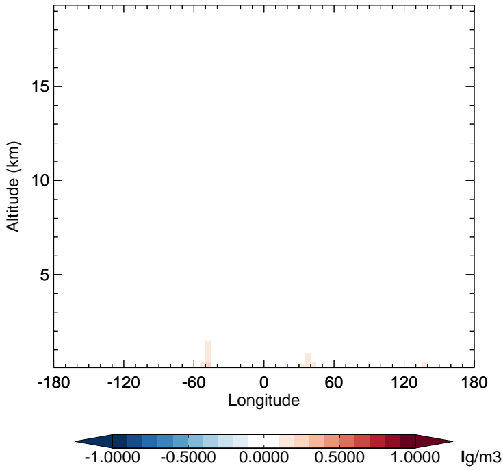
v11-02e-Run1 - v11-02e-Run0 BCPO - Diff along 15S for Oct
