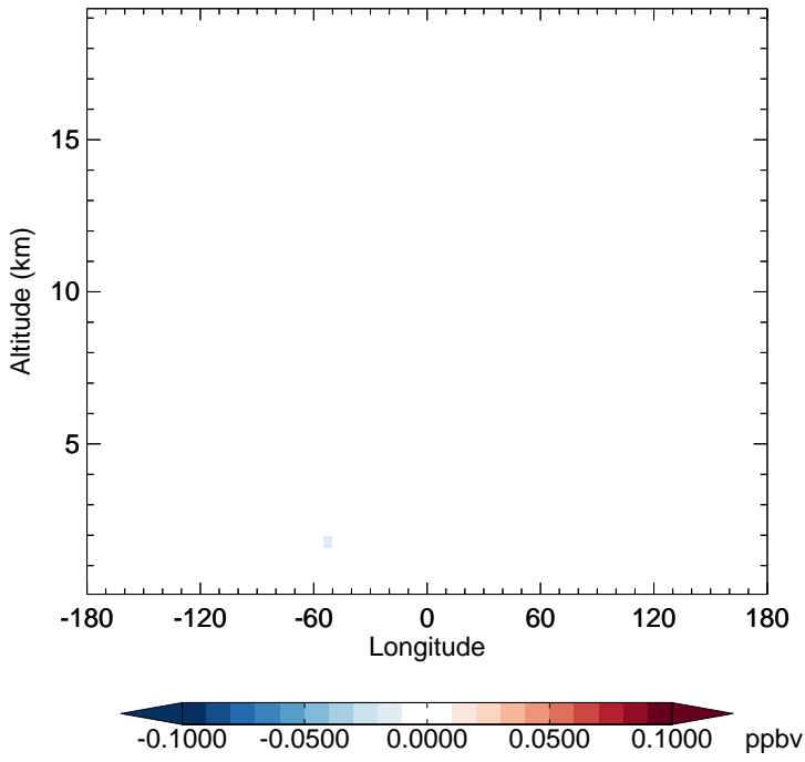
v11-02e-Run1 - v11-02e-Run0 LVOCOA - Diff along 15S for Oct
