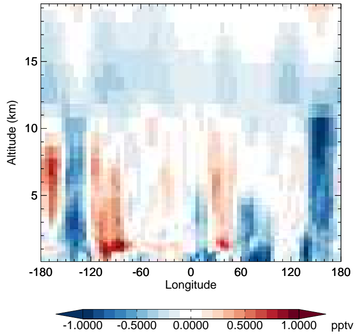
v11-02e-Run1 - v11-02d-Run1 HO2 - Diff along 42N for Oct
