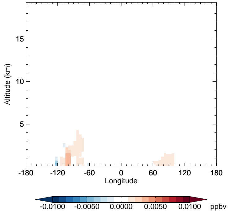
v11-02e-Run1 - v11-02e-Run0 R4N2 - Diff along 42N for Oct
