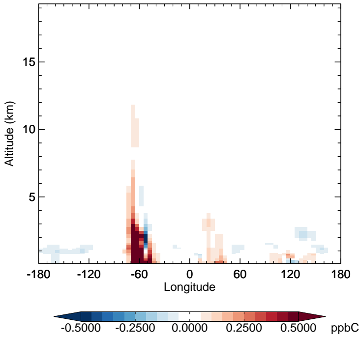
v11-02e-Run1 - v11-02e-Run0 ALD2 - Diff along 15S for Oct
