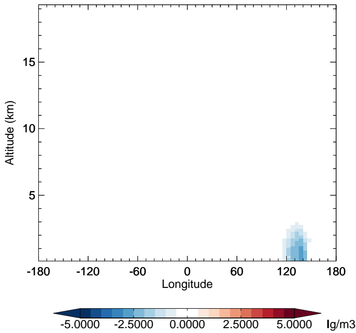
v11-02e-Run1 - v11-02d-Run1 DST4 - Diff along 15S for Oct
