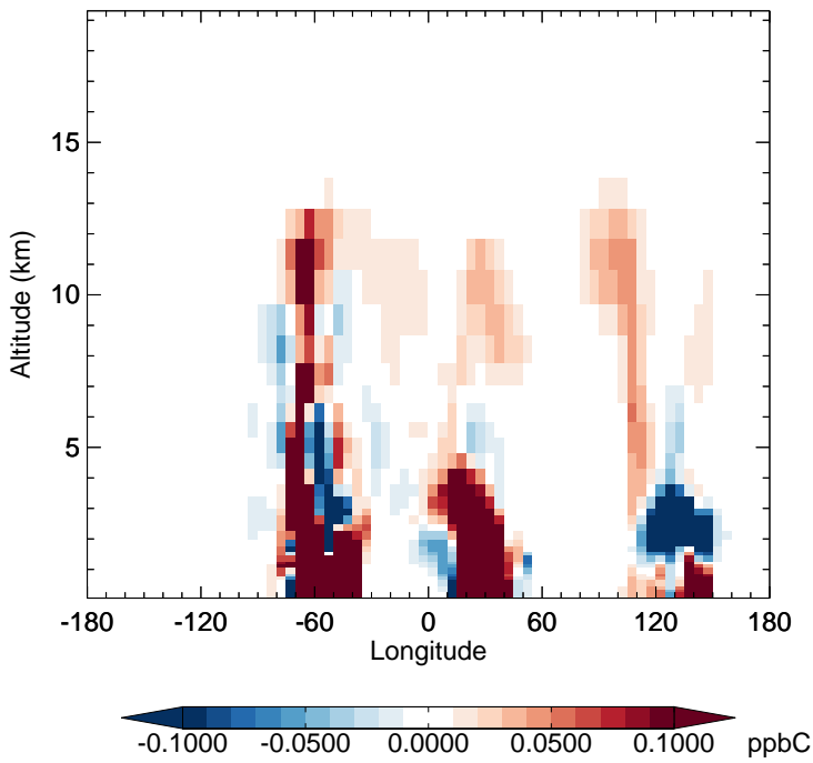
v11-02e-Run1 - v11-02d-Run1 MEK - Diff along 15S for Oct
