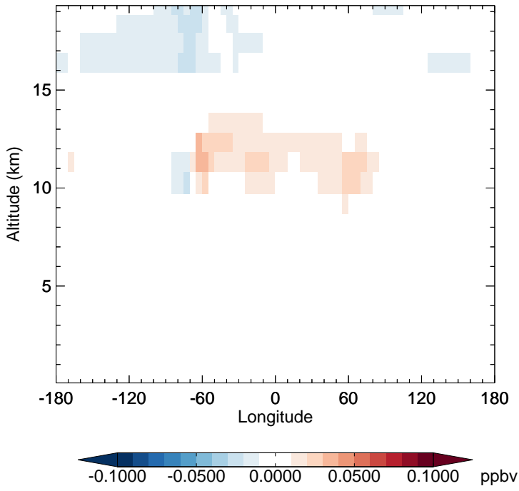
v11-02e-Run1 - v11-02e-Run0 MPN - Diff along 15S for Oct
