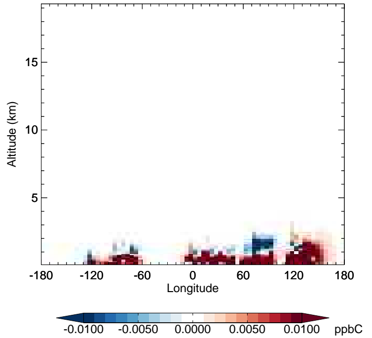
v11-02e-Run1 - v11-02d-Run1 PRPE - Diff along 42N for Oct
