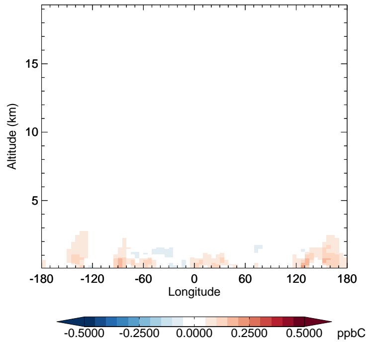
v11-02e-Run1 - v11-02d-Run1 ALD2 - Diff along 42N for Oct
