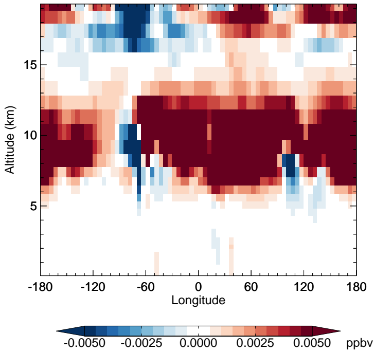
v11-02e-Run1 - v11-02d-Run1 HNO 4 - Diff along 15S for Oct
