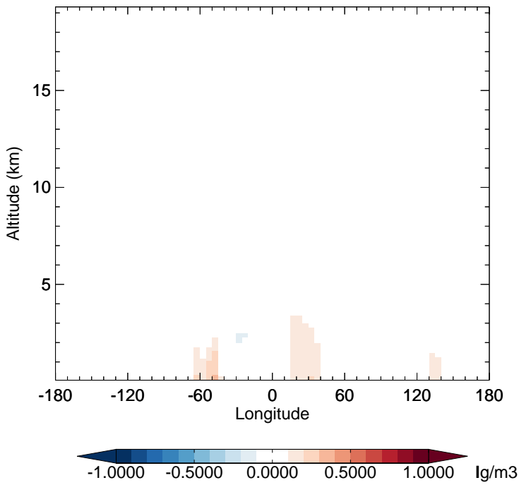
v11-02e-Run1 - v11-02d-Run1 BCPI - Diff along 15S for Oct
