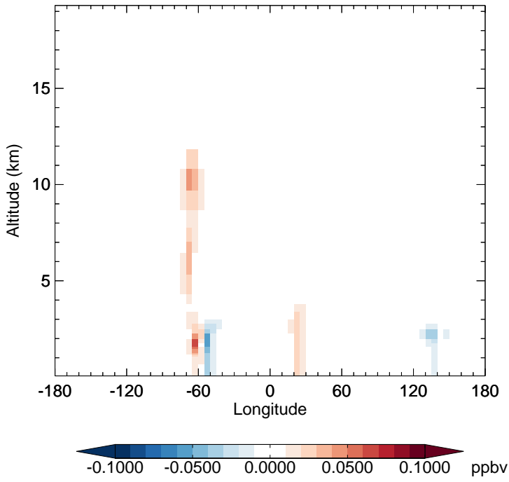
v11-02e-Run1 - v11-02e-Run0 IEPOXB - Diff along 15S for Oct
