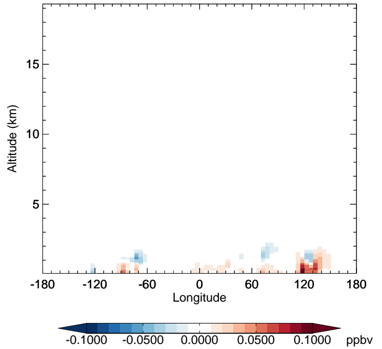
v11-02e-Run1 - v11-02d-Run1 SOAP - Diff along 42N for Oct
