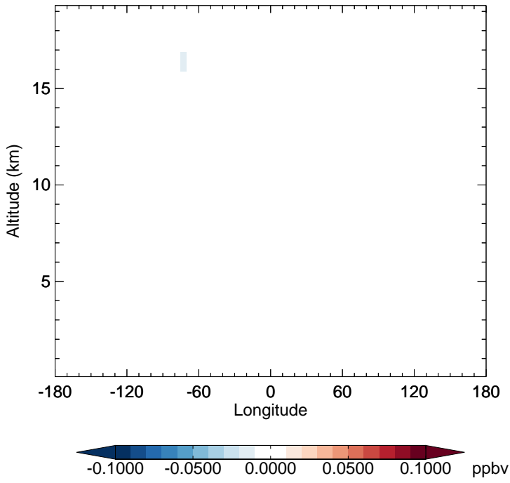
v11-02e-Run1 - v11-02e-Run0 HOCl - Diff along 15S for Oct
