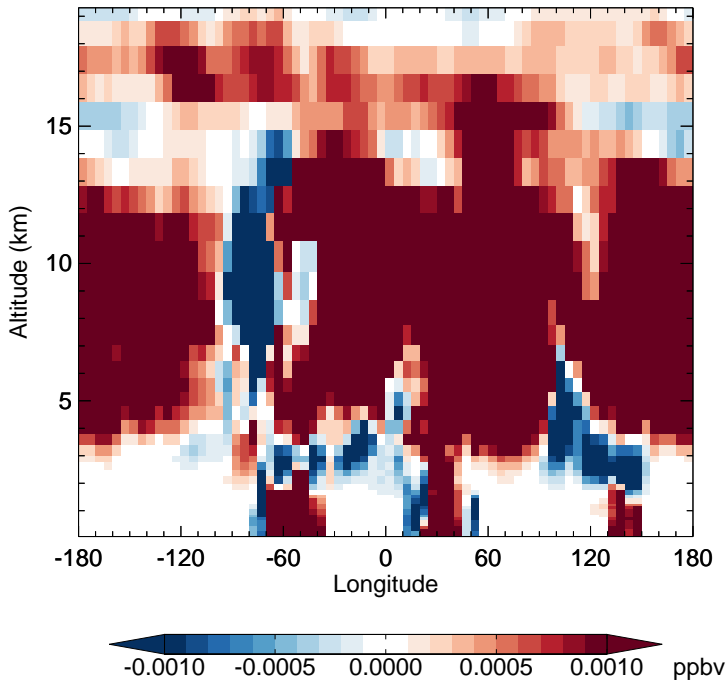
v11-02e-Run1 - v11-02e-Run0 PPN - Diff along 15S for Oct
