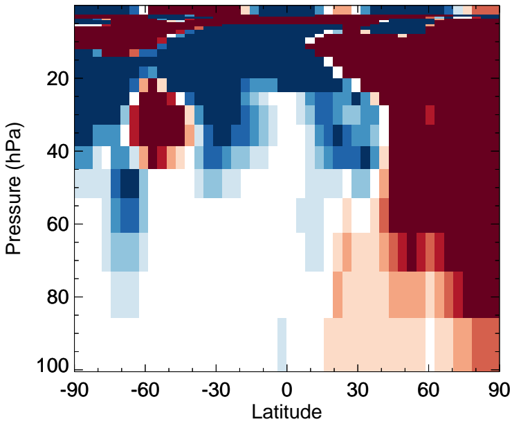
v11-02e-Run1 - v11-02e-Run0 O3 - Strat zonal mean abs diff for Apr
