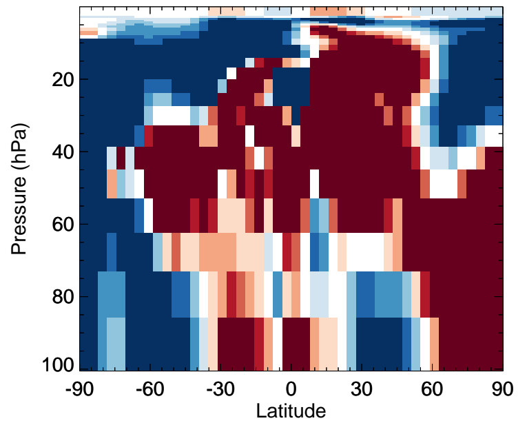
v11-02e-Run1 / v11-02e-Run0 Cl2 - Strat zonal mean % diff for Apr
