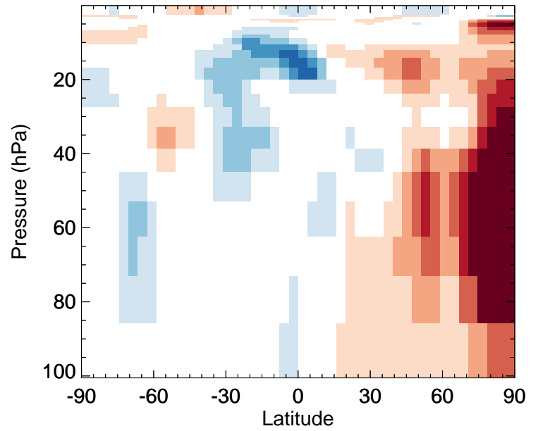
v11-02e-Run1 / v11-02e-Run0 O3 - Strat zonal mean % diff for Apr
