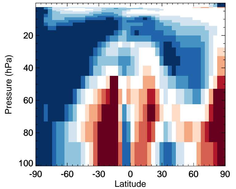
BrNO3 - Strat zonal mean % diff for Apr
