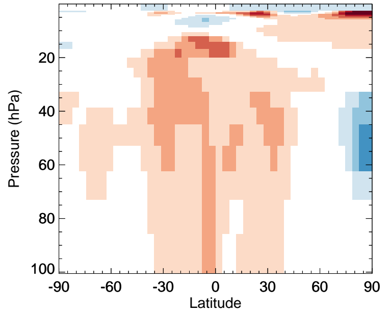
v11-02e-Run1 / v11-02e-Run0 CO - Strat zonal mean % diff for Apr
