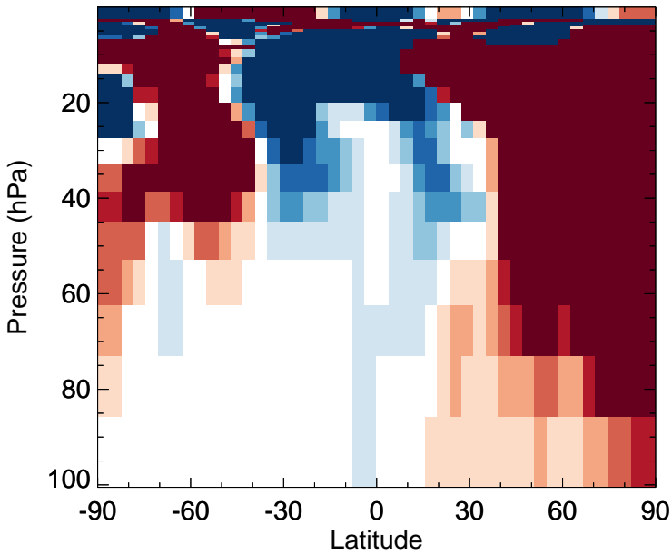
v11-02e-Run1 - v11-02d-Run1 O3 - Strat zonal mean abs diff for Apr
