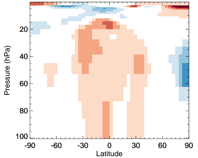
v11-02e-Run1 / v11-02d-Run1 CO - Strat zonal mean % diff for Apr
