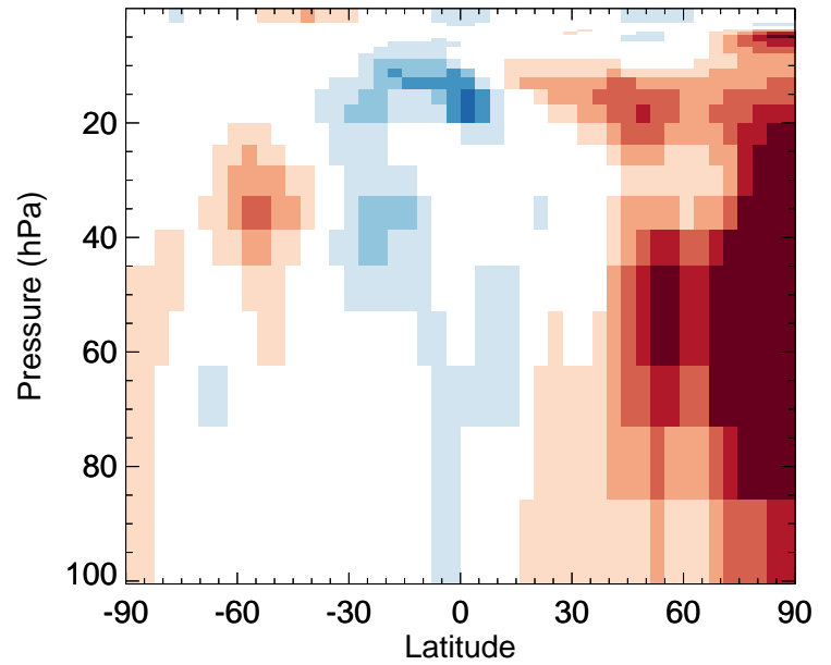
v11-02e-Run1 / v11-02d-Run1 O3 - Strat zonal mean % diff for Apr
