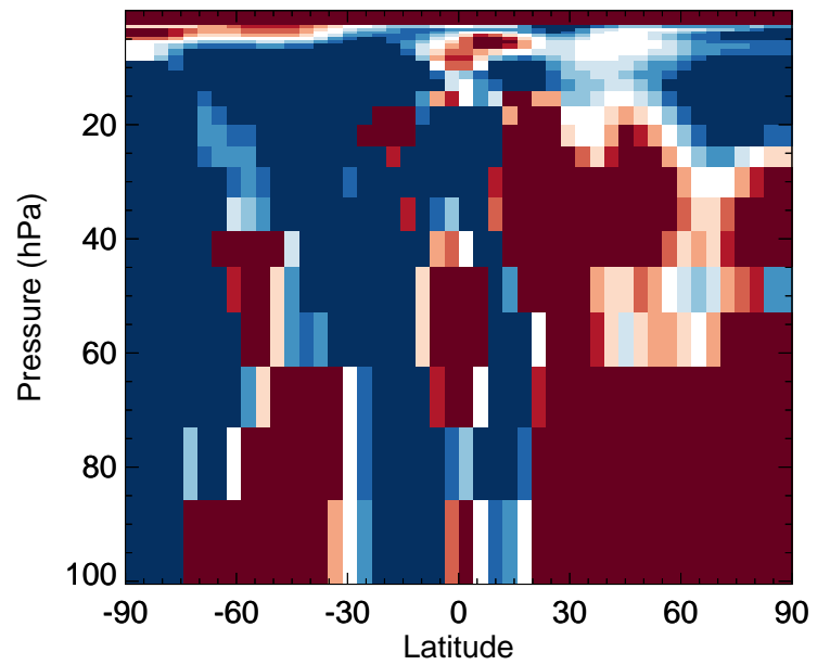
v11-02e-Run1 / v11-02d-Run1 Cl2 - Strat zonal mean % diff for Apr
