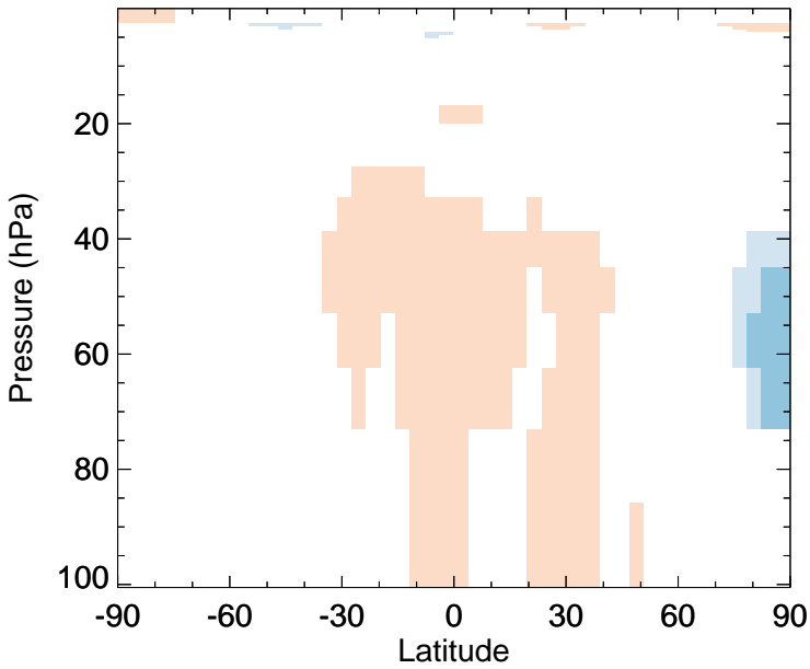
v11-02e-Run1 - v11-02d-Run1 CO - Strat zonal mean abs diff for Apr
