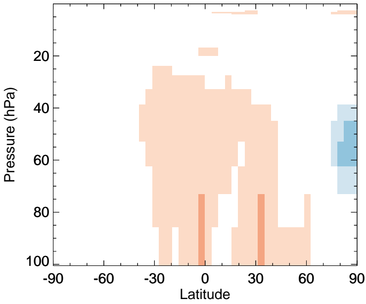
v11-02e-Run1 - v11-02e-Run0 CO - Strat zonal mean abs diff for Apr
