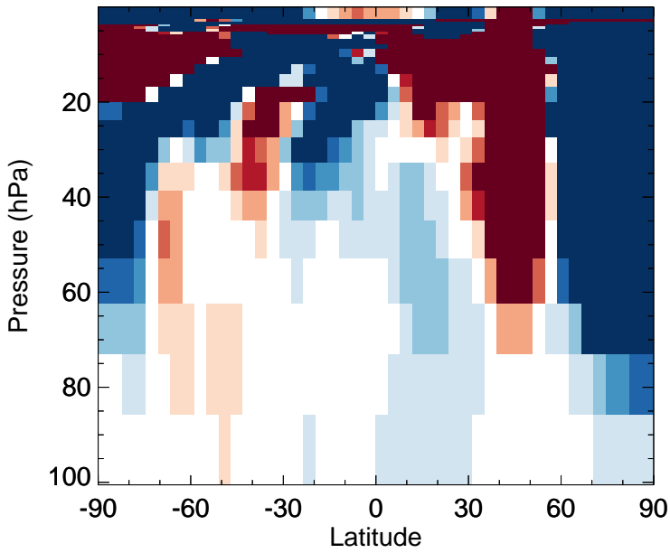
v11-02e-Run1 - v11-02e-Run0 O3 - Strat zonal mean abs diff for Jan
