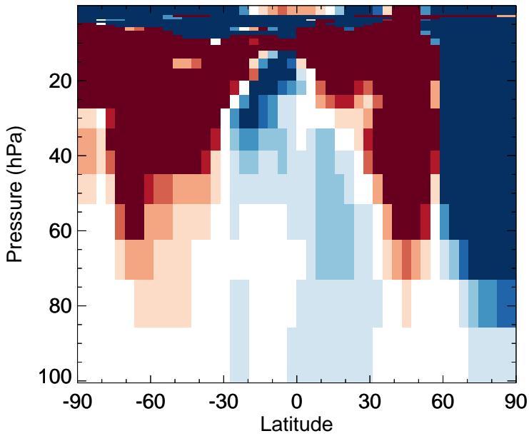
v11-02e-Run1 - v11-02d-Run1 O3 - Strat zonal mean abs diff for Jan
