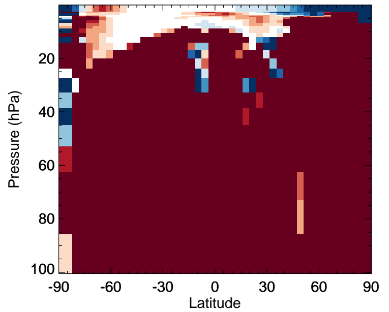
RIPD - Strat zonal mean % diff for Jan
