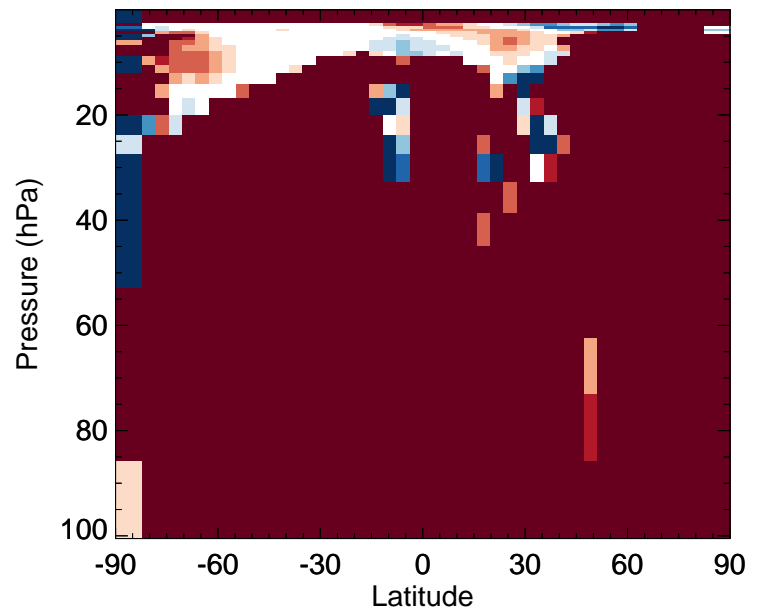
RIPB - Strat zonal mean % diff for Jan
