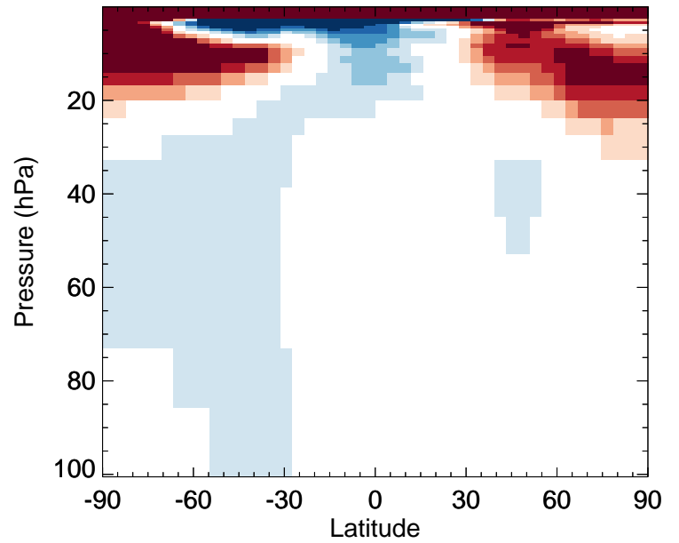
CH3Cl - Strat zonal mean % diff for Jan
