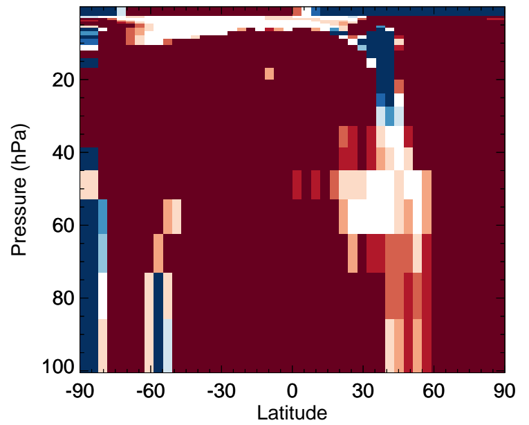
PRPE - Strat zonal mean % diff for Jan
