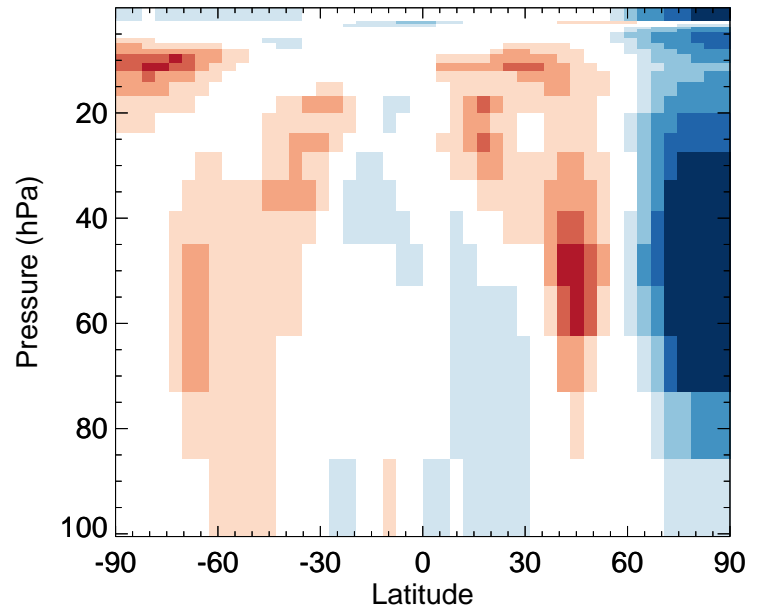
v11-02e-Run1 / v11-02d-Run1 O3 - Strat zonal mean % diff for Jan
