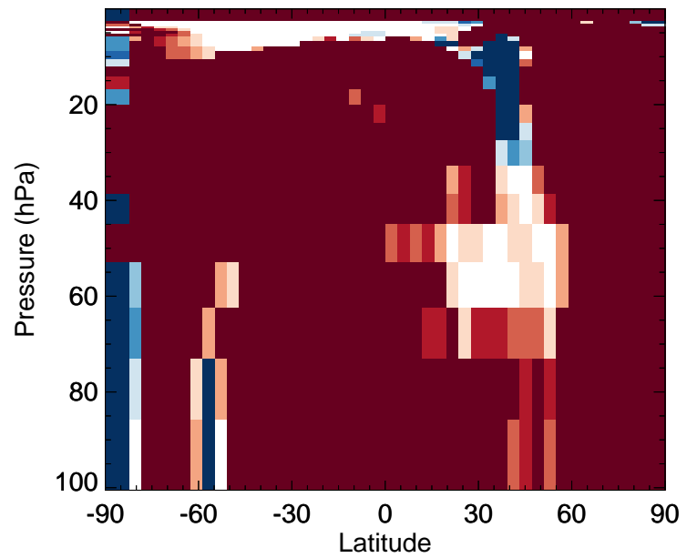
PRPE - Strat zonal mean % diff for Jan
