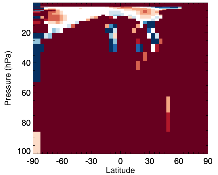
RIPD - Strat zonal mean % diff for Jan
