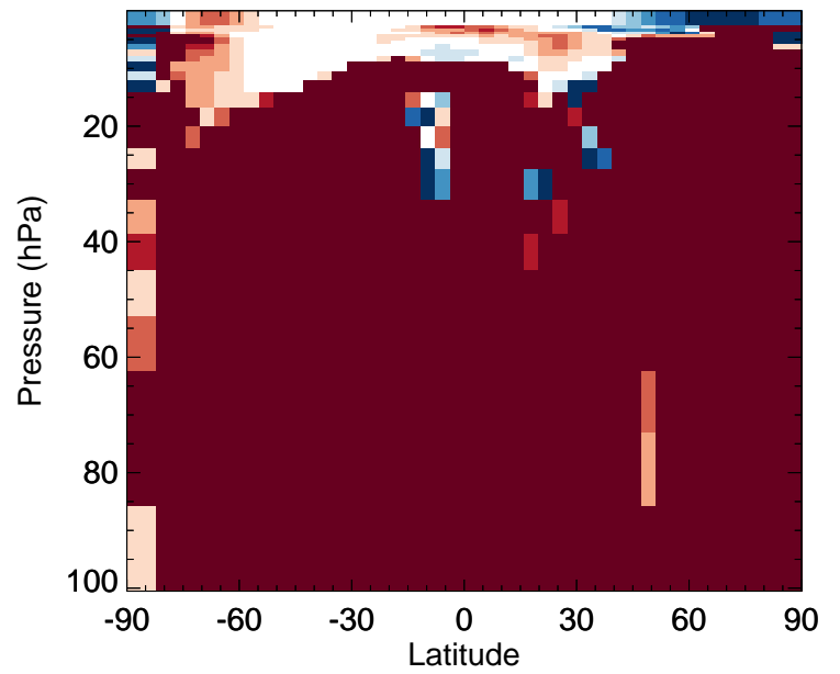
RIPB - Strat zonal mean % diff for Jan
