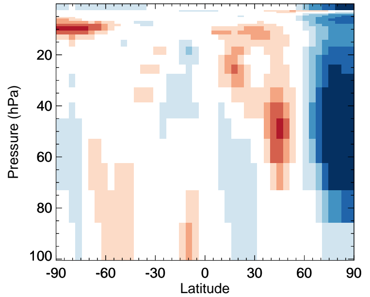
v11-02e-Run1 / v11-02e-Run0 O3 - Strat zonal mean % diff for Jan
