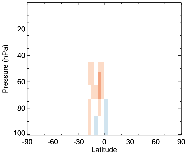
PRPE - Strat zonal mean abs diff for Jan
