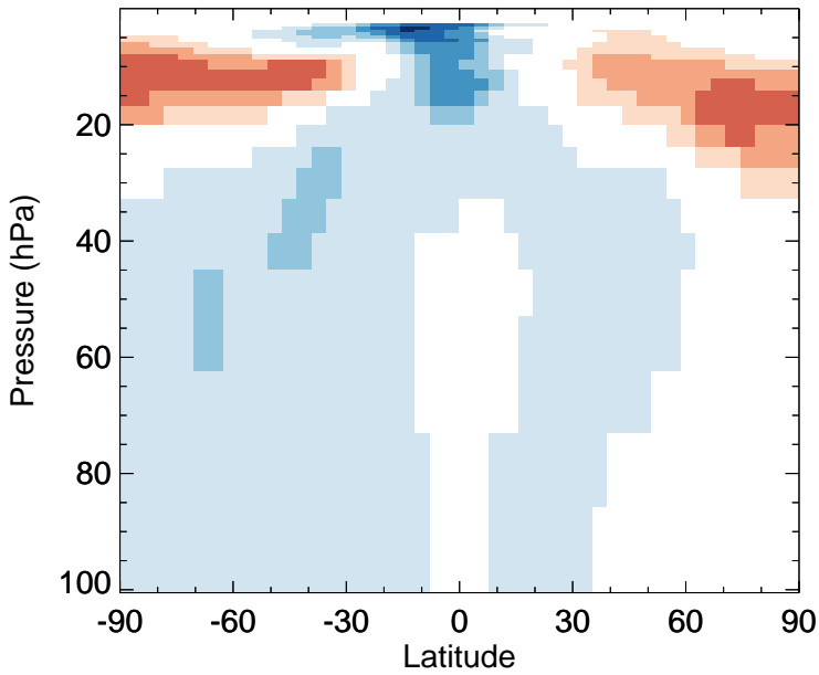
CH3Cl - Strat zonal mean abs diff for Jan
