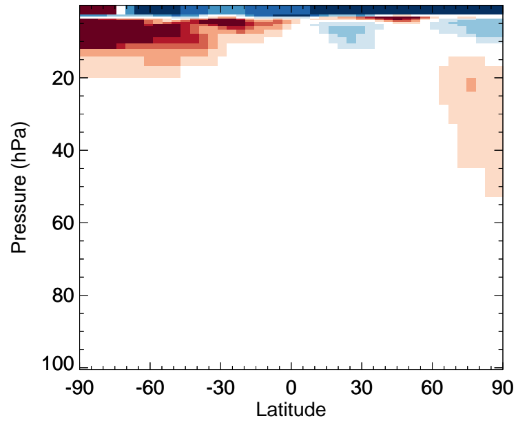
CH3Cl - Strat zonal mean % diff for Jan
