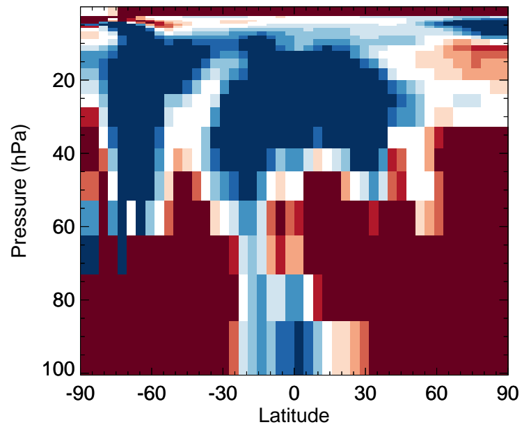
v11-02e-Run1 / v11-02d-Run1 ClO - Strat zonal mean % diff for Jul
