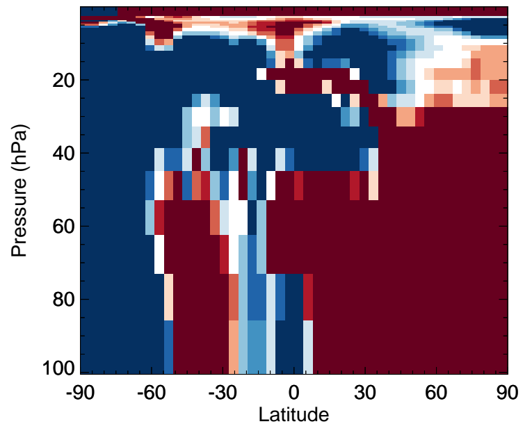
v11-02e-Run1 / v11-02d-Run1 Cl2 - Strat zonal mean % diff for Jul
