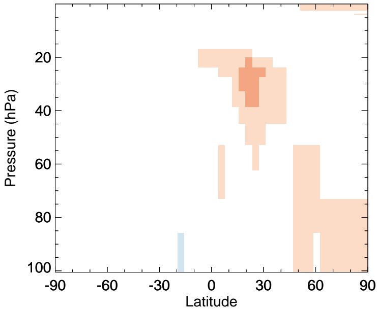
v11-02e-Run1 - v11-02d-Run1 CO - Strat zonal mean abs diff for Jul
