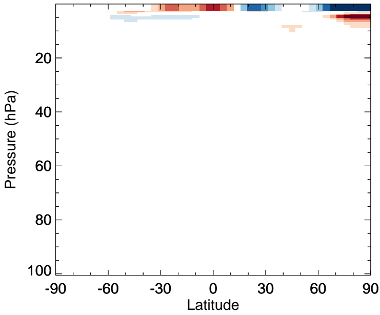
v11-02e-Run1 - v11-02e-Run0 NO - Strat zonal mean abs diff for Jul
