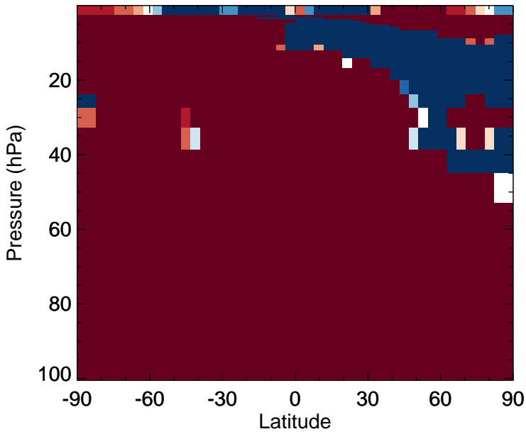
N2O - Strat zonal mean abs diff for Jul
