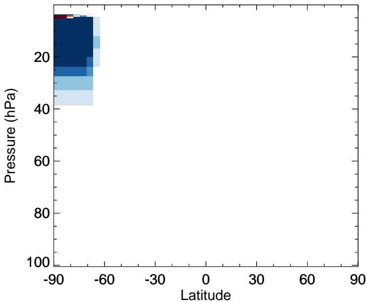
v11-02e-Run1 - v11-02d-Run1 Cl2 - Strat zonal mean abs diff for Jul
