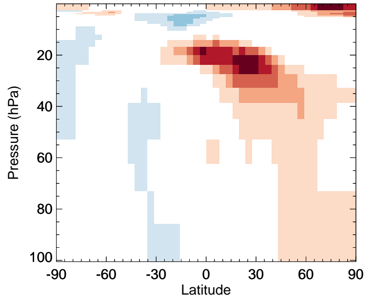
v11-02e-Run1 / v11-02d-Run1 CO - Strat zonal mean % diff for Jul
