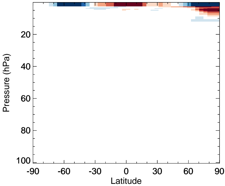
v11-02e-Run1 - v11-02d-Run1 NO - Strat zonal mean abs diff for Jul
