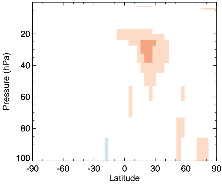
v11-02e-Run1 - v11-02e-Run0 CO - Strat zonal mean abs diff for Jul
