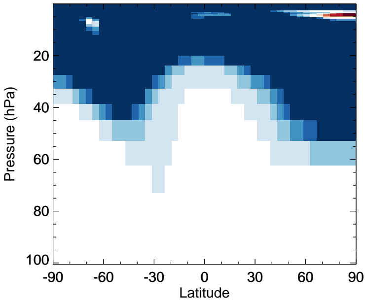
v11-02e-Run1 - v11-02d-Run1 HCl - Strat zonal mean abs diff for Jul
