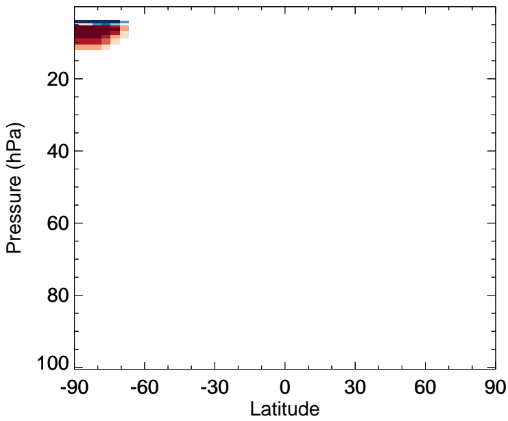
v11-02e-Run1 - v11-02e-Run0 Cl2 - Strat zonal mean abs diff for Jul
