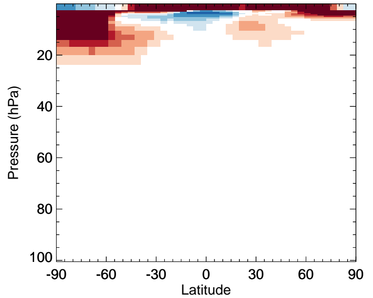
N2O - Strat zonal mean % diff for Jul
