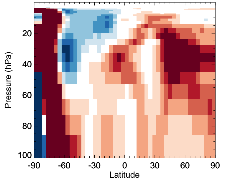
v11-02e-Run1 / v11-02e-Run0 HCl - Strat zonal mean % diff for Jul
