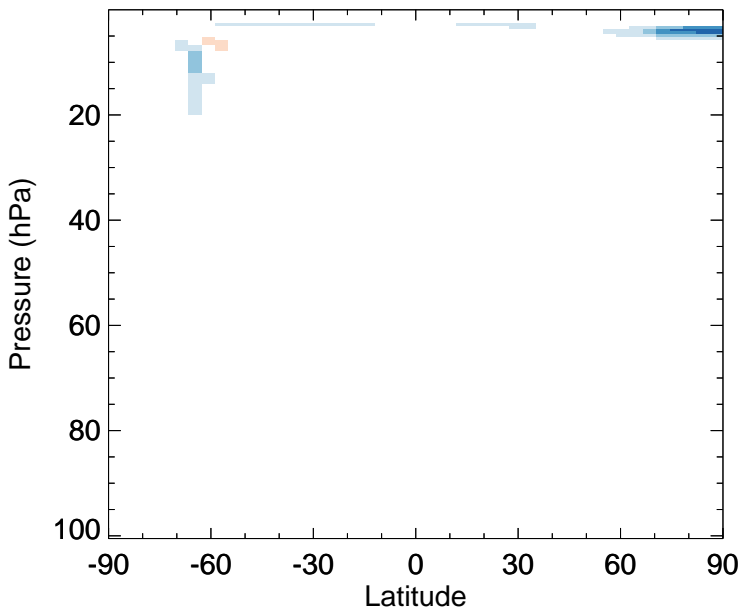
v11-02e-Run1 - v11-02e-Run0 ClO - Strat zonal mean abs diff for Jul
