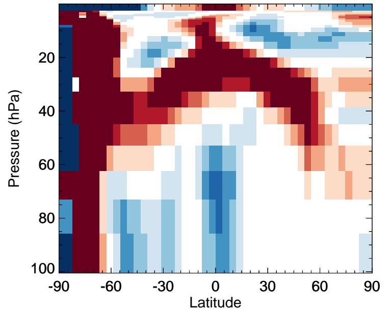
v11-02e-Run1 / v11-02d-Run1 NO - Strat zonal mean % diff for Jul
