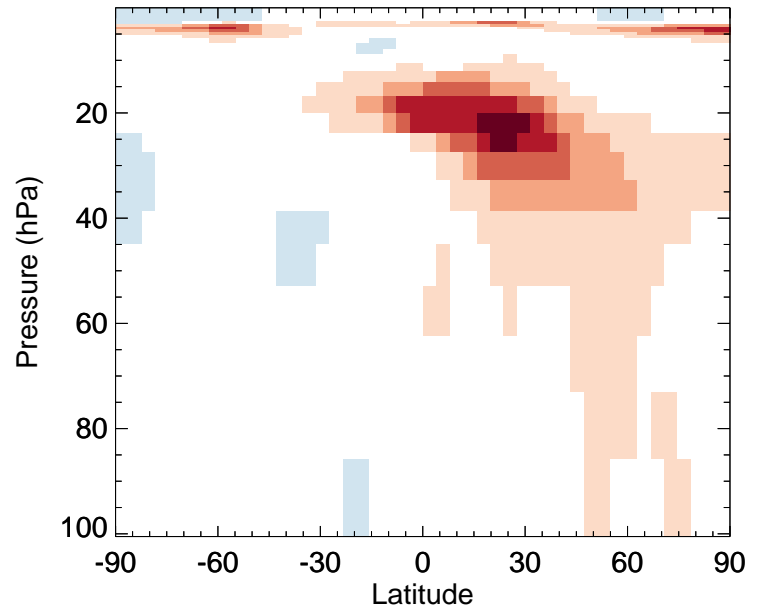
v11-02e-Run1 / v11-02e-Run0 CO - Strat zonal mean % diff for Jul
