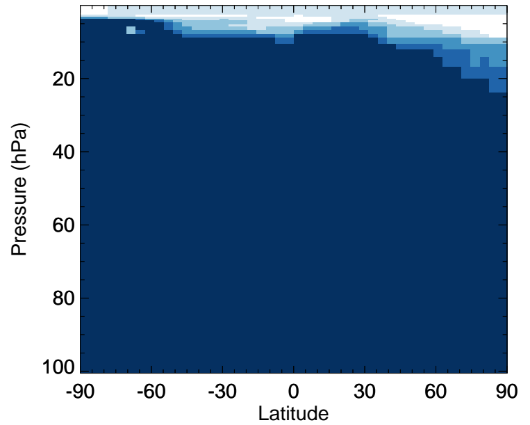
v11-02e-Run1 / v11-02d-Run1 HCl - Strat zonal mean % diff for Jul
