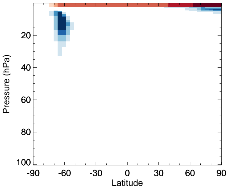
v11-02e-Run1 - v11-02d-Run1 ClO - Strat zonal mean abs diff for Jul
