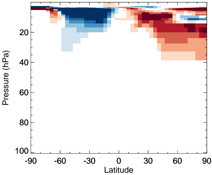
v11-02e-Run1 - v11-02e-Run0 HCl - Strat zonal mean abs diff for Jul
