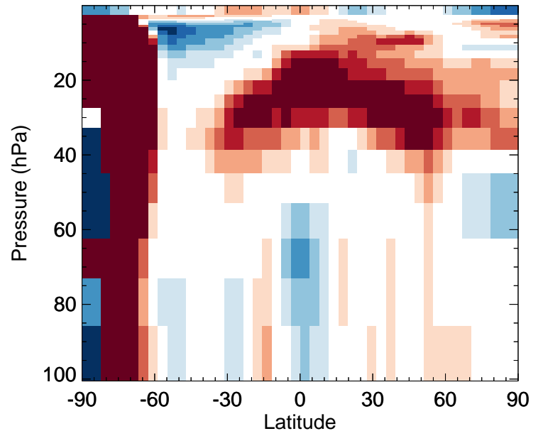
v11-02e-Run1 / v11-02e-Run0 NO - Strat zonal mean % diff for Jul
