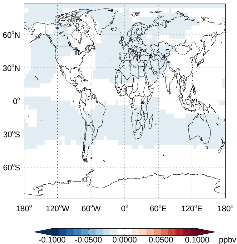
v11-02e-Run1 - v11-02d-Run1 HCFC141b- Diff @ 500 hPa for Jul
