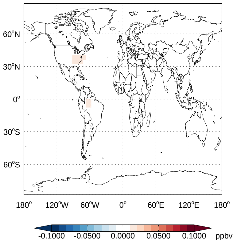
v11-02e-Run1 - v11-02d-Run1 LVOCOA - Diff @ Surface for Jul
