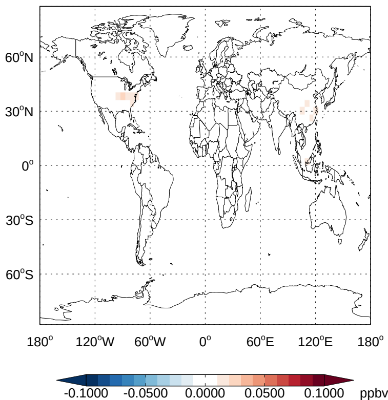
v11-02e-Run1 - v11-02d-Run1 PROPNN - Diff @ Surface for Jul
