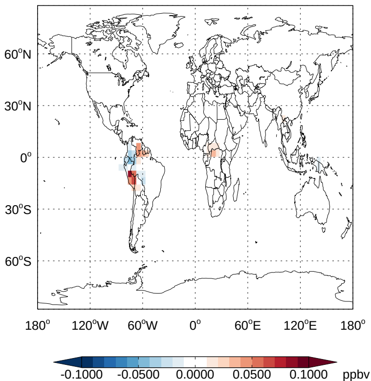
v11-02e-Run1 - v11-02d-Run1 IEPOXA- Diff @ 500 hPa for Oct
