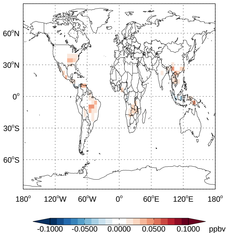
v11-02e-Run1 - v11-02d-Run1 MONITA - Diff @ Surface for Oct
