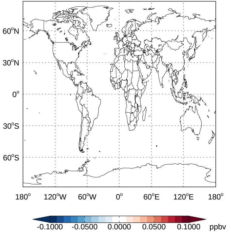
v11-02e-Run1 - v11-02d-Run1 CFC115- Diff @ 500 hPa for Oct
