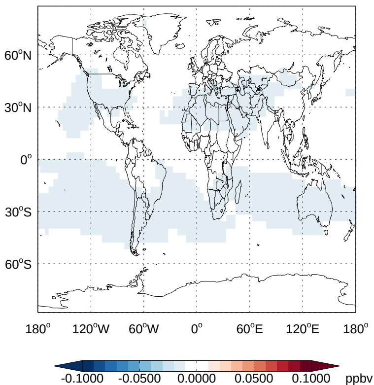
v11-02e-Run1 - v11-02d-Run1 HCFC141b- Diff @ 500 hPa for Oct
