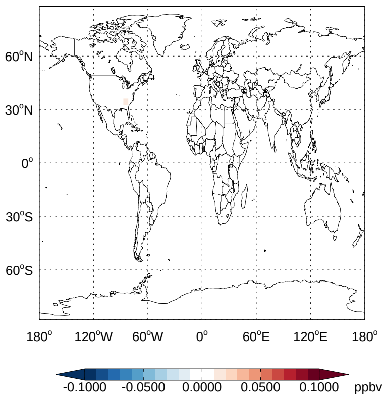
v11-02e-Run1 - v11-02d-Run1 MONITS - Diff @ Surface for Oct
