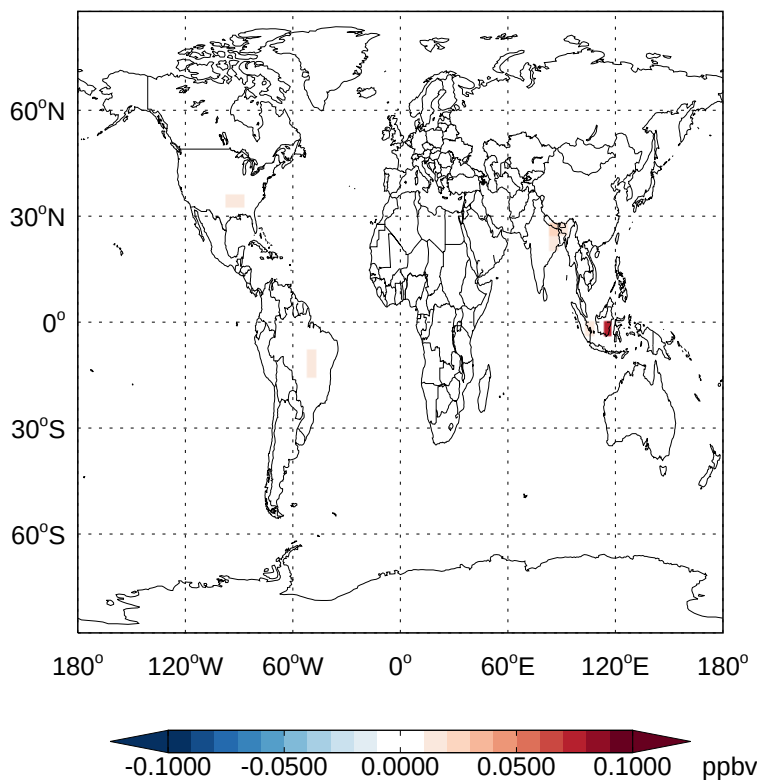
v11-02e-Run1 - v11-02d-Run1 PROPNN - Diff @ Surface for Oct
