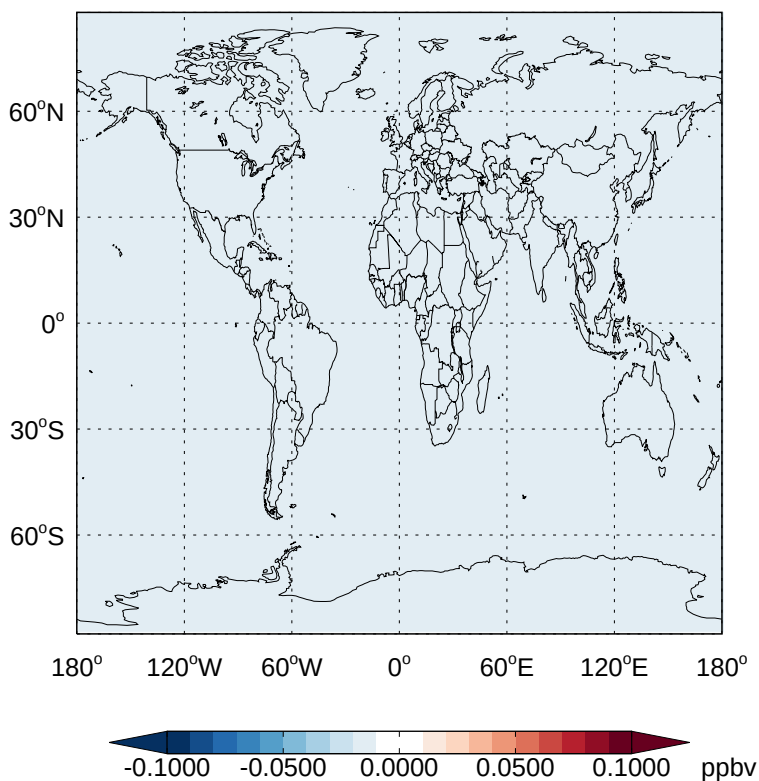
v11-02e-Run1 - v11-02d-Run1 HCFC22- Diff @ 500 hPa for Oct
