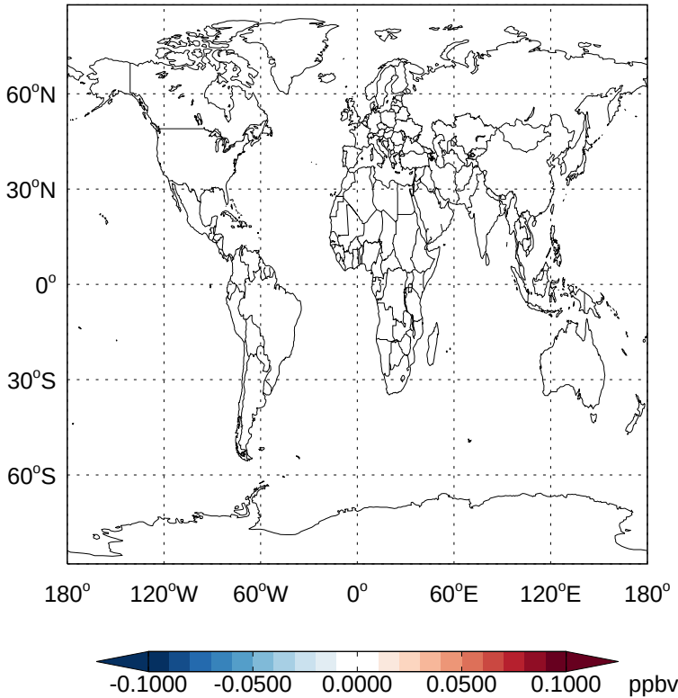
v11-02e-Run1 - v11-02d-Run1 CFC115 - Diff @ Surface for Oct
