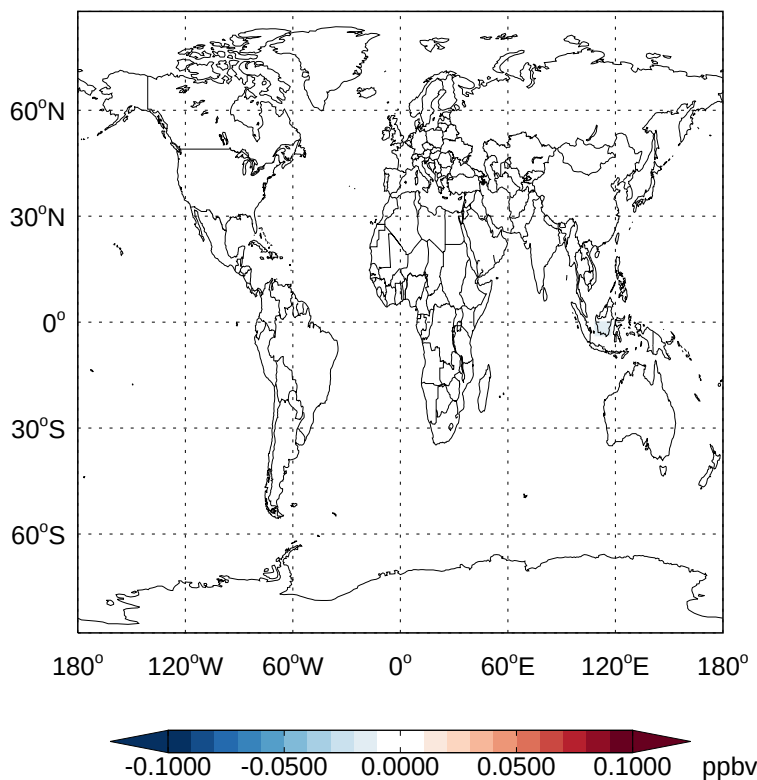
v11-02e-Run1 - v11-02d-Run1 LVOCOA - Diff @ Surface for Oct
