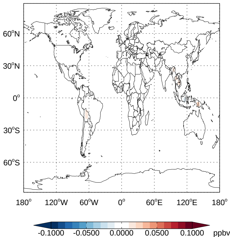
v11-02e-Run1 - v11-02d-Run1 ISOPNB - Diff @ Surface for Oct
