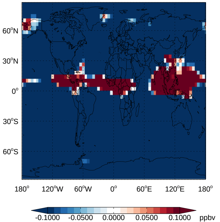
v11-02e-Run1 - v11-02d-Run1 N 2 O - Diff @ 500 hPa for Oct
