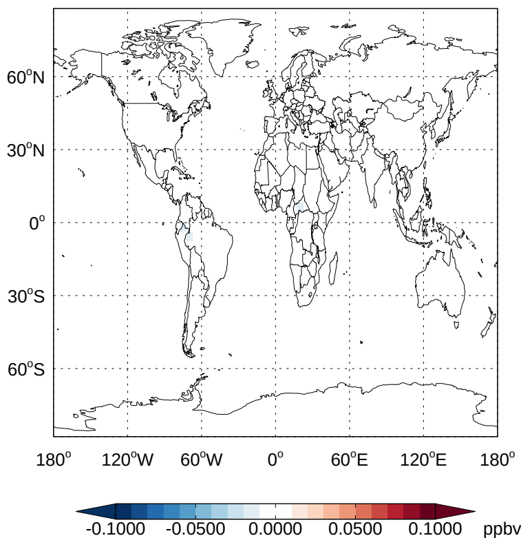
v11-02e-Run1 - v11-02d-Run1 IEPOXD - Diff @ Surface for Oct
