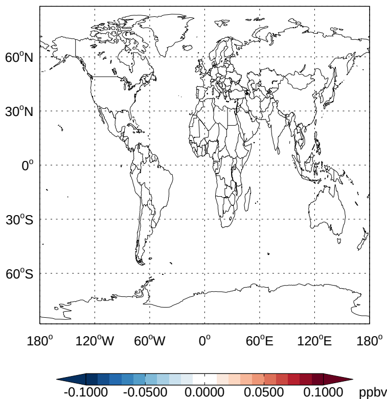
v11-02e-Run1 - v11-02d-Run1 ISN1OG - Diff @ Surface for Oct
