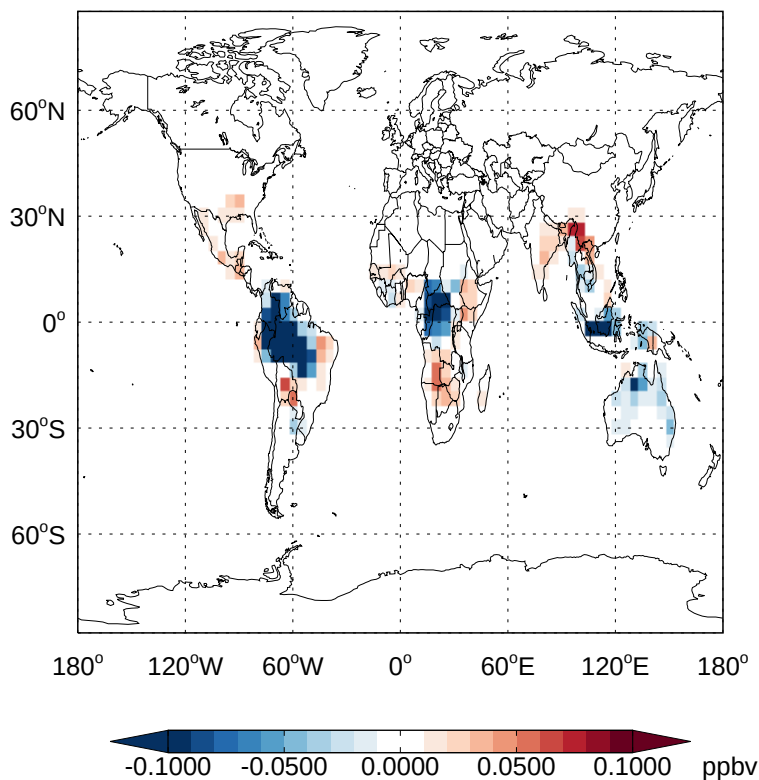
v11-02e-Run1 - v11-02d-Run1 IEPOXA - Diff @ Surface for Oct
