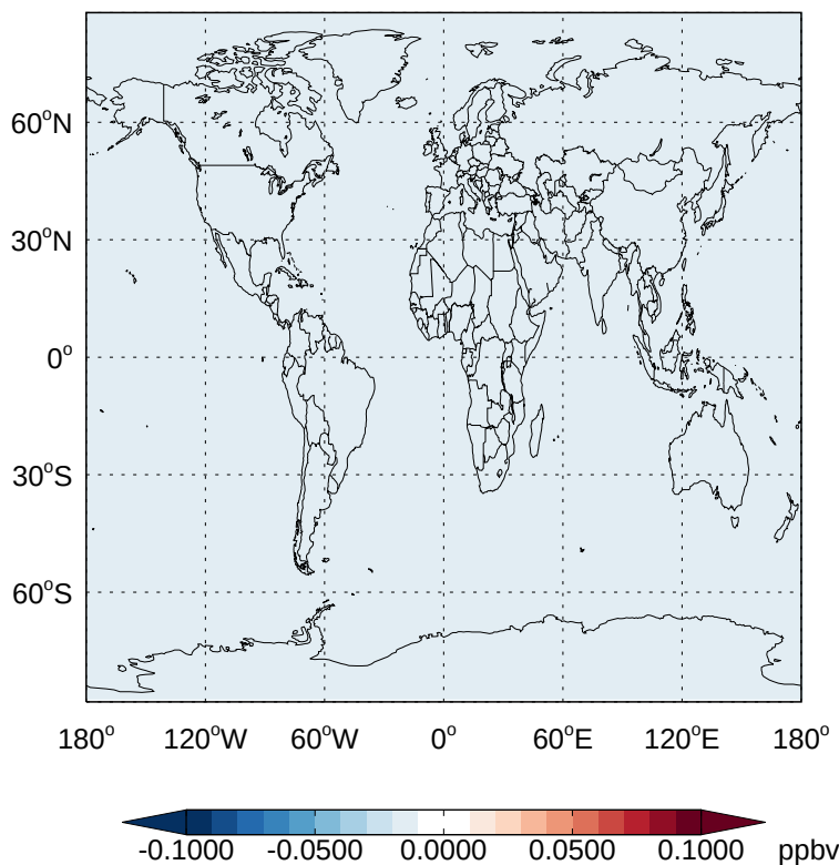
v11-02e-Run1 - v11-02d-Run1 HCFC22 - Diff @ Surface for Oct
