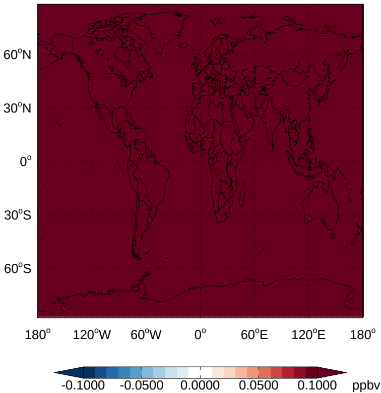
v11-02e-Run1 - v11-02d-Run1 N 2 O - Diff @ Surface for Oct
