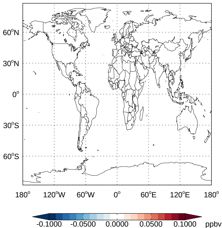
v11-02e-Run1 - v11-02d-Run1 HCFC142b - Diff @ Surface for Oct
