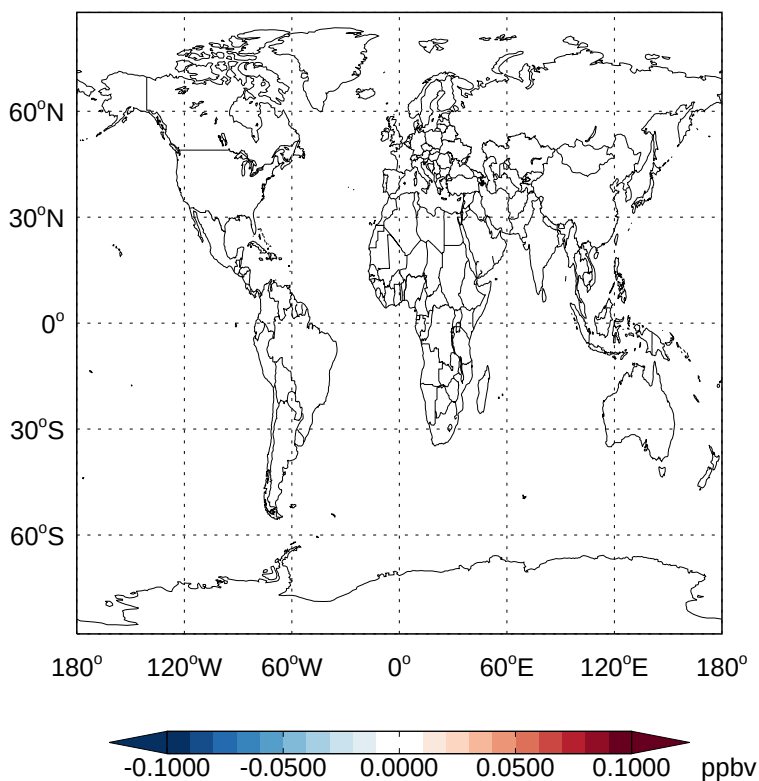
v11-02e-Run1 - v11-02d-Run1 LVOCOA- Diff @ 500 hPa for Oct
