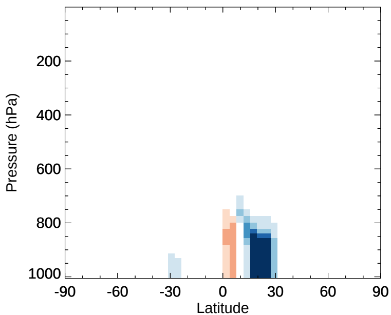
v11-02e-Run1 - v11-02e-Run0 DST2 - Zonal mean abs diff for Jan
