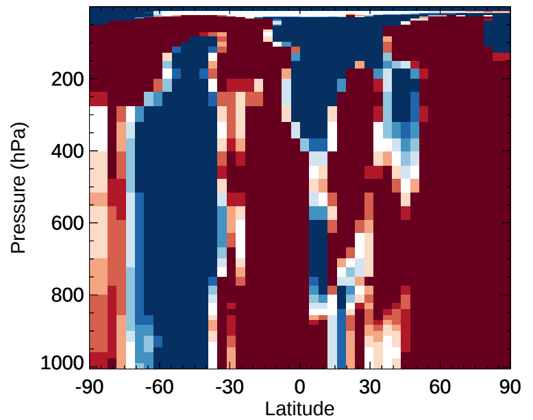
v11-02e-Run1 / v11-02d-Run1 DST4 - Zonal mean % diff for Jan
