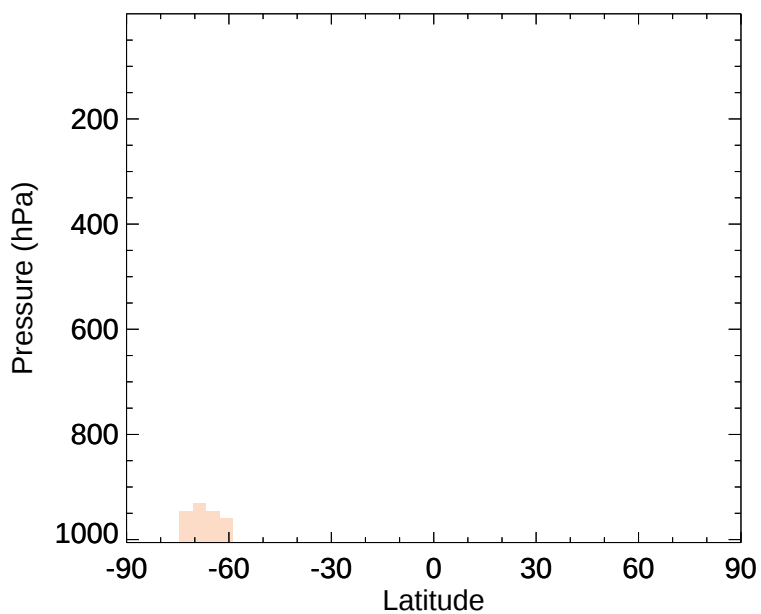
v11-02e-Run1 - v11-02e-Run0 DMS - Zonal mean abs diff for Jan
