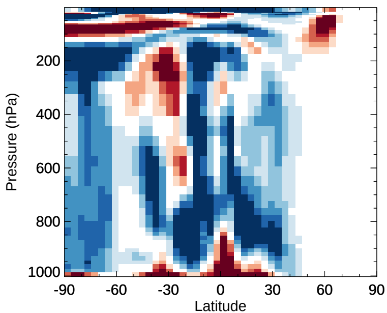
v11-02e-Run1 - v11-02d-Run1 OH - Zonal mean abs diff for Jan
