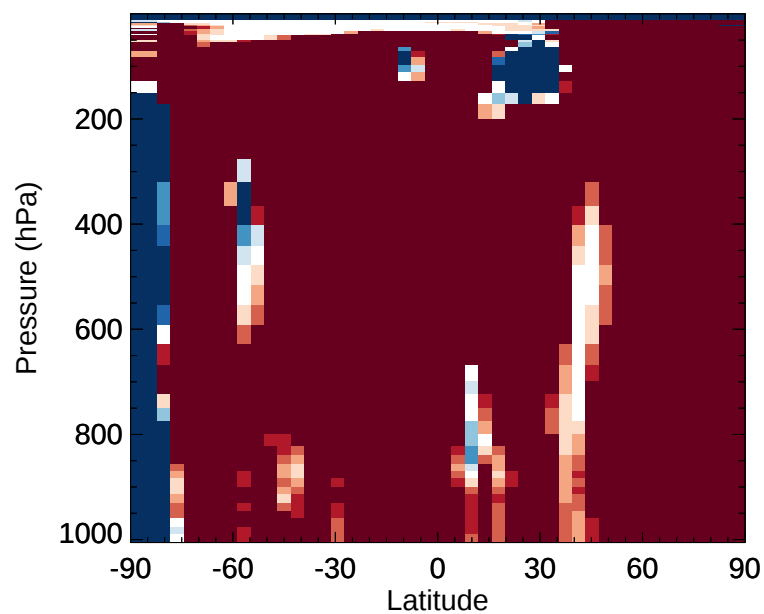
v11-02e-Run1 / v11-02e-Run0 MVK - Zonal mean % diff for Jan
