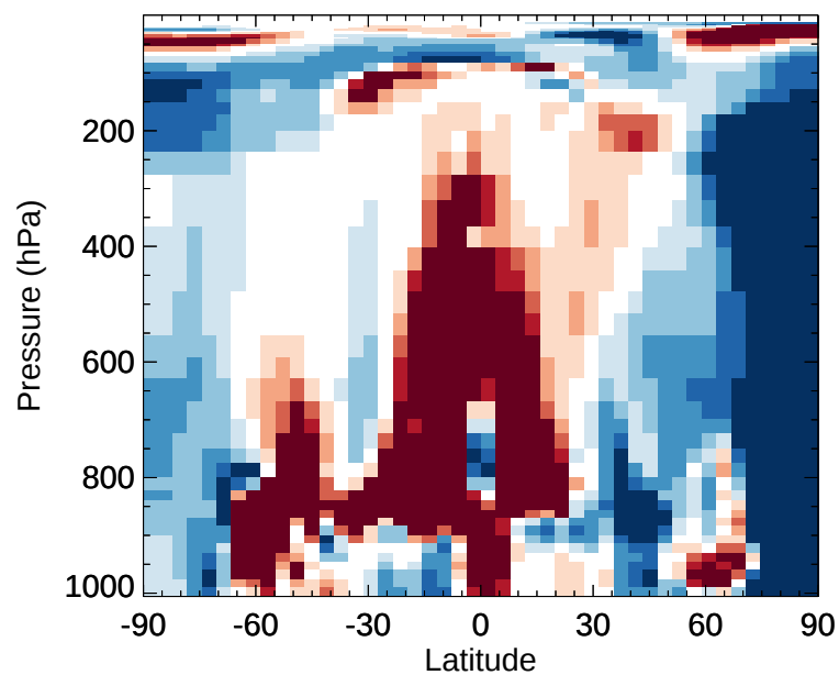
v11-02e-Run1 / v11-02e-Run0 HOBr - Zonal mean % diff for Jan
