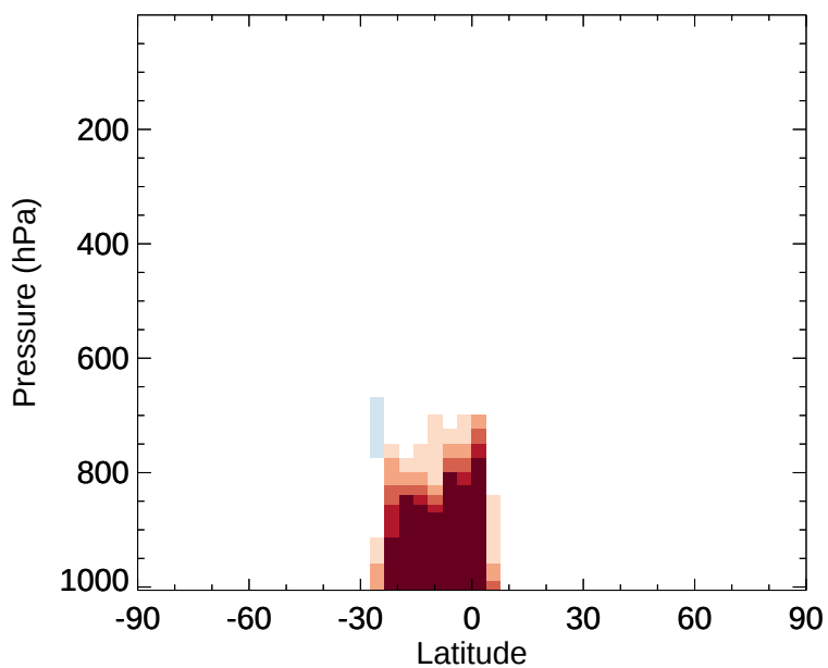
v11-02e-Run1 - v11-02e-Run0 ISOP - Zonal mean abs diff for Jan
