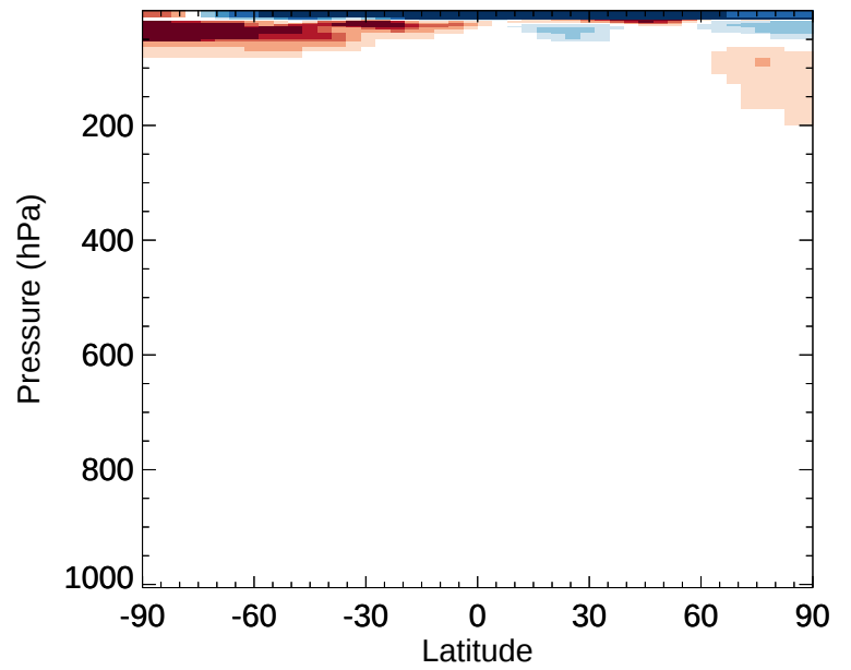
v11-02e-Run1 / v11-02e-Run0 CH3Cl - Zonal mean % diff for Jan
