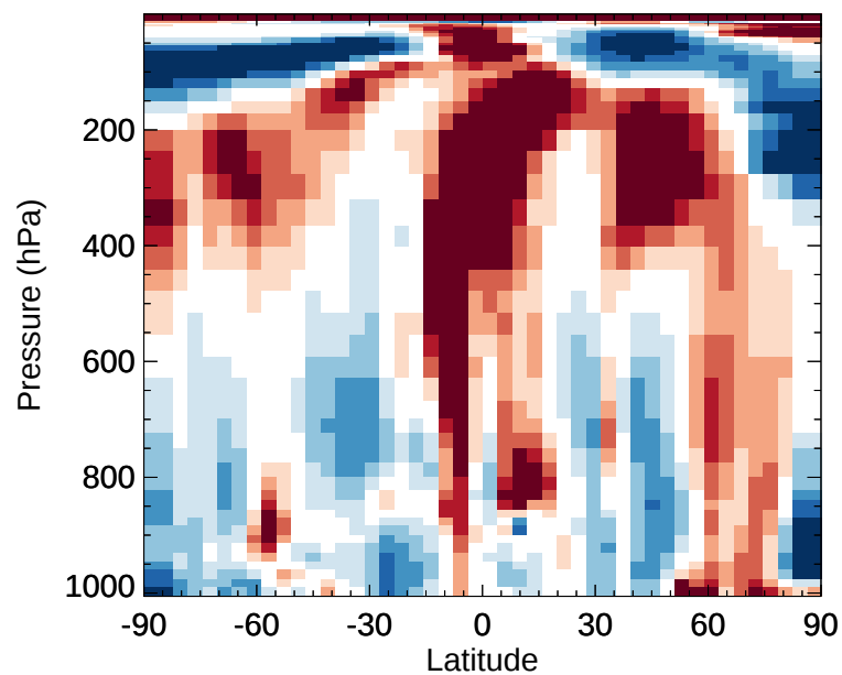
v11-02e-Run1 / v11-02d-Run1 HNO 3 - Zonal mean % diff for Jan
