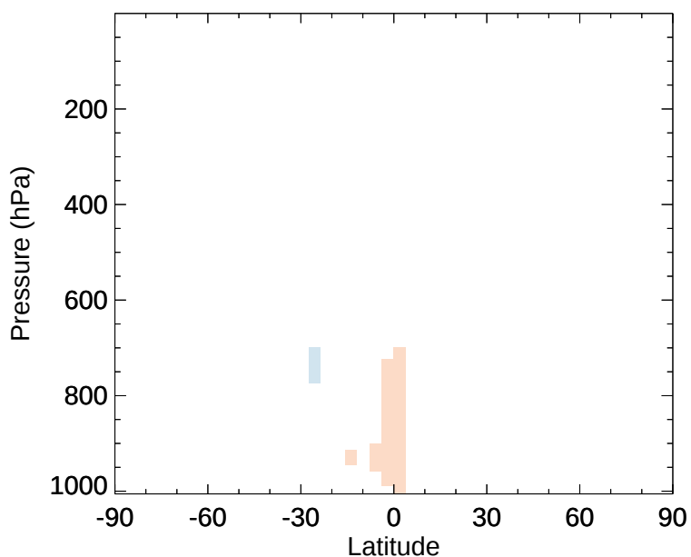
v11-02e-Run1 - v11-02d-Run1 GLYC - Zonal mean abs diff for Jan
