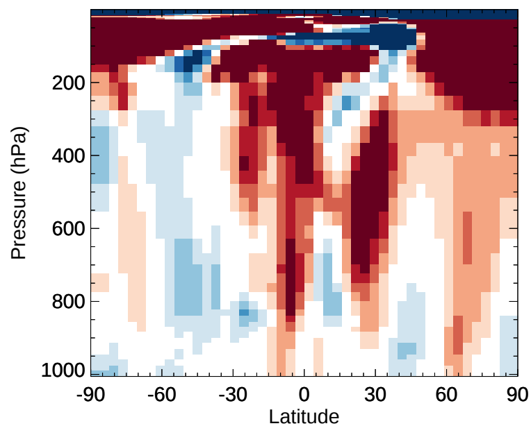
v11-02e-Run1 / v11-02e-Run0 MAP - Zonal mean % diff for Jan
