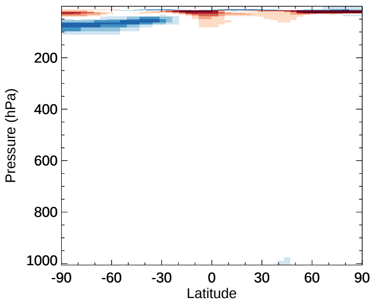
v11-02e-Run1 - v11-02d-Run1 NO2 - Zonal mean abs diff for Jan
