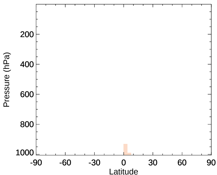
v11-02e-Run1 - v11-02d-Run1 CH 2 O - Zonal mean abs diff for Jan
