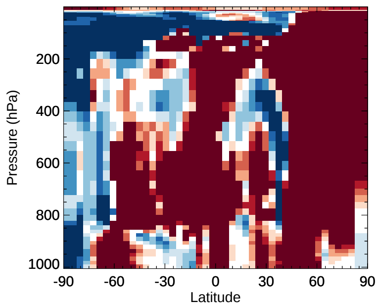
v11-02e-Run1 / v11-02e-Run0 Cl2 - Zonal mean % diff for Jan
