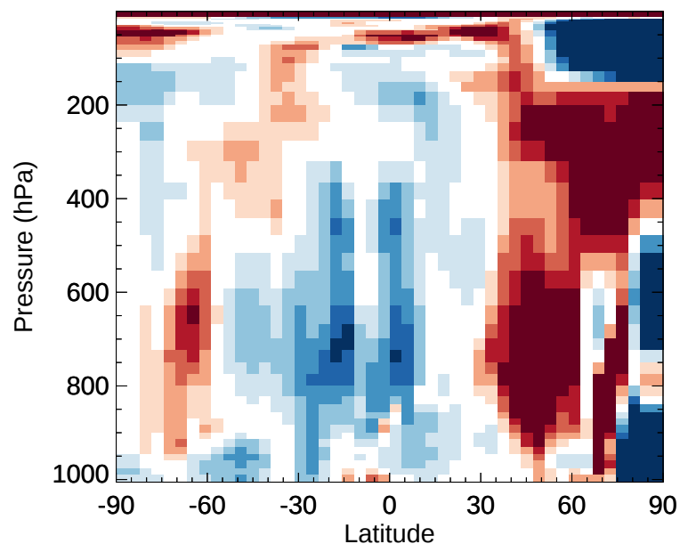
v11-02e-Run1 / v11-02d-Run1 HNO 4 - Zonal mean % diff for Jan
