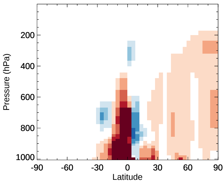
v11-02e-Run1 - v11-02e-Run0 MEK - Zonal mean abs diff for Jan
