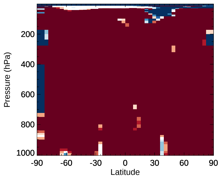
v11-02e-Run1 / v11-02e-Run0 LVOC - Zonal mean % diff for Jan
