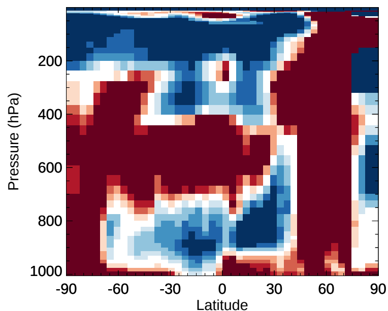
v11-02e-Run1 / v11-02d-Run1 C100 - Zonal mean % diff for Jan
