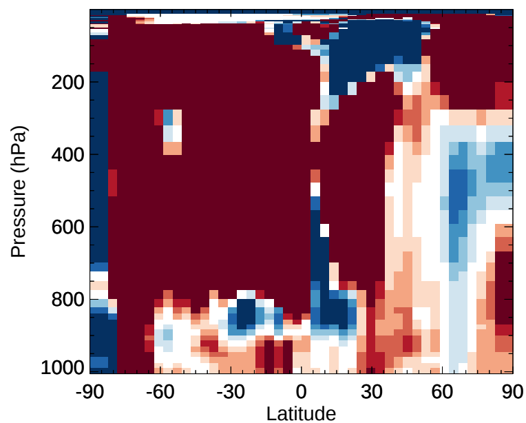
v11-02e-Run1 / v11-02e-Run0 XYLE - Zonal mean % diff for Jan
