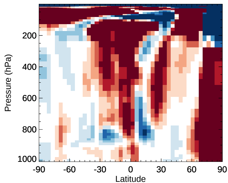
v11-02e-Run1 / v11-02e-Run0 ACTA - Zonal mean % diff for Jan
