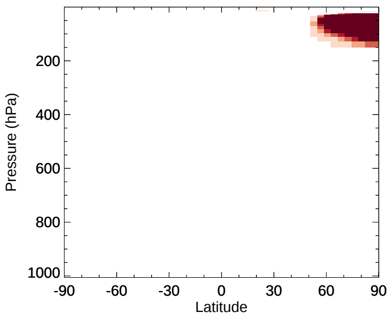
v11-02e-Run1 - v11-02e-Run0 HOCl - Zonal mean abs diff for Jan
