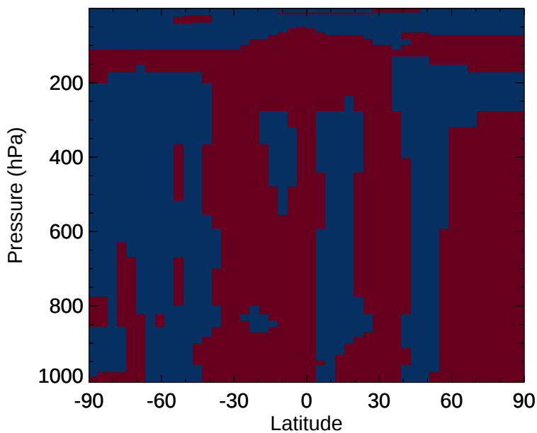
v11-02e-Run1 - v11-02e-Run0 H 2 O - Zonal mean abs diff for Jan
