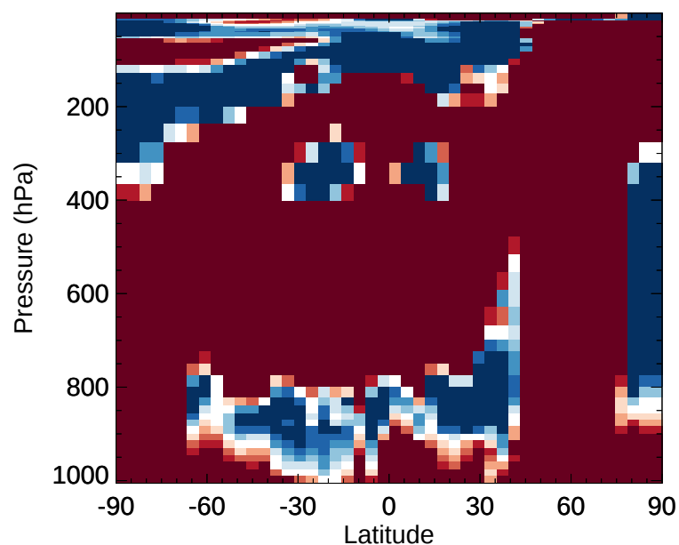
v11-02e-Run1 / v11-02d-Run1 Cl2O2 - Zonal mean % diff for Jan
