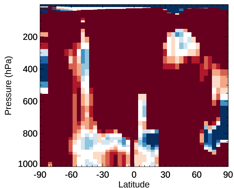
v11-02e-Run1 / v11-02d-Run1 DMS - Zonal mean % diff for Jan
