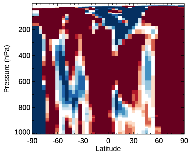
v11-02e-Run1 / v11-02e-Run0 SOAP - Zonal mean % diff for Jan
