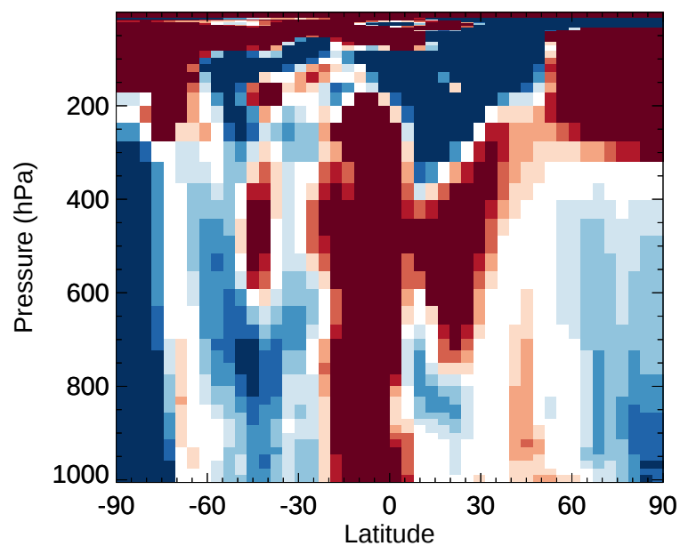
v11-02e-Run1 / v11-02e-Run0 EOH - Zonal mean % diff for Jan
