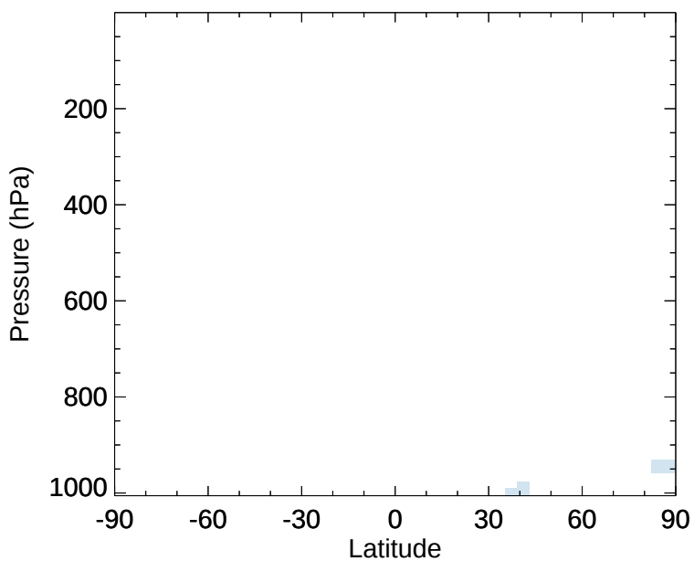
v11-02e-Run1 - v11-02e-Run0 SO 2 - Zonal mean abs diff for Jan
