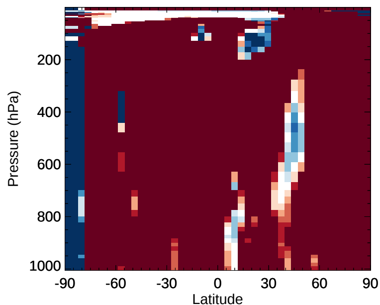
v11-02e-Run1 / v11-02d-Run1 ISN1 - Zonal mean % diff for Jan
