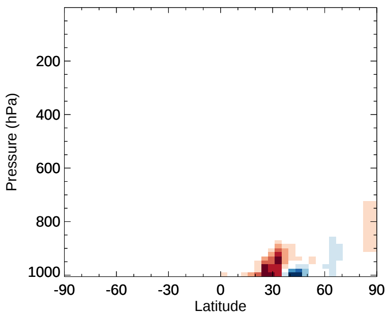
v11-02e-Run1 - v11-02d-Run1 XYLE - Zonal mean abs diff for Jan
