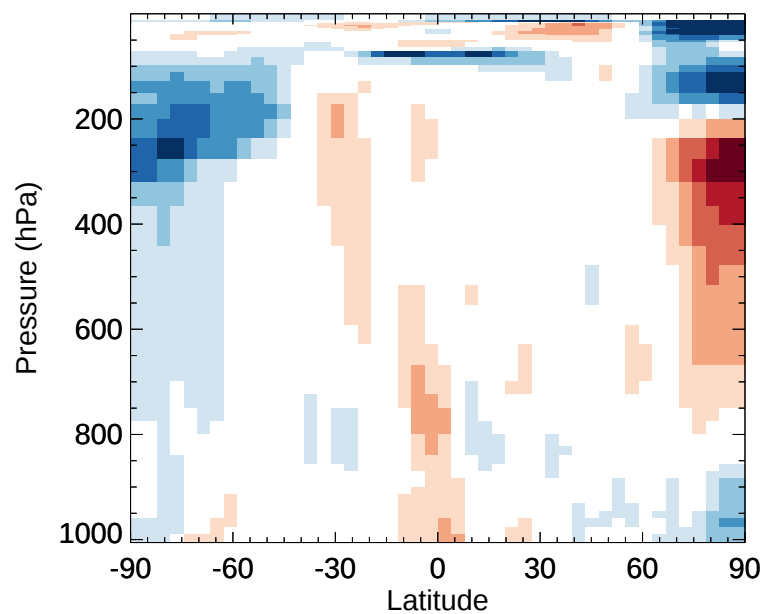
v11-02e-Run1 / v11-02e-Run0 CH 2 O - Zonal mean % diff for Jan
