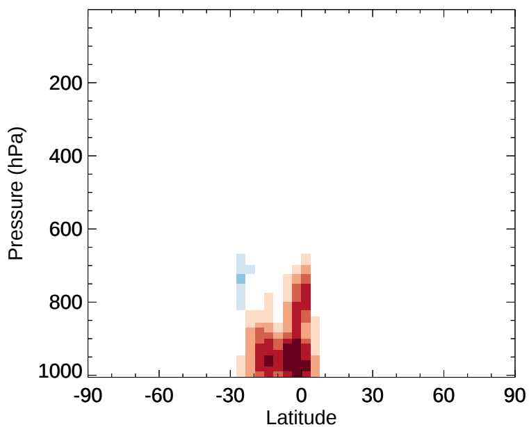
v11-02e-Run1 - v11-02e-Run0 MVK - Zonal mean abs diff for Jan
