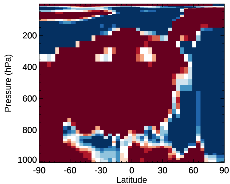
v11-02e-Run1 / v11-02d-Run1 OCIO - Zonal mean % diff for Jan
