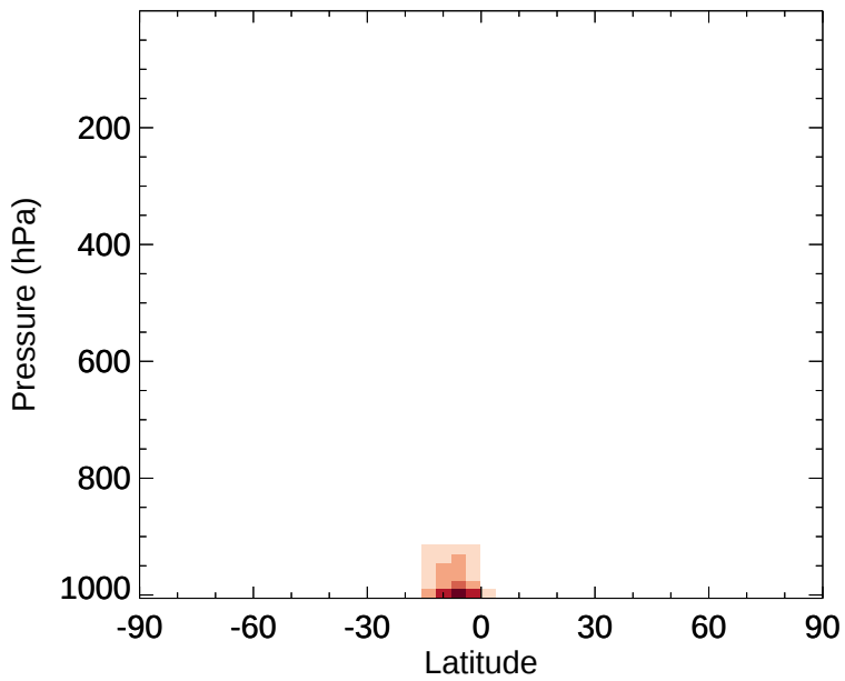
v11-02e-Run1 - v11-02d-Run1 MTPA - Zonal mean abs diff for Jan
