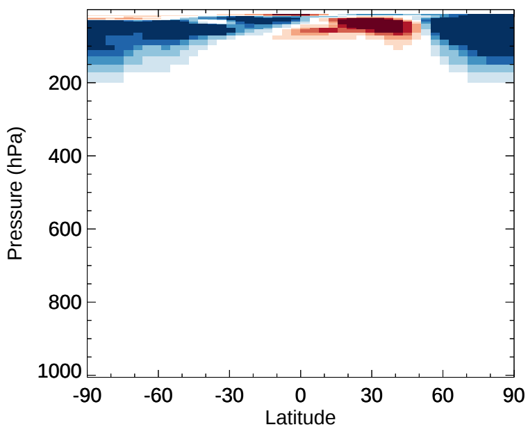
v11-02e-Run1 - v11-02e-Run0 HCl - Zonal mean abs diff for Jan
