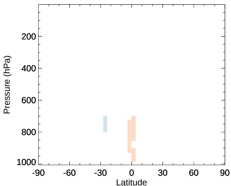
v11-02e-Run1 - v11-02d-Run1 HAC - Zonal mean abs diff for Jan
