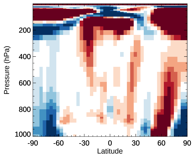
v11-02e-Run1 / v11-02d-Run1 H2O2 - Zonal mean % diff for Jan
