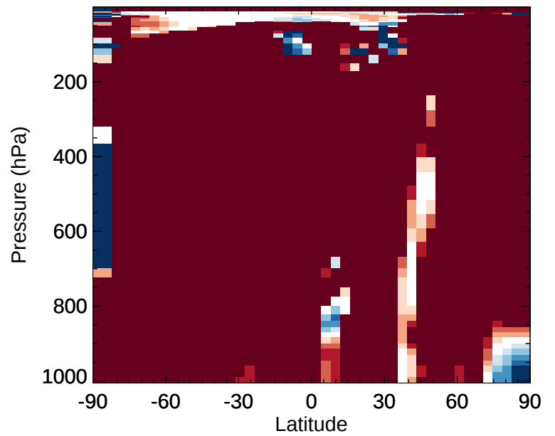
v11-02e-Run1 / v11-02d-Run1 RIPA - Zonal mean % diff for Jan
