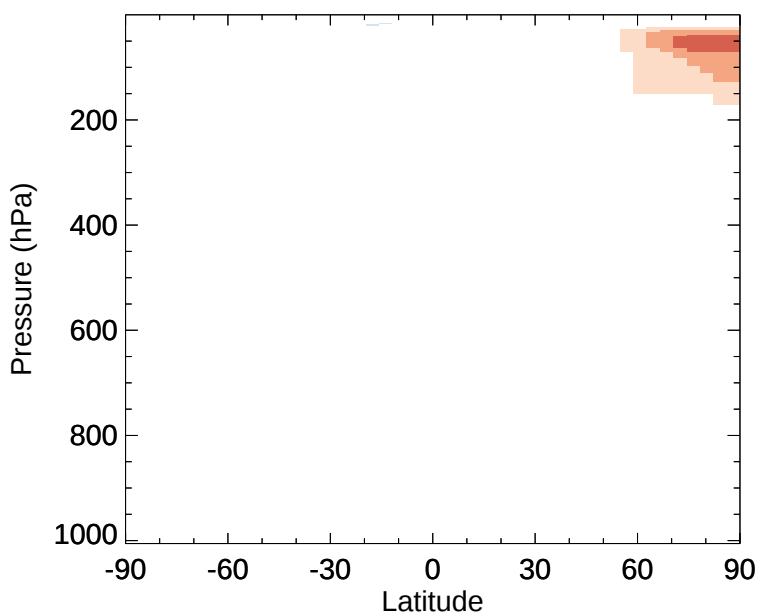
v11-02e-Run1 - v11-02d-Run1 MPN - Zonal mean abs diff for Jan
