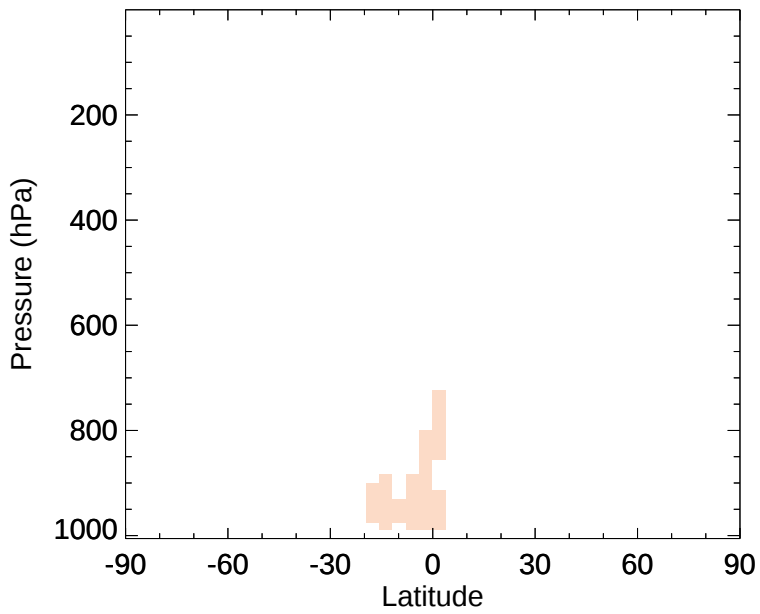
v11-02e-Run1 - v11-02e-Run0 RIPA - Zonal mean abs diff for Jan
