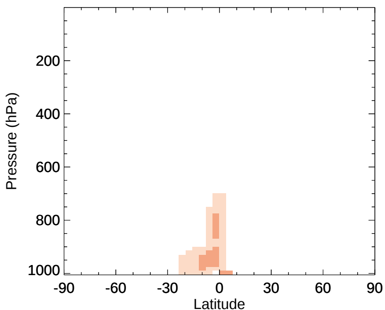
v11-02e-Run1 - v11-02d-Run1 ALD2 - Zonal mean abs diff for Jan
