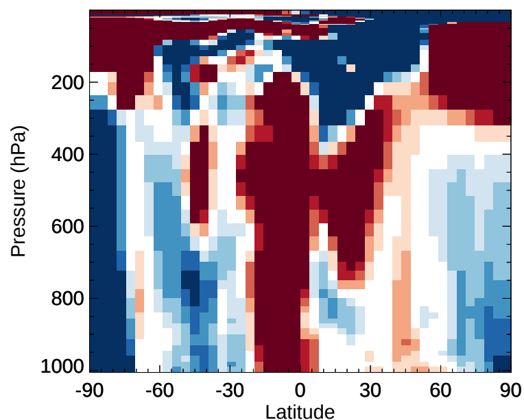
v11-02e-Run1 / v11-02d-Run1 EOH - Zonal mean % diff for Jan
