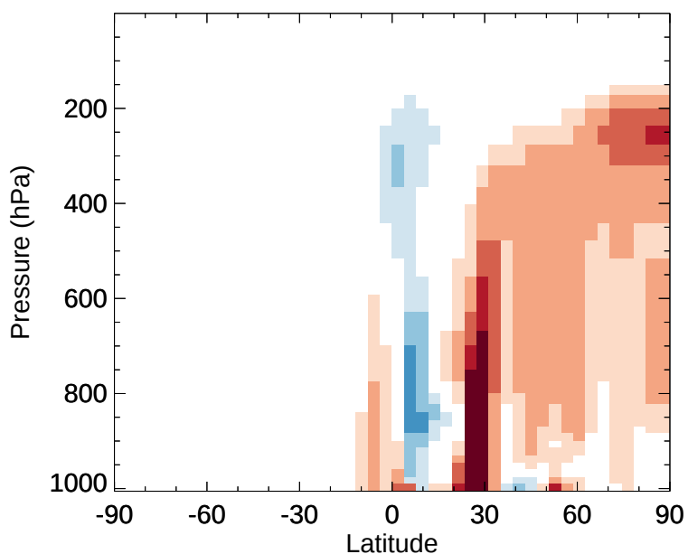
v11-02e-Run1 - v11-02d-Run1 BENZ - Zonal mean abs diff for Jan
