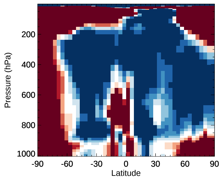
v11-02e-Run1 / v11-02e-Run0 SALC - Zonal mean % diff for Jan
