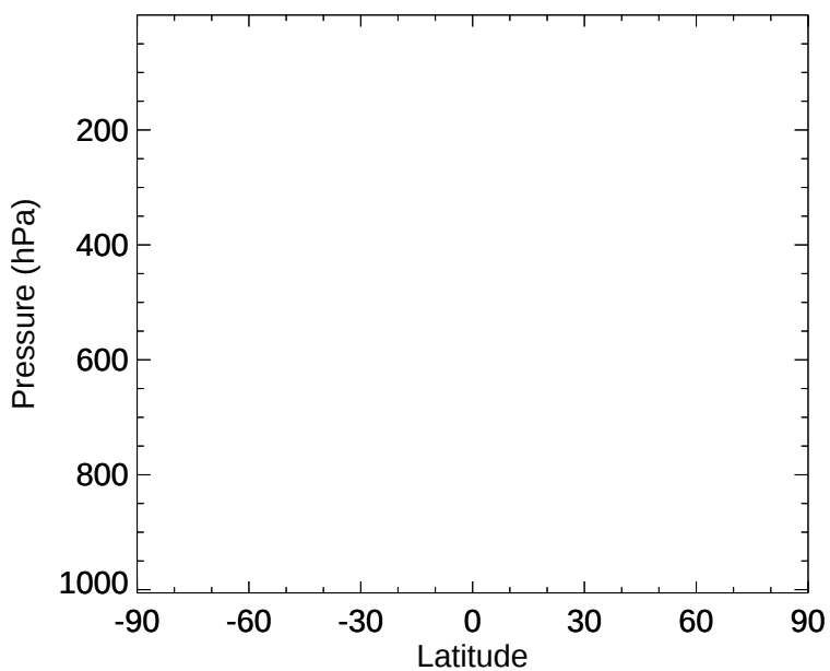
v11-02e-Run1 - v11-02e-Run0 LVOC - Zonal mean abs diff for Jan
