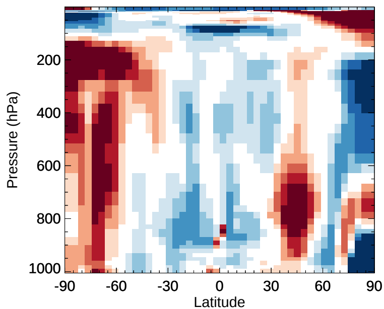
v11-02e-Run1 / v11-02e-Run0 MPN - Zonal mean % diff for Jan
