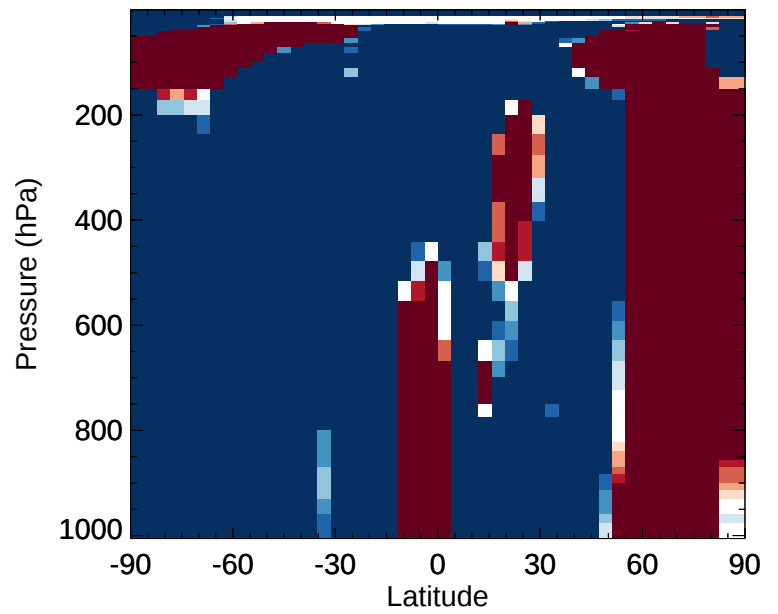
v11-02e-Run1 / v11-02e-Run0 DST4 - Zonal mean % diff for Jan
