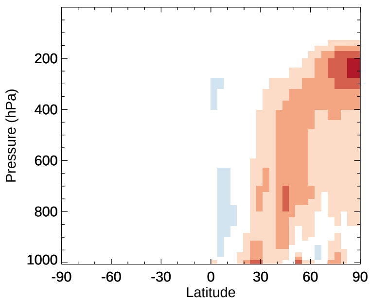
v11-02e-Run1 - v11-02d-Run1 C2H6 - Zonal mean abs diff for Jan
