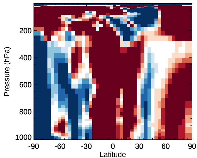
v11-02e-Run1 / v11-02e-Run0 IMAE - Zonal mean % diff for Jan
