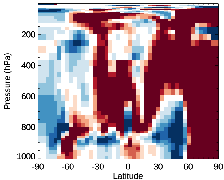
v11-02e-Run1 / v11-02e-Run0 Br2 - Zonal mean % diff for Jan
