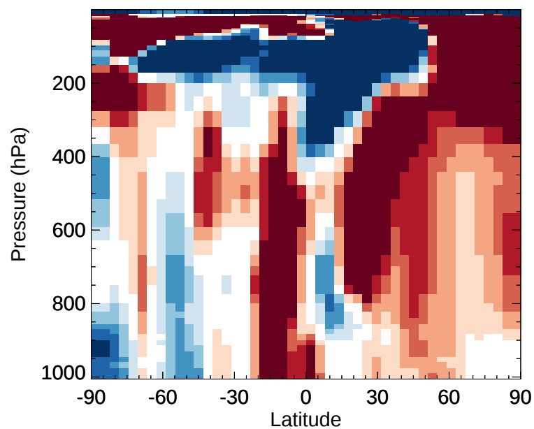
v11-02e-Run1 / v11-02e-Run0 ALK4 - Zonal mean % diff for Jan
