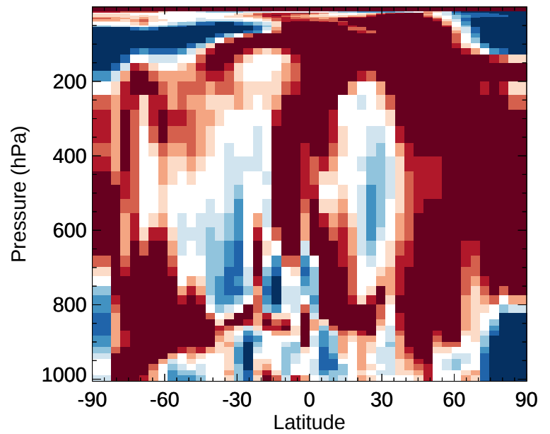
v11-02e-Run1 / v11-02d-Run1 N2O5 - Zonal mean % diff for Jan
