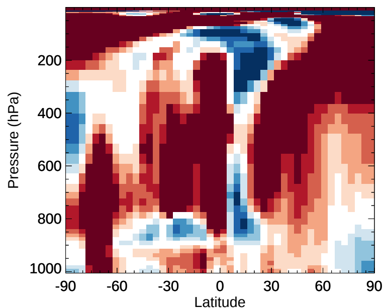
v11-02e-Run1 / v11-02d-Run1 ALD2 - Zonal mean % diff for Jan
