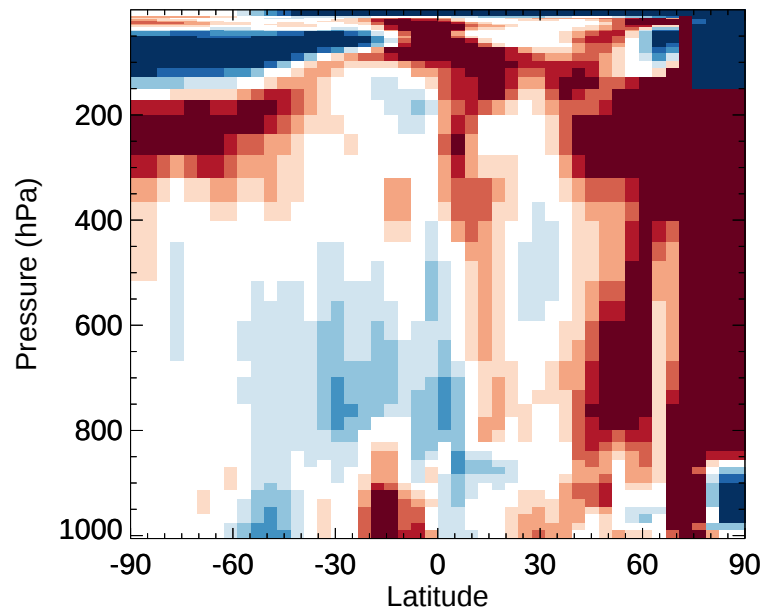
v11-02e-Run1 / v11-02d-Run1 NO - Zonal mean % diff for Jan
