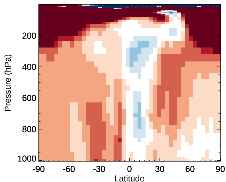
v11-02e-Run1 / v11-02d-Run1 C2H6 - Zonal mean % diff for Jan
