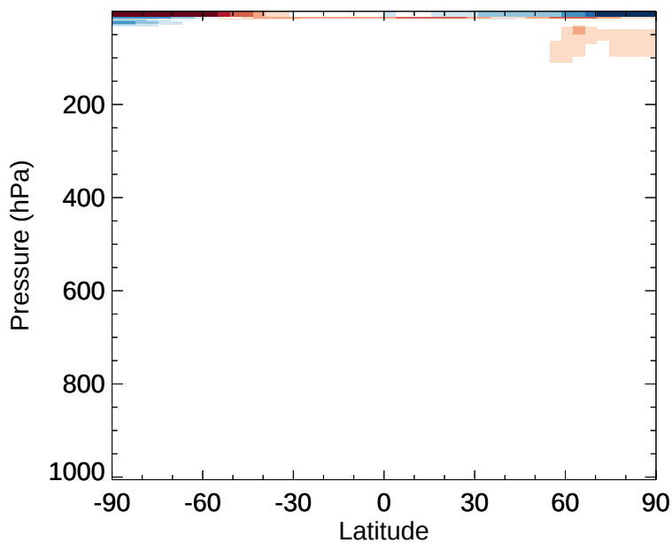
v11-02e-Run1 - v11-02d-Run1 C1O - Zonal mean abs diff for Jan
