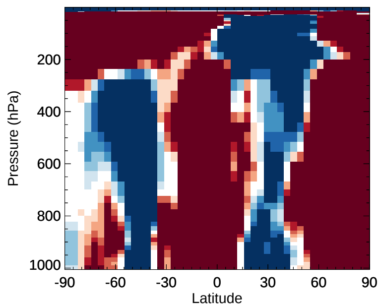
v11-02e-Run1 / v11-02d-Run1 DST2 - Zonal mean % diff for Jan
