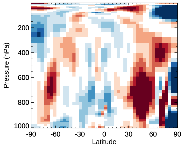
v11-02e-Run1 / v11-02e-Run0 HNO 4 - Zonal mean % diff for Jan
