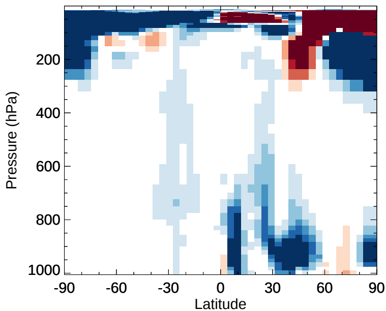
v11-02e-Run1 - v11-02e-Run0 HNO 3 - Zonal mean abs diff for Jan
