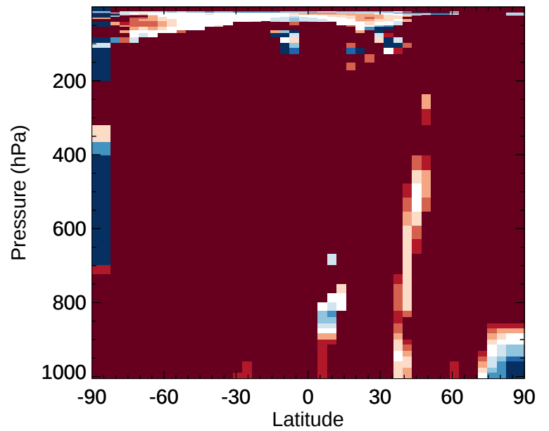
v11-02e-Run1 / v11-02d-Run1 RIPB - Zonal mean % diff for Jan
