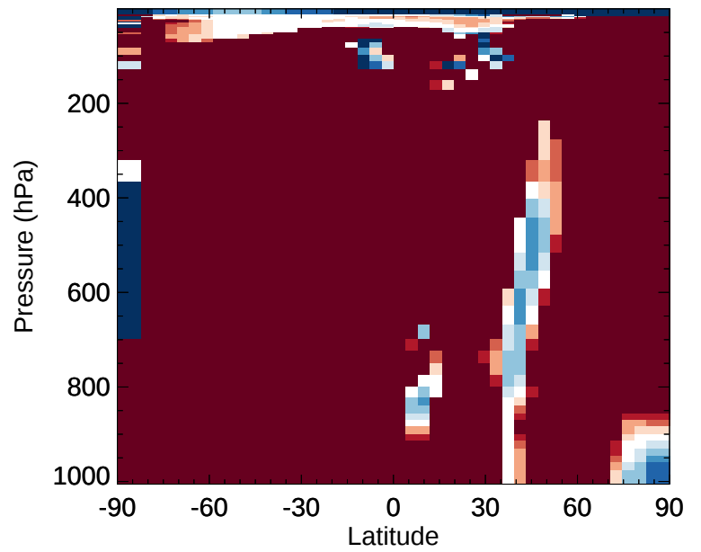
v11-02e-Run1 / v11-02e-Run0 RIPA - Zonal mean % diff for Jan
