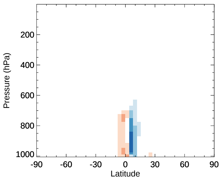
v11-02e-Run1 - v11-02d-Run1 OCPI - Zonal mean abs diff for Jan
