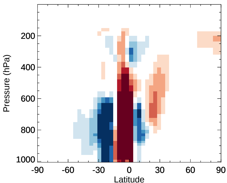
v11-02e-Run1 - v11-02d-Run1 MAP - Zonal mean abs diff for Jan
