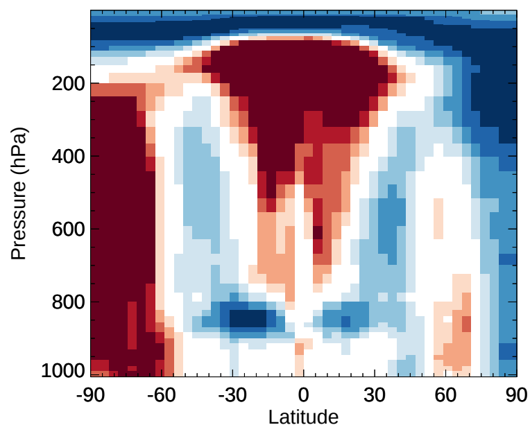
v11-02e-Run1 / v11-02d-Run1 MSA - Zonal mean % diff for Jan
