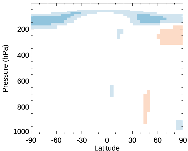
v11-02e-Run1 - v11-02d-Run1 PAN - Zonal mean abs diff for Jan
