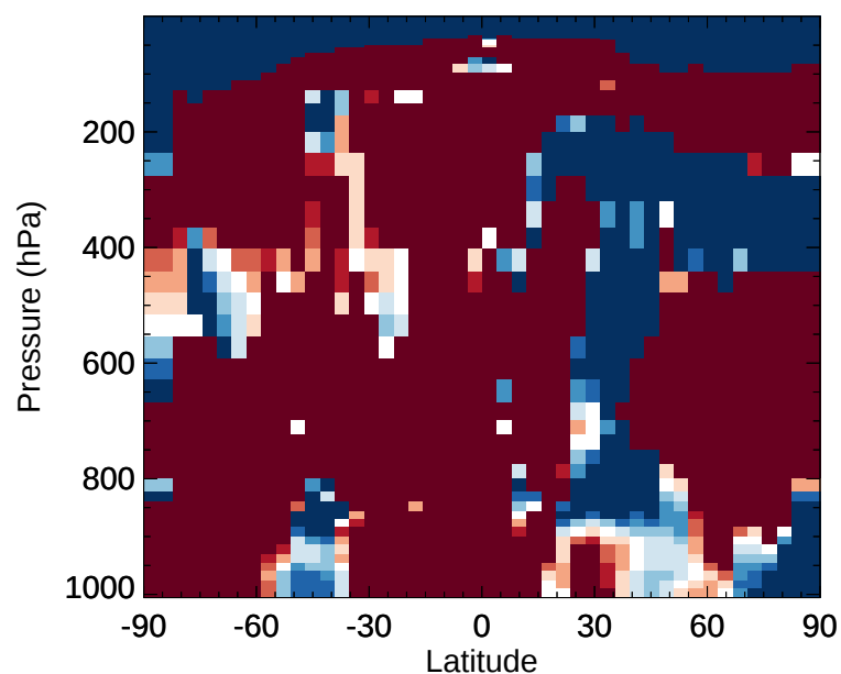
v11-02e-Run1 / v11-02d-Run1 NIT - Zonal mean % diff for Jan
