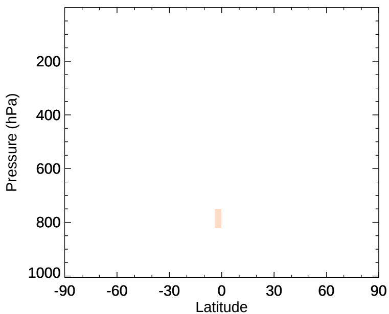
v11-02e-Run1 - v11-02d-Run1 IMAE - Zonal mean abs diff for Jan
