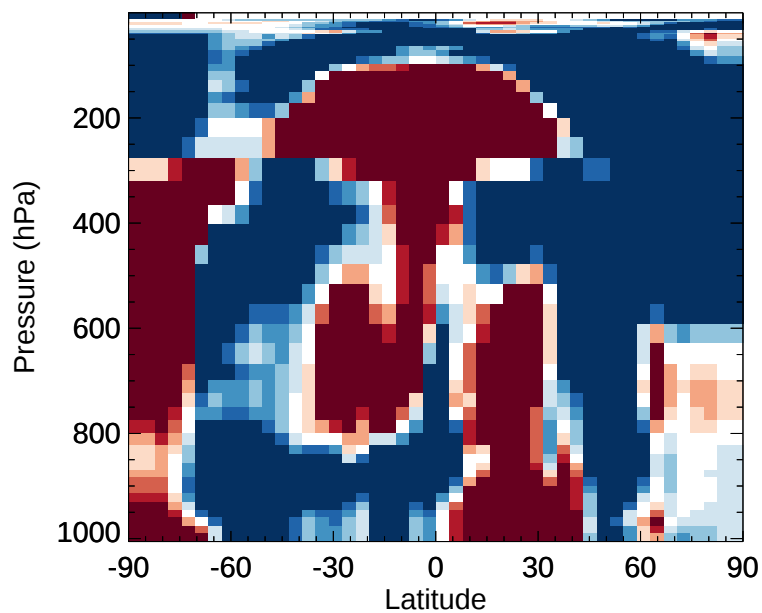
v11-02e-Run1 / v11-02d-Run1 Br2 - Zonal mean % diff for Jan
