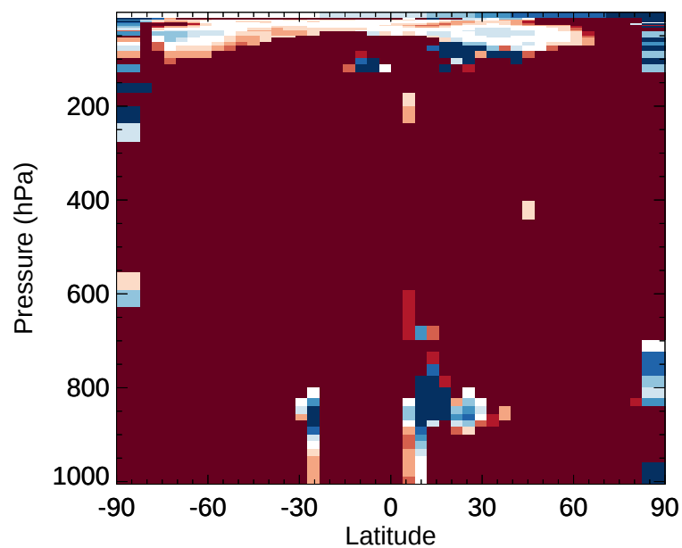
v11-02e-Run1 / v11-02e-Run0 LIMO - Zonal mean % diff for Jan
