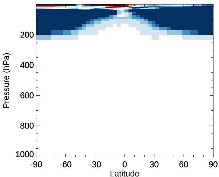
v11-02e-Run1 - v11-02d-Run1 HCl - Zonal mean abs diff for Jan
