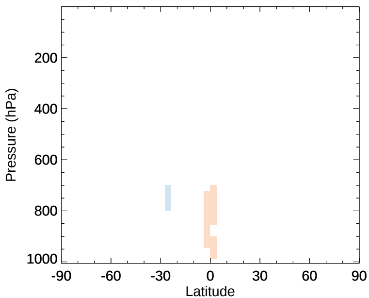
v11-02e-Run1 - v11-02e-Run0 HAC - Zonal mean abs diff for Jan
