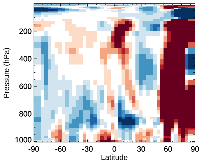
v11-02e-Run1 / v11-02e-Run0 HNO 2 - Zonal mean % diff for Jan
