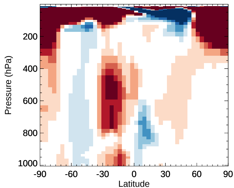
v11-02e-Run1 / v11-02e-Run0 CHBr3 - Zonal mean % diff for Jan
