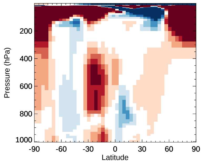
v11-02e-Run1 / v11-02d-Run1 CHBr3 - Zonal mean % diff for Jan
