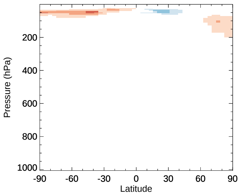
v11-02e-Run1 - v11-02e-Run0 OCS - Zonal mean abs diff for Jan
