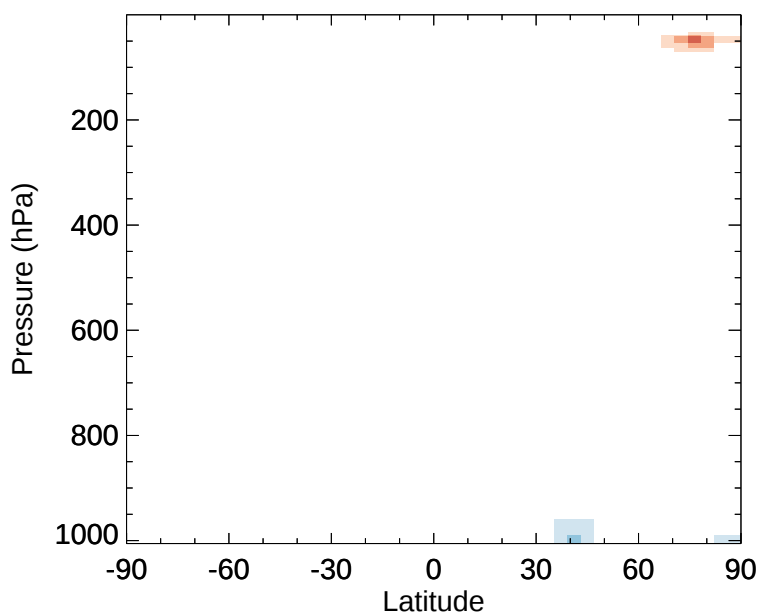
v11-02e-Run1 - v11-02d-Run1 NIT - Zonal mean abs diff for Jan
