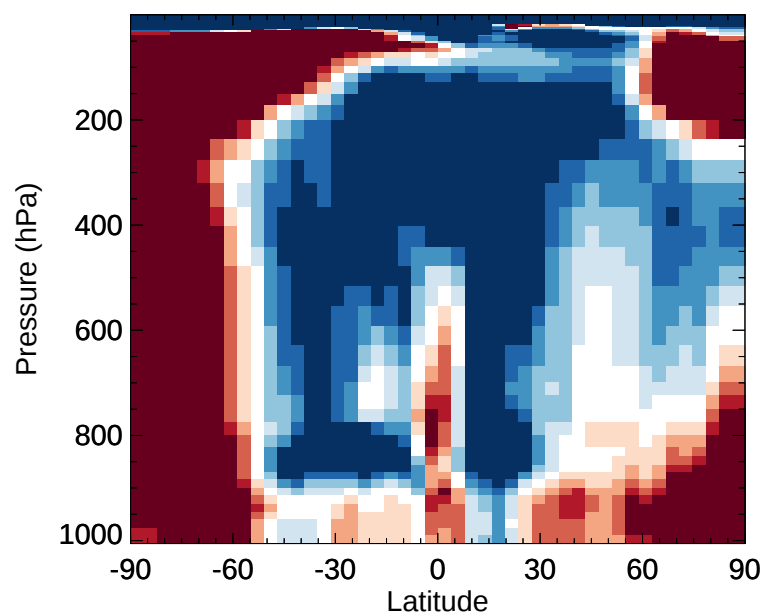
v11-02e-Run1 / v11-02d-Run1 SALA - Zonal mean % diff for Jan
