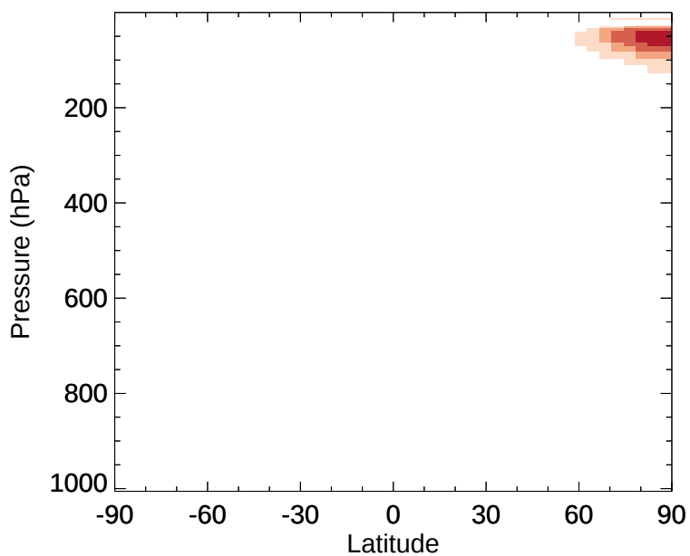
v11-02e-Run1 - v11-02e-Run0 OCIO - Zonal mean abs diff for Jan
