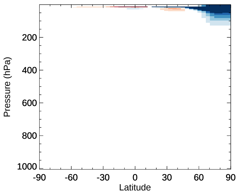
v11-02e-Run1 - v11-02d-Run1 NO 3 - Zonal mean abs diff for Jan
