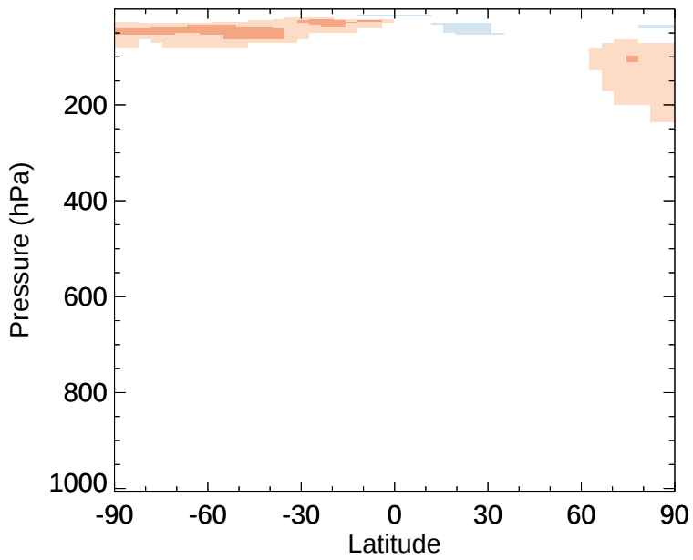
v11-02e-Run1 - v11-02e-Run0 CH3Cl - Zonal mean abs diff for Jan
