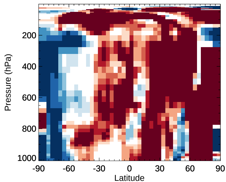
v11-02e-Run1 / v11-02e-Run0 HBr - Zonal mean % diff for Jan
