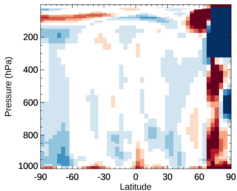
v11-02e-Run1 / v11-02d-Run1 OH - Zonal mean % diff for Jan
