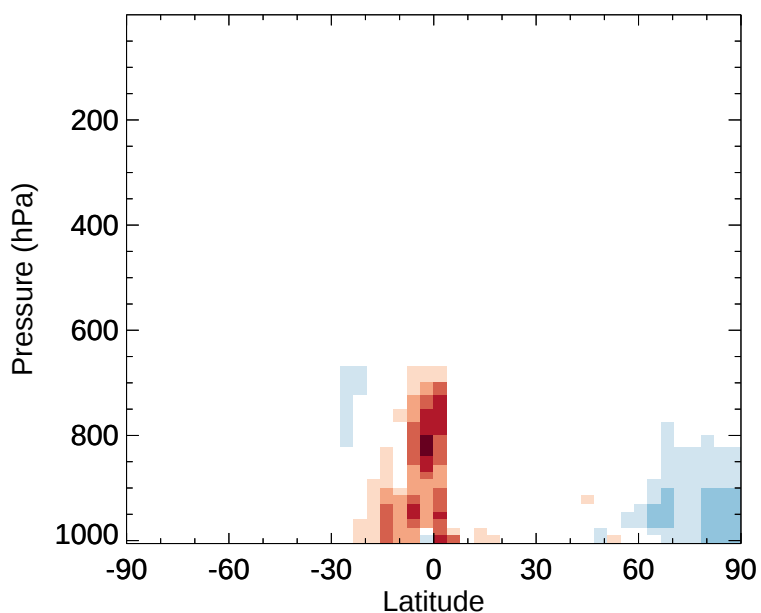
v11-02e-Run1 - v11-02d-Run1 EOH - Zonal mean abs diff for Jan
