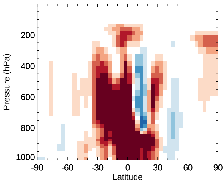
v11-02e-Run1 - v11-02e-Run0 MP - Zonal mean abs diff for Jan
