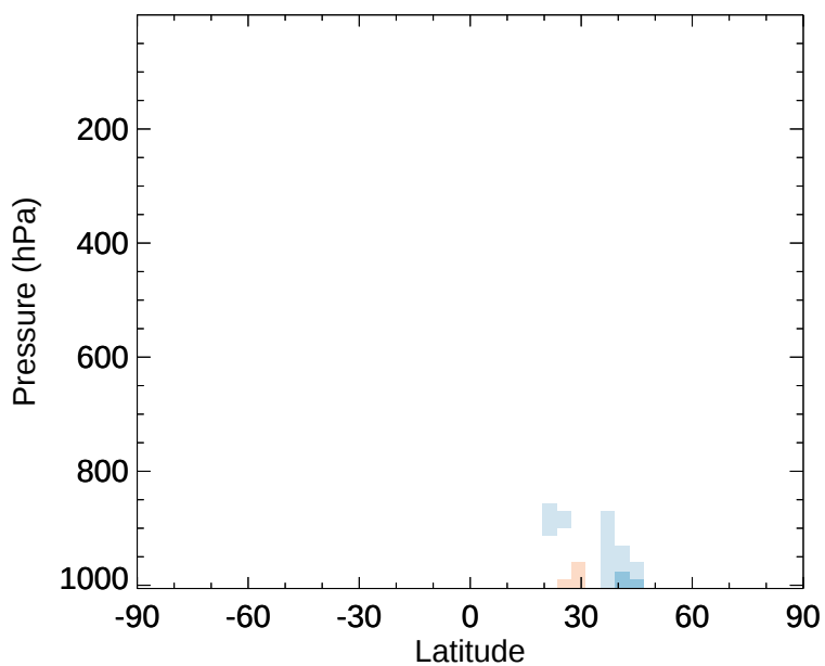
v11-02e-Run1 - v11-02e-Run0 NH4 - Zonal mean abs diff for Jan
