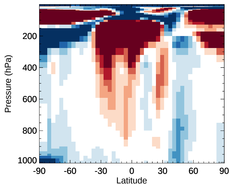
v11-02e-Run1 / v11-02d-Run1 MP - Zonal mean % diff for Jan
