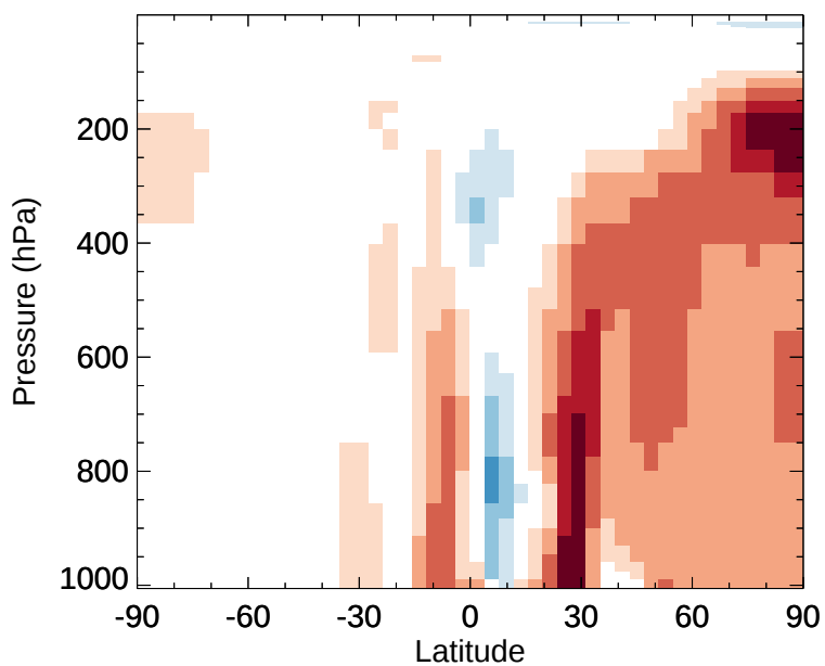
v11-02e-Run1 - v11-02e-Run0 CO - Zonal mean abs diff for Jan
