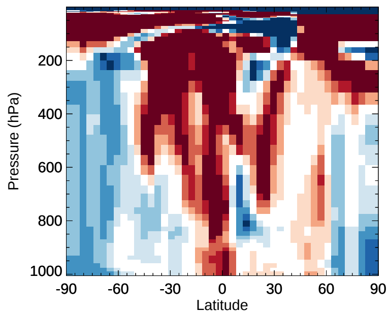
v11-02e-Run1 / v11-02e-Run0 MGLY - Zonal mean % diff for Jan
