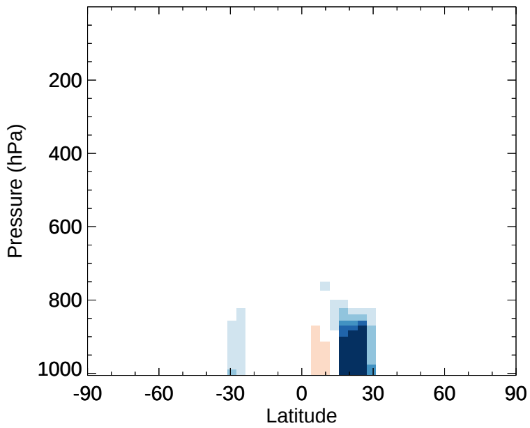
v11-02e-Run1 - v11-02e-Run0 DST4 - Zonal mean abs diff for Jan
