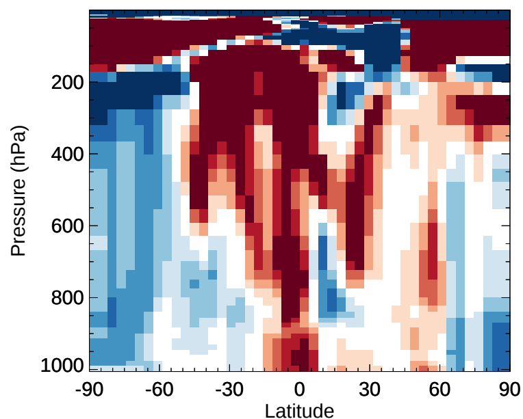
v11-02e-Run1 / v11-02d-Run1 MGLY - Zonal mean % diff for Jan
