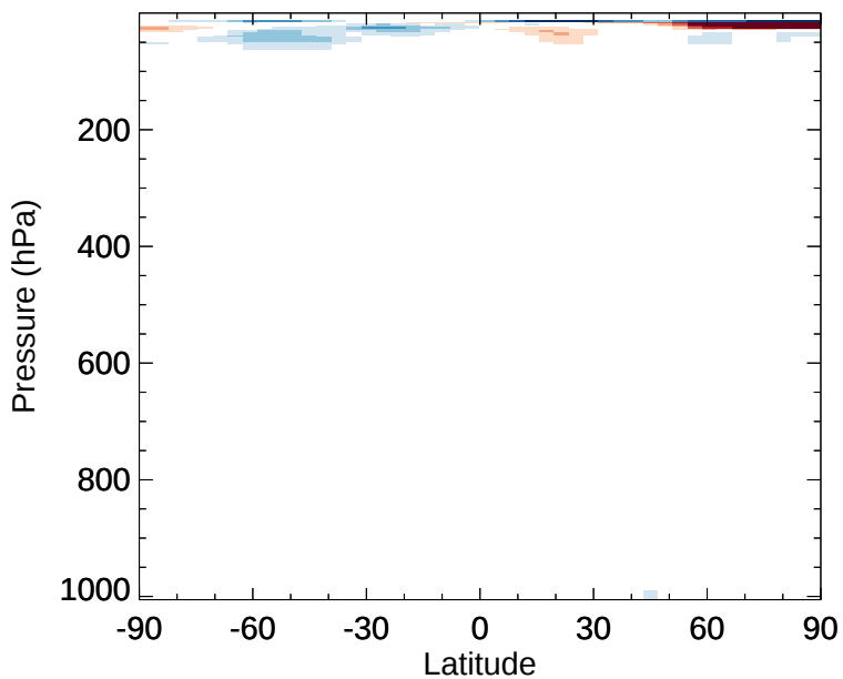
v11-02e-Run1 - v11-02e-Run0 NO2 - Zonal mean abs diff for Jan
