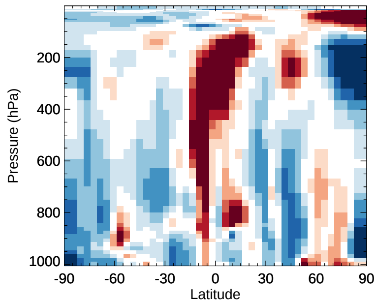
v11-02e-Run1 / v11-02e-Run0 HNO 3 - Zonal mean % diff for Jan
