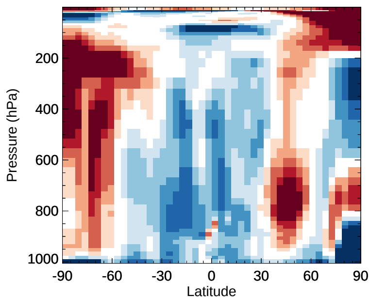
v11-02e-Run1 / v11-02d-Run1 MPN - Zonal mean % diff for Jan
