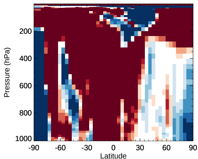
v11-02e-Run1 / v11-02d-Run1 GLYC - Zonal mean % diff for Jan
