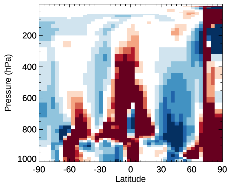
v11-02e-Run1 / v11-02e-Run0 BrO - Zonal mean % diff for Jan
