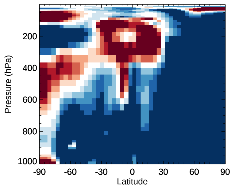
v11-02e-Run1 / v11-02d-Run1 HOBr - Zonal mean % diff for Jan
