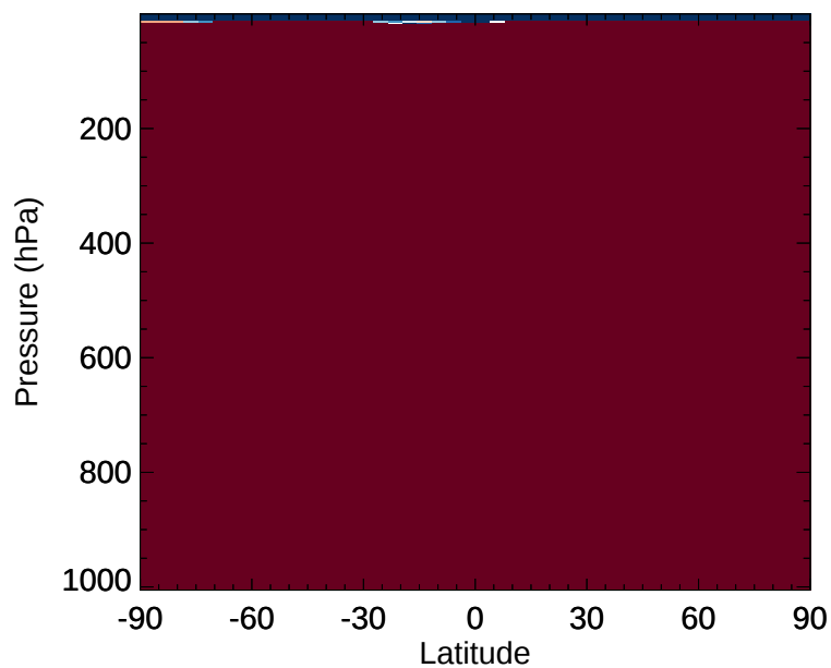
v11-02e-Run1 / v11-02d-Run1 DST1 - Zonal mean % diff for Jan
