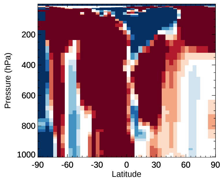
v11-02e-Run1 / v11-02e-Run0 TOLU - Zonal mean % diff for Jan
