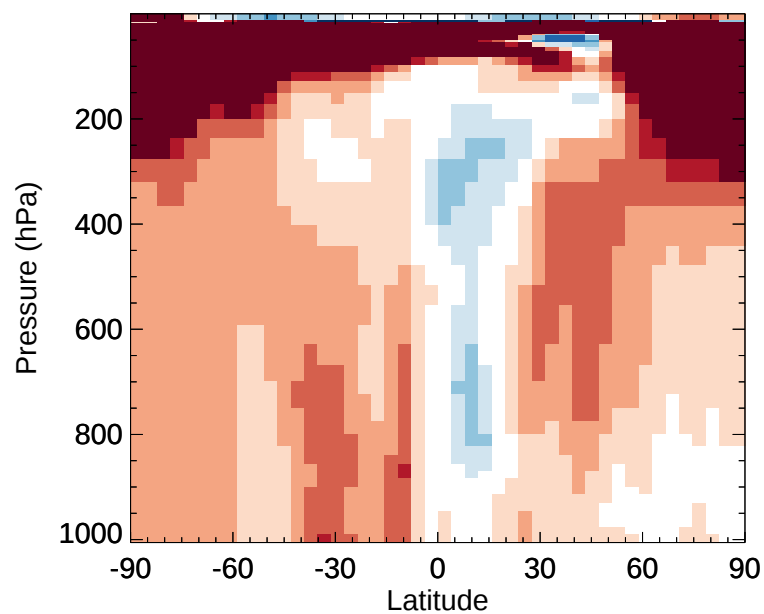
v11-02e-Run1 / v11-02e-Run0 C2H6 - Zonal mean % diff for Jan
