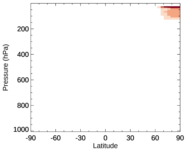
v11-02e-Run1 - v11-02e-Run0 Cl2 - Zonal mean abs diff for Jan
