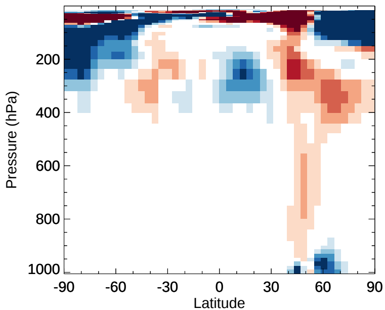
v11-02e-Run1 - v11-02e-Run0 HNO 4 - Zonal mean abs diff for Jan
