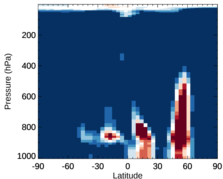
v11-02e-Run1 / v11-02d-Run1 HCl - Zonal mean % diff for Jan
