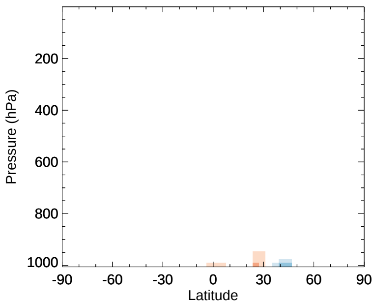
v11-02e-Run1 - v11-02e-Run0 SOAP - Zonal mean abs diff for Jan
