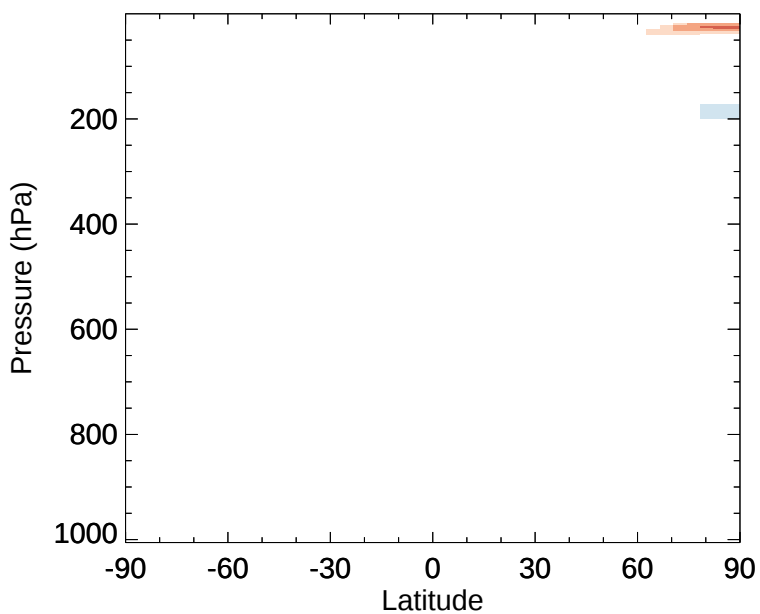
v11-02e-Run1 - v11-02e-Run0 HOBr - Zonal mean abs diff for Jan
