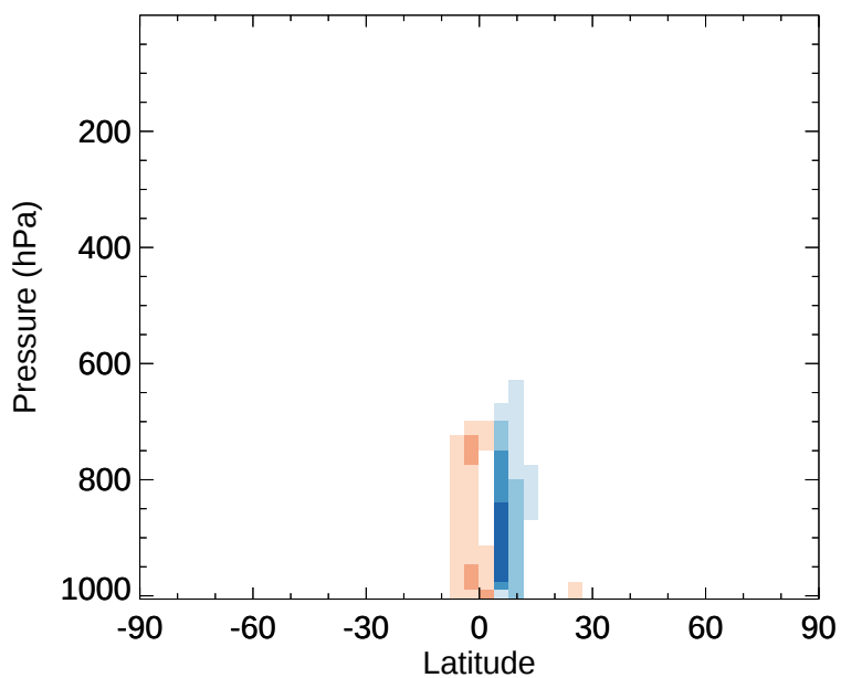
v11-02e-Run1 - v11-02e-Run0 OCPI - Zonal mean abs diff for Jan
