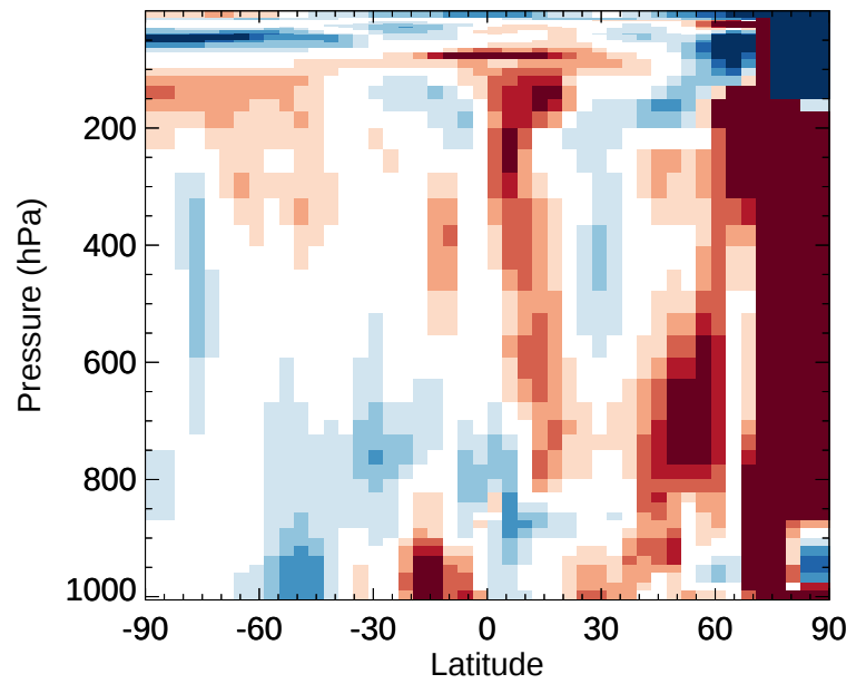
v11-02e-Run1 / v11-02e-Run0 NO - Zonal mean % diff for Jan
