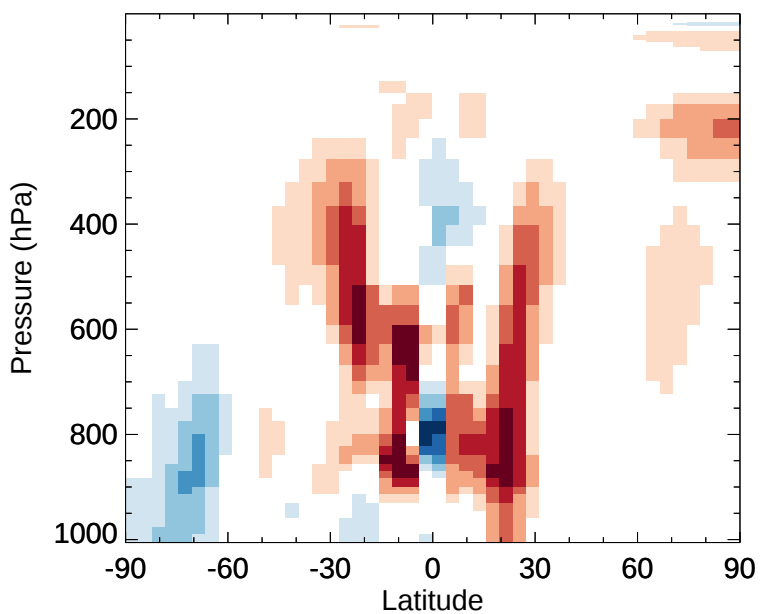
v11-02e-Run1 - v11-02e-Run0 H2O2 - Zonal mean abs diff for Jan
