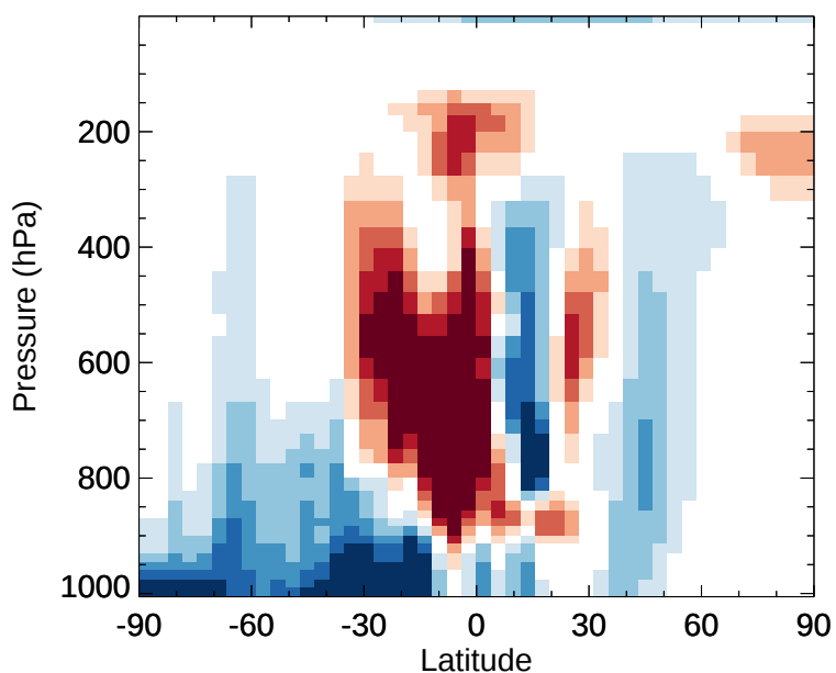
v11-02e-Run1 - v11-02d-Run1 MP - Zonal mean abs diff for Jan
