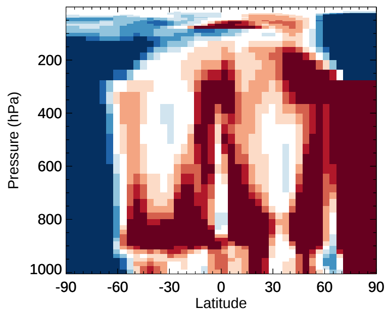
v11-02e-Run1 / v11-02e-Run0 HCl - Zonal mean % diff for Jan
