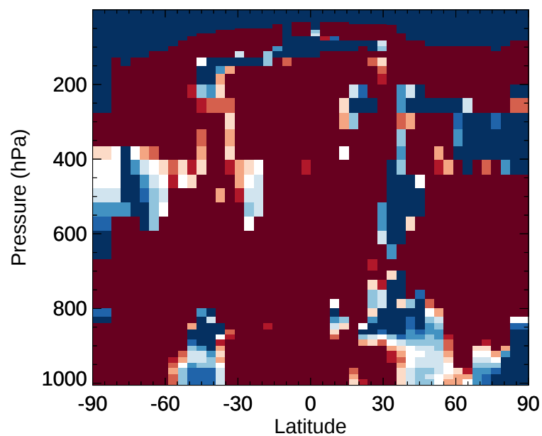
v11-02e-Run1 / v11-02e-Run0 NIT - Zonal mean % diff for Jan
