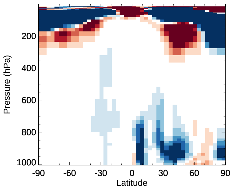
v11-02e-Run1 - v11-02d-Run1 HNO 3 - Zonal mean abs diff for Jan
