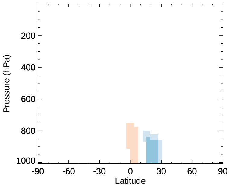
v11-02e-Run1 - v11-02d-Run1 DST1 - Zonal mean abs diff for Jan
