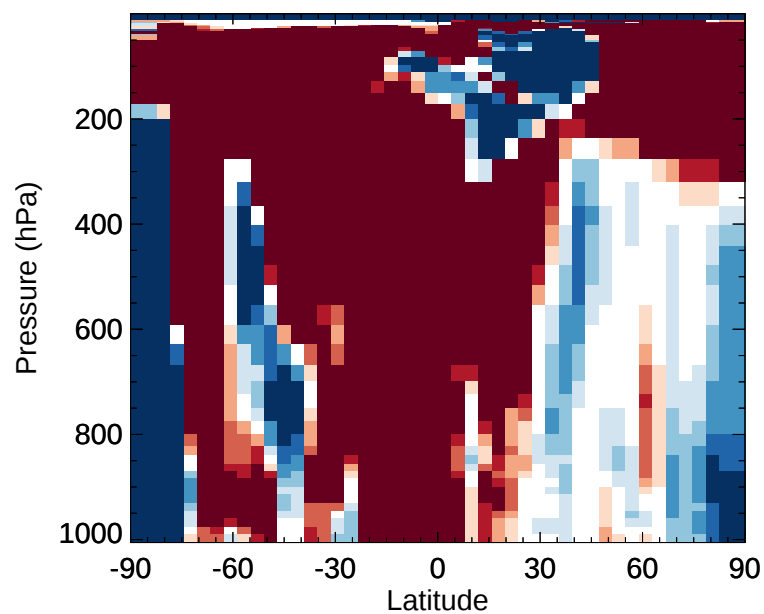
v11-02e-Run1 / v11-02e-Run0 GLYC - Zonal mean % diff for Jan
