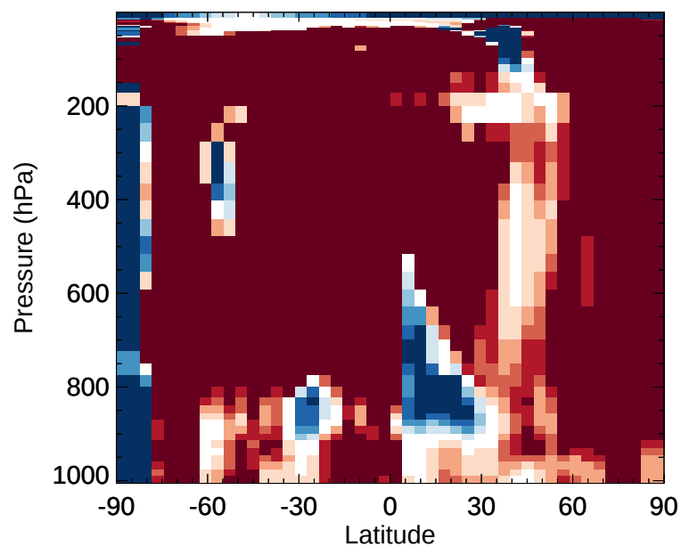
v11-02e-Run1 / v11-02e-Run0 PRPE - Zonal mean % diff for Jan
