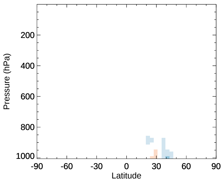
v11-02e-Run1 - v11-02d-Run1 NH4 - Zonal mean abs diff for Jan
