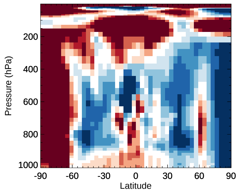
v11-02e-Run1 / v11-02d-Run1 SO 2 - Zonal mean % diff for Jan
