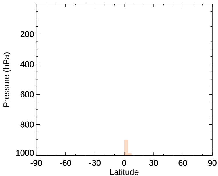
v11-02e-Run1 - v11-02e-Run0 CH 2 O - Zonal mean abs diff for Jan
