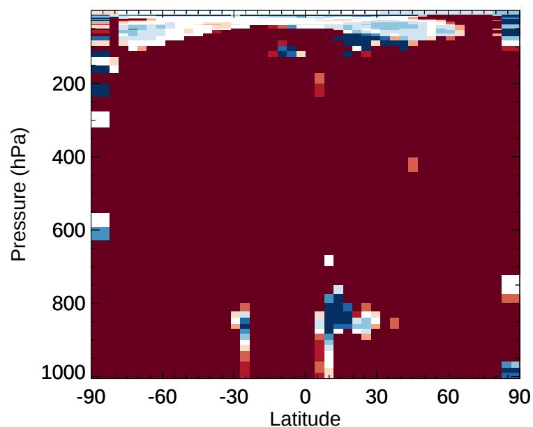
v11-02e-Run1 / v11-02d-Run1 LIMO - Zonal mean % diff for Jan
