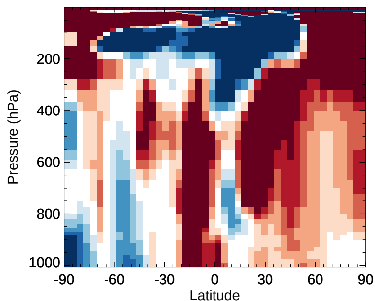
v11-02e-Run1 / v11-02d-Run1 ALK4 - Zonal mean % diff for Jan
