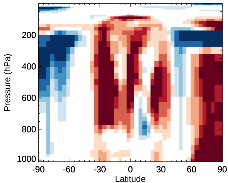
v11-02e-Run1 / v11-02e-Run0 H 2 O - Zonal mean % diff for Jan
