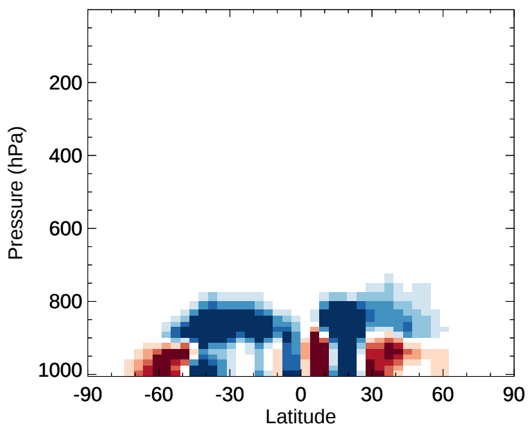
v11-02e-Run1 - v11-02e-Run0 SALC - Zonal mean abs diff for Jan
