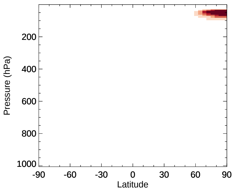
v11-02e-Run1 - v11-02d-Run1 Cl2O2 - Zonal mean abs diff for Jan
