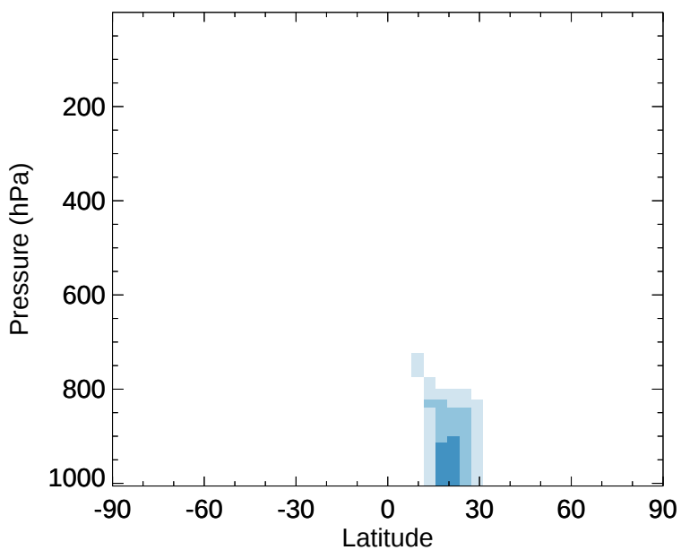
v11-02e-Run1 - v11-02e-Run0 DST1 - Zonal mean abs diff for Jan
