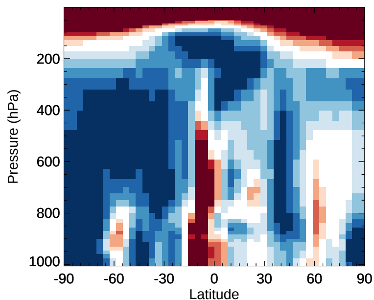
v11-02e-Run1 / v11-02d-Run1 SOAS - Zonal mean % diff for Jan
