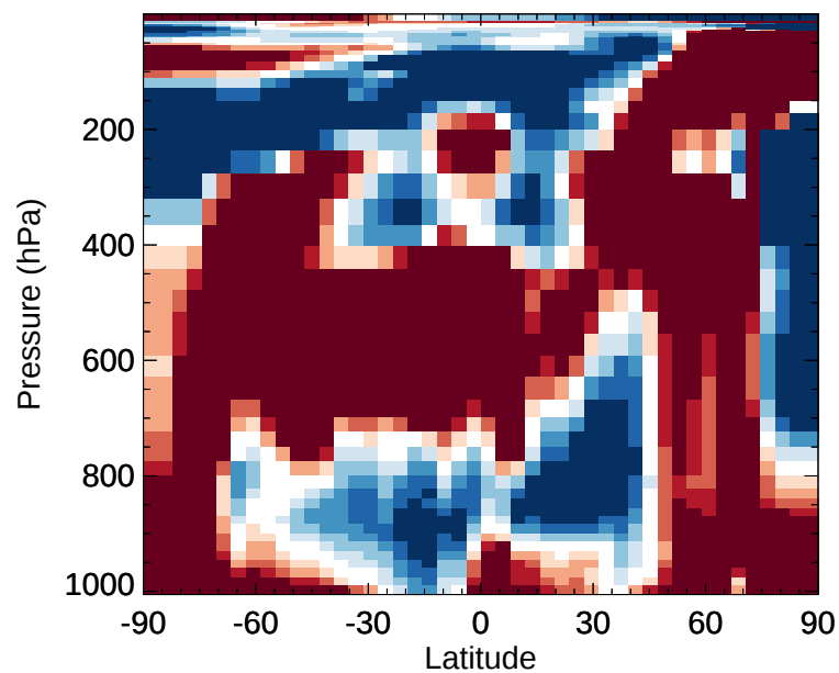
v11-02e-Run1 / v11-02d-Run1 C1O - Zonal mean % diff for Jan
