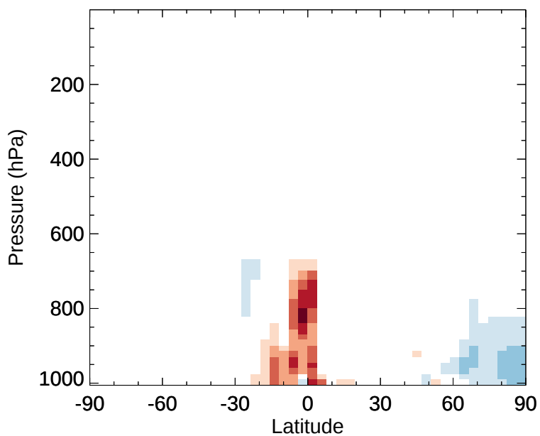
v11-02e-Run1 - v11-02e-Run0 EOH - Zonal mean abs diff for Jan
