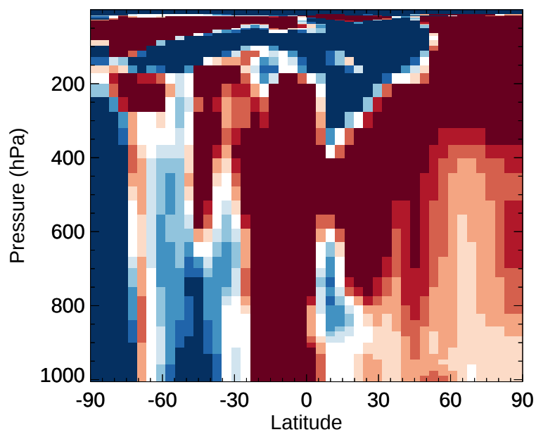
v11-02e-Run1 / v11-02e-Run0 MEK - Zonal mean % diff for Jan
