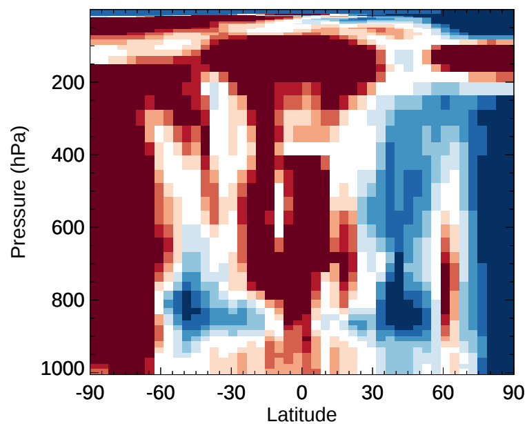
v11-02e-Run1 / v11-02e-Run0 SO 2 - Zonal mean % diff for Jan
