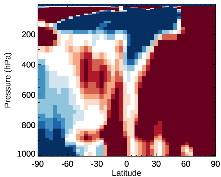
v11-02e-Run1 / v11-02e-Run0 R4N2 - Zonal mean % diff for Jan
