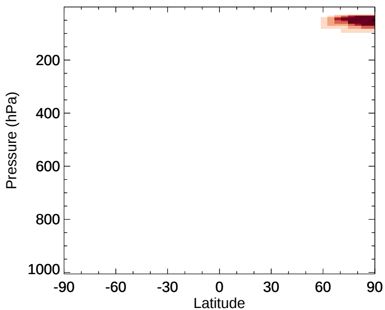
v11-02e-Run1 - v11-02e-Run0 Cl2O2 - Zonal mean abs diff for Jan
