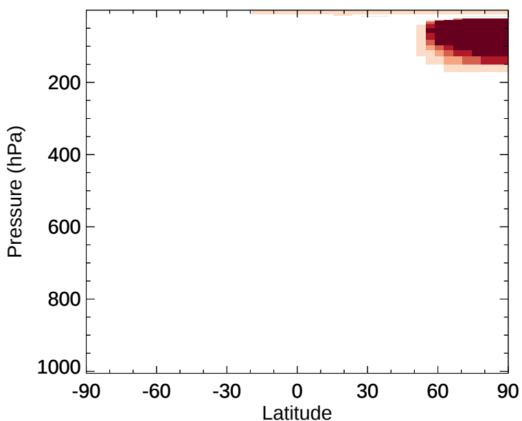
v11-02e-Run1 - v11-02d-Run1 HOCl - Zonal mean abs diff for Jan
