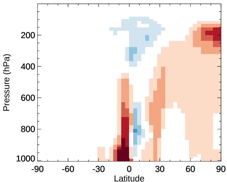
v11-02e-Run1 - v11-02d-Run1 ACET - Zonal mean abs diff for Jan
