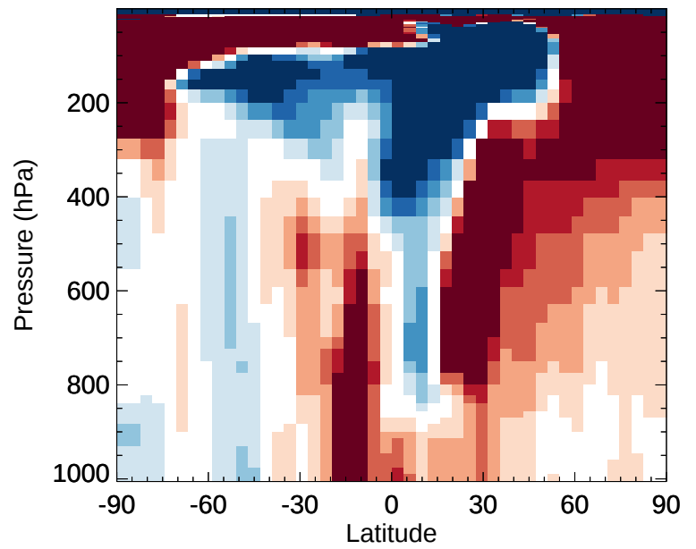
v11-02e-Run1 / v11-02e-Run0 C3H8 - Zonal mean % diff for Jan
