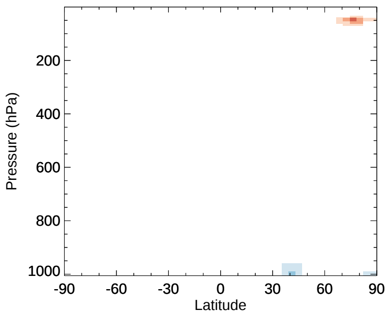
v11-02e-Run1 - v11-02e-Run0 NIT - Zonal mean abs diff for Jan
