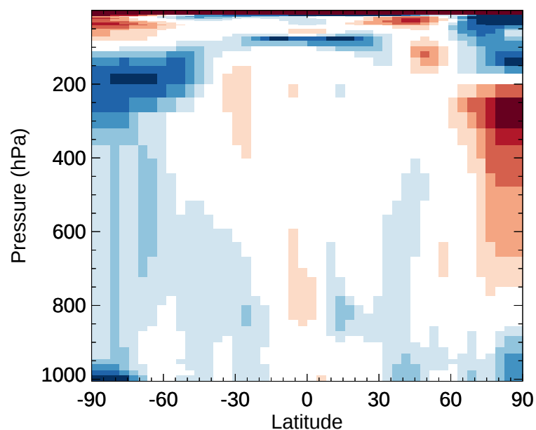
v11-02e-Run1 / v11-02d-Run1 CH 2 O - Zonal mean % diff for Jan
