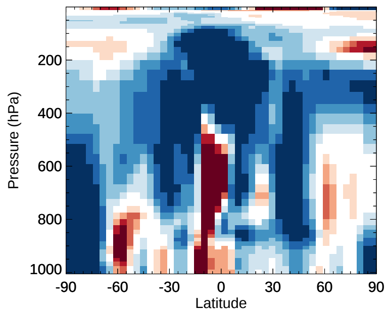
v11-02e-Run1 / v11-02e-Run0 BCPI - Zonal mean % diff for Jan
