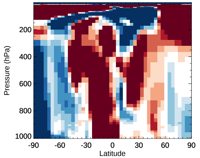
v11-02e-Run1 / v11-02e-Run0 GLYX - Zonal mean % diff for Jan
