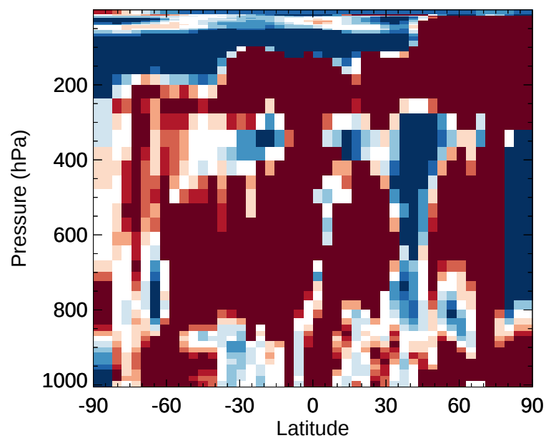
v11-02e-Run1 / v11-02e-Run0 Cl2O2 - Zonal mean % diff for Jan
