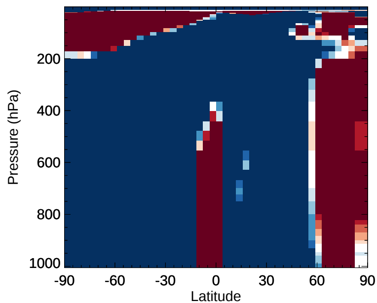
v11-02e-Run1 / v11-02e-Run0 DST3 - Zonal mean % diff for Jan
