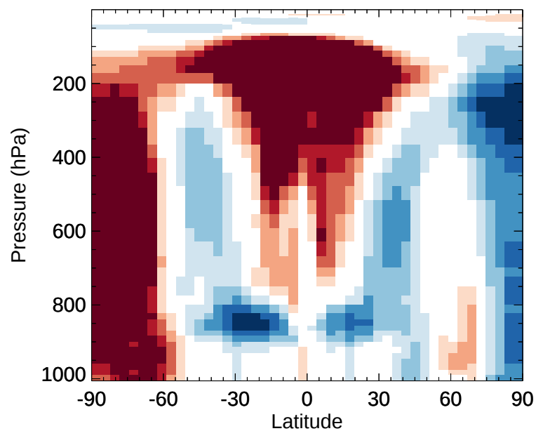
v11-02e-Run1 / v11-02e-Run0 MSA - Zonal mean % diff for Jan
