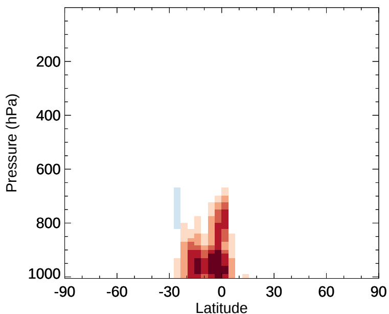
v11-02e-Run1 - v11-02d-Run1 MVK - Zonal mean abs diff for Jan
