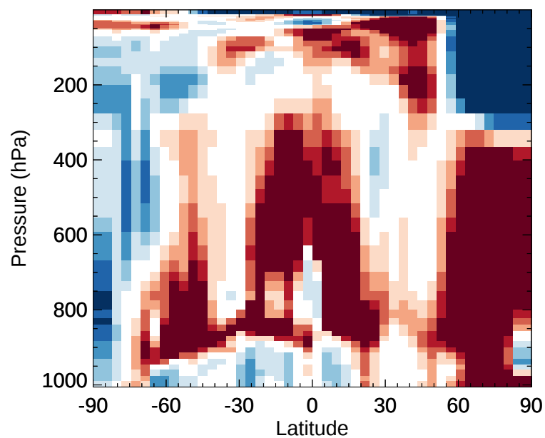
v11-02e-Run1 / v11-02e-Run0 NO 3 - Zonal mean % diff for Jan
