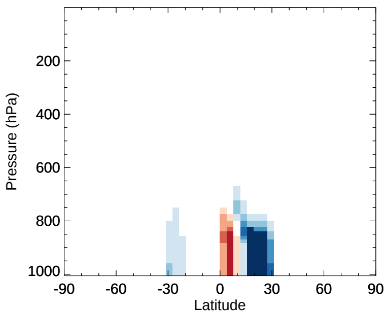
v11-02e-Run1 - v11-02d-Run1 DST3 - Zonal mean abs diff for Jan
