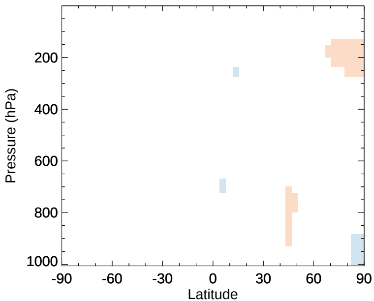
v11-02e-Run1 - v11-02e-Run0 PAN - Zonal mean abs diff for Jan
