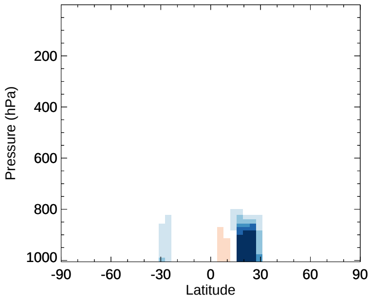
v11-02e-Run1 - v11-02d-Run1 DST4 - Zonal mean abs diff for Jan
