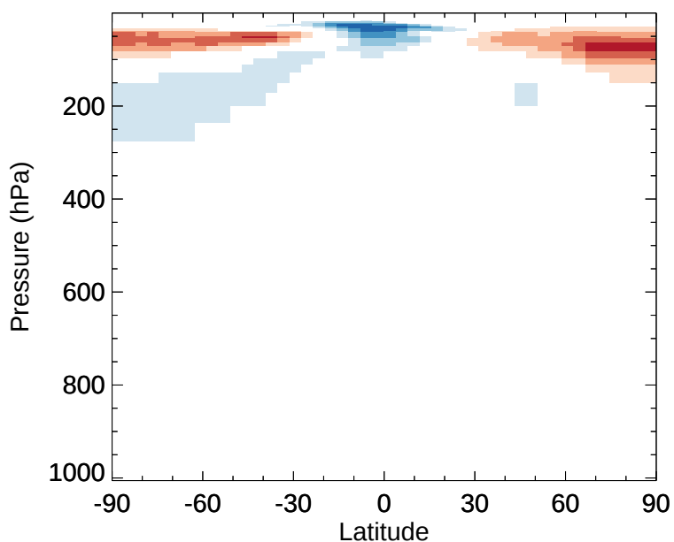
v11-02e-Run1 - v11-02d-Run1 OCS - Zonal mean abs diff for Jan
