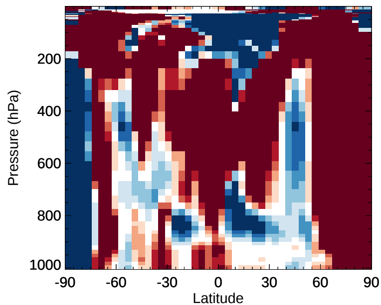
v11-02e-Run1 / v11-02d-Run1 BCPO - Zonal mean % diff for Jan
