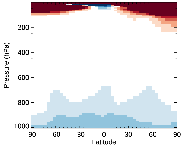
v11-02e-Run1 / v11-02d-Run1 CCl4 - Zonal mean % diff for Jan
