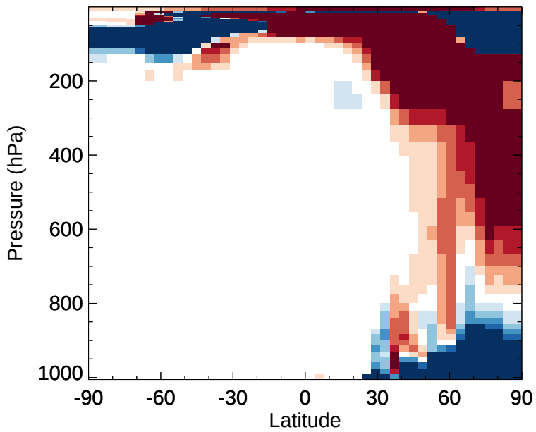
v11-02e-Run1 - v11-02d-Run1 N2O5 - Zonal mean abs diff for Jan
