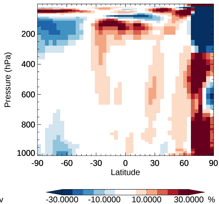
v11-02e-Run1 / v11-02e-Run0 HO2 - Zonal mean % diff for Jan
