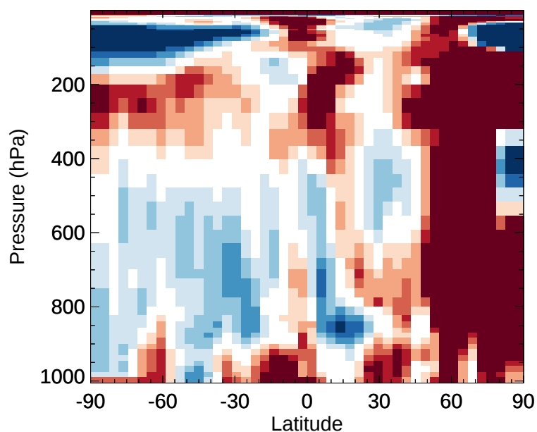
v11-02e-Run1 / v11-02d-Run1 HNO 2 - Zonal mean % diff for Jan
