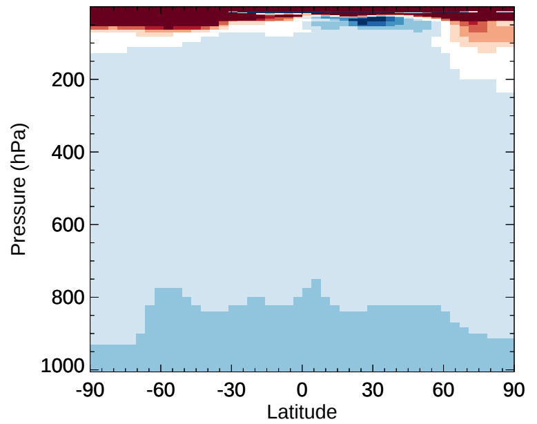
v11-02e-Run1 / v11-02e-Run0 CCl4 - Zonal mean % diff for Jan
