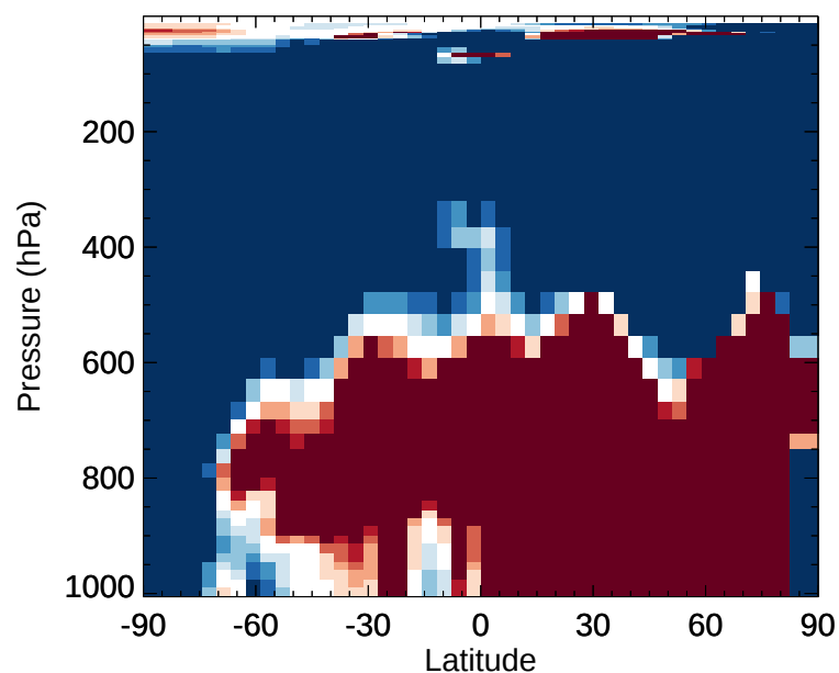
v11-02e-Run1 / v11-02d-Run1 HBr - Zonal mean % diff for Jan
