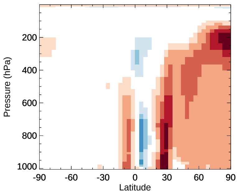
v11-02e-Run1 - v11-02d-Run1 CO - Zonal mean abs diff for Jan
