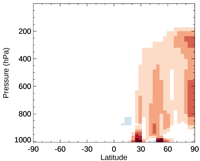
v11-02e-Run1 - v11-02e-Run0 ALK4 - Zonal mean abs diff for Jan
