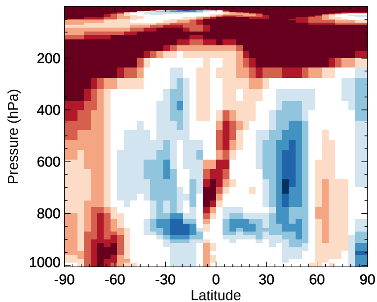
v11-02e-Run1 / v11-02d-Run1 SO4 - Zonal mean % diff for Jan
