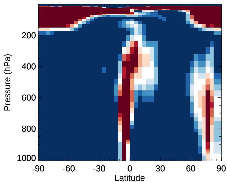
v11-02e-Run1 / v11-02e-Run0 DST1 - Zonal mean % diff for Jan
