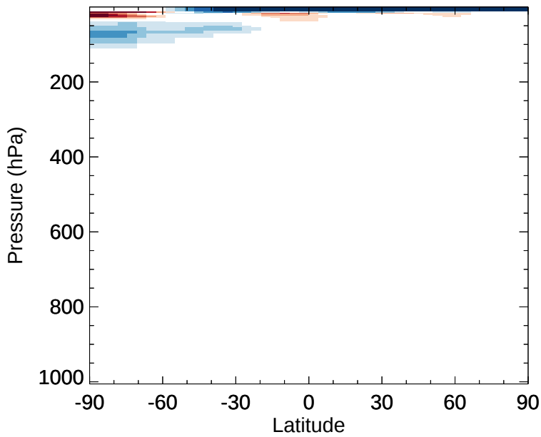
v11-02e-Run1 - v11-02d-Run1 NO - Zonal mean abs diff for Jan
