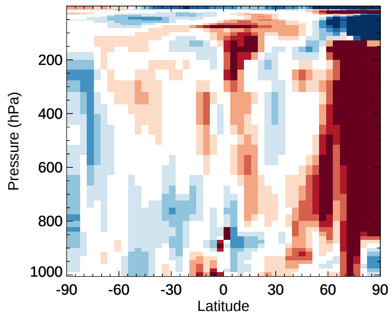
v11-02e-Run1 / v11-02e-Run0 NO2 - Zonal mean % diff for Jan
