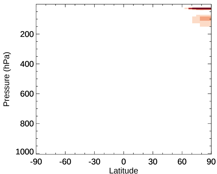
v11-02e-Run1 - v11-02d-Run1 Cl2 - Zonal mean abs diff for Jan
