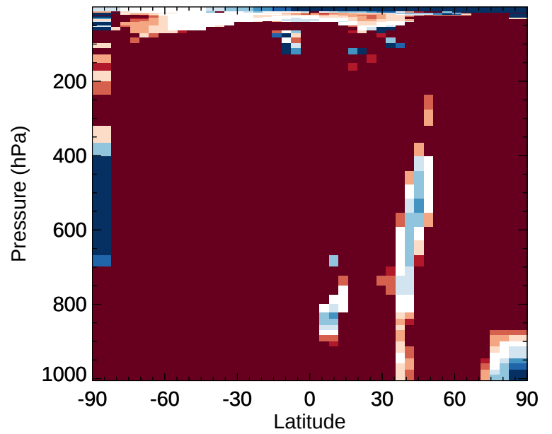
v11-02e-Run1 / v11-02e-Run0 RIPB - Zonal mean % diff for Jan
