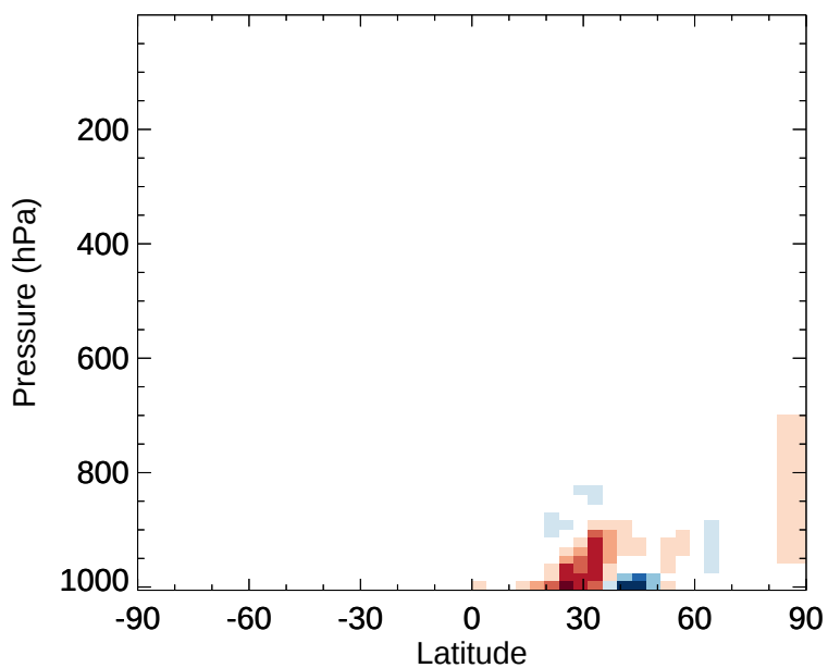
v11-02e-Run1 - v11-02e-Run0 XYLE - Zonal mean abs diff for Jan
