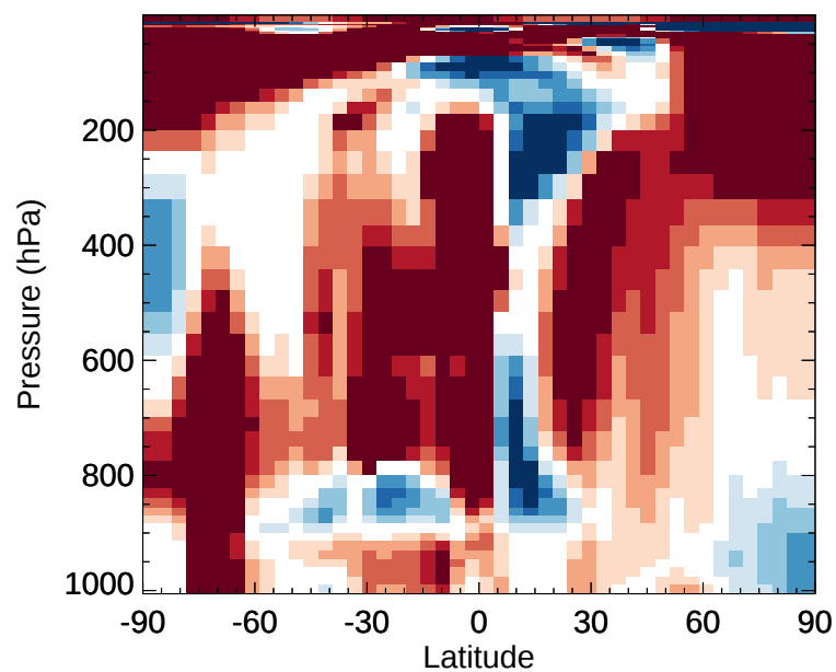
v11-02e-Run1 / v11-02e-Run0 ALD2 - Zonal mean % diff for Jan
