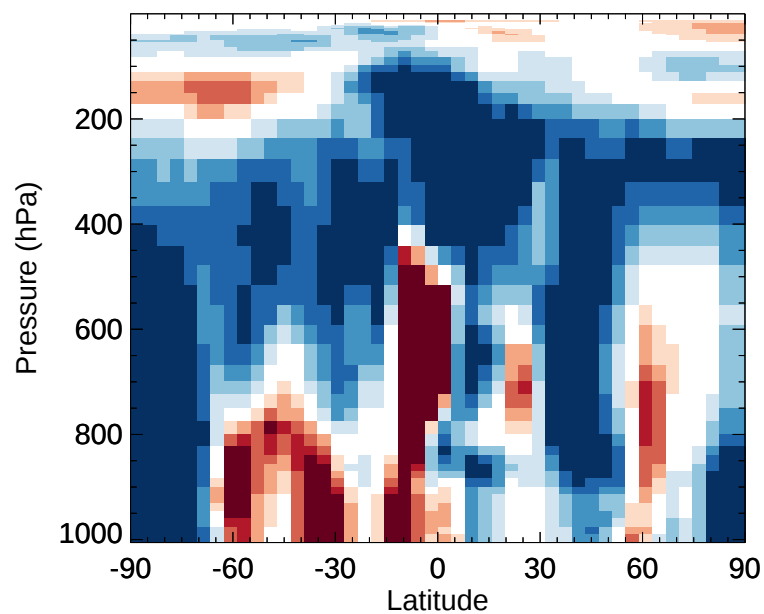
v11-02e-Run1 / v11-02e-Run0 OCPI - Zonal mean % diff for Jan
