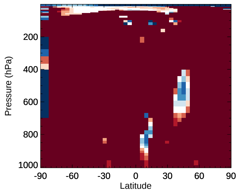
v11-02e-Run1 / v11-02e-Run0 ISOP - Zonal mean % diff for Jan
