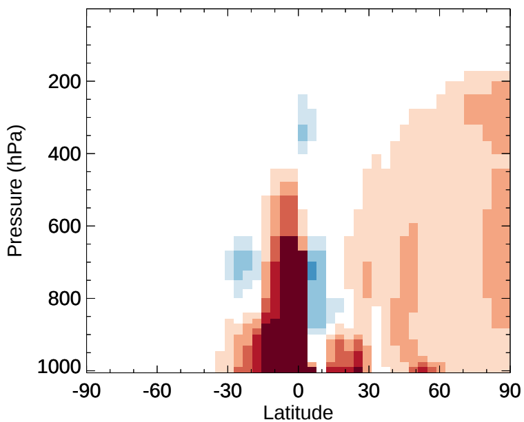
v11-02e-Run1 - v11-02d-Run1 MEK - Zonal mean abs diff for Jan
