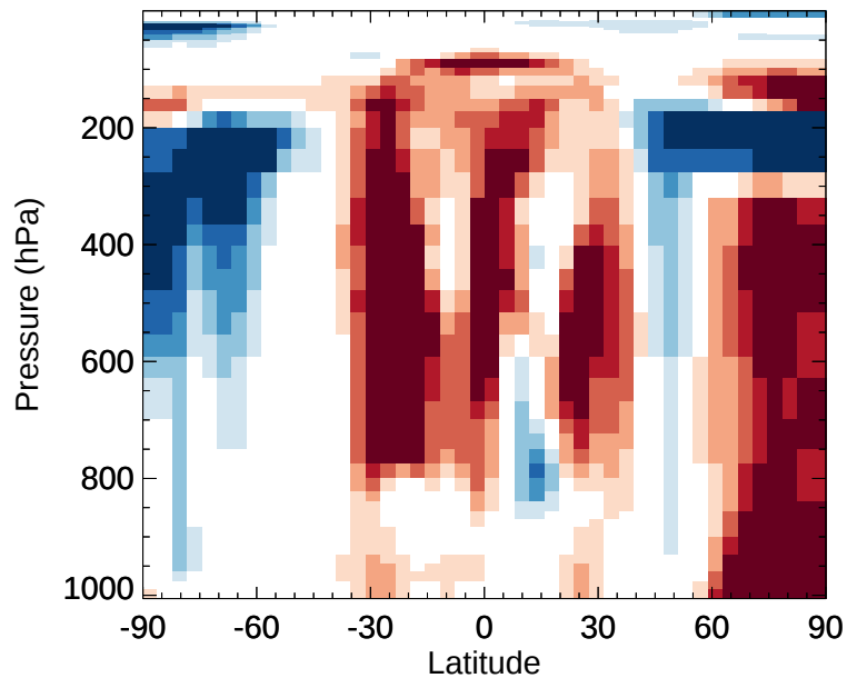
v11-02e-Run1 / v11-02d-Run1 H 2 O - Zonal mean % diff for Jan
