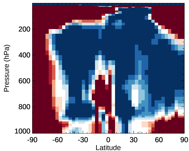
v11-02e-Run1 / v11-02d-Run1 SALC - Zonal mean % diff for Jan
