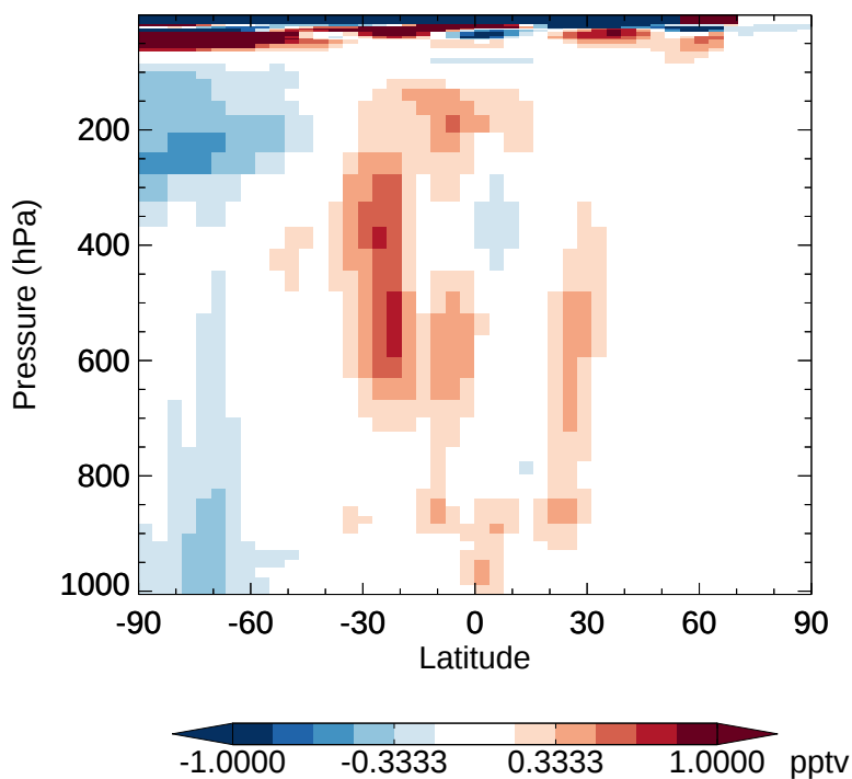
v11-02e-Run1 - v11-02e-Run0 HO2 - Zonal mean abs diff for Jan
