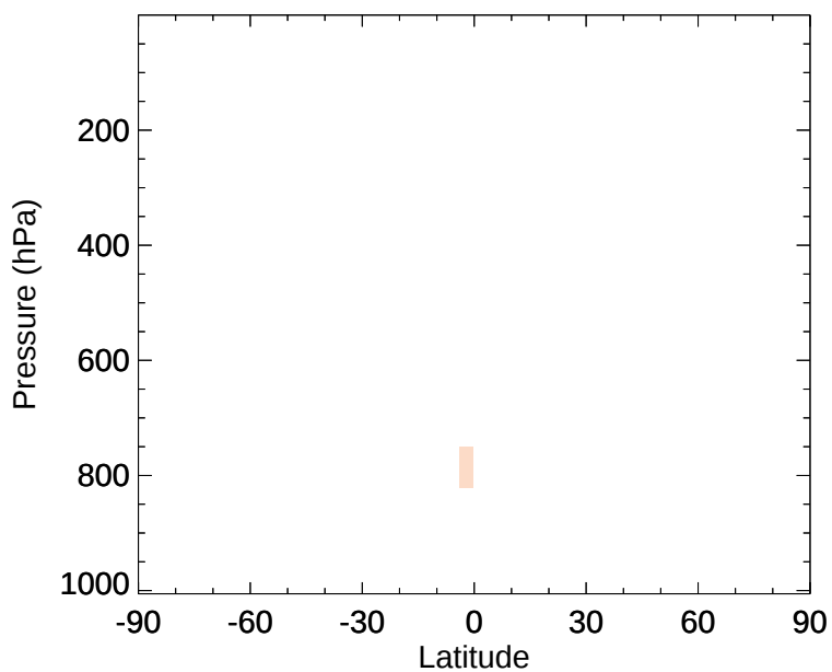
v11-02e-Run1 - v11-02e-Run0 IMAE - Zonal mean abs diff for Jan
