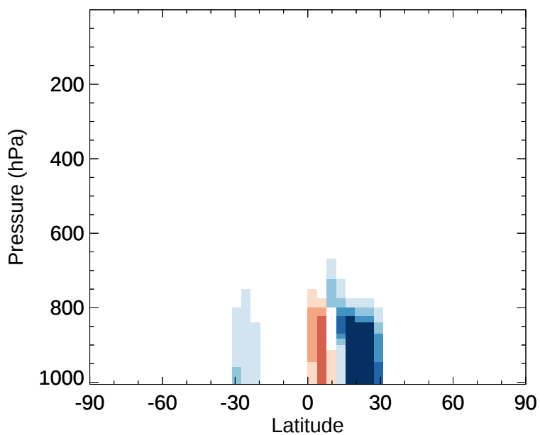
v11-02e-Run1 - v11-02e-Run0 DST3 - Zonal mean abs diff for Jan
