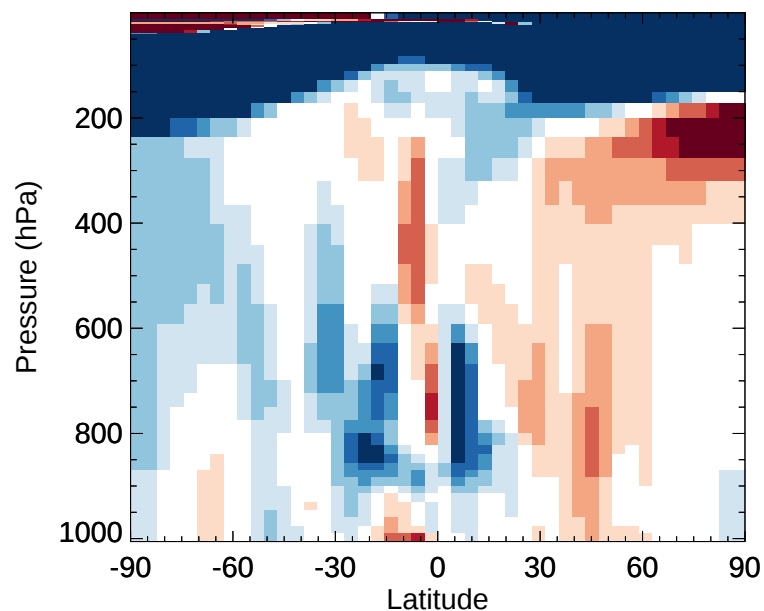
v11-02e-Run1 / v11-02d-Run1 PAN - Zonal mean % diff for Jan
