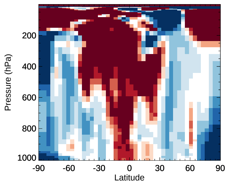
v11-02e-Run1 / v11-02d-Run1 HAC - Zonal mean % diff for Jan
