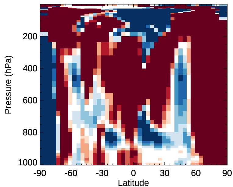
v11-02e-Run1 / v11-02e-Run0 BCPO - Zonal mean % diff for Jan
