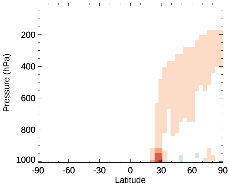
v11-02e-Run1 - v11-02d-Run1 C3H8 - Zonal mean abs diff for Jan
