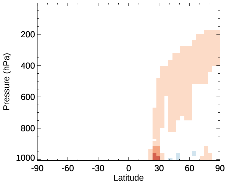
v11-02e-Run1 - v11-02e-Run0 C3H8 - Zonal mean abs diff for Jan
