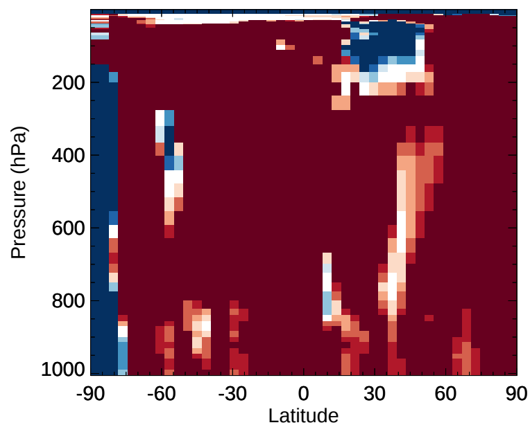
v11-02e-Run1 / v11-02e-Run0 IPMN - Zonal mean % diff for Jan
