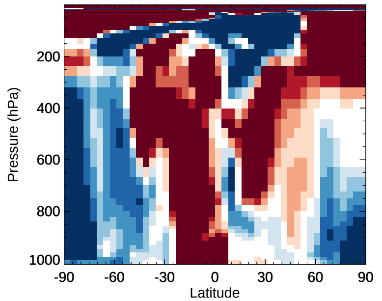
v11-02e-Run1 / v11-02d-Run1 GLYX - Zonal mean % diff for Jan
