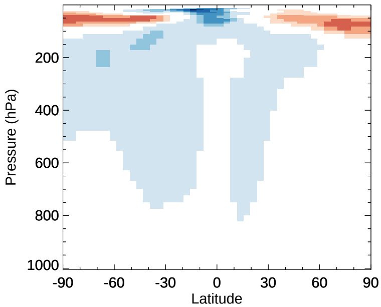
v11-02e-Run1 - v11-02d-Run1 CH3Cl - Zonal mean abs diff for Jan
