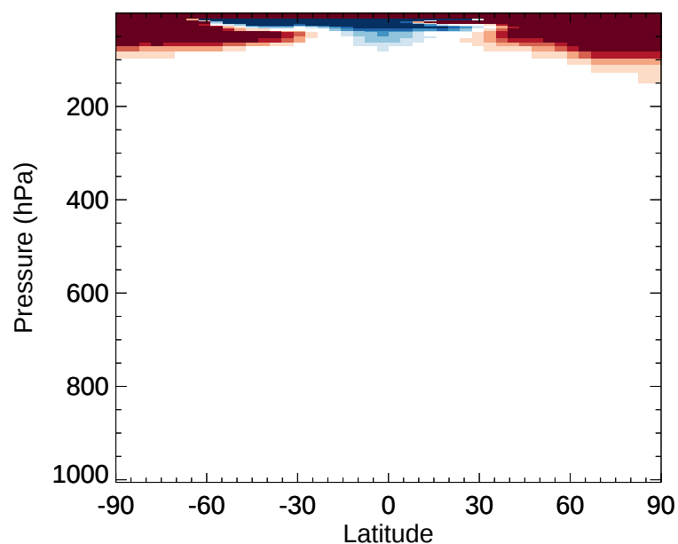
v11-02e-Run1 / v11-02d-Run1 OCS - Zonal mean % diff for Jan
