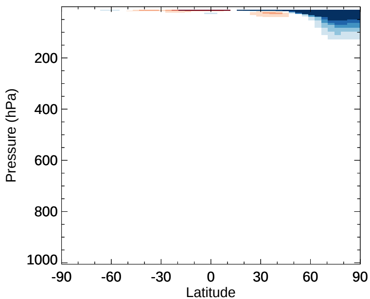
v11-02e-Run1 - v11-02e-Run0 NO 3 - Zonal mean abs diff for Jan
