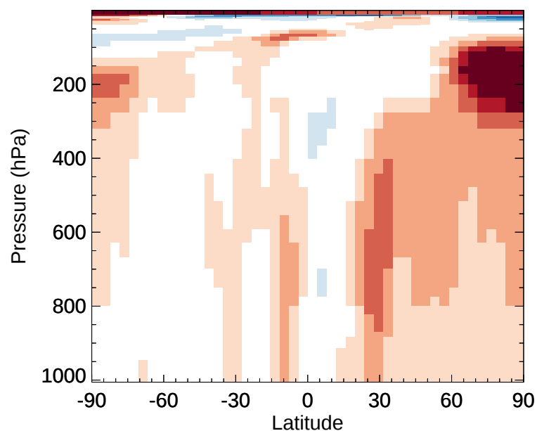
v11-02e-Run1 / v11-02d-Run1 CO - Zonal mean % diff for Jan
