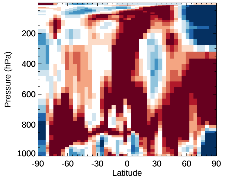
v11-02e-Run1 / v11-02e-Run0 N2O5 - Zonal mean % diff for Jan
