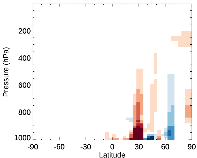
v11-02e-Run1 - v11-02d-Run1 TOLU - Zonal mean abs diff for Jan
