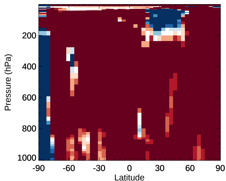
v11-02e-Run1 / v11-02d-Run1 IPMN - Zonal mean % diff for Jan
