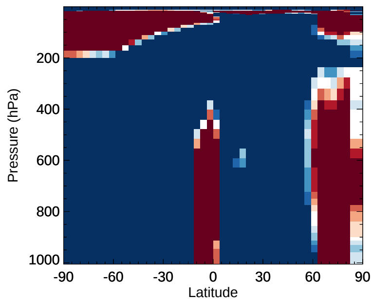
v11-02e-Run1 / v11-02e-Run0 DST2 - Zonal mean % diff for Jan
