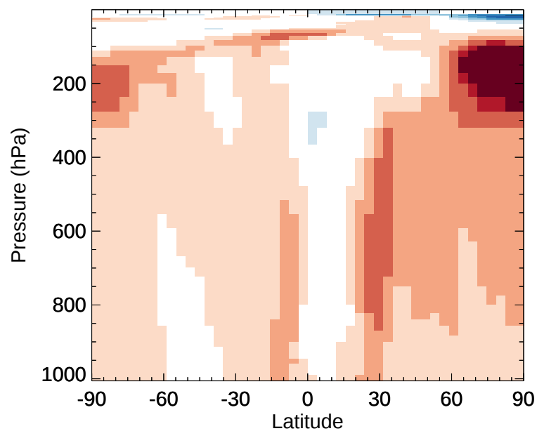
v11-02e-Run1 / v11-02e-Run0 CO - Zonal mean % diff for Jan
