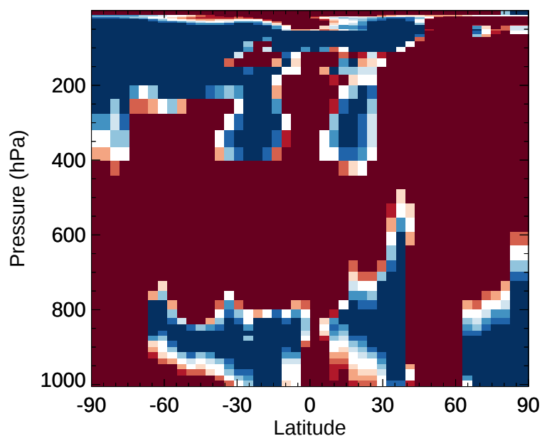
v11-02e-Run1 / v11-02d-Run1 Cl2 - Zonal mean % diff for Jan
