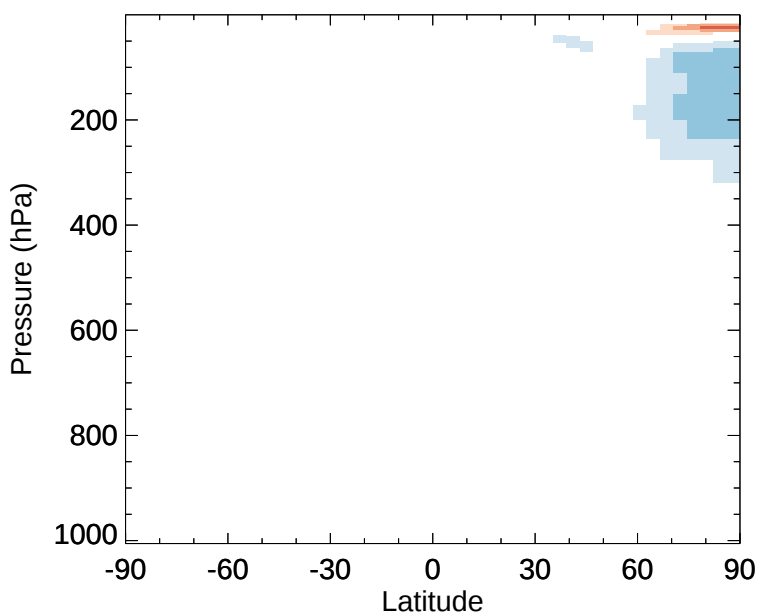
v11-02e-Run1 - v11-02d-Run1 HOBr - Zonal mean abs diff for Jan
