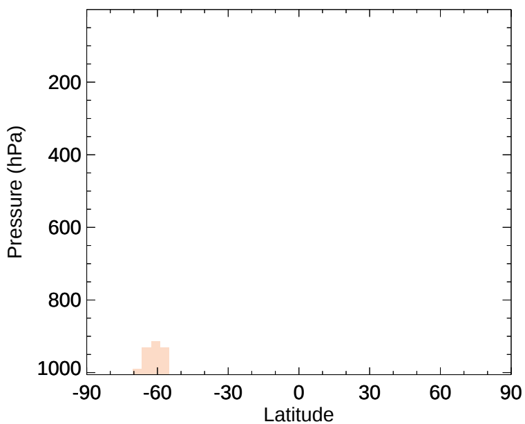
v11-02e-Run1 - v11-02e-Run0 SALA - Zonal mean abs diff for Jan
