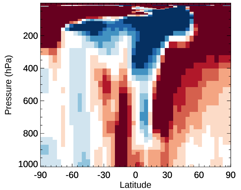
v11-02e-Run1 / v11-02d-Run1 C3H8 - Zonal mean % diff for Jan
