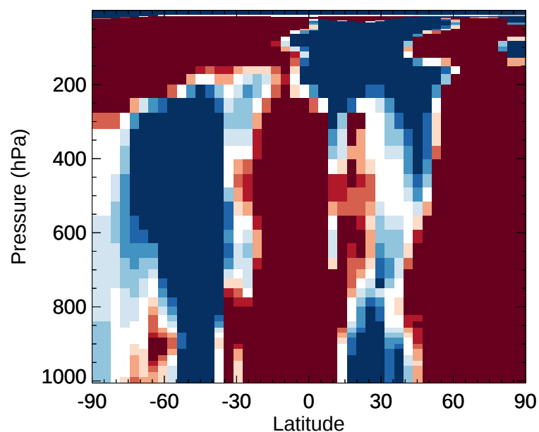
v11-02e-Run1 / v11-02d-Run1 DST3 - Zonal mean % diff for Jan
