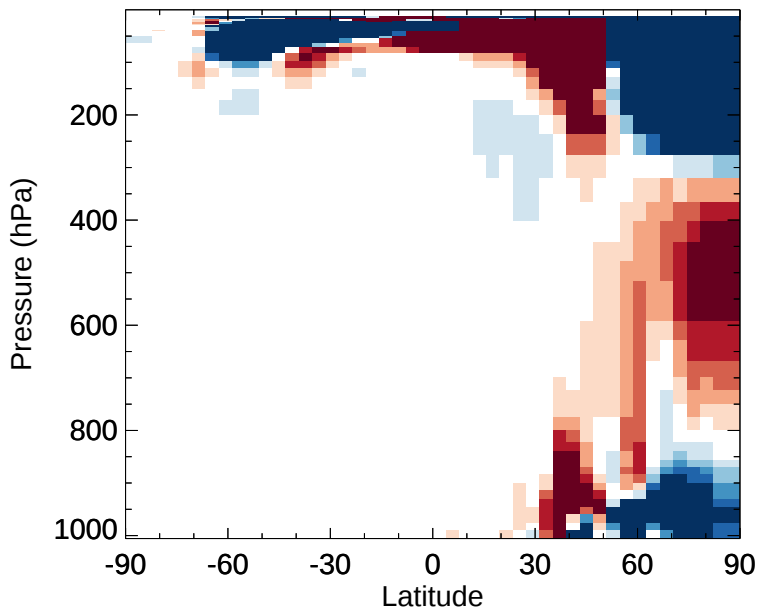
v11-02e-Run1 - v11-02e-Run0 N2O5 - Zonal mean abs diff for Jan
