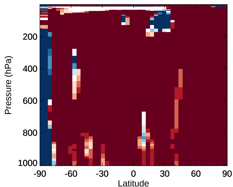
v11-02e-Run1 / v11-02d-Run1 MVK - Zonal mean % diff for Jan
