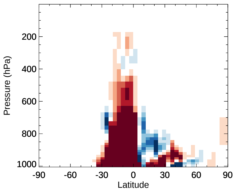
v11-02e-Run1 - v11-02e-Run0 PRPE - Zonal mean abs diff for Jan
