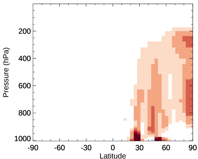
v11-02e-Run1 - v11-02d-Run1 ALK4 - Zonal mean abs diff for Jan
