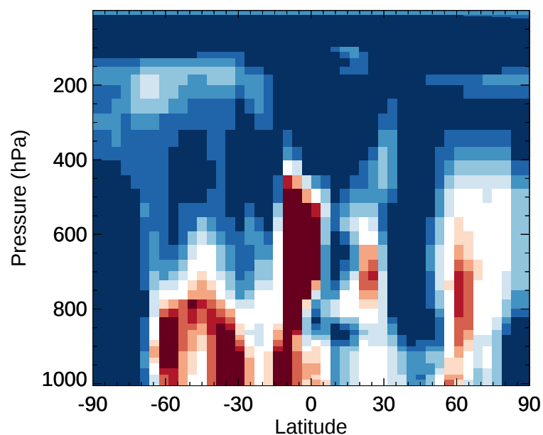
v11-02e-Run1 / v11-02d-Run1 OCPI - Zonal mean % diff for Jan
