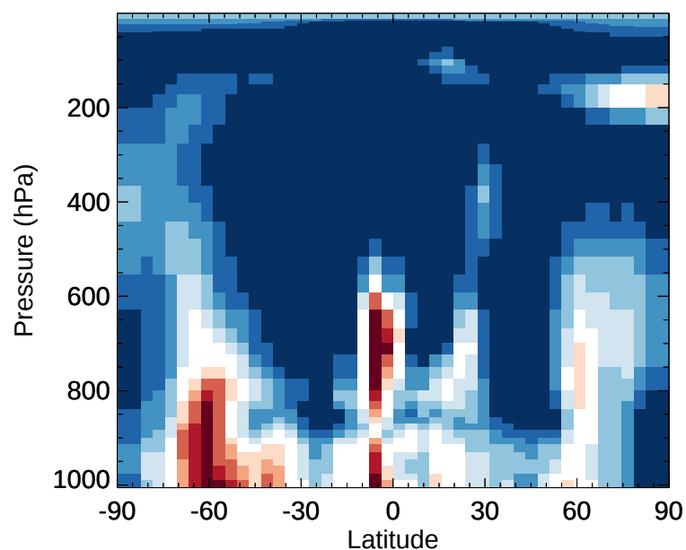
v11-02e-Run1 / v11-02d-Run1 NH4 - Zonal mean % diff for Jan
