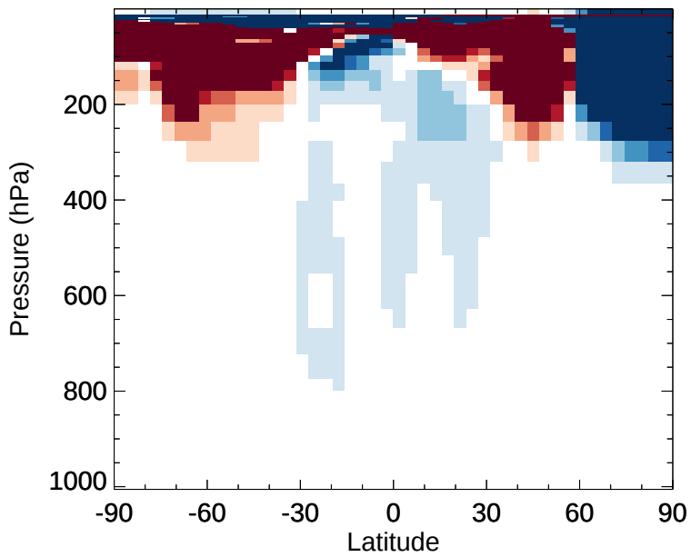
v11-02e-Run1 - v11-02d-Run1 O3 - Zonal mean abs diff for Jan
