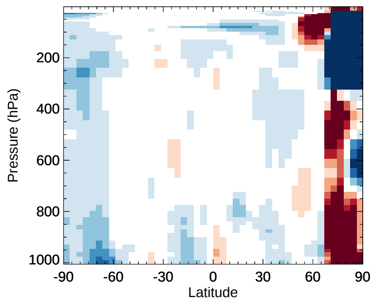
v11-02e-Run1 / v11-02e-Run0 OH - Zonal mean % diff for Jan
