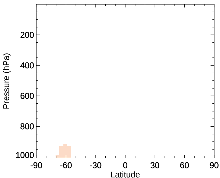
v11-02e-Run1 - v11-02d-Run1 SALA - Zonal mean abs diff for Jan
