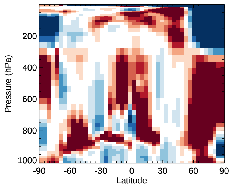
v11-02e-Run1 / v11-02d-Run1 NO 3 - Zonal mean % diff for Jan
