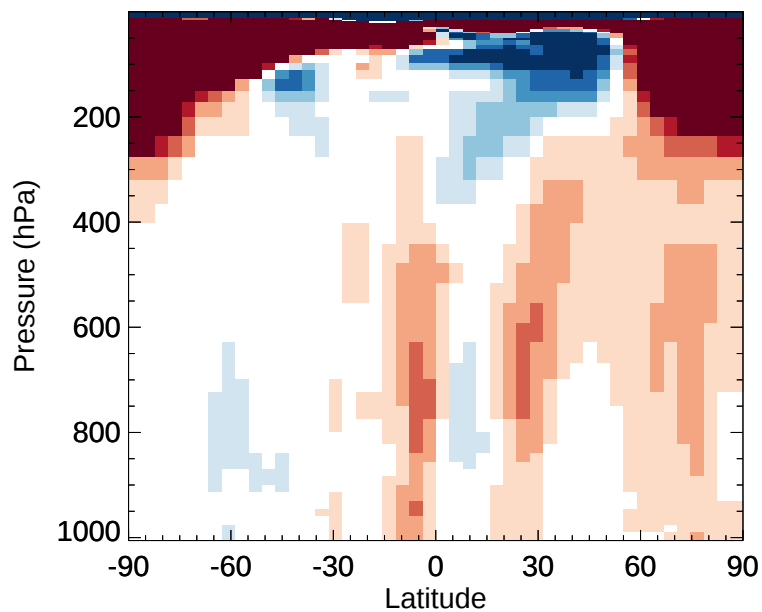
v11-02e-Run1 / v11-02e-Run0 ACET - Zonal mean % diff for Jan
