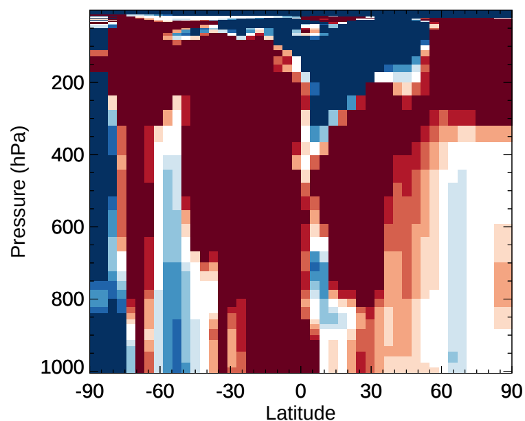
v11-02e-Run1 / v11-02d-Run1 TOLU - Zonal mean % diff for Jan
