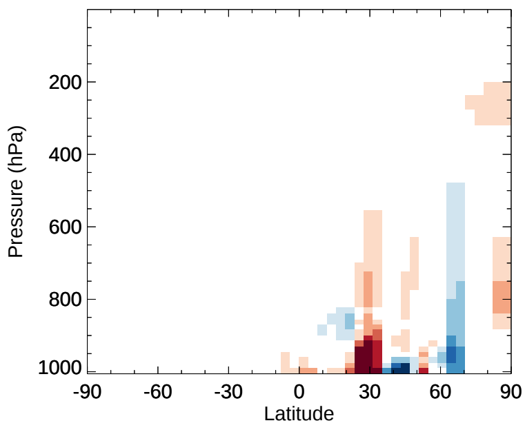
v11-02e-Run1 - v11-02e-Run0 TOLU - Zonal mean abs diff for Jan
