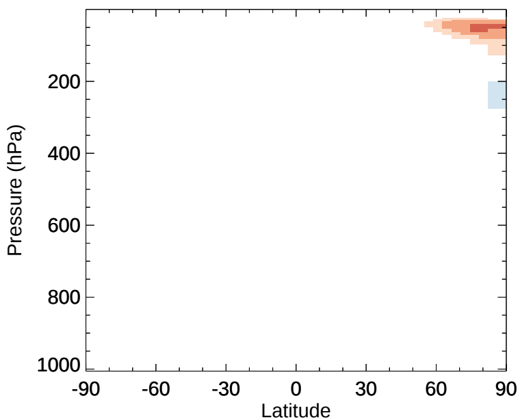
v11-02e-Run1 - v11-02e-Run0 MPN - Zonal mean abs diff for Jan
