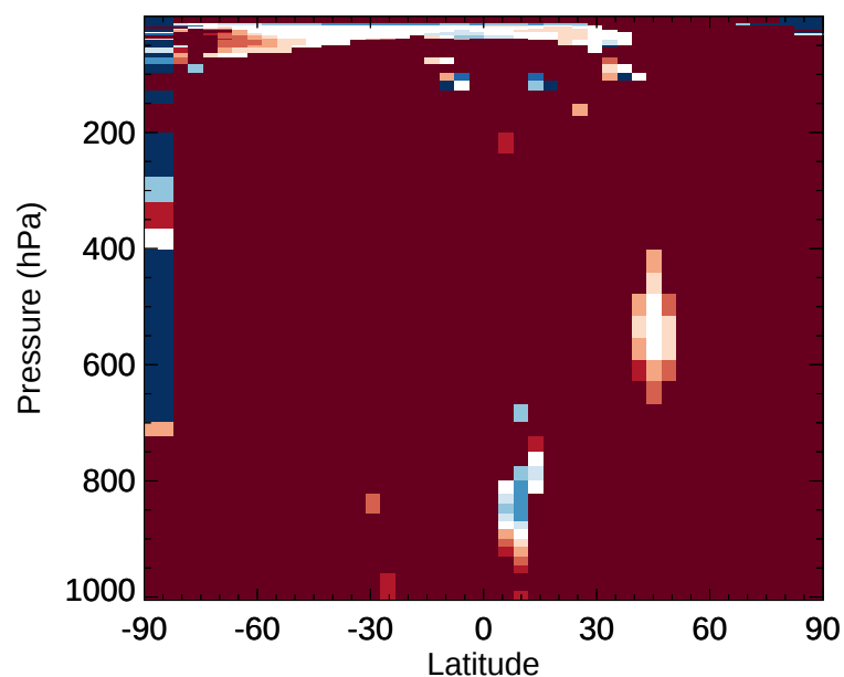
v11-02e-Run1 / v11-02d-Run1 ISOP - Zonal mean % diff for Jan
