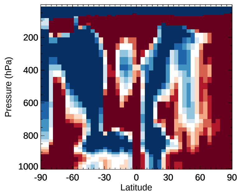
v11-02e-Run1 / v11-02d-Run1 SO4s - Zonal mean % diff for Jan
