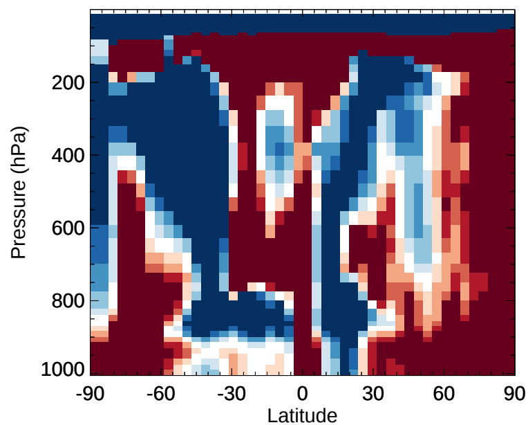
v11-02e-Run1 / v11-02e-Run0 SO4s - Zonal mean % diff for Jan
