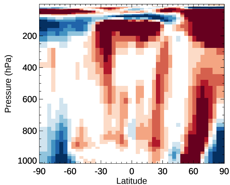
v11-02e-Run1 / v11-02e-Run0 H2O2 - Zonal mean % diff for Jan
