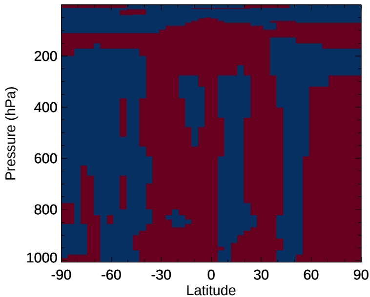
v11-02e-Run1 - v11-02d-Run1 H 2 O - Zonal mean abs diff for Jan
