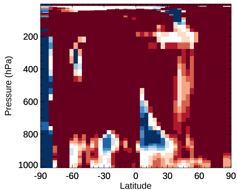
v11-02e-Run1 / v11-02d-Run1 PRPE - Zonal mean % diff for Jan
