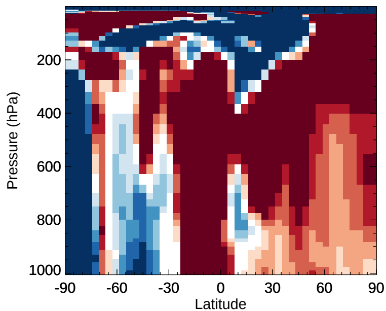
v11-02e-Run1 / v11-02d-Run1 MEK - Zonal mean % diff for Jan
