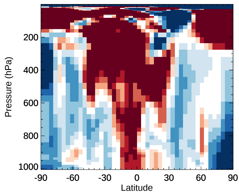
v11-02e-Run1 / v11-02e-Run0 HAC - Zonal mean % diff for Jan
