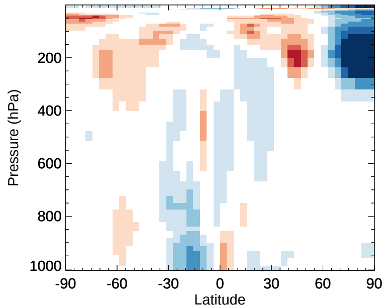
v11-02e-Run1 / v11-02d-Run1 O3 - Zonal mean % diff for Jan
