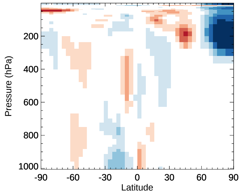
v11-02e-Run1 / v11-02e-Run0 O3 - Zonal mean % diff for Jan
