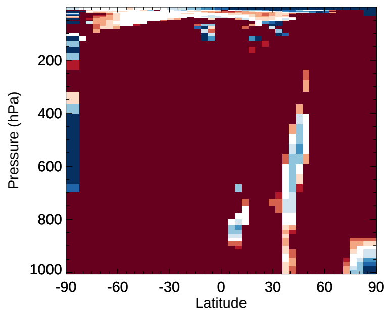
v11-02e-Run1 / v11-02e-Run0 RIPD - Zonal mean % diff for Jan
