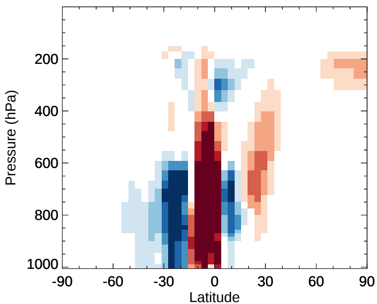
v11-02e-Run1 - v11-02e-Run0 MAP - Zonal mean abs diff for Jan
