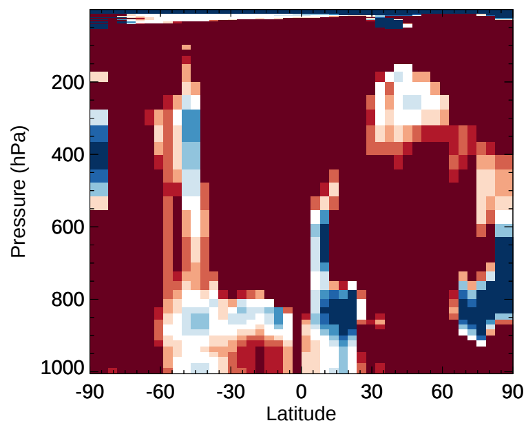
v11-02e-Run1 / v11-02e-Run0 DMS - Zonal mean % diff for Jan
