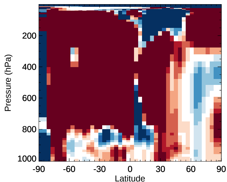
v11-02e-Run1 / v11-02d-Run1 XYLE - Zonal mean % diff for Jan
