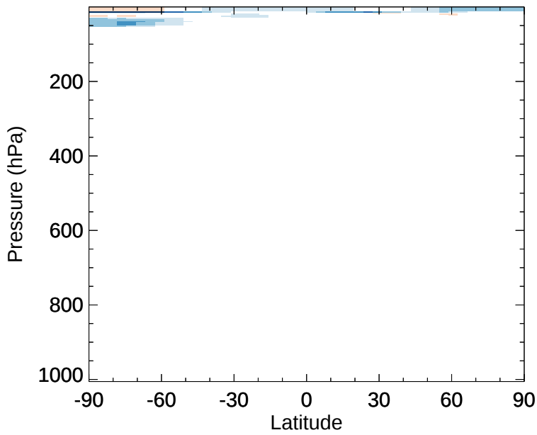
v11-02e-Run1 - v11-02e-Run0 NO - Zonal mean abs diff for Jan
