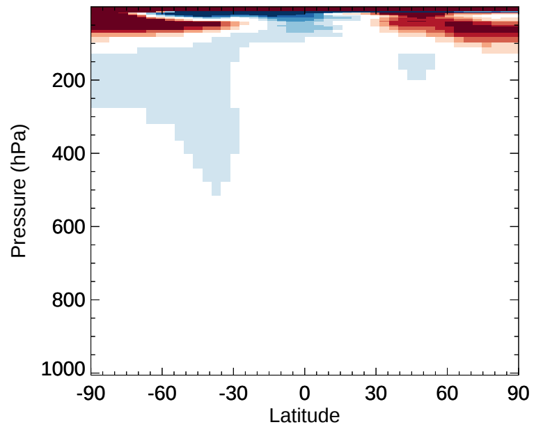
v11-02e-Run1 / v11-02d-Run1 CH3Cl - Zonal mean % diff for Jan
