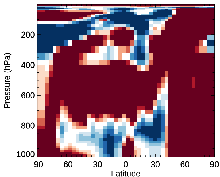
v11-02e-Run1 / v11-02d-Run1 HOCl - Zonal mean % diff for Jan
