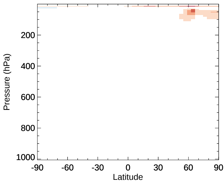
v11-02e-Run1 - v11-02e-Run0 C1O - Zonal mean abs diff for Jan
