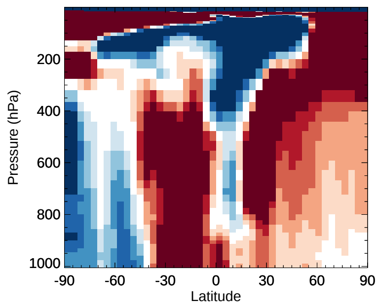
v11-02e-Run1 / v11-02d-Run1 BENZ - Zonal mean % diff for Jan
