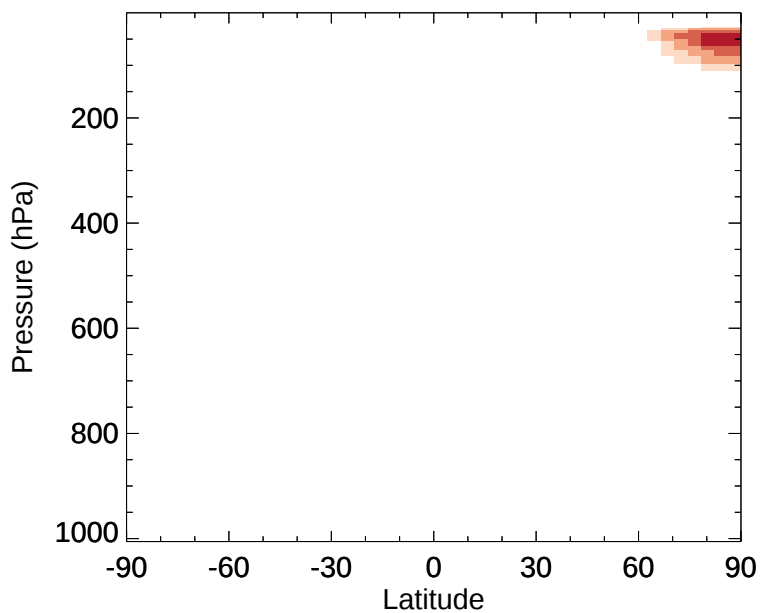
v11-02e-Run1 - v11-02d-Run1 OCIO - Zonal mean abs diff for Jan
