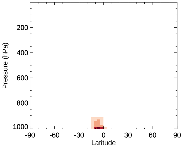
v11-02e-Run1 - v11-02e-Run0 MTPA - Zonal mean abs diff for Jan
