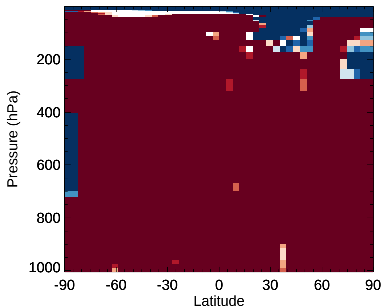
v11-02e-Run1 / v11-02d-Run1 LVOC - Zonal mean % diff for Jan
