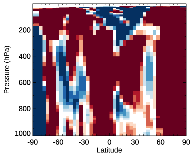
v11-02e-Run1 / v11-02d-Run1 SOAP - Zonal mean % diff for Jan
