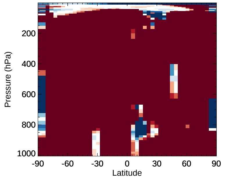
v11-02e-Run1 / v11-02e-Run0 MTPA - Zonal mean % diff for Jan
