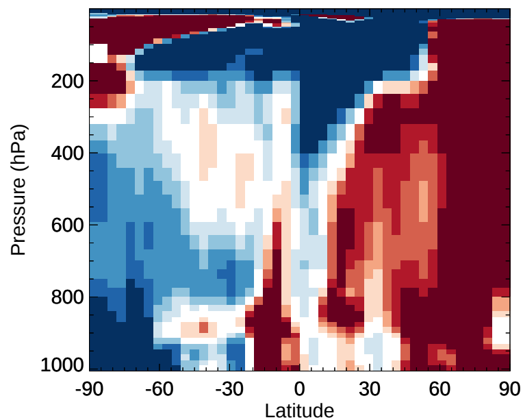
v11-02e-Run1 / v11-02d-Run1 R4N2 - Zonal mean % diff for Jan
