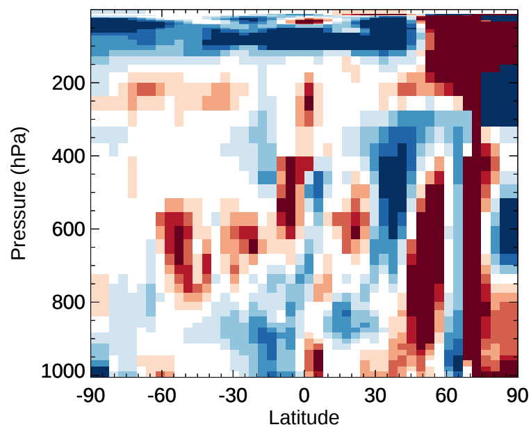
v11-02e-Run1 / v11-02e-Run0 C100 - Zonal mean % diff for Jan
