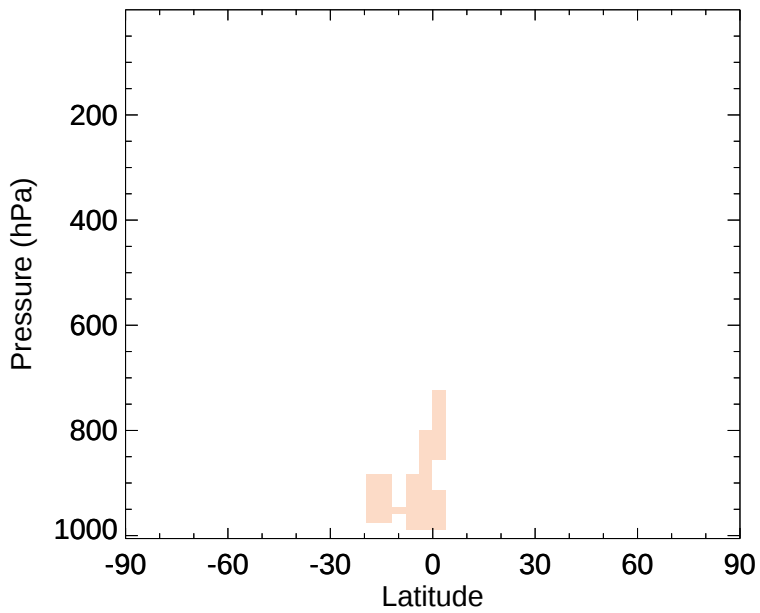
v11-02e-Run1 - v11-02d-Run1 RIPA - Zonal mean abs diff for Jan
