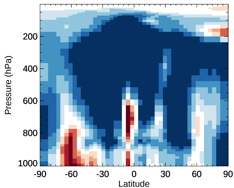
v11-02e-Run1 / v11-02e-Run0 NH4 - Zonal mean % diff for Jan
