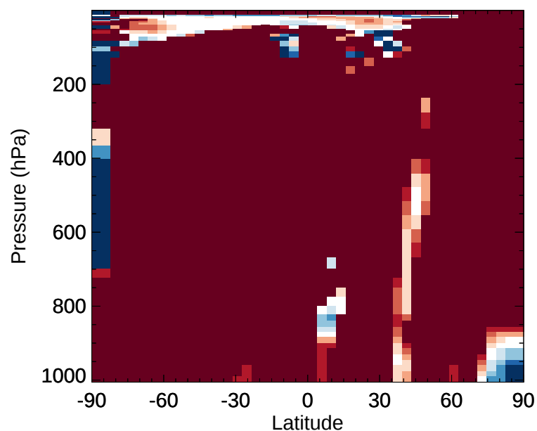
v11-02e-Run1 / v11-02d-Run1 RIPD - Zonal mean % diff for Jan
