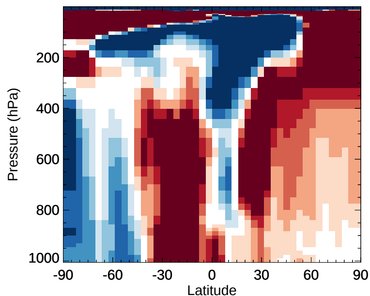
v11-02e-Run1 / v11-02e-Run0 BENZ - Zonal mean % diff for Jan
