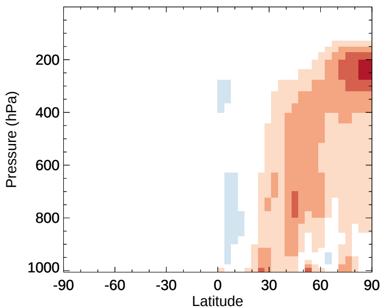
v11-02e-Run1 - v11-02e-Run0 C2H6 - Zonal mean abs diff for Jan
