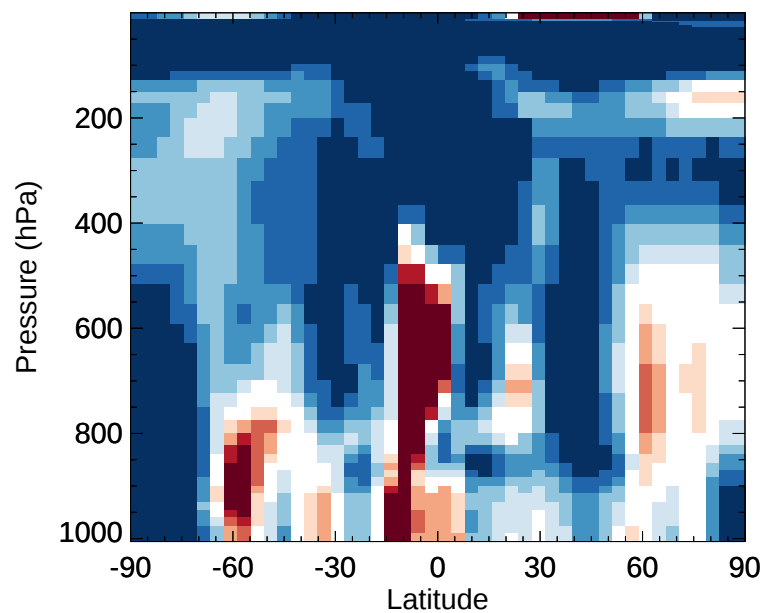
v11-02e-Run1 / v11-02d-Run1 BCPI - Zonal mean % diff for Jan
