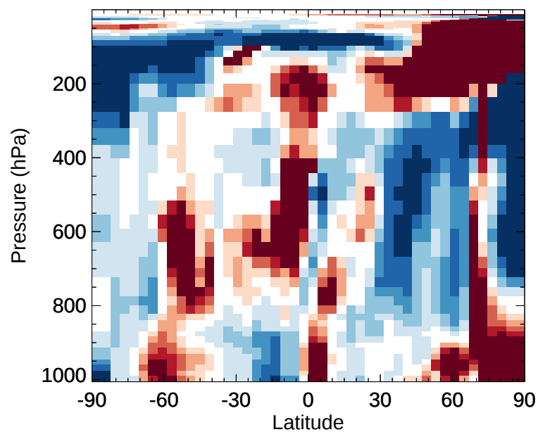
v11-02e-Run1 / v11-02e-Run0 C1O - Zonal mean % diff for Jan
