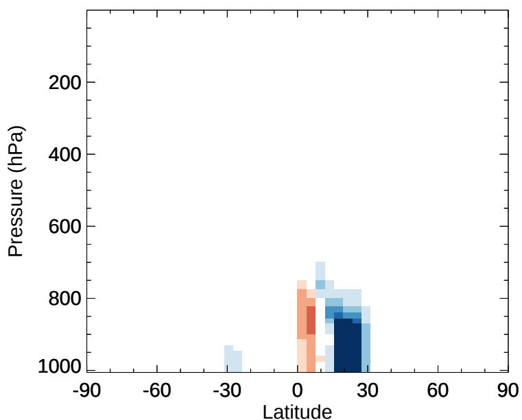
v11-02e-Run1 - v11-02d-Run1 DST2 - Zonal mean abs diff for Jan
