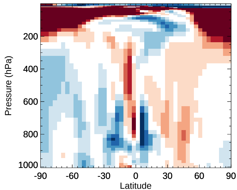
v11-02e-Run1 / v11-02e-Run0 PAN - Zonal mean % diff for Jan
