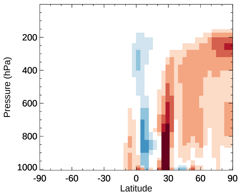
v11-02e-Run1 - v11-02e-Run0 BENZ - Zonal mean abs diff for Jan
