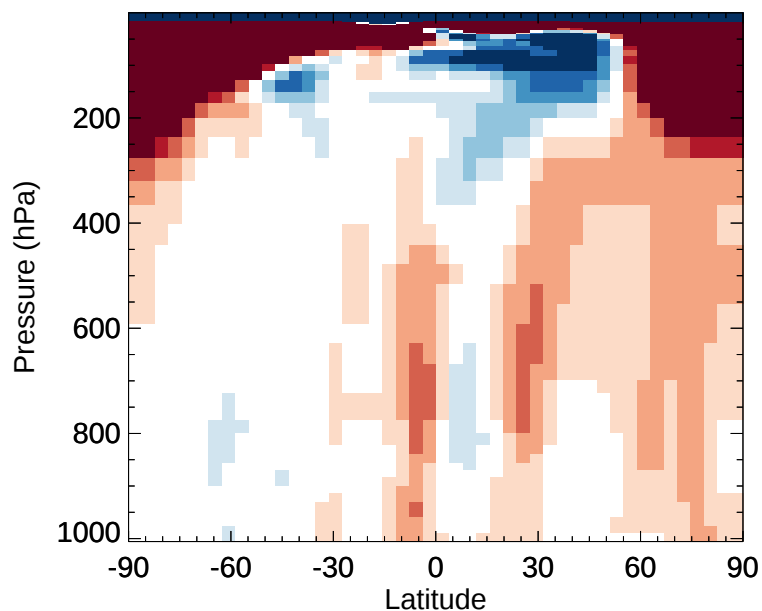
v11-02e-Run1 / v11-02d-Run1 ACET - Zonal mean % diff for Jan
