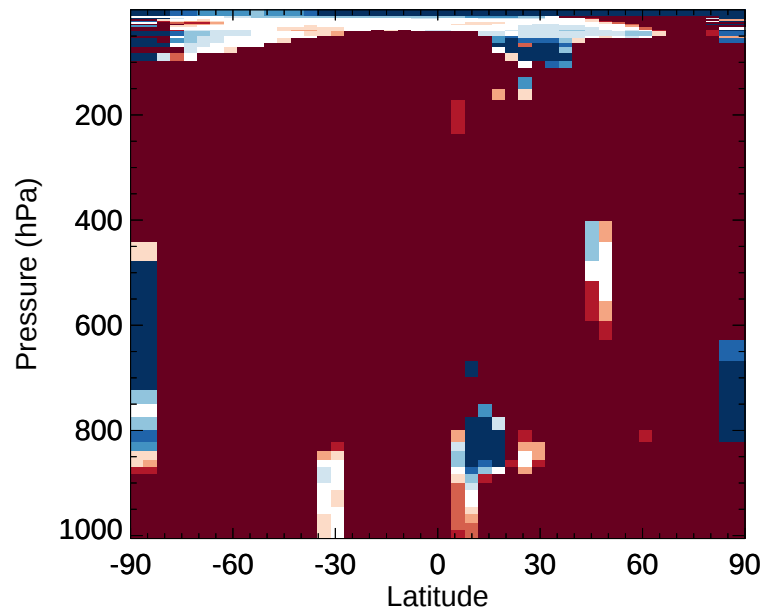
v11-02e-Run1 / v11-02d-Run1 MTPA - Zonal mean % diff for Jan
