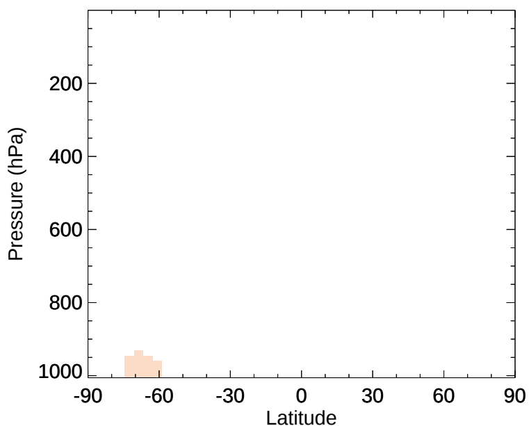
v11-02e-Run1 - v11-02d-Run1 DMS - Zonal mean abs diff for Jan
