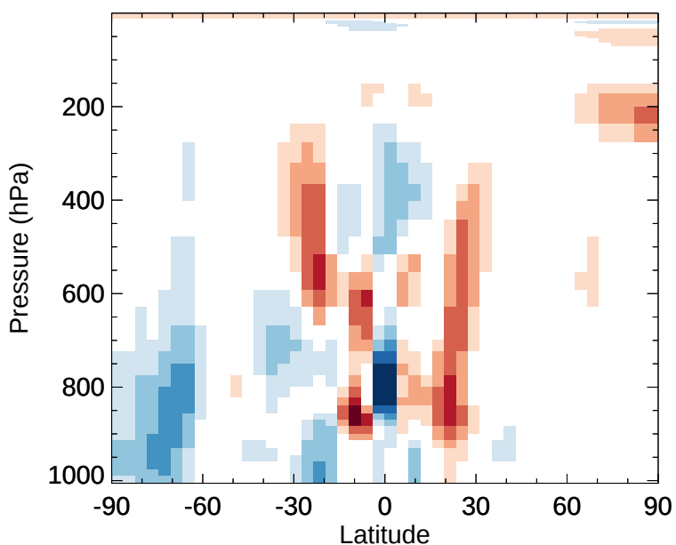
v11-02e-Run1 - v11-02d-Run1 H2O2 - Zonal mean abs diff for Jan
