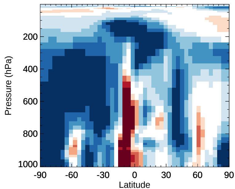
v11-02e-Run1 / v11-02e-Run0 SOAS - Zonal mean % diff for Jan
