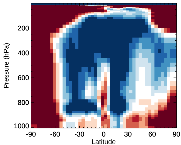
v11-02e-Run1 / v11-02e-Run0 SALA - Zonal mean % diff for Jan
