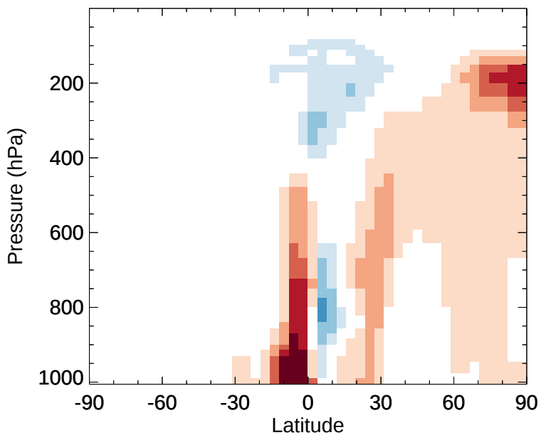
v11-02e-Run1 - v11-02e-Run0 ACET - Zonal mean abs diff for Jan
