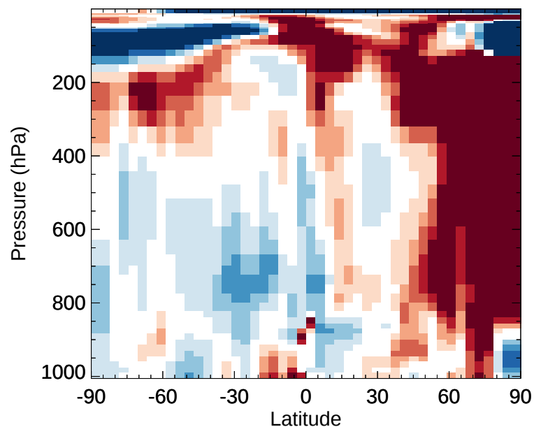
v11-02e-Run1 / v11-02d-Run1 NO2 - Zonal mean % diff for Jan
