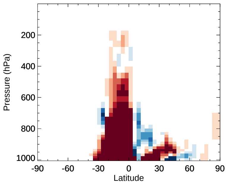
v11-02e-Run1 - v11-02d-Run1 PRPE - Zonal mean abs diff for Jan
