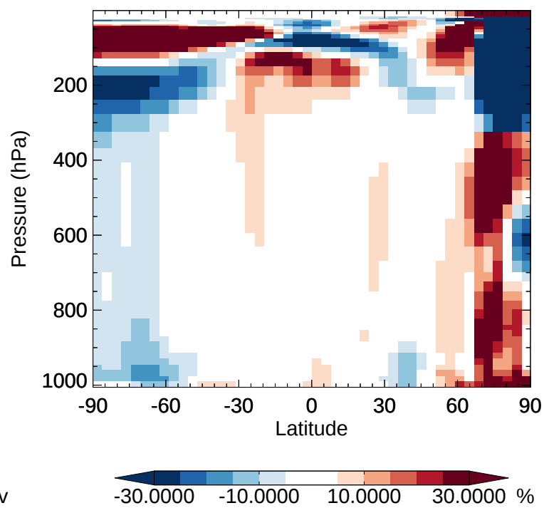
v11-02e-Run1 / v11-02d-Run1 HO2 - Zonal mean % diff for Jan
