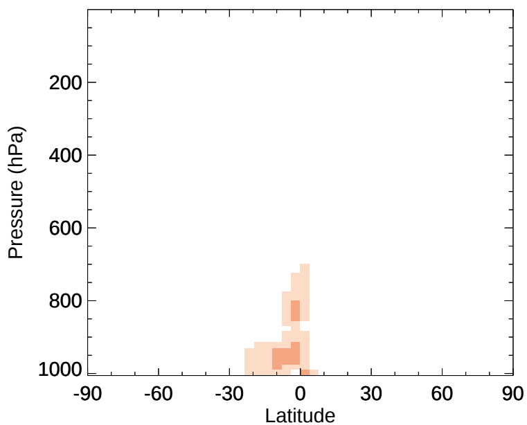
v11-02e-Run1 - v11-02e-Run0 ALD2 - Zonal mean abs diff for Jan
