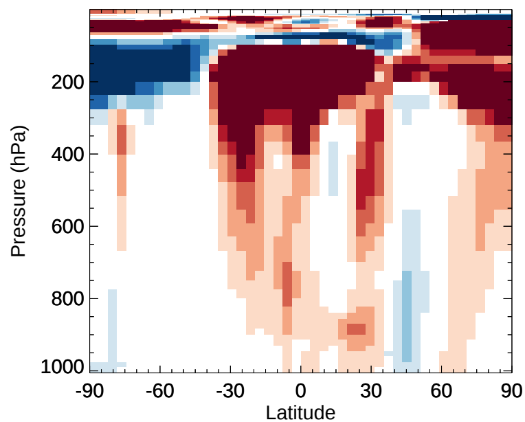
v11-02e-Run1 / v11-02e-Run0 MP - Zonal mean % diff for Jan
