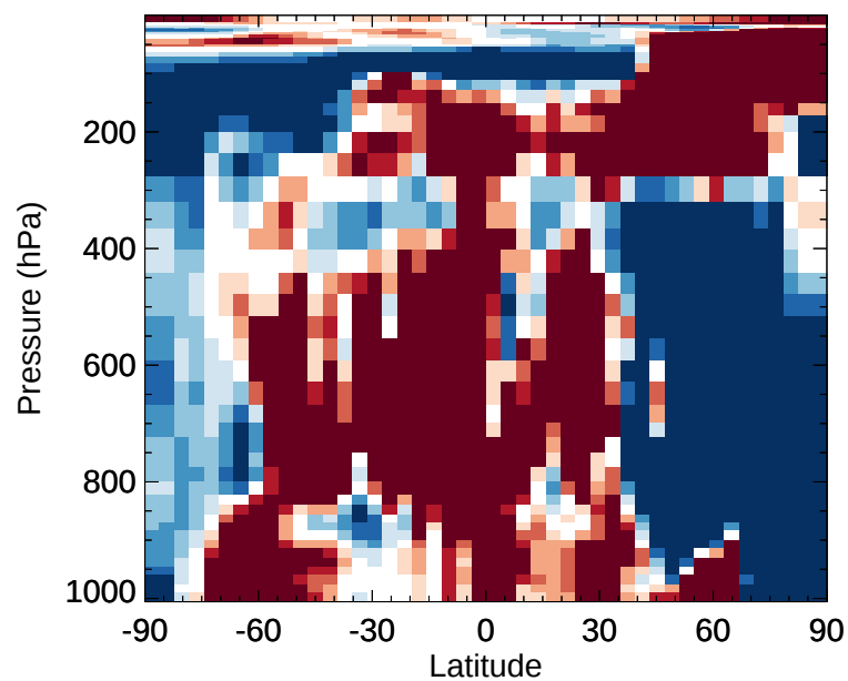
v11-02e-Run1 / v11-02e-Run0 OCIO - Zonal mean % diff for Jan
