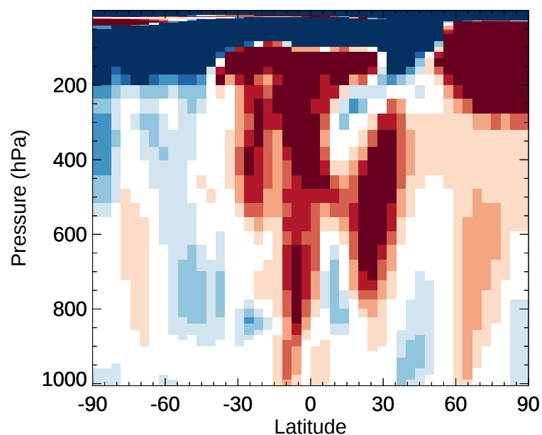
v11-02e-Run1 / v11-02d-Run1 MAP - Zonal mean % diff for Jan
