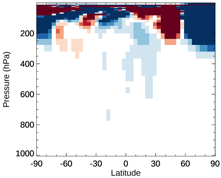
v11-02e-Run1 - v11-02e-Run0 O3 - Zonal mean abs diff for Jan
