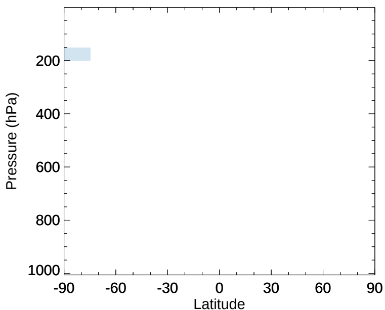
v11-02e-Run1 - v11-02d-Run1 BrO - Zonal mean abs diff for Jan
