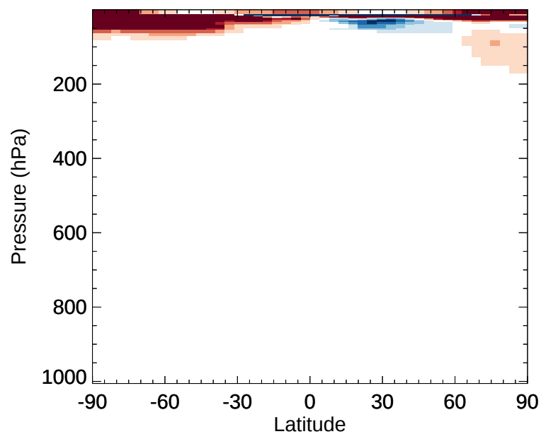
v11-02e-Run1 / v11-02e-Run0 OCS - Zonal mean % diff for Jan
