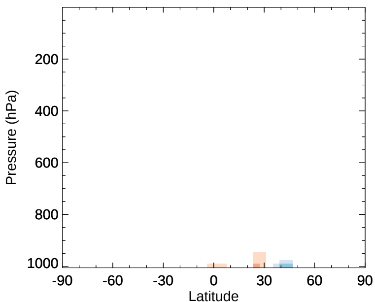
v11-02e-Run1 - v11-02d-Run1 SOAP - Zonal mean abs diff for Jan
