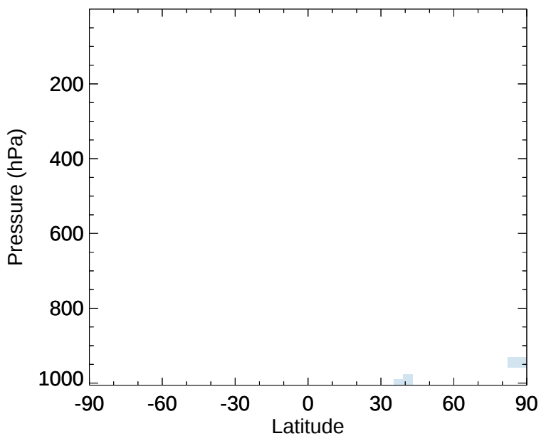
v11-02e-Run1 - v11-02d-Run1 SO 2 - Zonal mean abs diff for Jan
