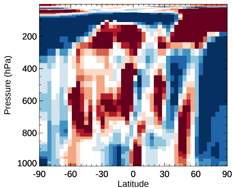
v11-02e-Run1 / v11-02e-Run0 HOCl - Zonal mean % diff for Jan
