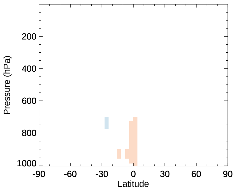
v11-02e-Run1 - v11-02e-Run0 GLYC - Zonal mean abs diff for Jan
