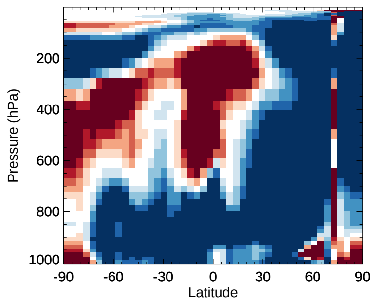
v11-02e-Run1 / v11-02d-Run1 BrO - Zonal mean % diff for Jan
