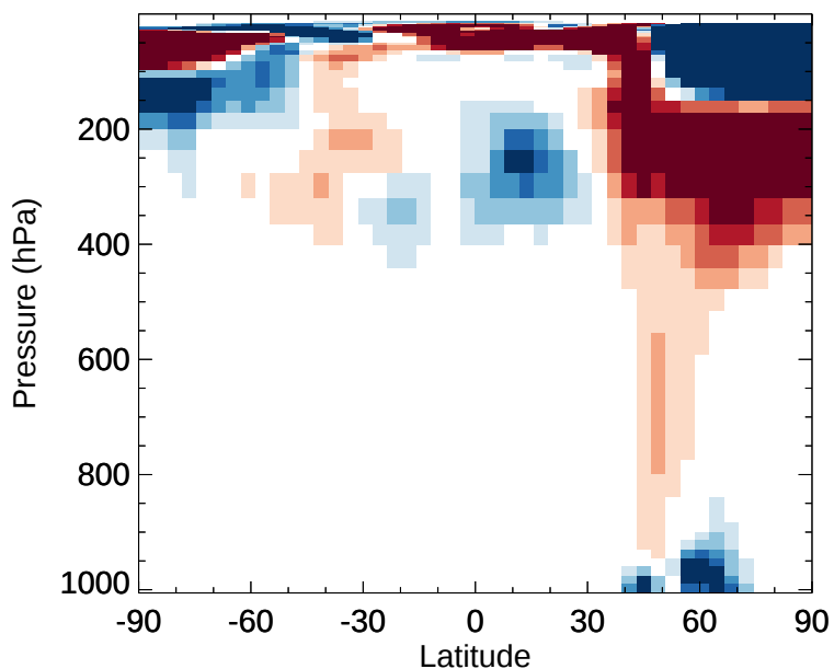
v11-02e-Run1 - v11-02d-Run1 HNO 4 - Zonal mean abs diff for Jan
