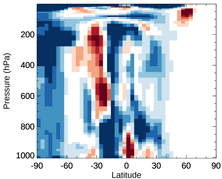
v11-02e-Run1 - v11-02e-Run0 OH - Zonal mean abs diff for Jan
