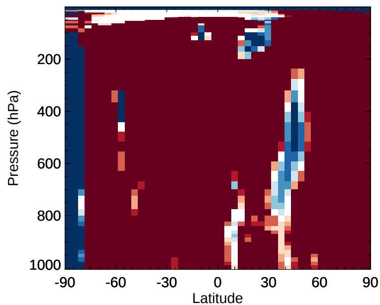
v11-02e-Run1 / v11-02e-Run0 ISN1 - Zonal mean % diff for Jan
