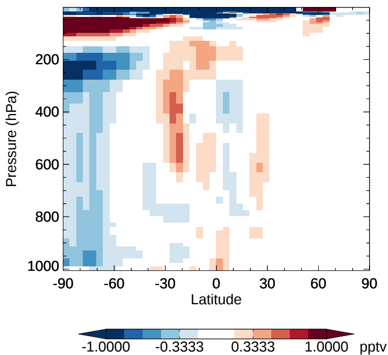
v11-02e-Run1 - v11-02d-Run1 HO2 - Zonal mean abs diff for Jan
