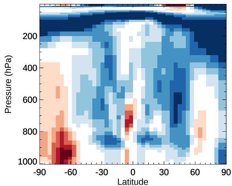
v11-02e-Run1 / v11-02e-Run0 SO4 - Zonal mean % diff for Jan
