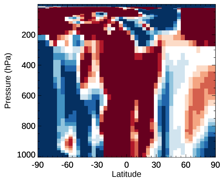
v11-02e-Run1 / v11-02d-Run1 IMAE - Zonal mean % diff for Jan
