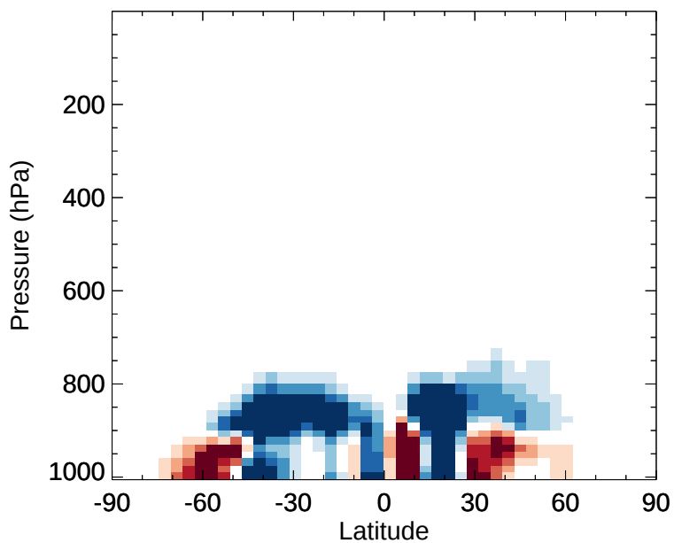
v11-02e-Run1 - v11-02d-Run1 SALC - Zonal mean abs diff for Jan
