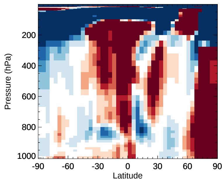
v11-02e-Run1 / v11-02d-Run1 ACTA - Zonal mean % diff for Jan
