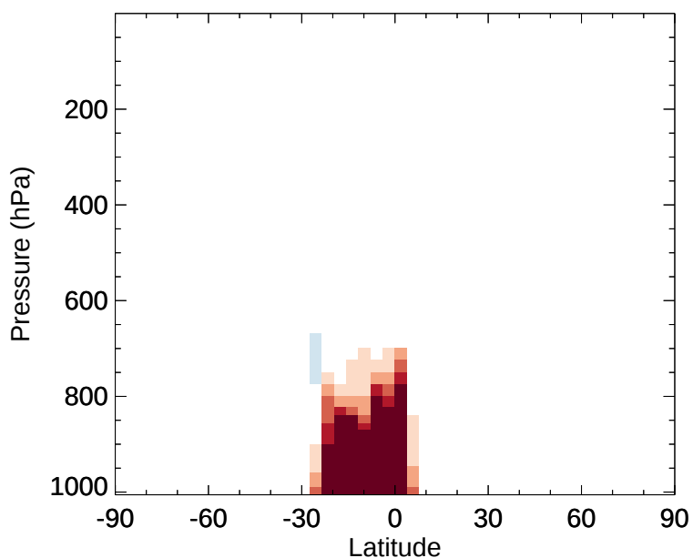
v11-02e-Run1 - v11-02d-Run1 ISOP - Zonal mean abs diff for Jan
