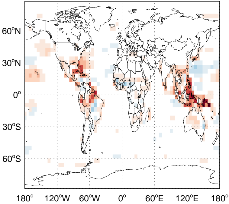
v11-02f-Run1 - v11-02e-Run0 ACET biogenic emissions for Oct
