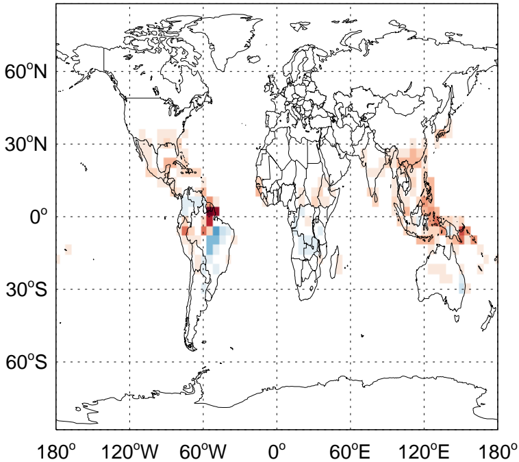
v11-02f-Run1 - v11-02e-Run0 ACET from MONOT emissions for Oct
