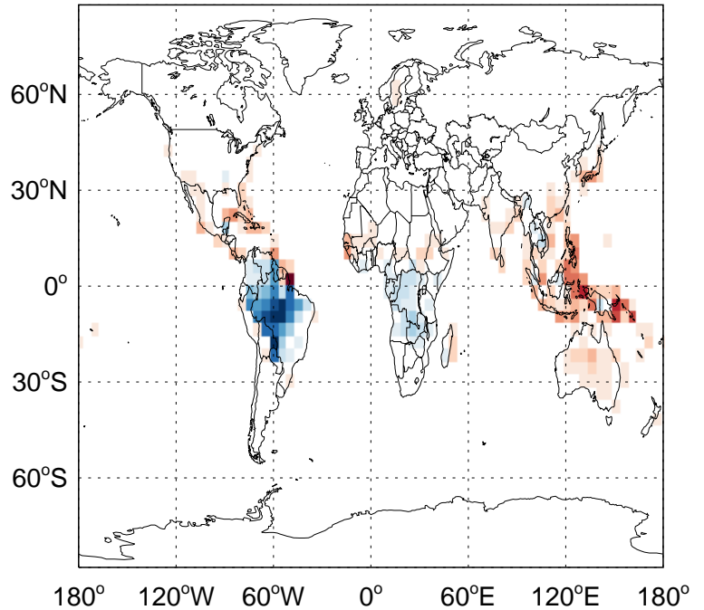
v11-02f-Run1 - v11-02e-Run1 ACET from MONOT emissions for Oct
