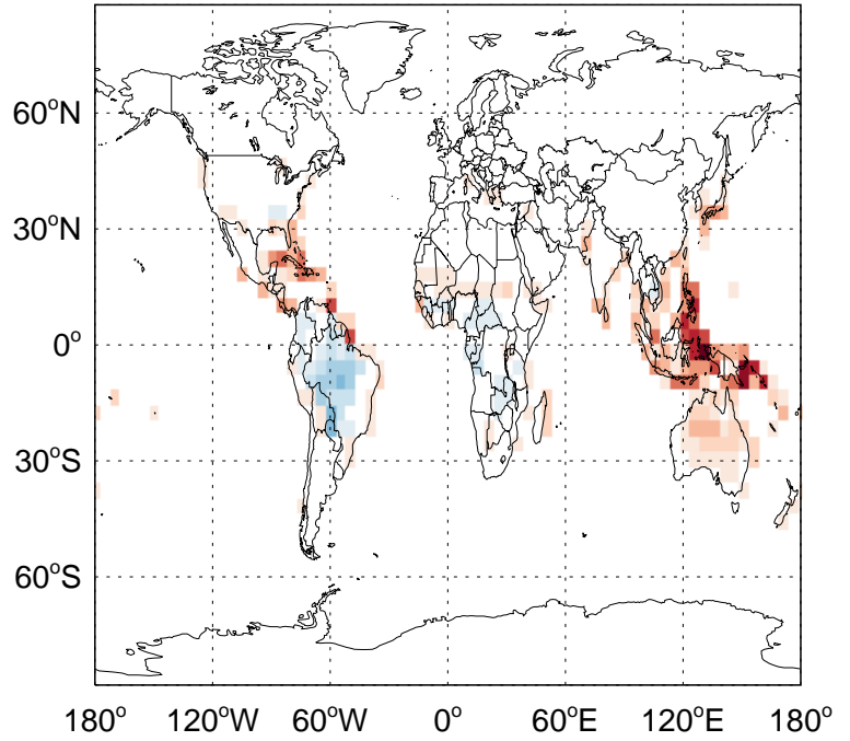
v11-02f-Run1 - v11-02e-Run1 ACET biogenic emissions for Oct
