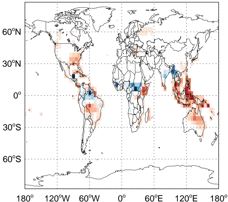
v11-02f-Run1 - v11-02e-Run0 CO from MONOT emissions for Apr
