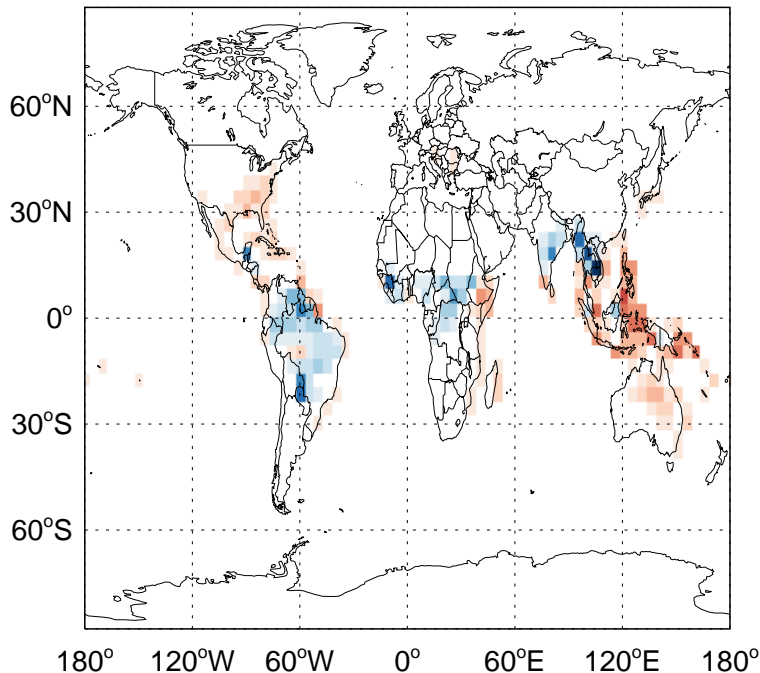
v11-02f-Run1 - v11-02e-Run1 CO from MONOT emissions for Apr
