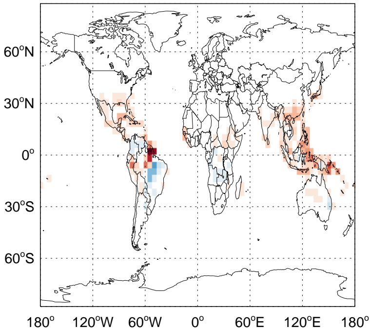
v11-02f-Run1 - v11-02e-Run0 CO from MONOT emissions for Oct
