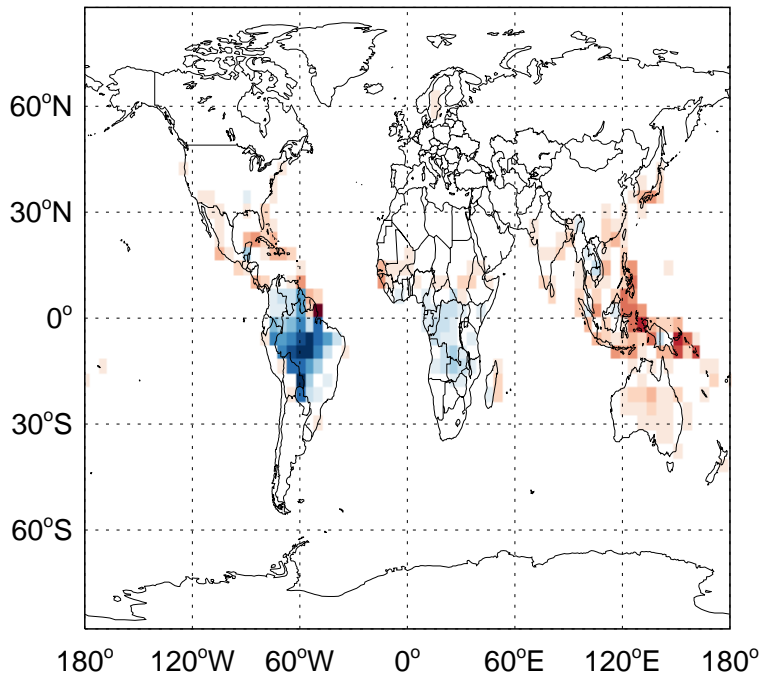
v11-02f-Run1 - v11-02e-Run1 CO from MONOT emissions for Oct
