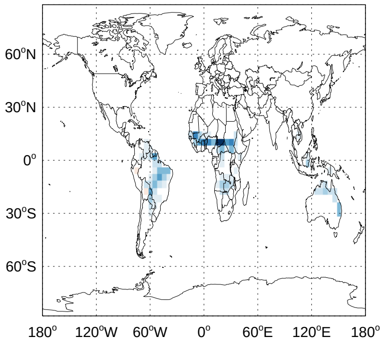
v11-02f-Run1 - v11-02e-Run0 ISOP biogenic emissions for Oct
