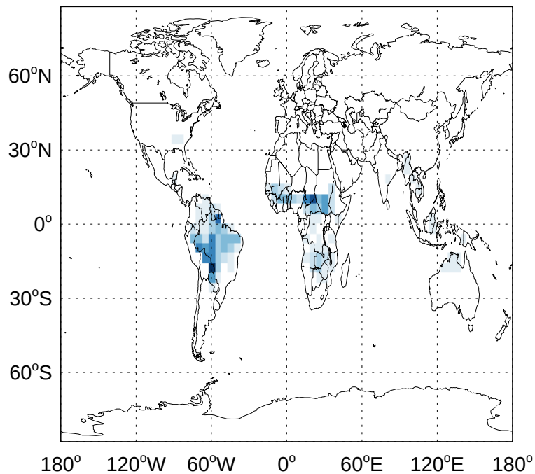
v11-02f-Run1 - v11-02e-Run1 ISOP biogenic emissions for Oct
