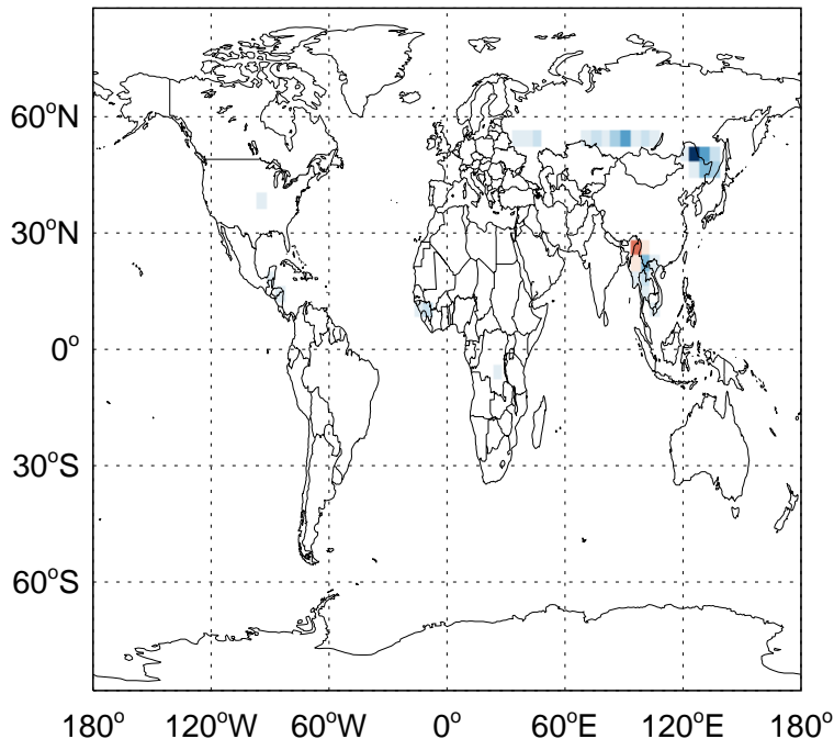
OC biomass emissions for Apr
