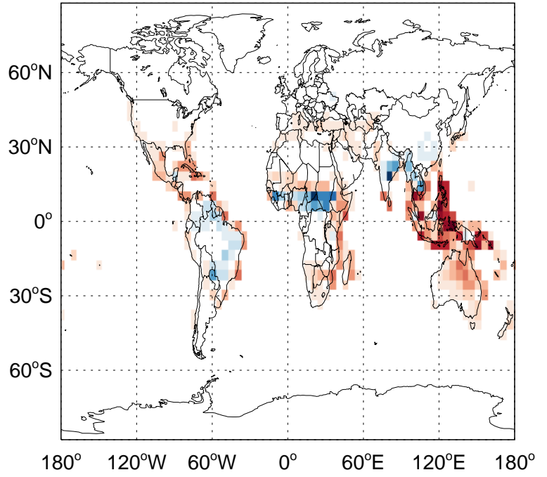
v11-02f-Run1 - v11-02e-Run1 PRPE biogenic emissions for Apr
