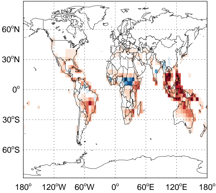
v11-02f-Run1 - v11-02e-Run0 PRPE biogenic emissions for Apr
