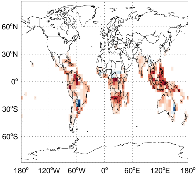
v11-02f-Run1 - v11-02e-Run0 PRPE biogenic emissions for Jan
