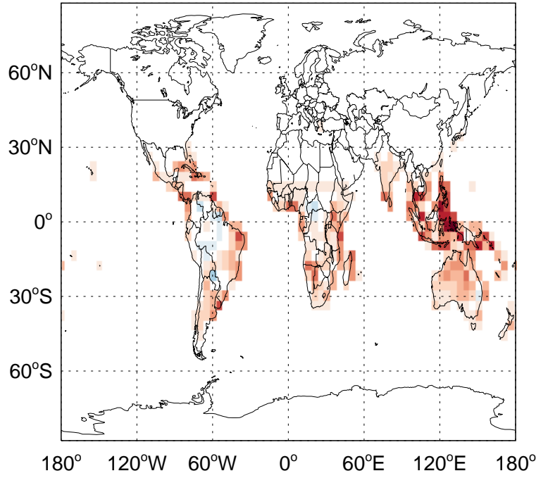
v11-02f-Run1 - v11-02e-Run1 PRPE biogenic emissions for Jan
